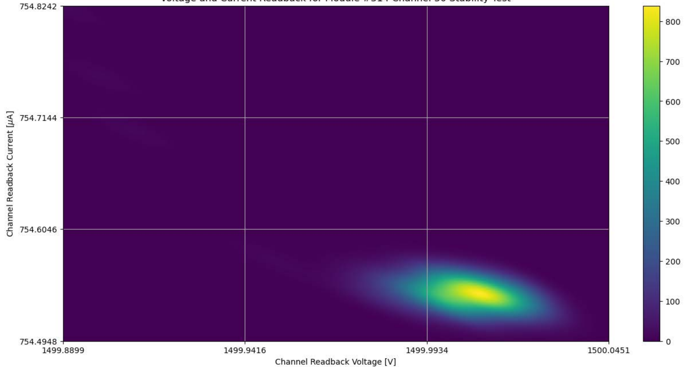
Voltage and Current Readback for Module #314 Channel 30 Stability Test
