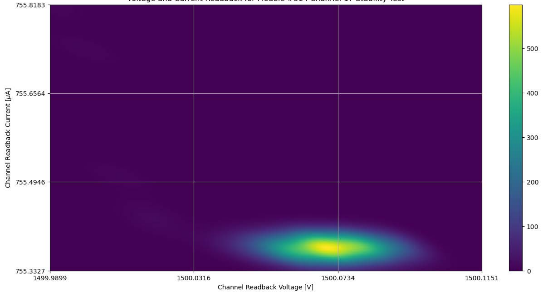
Voltage and Current Readback for Module #314 Channel 17 Stability Test
