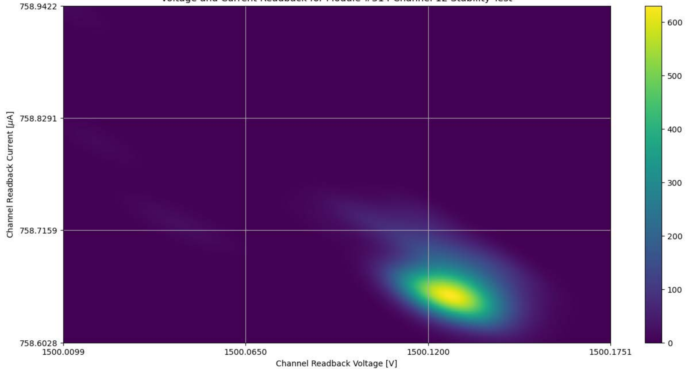
Voltage and Current Readback for Module #314 Channel 12 Stability Test
