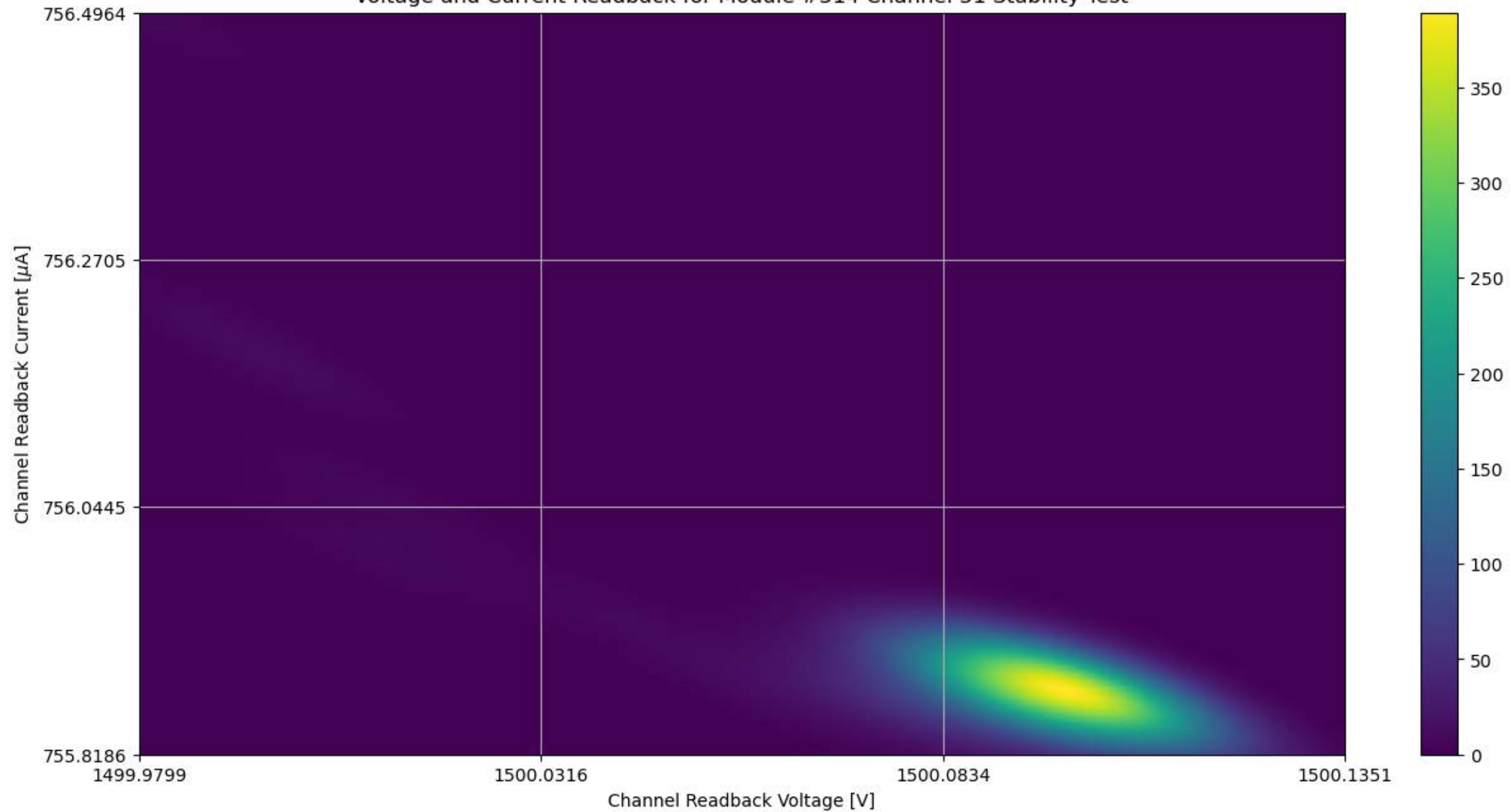
Voltage and Current Readback for Module #314 Channel 31 Stability Test
