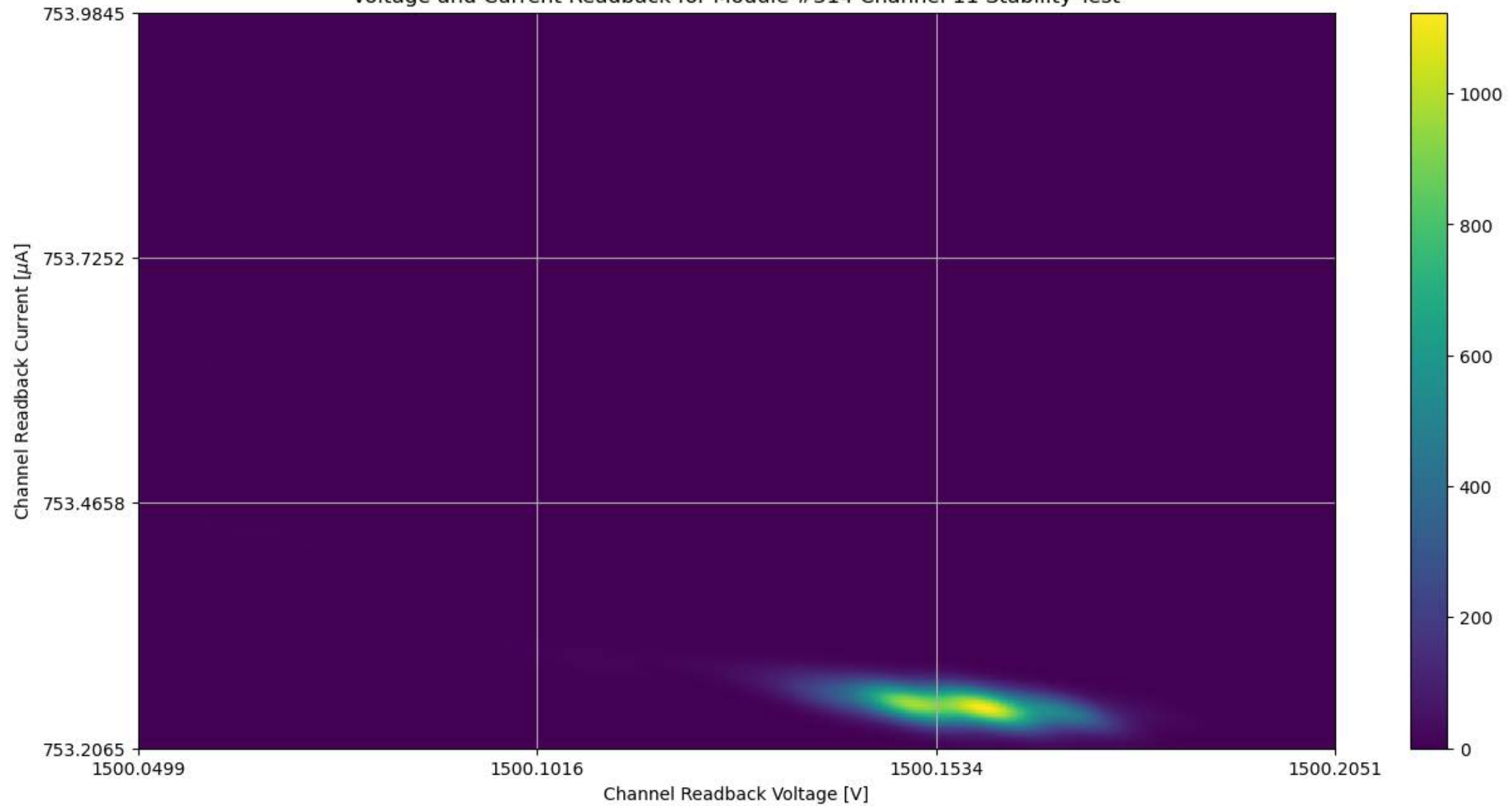
Voltage and Current Readback for Module #314 Channel 11 Stability Test
