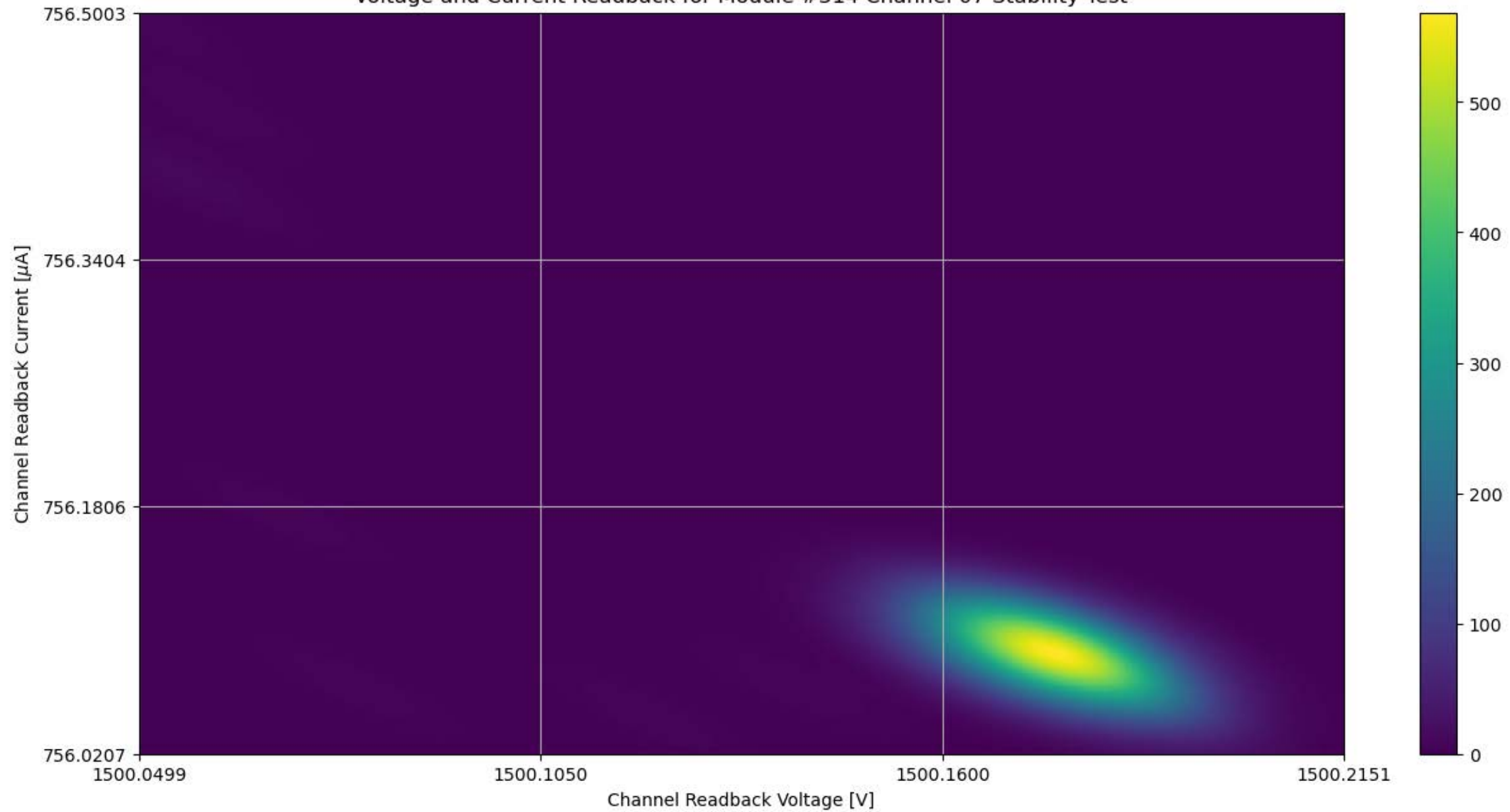
Voltage and Current Readback for Module #314 Channel 07 Stability Test
