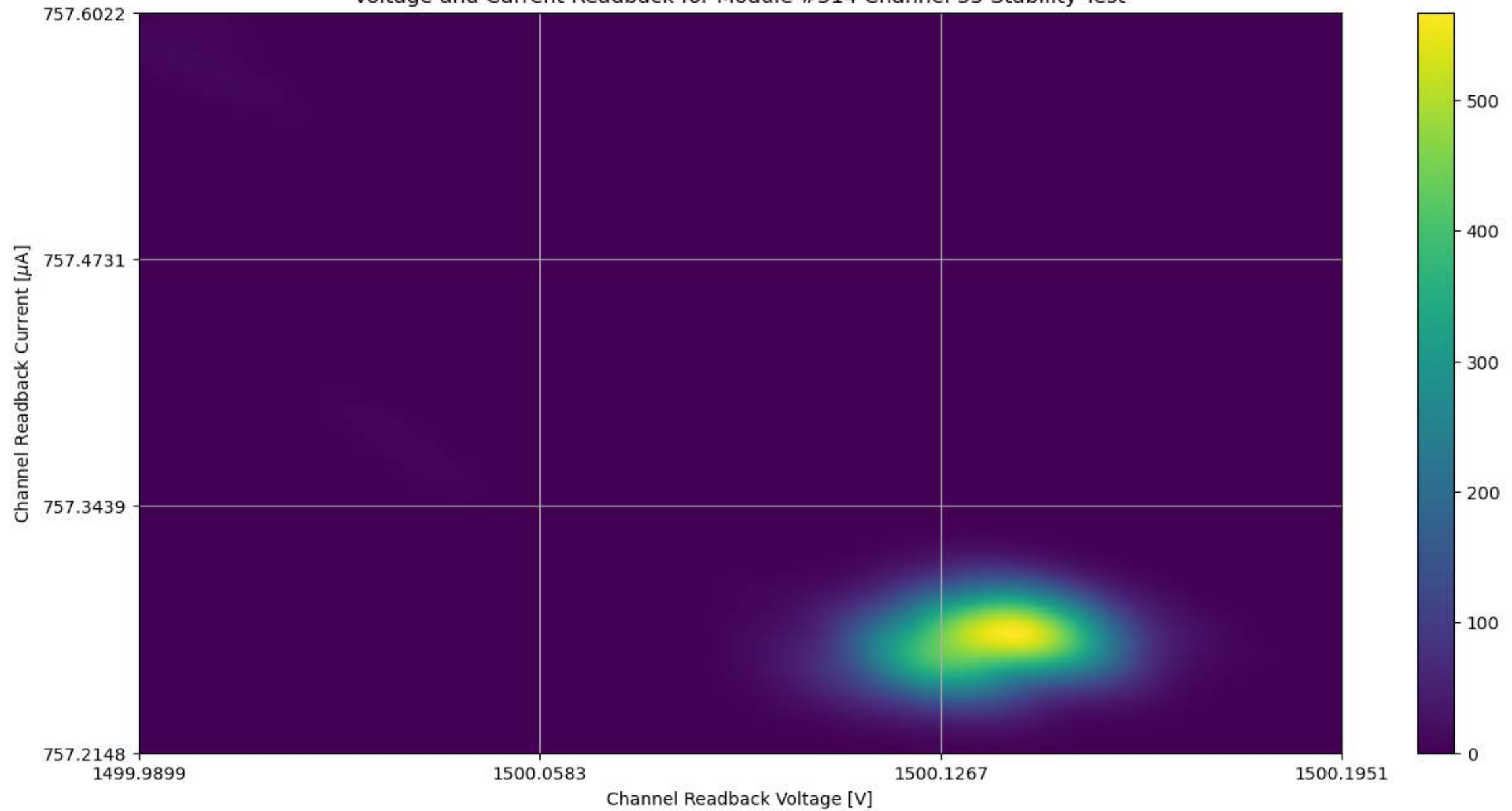
Voltage and Current Readback for Module #314 Channel 35 Stability Test
