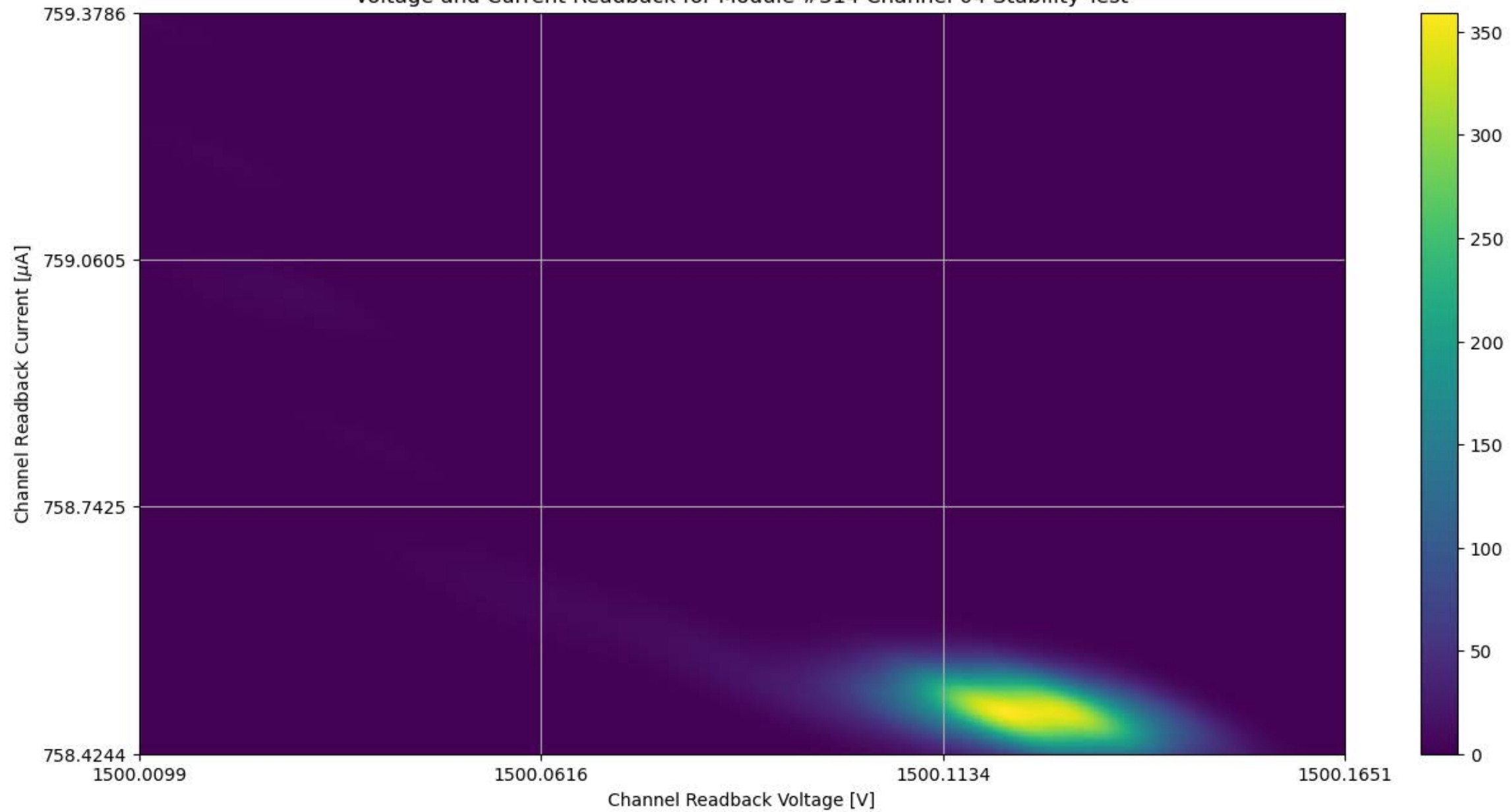
Voltage and Current Readback for Module #314 Channel 04 Stability Test
