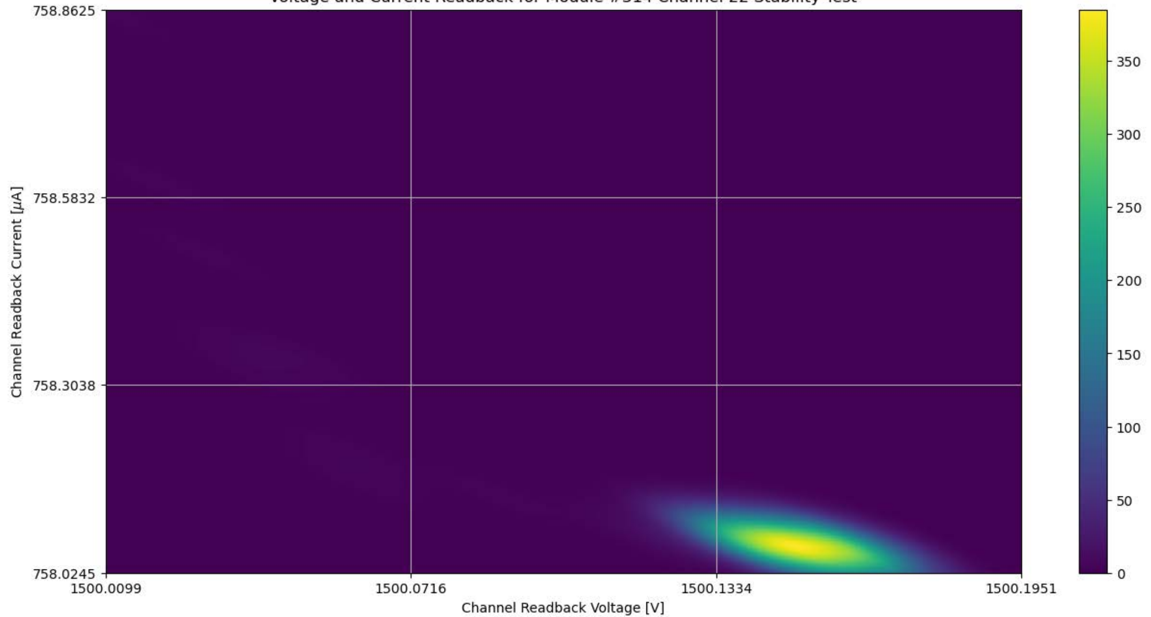
Voltage and Current Readback for Module #314 Channel 22 Stability Test
