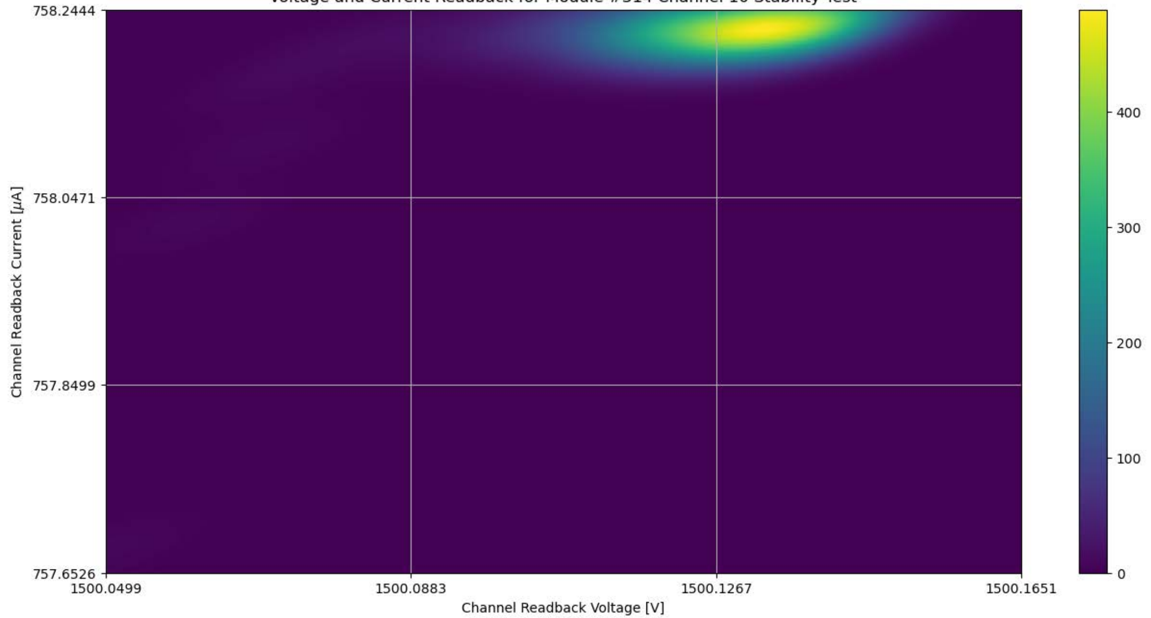
Voltage and Current Readback for Module #314 Channel 10 Stability Test
