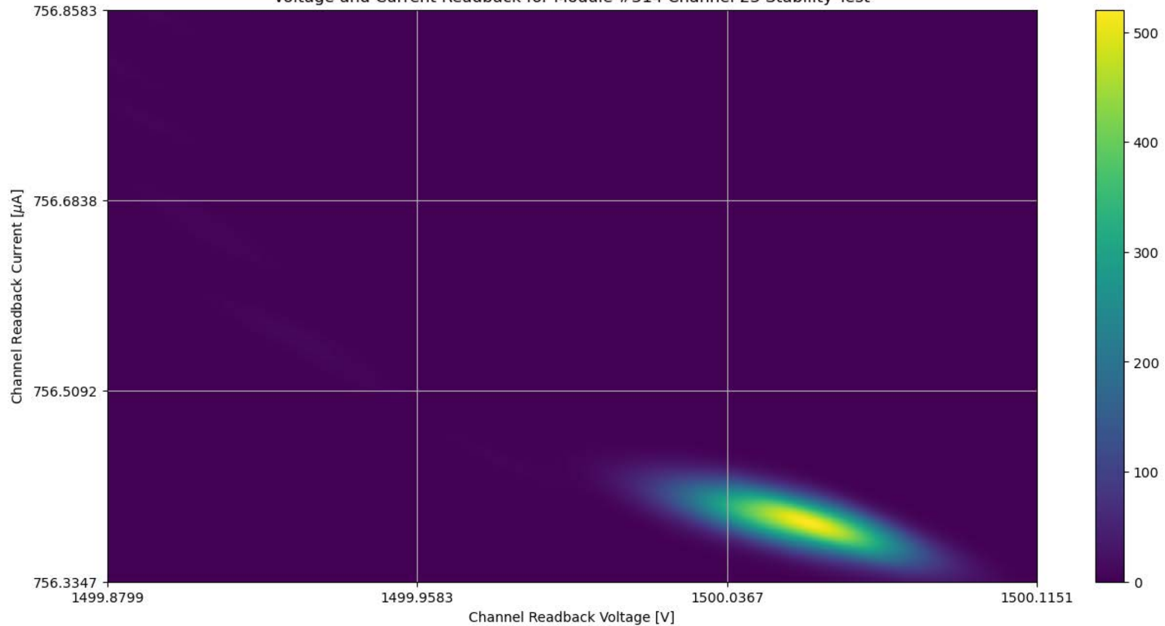
Voltage and Current Readback for Module #314 Channel 23 Stability Test
