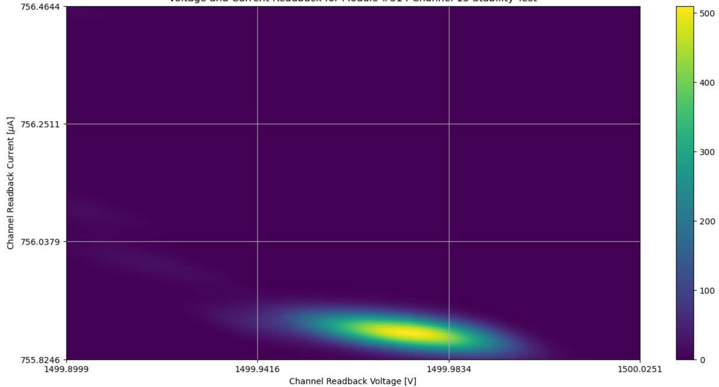
Voltage and Current Readback for Module #314 Channel 15 Stability Test
