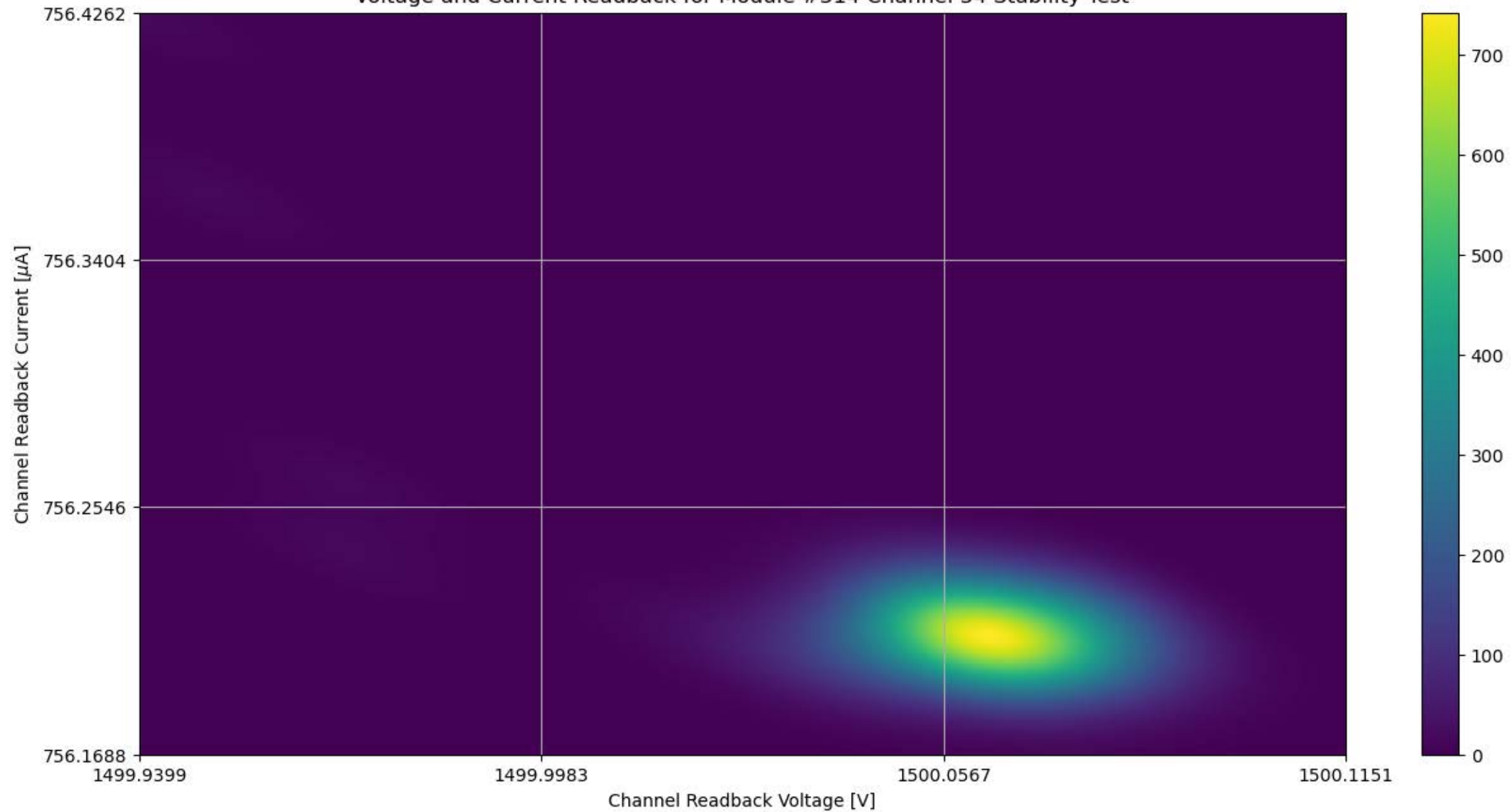
Voltage and Current Readback for Module #314 Channel 34 Stability Test
