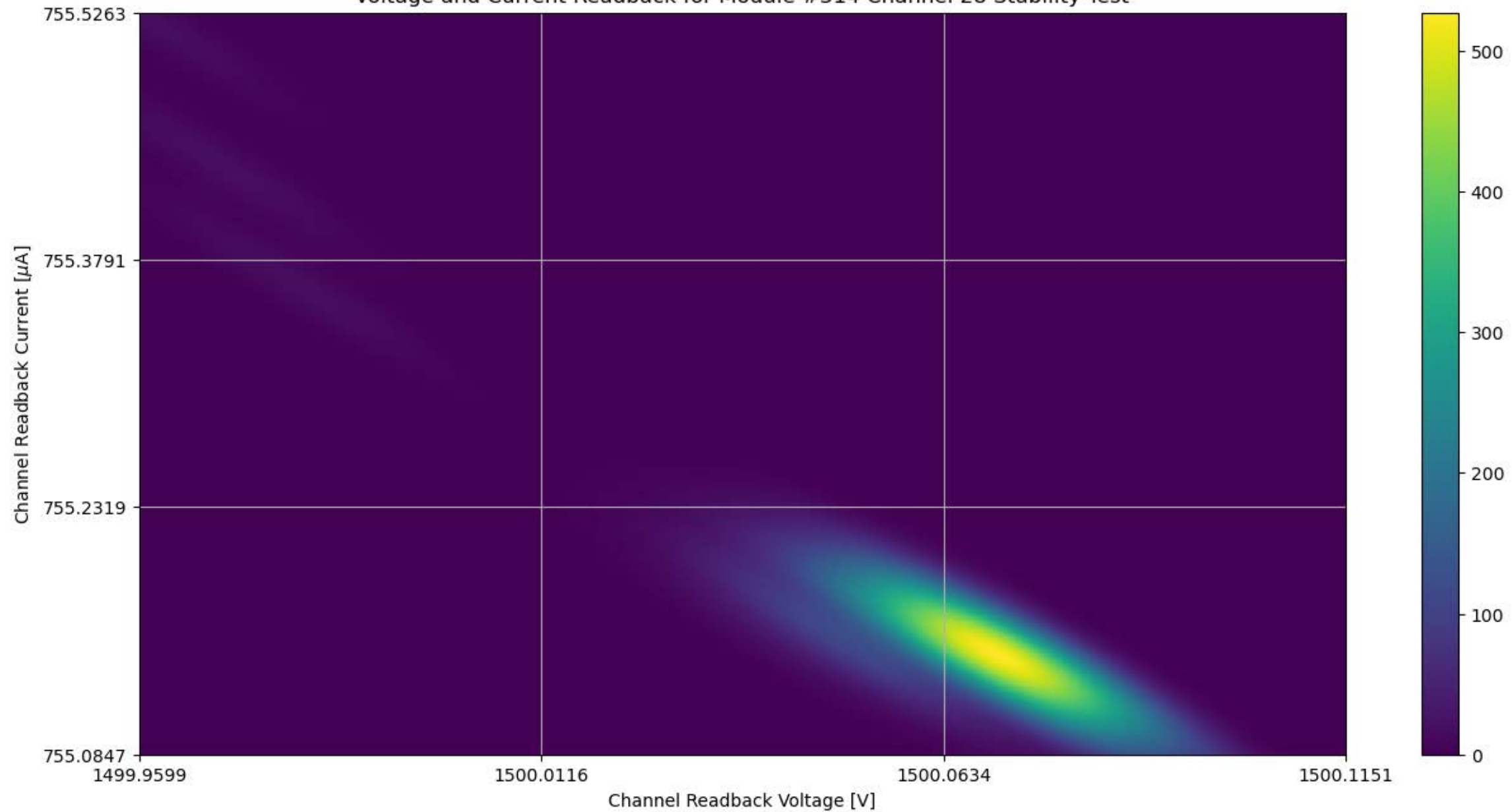
Voltage and Current Readback for Module #314 Channel 28 Stability Test
