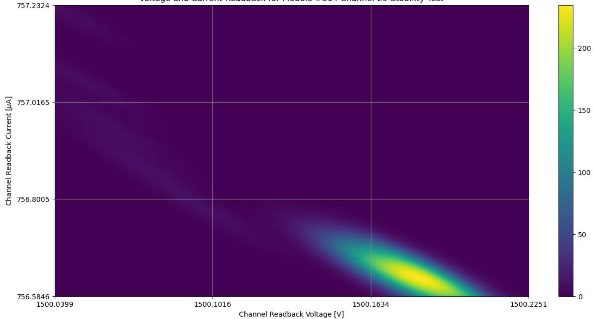
Voltage and Current Readback for Module #314 Channel 29 Stability Test
