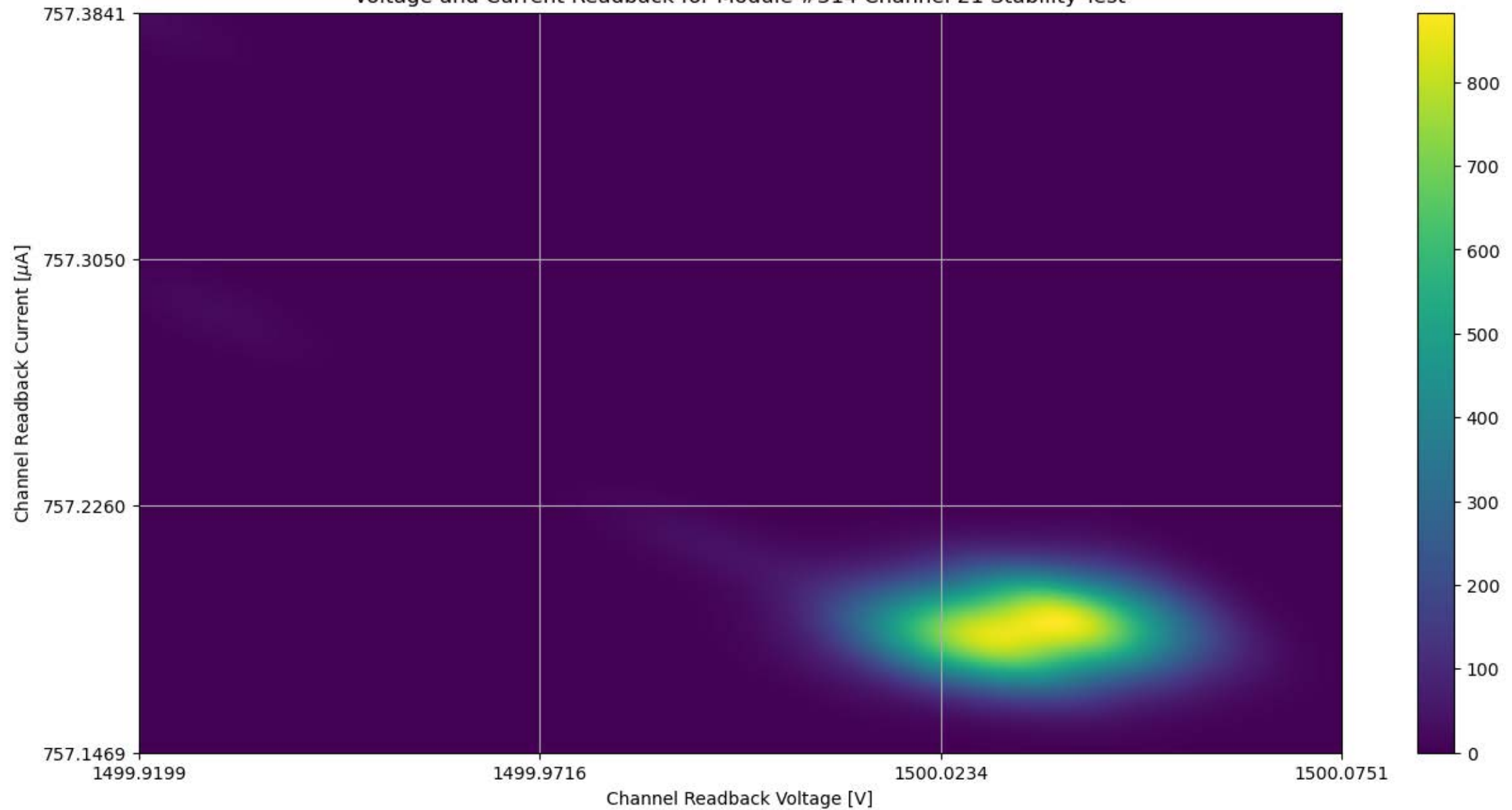
Voltage and Current Readback for Module #314 Channel 21 Stability Test
