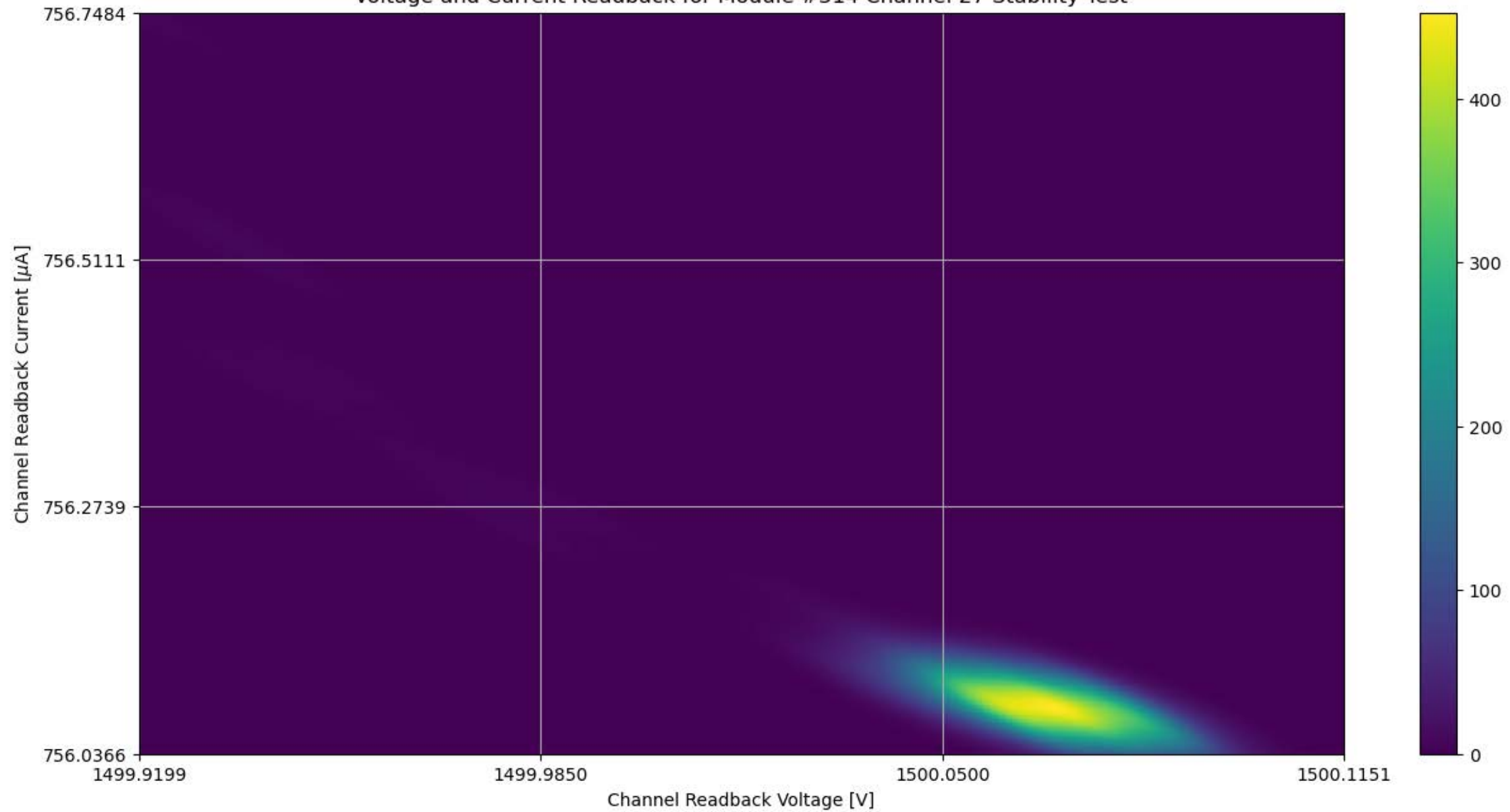
Voltage and Current Readback for Module #314 Channel 27 Stability Test
