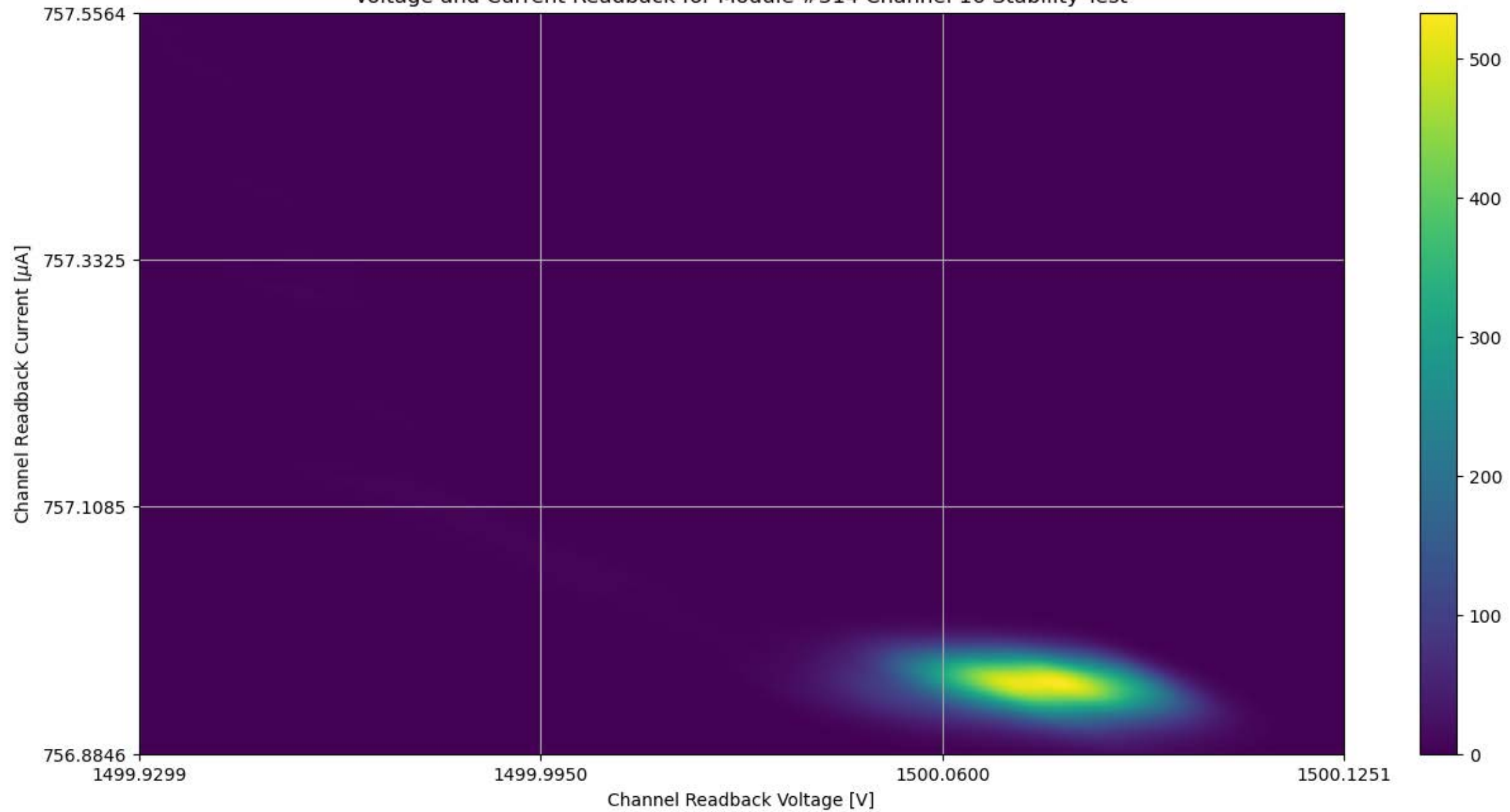
Voltage and Current Readback for Module #314 Channel 16 Stability Test
