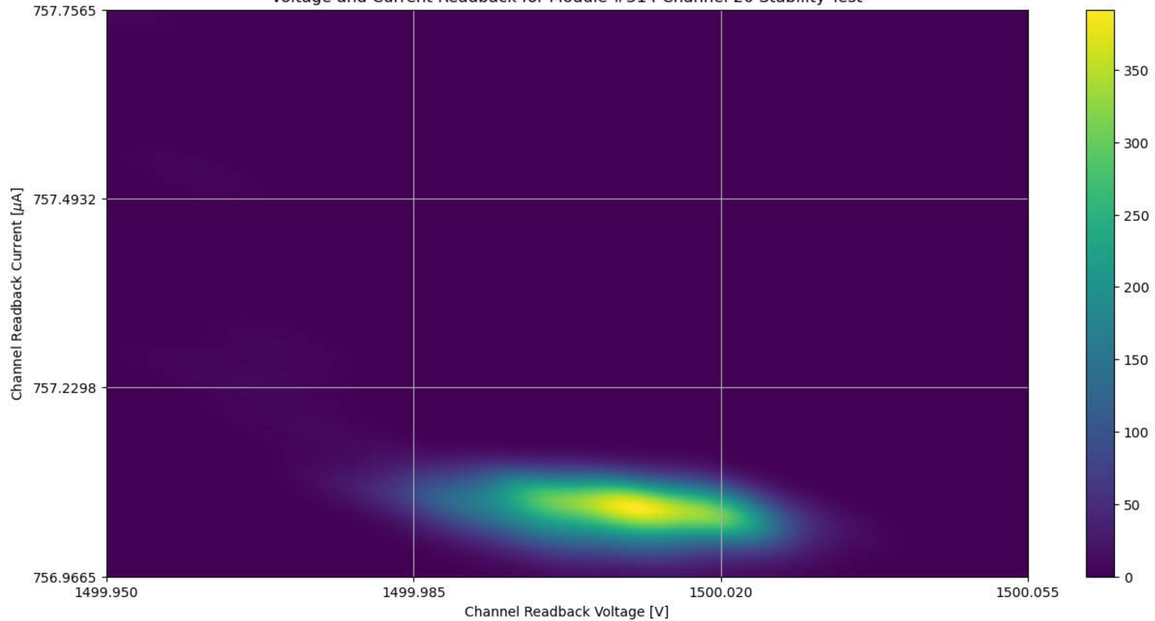
Voltage and Current Readback for Module #314 Channel 20 Stability Test
