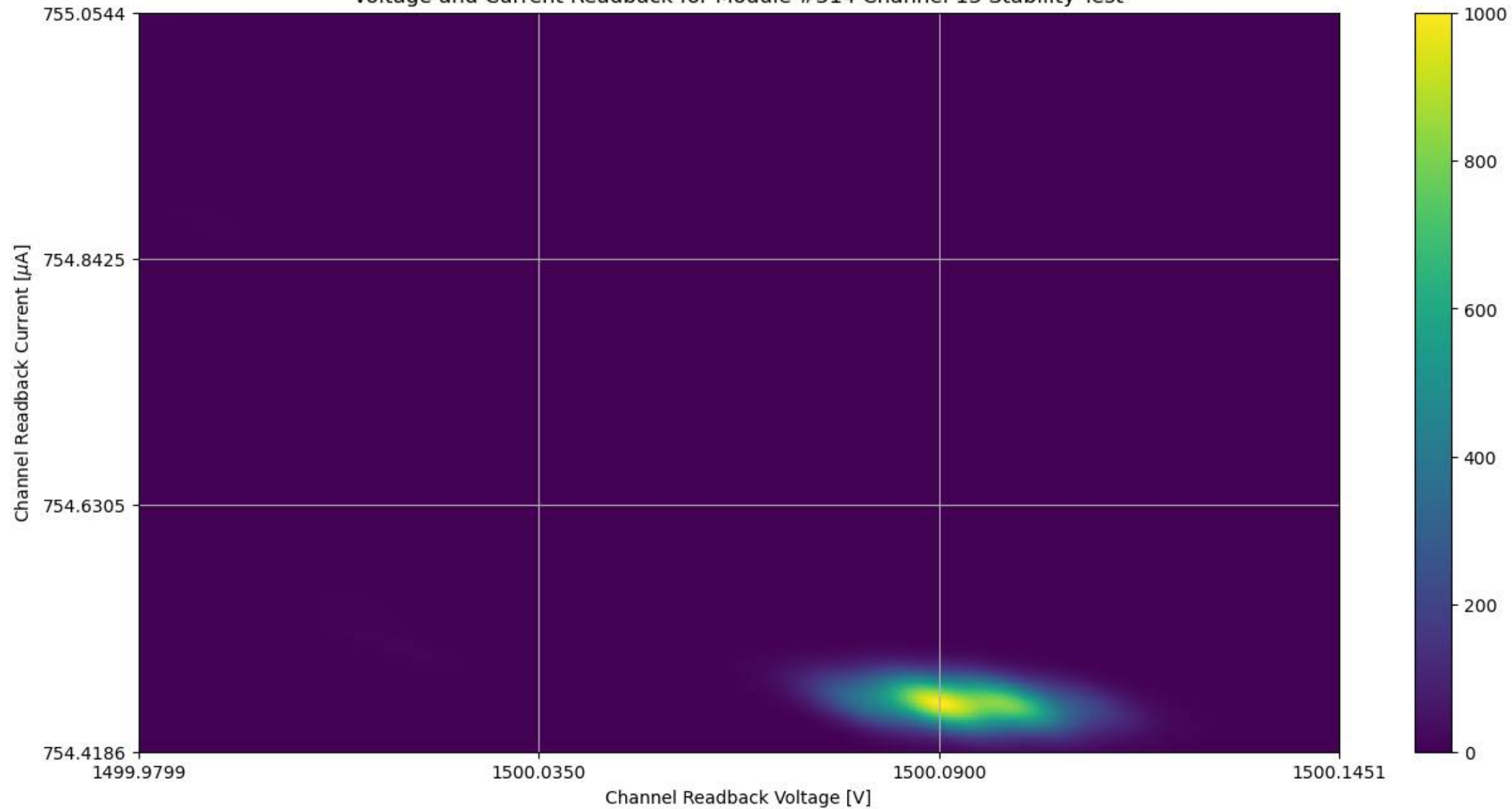
Voltage and Current Readback for Module #314 Channel 13 Stability Test
