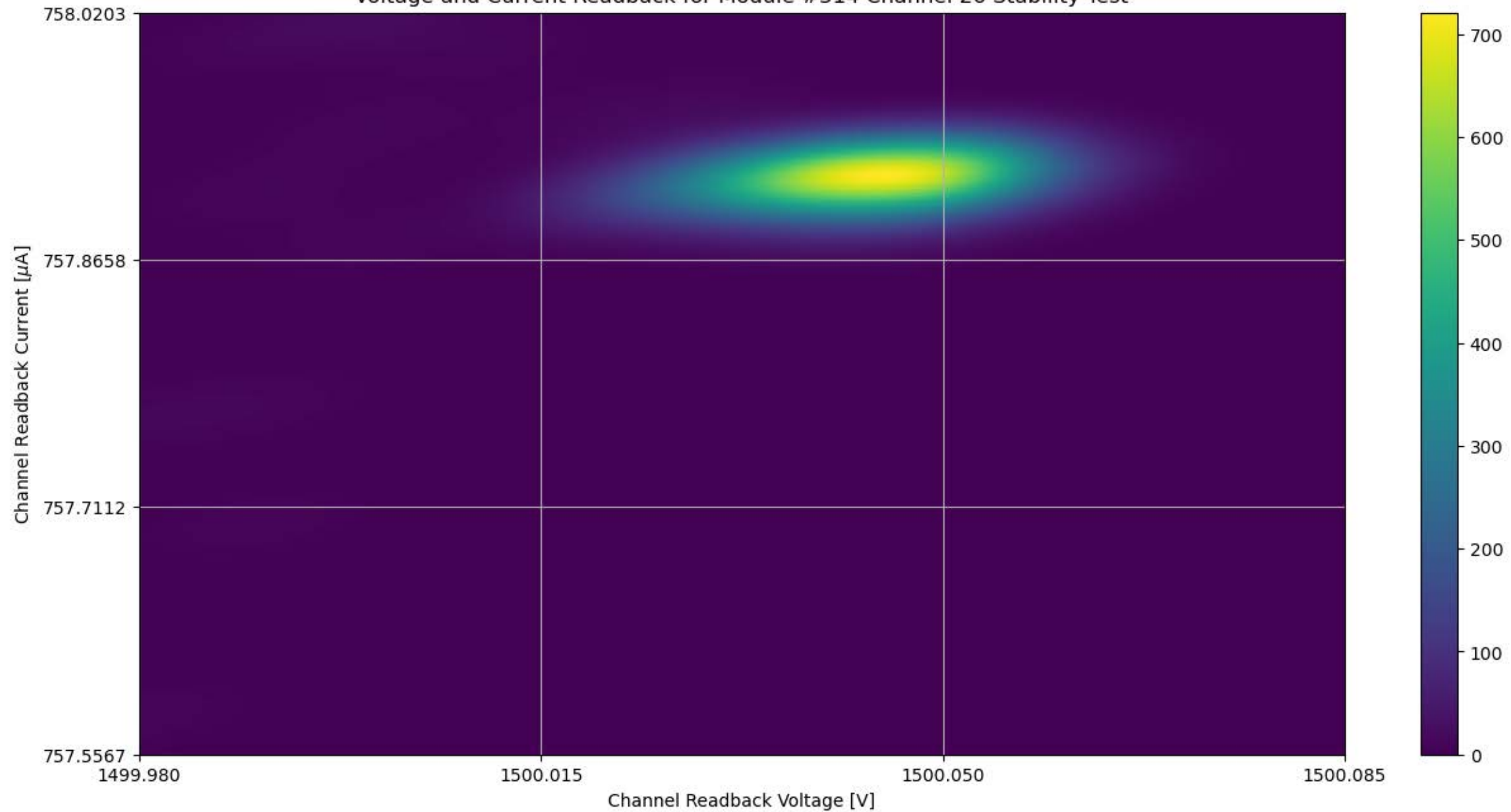
Voltage and Current Readback for Module #314 Channel 26 Stability Test
