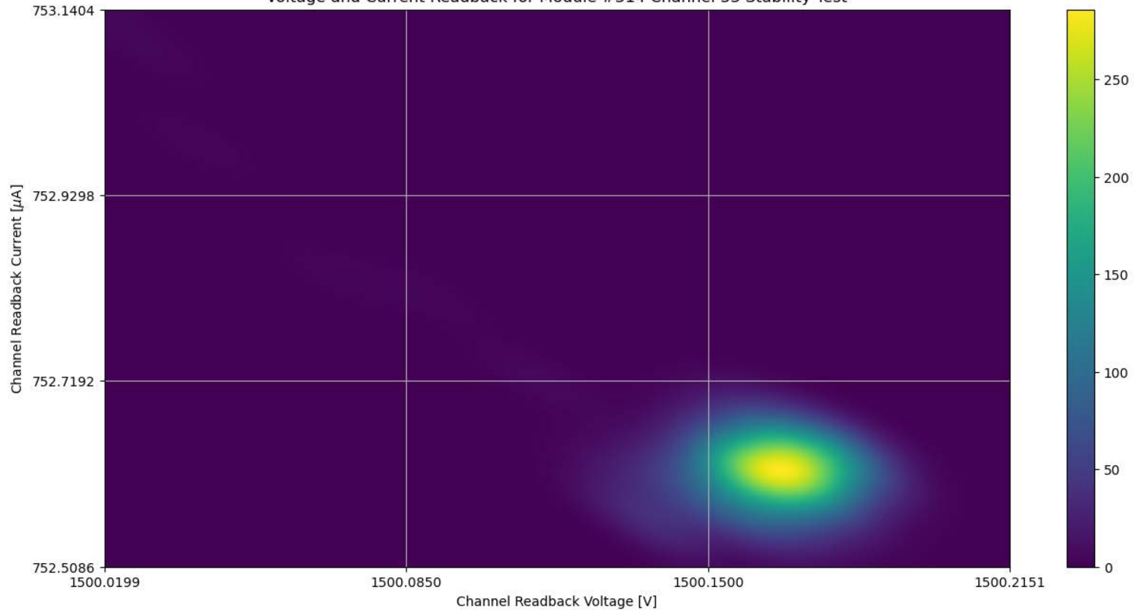
Voltage and Current Readback for Module #314 Channel 33 Stability Test
