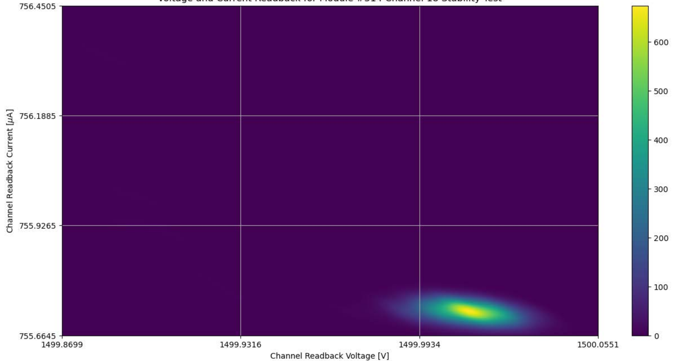
Voltage and Current Readback for Module #314 Channel 18 Stability Test
