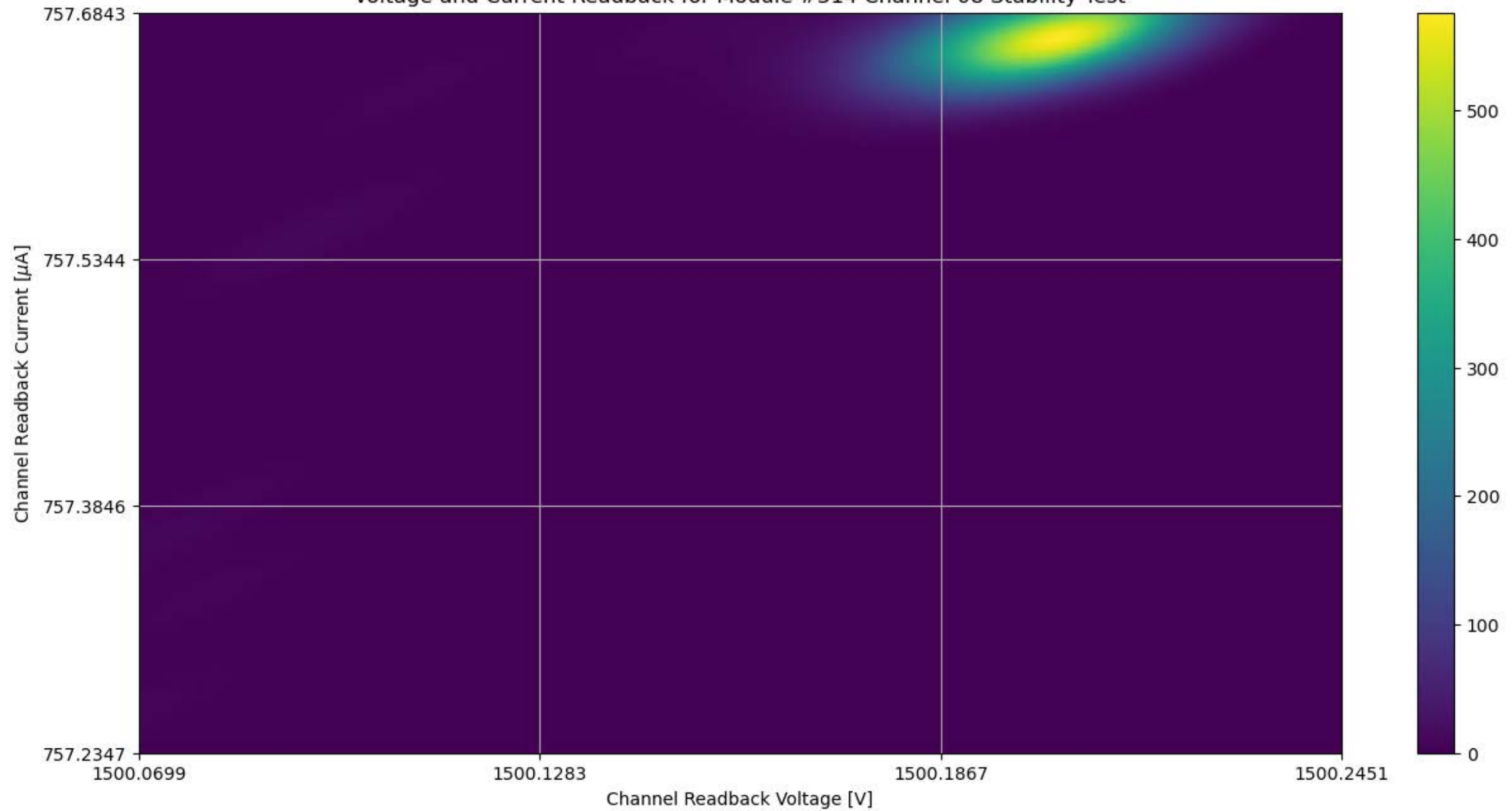
Voltage and Current Readback for Module #314 Channel 08 Stability Test
