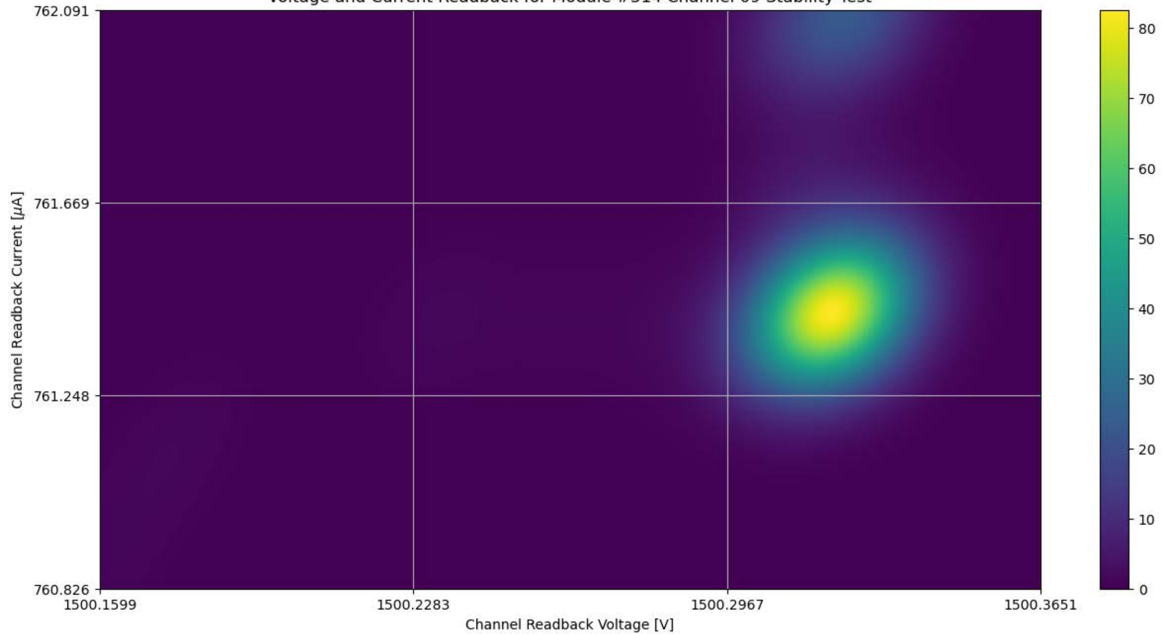
Voltage and Current Readback for Module #314 Channel 09 Stability Test
