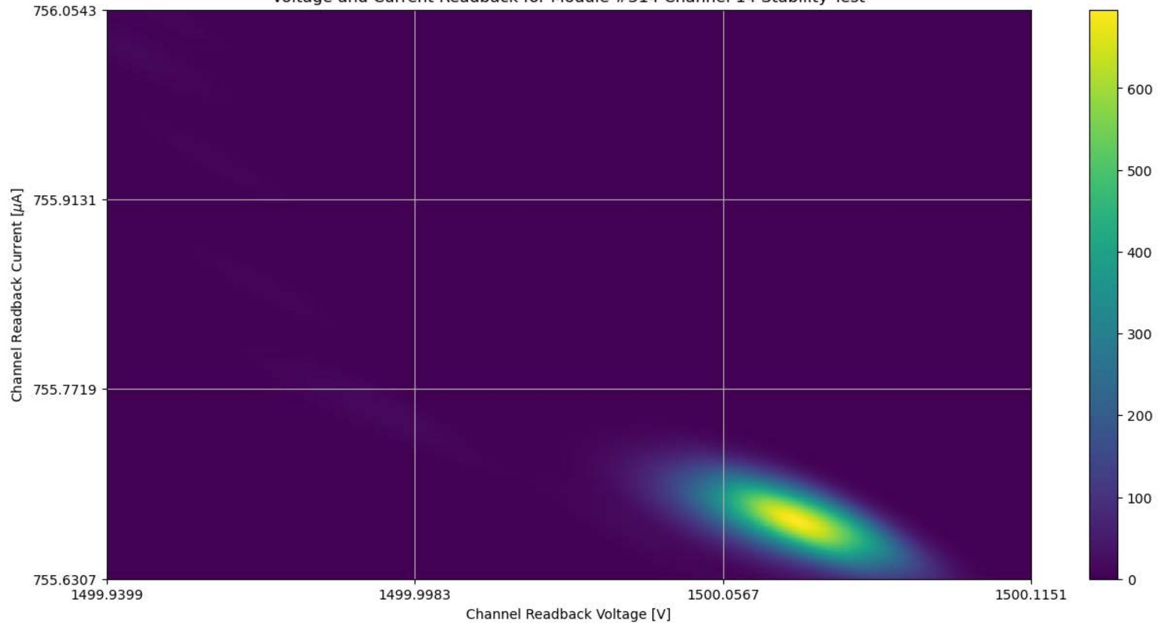
Voltage and Current Readback for Module #314 Channel 14 Stability Test
