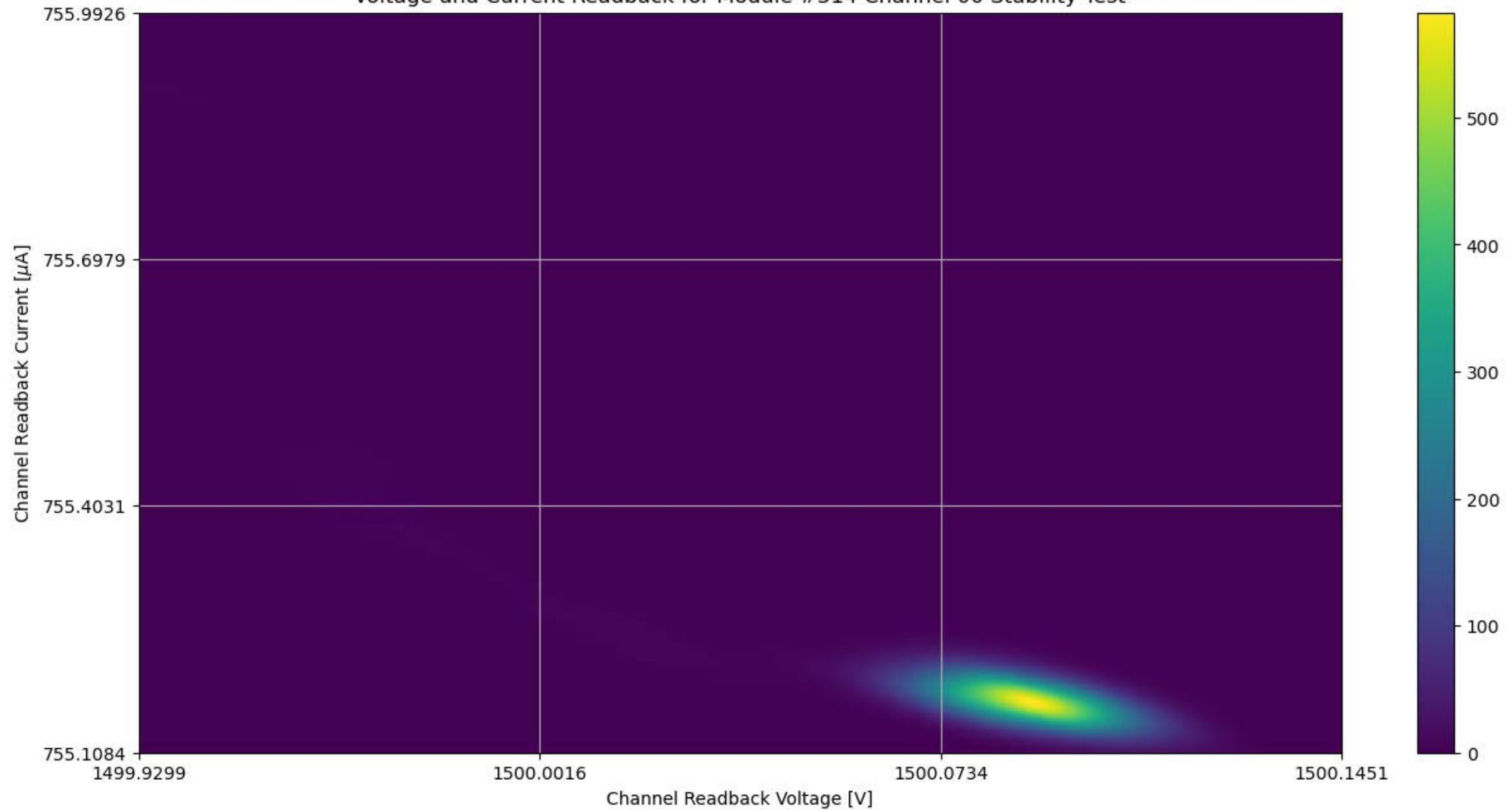
Voltage and Current Readback for Module #314 Channel 00 Stability Test
