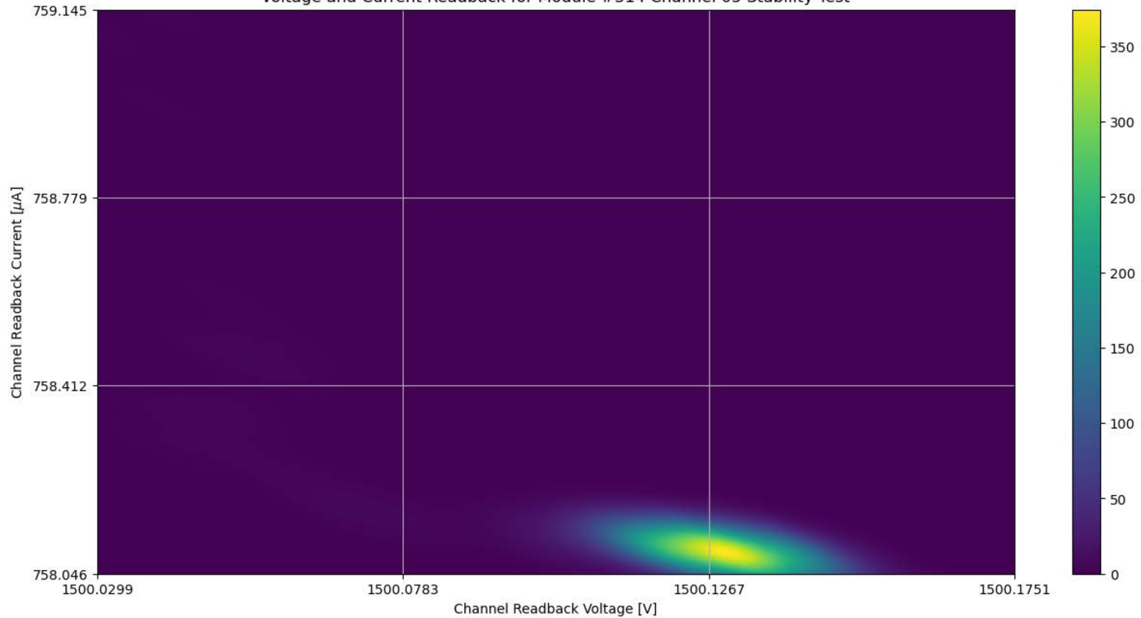
Voltage and Current Readback for Module #314 Channel 05 Stability Test
