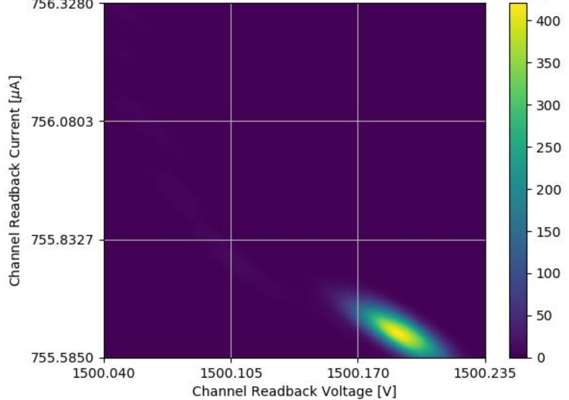
Voltage and Current Readback for Module #316 Channel 02 Stability Test
