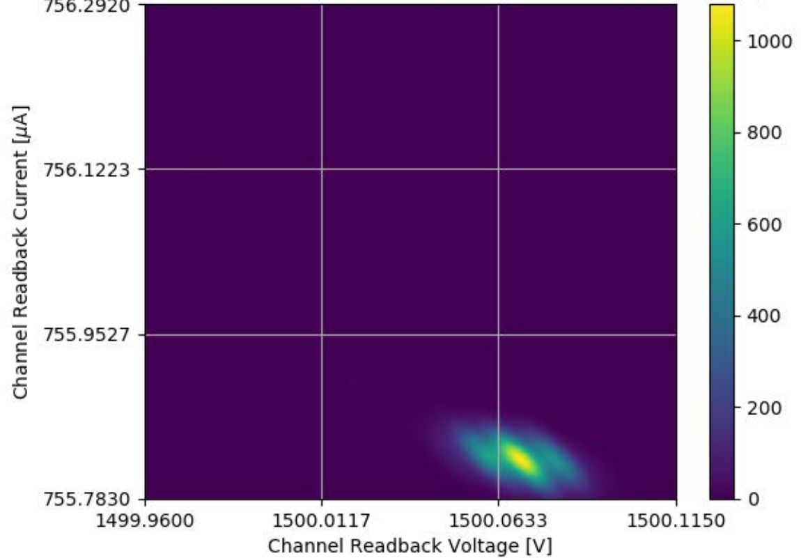
Voltage and Current Readback for Module #316 Channel 31 Stability Test
