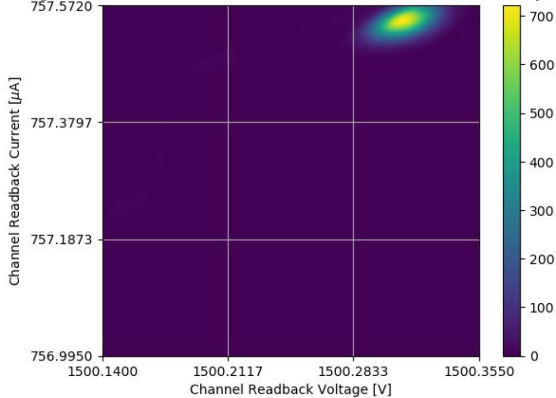
Voltage and Current Readback for Module #316 Channel 08 Stability Test
