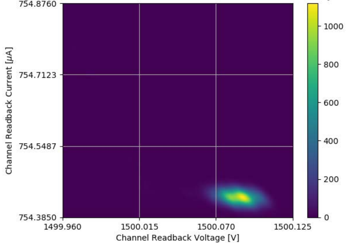
Voltage and Current Readback for Module #316 Channel 00 Stability Test
