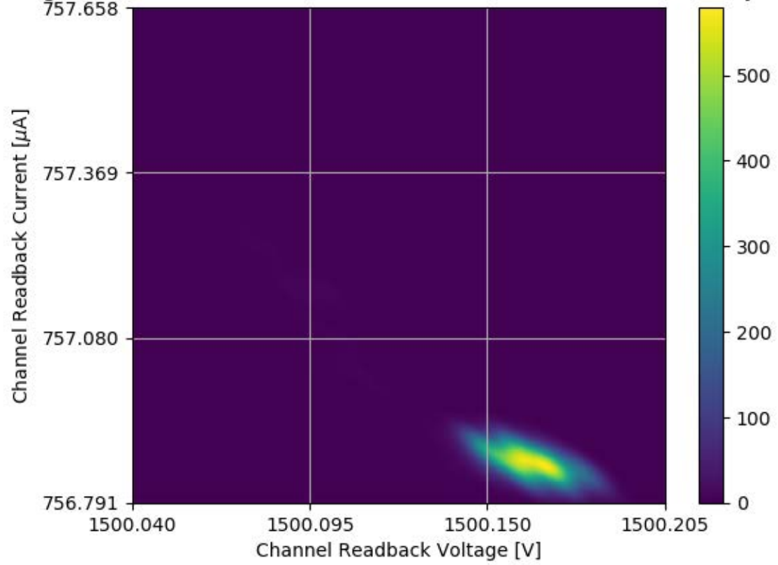
Voltage and Current Readback for Module #316 Channel 29 Stability Test
