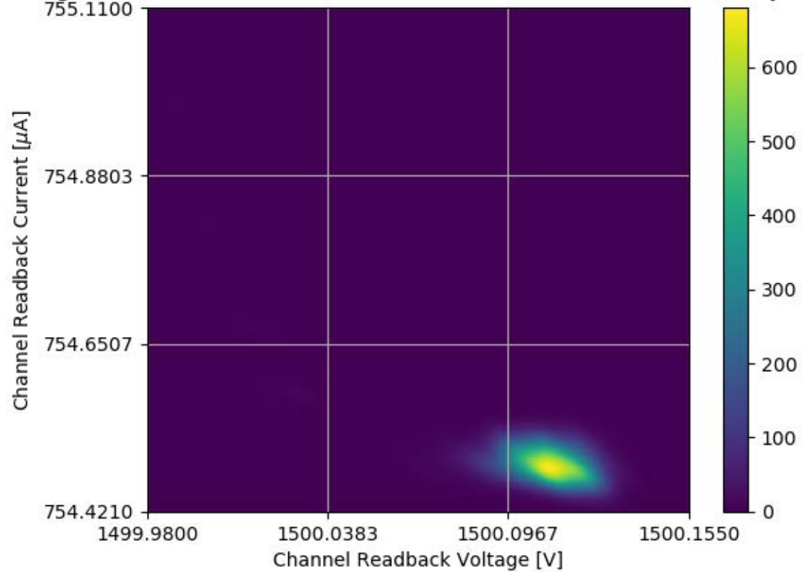
Voltage and Current Readback for Module #316 Channel 13 Stability Test
