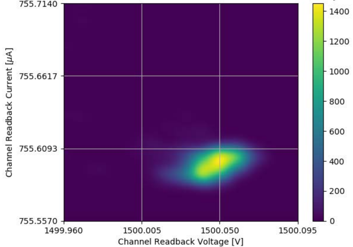
Voltage and Current Readback for Module #316 Channel 15 Stability Test
