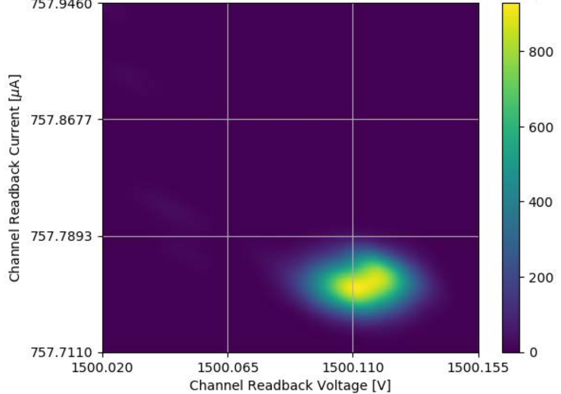
Voltage and Current Readback for Module #316 Channel 16 Stability Test
