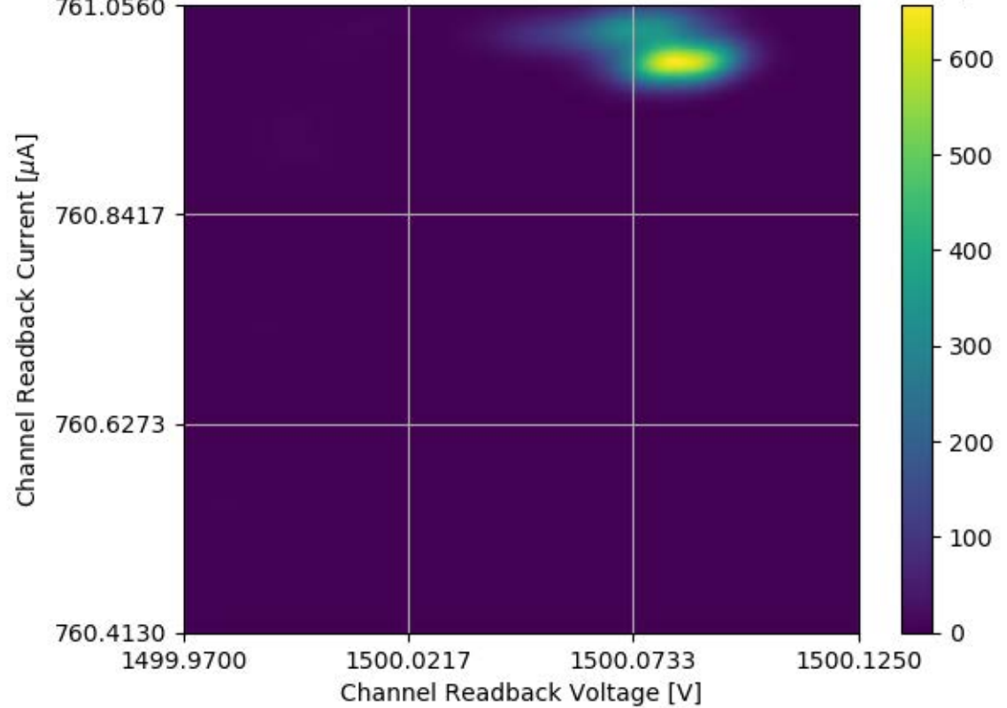
Voltage and Current Readback for Module #316 Channel 09 Stability Test
