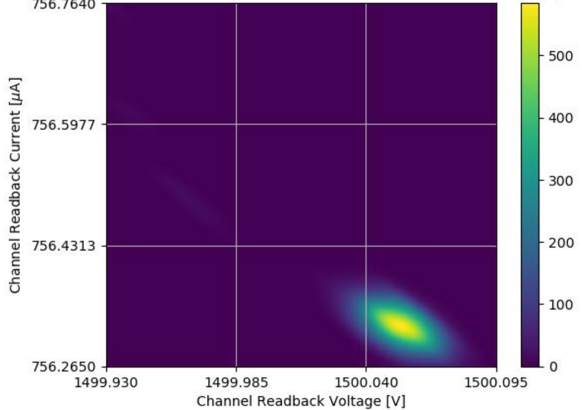
Voltage and Current Readback for Module #316 Channel 06 Stability Test
