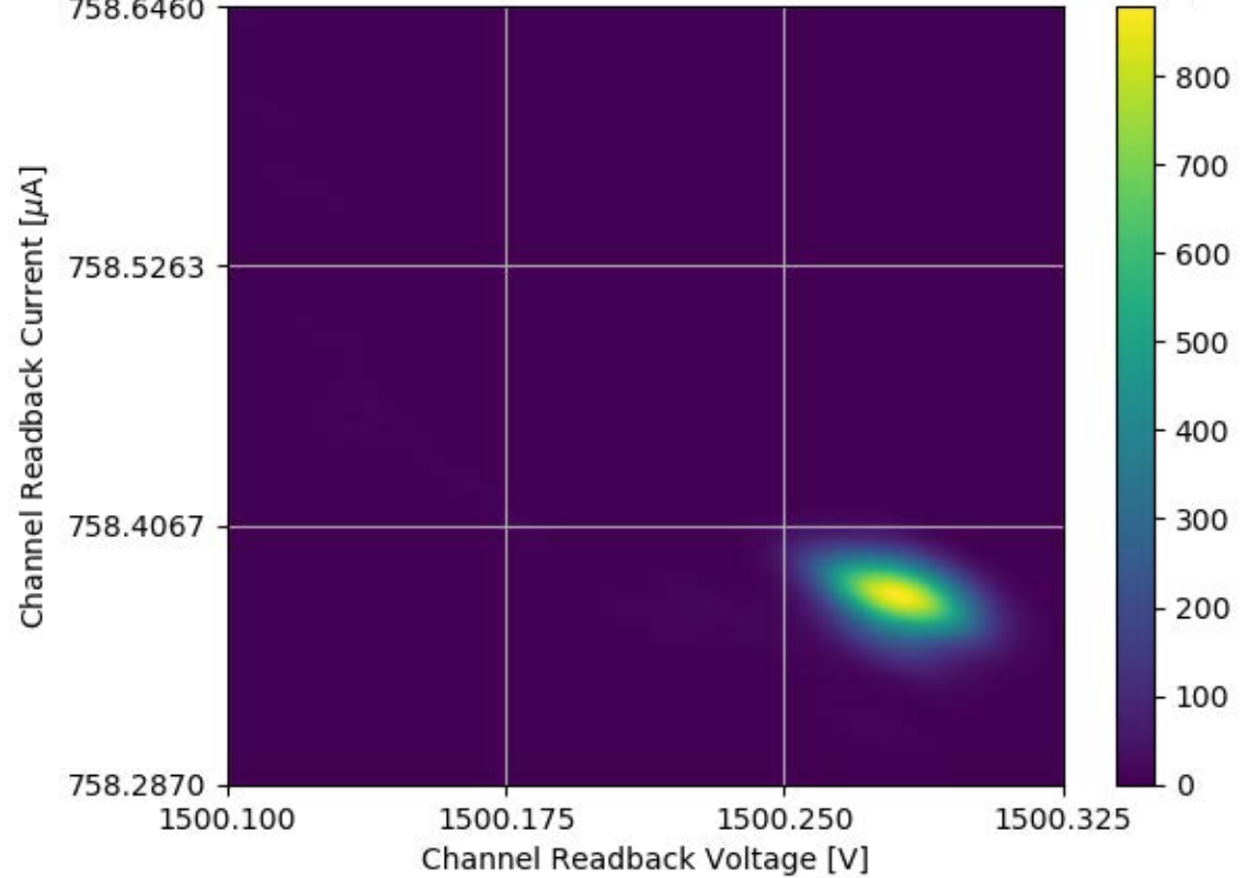
Voltage and Current Readback for Module #316 Channel 12 Stability Test
