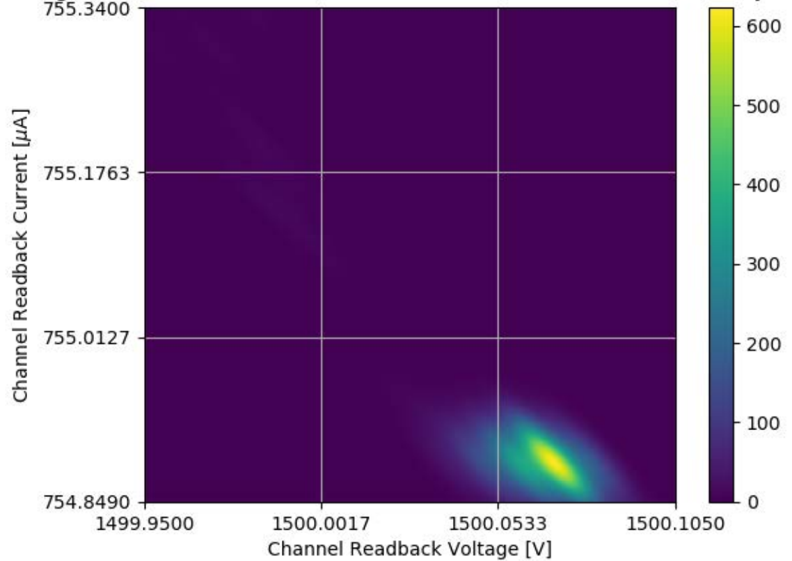
Voltage and Current Readback for Module #316 Channel 01 Stability Test
