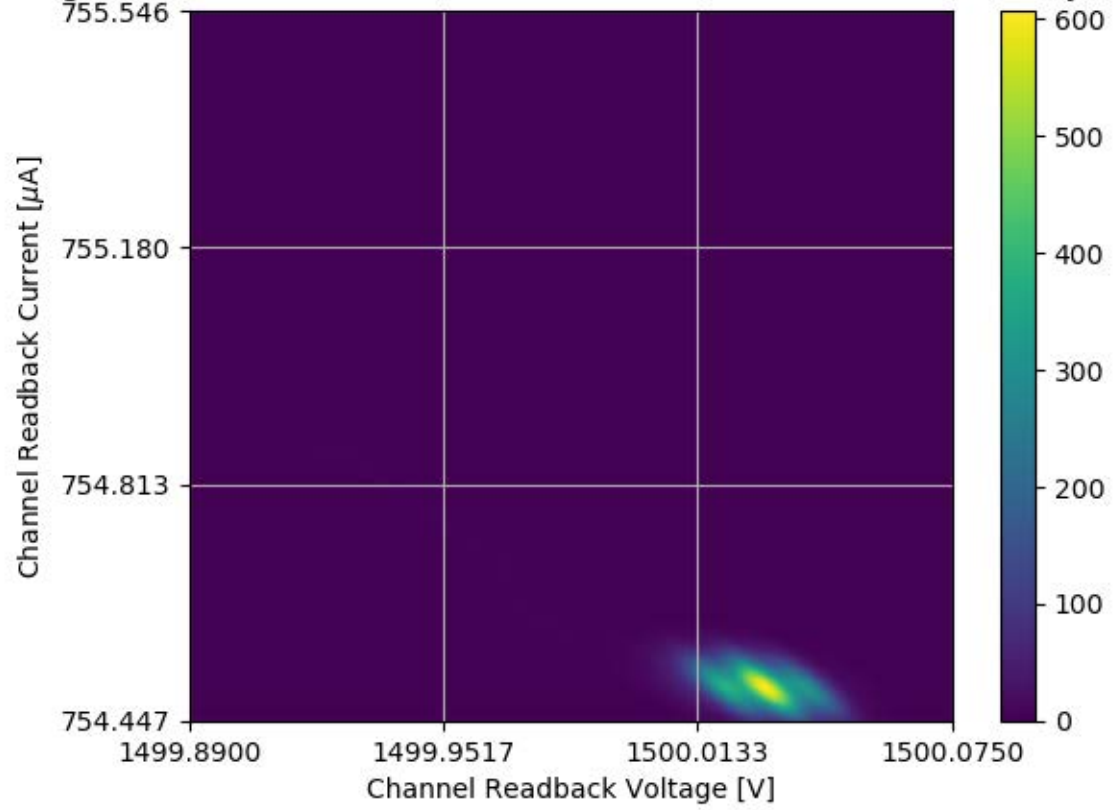
Voltage and Current Readback for Module #316 Channel 03 Stability Test
