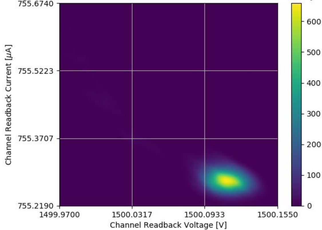
Voltage and Current Readback for Module #316 Channel 17 Stability Test
