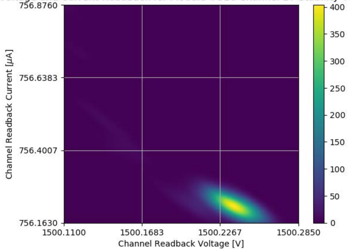
Voltage and Current Readback for Module #316 Channel 27 Stability Test
