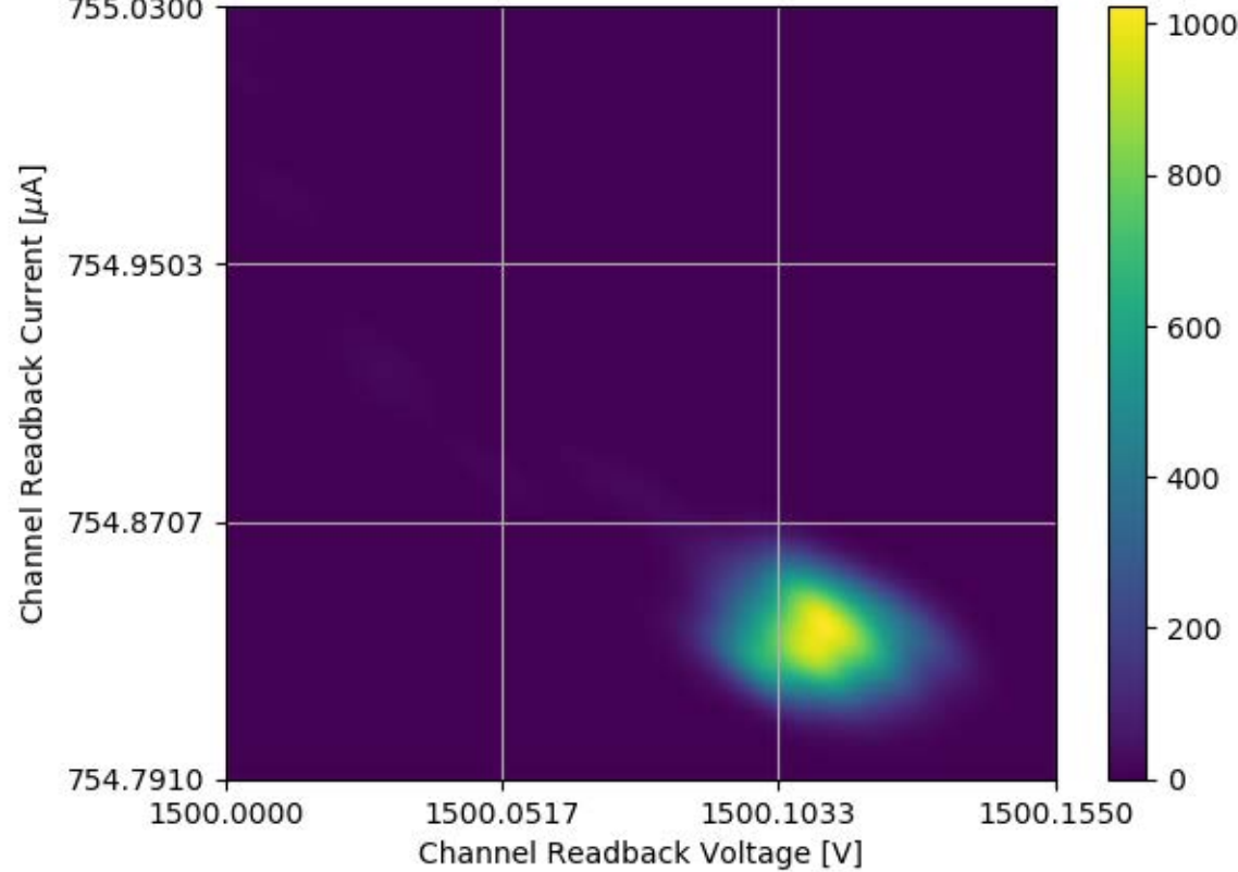
Voltage and Current Readback for Module #316 Channel 30 Stability Test
