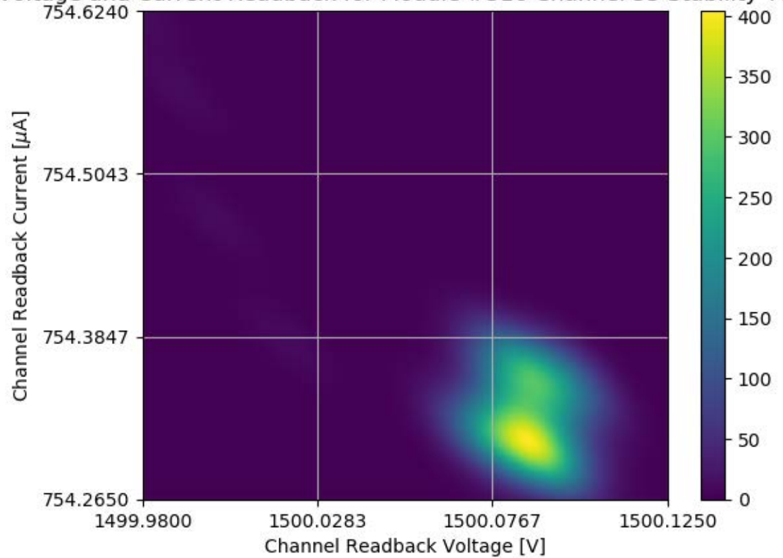
Voltage and Current Readback for Module #316 Channel 33 Stability Test
