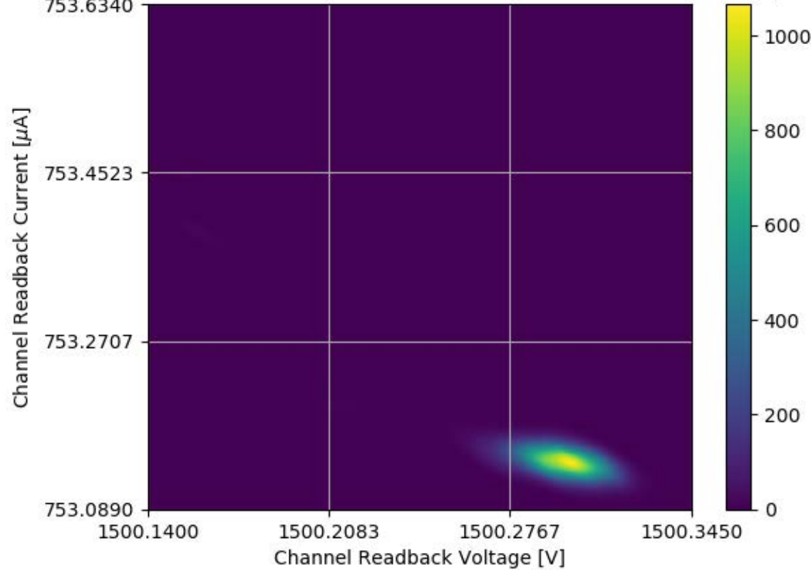
Voltage and Current Readback for Module #316 Channel 11 Stability Test
