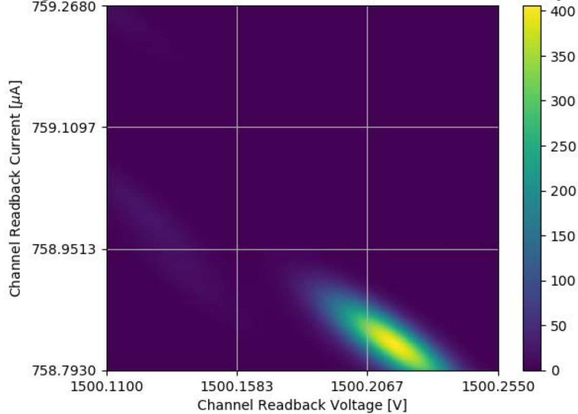
Voltage and Current Readback for Module #316 Channel 05 Stability Test
