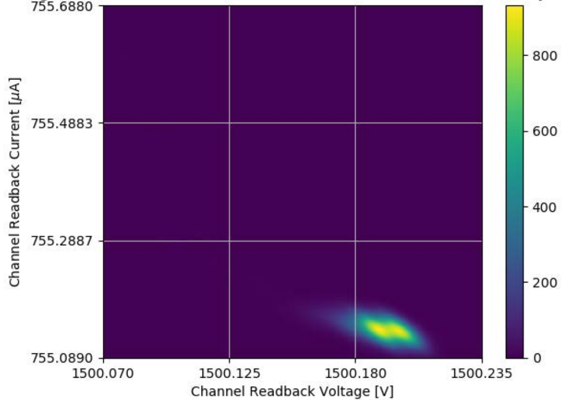
Voltage and Current Readback for Module #316 Channel 14 Stability Test
