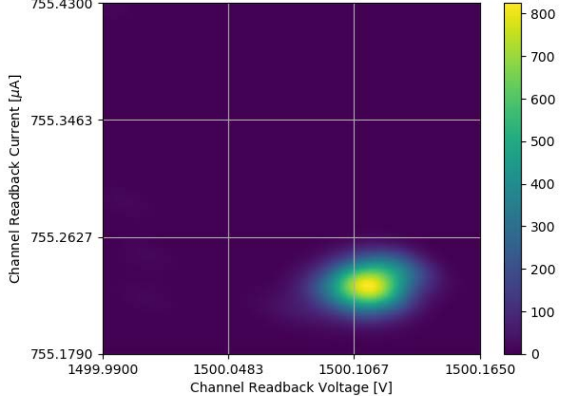
Voltage and Current Readback for Module #316 Channel 07 Stability Test
