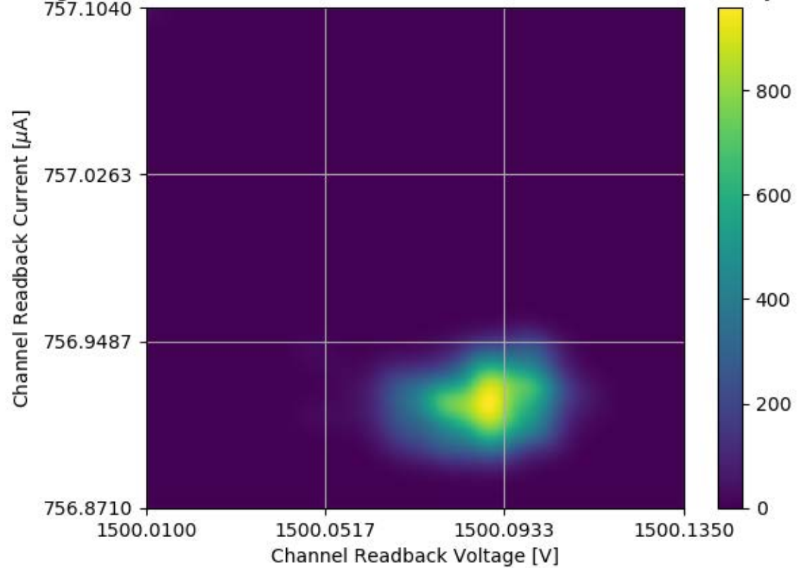
Voltage and Current Readback for Module #316 Channel 35 Stability Test
