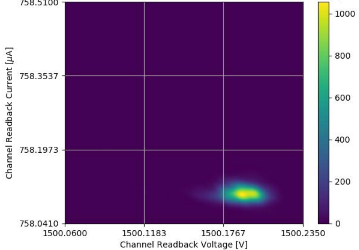
Voltage and Current Readback for Module #316 Channel 04 Stability Test
