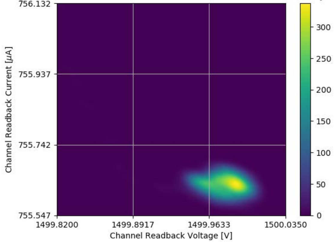
Voltage and Current Readback for Module #317 Channel 01 Stability Test
