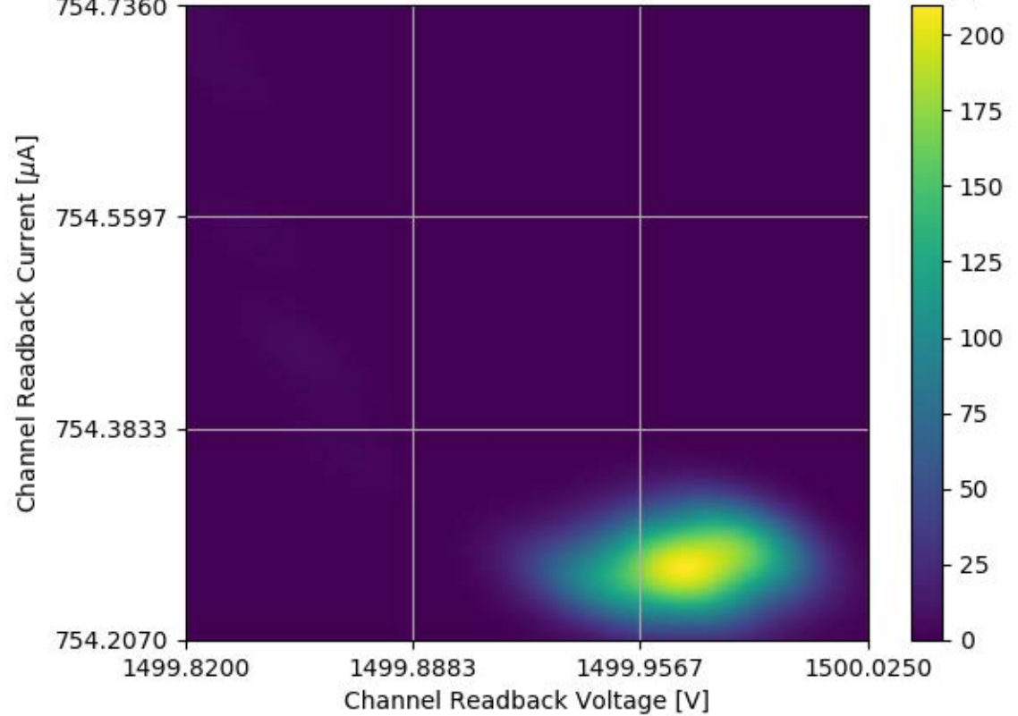
Voltage and Current Readback for Module #317 Channel 33 Stability Test
