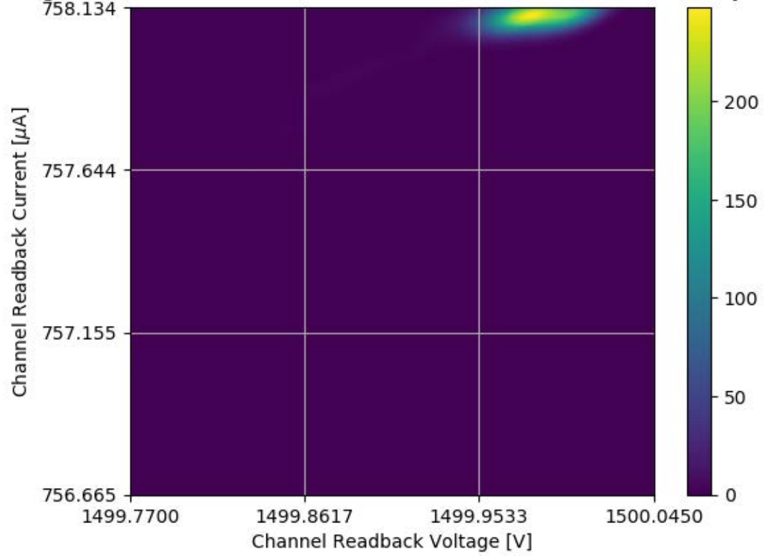
Voltage and Current Readback for Module #317 Channel 10 Stability Test
