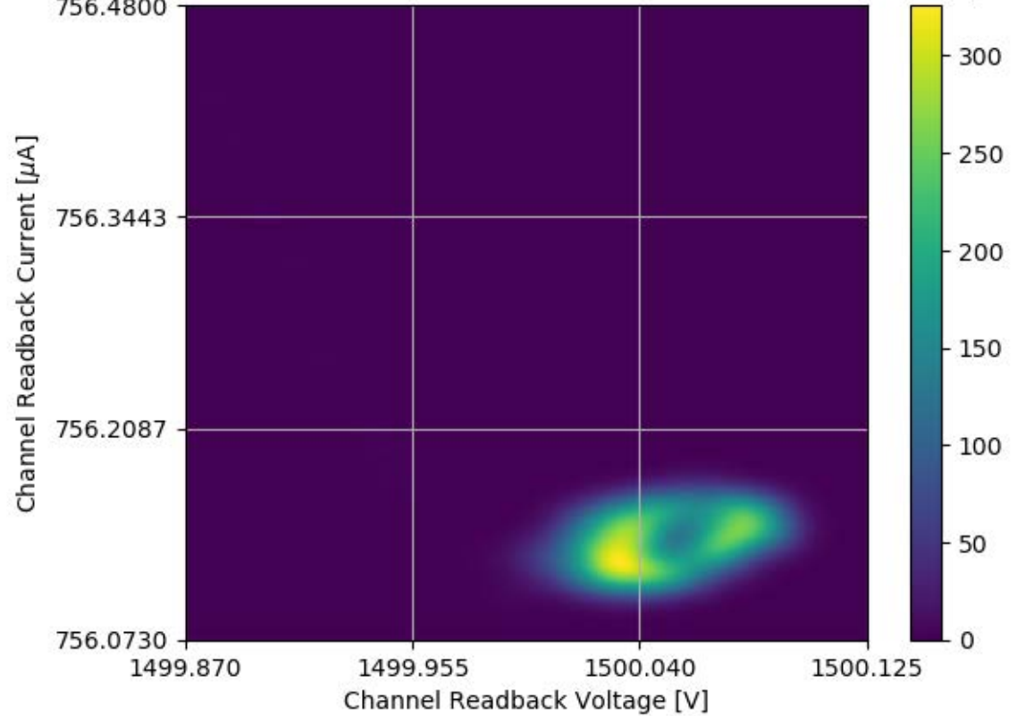
Voltage and Current Readback for Module #317 Channel 27 Stability Test
