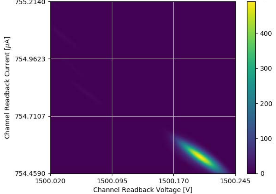
Voltage and Current Readback for Module #317 Channel 00 Stability Test
