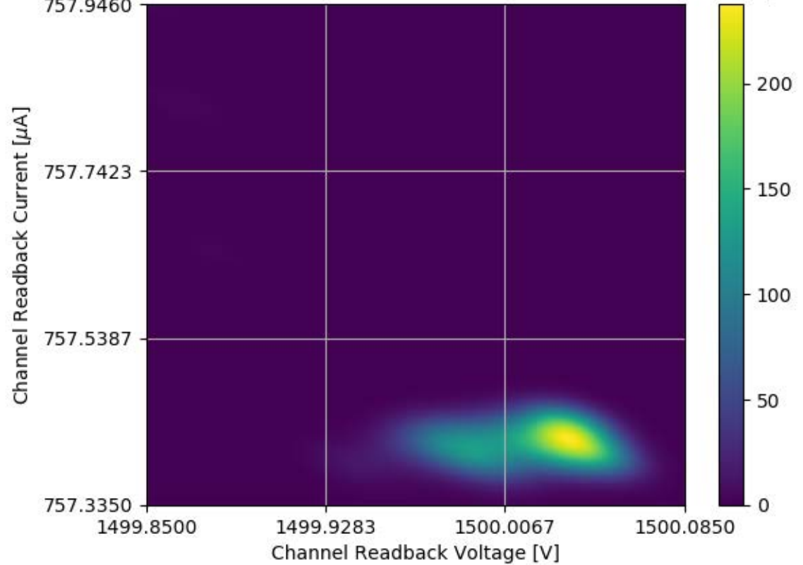
Voltage and Current Readback for Module #317 Channel 32 Stability Test
