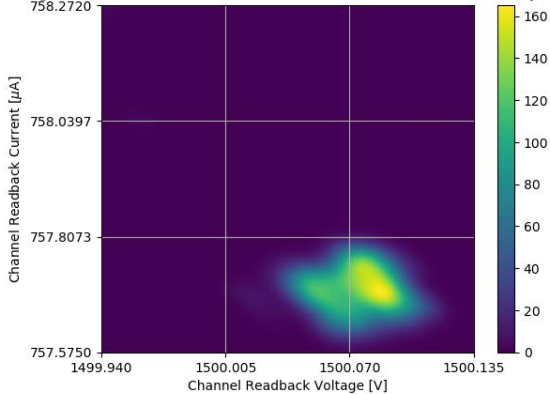
Voltage and Current Readback for Module #317 Channel 21 Stability Test
