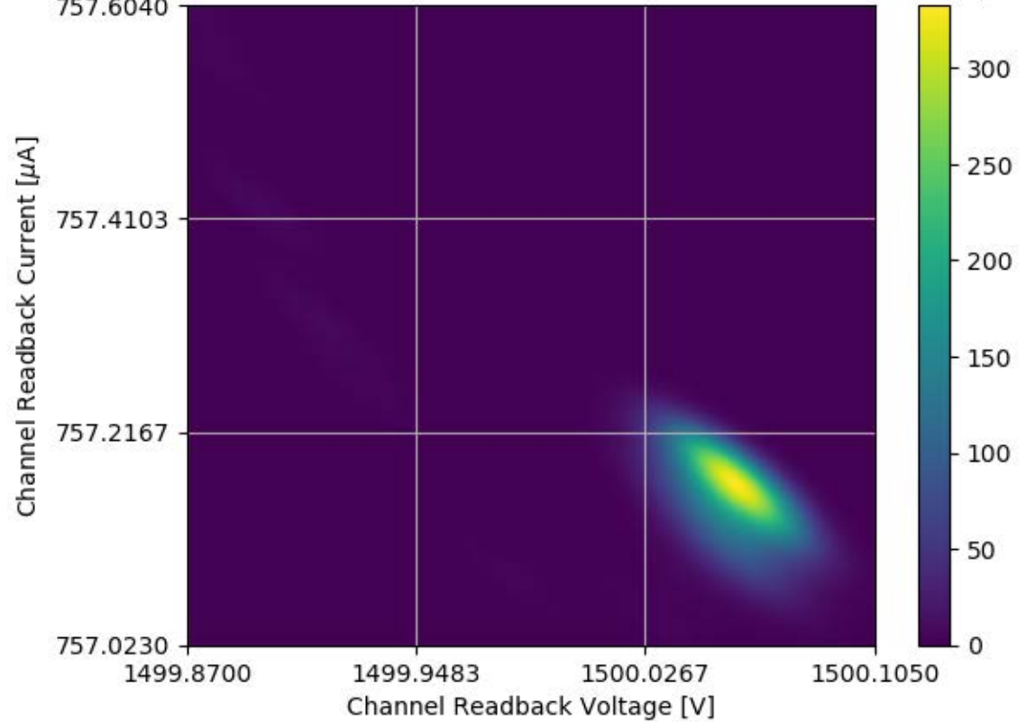
Voltage and Current Readback for Module #317 Channel 19 Stability Test
