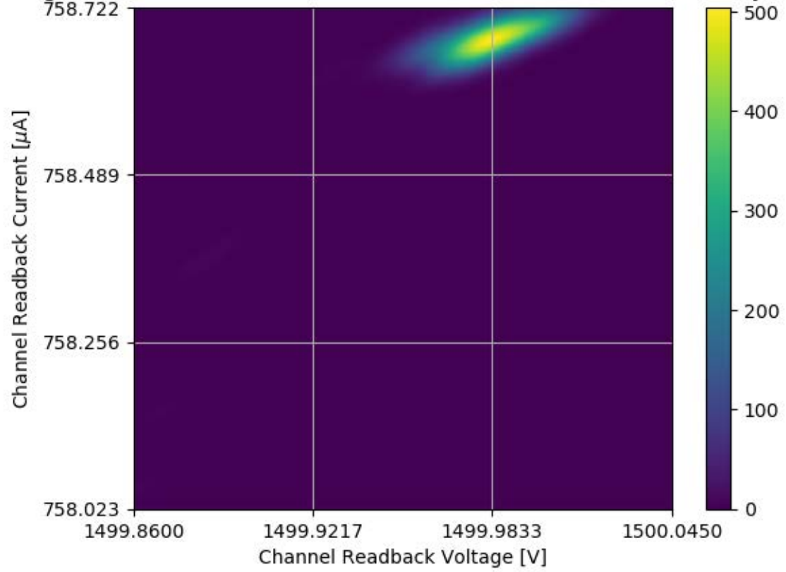
Voltage and Current Readback for Module #317 Channel 25 Stability Test
