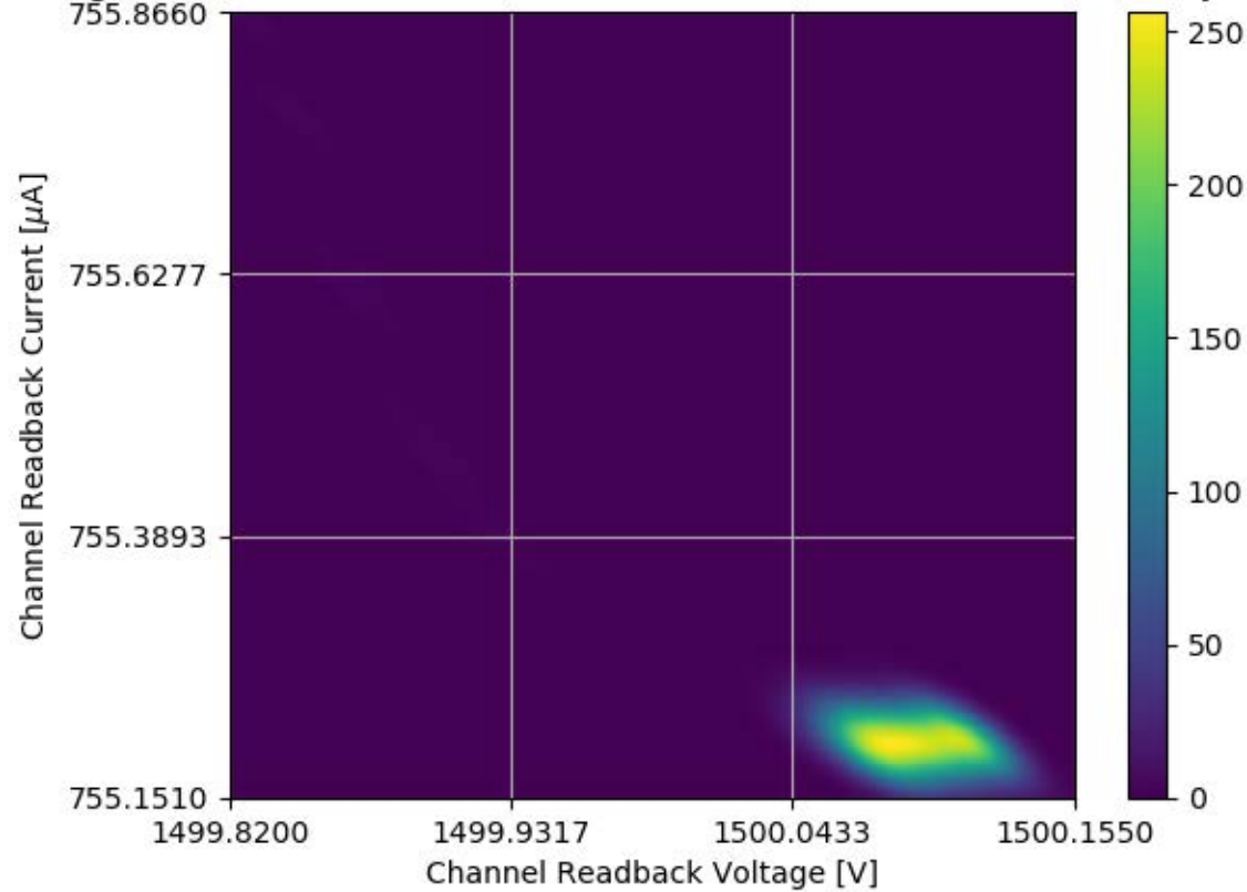
Voltage and Current Readback for Module #317 Channel 02 Stability Test
