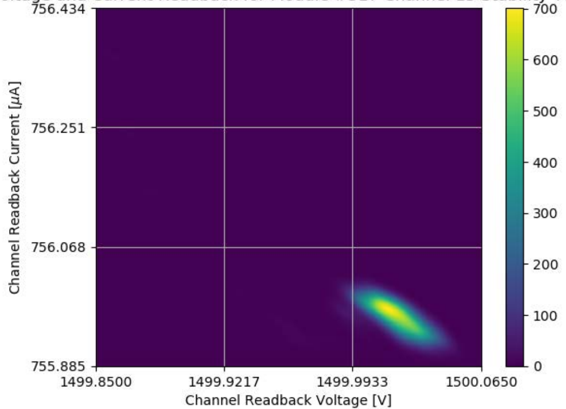
Voltage and Current Readback for Module #317 Channel 15 Stability Test
