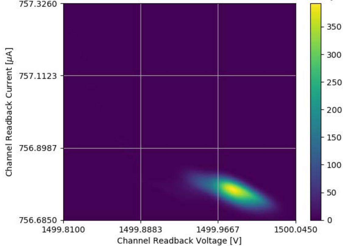
Voltage and Current Readback for Module #317 Channel 23 Stability Test
