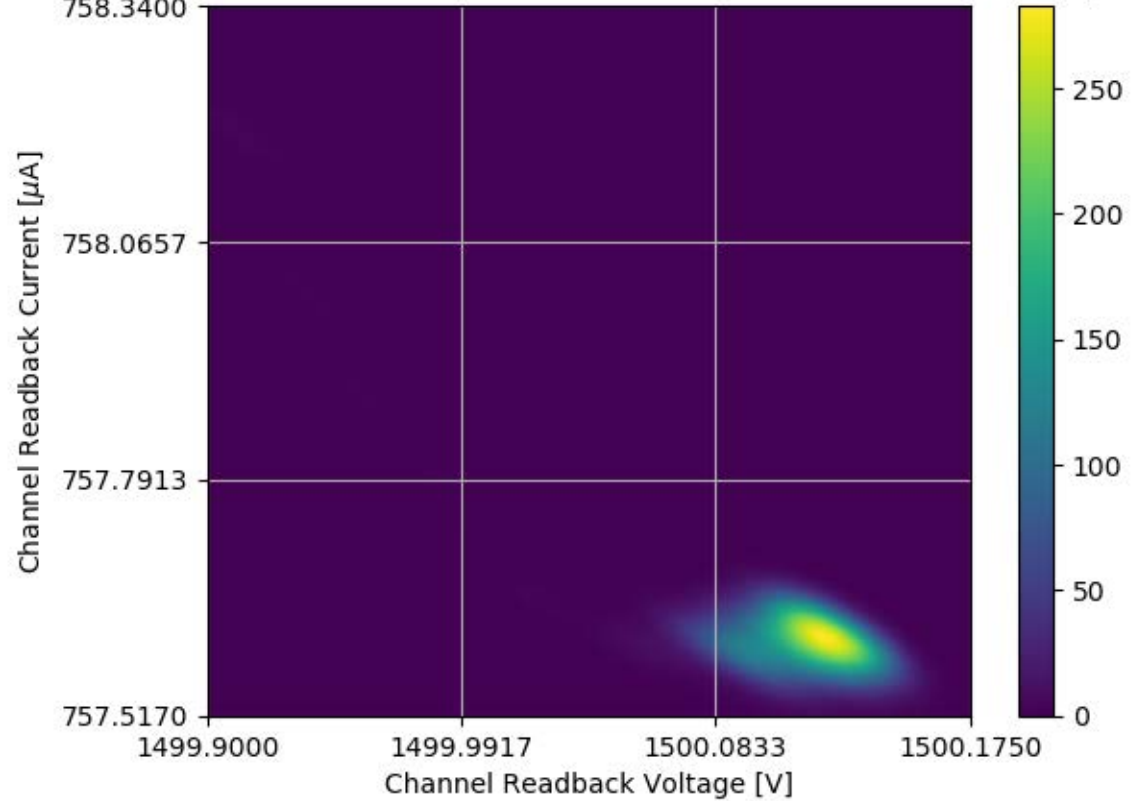
Voltage and Current Readback for Module #317 Channel 06 Stability Test
