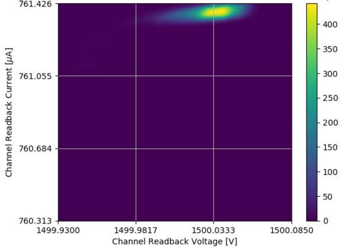
Voltage and Current Readback for Module #317 Channel 09 Stability Test
