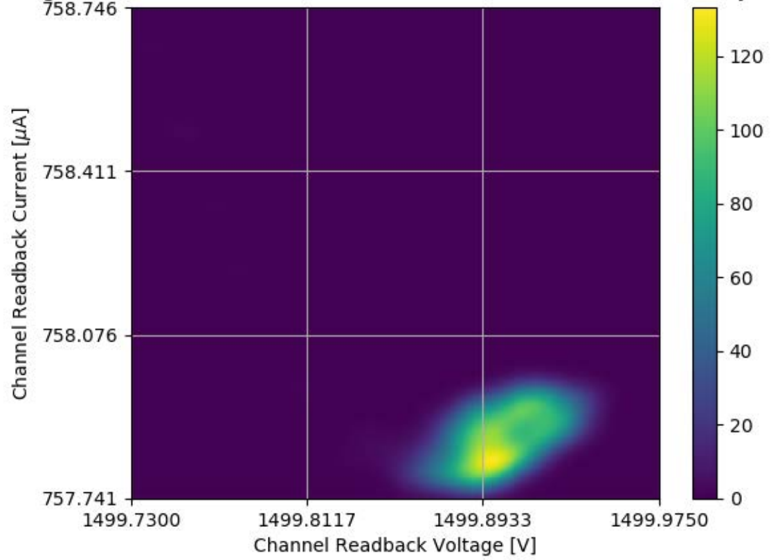
Voltage and Current Readback for Module #317 Channel 22 Stability Test
