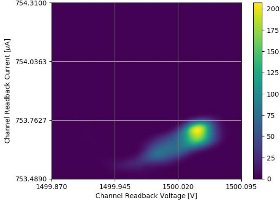
Voltage and Current Readback for Module #317 Channel 11 Stability Test
