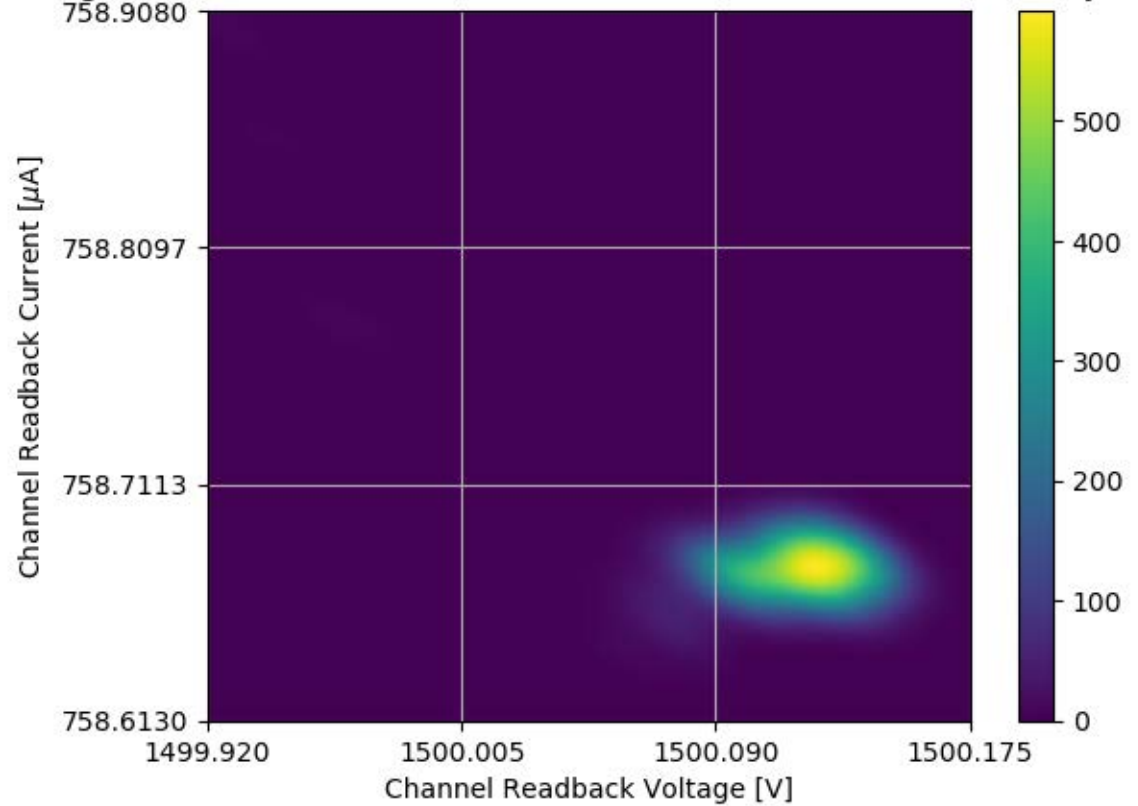
Voltage and Current Readback for Module #317 Channel 12 Stability Test
