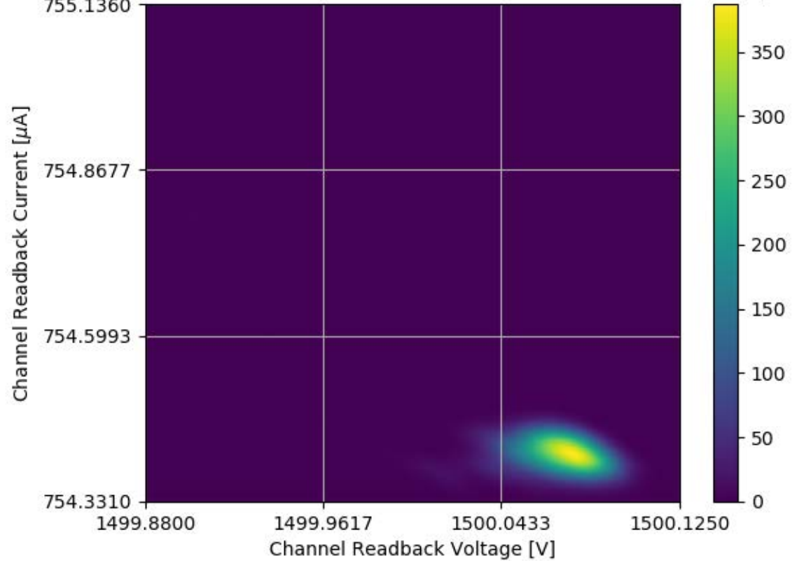
Voltage and Current Readback for Module #317 Channel 03 Stability Test
