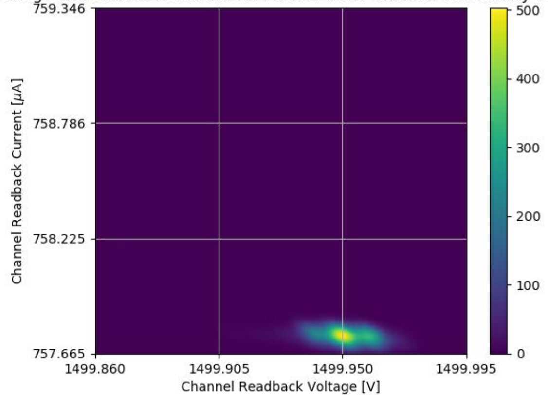
Voltage and Current Readback for Module #317 Channel 05 Stability Test
