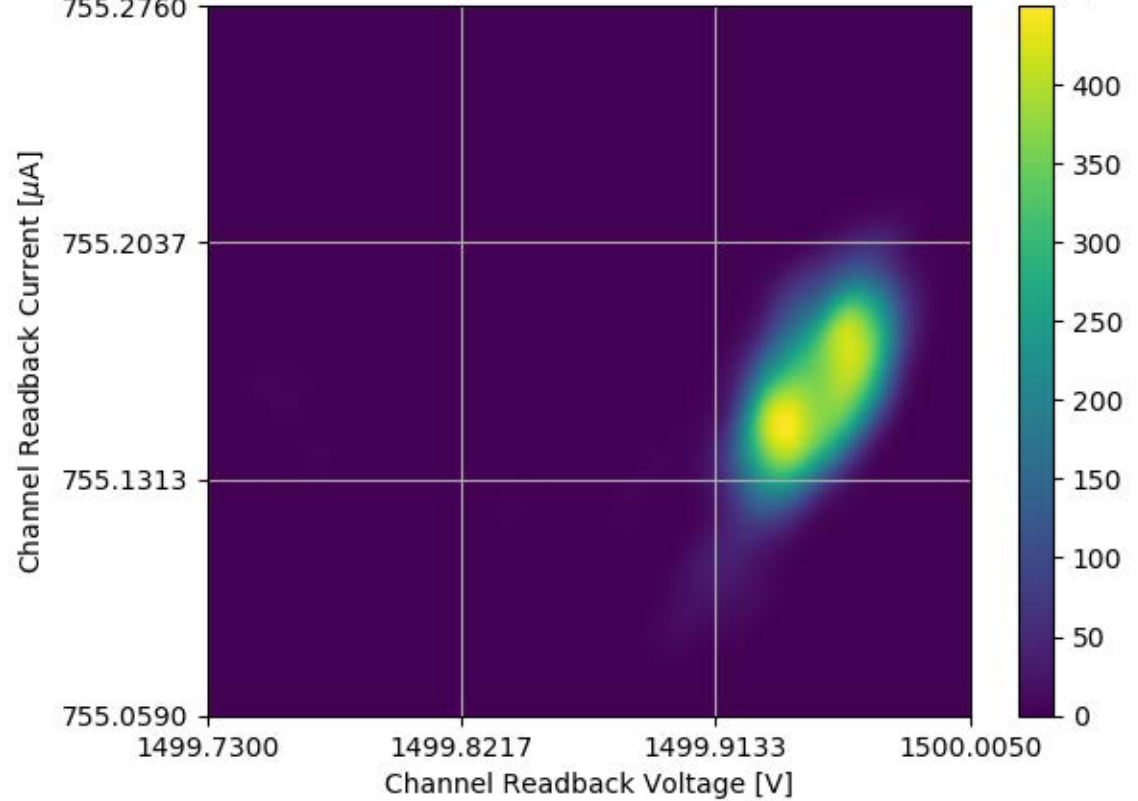
Voltage and Current Readback for Module #317 Channel 07 Stability Test
