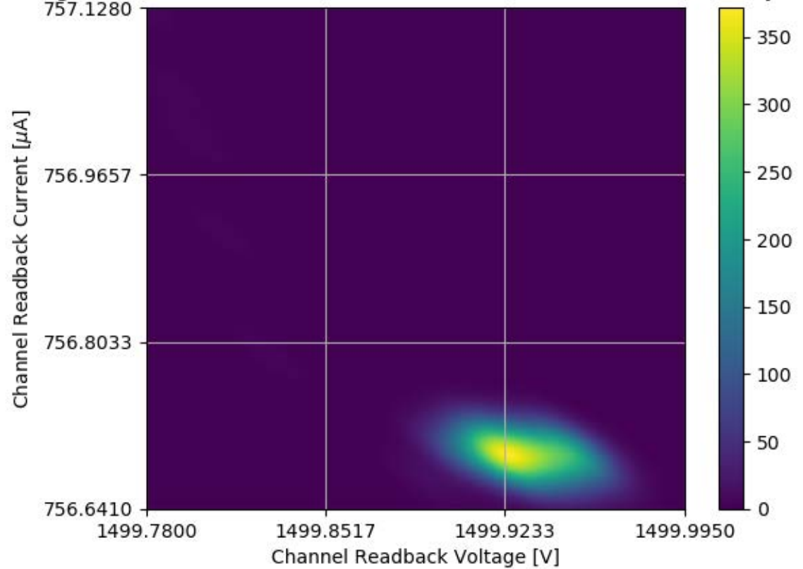
Voltage and Current Readback for Module #317 Channel 16 Stability Test
