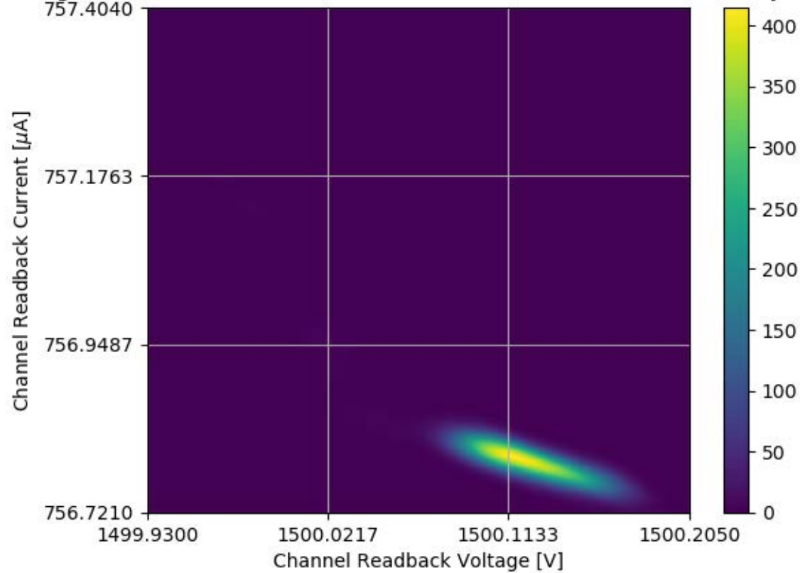
Voltage and Current Readback for Module #317 Channel 29 Stability Test
