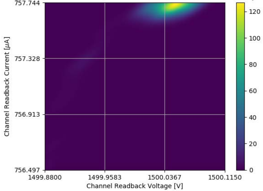
Voltage and Current Readback for Module #317 Channel 26 Stability Test
