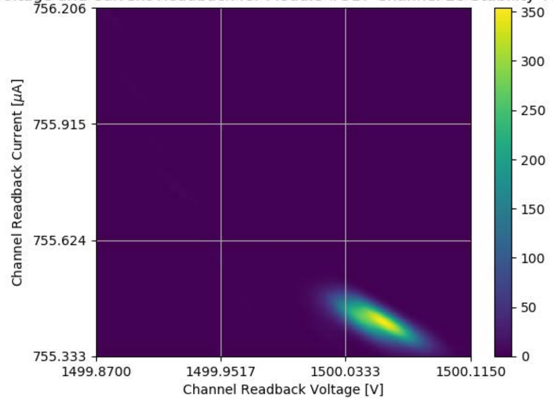
Voltage and Current Readback for Module #317 Channel 28 Stability Test
