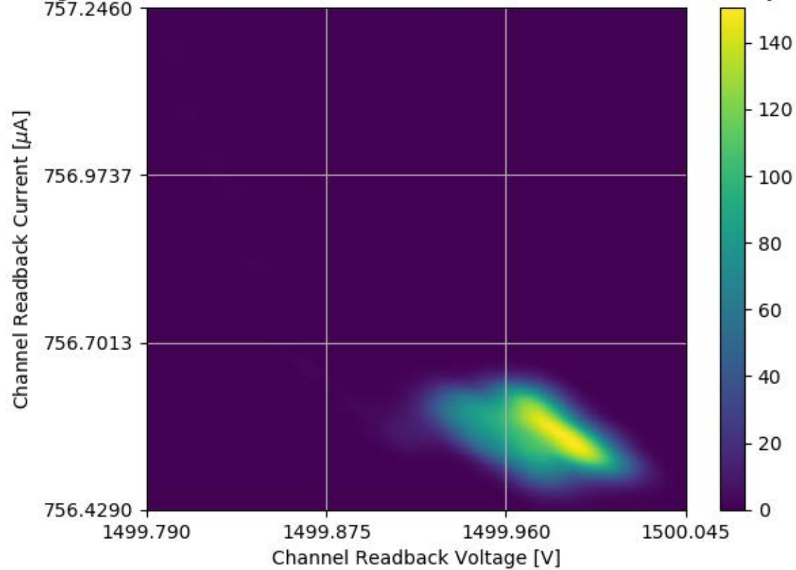
Voltage and Current Readback for Module #317 Channel 34 Stability Test
