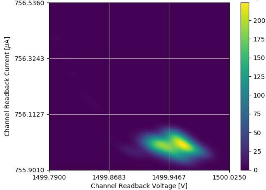
Voltage and Current Readback for Module #317 Channel 31 Stability Test
