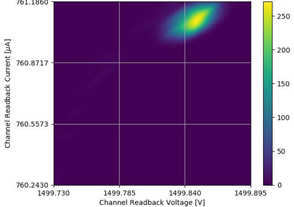
Voltage and Current Readback for Module #324 Channel 09 Stability Test
