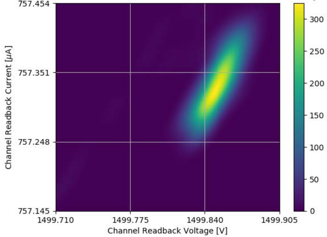
Voltage and Current Readback for Module #324 Channel 04 Stability Test
