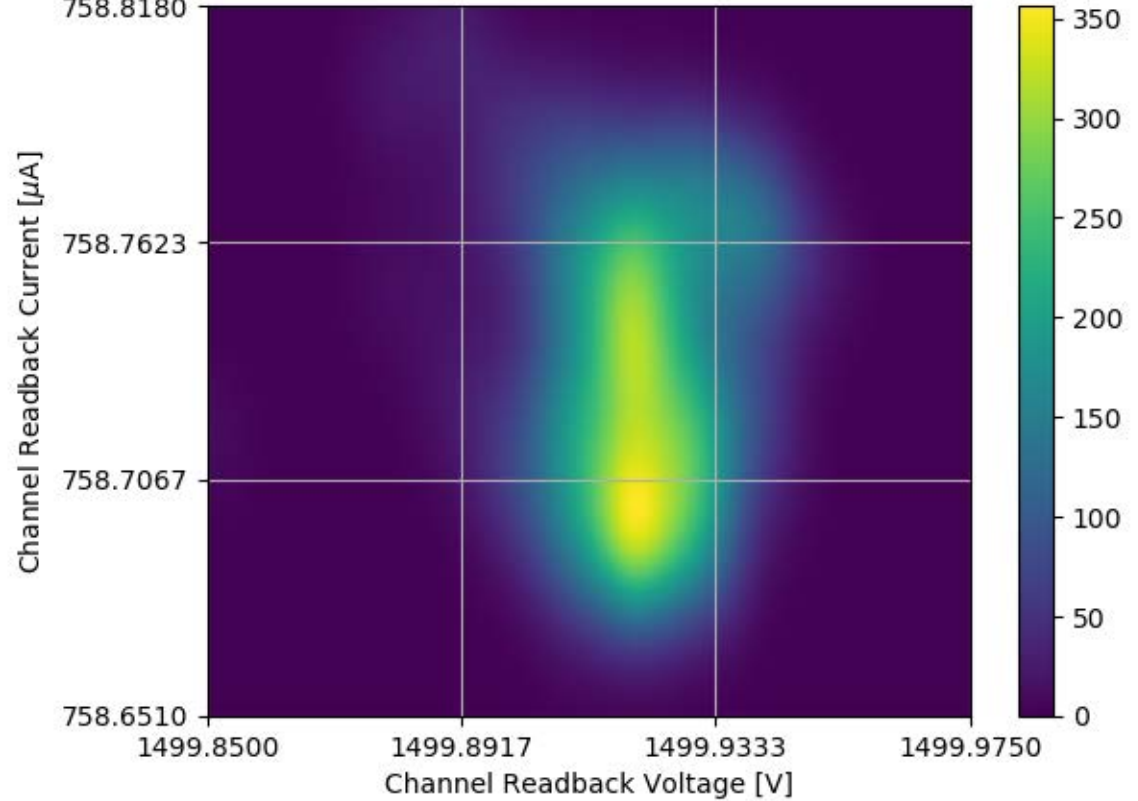
Voltage and Current Readback for Module #324 Channel 12 Stability Test
