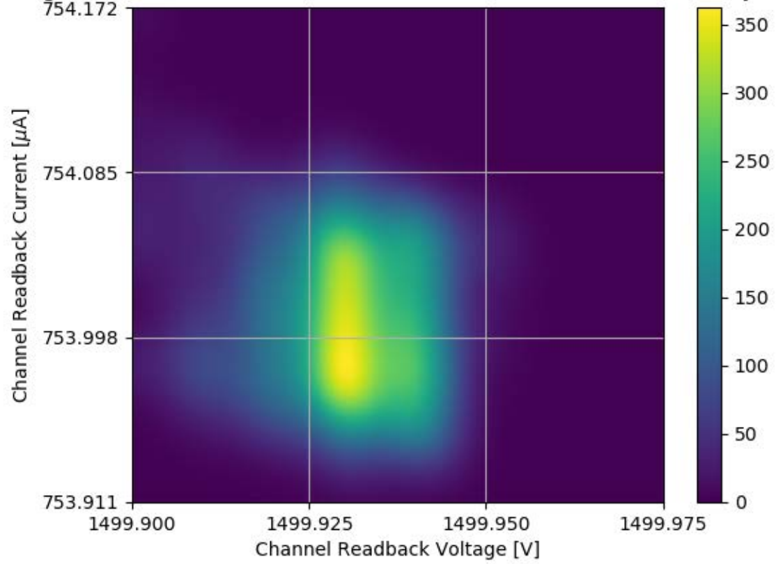
Voltage and Current Readback for Module #324 Channel 13 Stability Test
