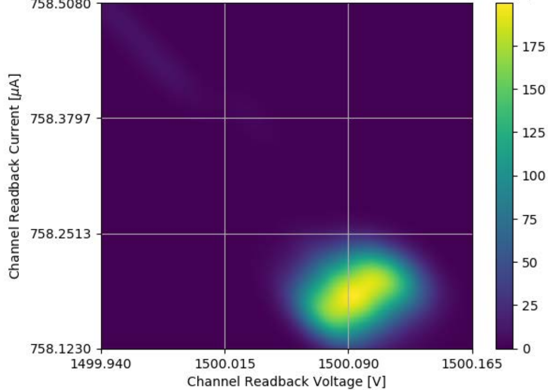
Voltage and Current Readback for Module #324 Channel 29 Stability Test
