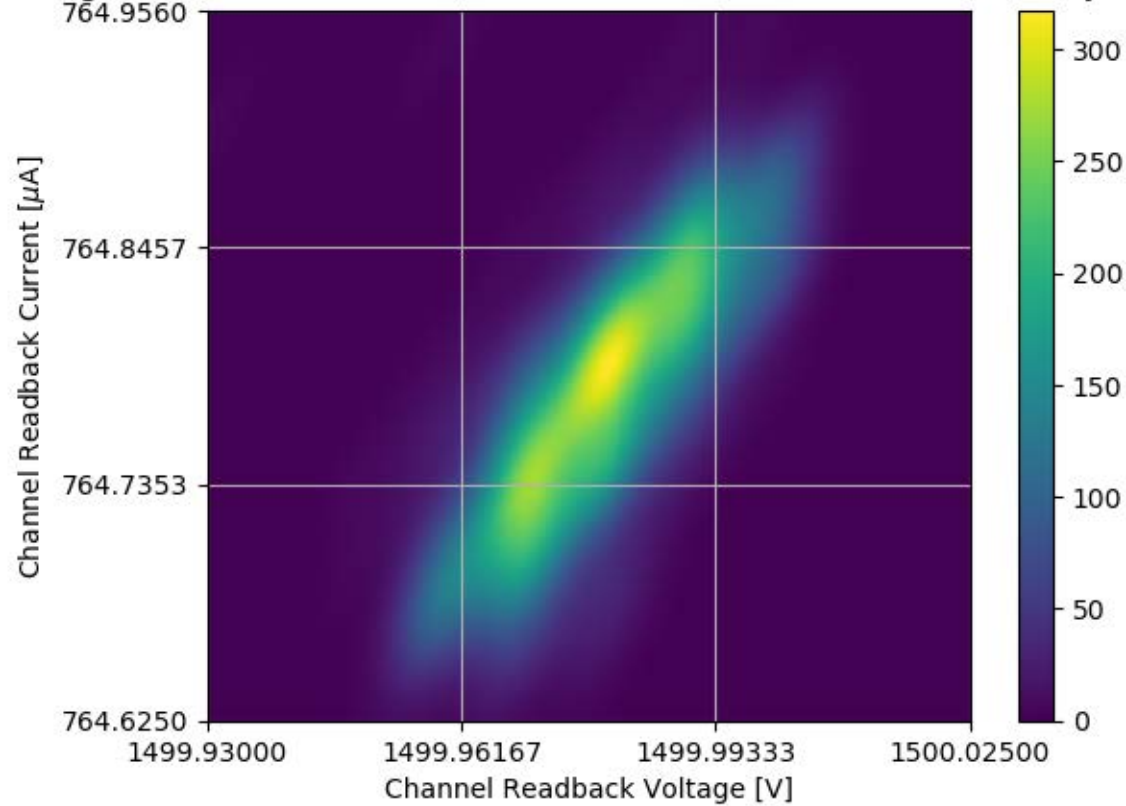
Voltage and Current Readback for Module #324 Channel 17 Stability Test
