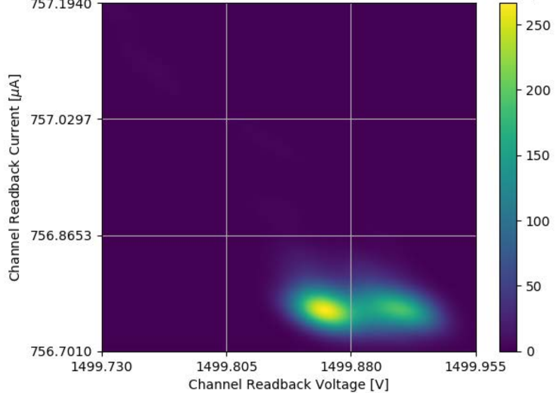
Voltage and Current Readback for Module #324 Channel 34 Stability Test
