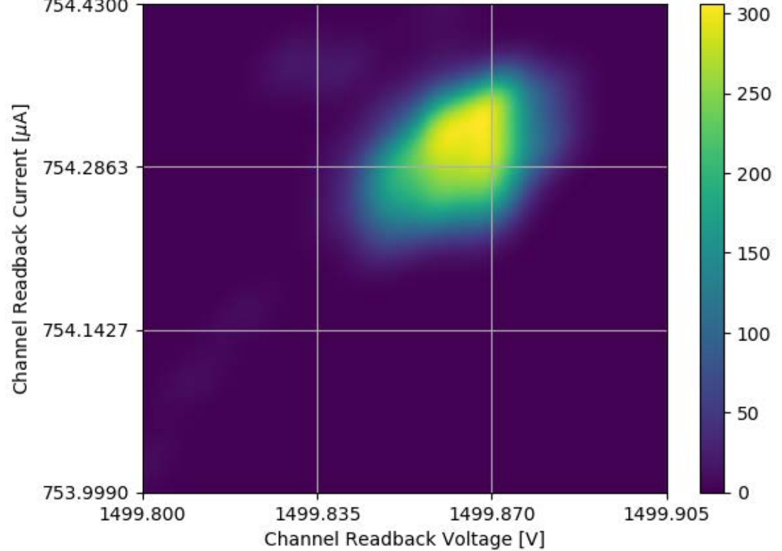
Voltage and Current Readback for Module #324 Channel 30 Stability Test
