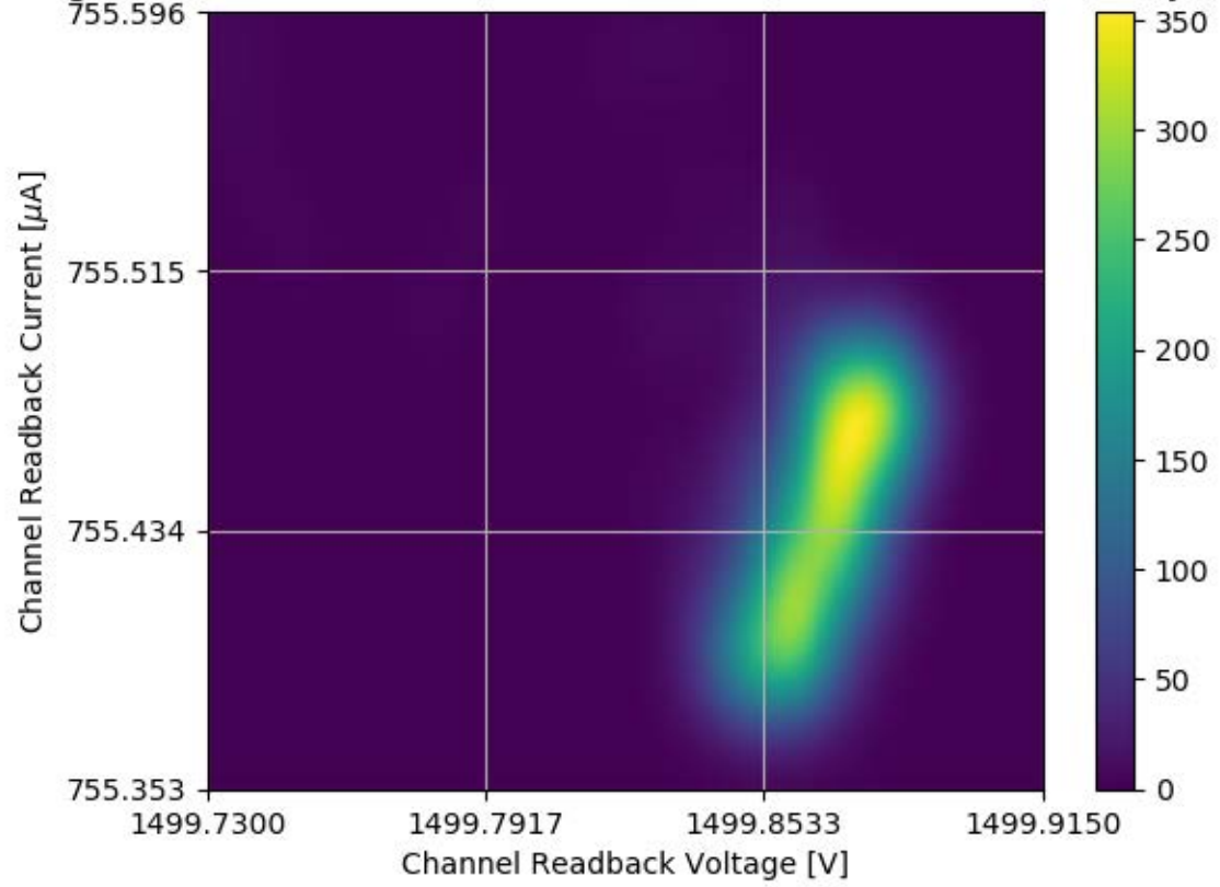
Voltage and Current Readback for Module #324 Channel 03 Stability Test
