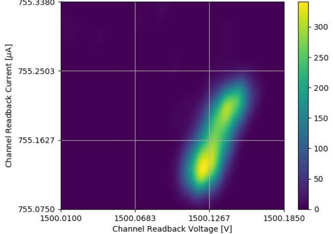
Voltage and Current Readback for Module #324 Channel 28 Stability Test
