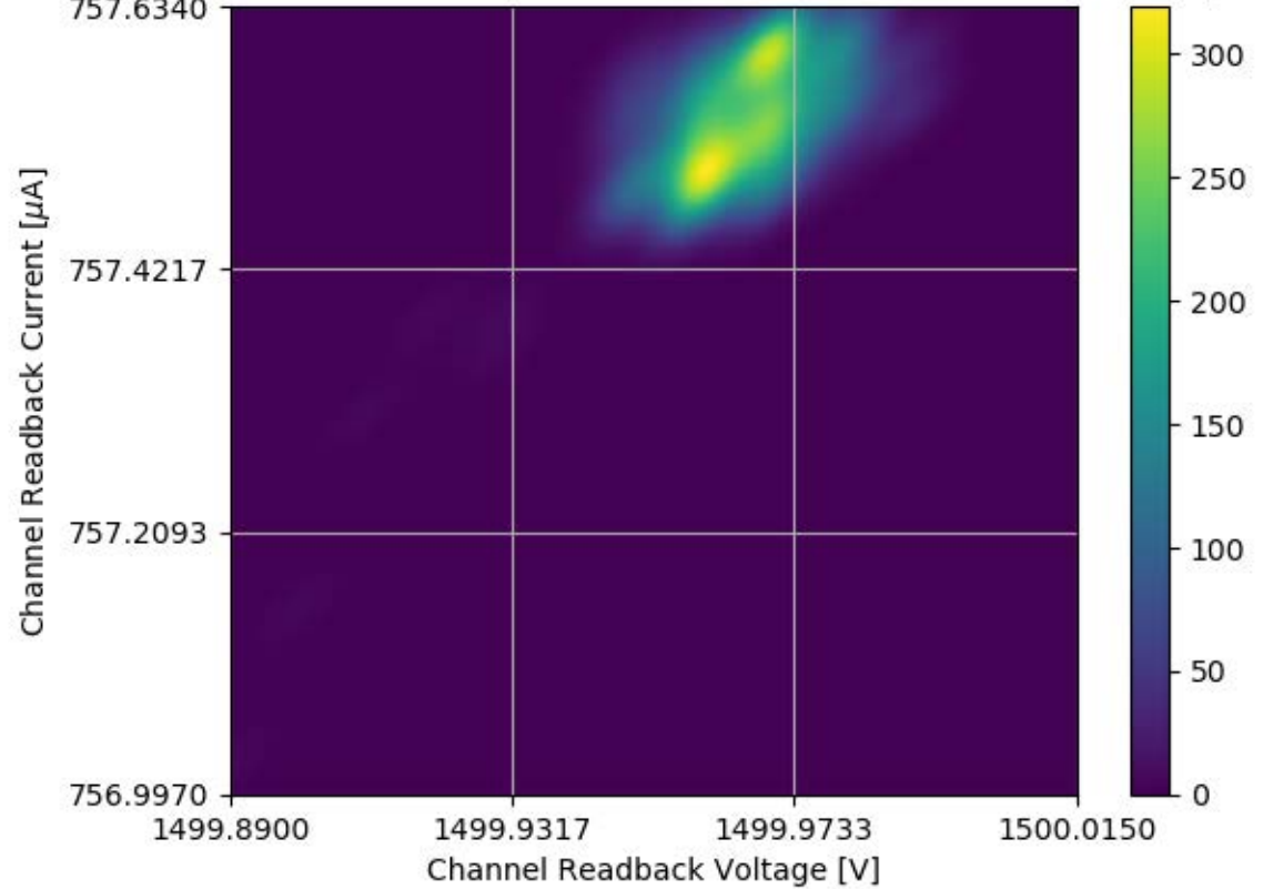
Voltage and Current Readback for Module #324 Channel 26 Stability Test
