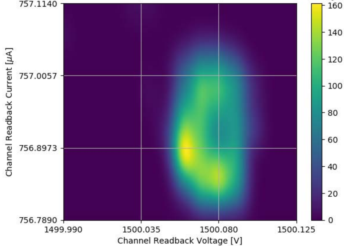
Voltage and Current Readback for Module #324 Channel 21 Stability Test
