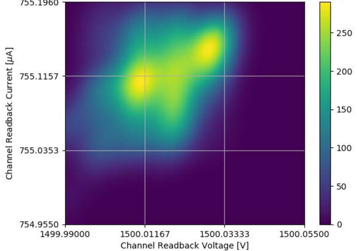
Voltage and Current Readback for Module #324 Channel 18 Stability Test
