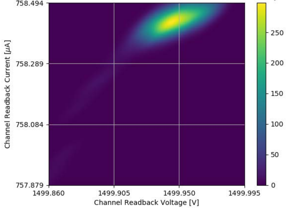
Voltage and Current Readback for Module #324 Channel 10 Stability Test
