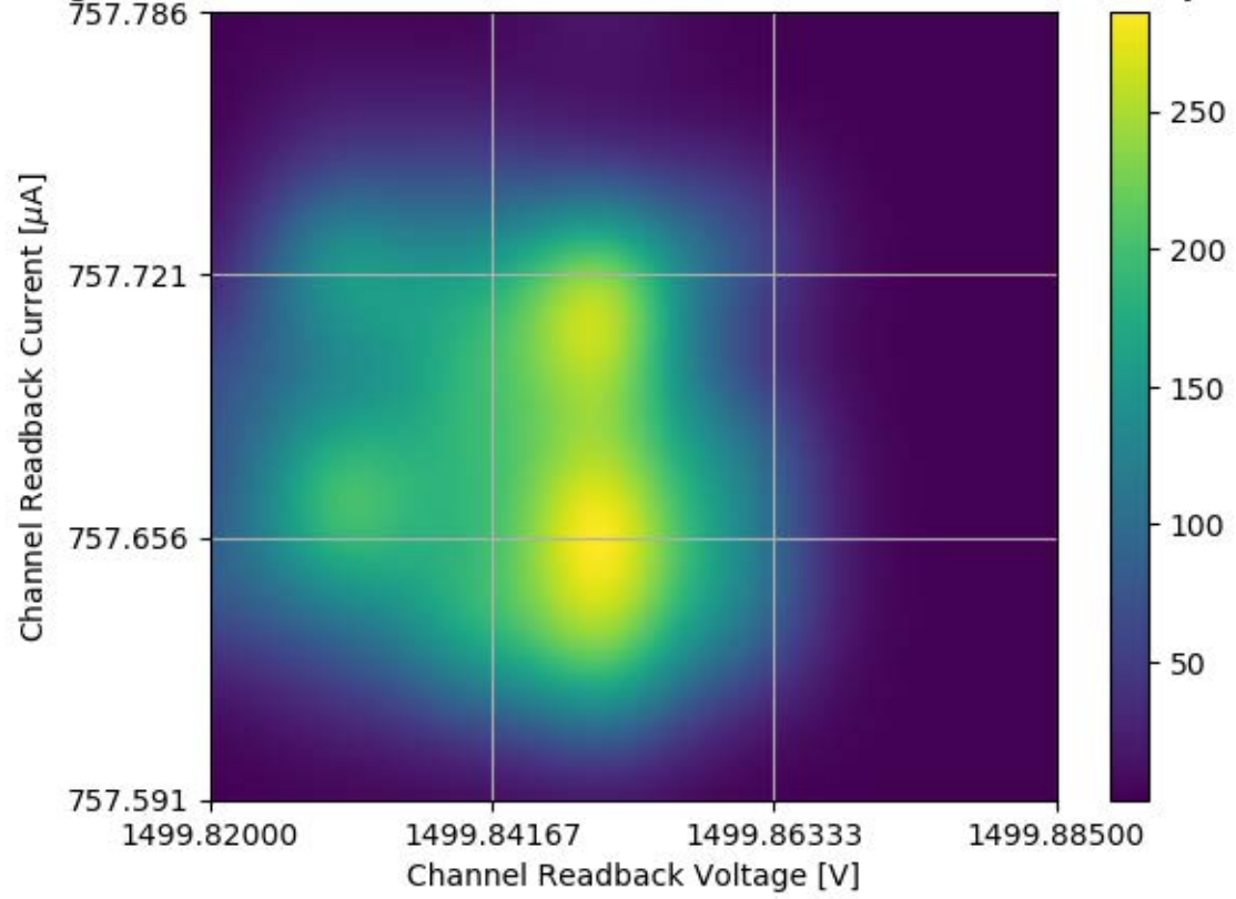
Voltage and Current Readback for Module #324 Channel 20 Stability Test
