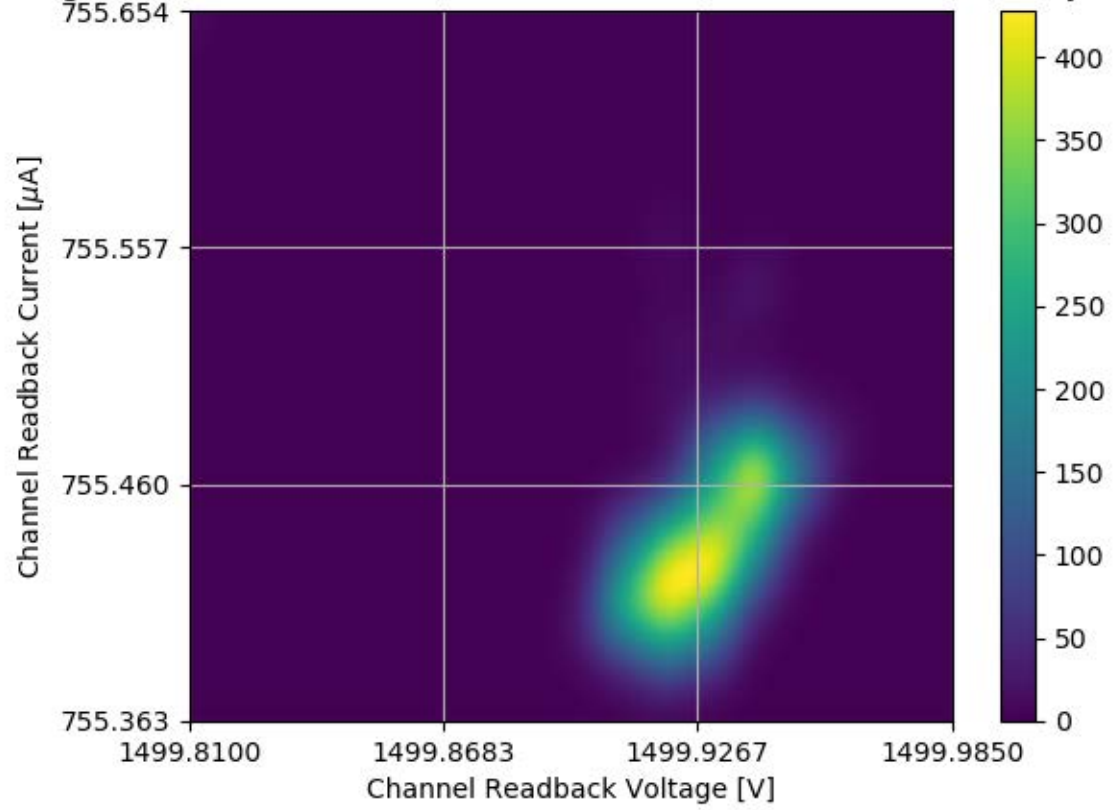
Voltage and Current Readback for Module #324 Channel 02 Stability Test
