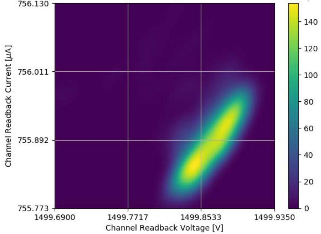
Voltage and Current Readback for Module #324 Channel 32 Stability Test
