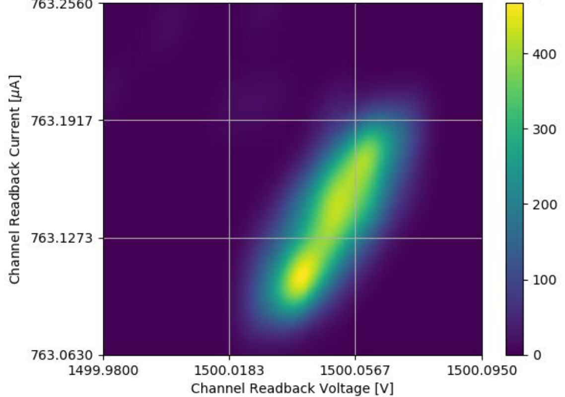
Voltage and Current Readback for Module #324 Channel 11 Stability Test
