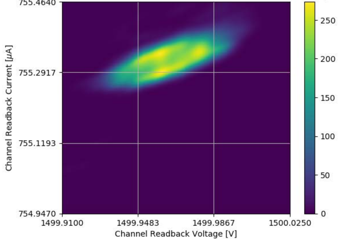
Voltage and Current Readback for Module #325 Channel 31 Stability Test
