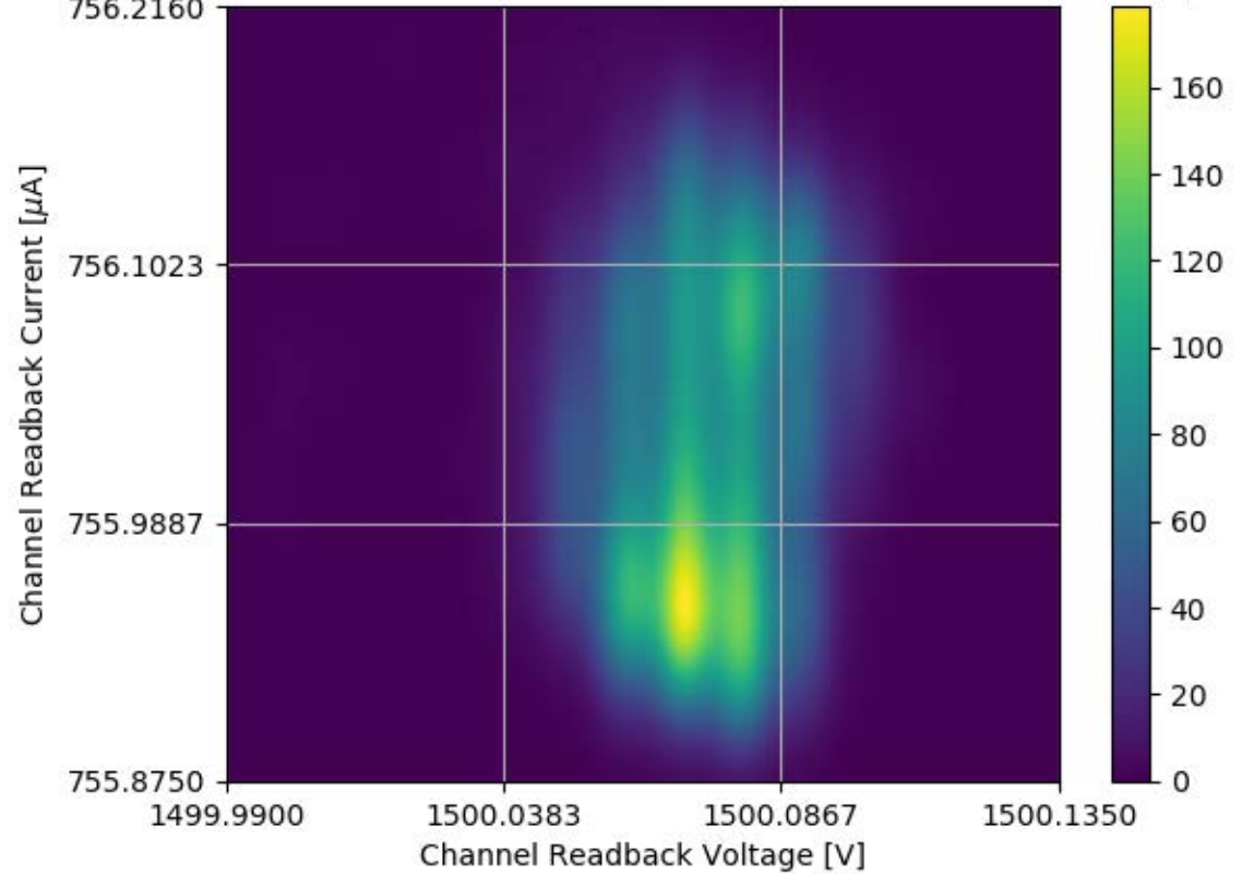
Voltage and Current Readback for Module #325 Channel 23 Stability Test
