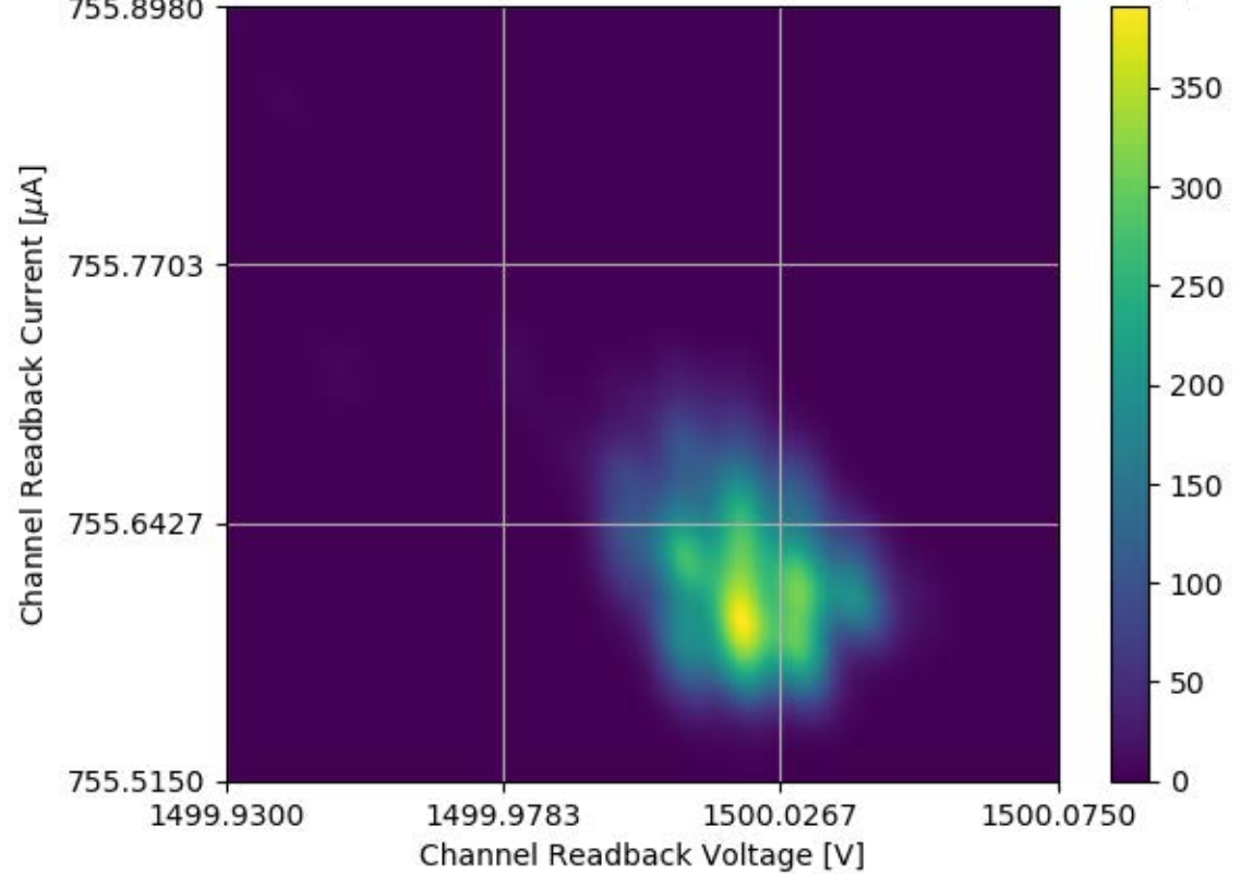
Voltage and Current Readback for Module #325 Channel 02 Stability Test
