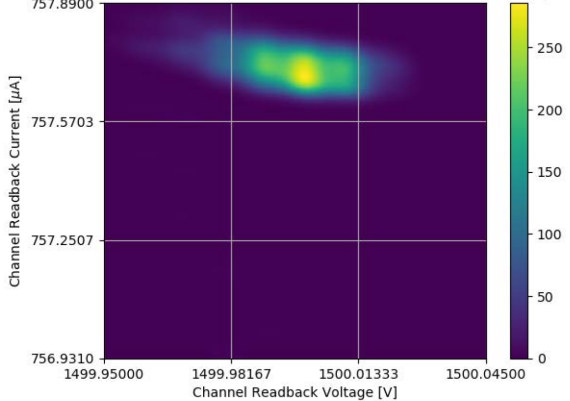
Voltage and Current Readback for Module #325 Channel 26 Stability Test
