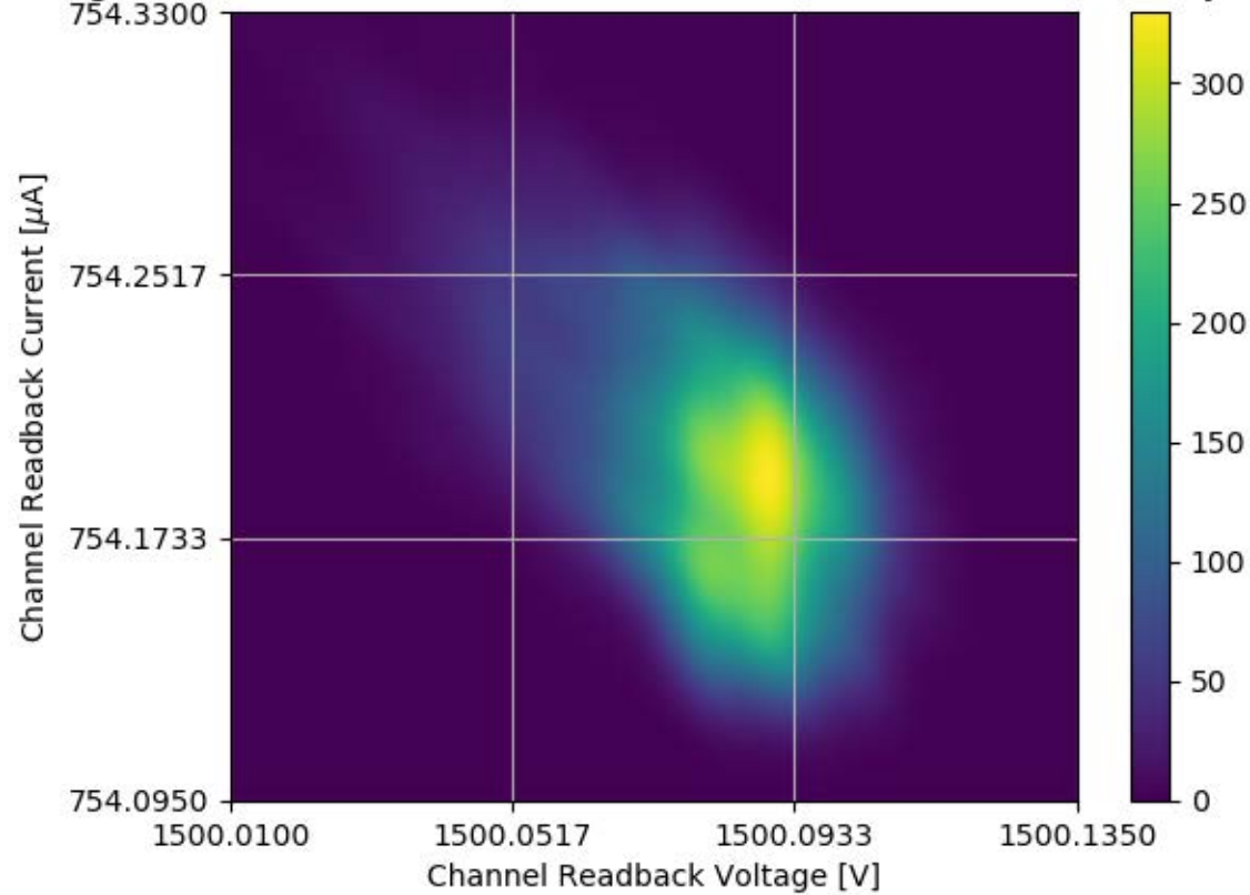
Voltage and Current Readback for Module #325 Channel 13 Stability Test
