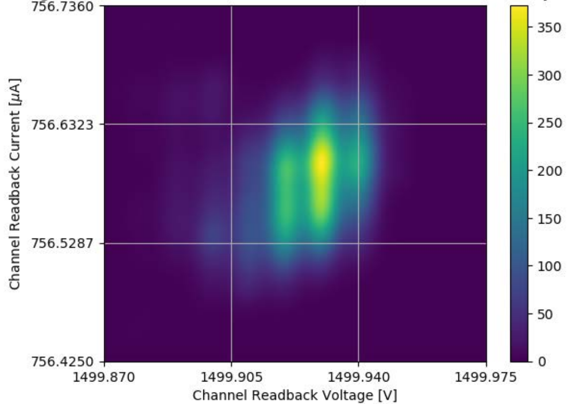
Voltage and Current Readback for Module #325 Channel 21 Stability Test
