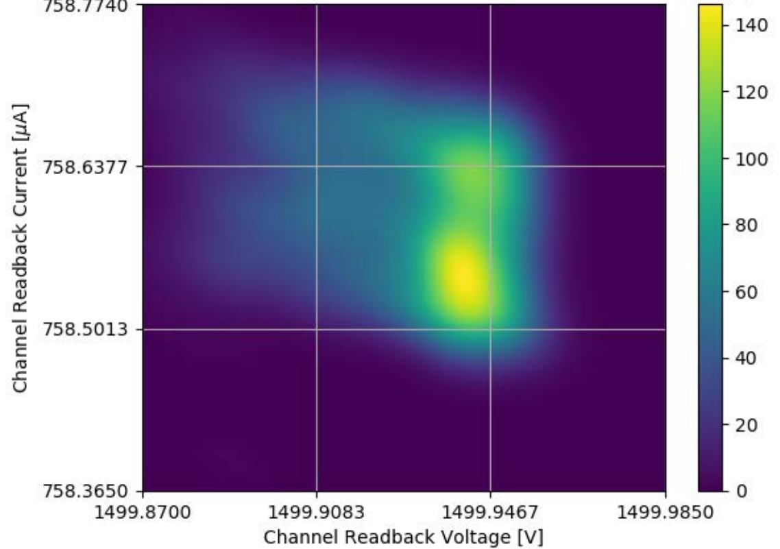
Voltage and Current Readback for Module #325 Channel 25 Stability Test
