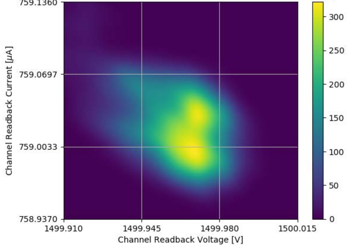
Voltage and Current Readback for Module #325 Channel 12 Stability Test
