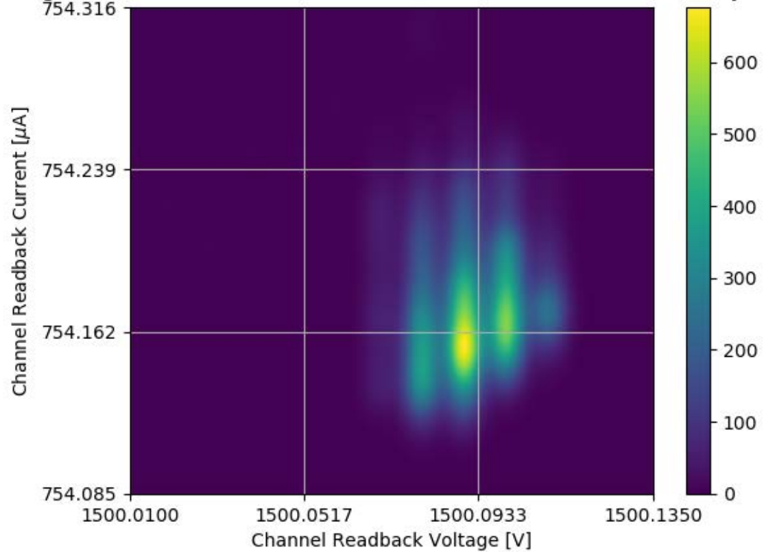
Voltage and Current Readback for Module #325 Channel 00 Stability Test
