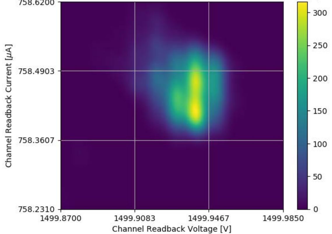
Voltage and Current Readback for Module #325 Channel 04 Stability Test
