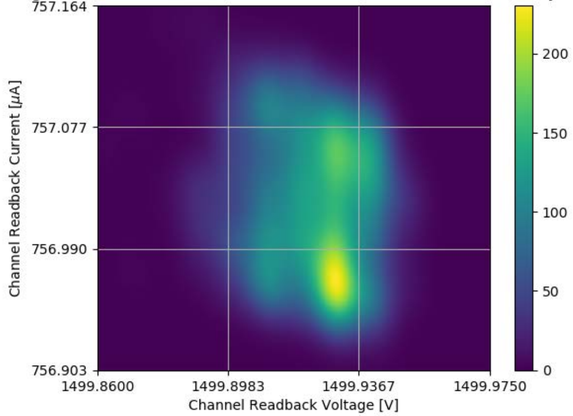
Voltage and Current Readback for Module #325 Channel 29 Stability Test
