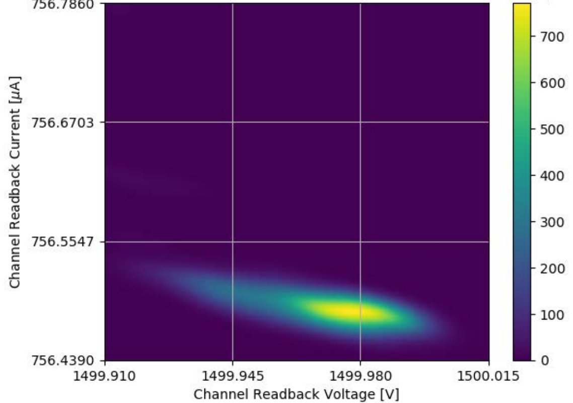
Voltage and Current Readback for Module #325 Channel 15 Stability Test
