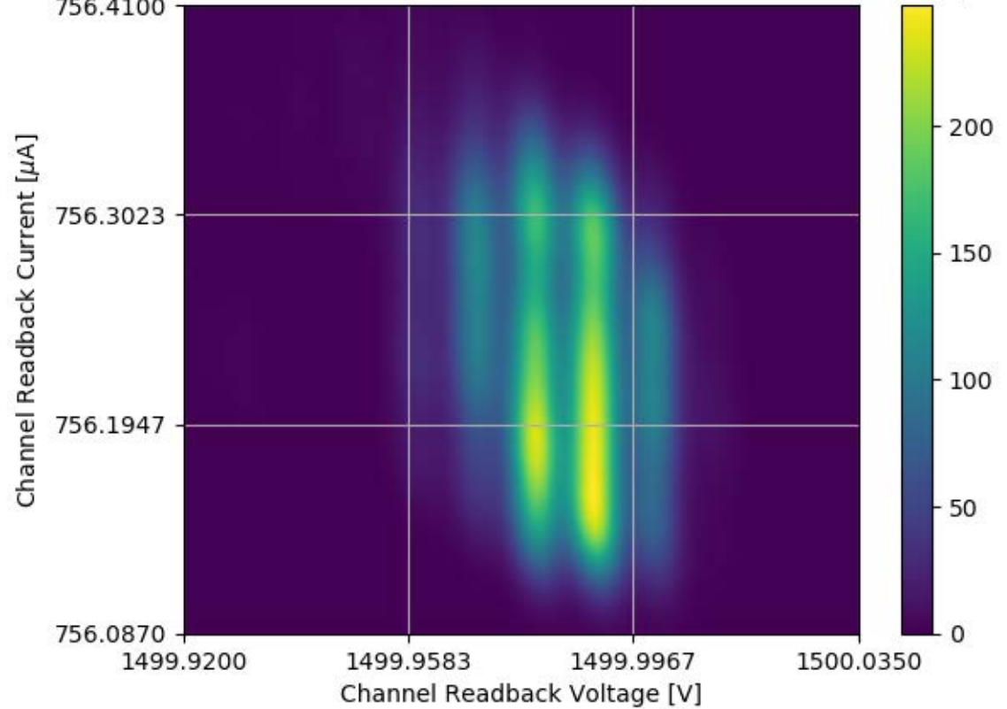
Voltage and Current Readback for Module #325 Channel 27 Stability Test
