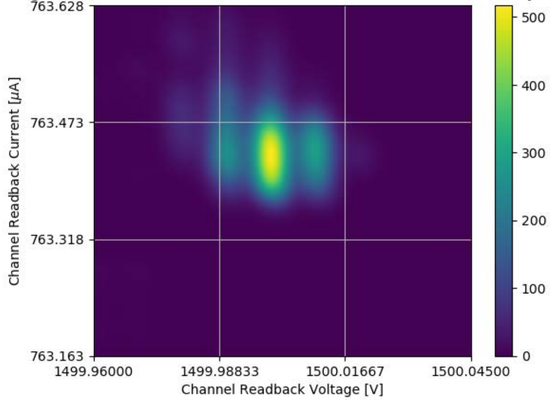
Voltage and Current Readback for Module #325 Channel 09 Stability Test
