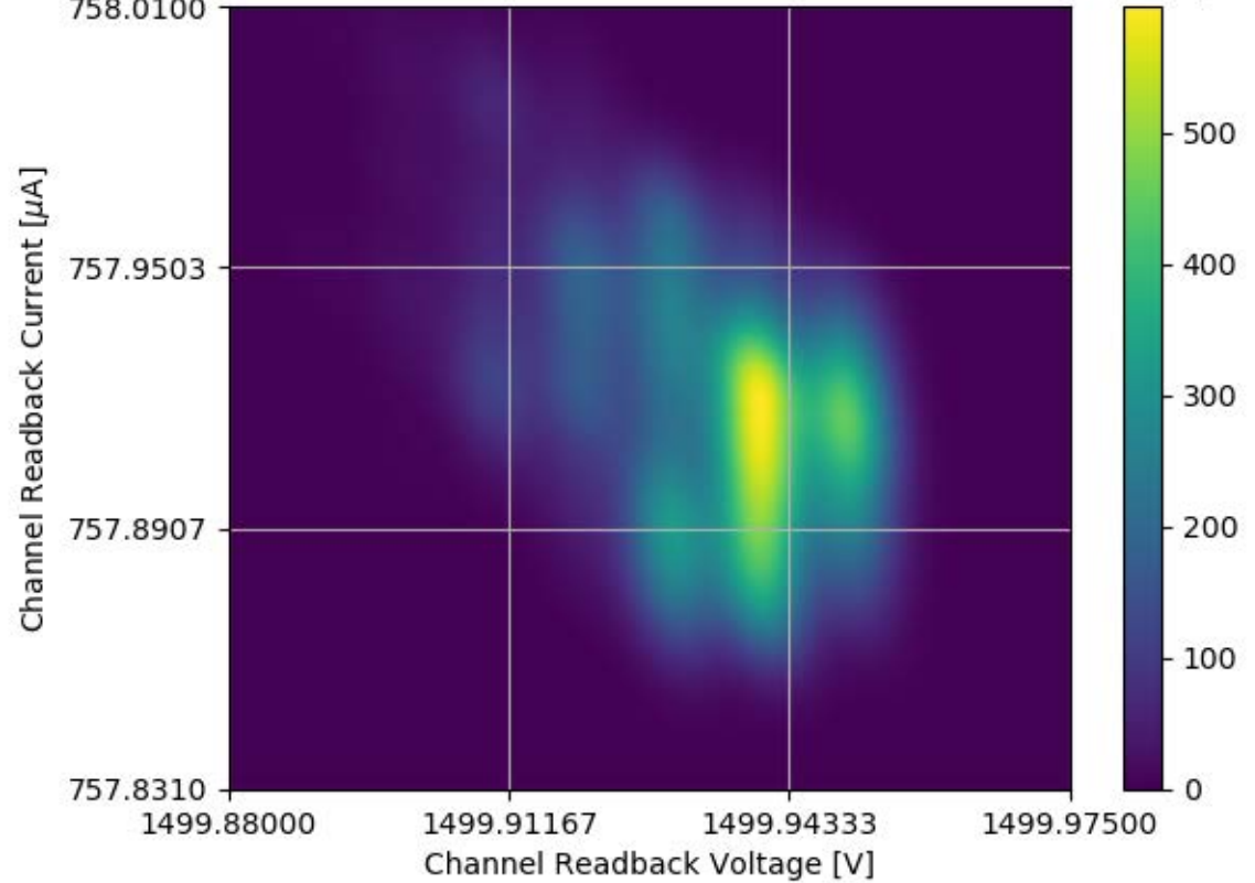
Voltage and Current Readback for Module #325 Channel 06 Stability Test
