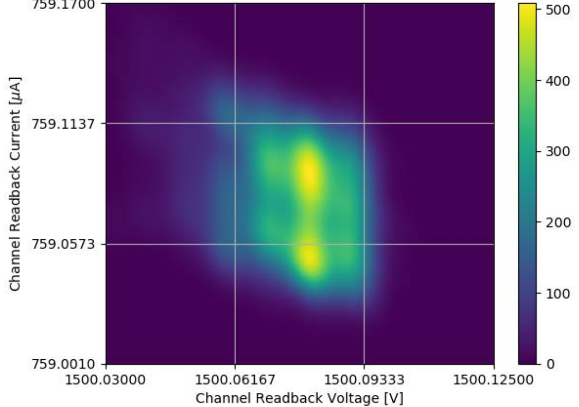
Voltage and Current Readback for Module #325 Channel 05 Stability Test
