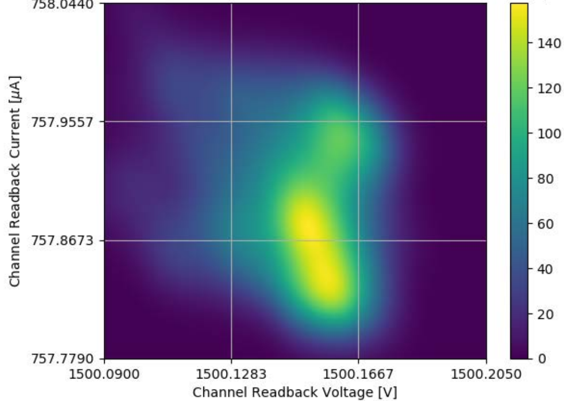
Voltage and Current Readback for Module #325 Channel 35 Stability Test
