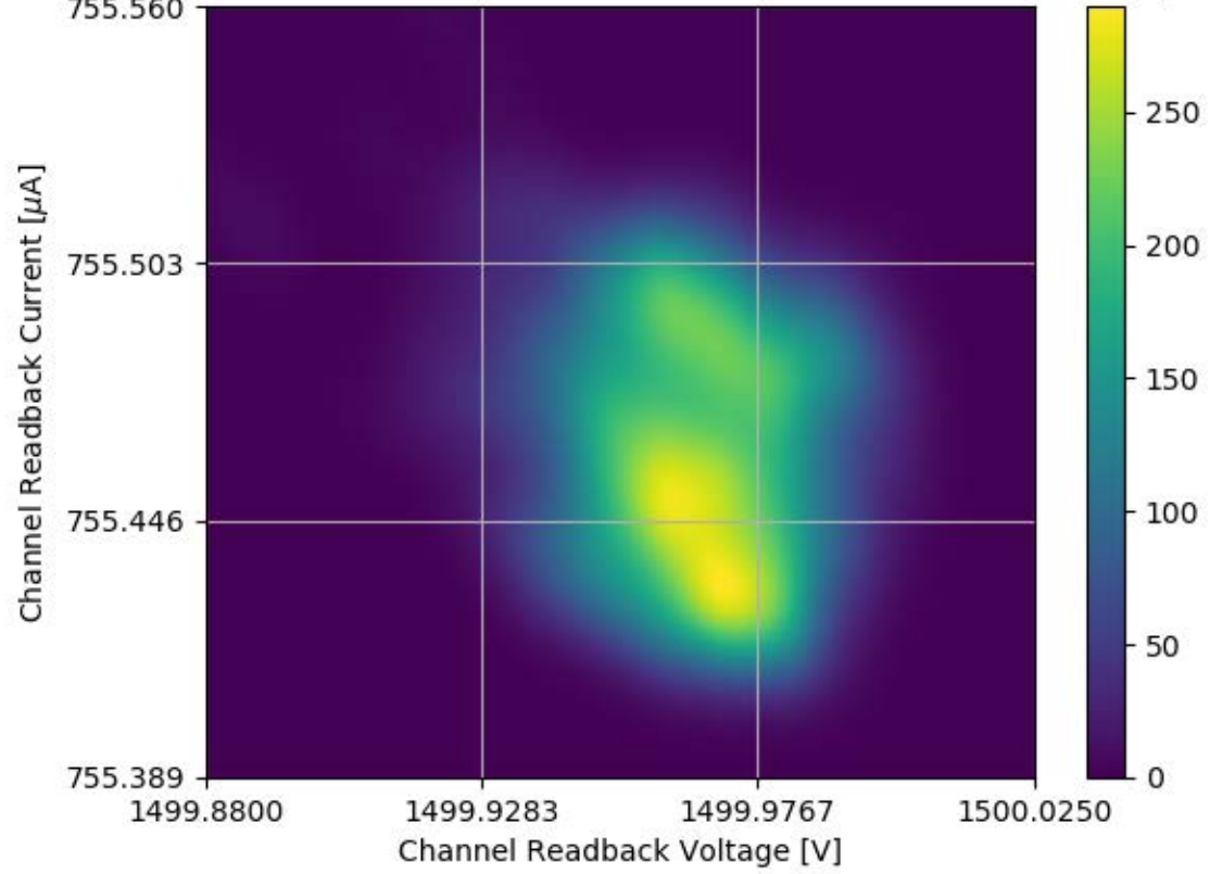
Voltage and Current Readback for Module #325 Channel 30 Stability Test
