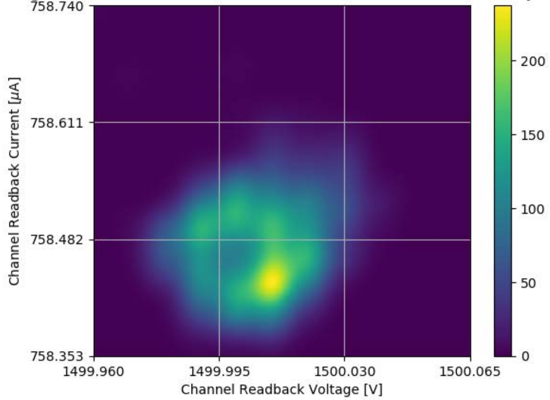
Voltage and Current Readback for Module #325 Channel 22 Stability Test
