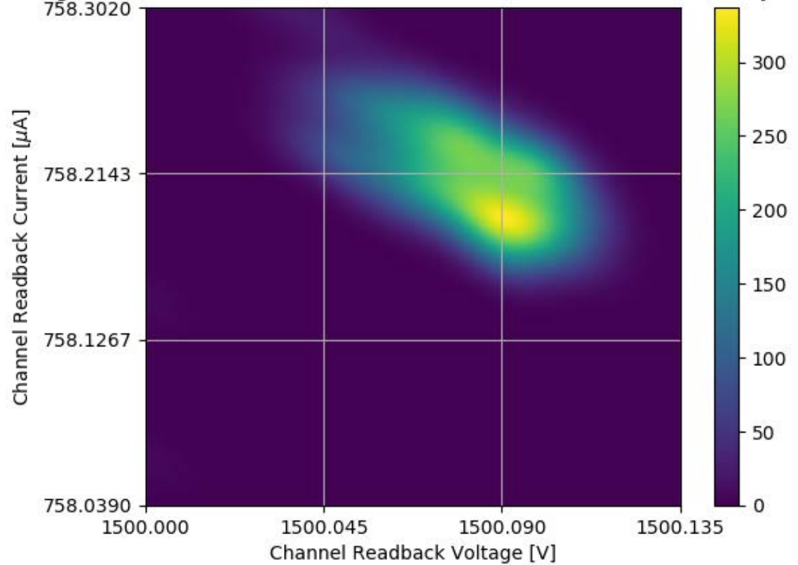
Voltage and Current Readback for Module #325 Channel 08 Stability Test
