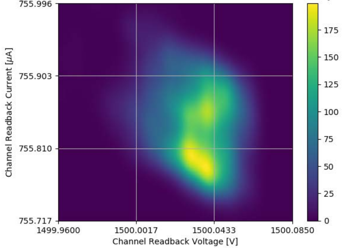
Voltage and Current Readback for Module #325 Channel 28 Stability Test
