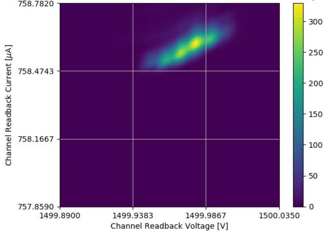
Voltage and Current Readback for Module #325 Channel 10 Stability Test
