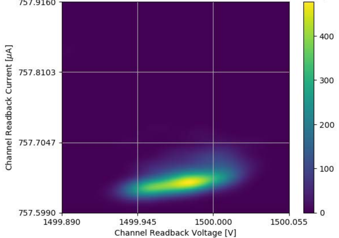
Voltage and Current Readback for Module #325 Channel 20 Stability Test
