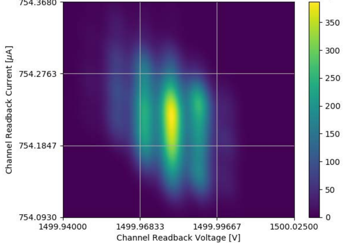
Voltage and Current Readback for Module #325 Channel 33 Stability Test
