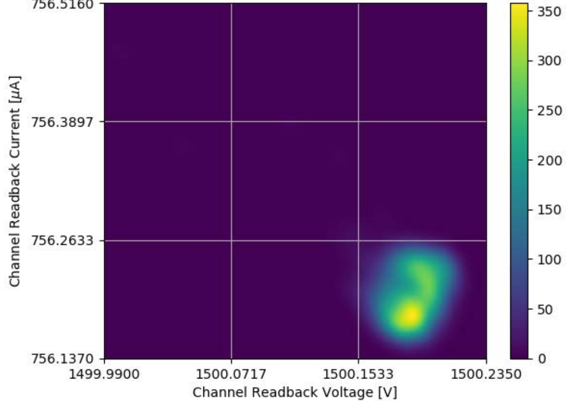
Voltage and Current Readback for Module #326 Channel 31 Stability Test
