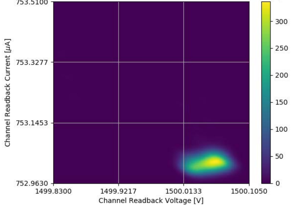
Voltage and Current Readback for Module #326 Channel 11 Stability Test
