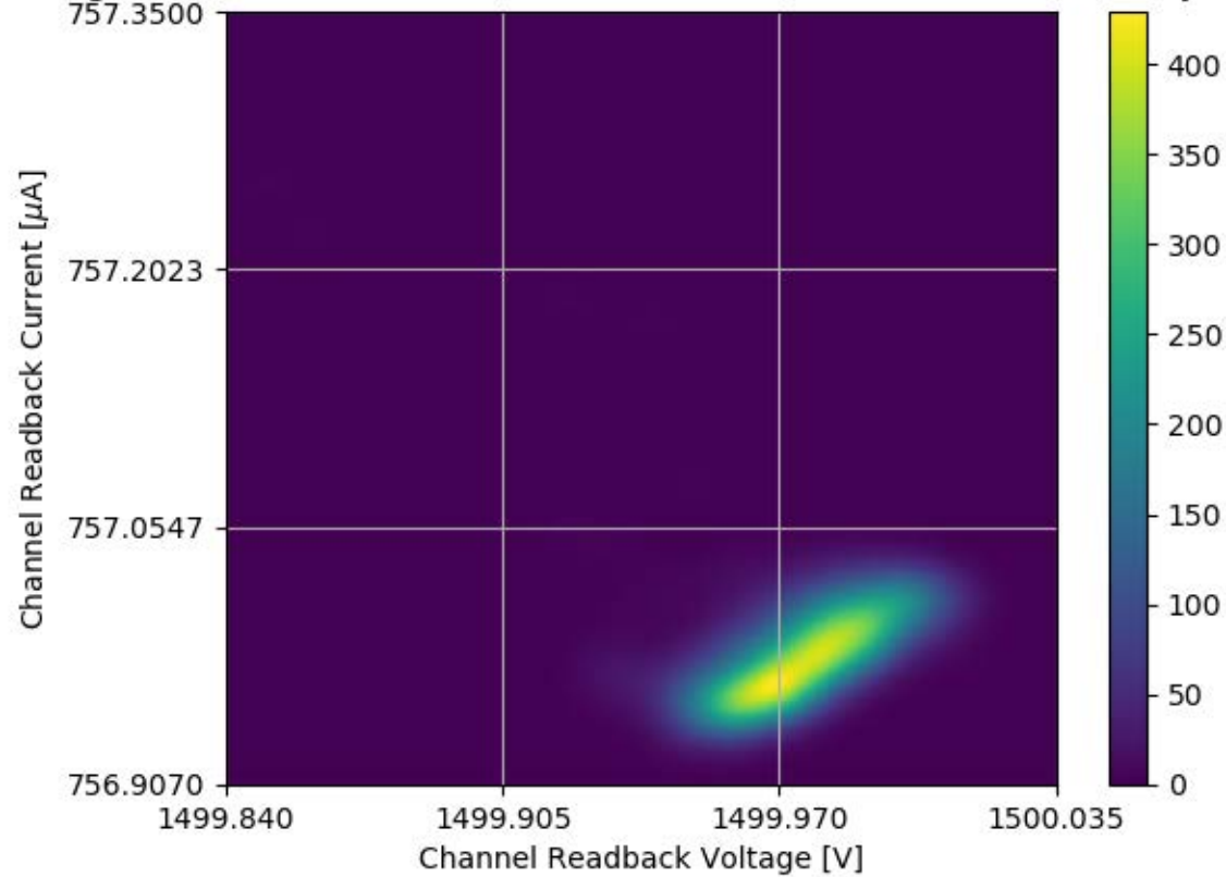
Voltage and Current Readback for Module #326 Channel 35 Stability Test
