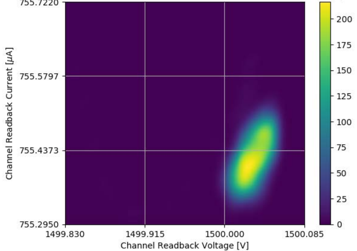
Voltage and Current Readback for Module #326 Channel 18 Stability Test
