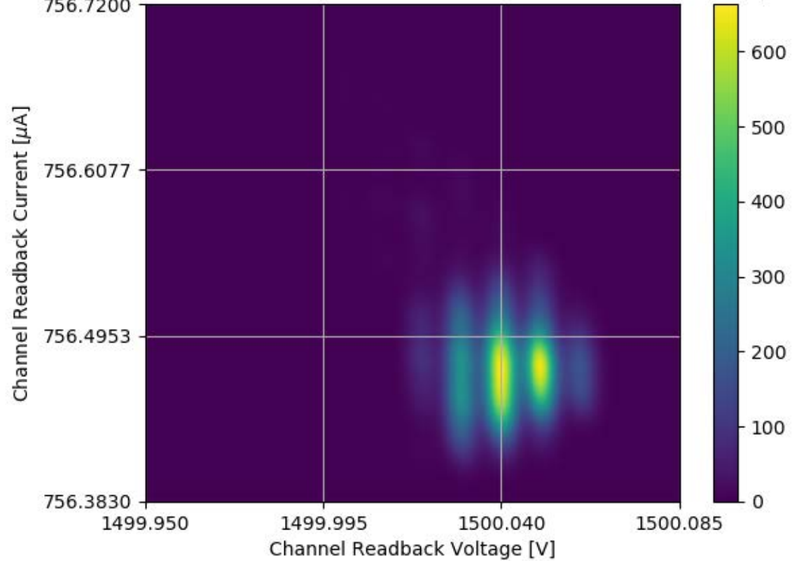
Voltage and Current Readback for Module #326 Channel 14 Stability Test
