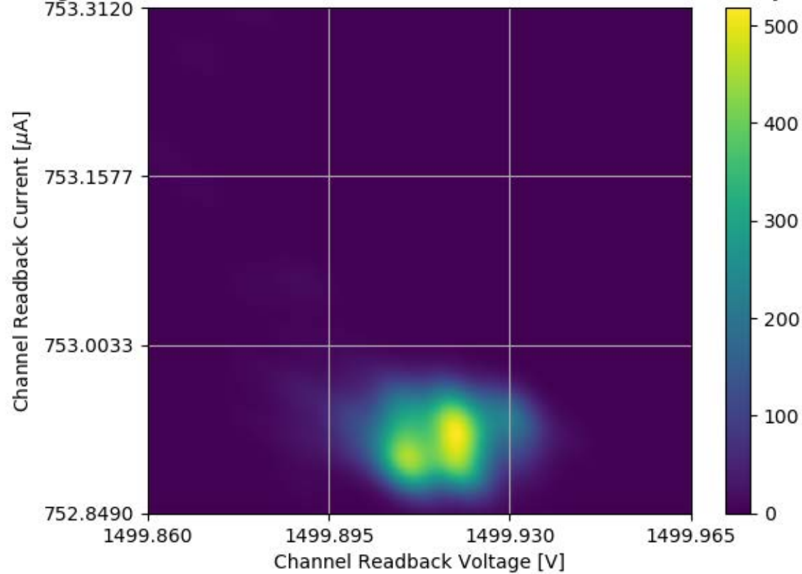
Voltage and Current Readback for Module #326 Channel 33 Stability Test
