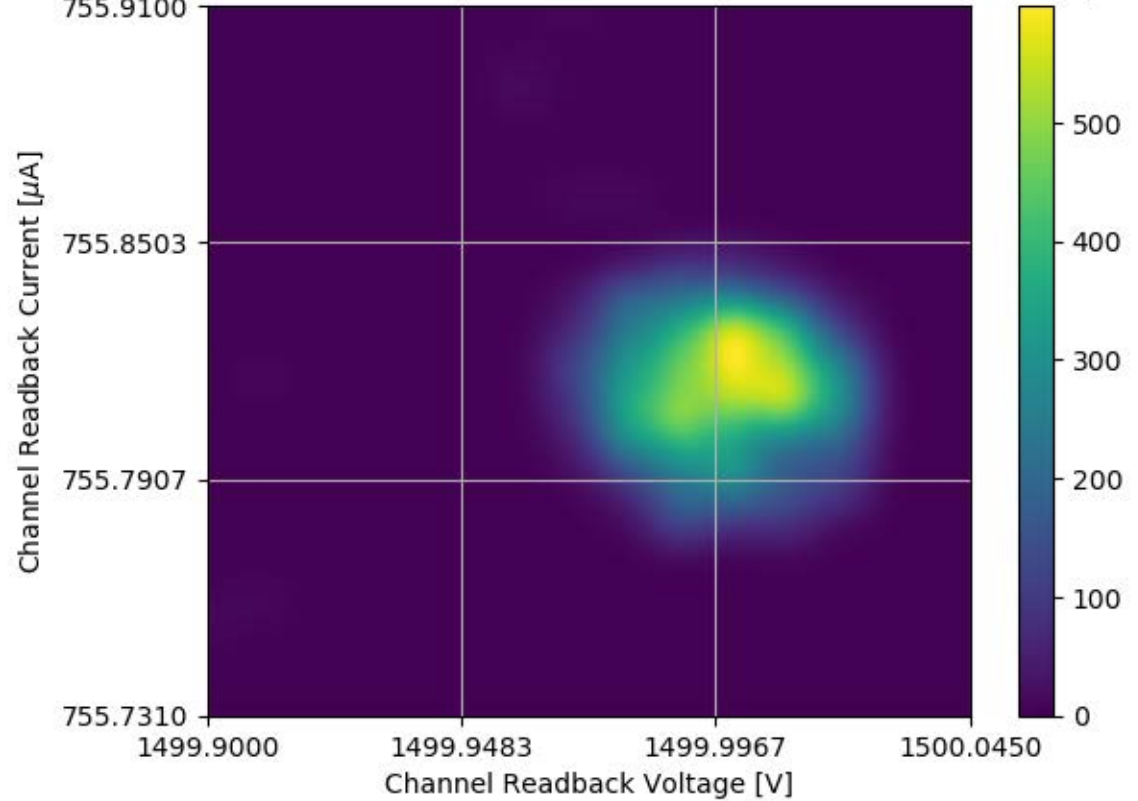
Voltage and Current Readback for Module #326 Channel 07 Stability Test
