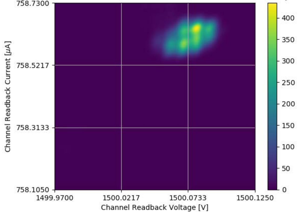
Voltage and Current Readback for Module #326 Channel 12 Stability Test
