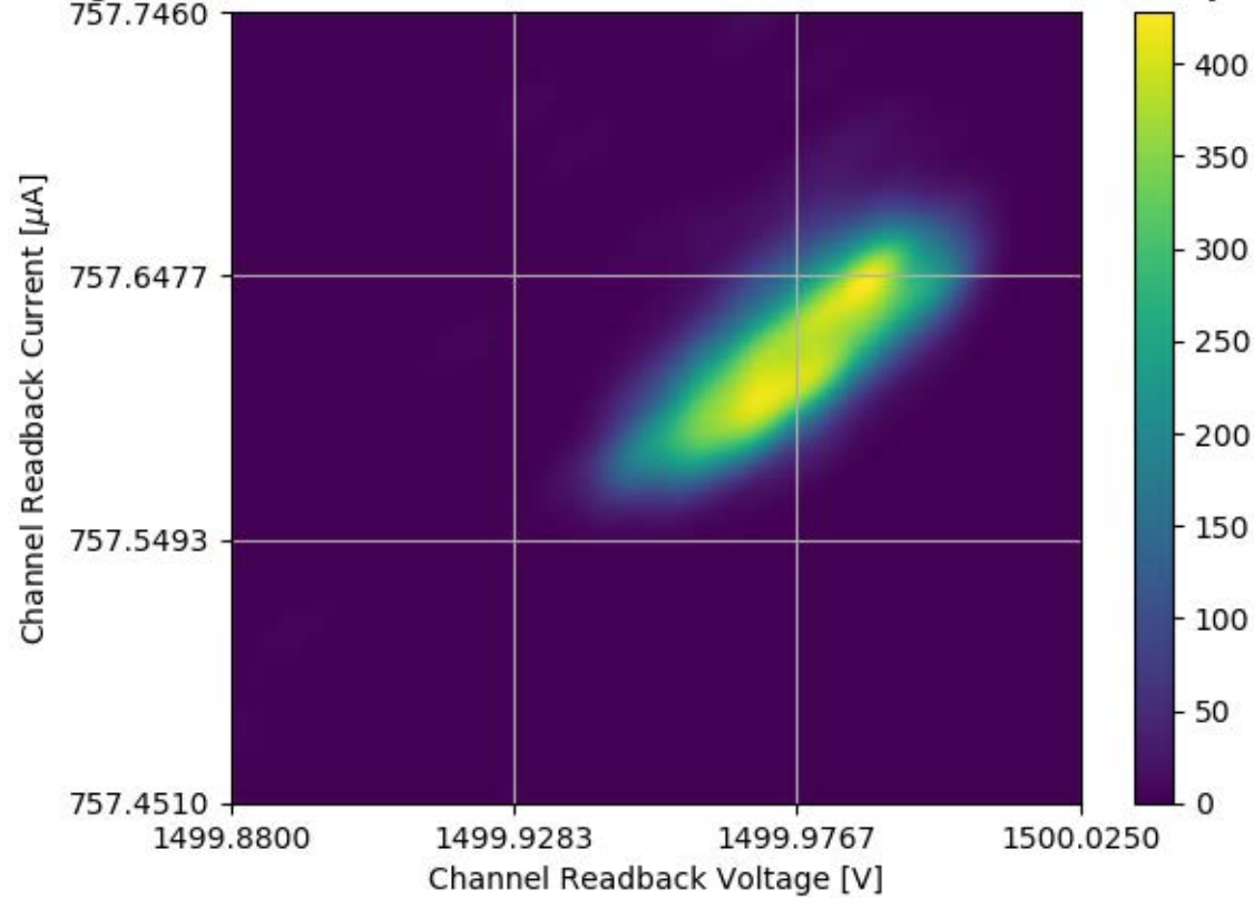
Voltage and Current Readback for Module #326 Channel 06 Stability Test
