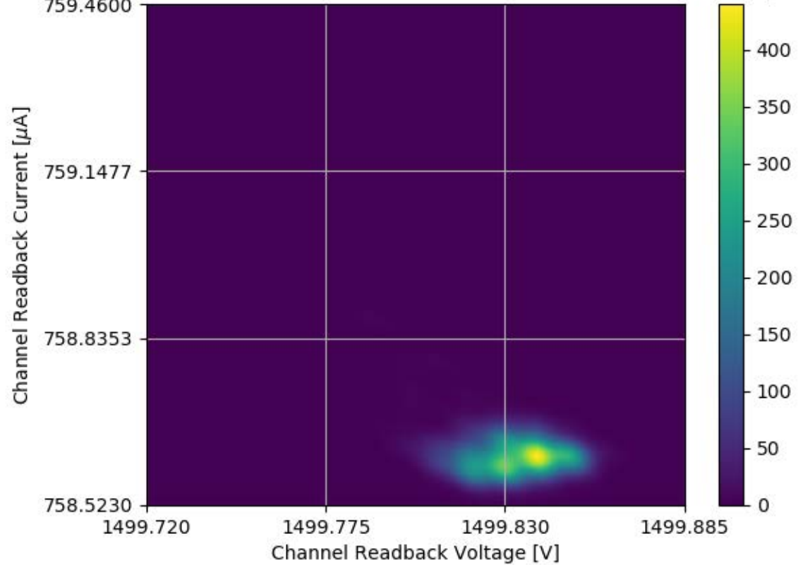
Voltage and Current Readback for Module #326 Channel 05 Stability Test
