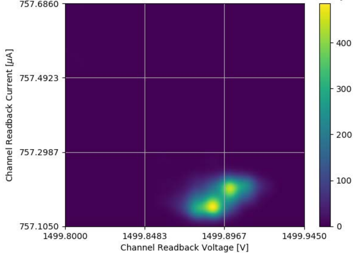
Voltage and Current Readback for Module #326 Channel 21 Stability Test
