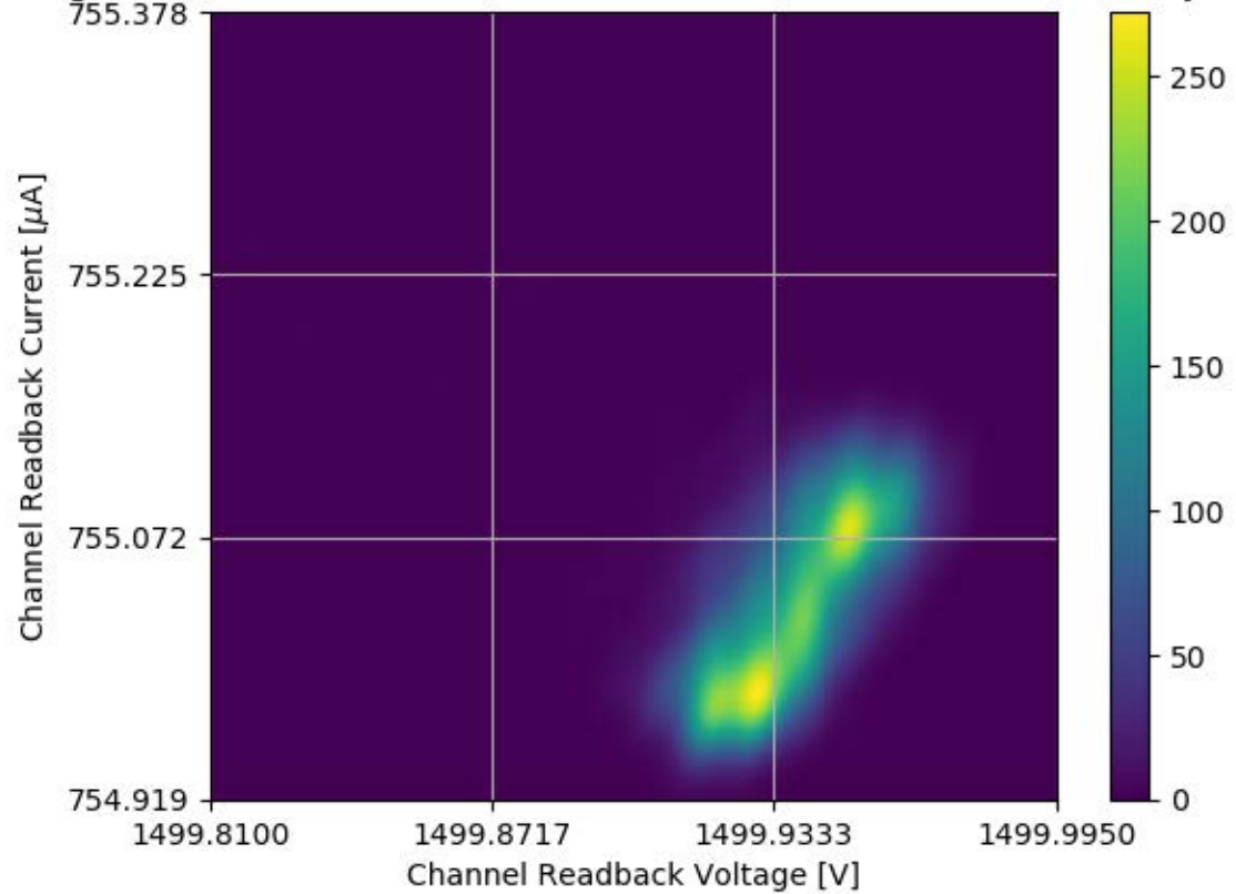
Voltage and Current Readback for Module #326 Channel 28 Stability Test
