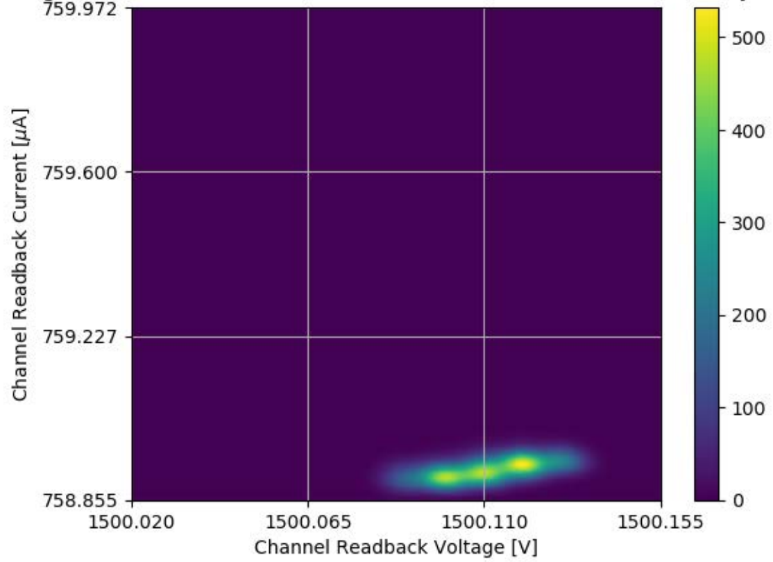
Voltage and Current Readback for Module #326 Channel 22 Stability Test
