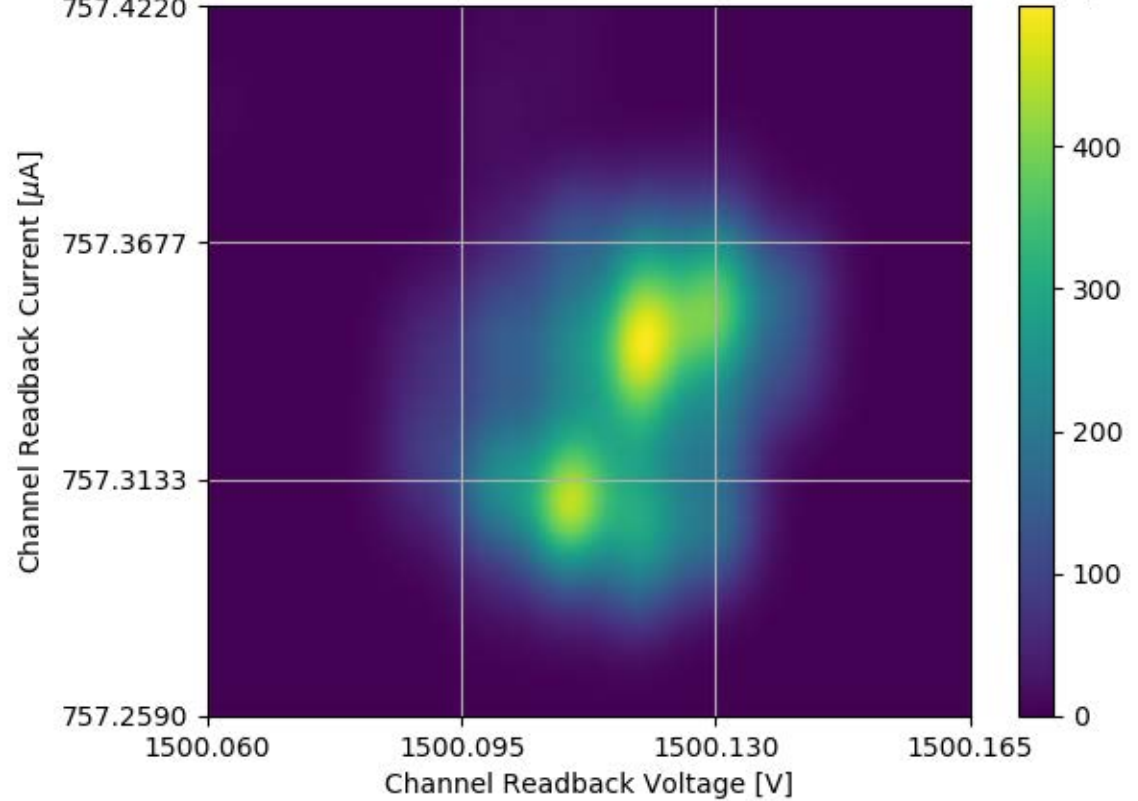
Voltage and Current Readback for Module #326 Channel 32 Stability Test
