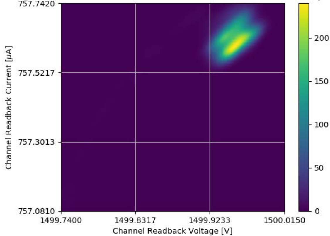
Voltage and Current Readback for Module #326 Channel 08 Stability Test
