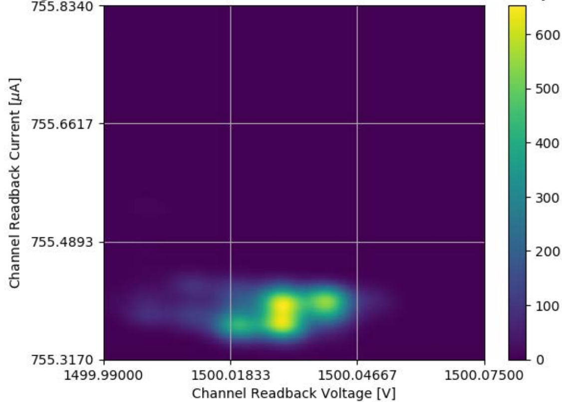
Voltage and Current Readback for Module #326 Channel 17 Stability Test
