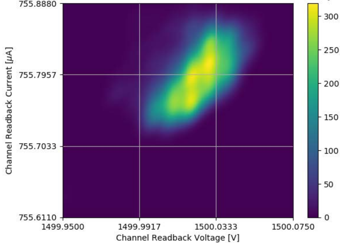
Voltage and Current Readback for Module #326 Channel 15 Stability Test
