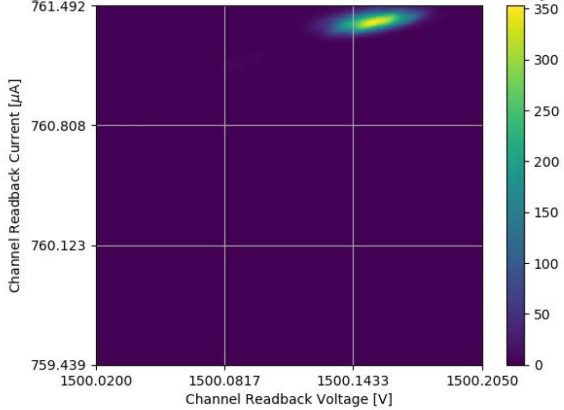
Voltage and Current Readback for Module #326 Channel 09 Stability Test
