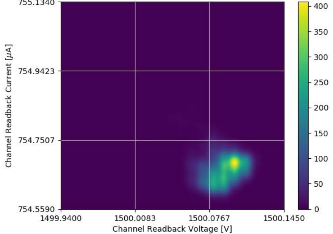
Voltage and Current Readback for Module #326 Channel 03 Stability Test
