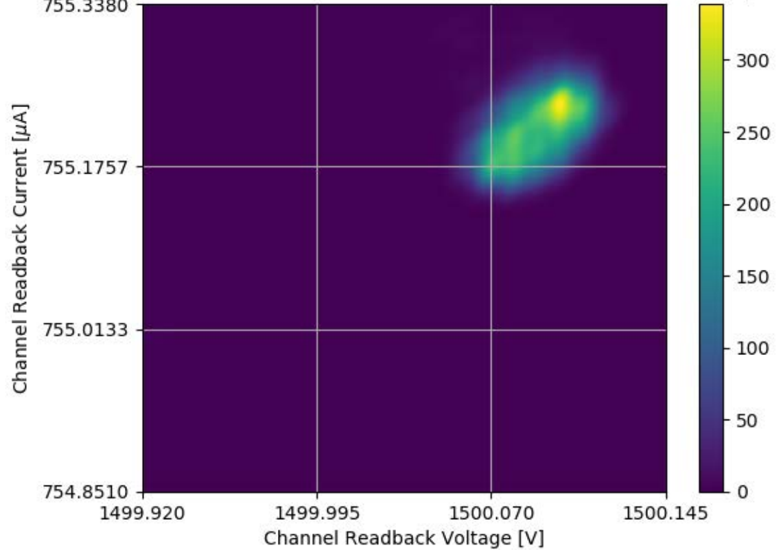
Voltage and Current Readback for Module #326 Channel 02 Stability Test
