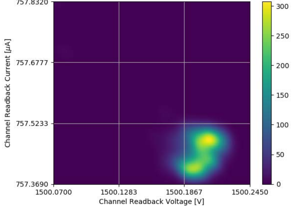
Voltage and Current Readback for Module #326 Channel 29 Stability Test
