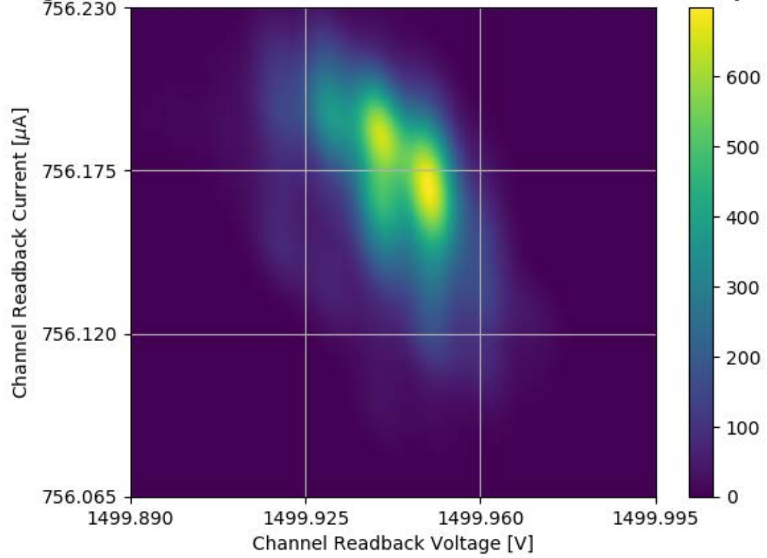
Voltage and Current Readback for Module #327 Channel 15 Stability Test
