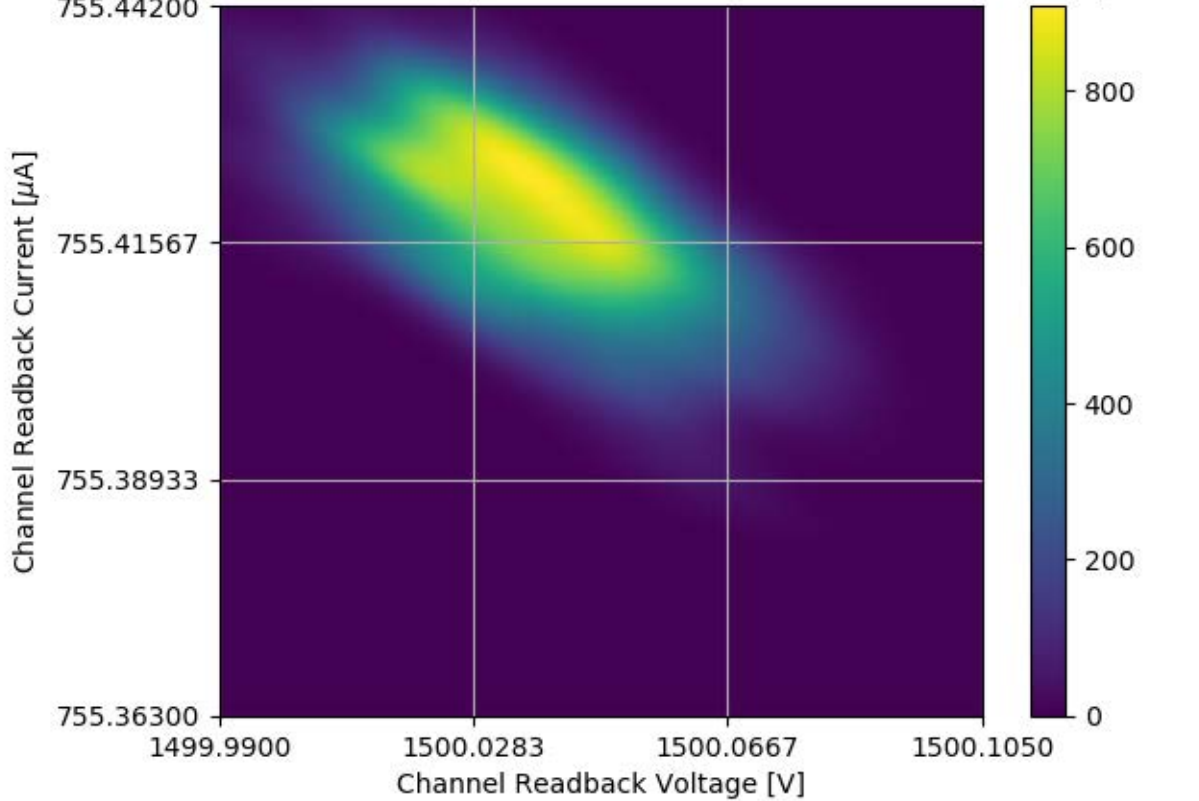
Voltage and Current Readback for Module #327 Channel 28 Stability Test
