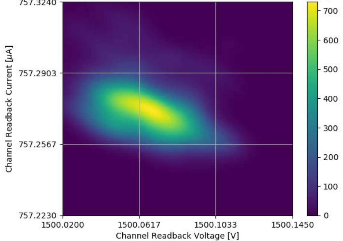
Voltage and Current Readback for Module #327 Channel 35 Stability Test
