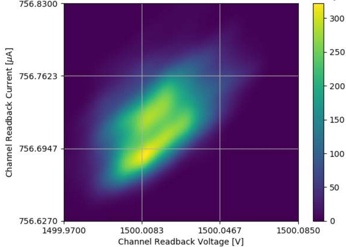
Voltage and Current Readback for Module #327 Channel 26 Stability Test
