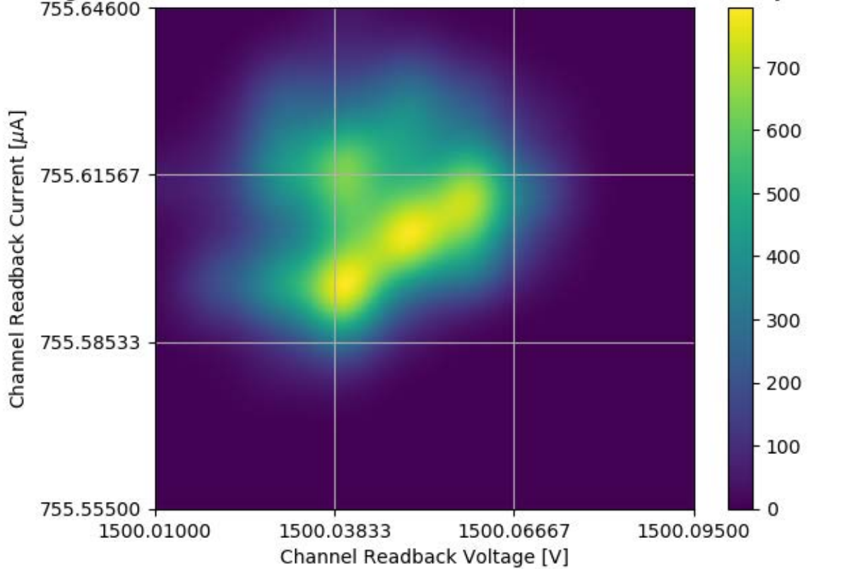
Voltage and Current Readback for Module #327 Channel 31 Stability Test
