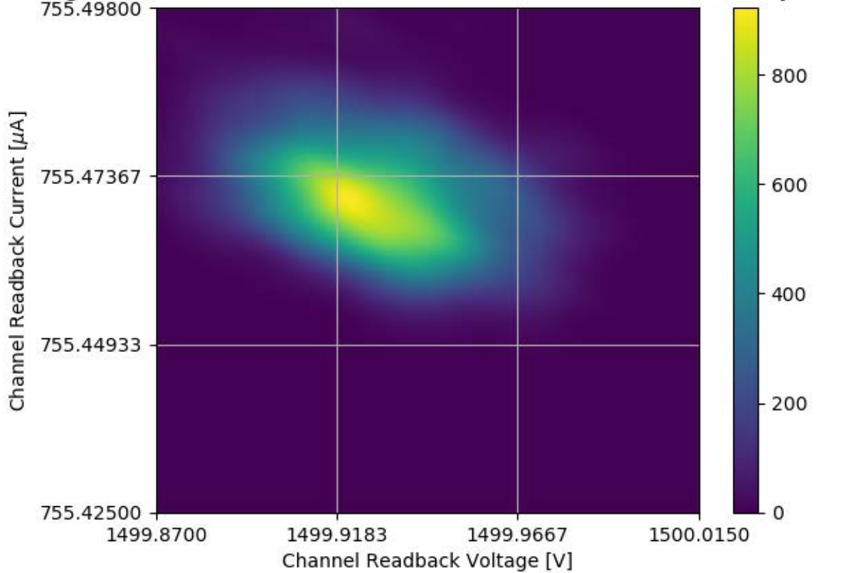
Voltage and Current Readback for Module #327 Channel 01 Stability Test
