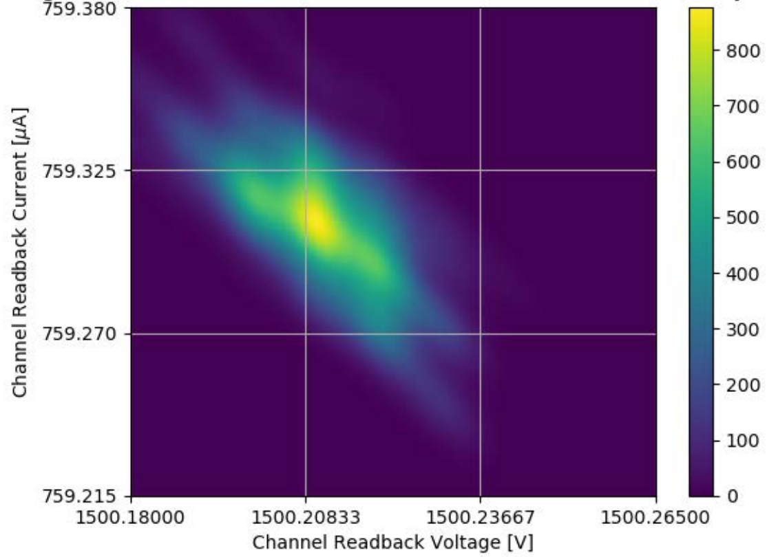
Voltage and Current Readback for Module #327 Channel 12 Stability Test
