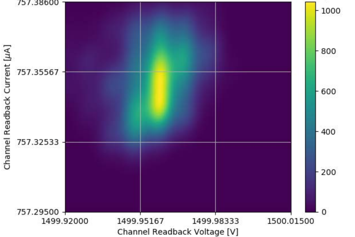
Voltage and Current Readback for Module #327 Channel 21 Stability Test
