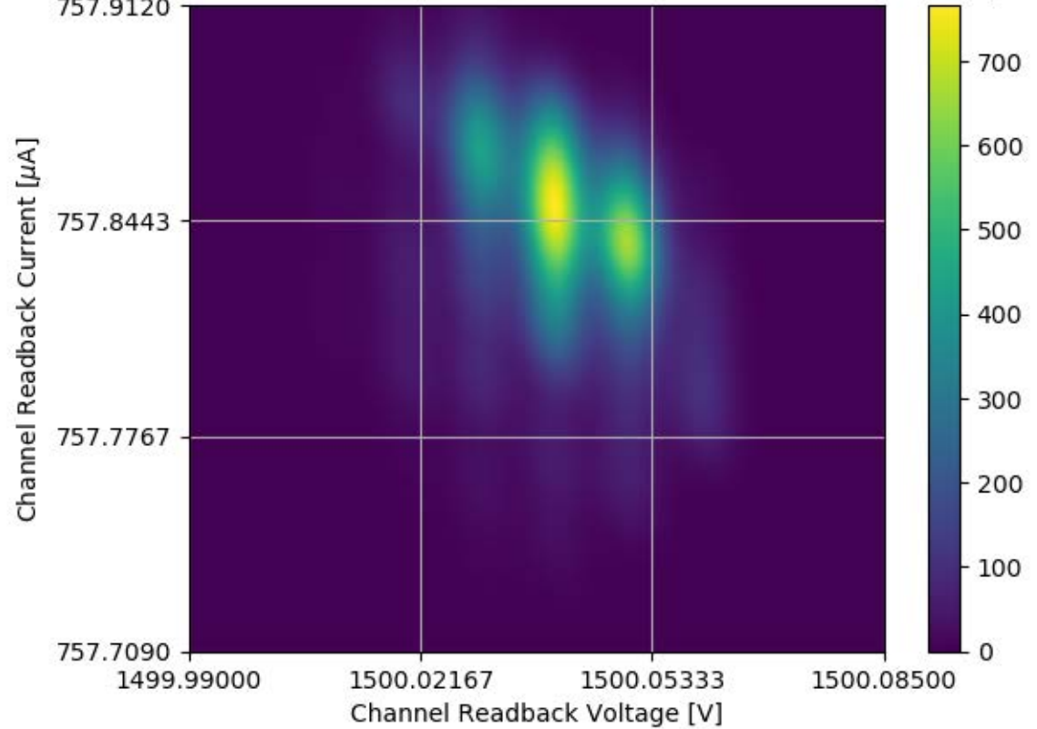
Voltage and Current Readback for Module #327 Channel 06 Stability Test
