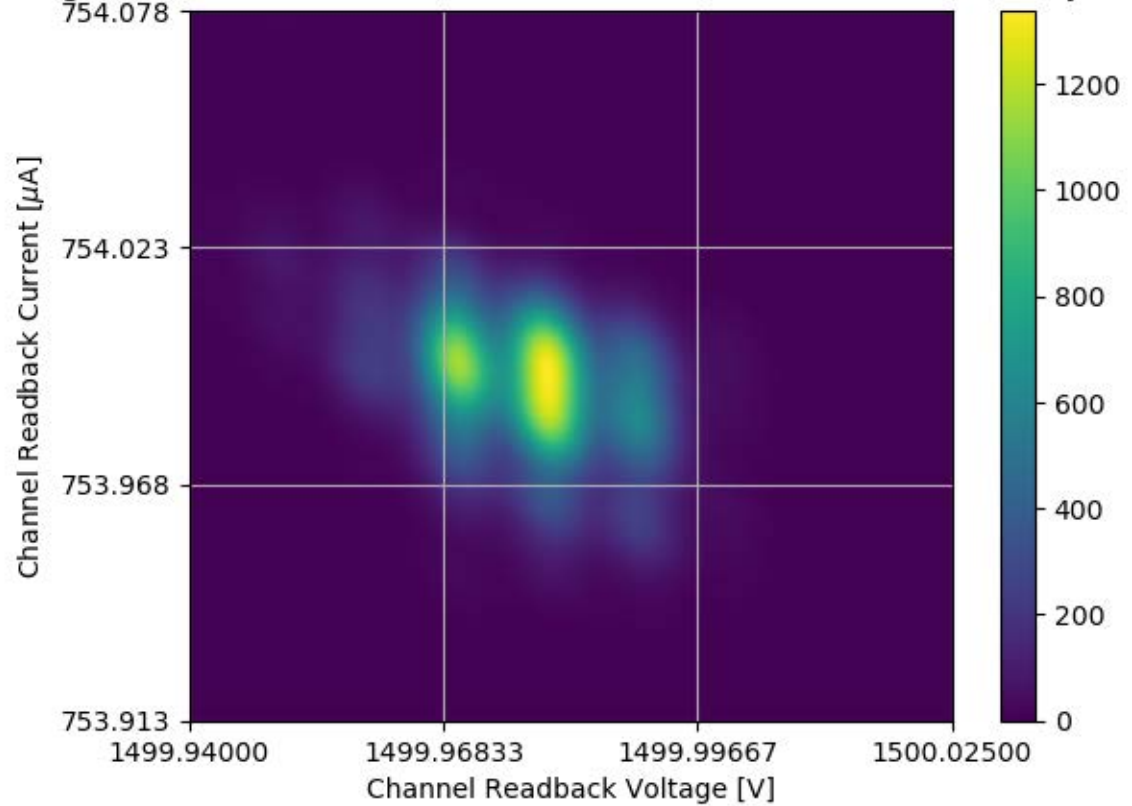
Voltage and Current Readback for Module #327 Channel 00 Stability Test
