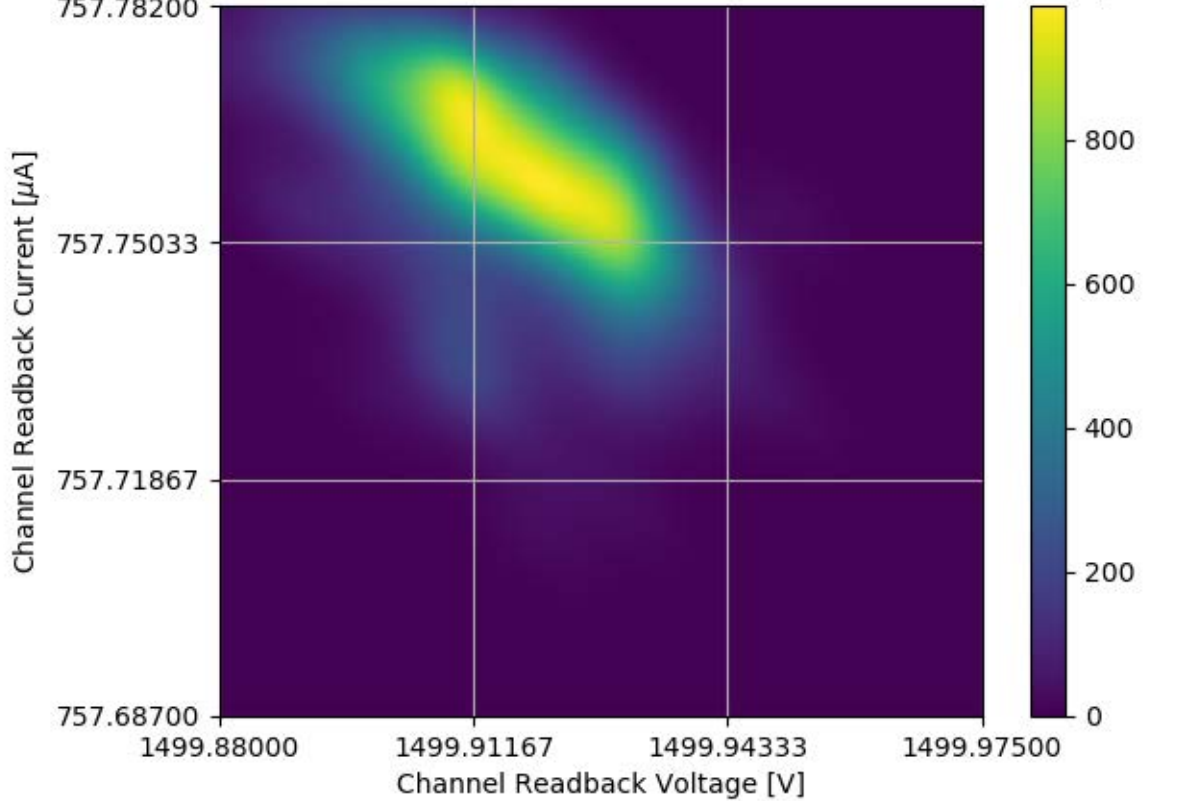
Voltage and Current Readback for Module #327 Channel 04 Stability Test
