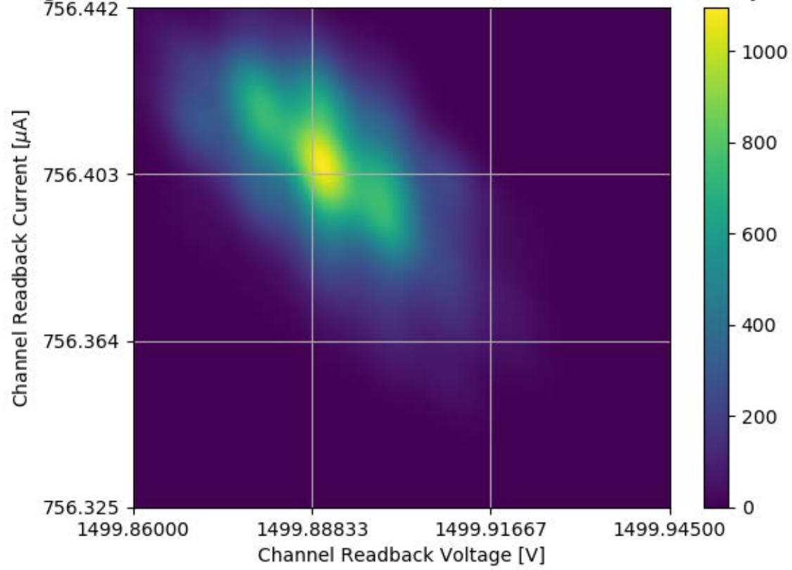
Voltage and Current Readback for Module #327 Channel 27 Stability Test
