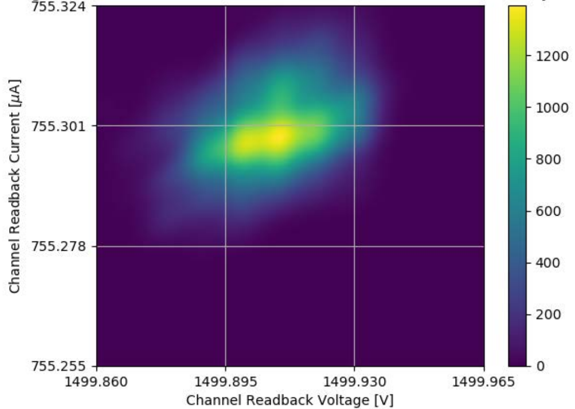
Voltage and Current Readback for Module #327 Channel 14 Stability Test
