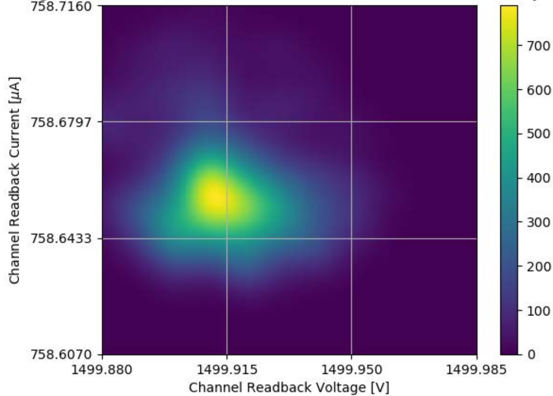
Voltage and Current Readback for Module #327 Channel 25 Stability Test
