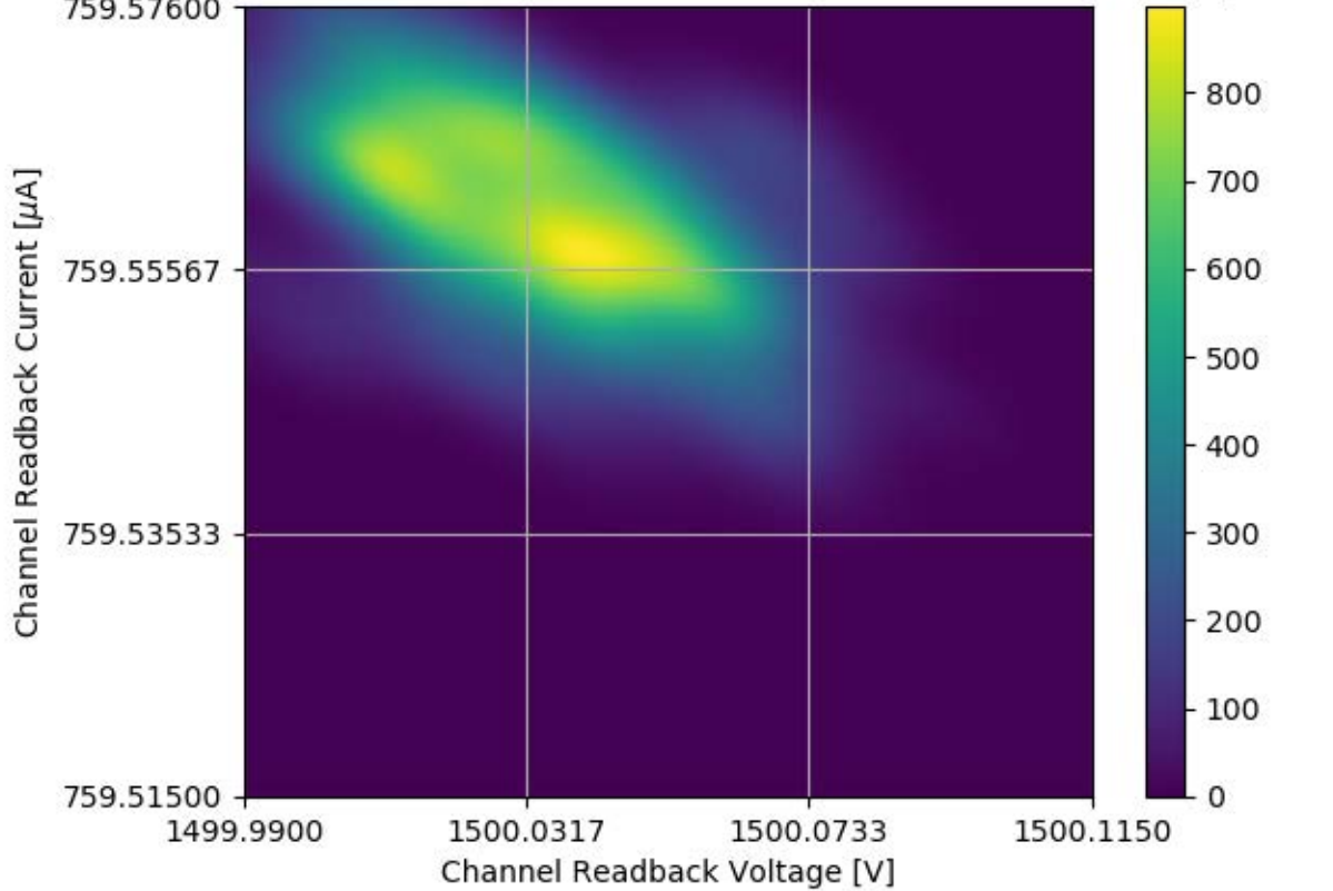
Voltage and Current Readback for Module #327 Channel 24 Stability Test
