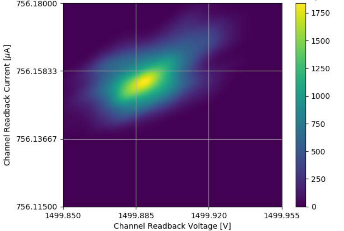
Voltage and Current Readback for Module #327 Channel 19 Stability Test
