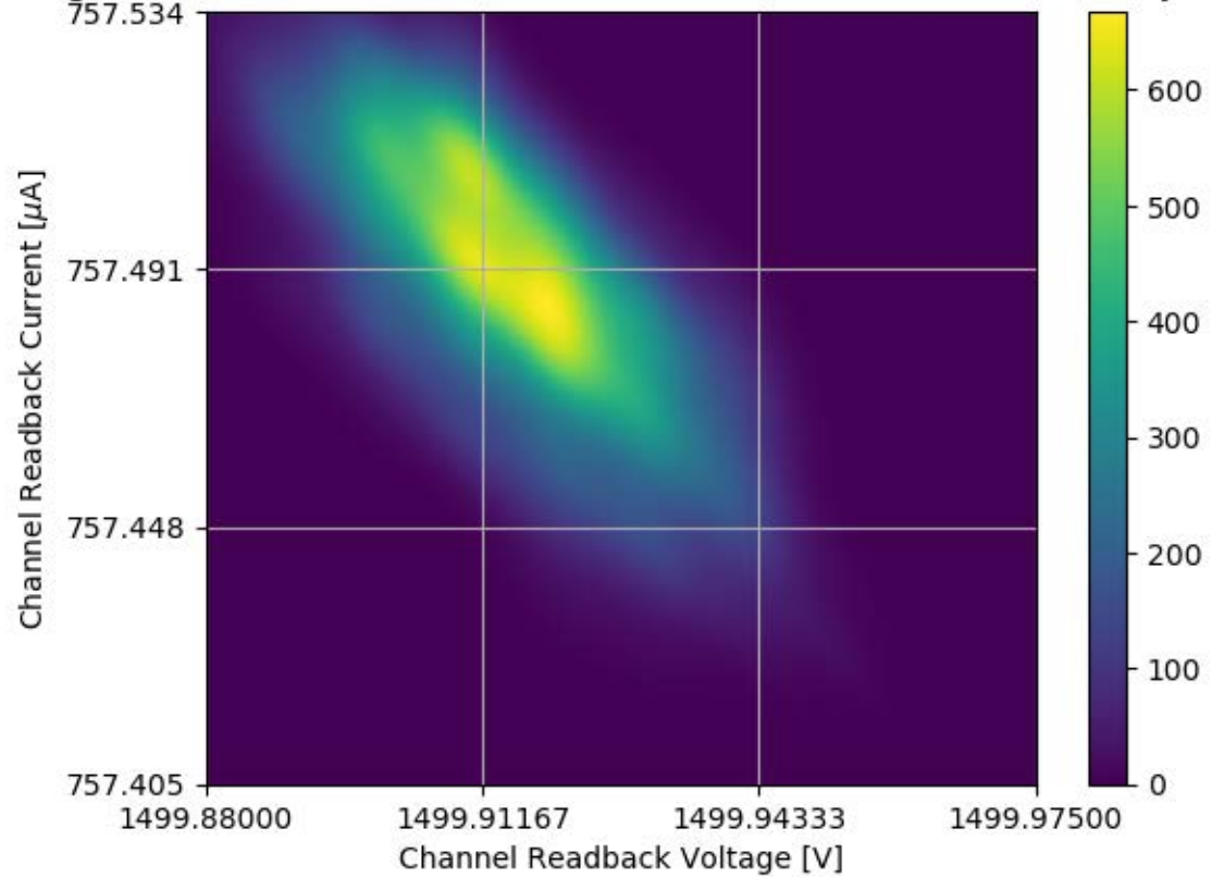
Voltage and Current Readback for Module #327 Channel 29 Stability Test
