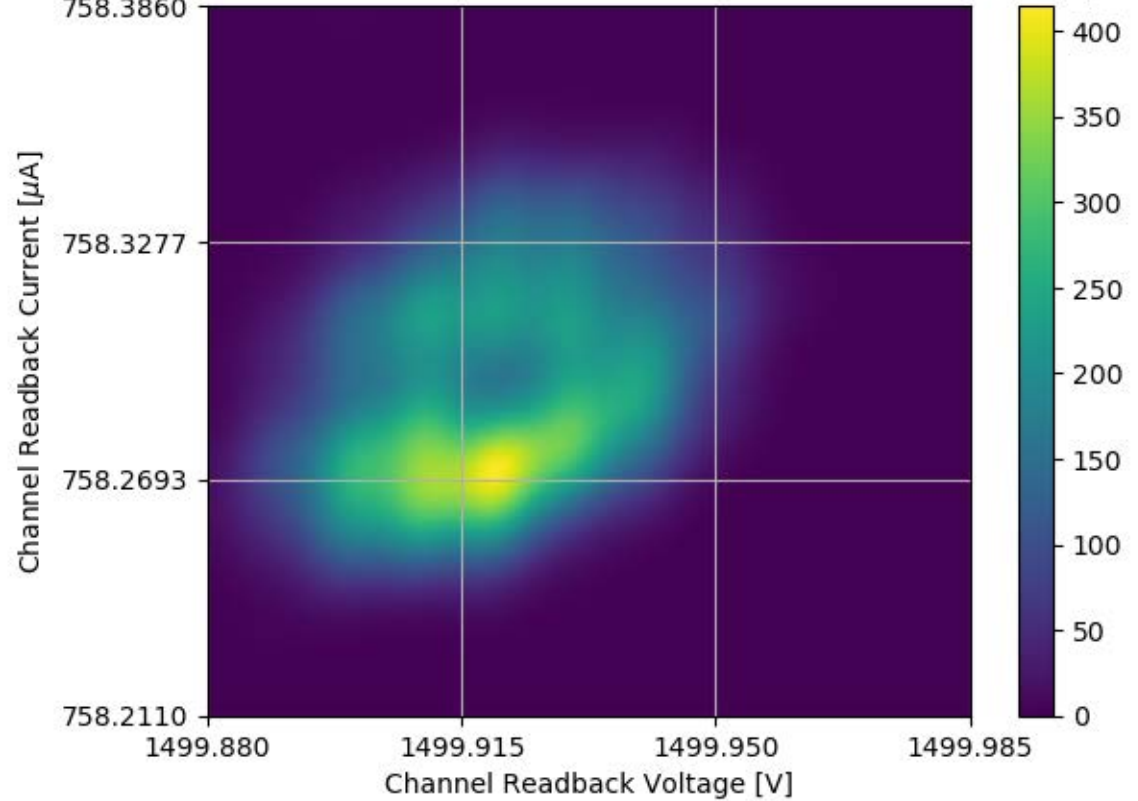
Voltage and Current Readback for Module #327 Channel 22 Stability Test
