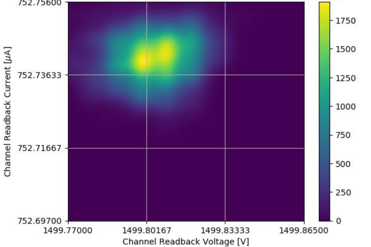
Voltage and Current Readback for Module #327 Channel 11 Stability Test
