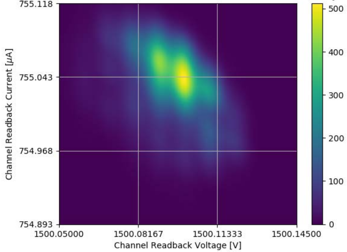
Voltage and Current Readback for Module #327 Channel 03 Stability Test
