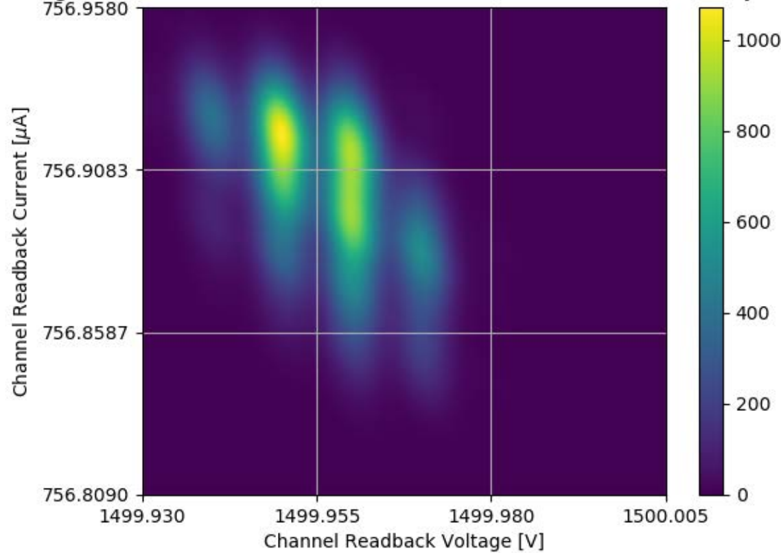
Voltage and Current Readback for Module #327 Channel 20 Stability Test
