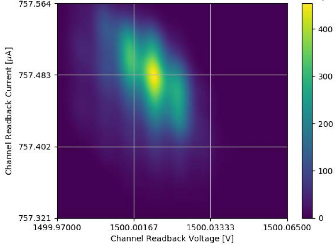
Voltage and Current Readback for Module #327 Channel 16 Stability Test
