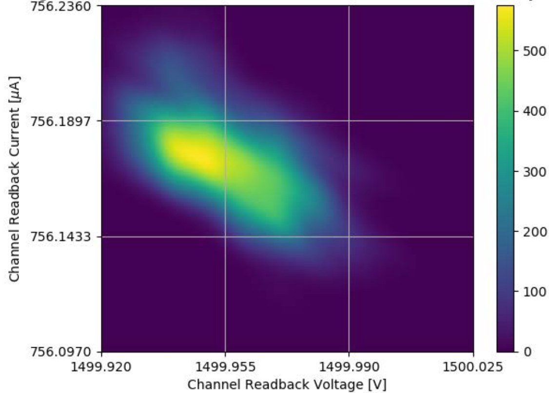
Voltage and Current Readback for Module #327 Channel 34 Stability Test
