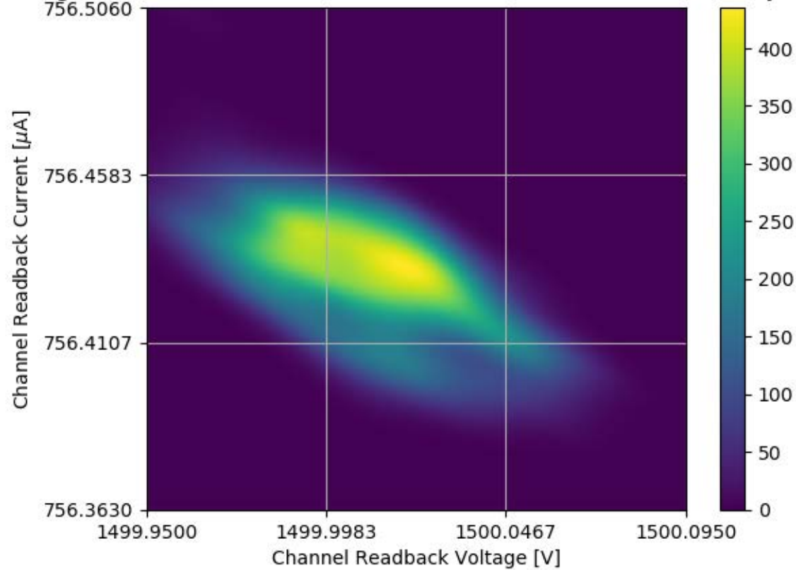
Voltage and Current Readback for Module #327 Channel 23 Stability Test
