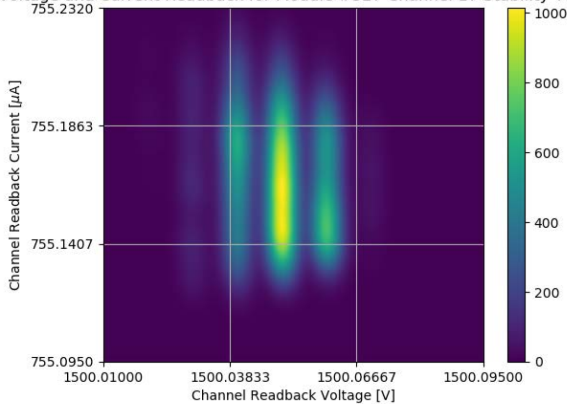
Voltage and Current Readback for Module #327 Channel 17 Stability Test
