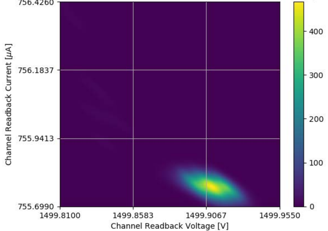
Voltage and Current Readback for Module #336 Channel 17 Stability Test
