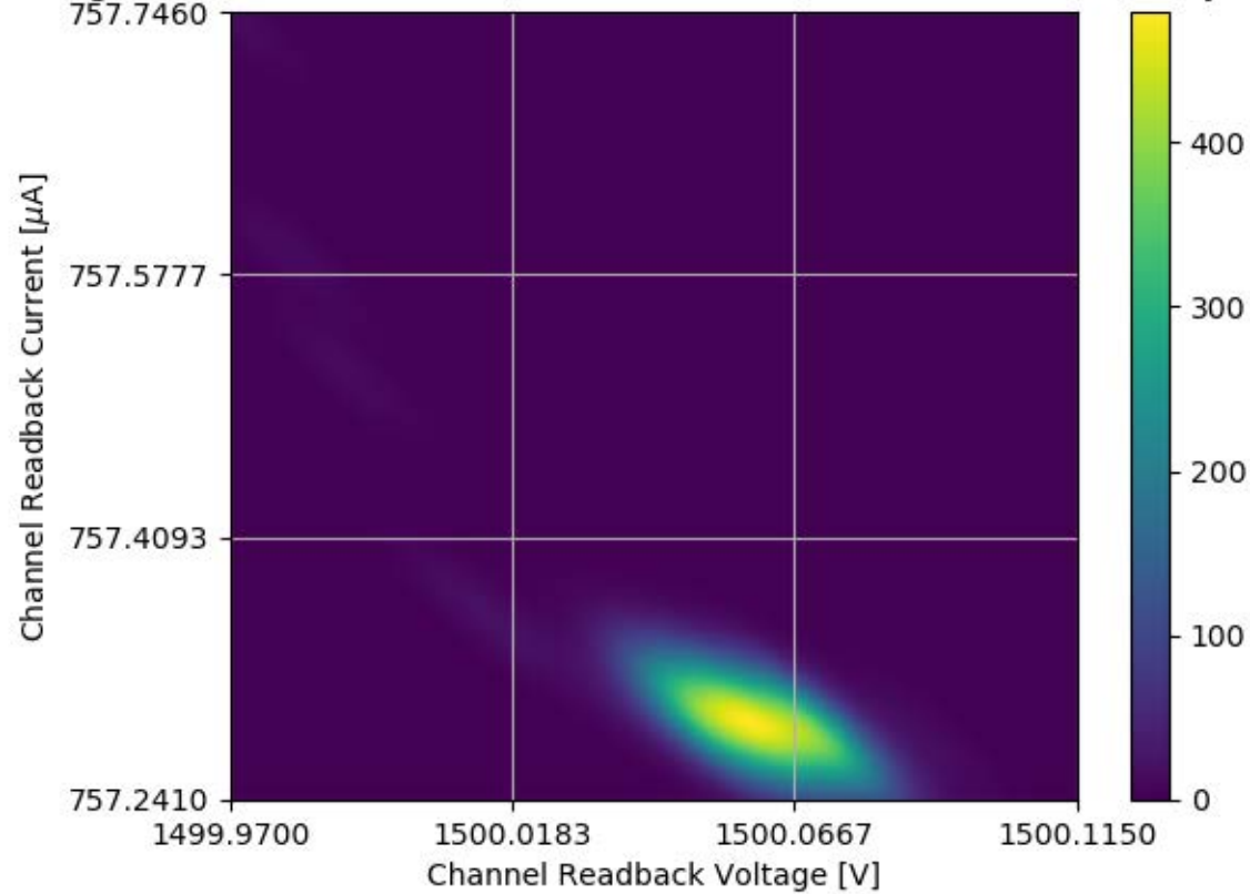
Voltage and Current Readback for Module #336 Channel 20 Stability Test
