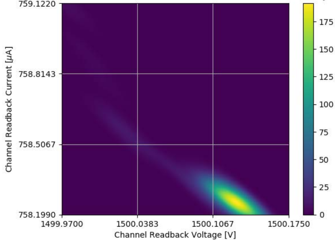
Voltage and Current Readback for Module #336 Channel 06 Stability Test
