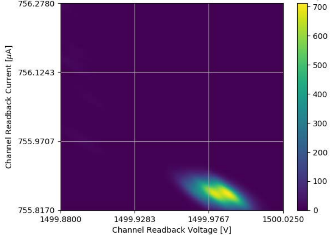
Voltage and Current Readback for Module #336 Channel 14 Stability Test
