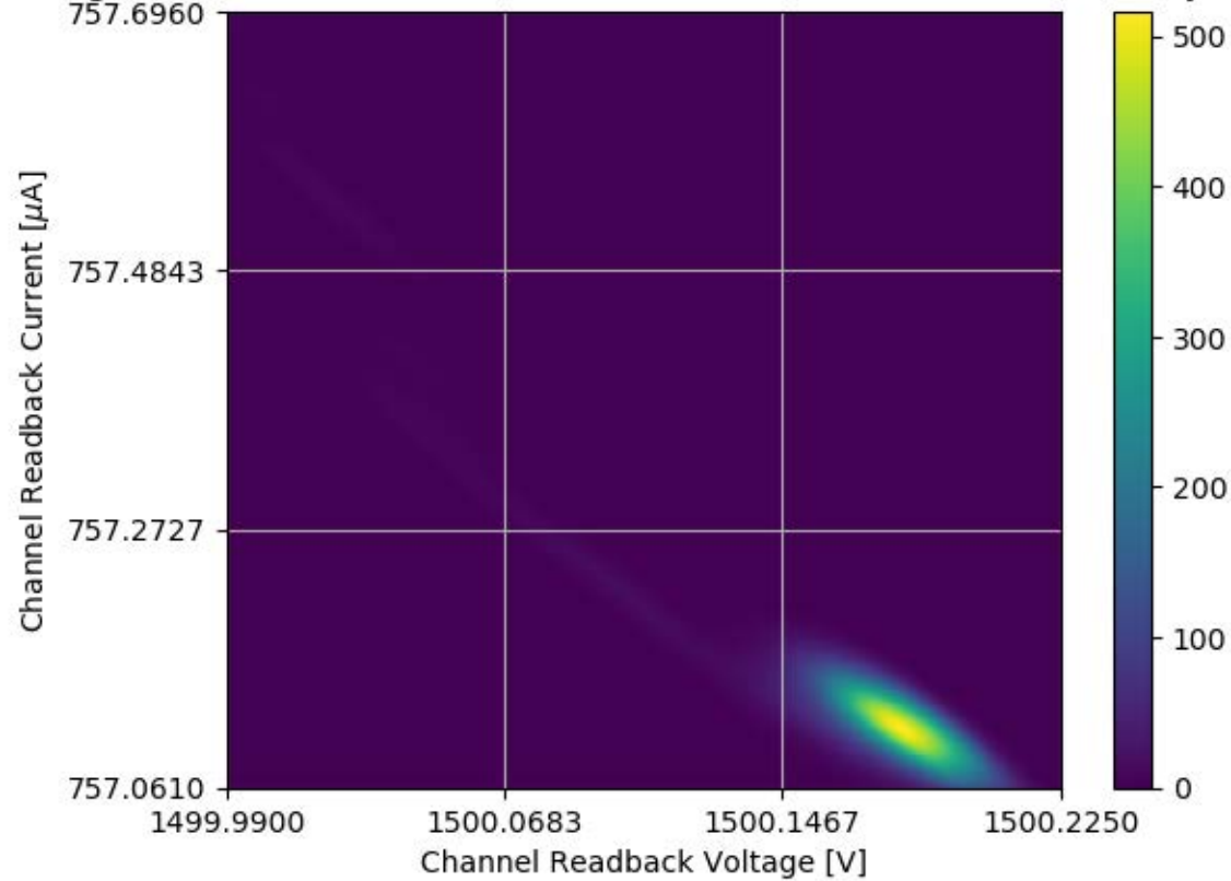
Voltage and Current Readback for Module #336 Channel 19 Stability Test
