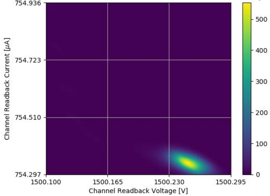
Voltage and Current Readback for Module #336 Channel 00 Stability Test
