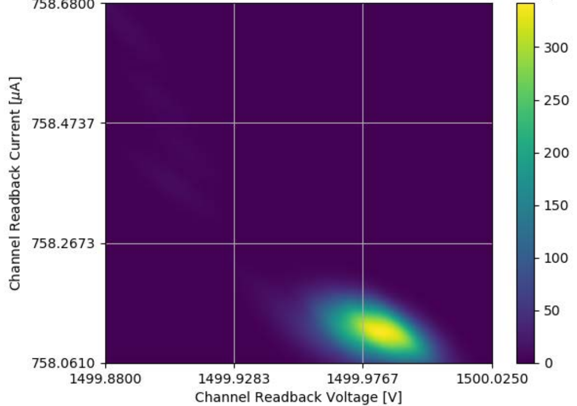
Voltage and Current Readback for Module #336 Channel 16 Stability Test
