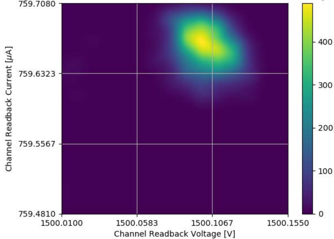
Voltage and Current Readback for Module #336 Channel 25 Stability Test
