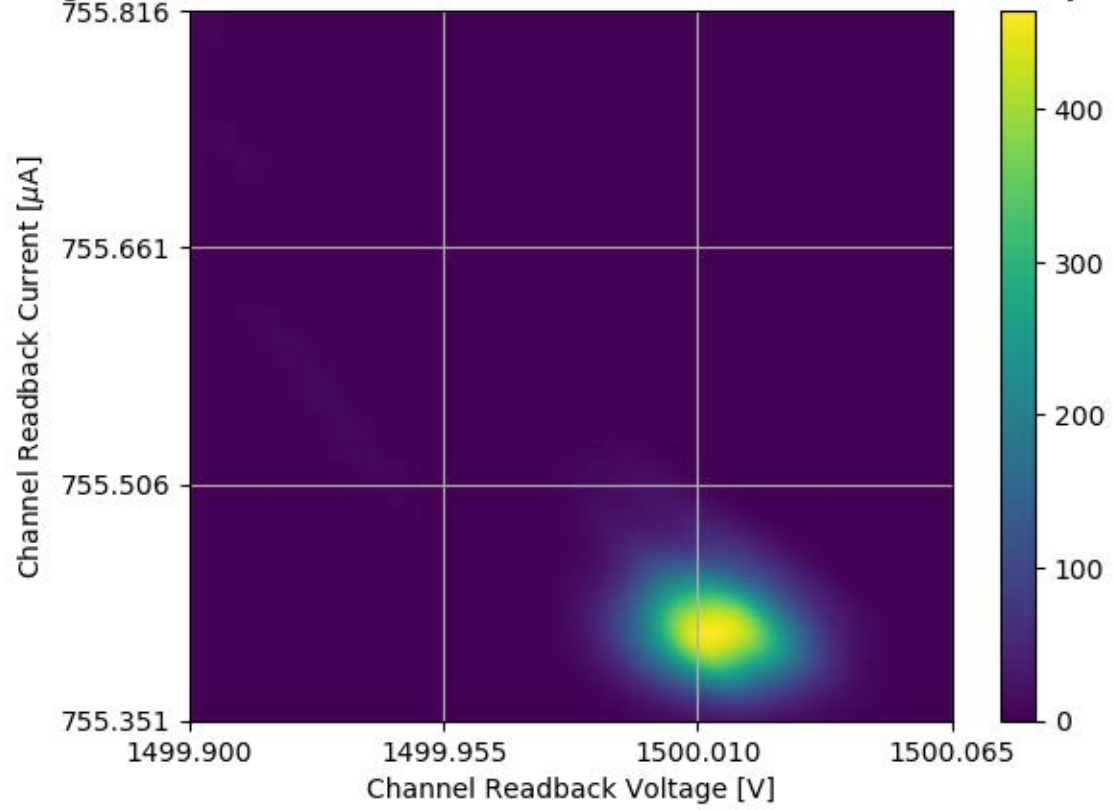
Voltage and Current Readback for Module #336 Channel 28 Stability Test
