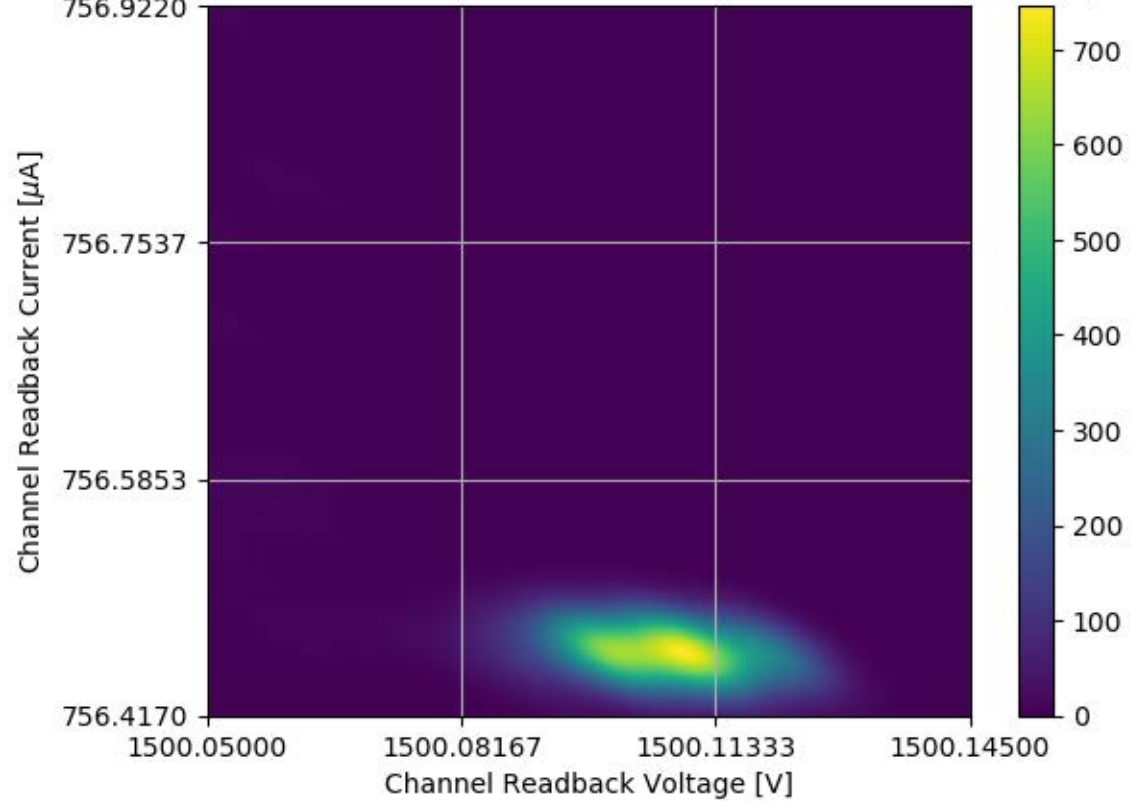
Voltage and Current Readback for Module #336 Channel 15 Stability Test
