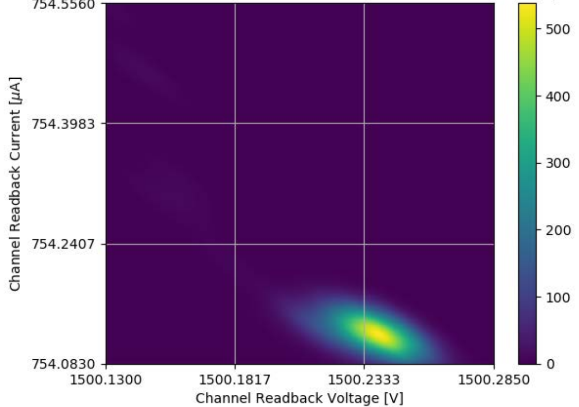
Voltage and Current Readback for Module #336 Channel 33 Stability Test
