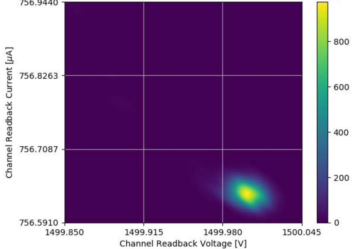
Voltage and Current Readback for Module #336 Channel 27 Stability Test
