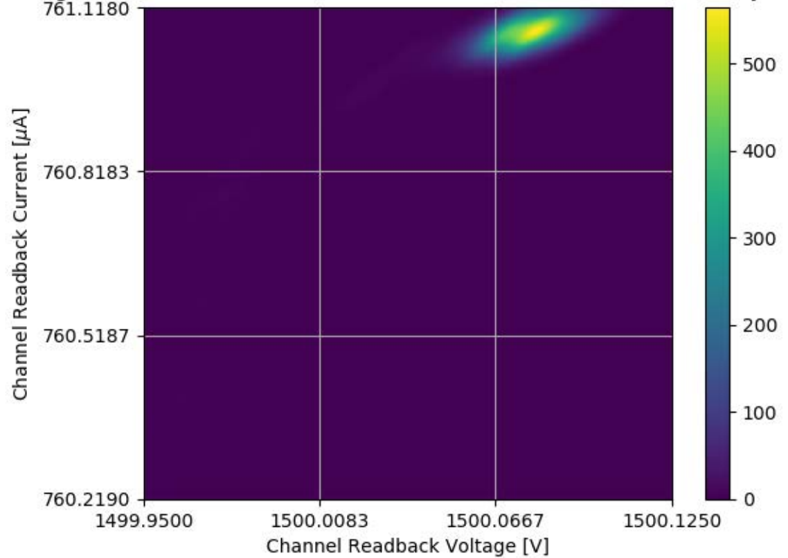
Voltage and Current Readback for Module #336 Channel 09 Stability Test
