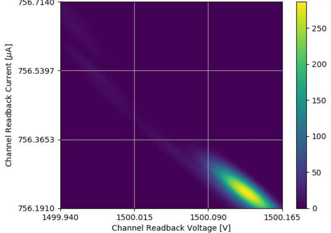
Voltage and Current Readback for Module #336 Channel 31 Stability Test
