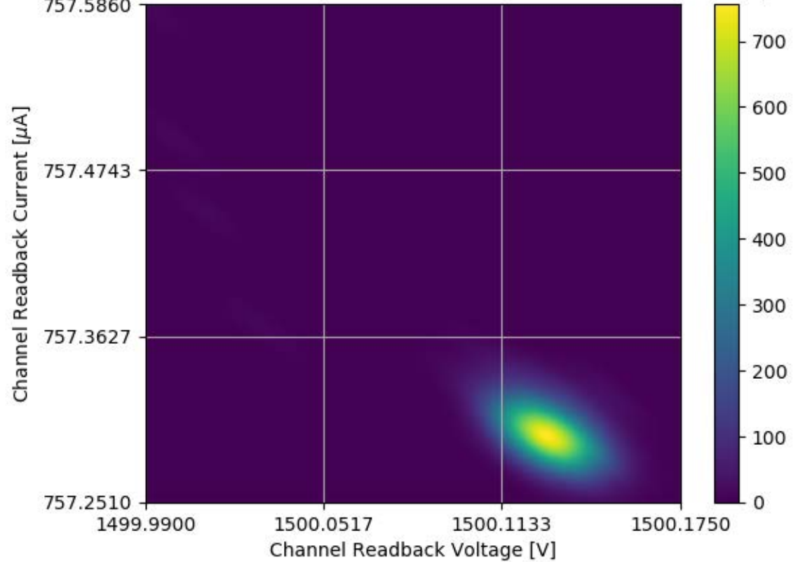
Voltage and Current Readback for Module #336 Channel 32 Stability Test
