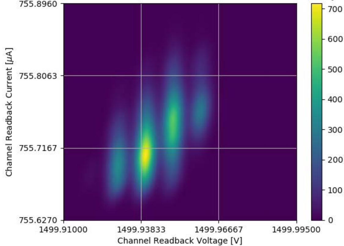
Voltage and Current Readback for Module #337 Channel 02 Stability Test
