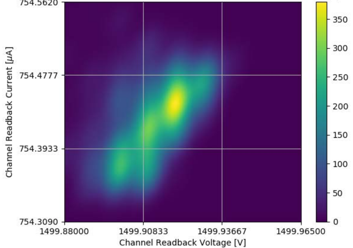
Voltage and Current Readback for Module #337 Channel 13 Stability Test
