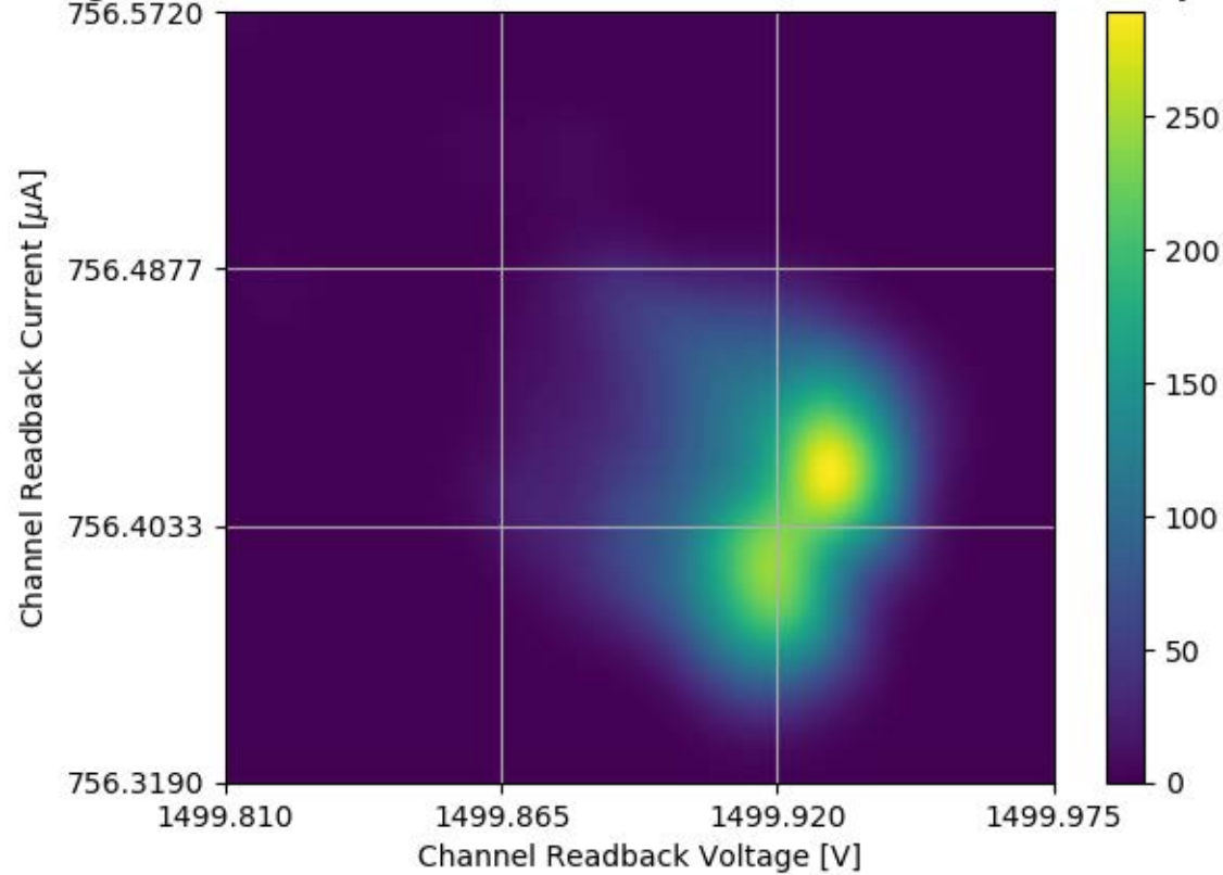
Voltage and Current Readback for Module #337 Channel 18 Stability Test
