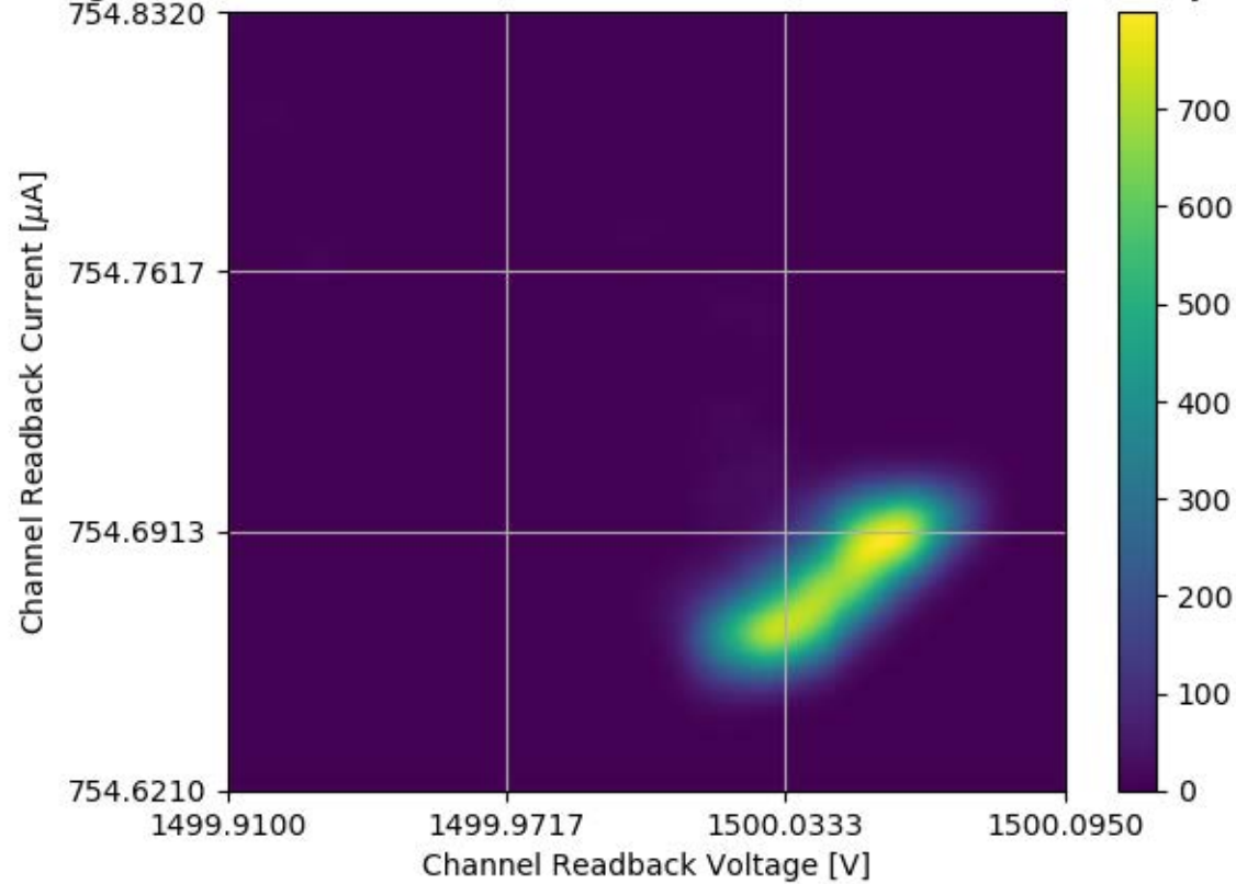
Voltage and Current Readback for Module #337 Channel 11 Stability Test
