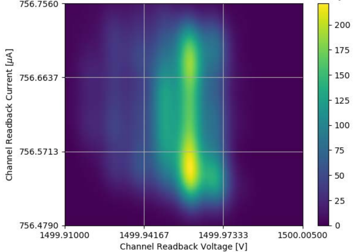
Voltage and Current Readback for Module #337 Channel 27 Stability Test
