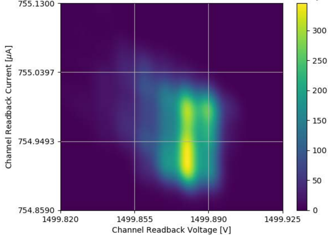
Voltage and Current Readback for Module #337 Channel 03 Stability Test
