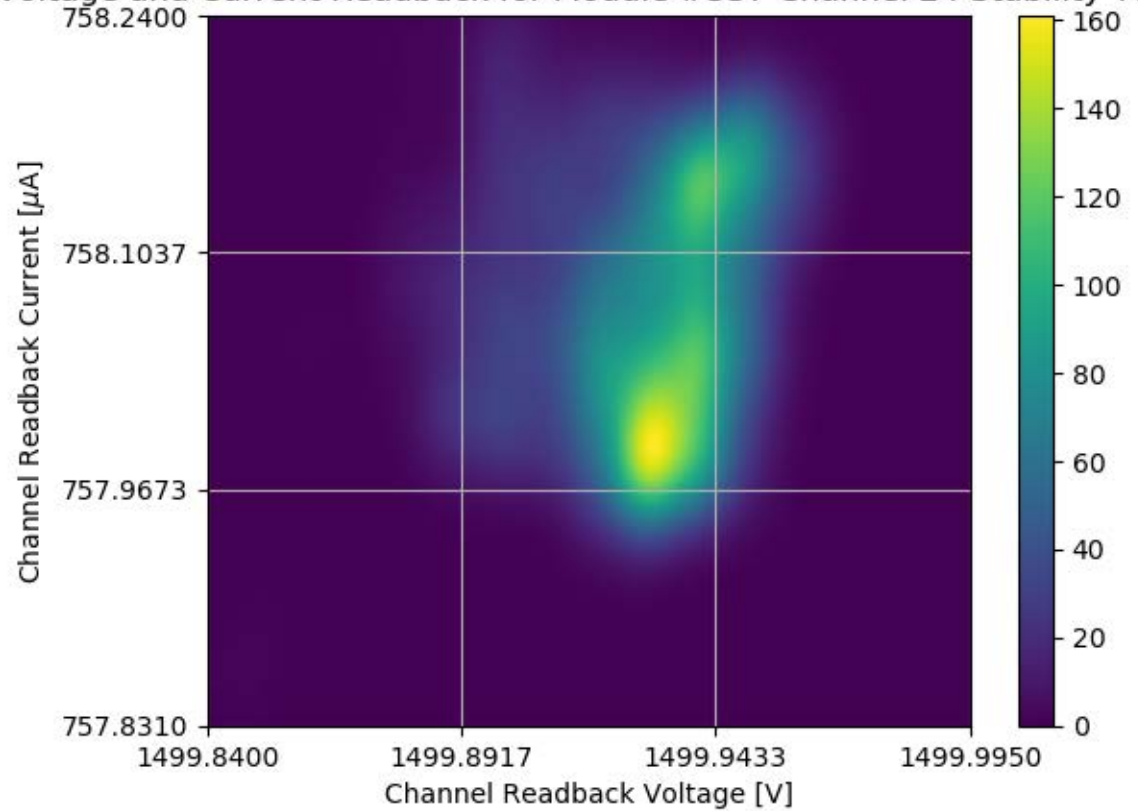
Voltage and Current Readback for Module #337 Channel 24 Stability Test
