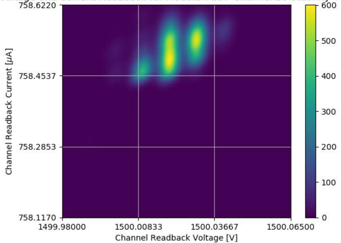
Voltage and Current Readback for Module #337 Channel 10 Stability Test
