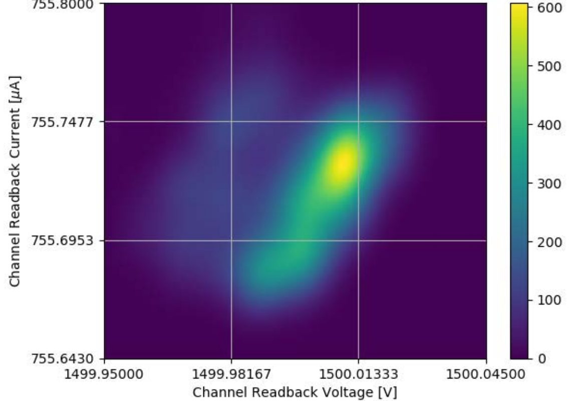
Voltage and Current Readback for Module #337 Channel 15 Stability Test
