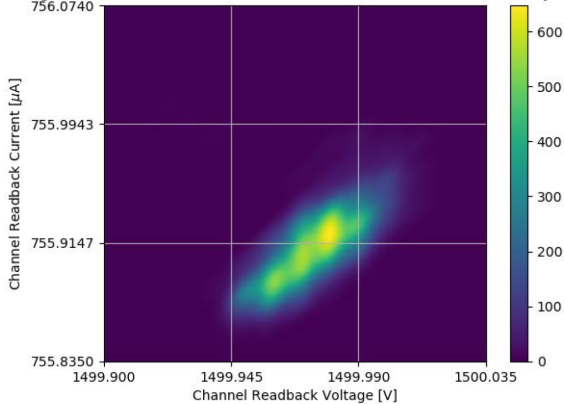
Voltage and Current Readback for Module #337 Channel 14 Stability Test
