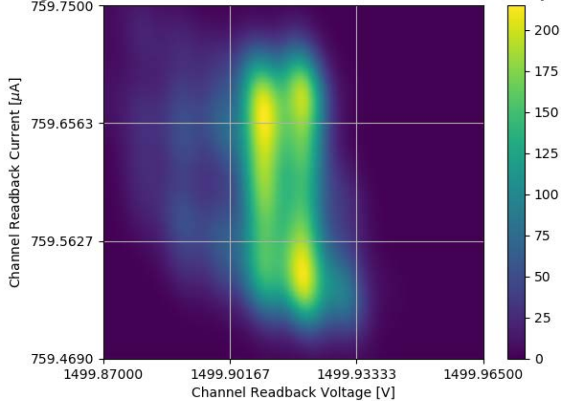
Voltage and Current Readback for Module #337 Channel 32 Stability Test
