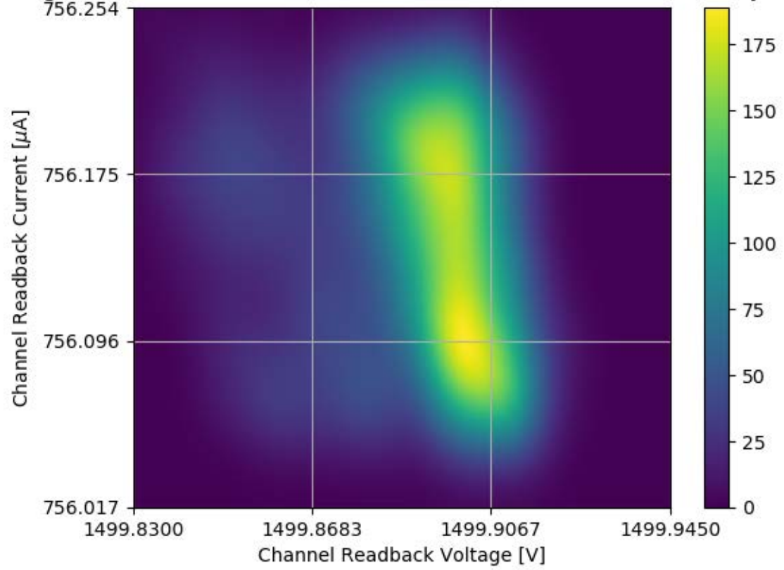
Voltage and Current Readback for Module #337 Channel 34 Stability Test
