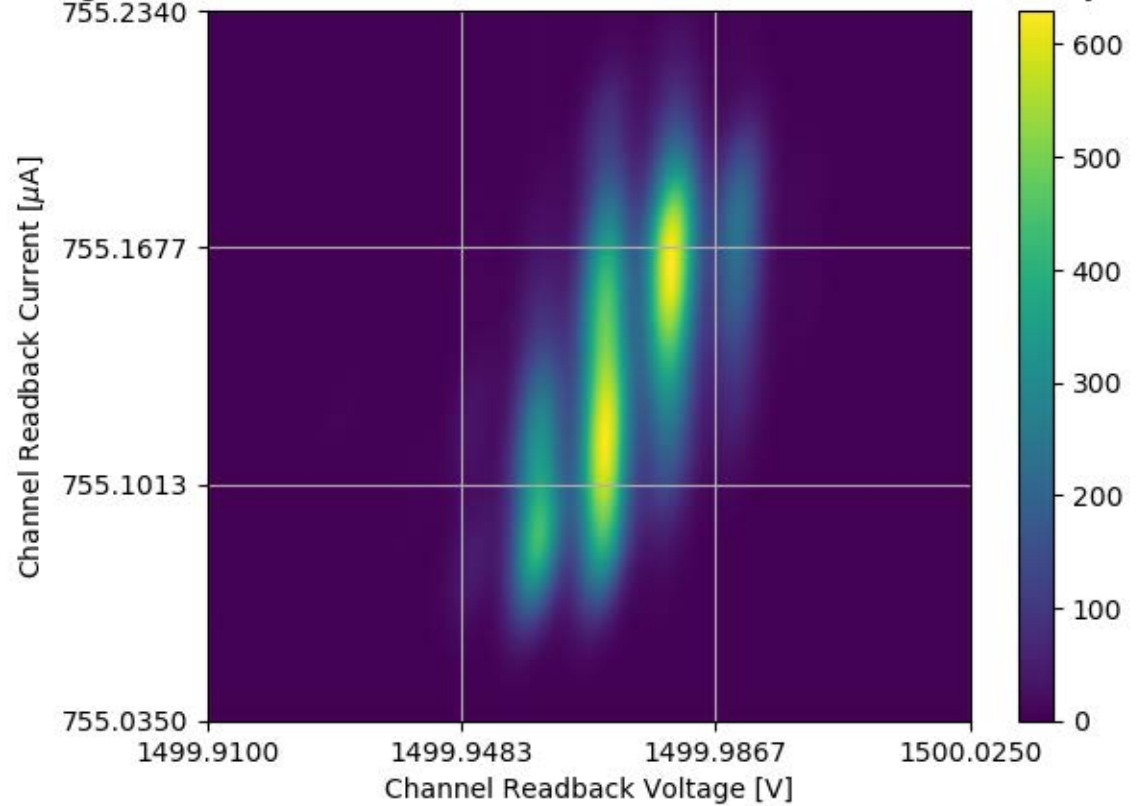
Voltage and Current Readback for Module #337 Channel 01 Stability Test
