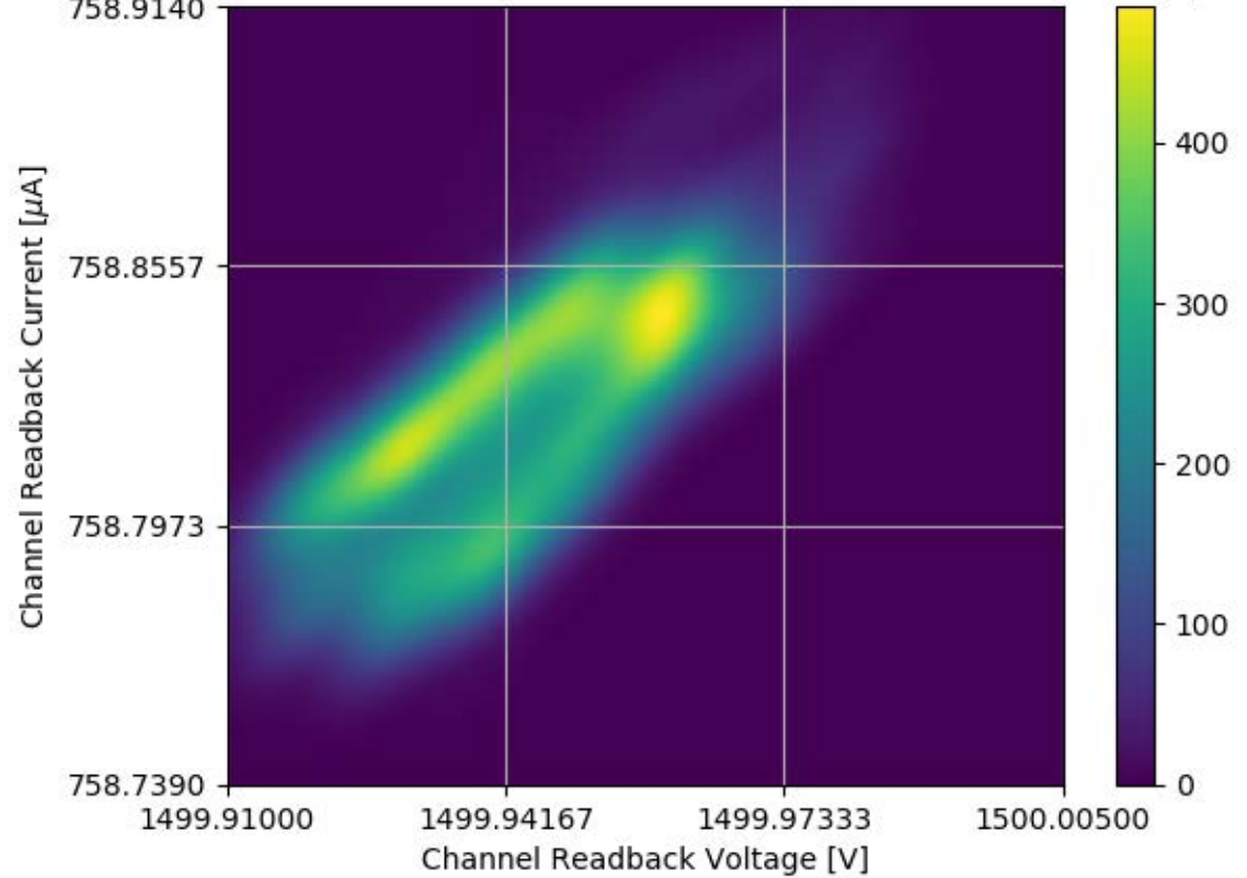
Voltage and Current Readback for Module #337 Channel 12 Stability Test
