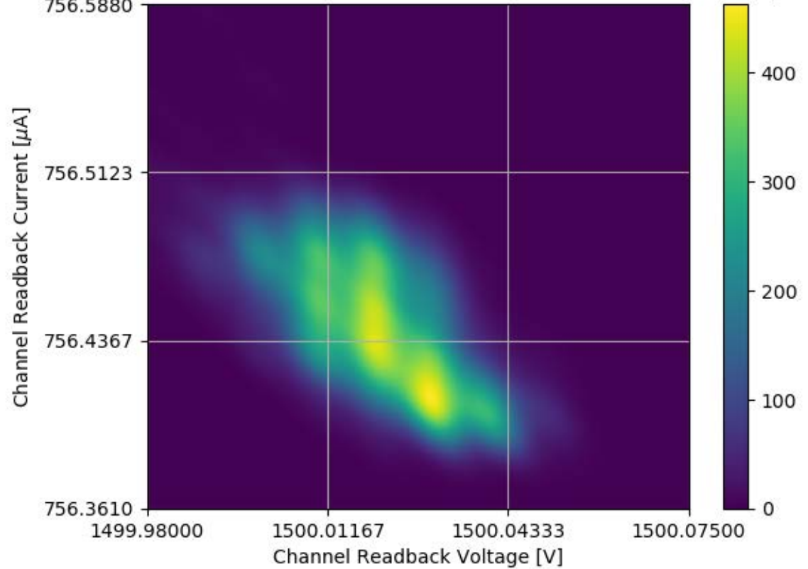
Voltage and Current Readback for Module #337 Channel 31 Stability Test
