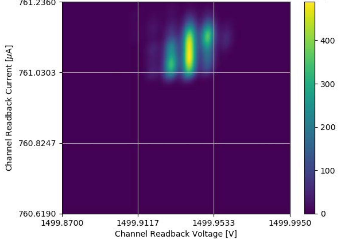
Voltage and Current Readback for Module #337 Channel 09 Stability Test
