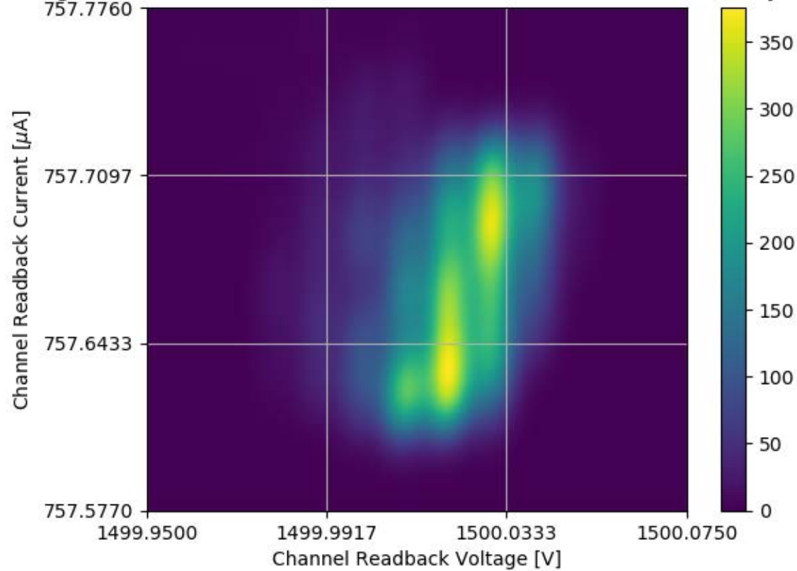
Voltage and Current Readback for Module #337 Channel 06 Stability Test
