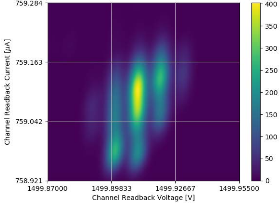
Voltage and Current Readback for Module #337 Channel 22 Stability Test
