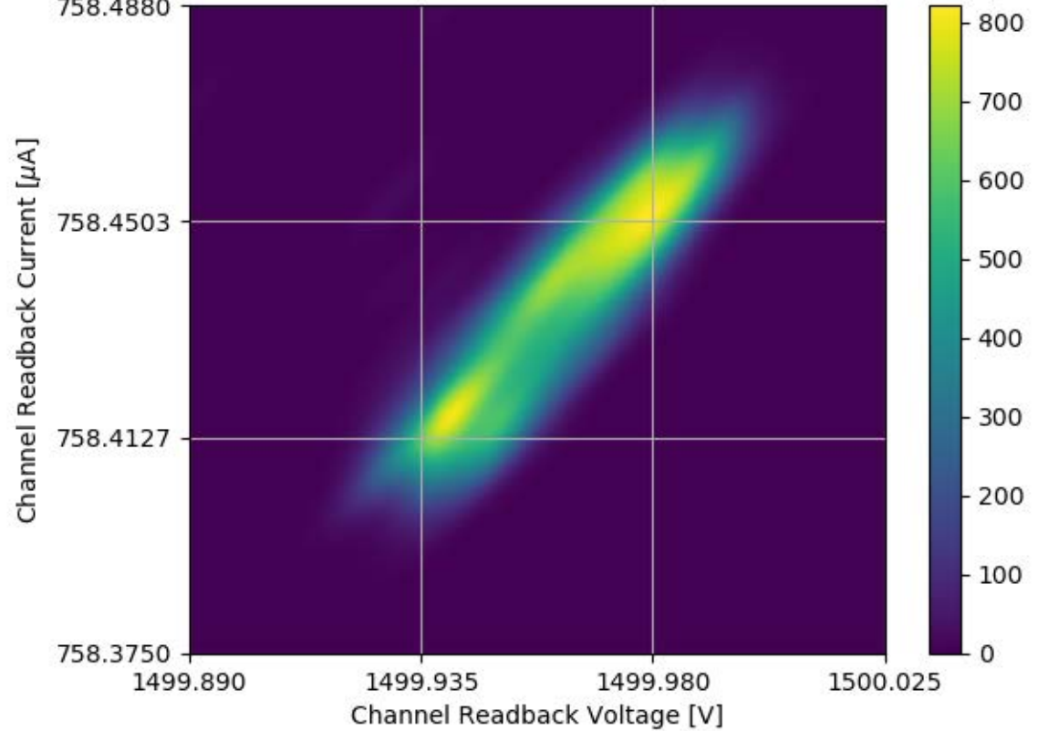
Voltage and Current Readback for Module #337 Channel 35 Stability Test
