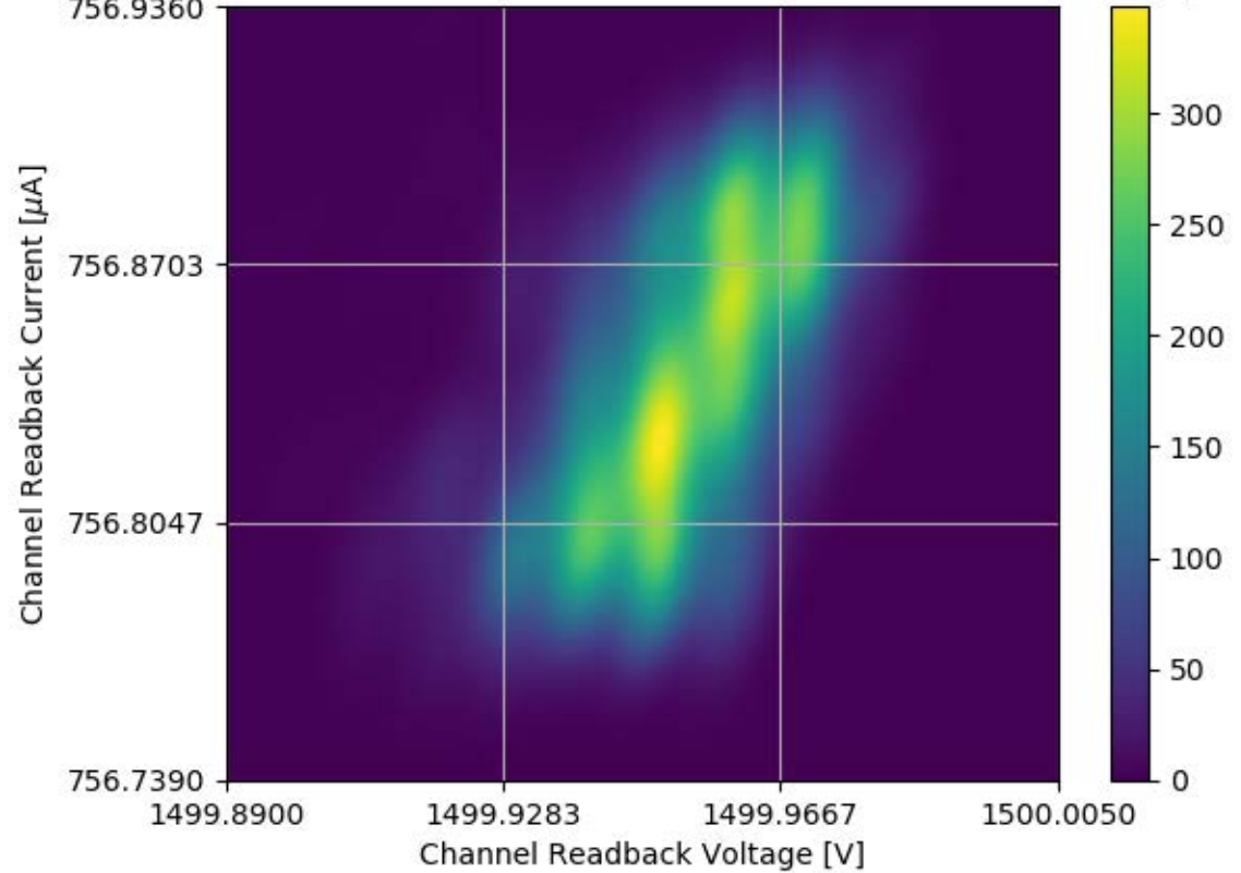
Voltage and Current Readback for Module #337 Channel 23 Stability Test
