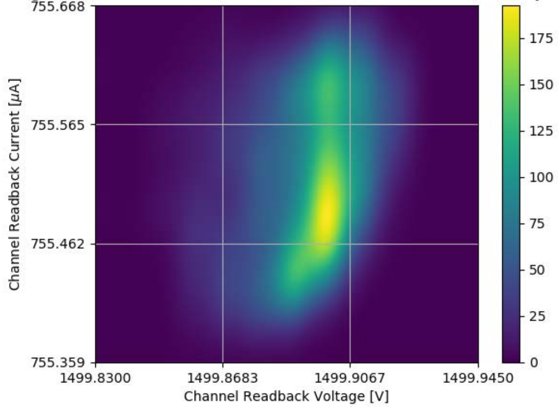
Voltage and Current Readback for Module #337 Channel 21 Stability Test
