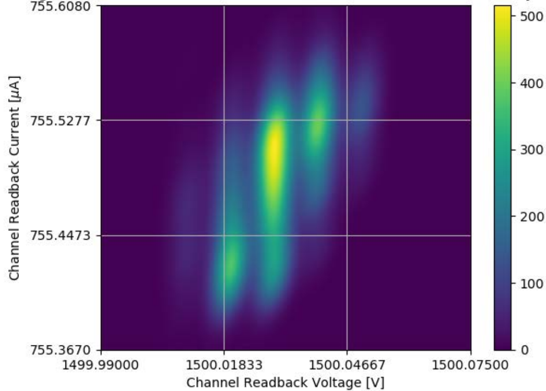
Voltage and Current Readback for Module #337 Channel 17 Stability Test
