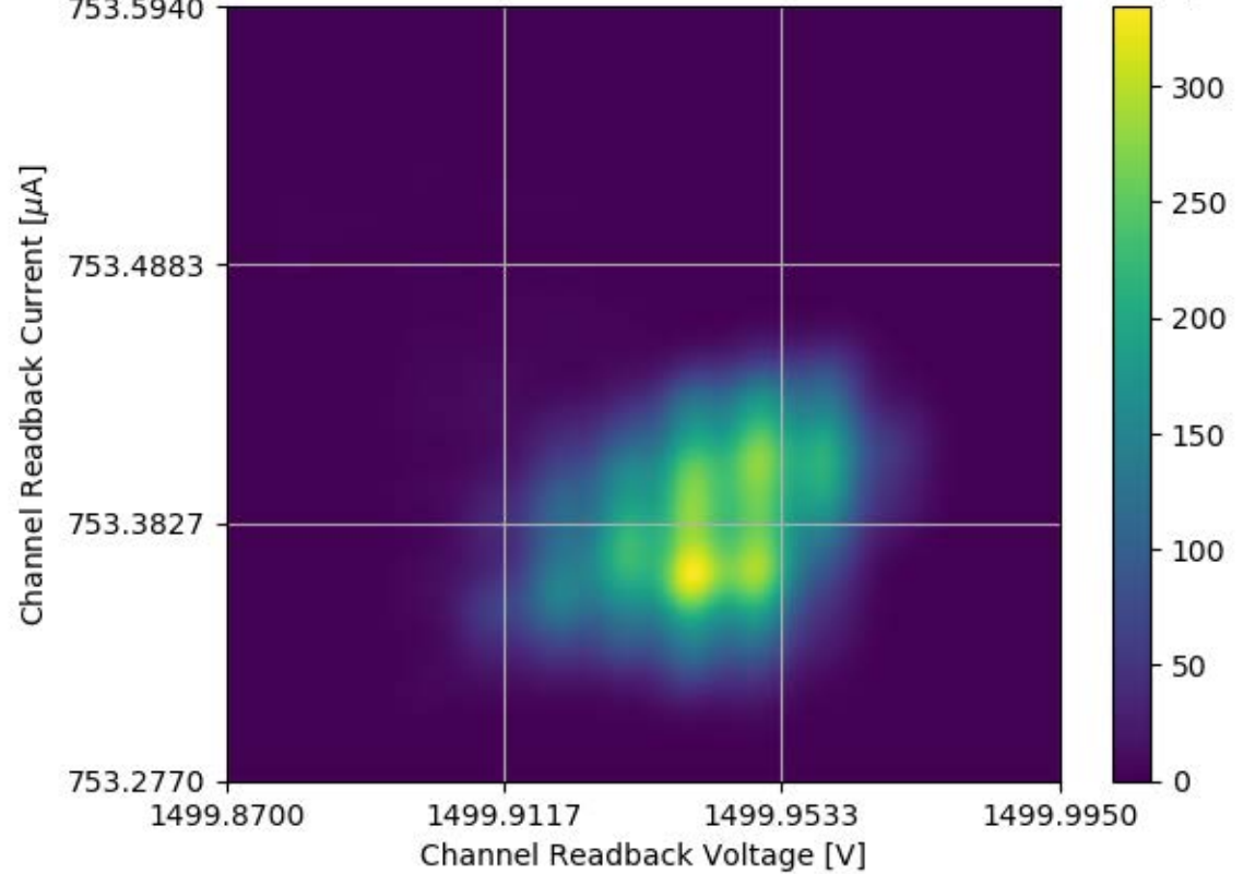
Voltage and Current Readback for Module #337 Channel 33 Stability Test
