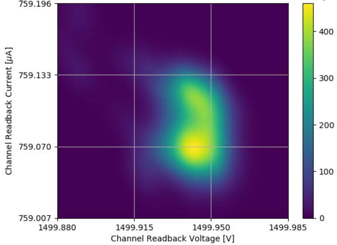
Voltage and Current Readback for Module #338 Channel 05 Stability Test
