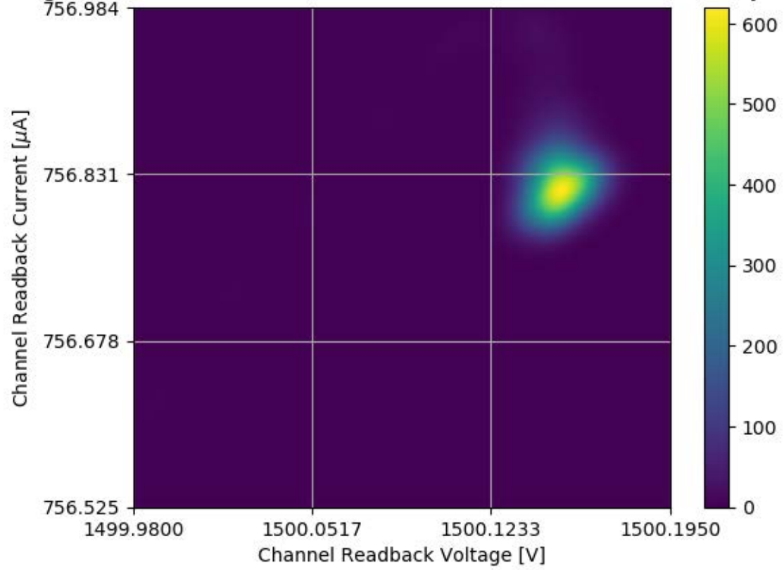
Voltage and Current Readback for Module #338 Channel 19 Stability Test
