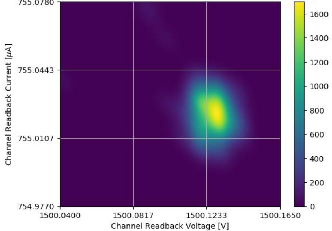
Voltage and Current Readback for Module #338 Channel 13 Stability Test
