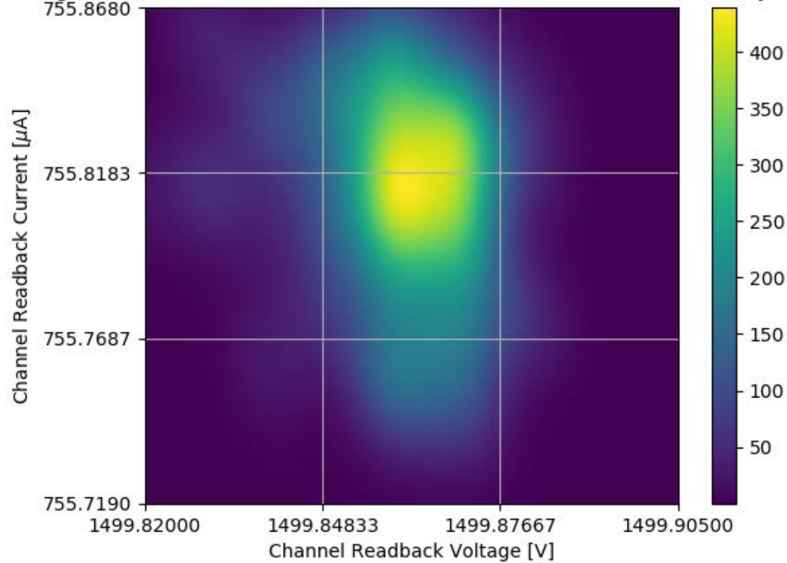
Voltage and Current Readback for Module #338 Channel 20 Stability Test
