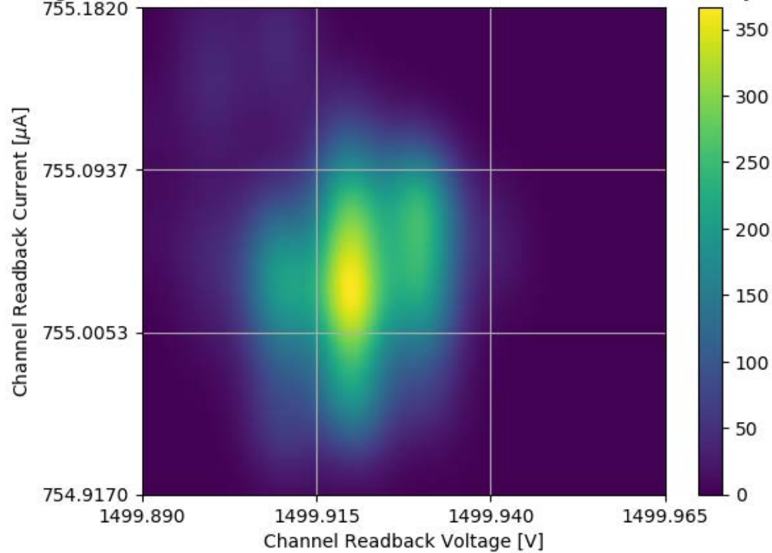
Voltage and Current Readback for Module #338 Channel 33 Stability Test
