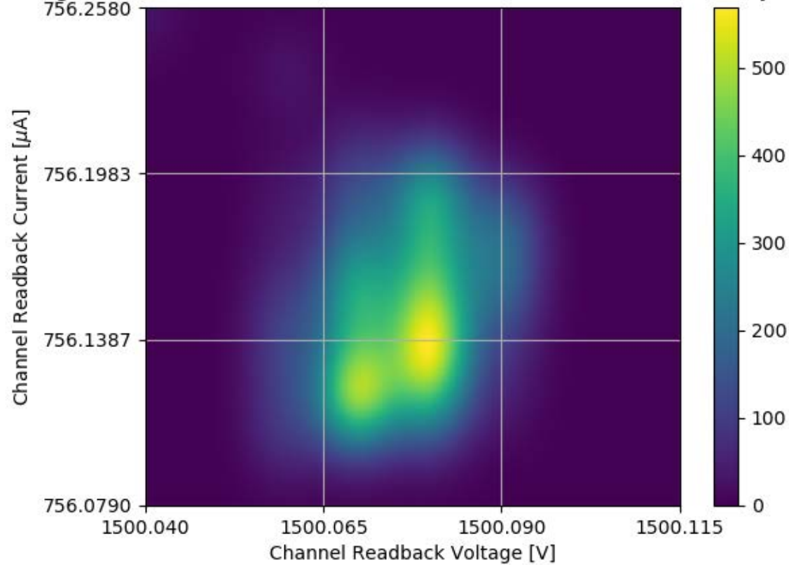
Voltage and Current Readback for Module #338 Channel 28 Stability Test
