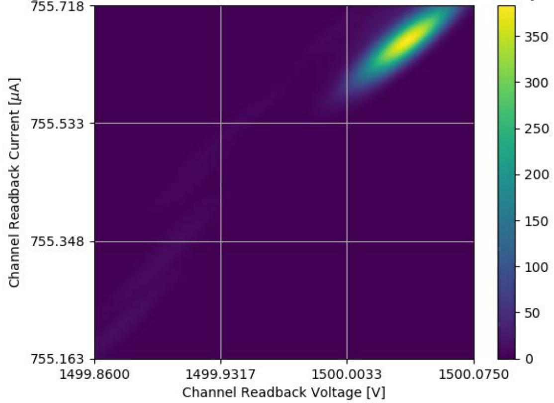
Voltage and Current Readback for Module #338 Channel 14 Stability Test
