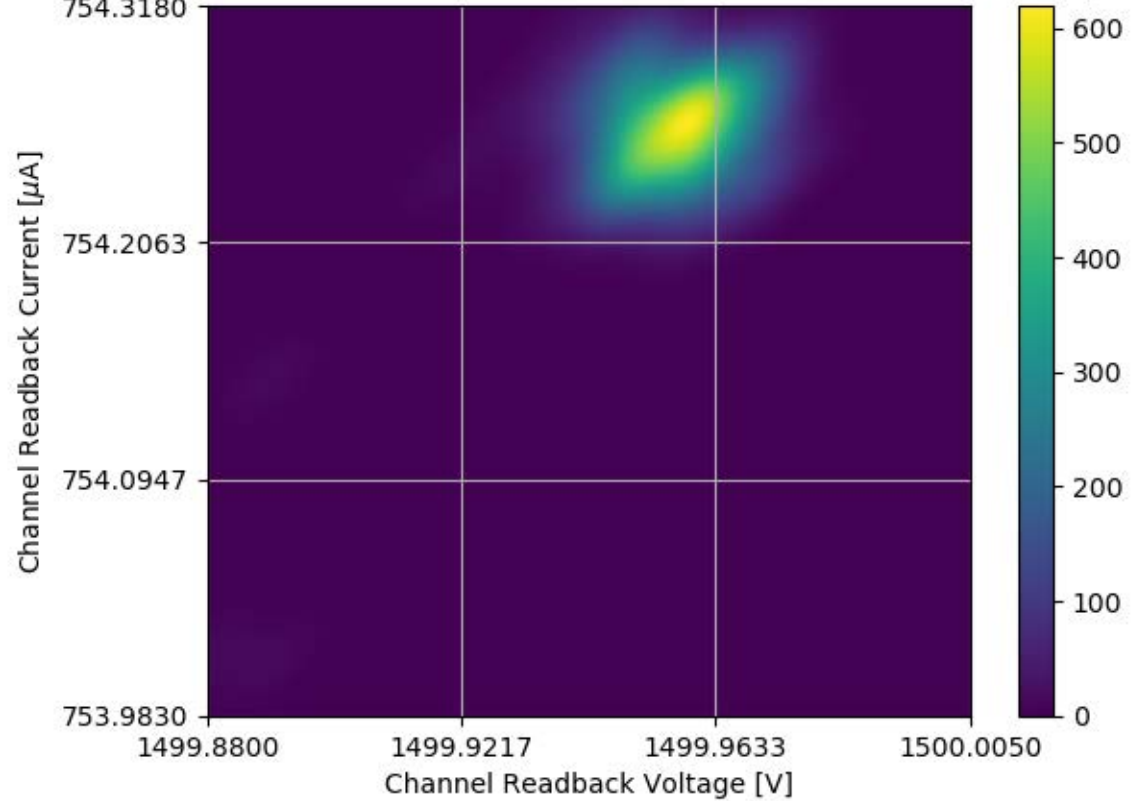
Voltage and Current Readback for Module #338 Channel 00 Stability Test
