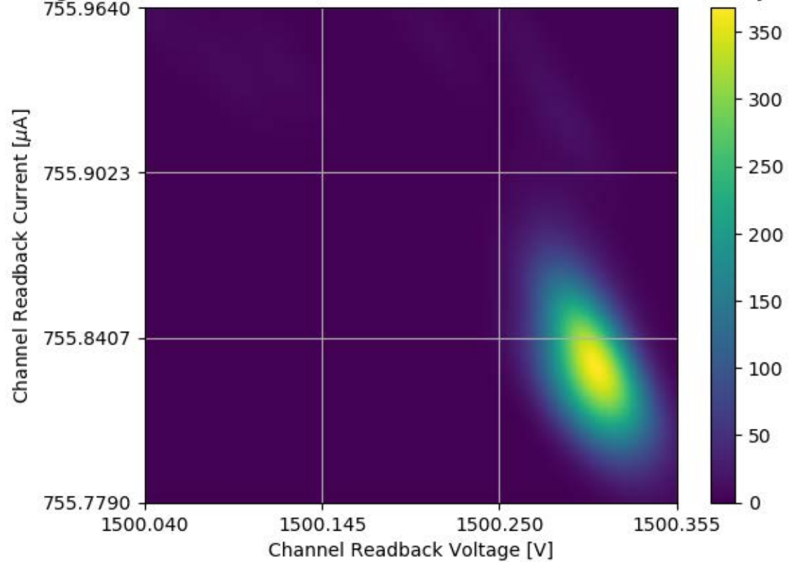
Voltage and Current Readback for Module #338 Channel 02 Stability Test
