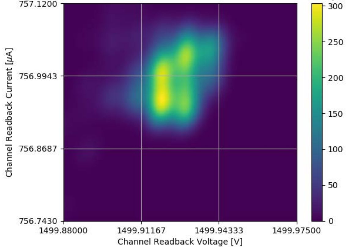
Voltage and Current Readback for Module #338 Channel 16 Stability Test
