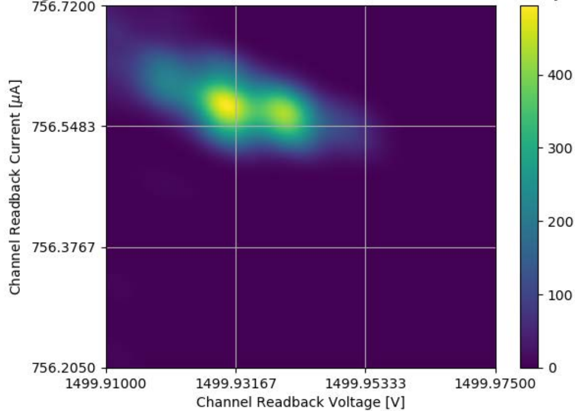
Voltage and Current Readback for Module #338 Channel 27 Stability Test
