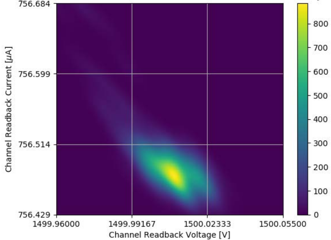
Voltage and Current Readback for Module #338 Channel 17 Stability Test
