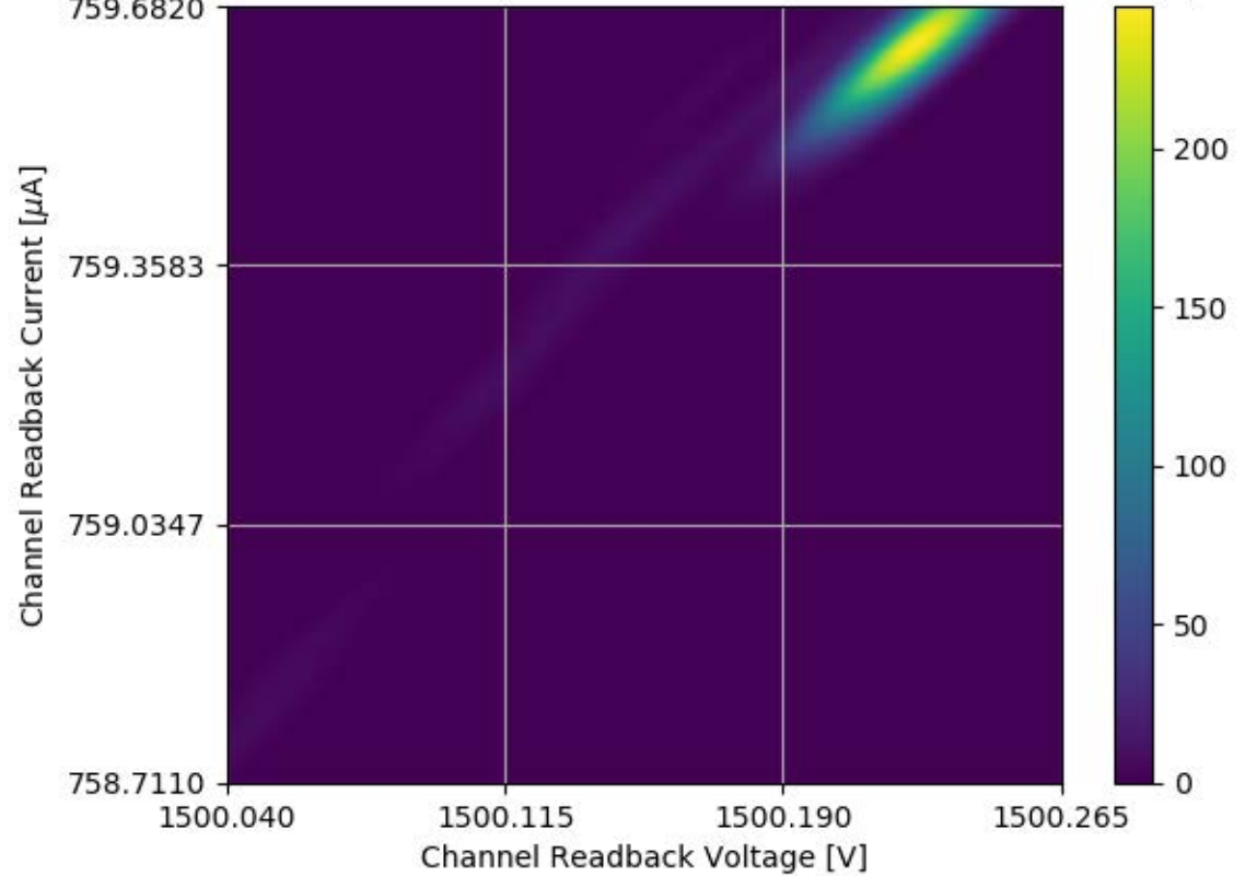
Voltage and Current Readback for Module #338 Channel 12 Stability Test
