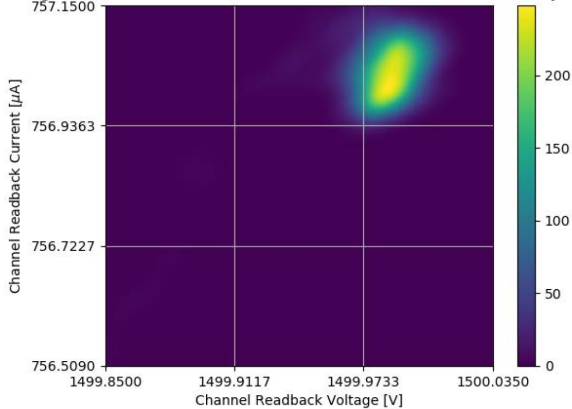
Voltage and Current Readback for Module #338 Channel 08 Stability Test
