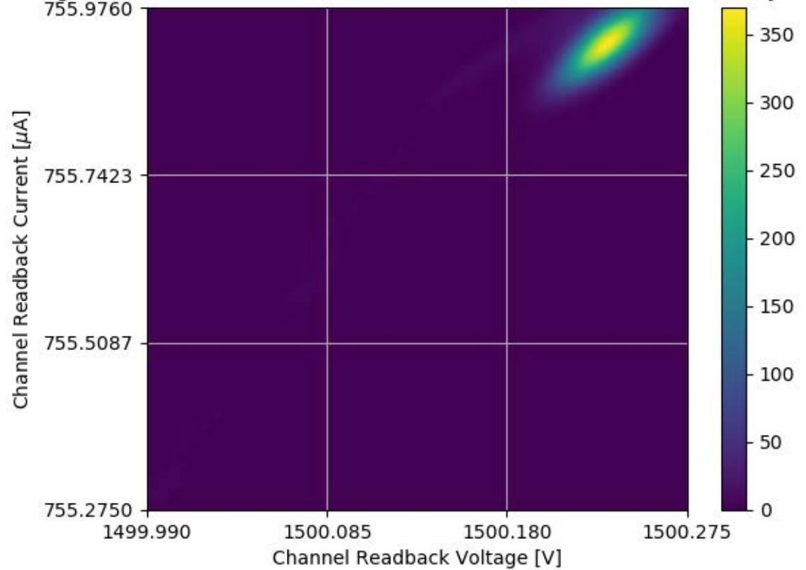
Voltage and Current Readback for Module #338 Channel 01 Stability Test
