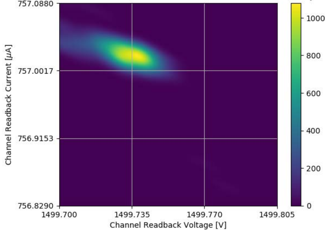
Voltage and Current Readback for Module #338 Channel 29 Stability Test
