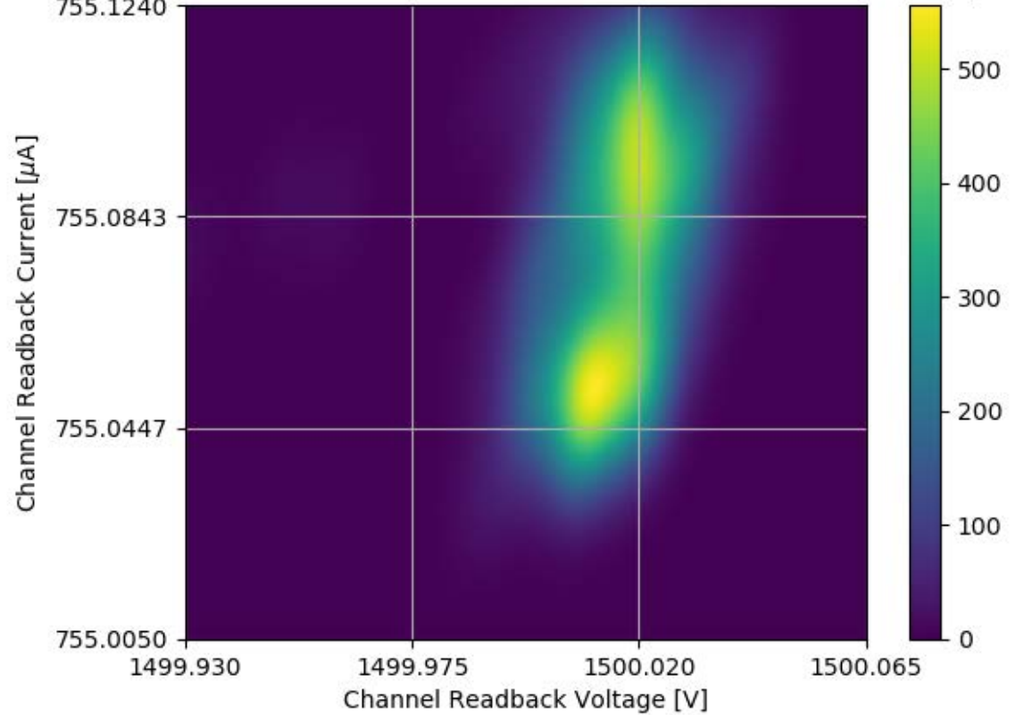
Voltage and Current Readback for Module #338 Channel 30 Stability Test
