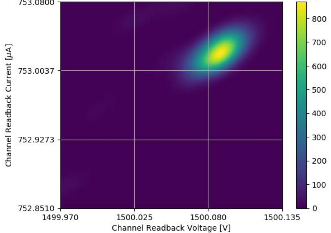
Voltage and Current Readback for Module #338 Channel 11 Stability Test
