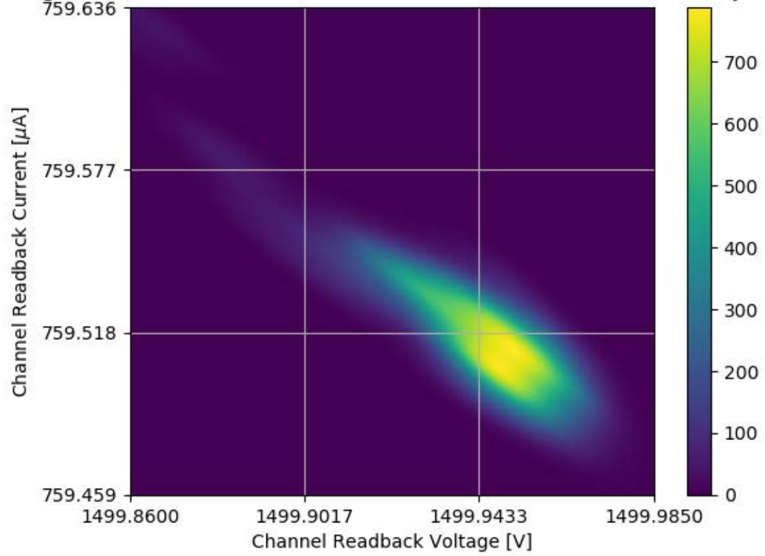
Voltage and Current Readback for Module #338 Channel 22 Stability Test
