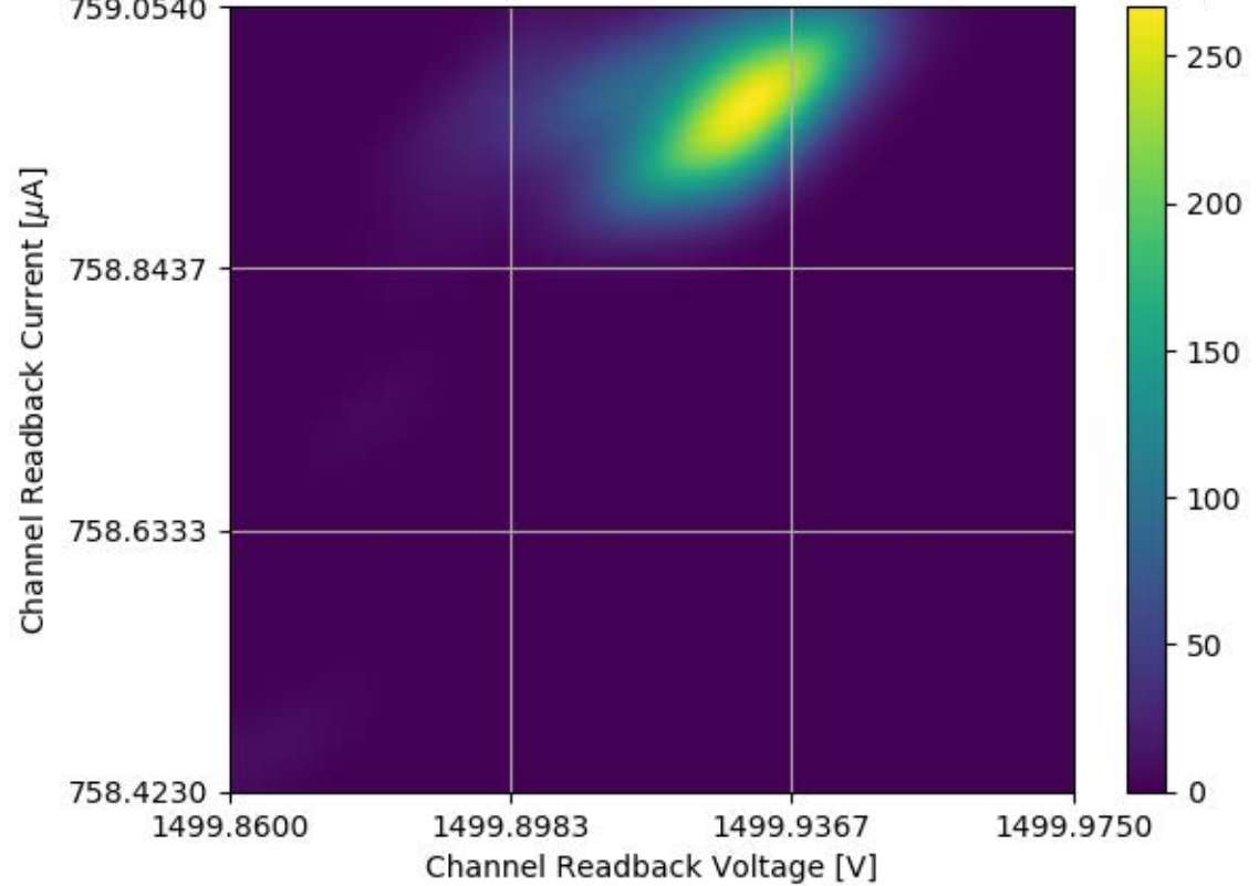
Voltage and Current Readback for Module #338 Channel 10 Stability Test
