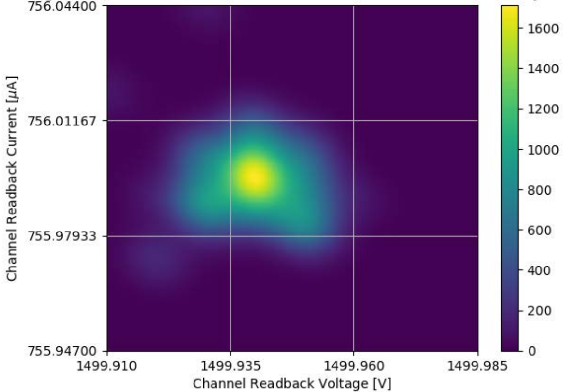
Voltage and Current Readback for Module #338 Channel 15 Stability Test
