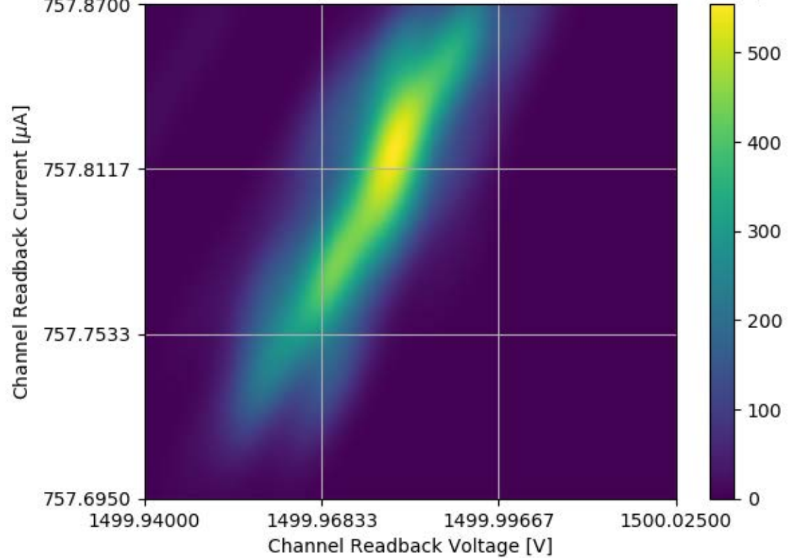
Voltage and Current Readback for Module #338 Channel 23 Stability Test
