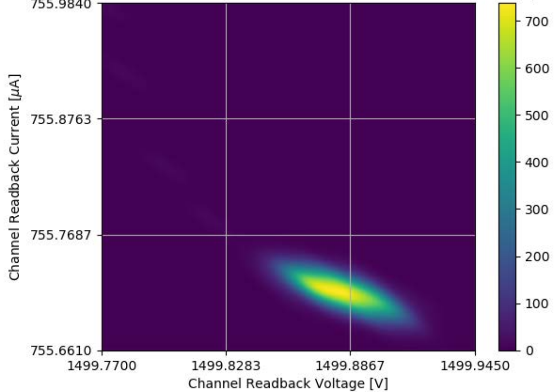
Voltage and Current Readback for Module #339 Channel 07 Stability Test
