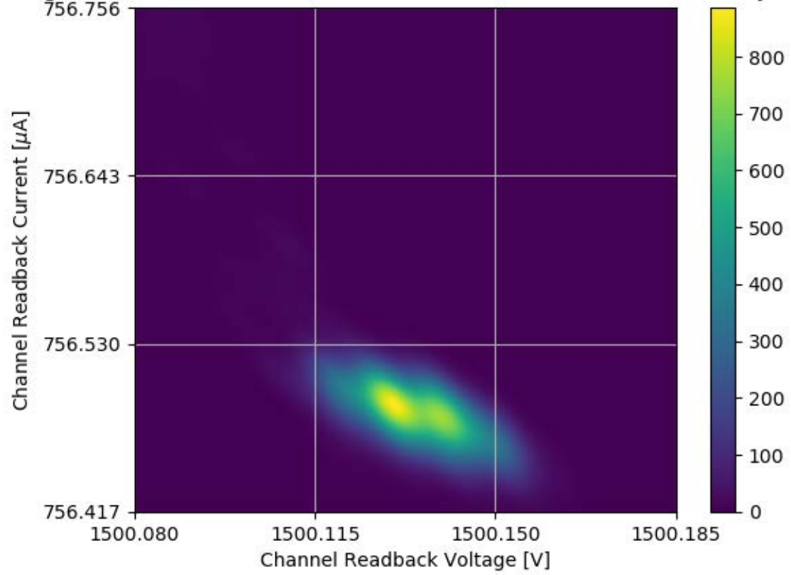
Voltage and Current Readback for Module #339 Channel 15 Stability Test
