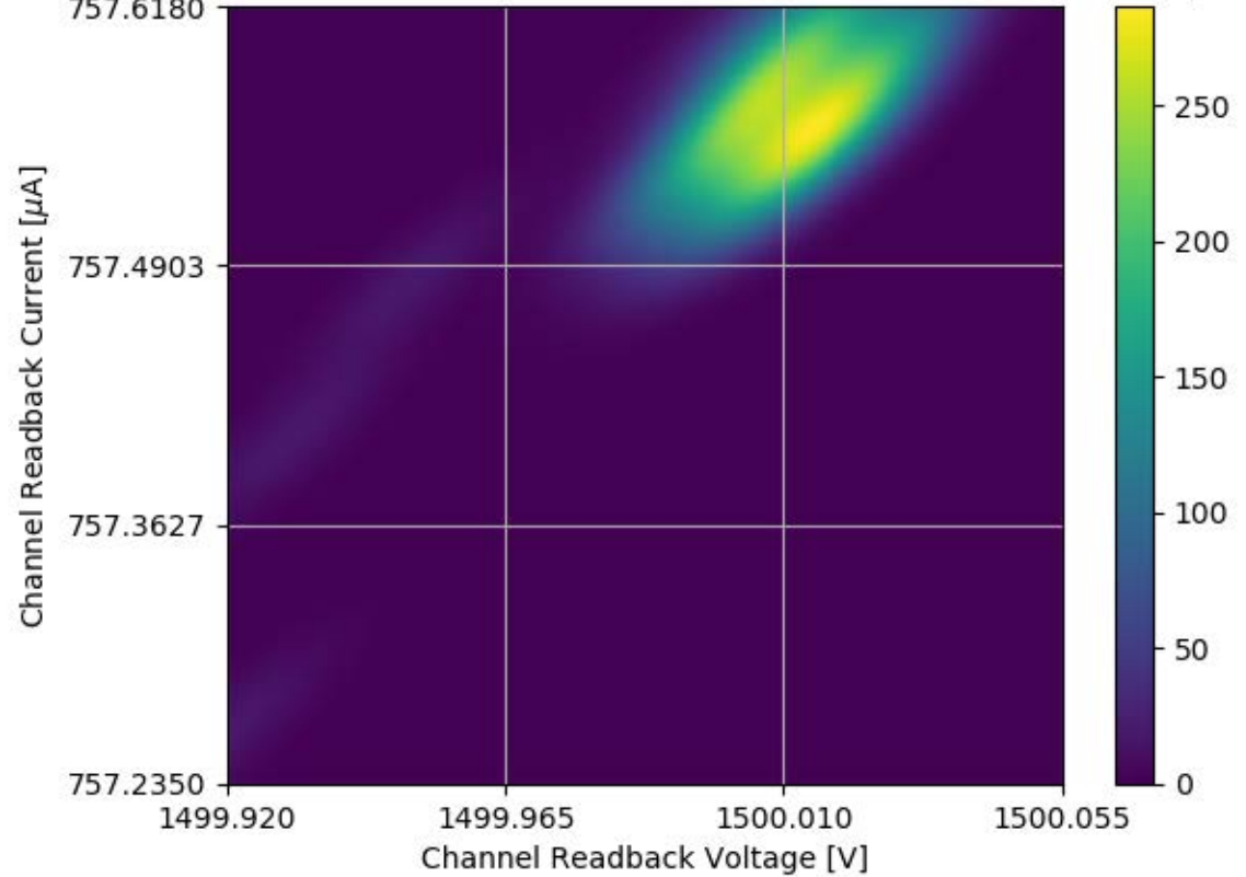
Voltage and Current Readback for Module #339 Channel 26 Stability Test
