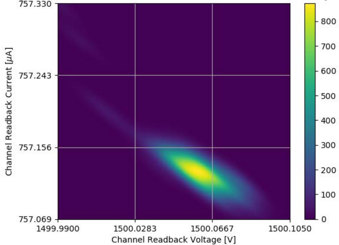
Voltage and Current Readback for Module #339 Channel 19 Stability Test
