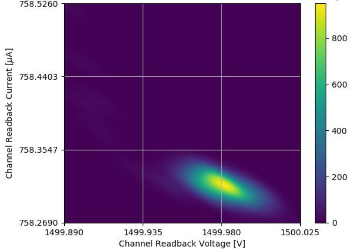
Voltage and Current Readback for Module #339 Channel 04 Stability Test
