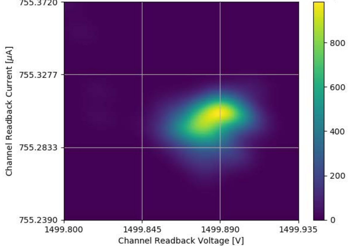
Voltage and Current Readback for Module #339 Channel 01 Stability Test
