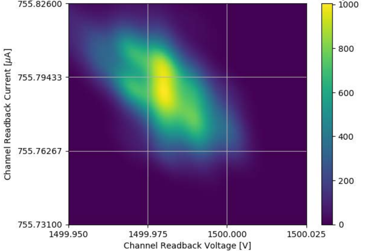
Voltage and Current Readback for Module #339 Channel 02 Stability Test
