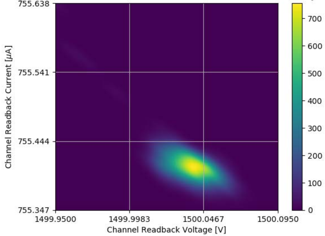
Voltage and Current Readback for Module #339 Channel 30 Stability Test
