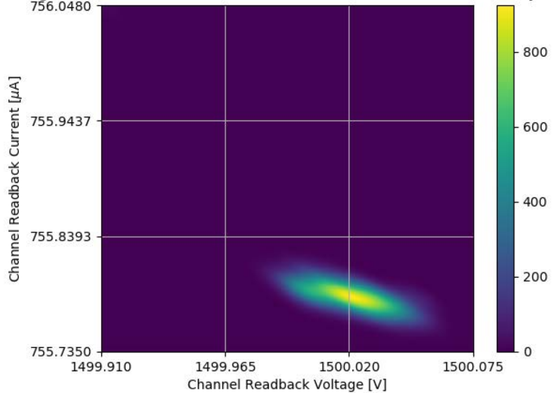
Voltage and Current Readback for Module #339 Channel 28 Stability Test
