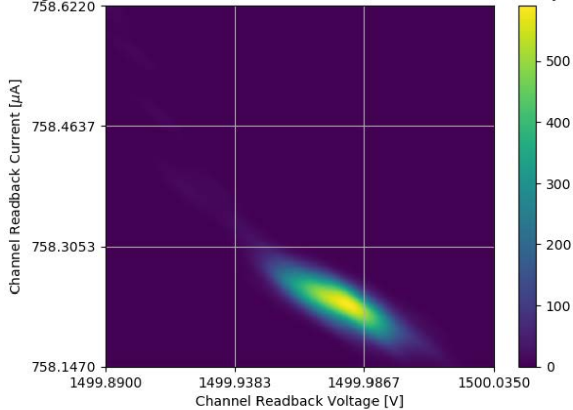
Voltage and Current Readback for Module #339 Channel 21 Stability Test
