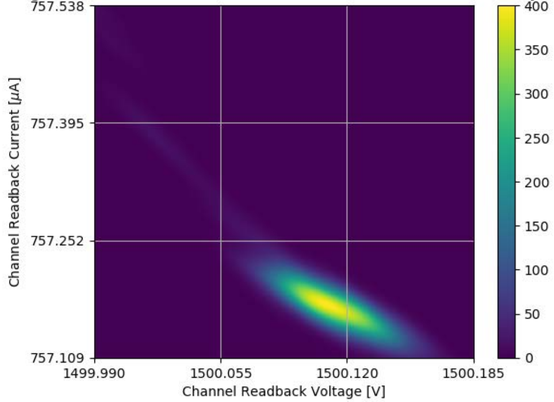
Voltage and Current Readback for Module #339 Channel 32 Stability Test
