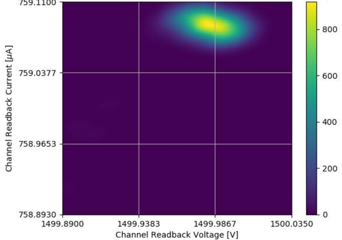
Voltage and Current Readback for Module #339 Channel 24 Stability Test
