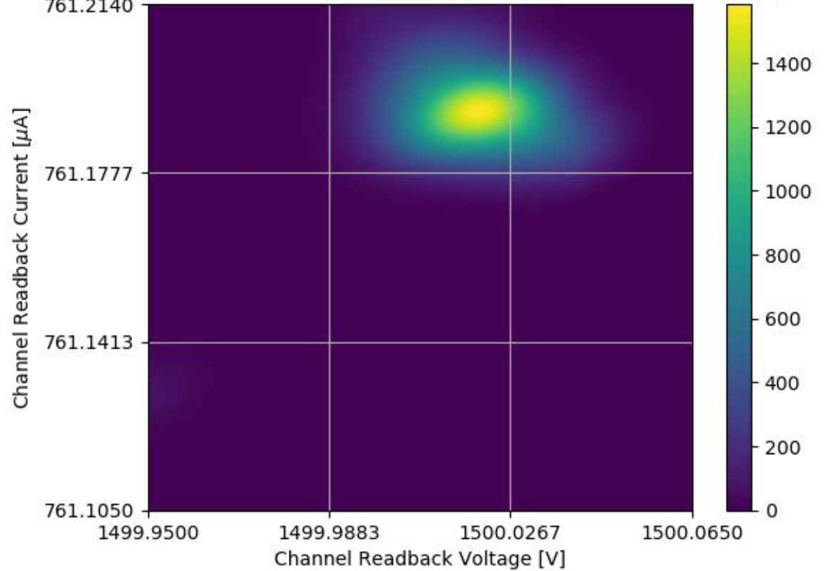
Voltage and Current Readback for Module #339 Channel 09 Stability Test
