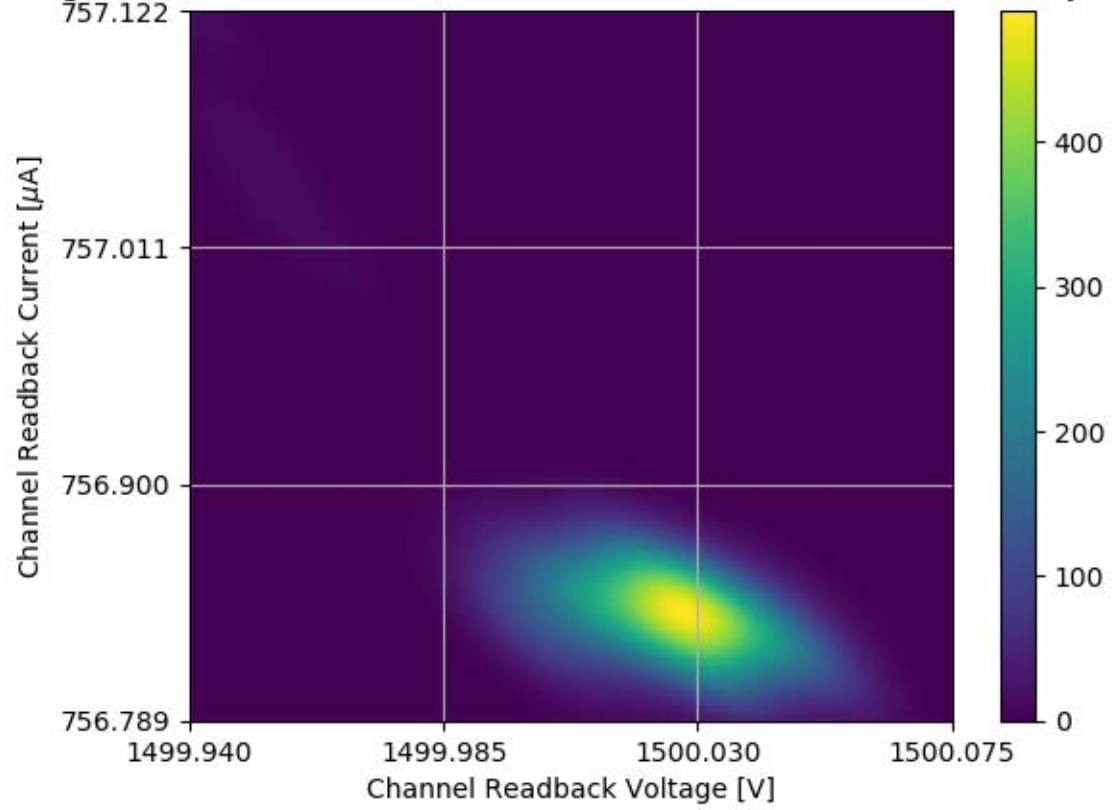
Voltage and Current Readback for Module #339 Channel 29 Stability Test
