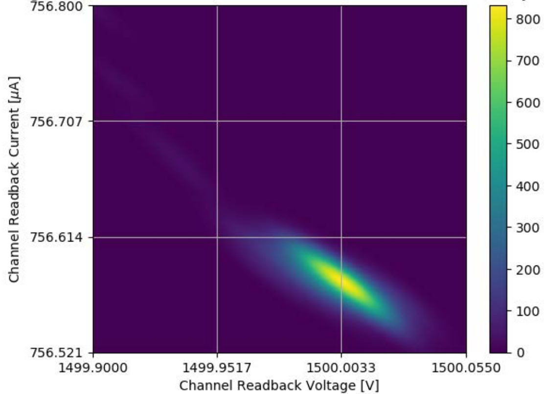
Voltage and Current Readback for Module #339 Channel 27 Stability Test
