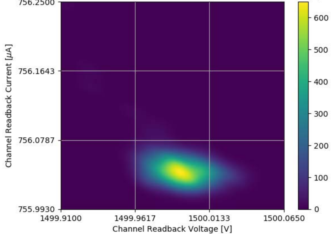
Voltage and Current Readback for Module #339 Channel 34 Stability Test
