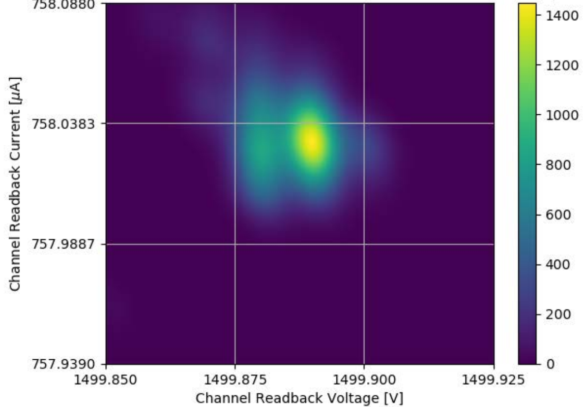
Voltage and Current Readback for Module #339 Channel 25 Stability Test
