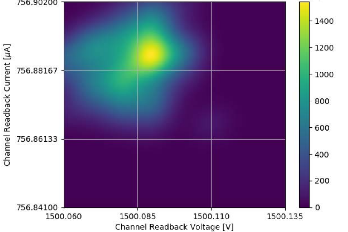
Voltage and Current Readback for Module #339 Channel 23 Stability Test
