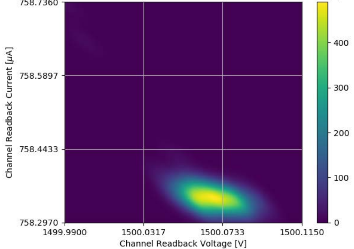
Voltage and Current Readback for Module #339 Channel 22 Stability Test
