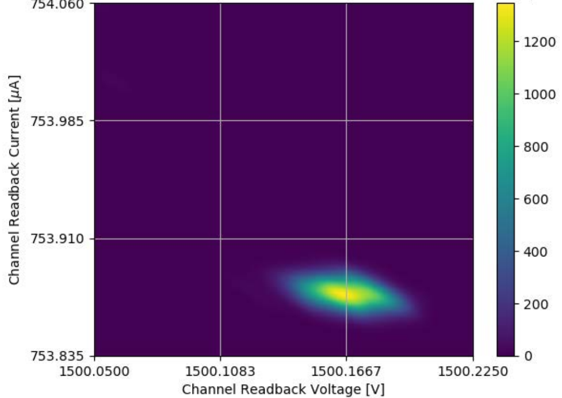
Voltage and Current Readback for Module #339 Channel 11 Stability Test
