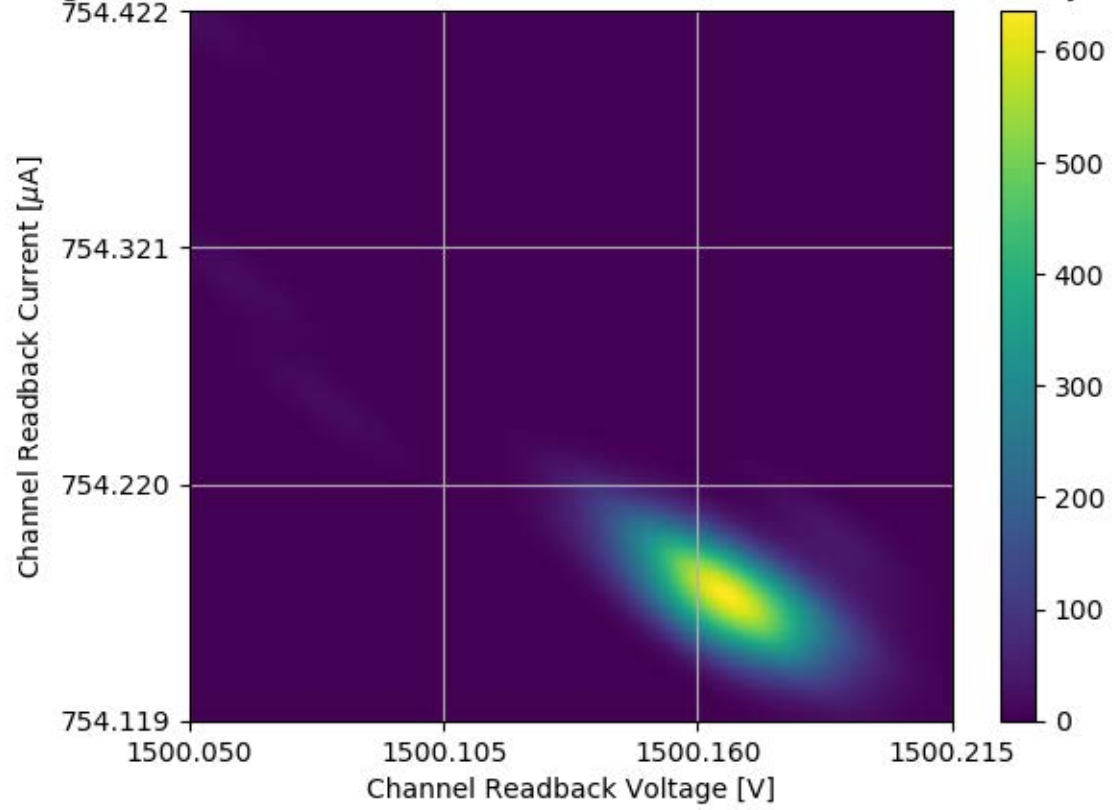
Voltage and Current Readback for Module #339 Channel 00 Stability Test
