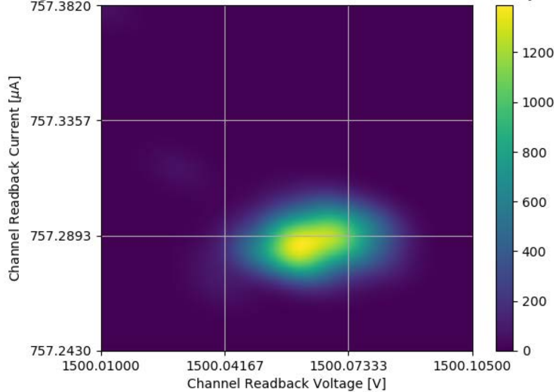
Voltage and Current Readback for Module #339 Channel 35 Stability Test
