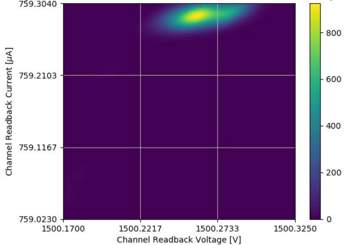
Voltage and Current Readback for Module #339 Channel 10 Stability Test
