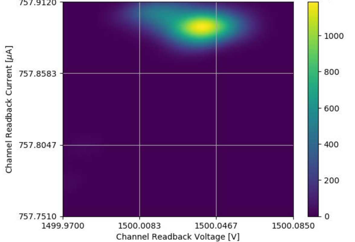
Voltage and Current Readback for Module #339 Channel 08 Stability Test
