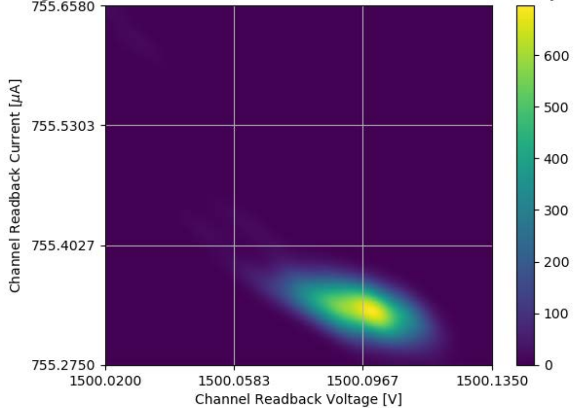
Voltage and Current Readback for Module #339 Channel 14 Stability Test
