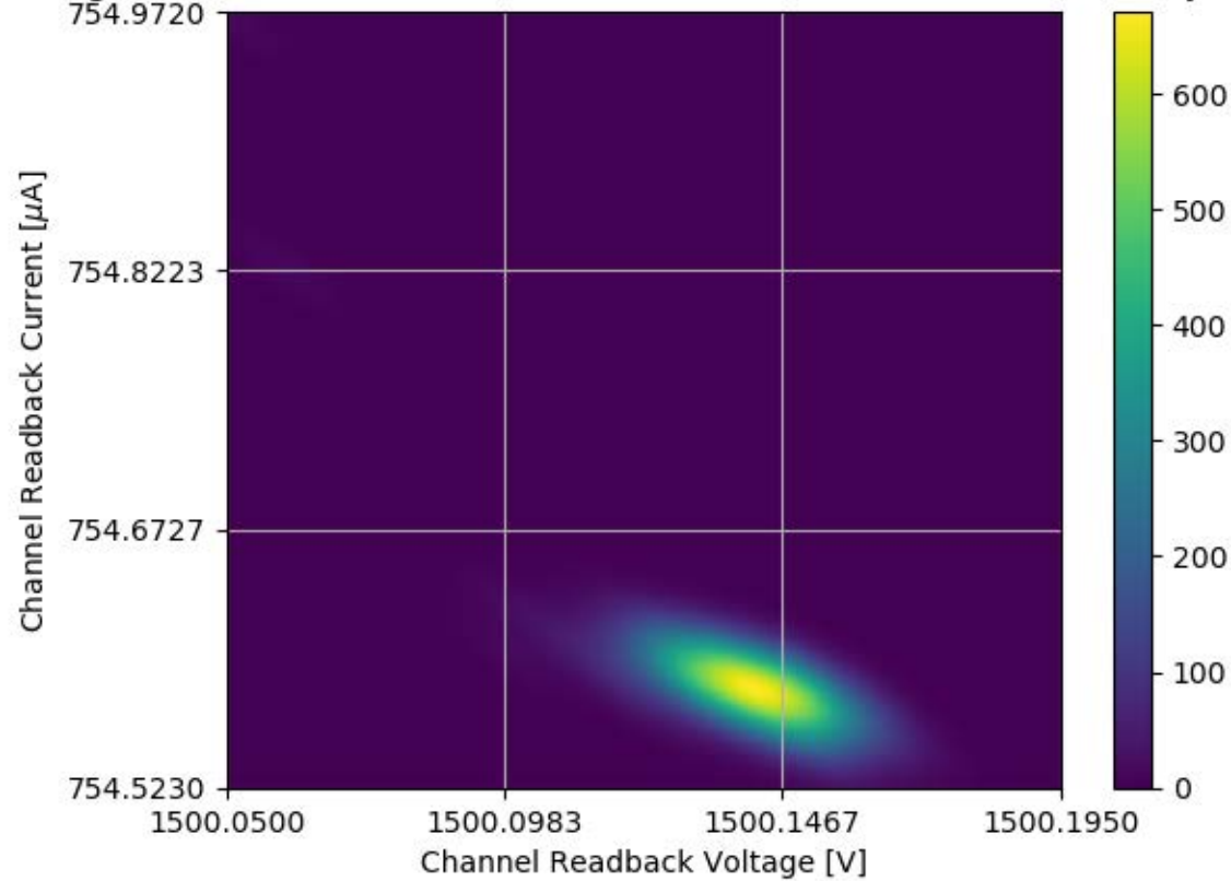
Voltage and Current Readback for Module #339 Channel 13 Stability Test
