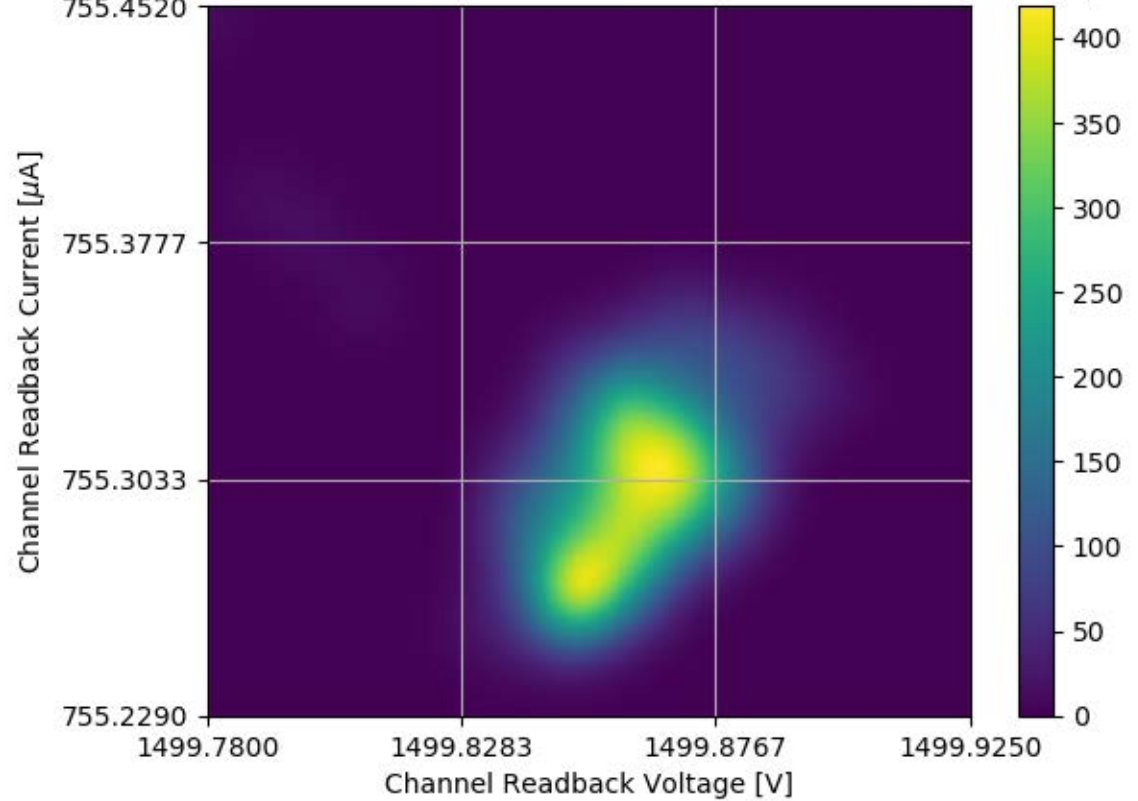
Voltage and Current Readback for Module #339 Channel 17 Stability Test
