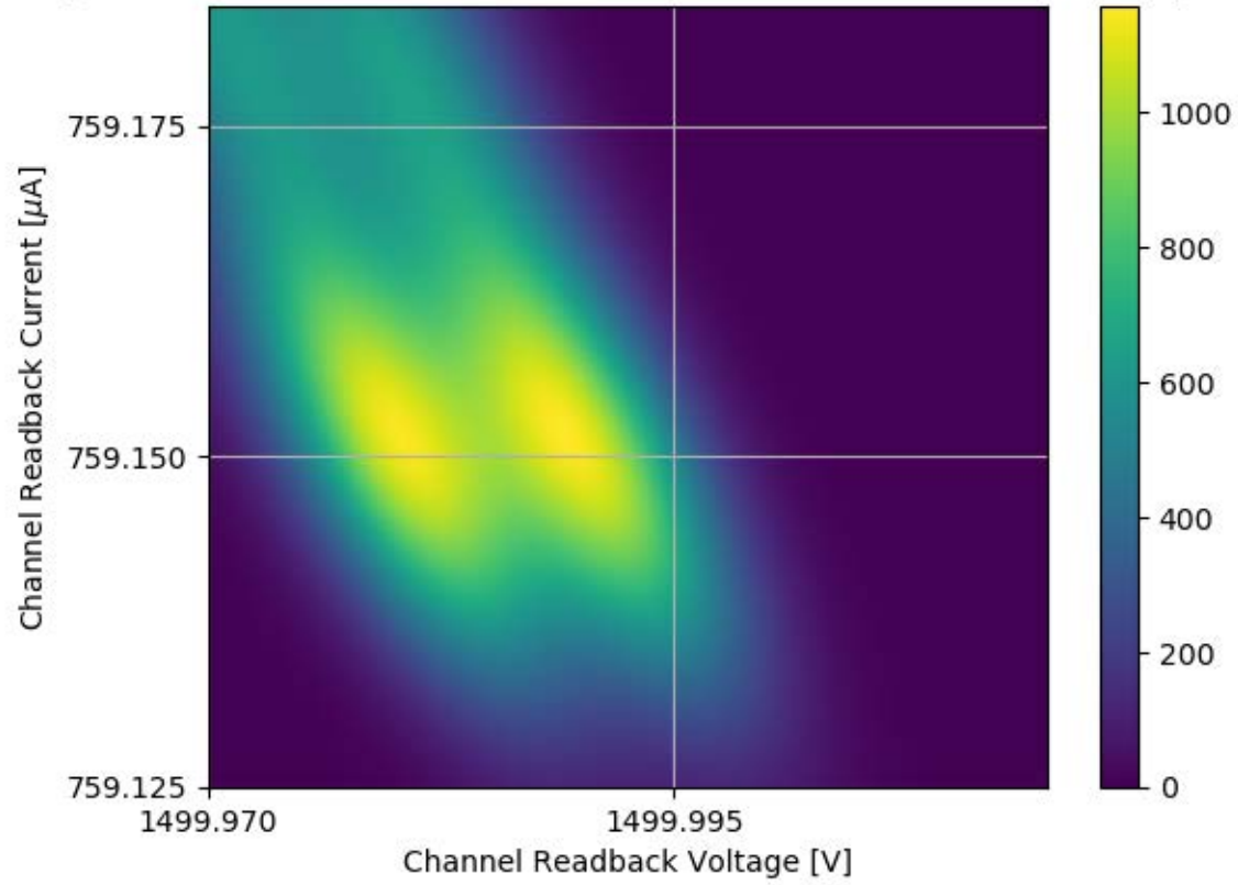
Voltage and Current Readback for Module #347 Channel 06 Stability Test
