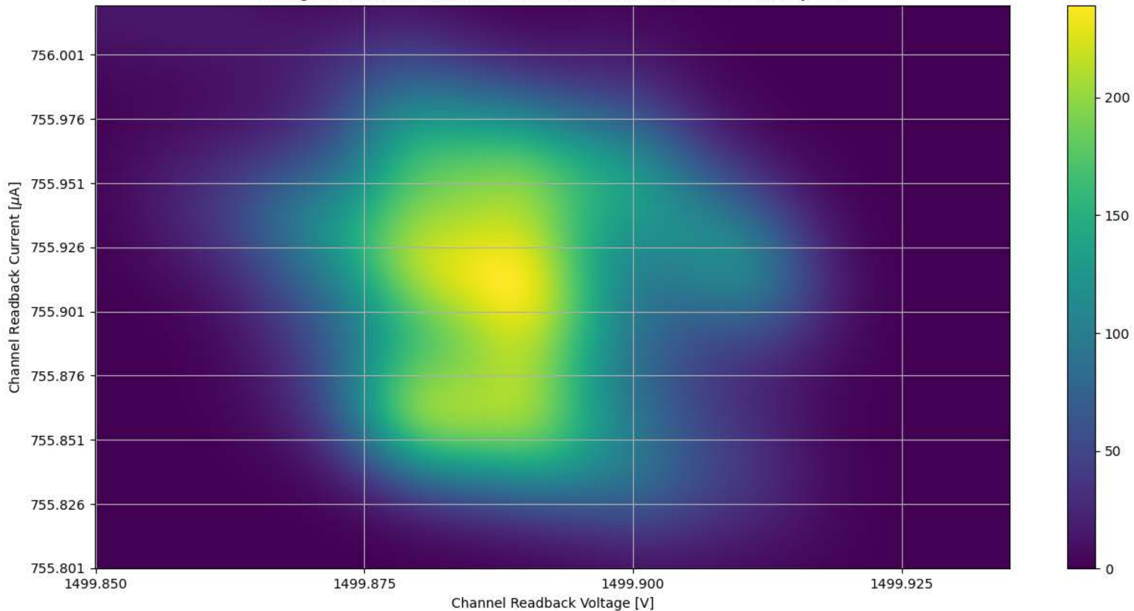
Voltage and Current Readback for Module #349 Channel 27 Stability Test
