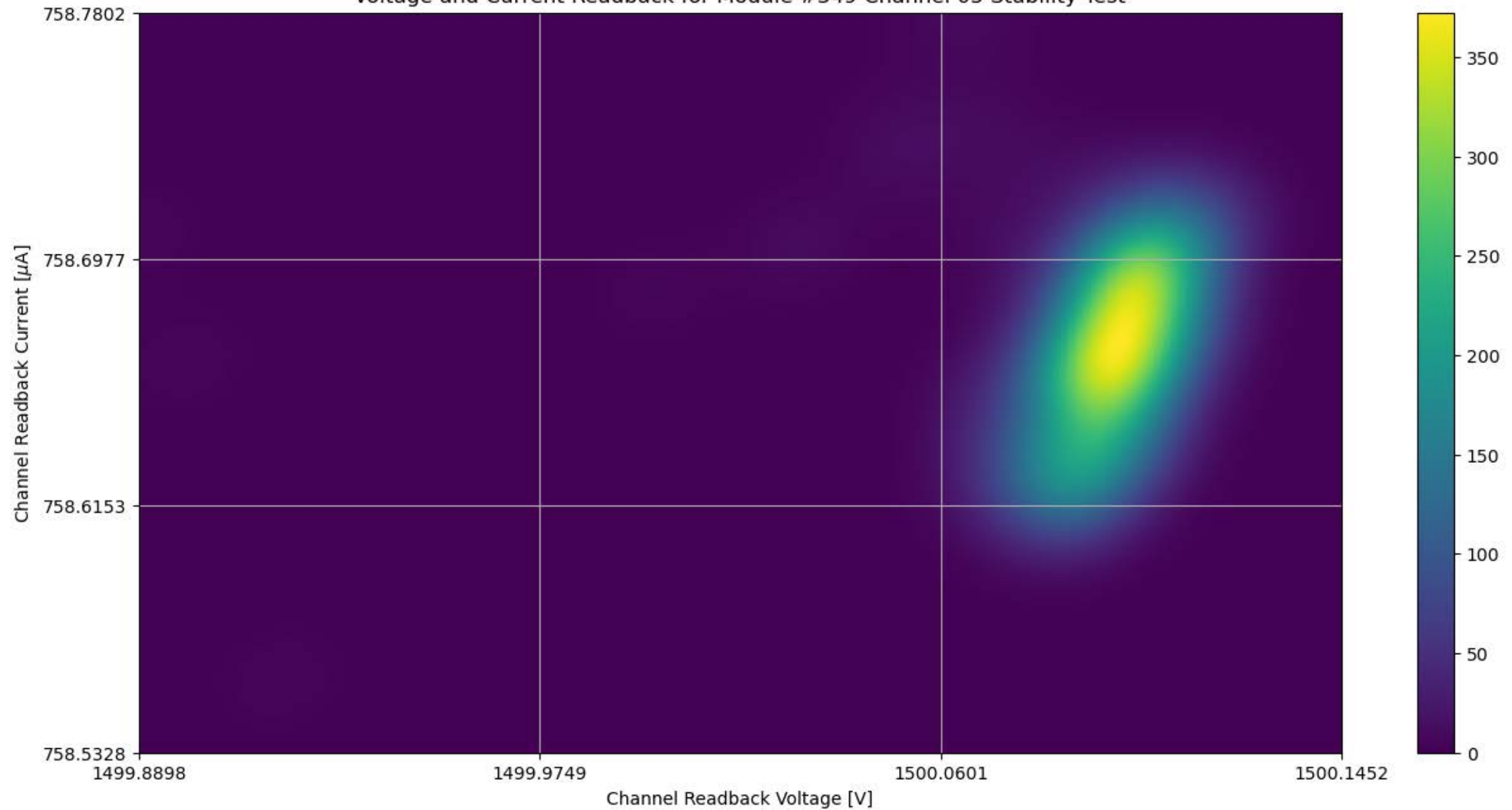
Voltage and Current Readback for Module #349 Channel 05 Stability Test
