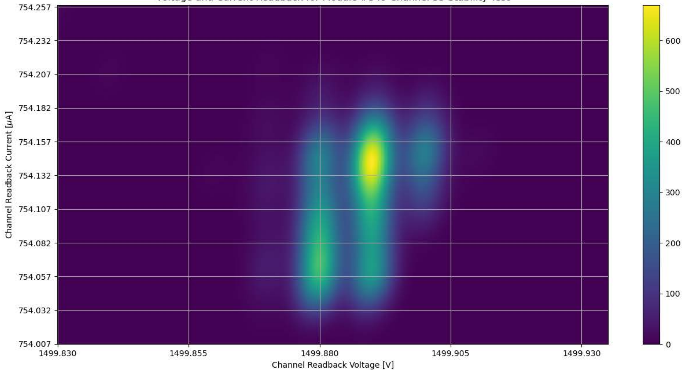
Voltage and Current Readback for Module #349 Channel 33 Stability Test
