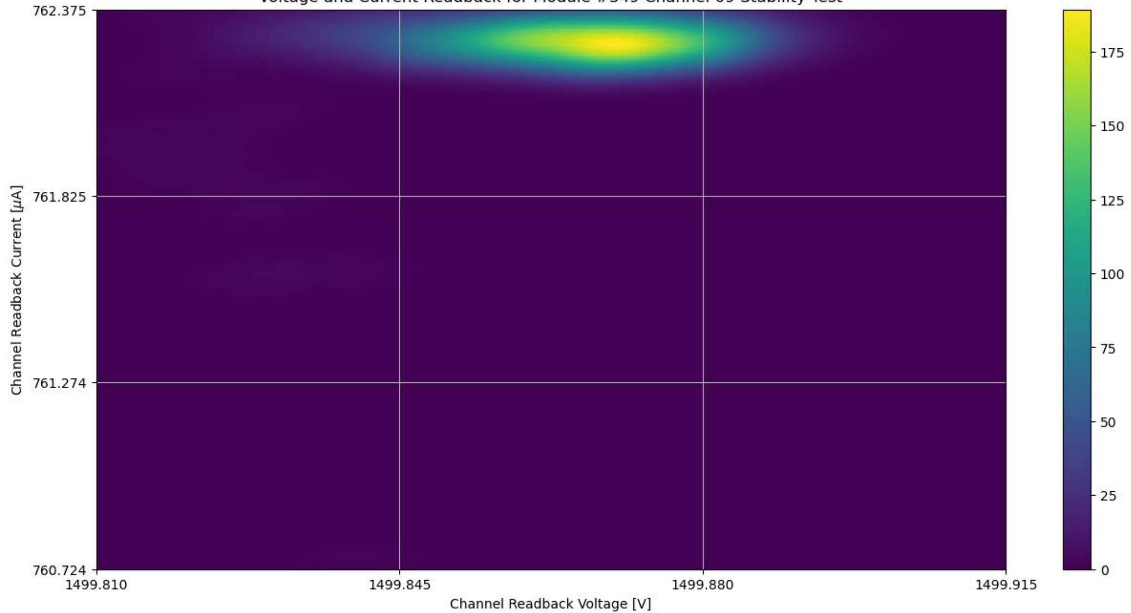
Voltage and Current Readback for Module #349 Channel 09 Stability Test
