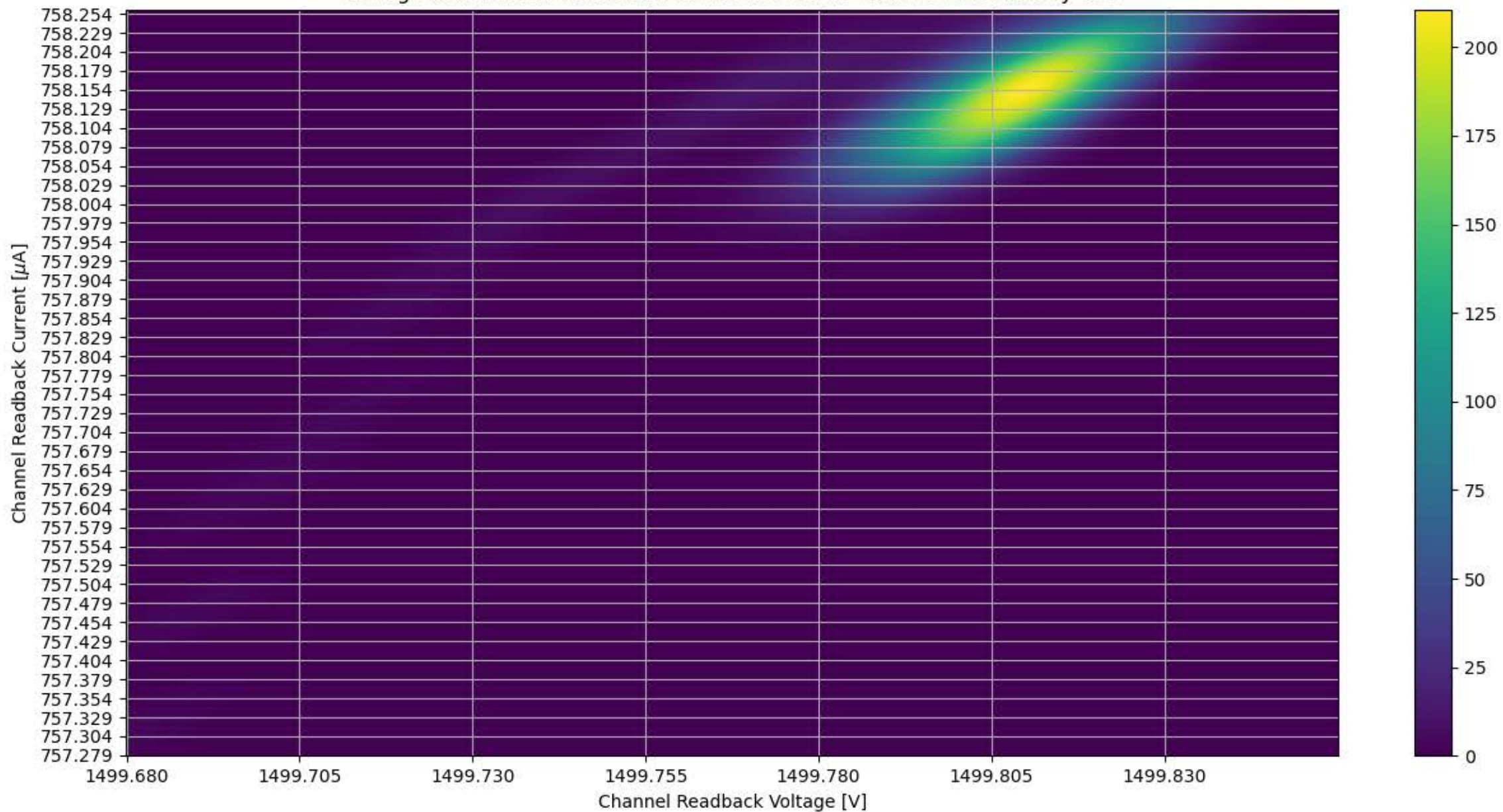
Voltage and Current Readback for Module #349 Channel 24 Stability Test
