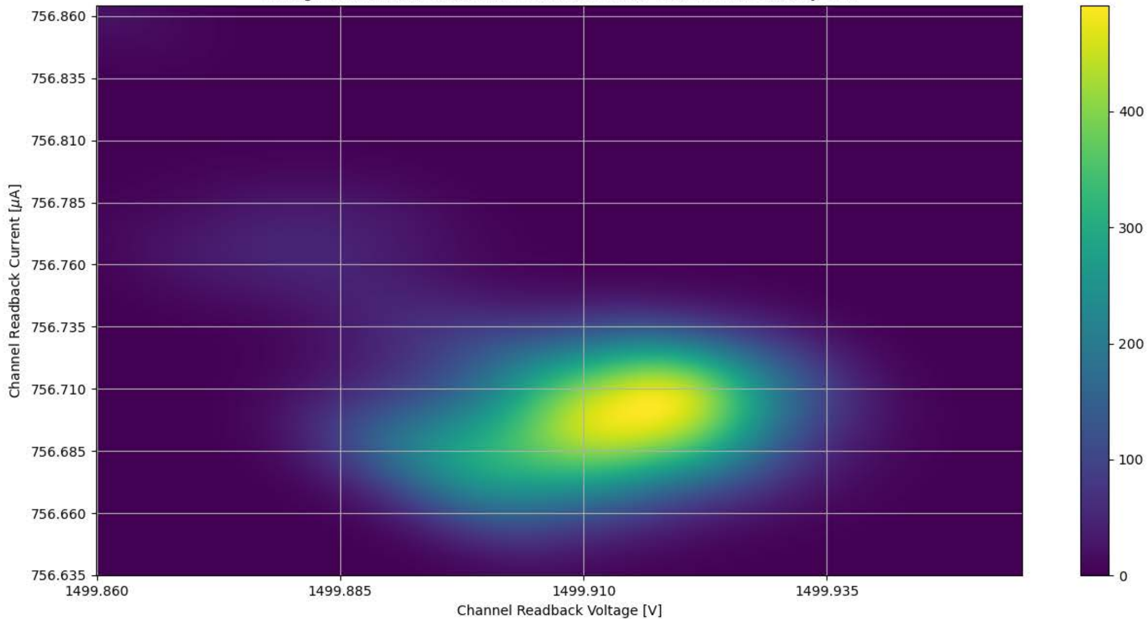
Voltage and Current Readback for Module #349 Channel 20 Stability Test
