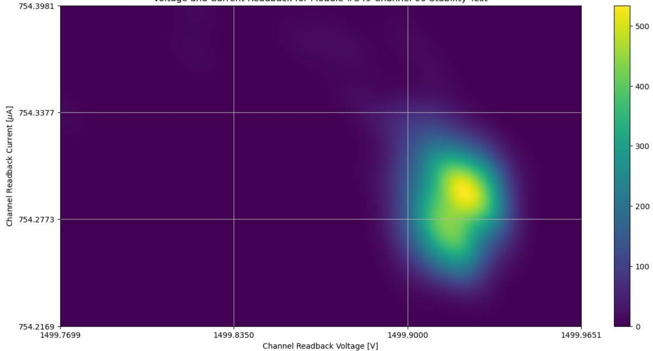
Voltage and Current Readback for Module #349 Channel 00 Stability Test
