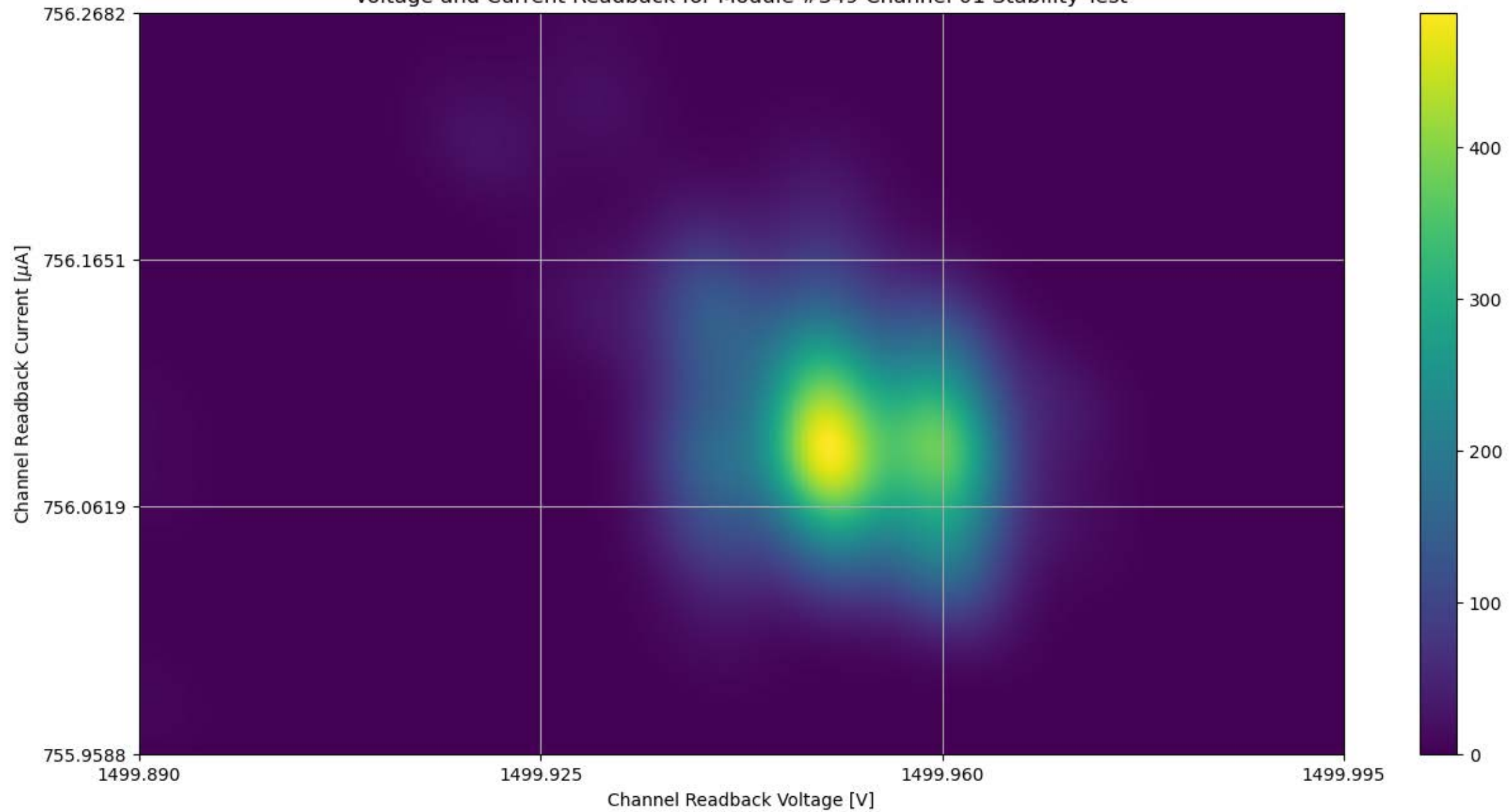
Voltage and Current Readback for Module #349 Channel 01 Stability Test
