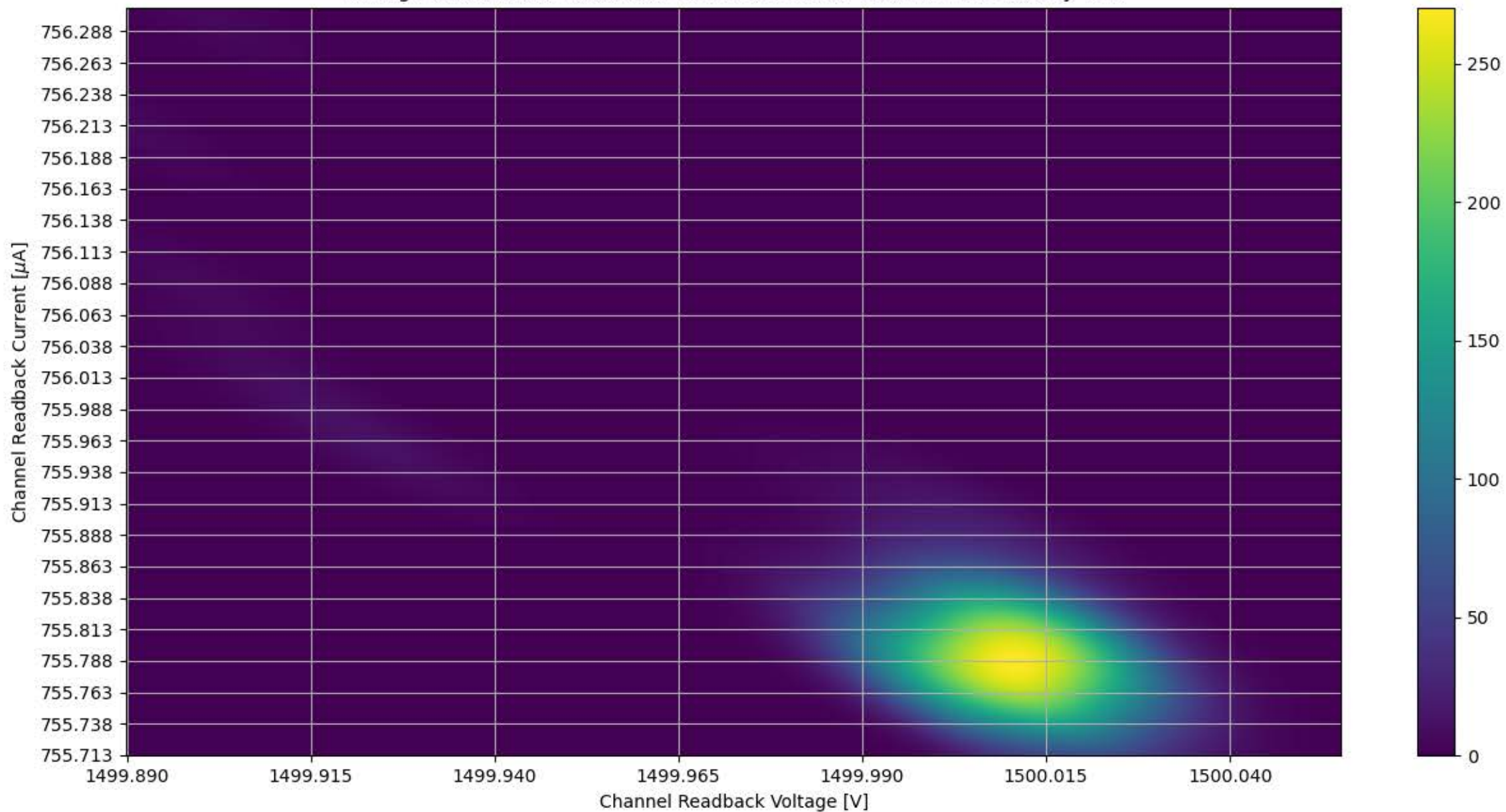
Voltage and Current Readback for Module #349 Channel 18 Stability Test
