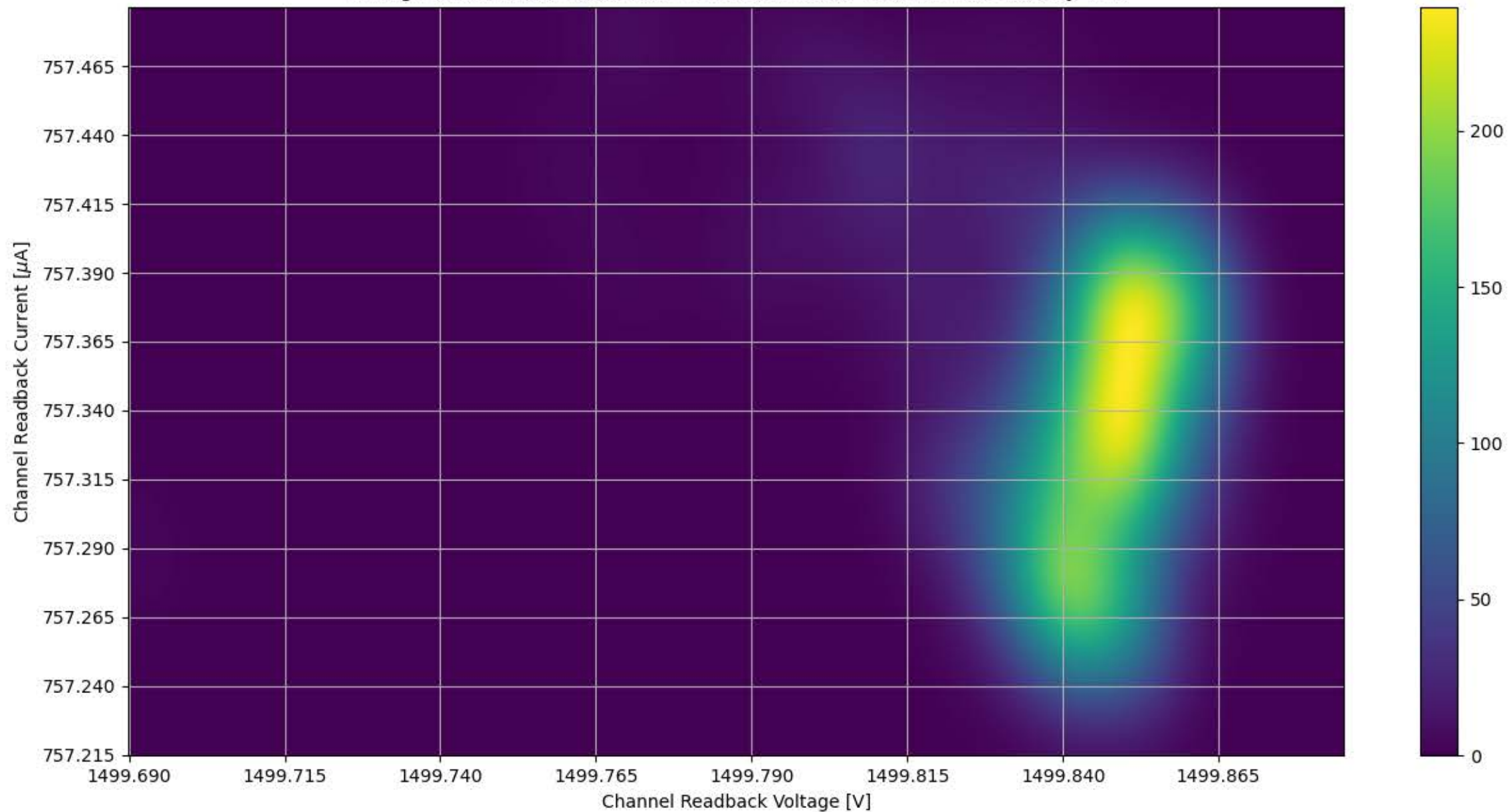
Voltage and Current Readback for Module #349 Channel 16 Stability Test
