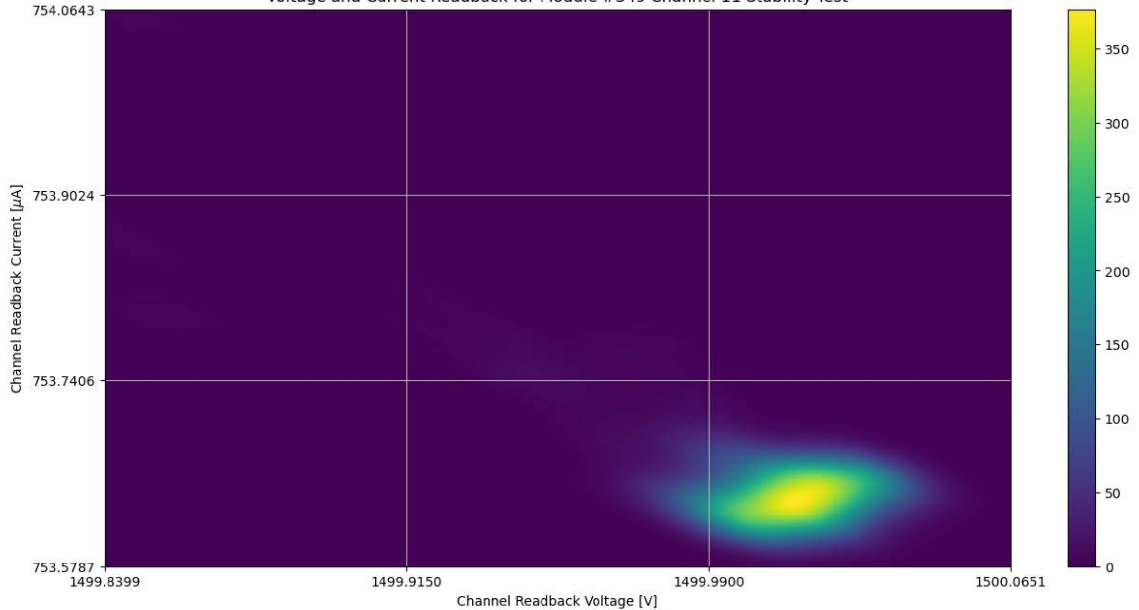
Voltage and Current Readback for Module #349 Channel 11 Stability Test
