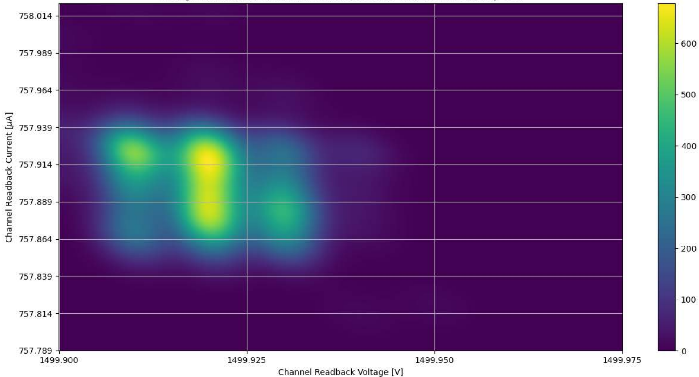
Voltage and Current Readback for Module #349 Channel 19 Stability Test
