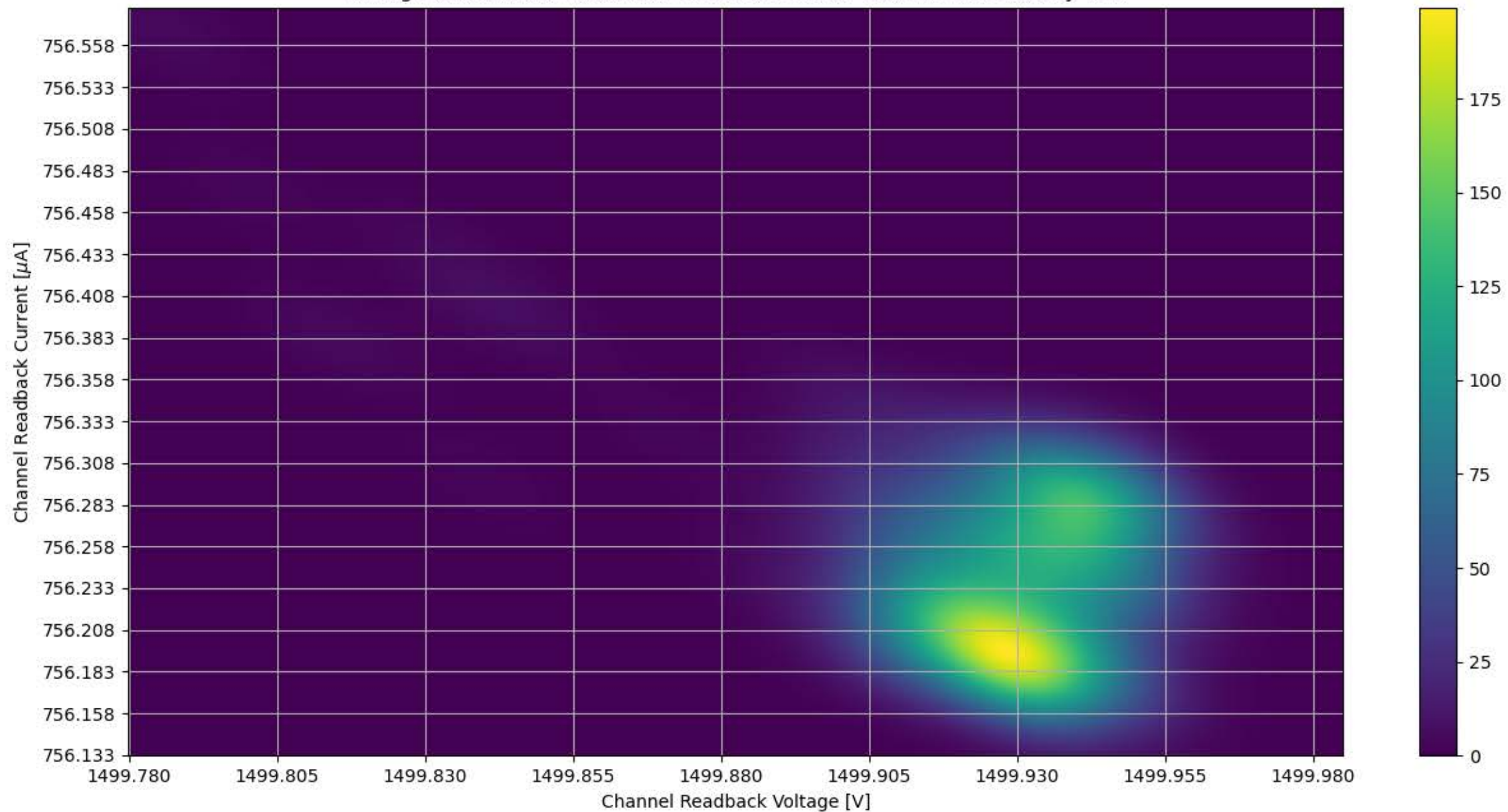
Voltage and Current Readback for Module #349 Channel 28 Stability Test
