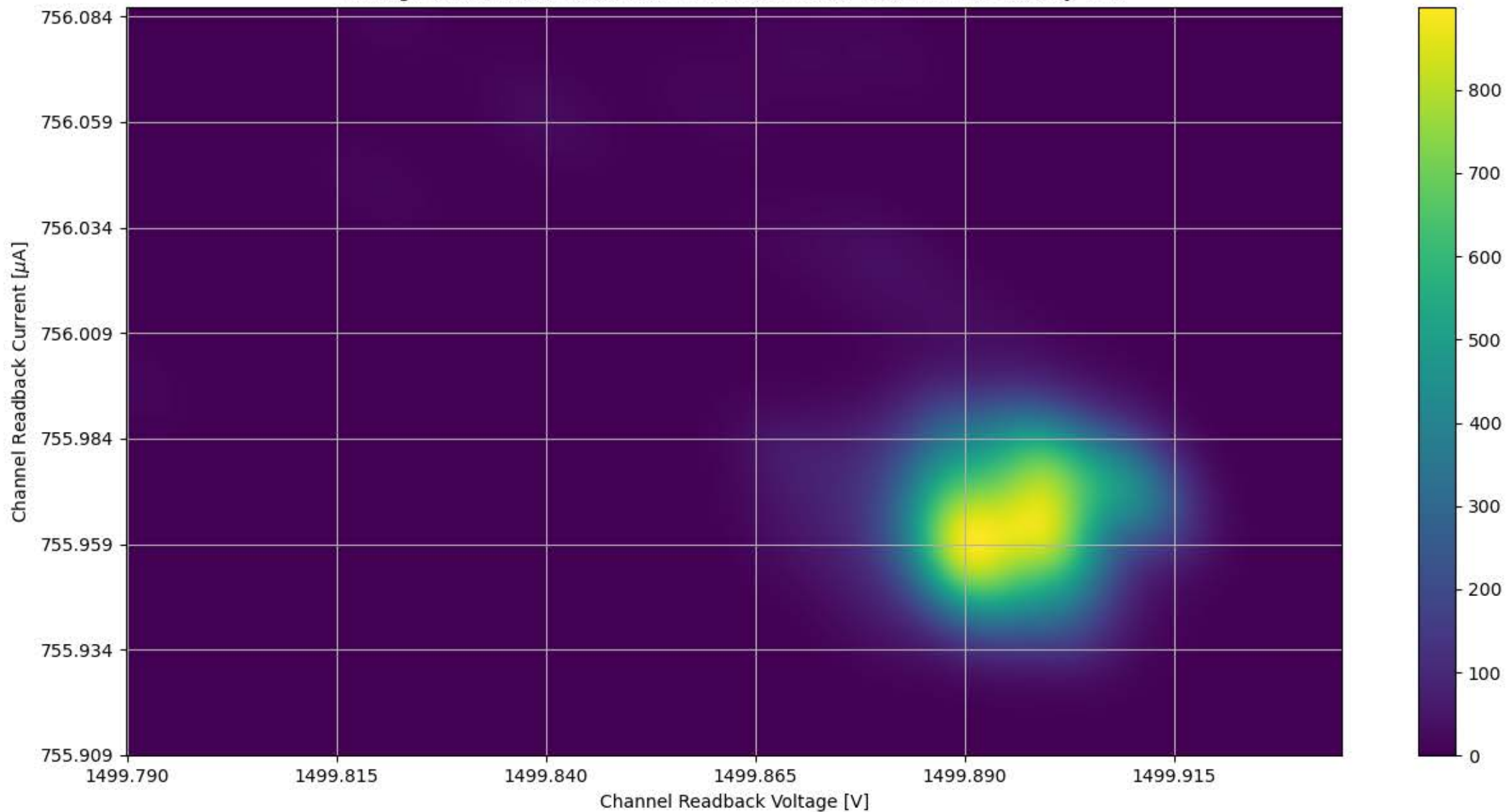
Voltage and Current Readback for Module #349 Channel 14 Stability Test
