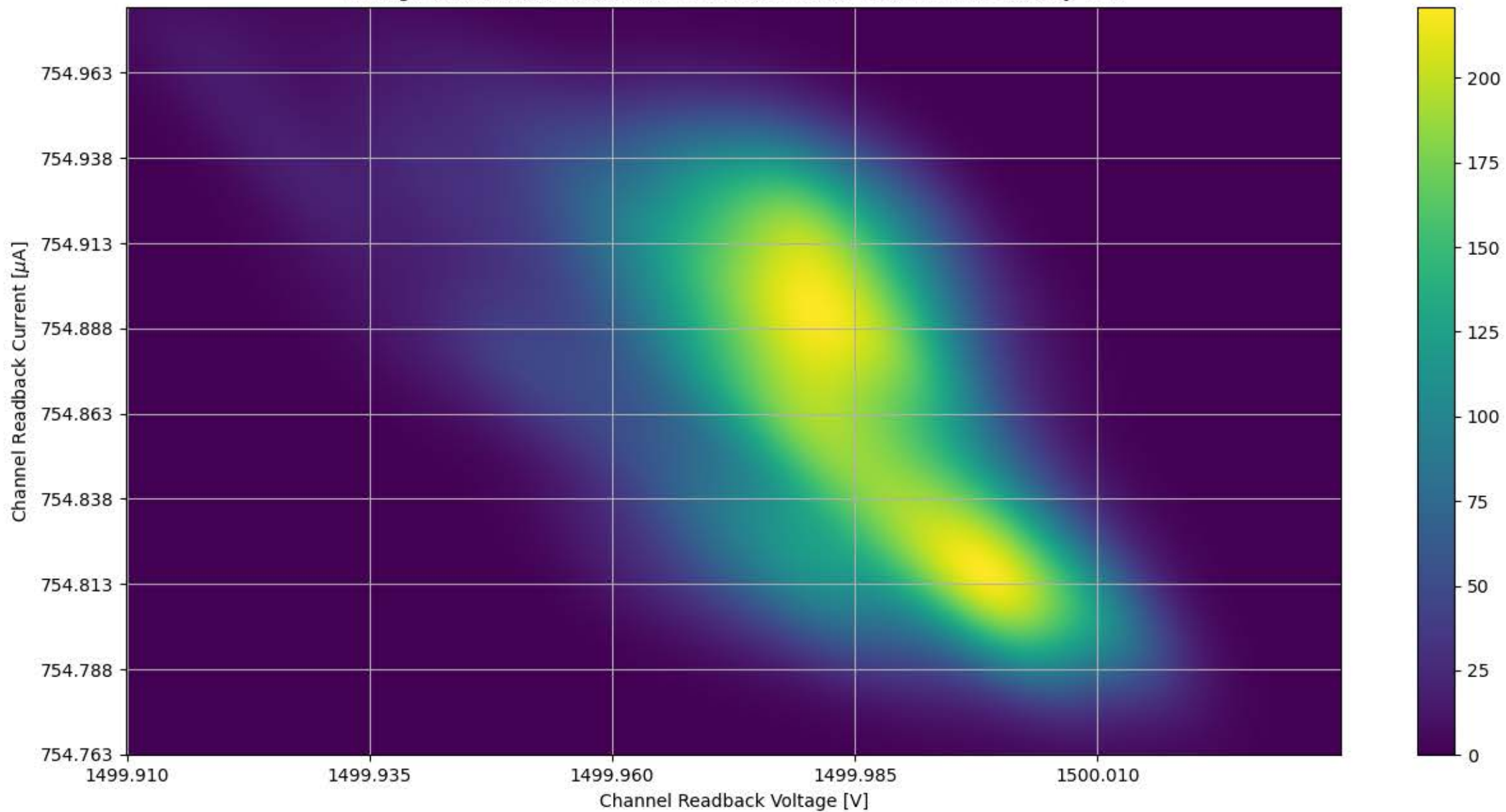
Voltage and Current Readback for Module #349 Channel 30 Stability Test
