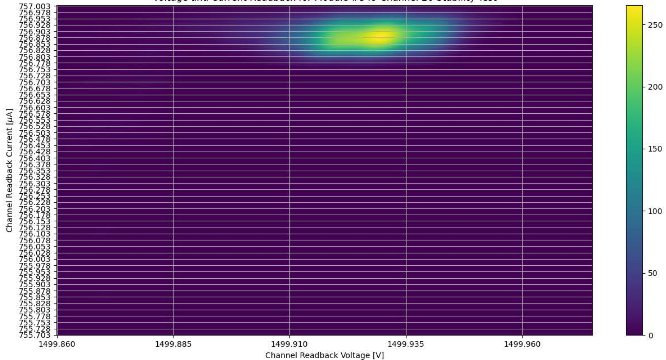
Voltage and Current Readback for Module #349 Channel 26 Stability Test
