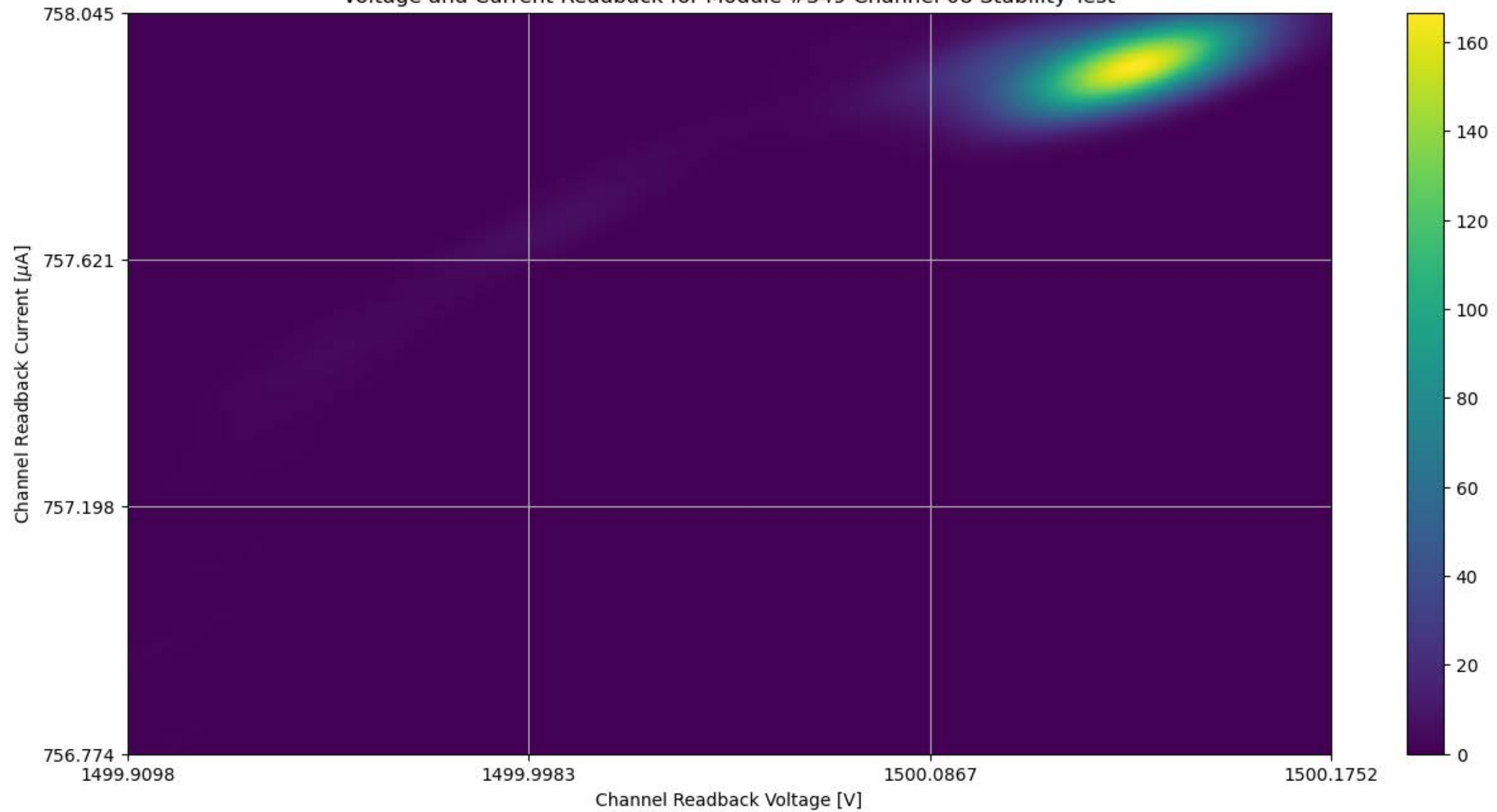
Voltage and Current Readback for Module #349 Channel 08 Stability Test
