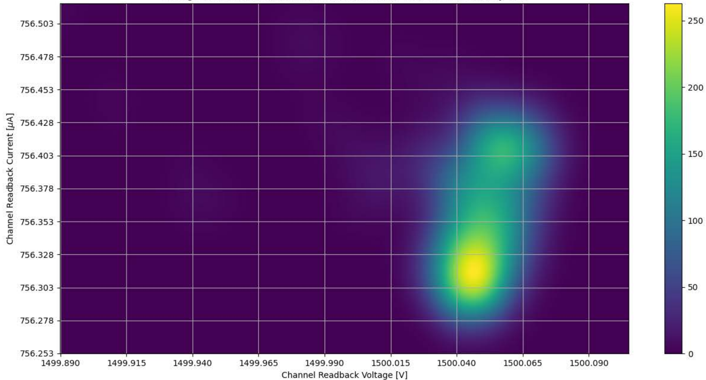
Voltage and Current Readback for Module #349 Channel 34 Stability Test
