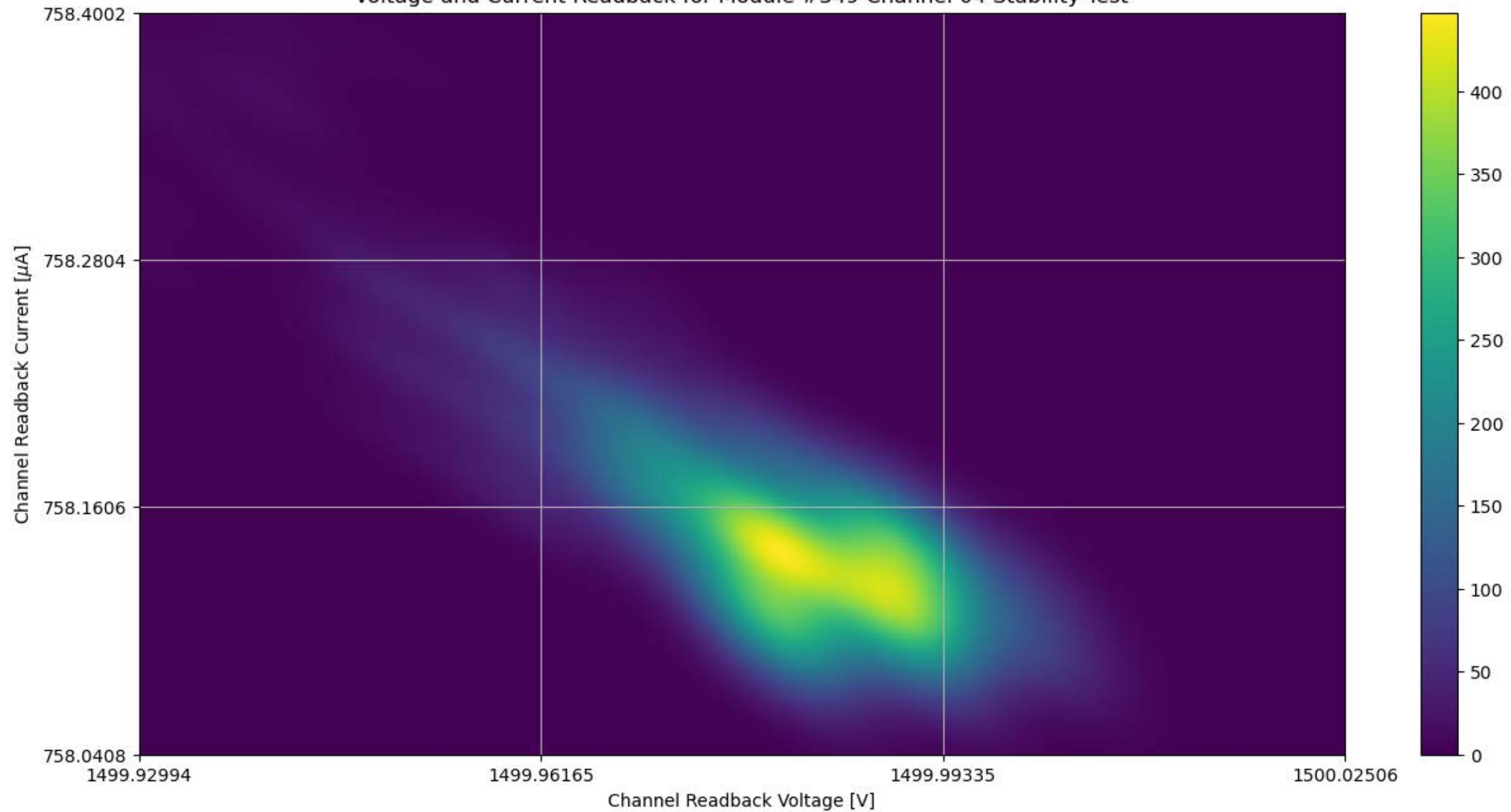
Voltage and Current Readback for Module #349 Channel 04 Stability Test
