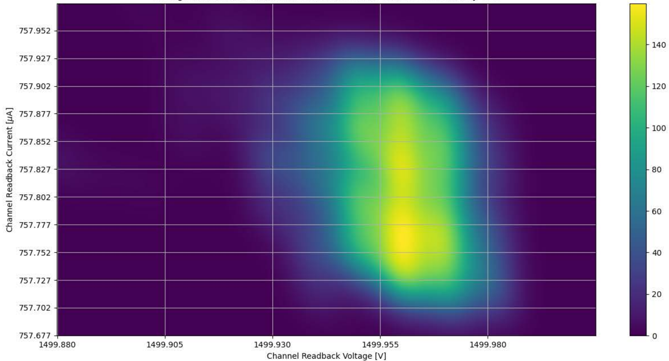
Voltage and Current Readback for Module #349 Channel 32 Stability Test
