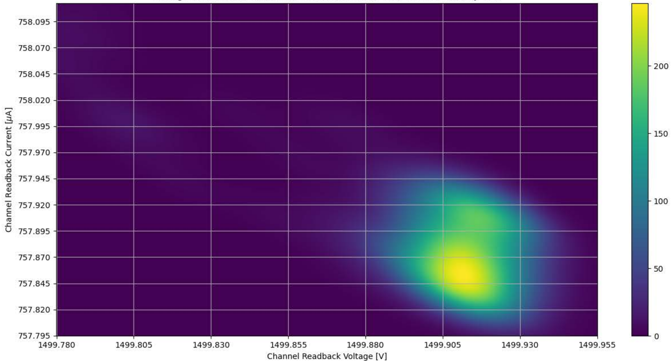
Voltage and Current Readback for Module #349 Channel 35 Stability Test
