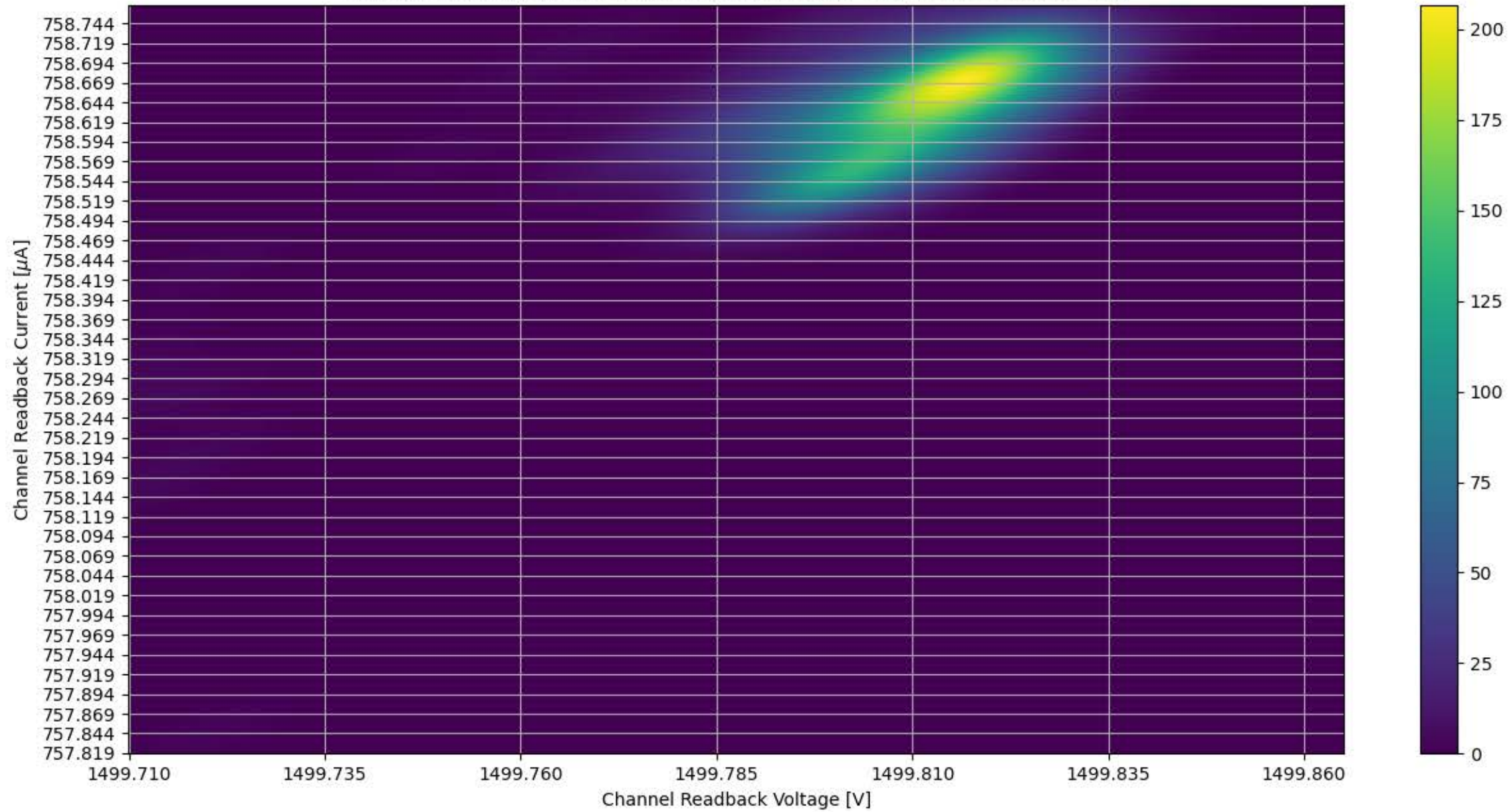
Voltage and Current Readback for Module #349 Channel 25 Stability Test
