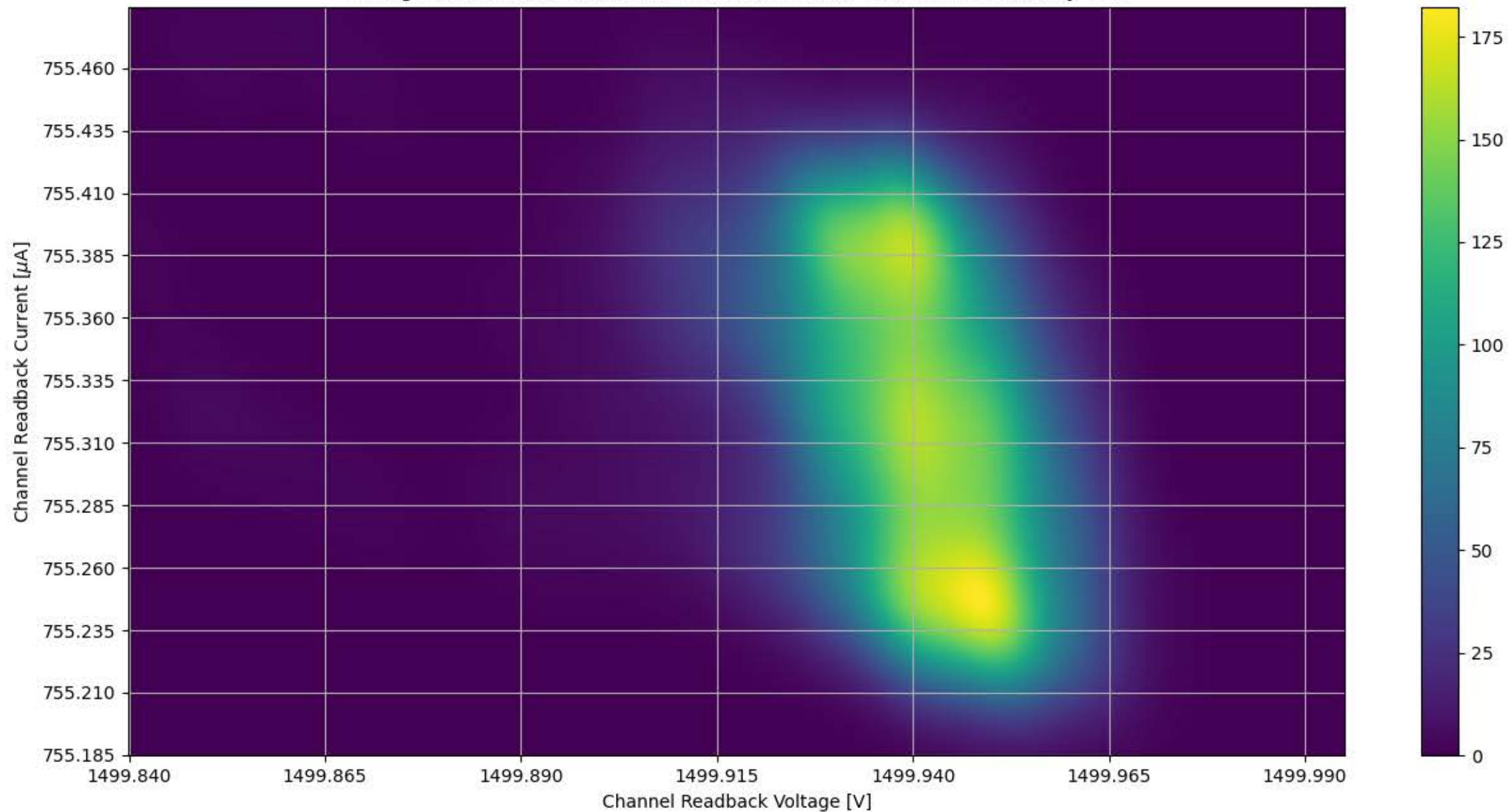
Voltage and Current Readback for Module #349 Channel 17 Stability Test
