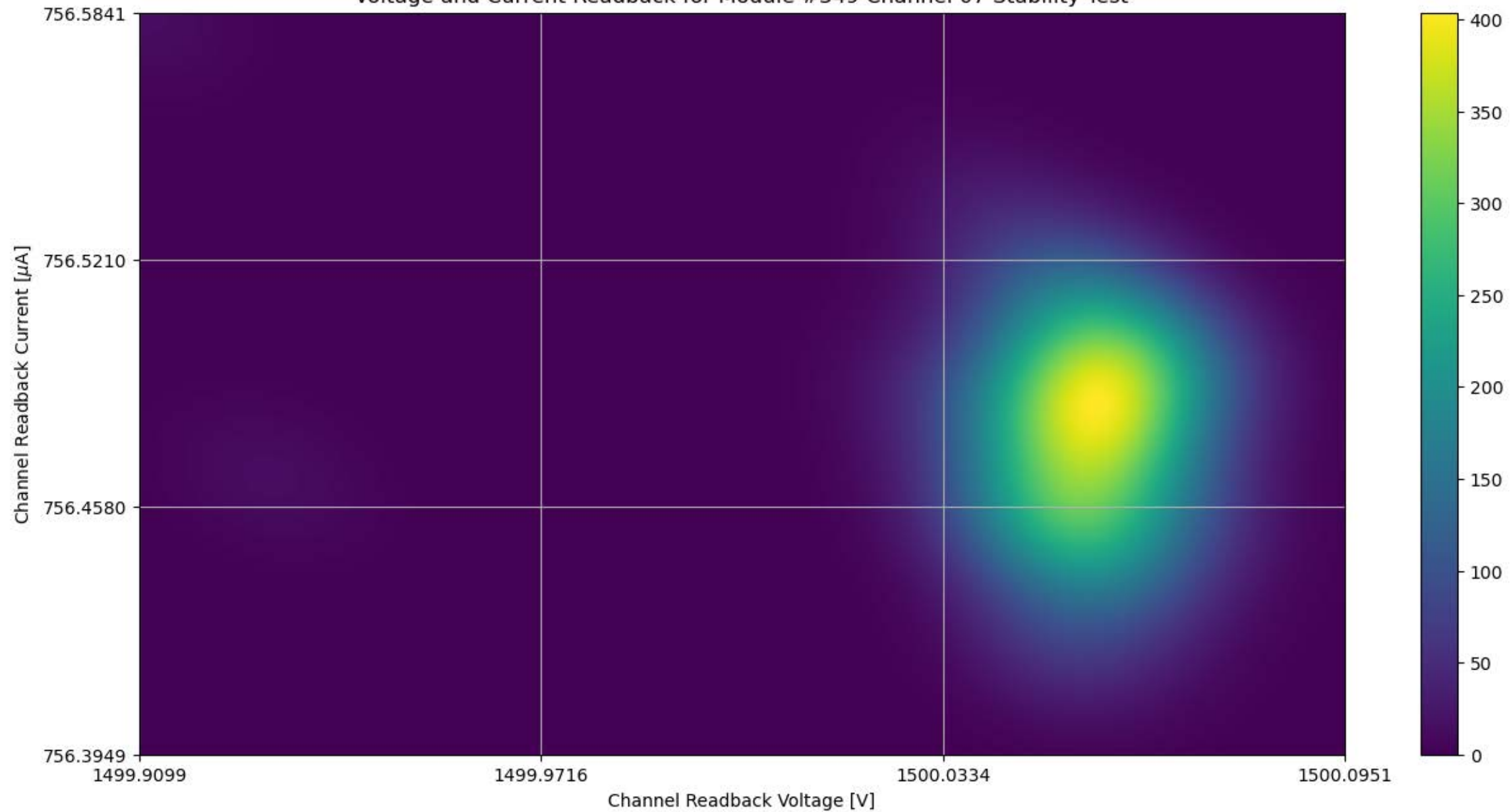
Voltage and Current Readback for Module #349 Channel 07 Stability Test
