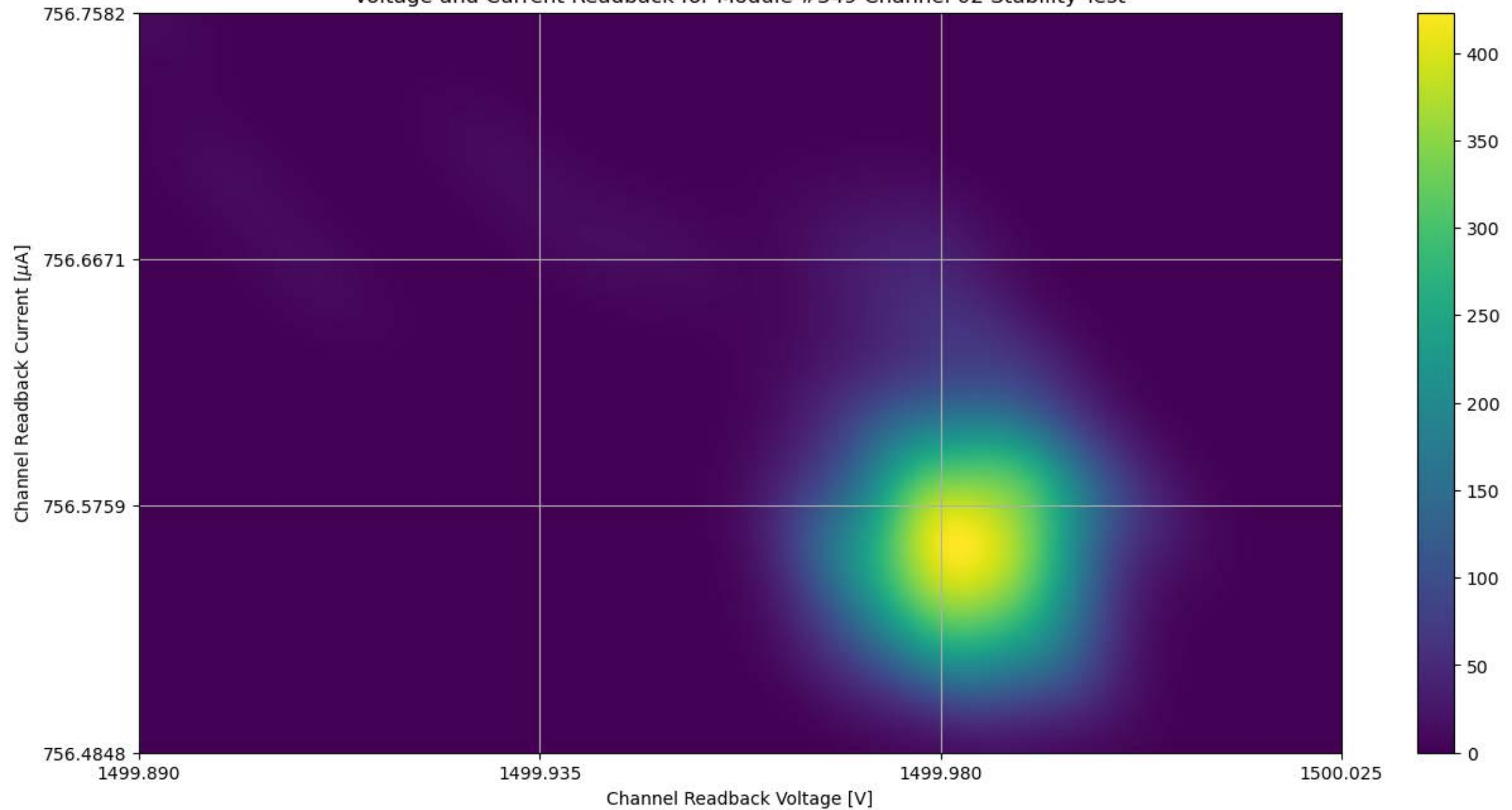
Voltage and Current Readback for Module #349 Channel 02 Stability Test
