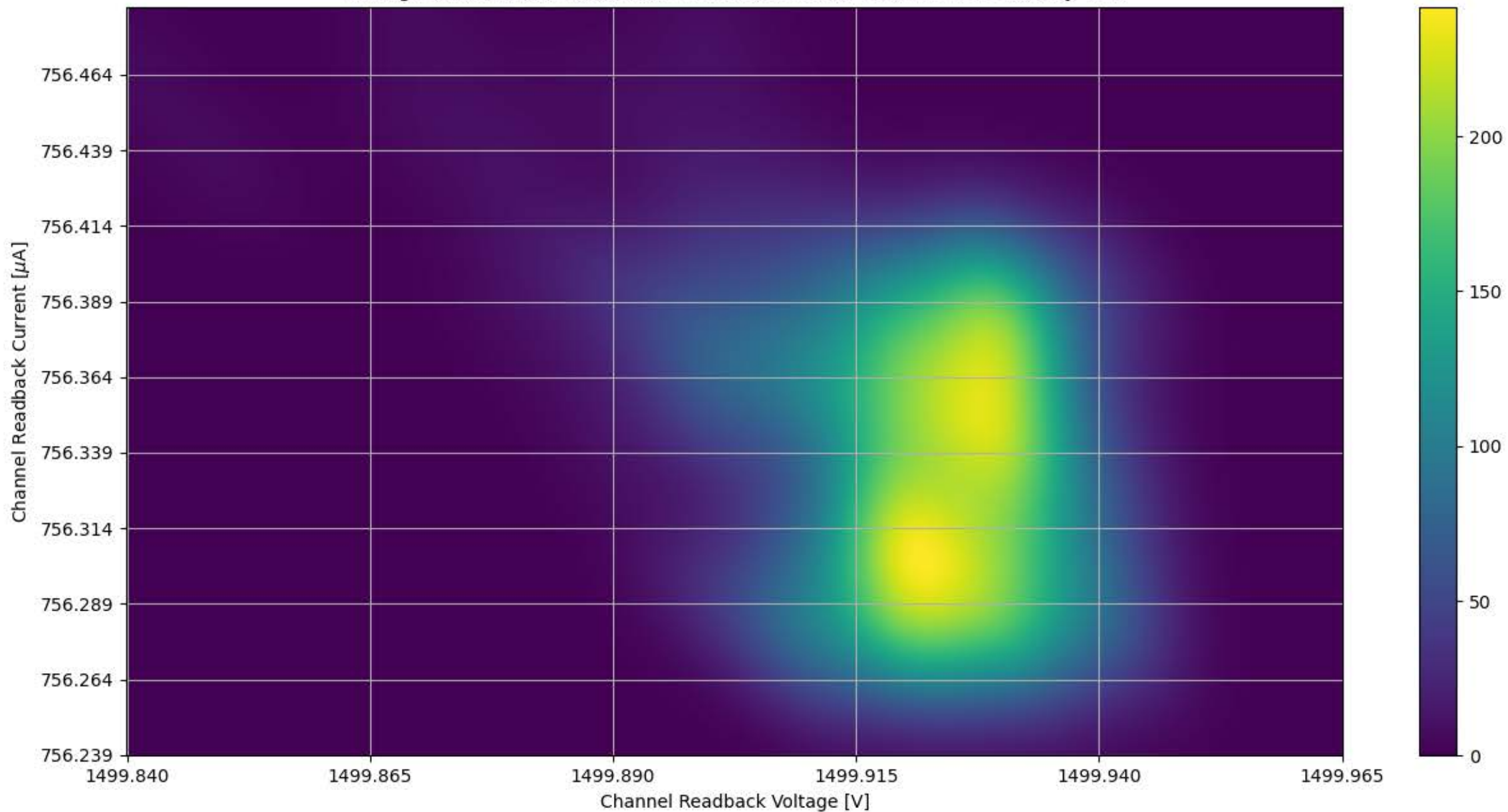
Voltage and Current Readback for Module #349 Channel 23 Stability Test
