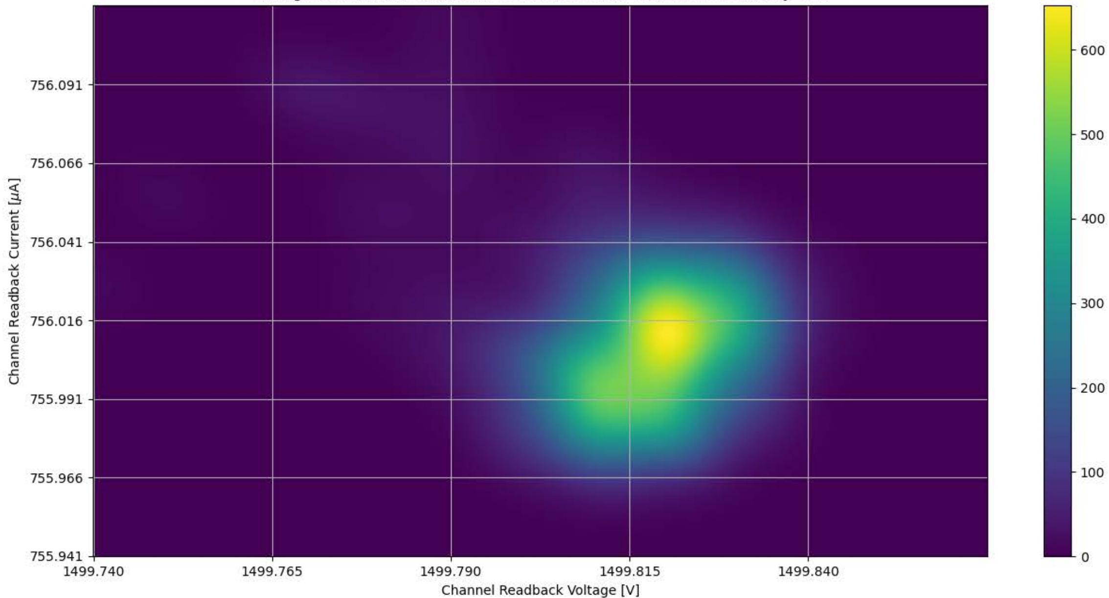
Voltage and Current Readback for Module #349 Channel 15 Stability Test
