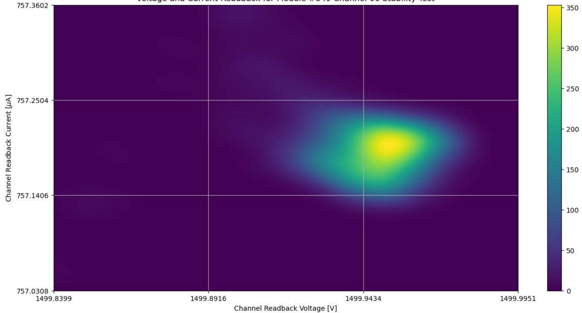
Voltage and Current Readback for Module #349 Channel 06 Stability Test
