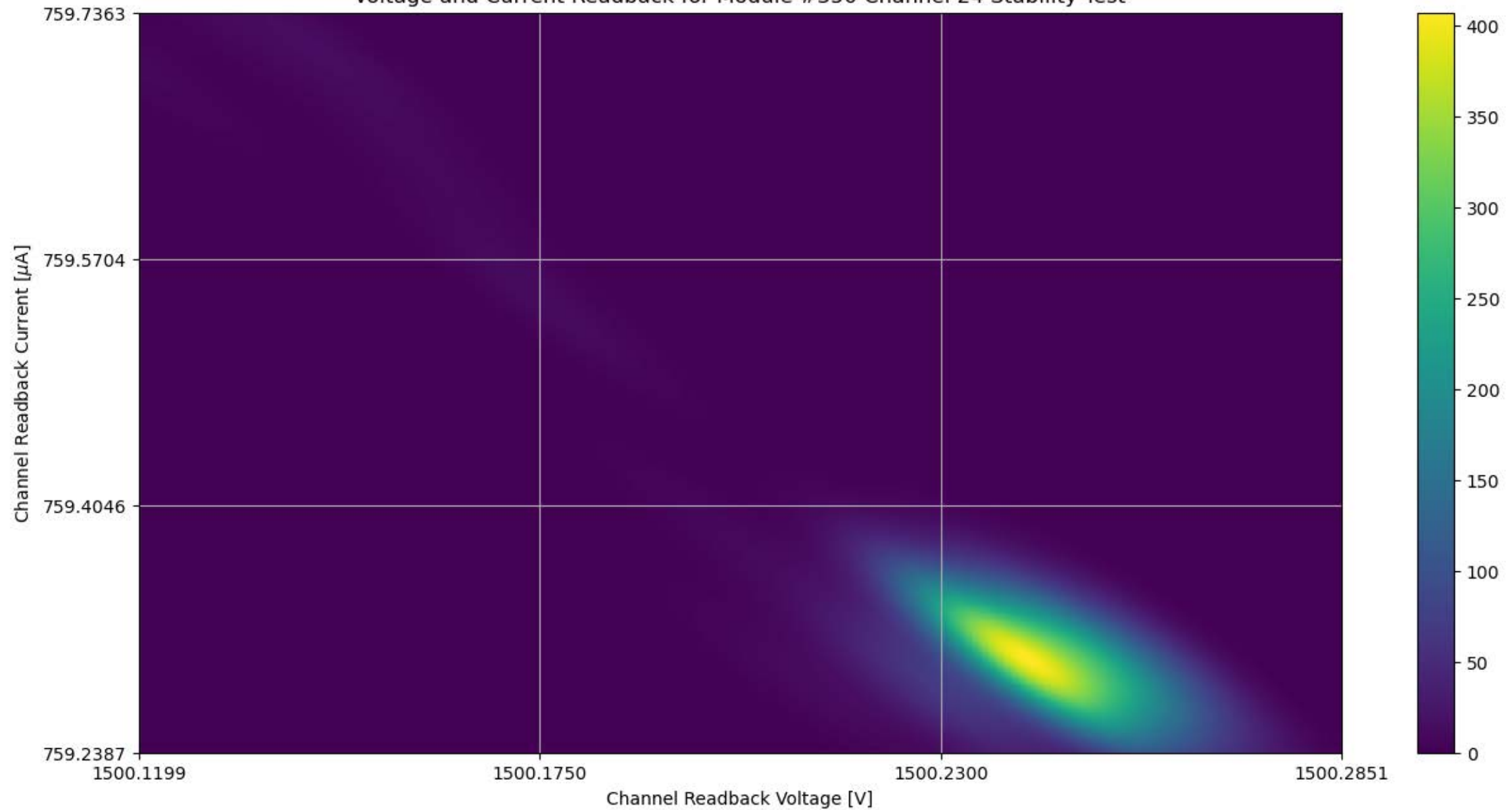
Voltage and Current Readback for Module #350 Channel 24 Stability Test
