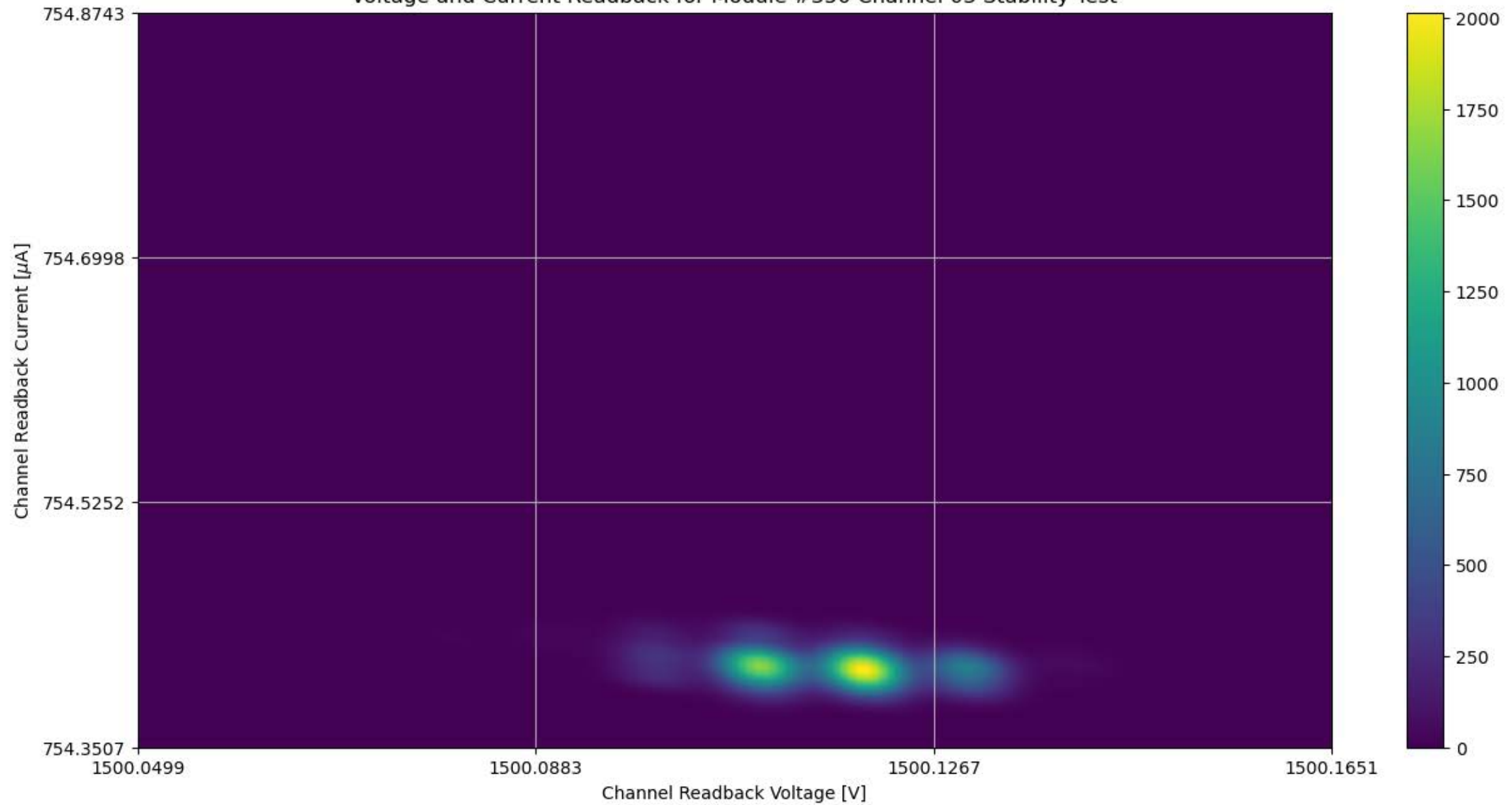
Voltage and Current Readback for Module #350 Channel 03 Stability Test
