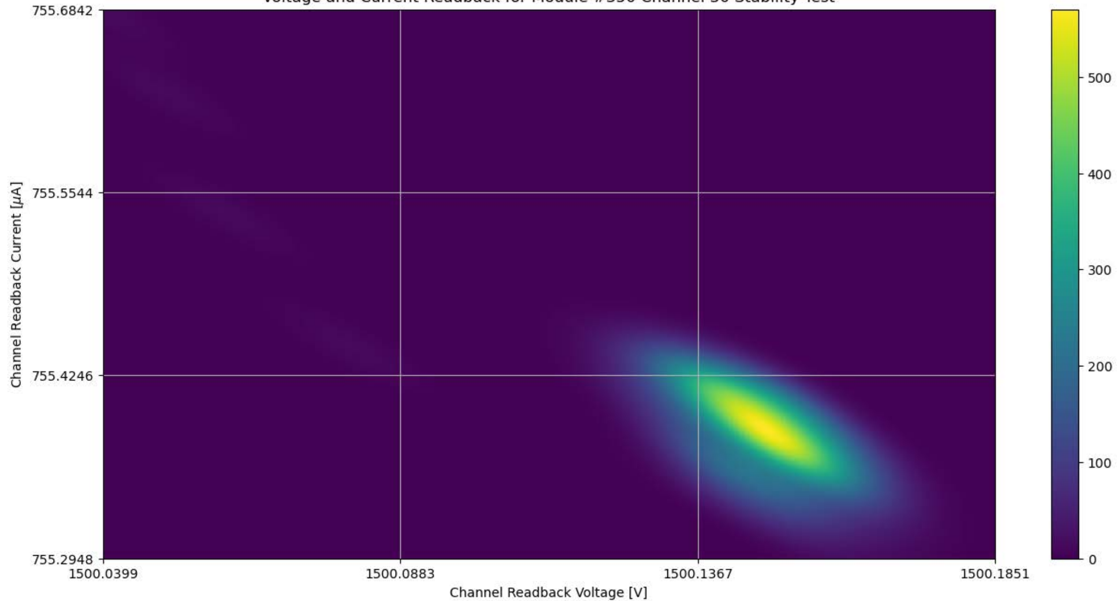
Voltage and Current Readback for Module #350 Channel 30 Stability Test
