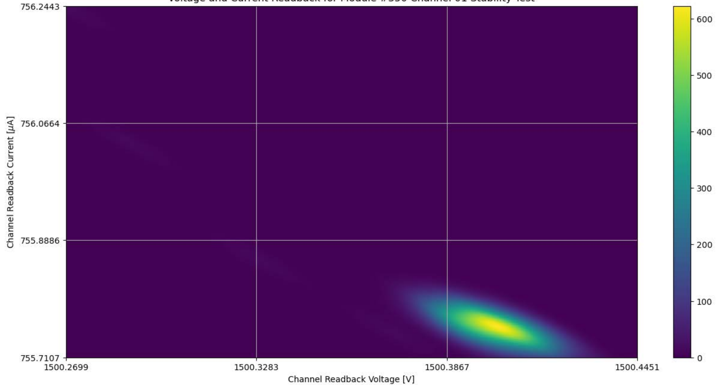
Voltage and Current Readback for Module #350 Channel 01 Stability Test
