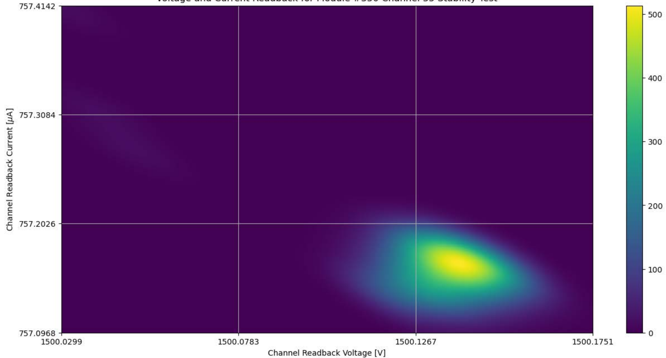
Voltage and Current Readback for Module #350 Channel 35 Stability Test
