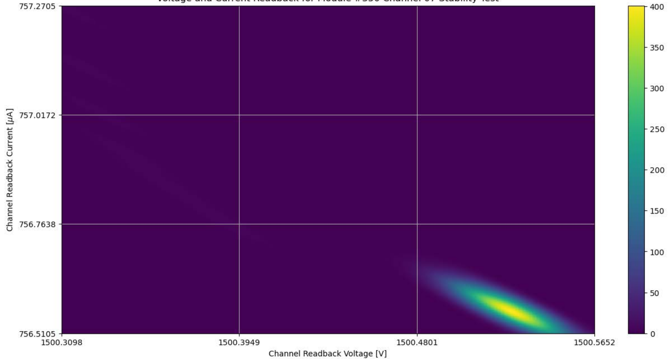
Voltage and Current Readback for Module #350 Channel 07 Stability Test
