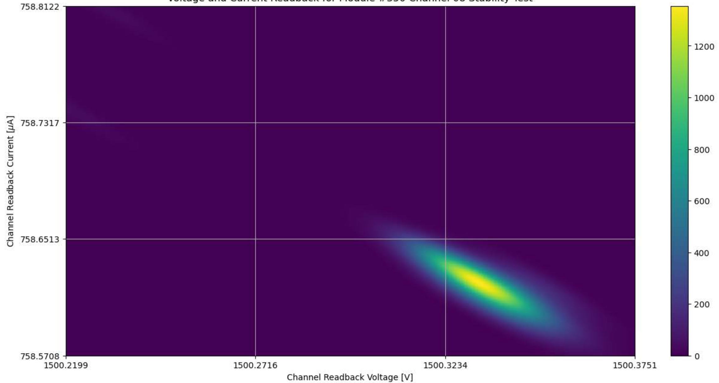
Voltage and Current Readback for Module #350 Channel 08 Stability Test
