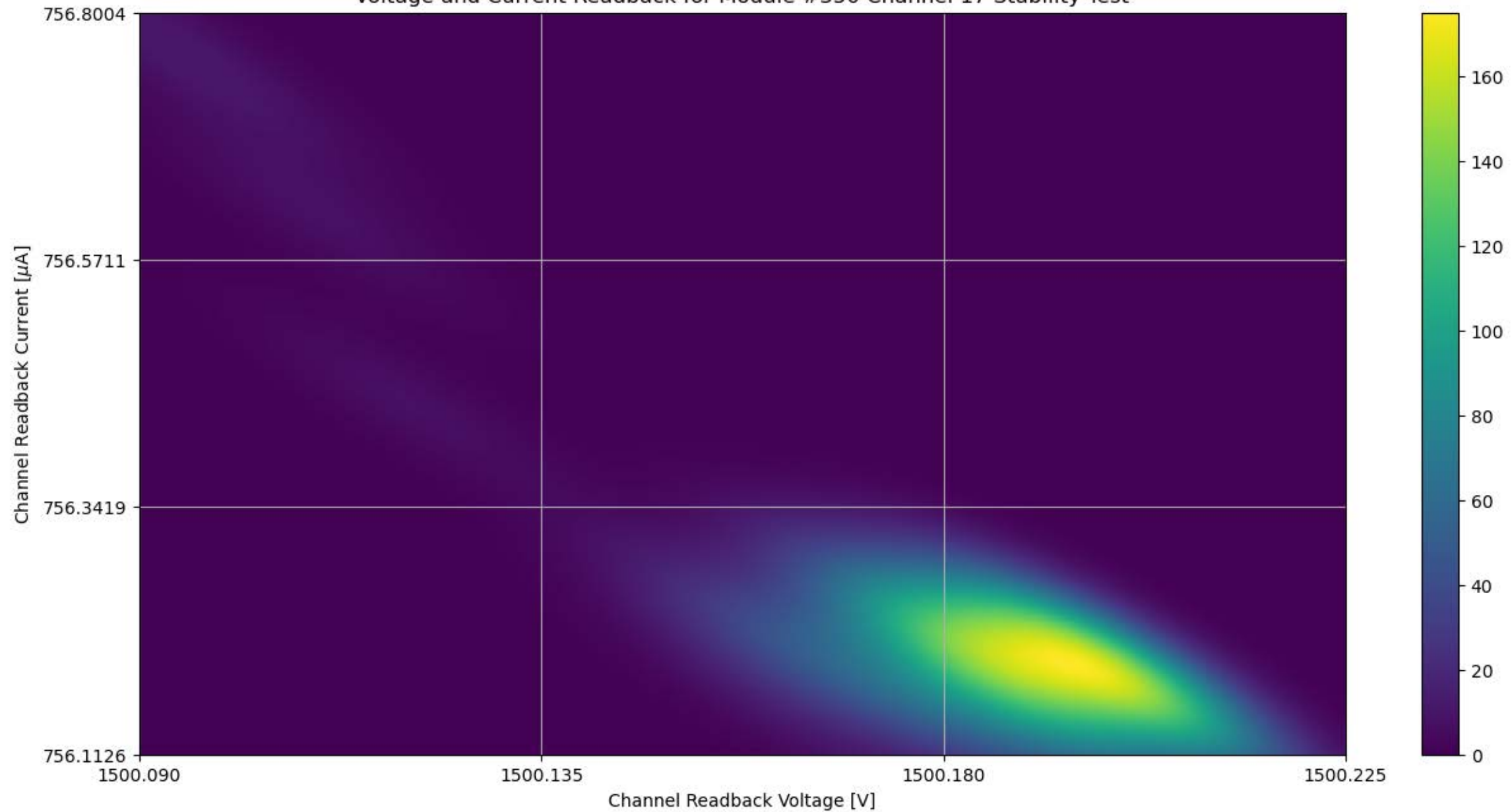
Voltage and Current Readback for Module #350 Channel 17 Stability Test
