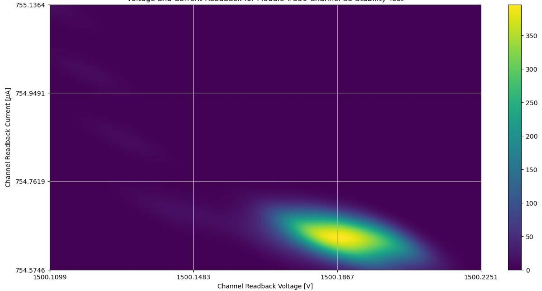
Voltage and Current Readback for Module #350 Channel 33 Stability Test
