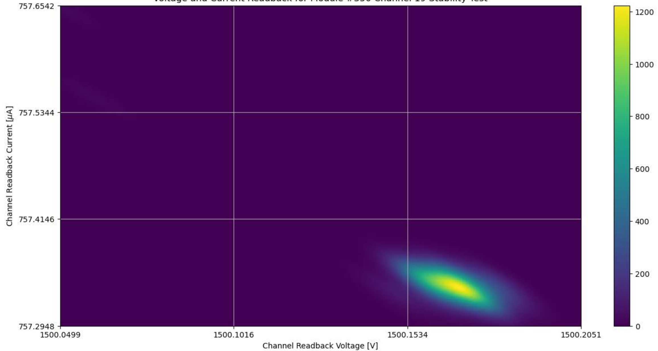
Voltage and Current Readback for Module #350 Channel 19 Stability Test
