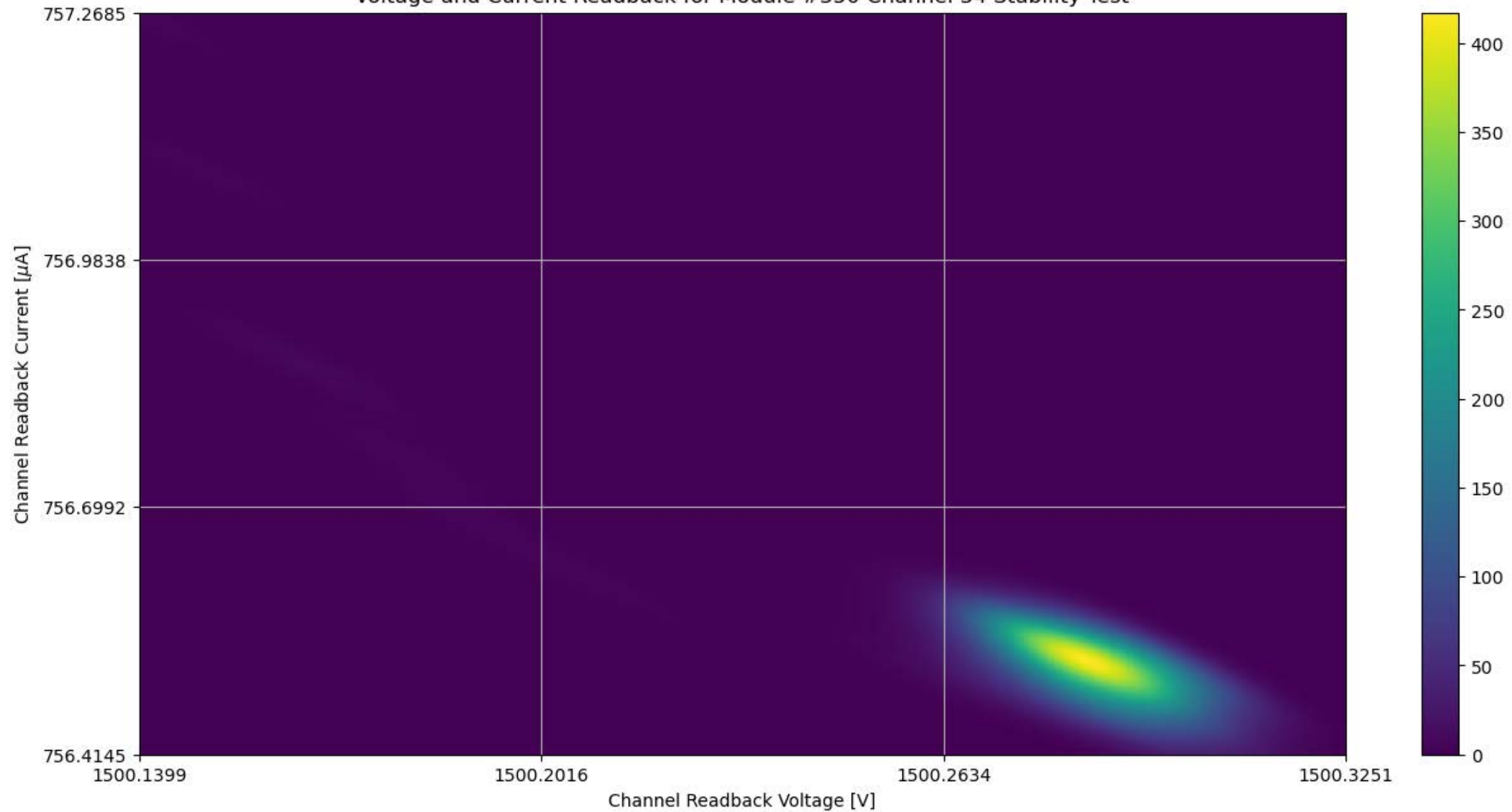
Voltage and Current Readback for Module #350 Channel 34 Stability Test
