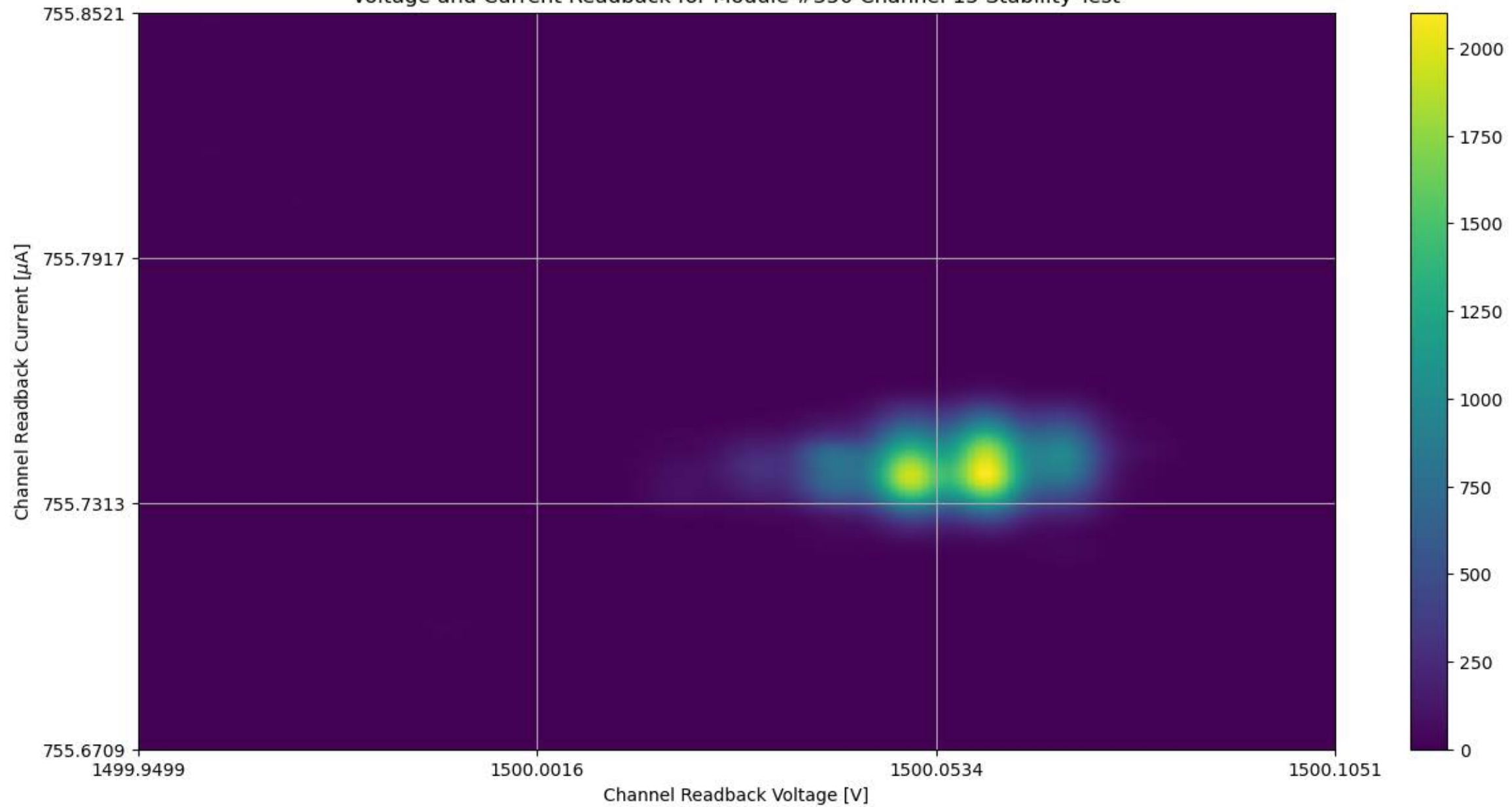
Voltage and Current Readback for Module #350 Channel 15 Stability Test
