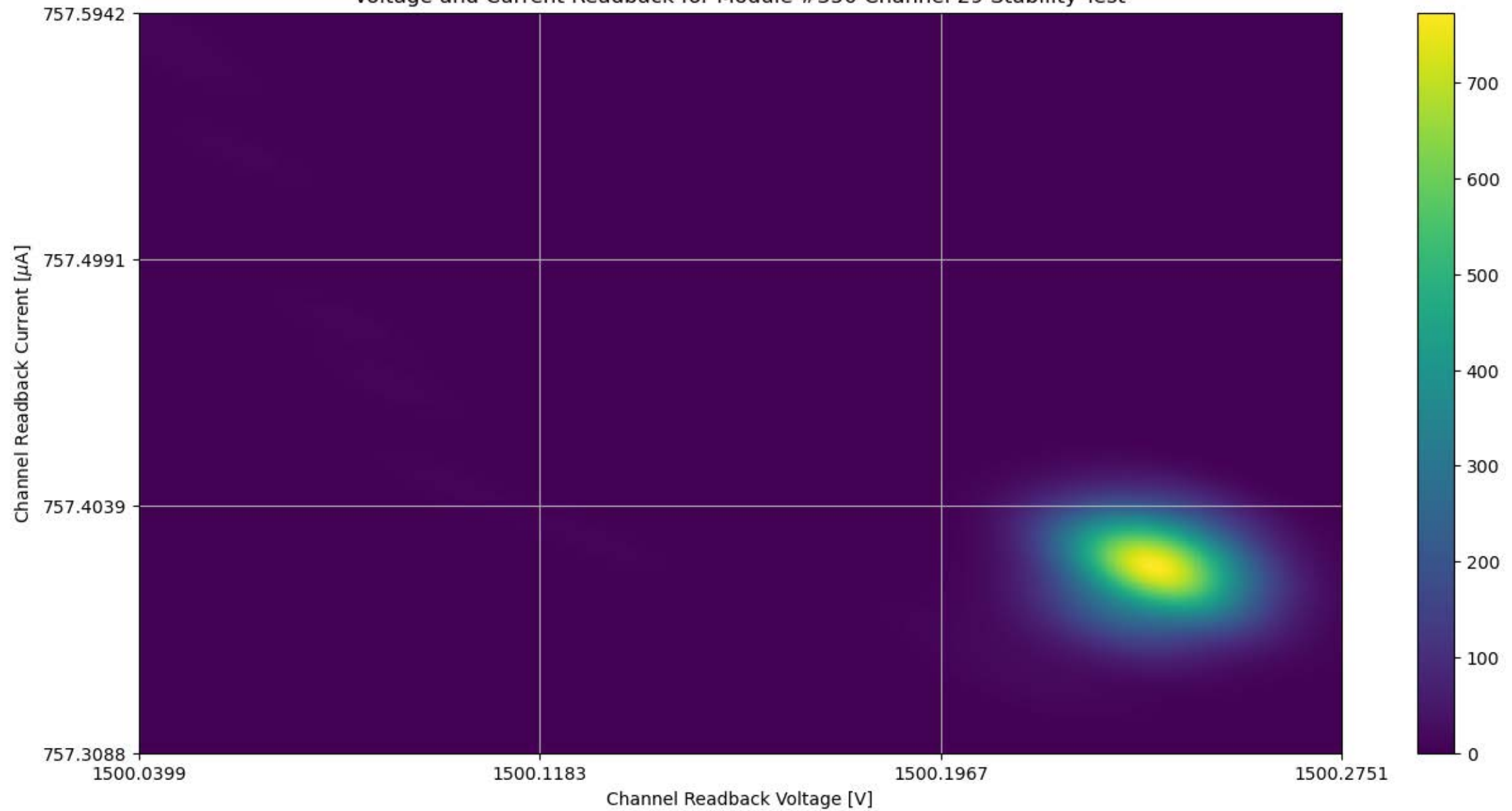
Voltage and Current Readback for Module #350 Channel 29 Stability Test
