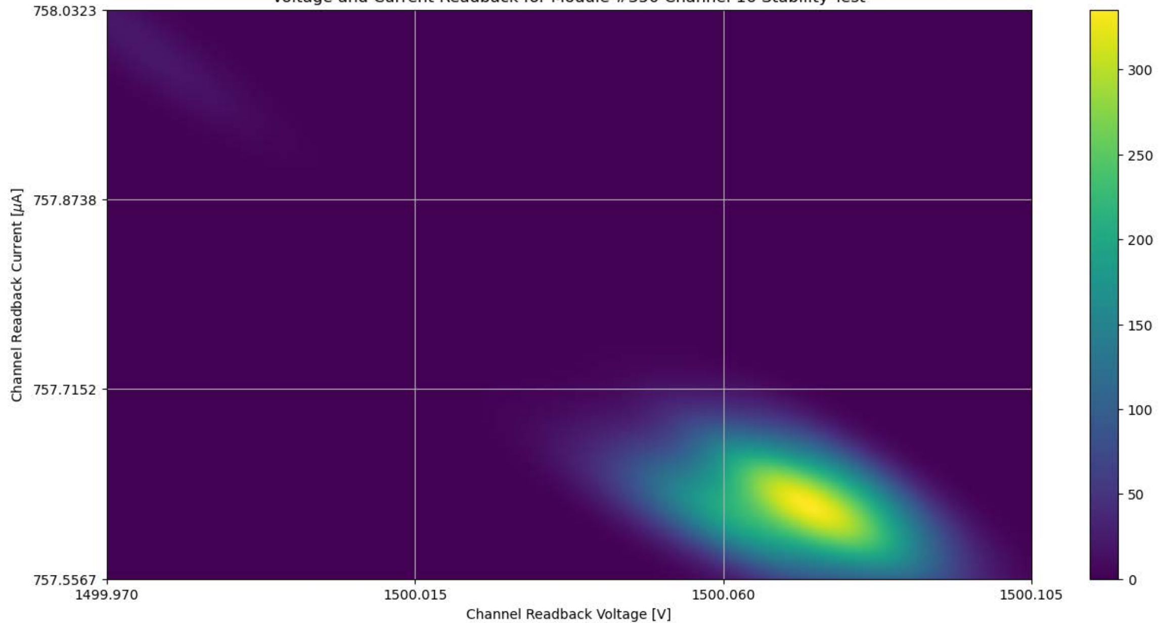
Voltage and Current Readback for Module #350 Channel 16 Stability Test
