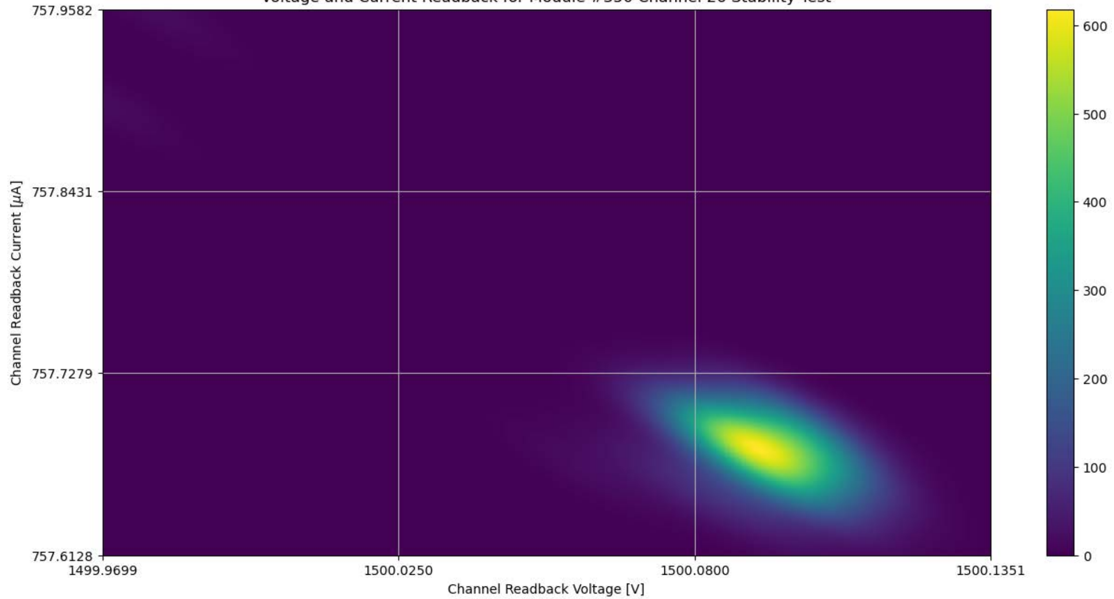
Voltage and Current Readback for Module #350 Channel 26 Stability Test
