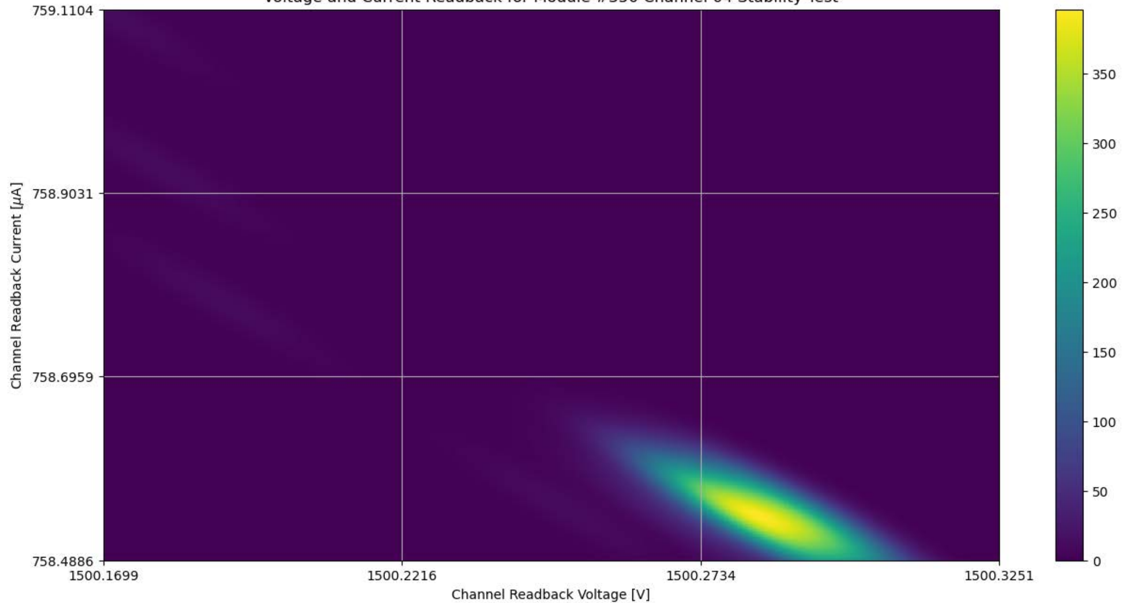
Voltage and Current Readback for Module #350 Channel 04 Stability Test
