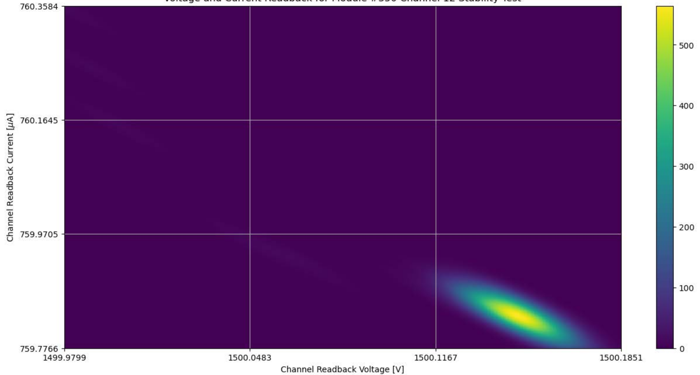
Voltage and Current Readback for Module #350 Channel 12 Stability Test
