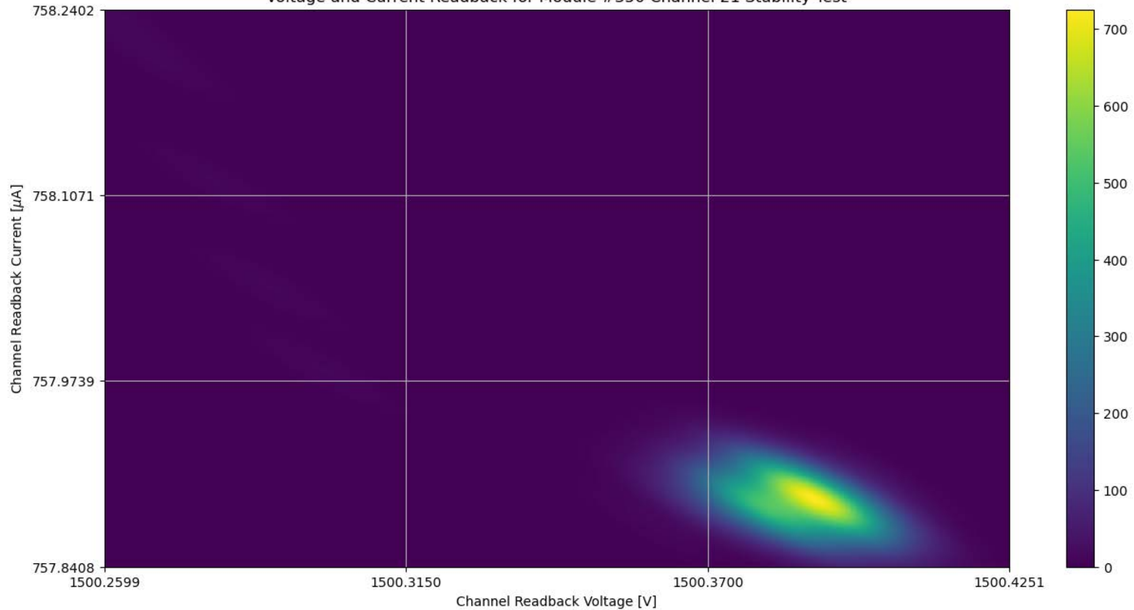
Voltage and Current Readback for Module #350 Channel 21 Stability Test
