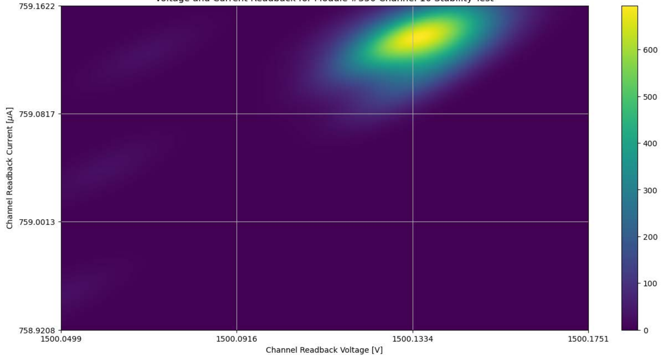
Voltage and Current Readback for Module #350 Channel 10 Stability Test
