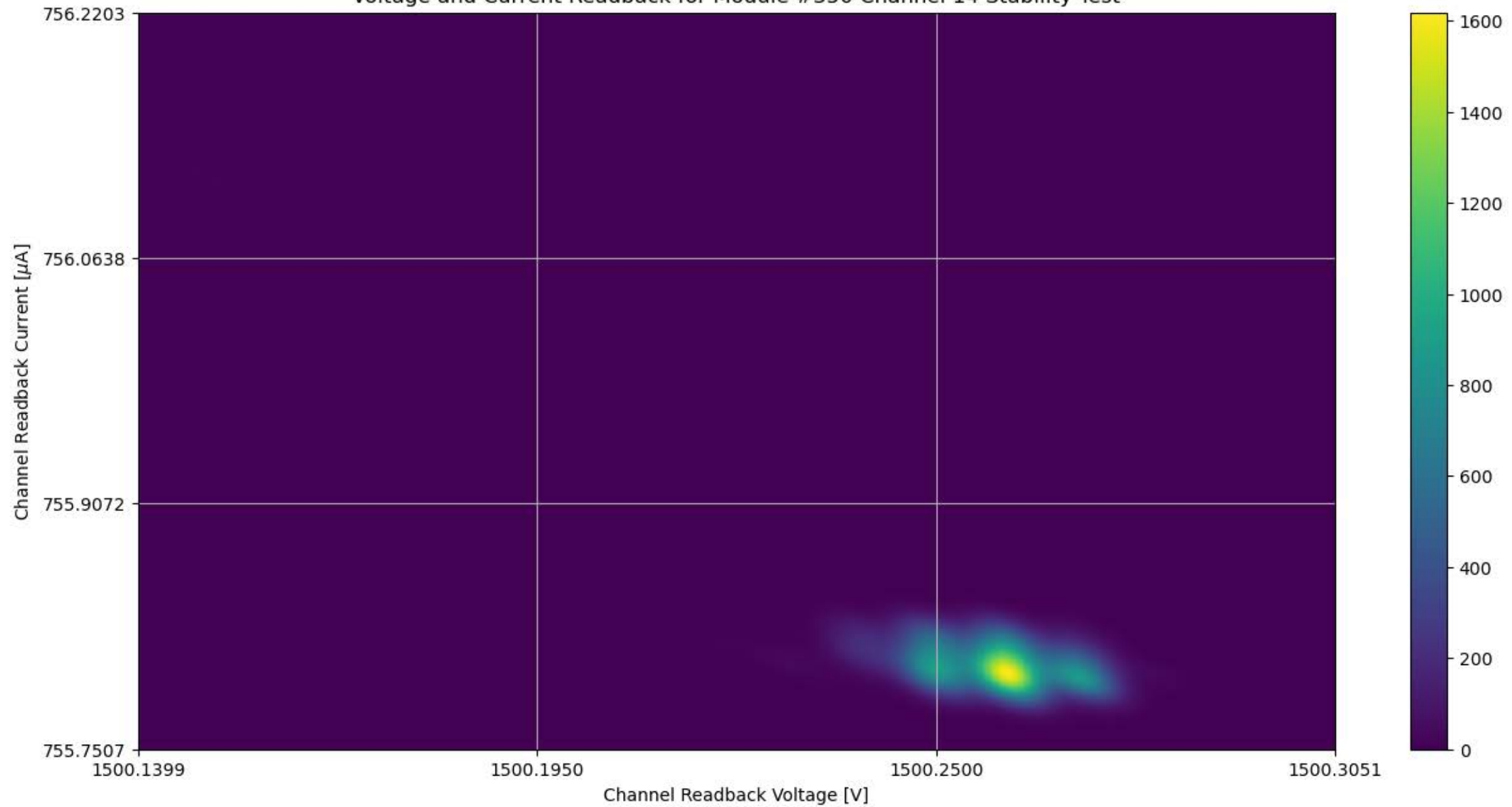
Voltage and Current Readback for Module #350 Channel 14 Stability Test
