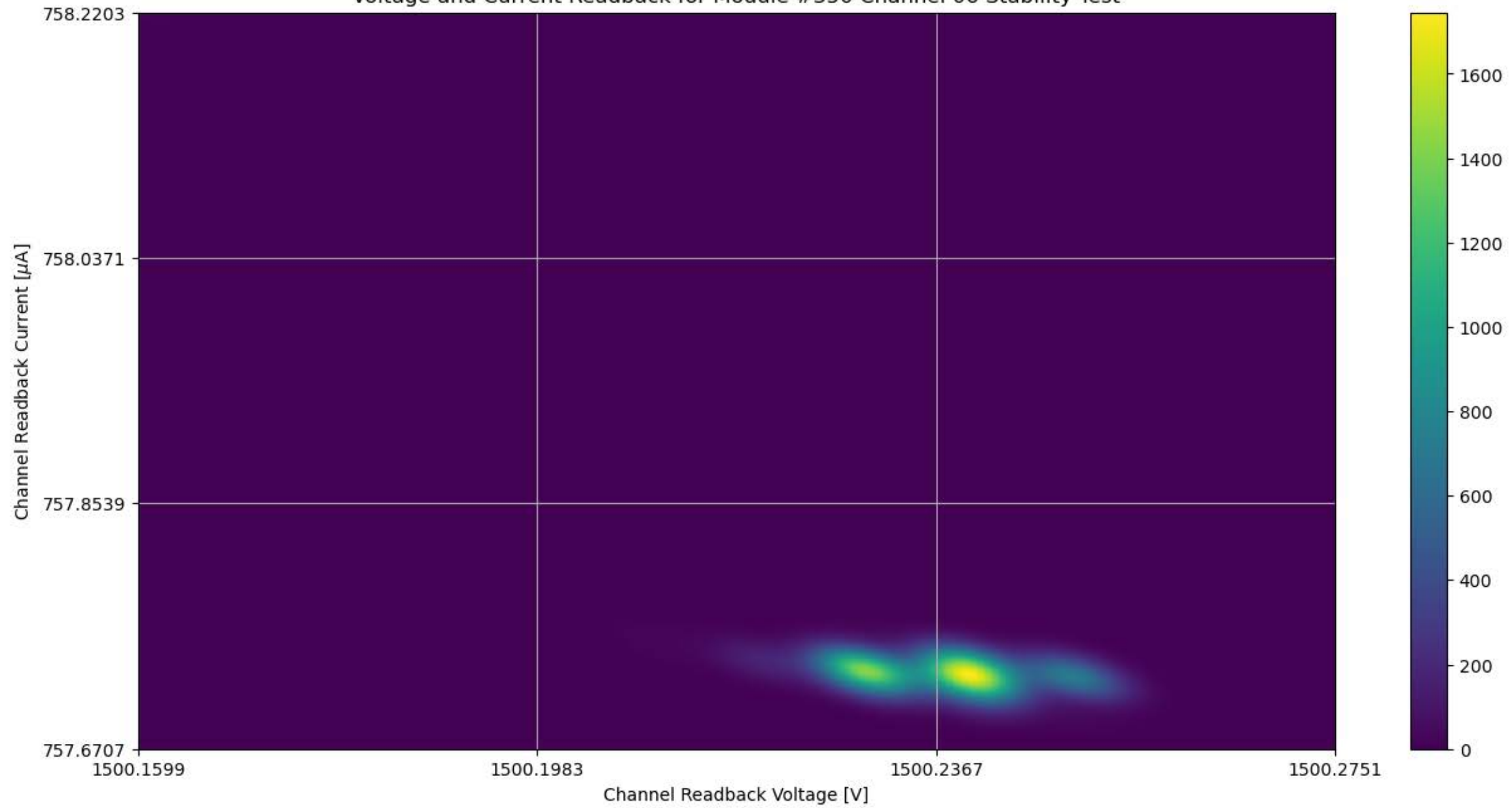
Voltage and Current Readback for Module #350 Channel 06 Stability Test
