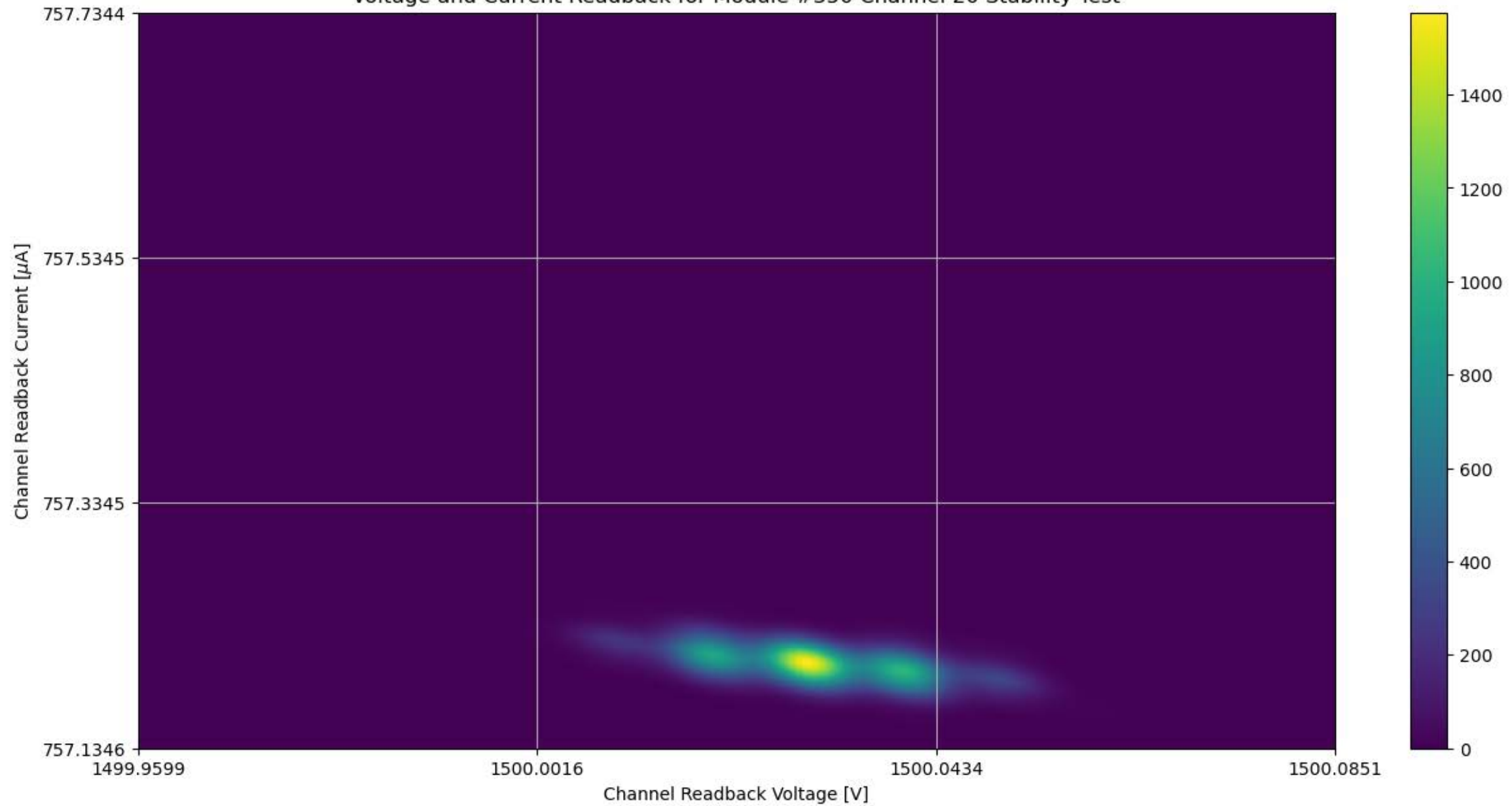
Voltage and Current Readback for Module #350 Channel 20 Stability Test
