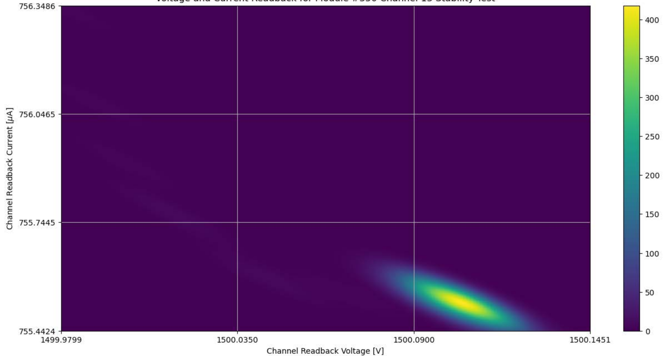
Voltage and Current Readback for Module #350 Channel 13 Stability Test
