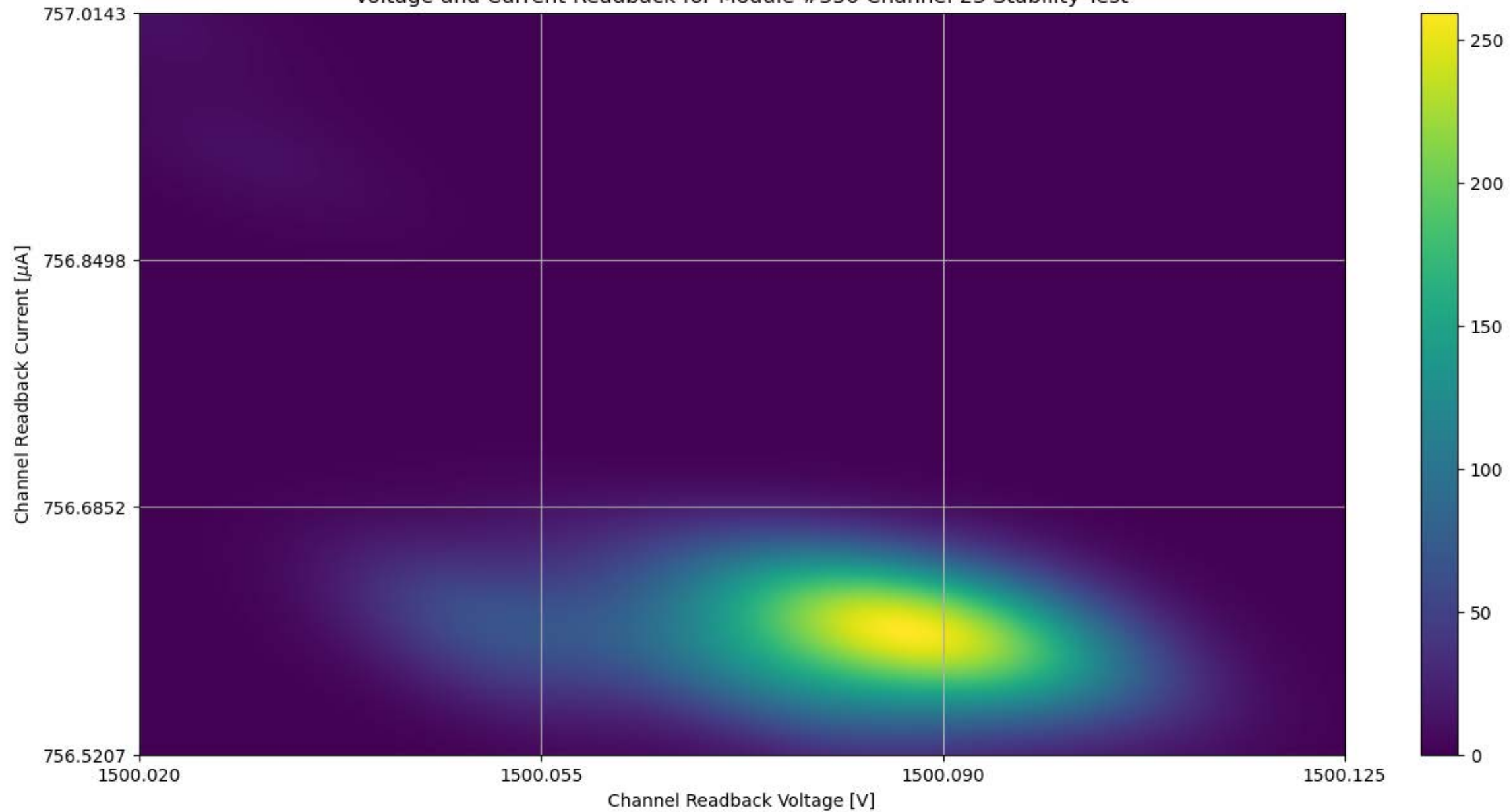
Voltage and Current Readback for Module #350 Channel 23 Stability Test
