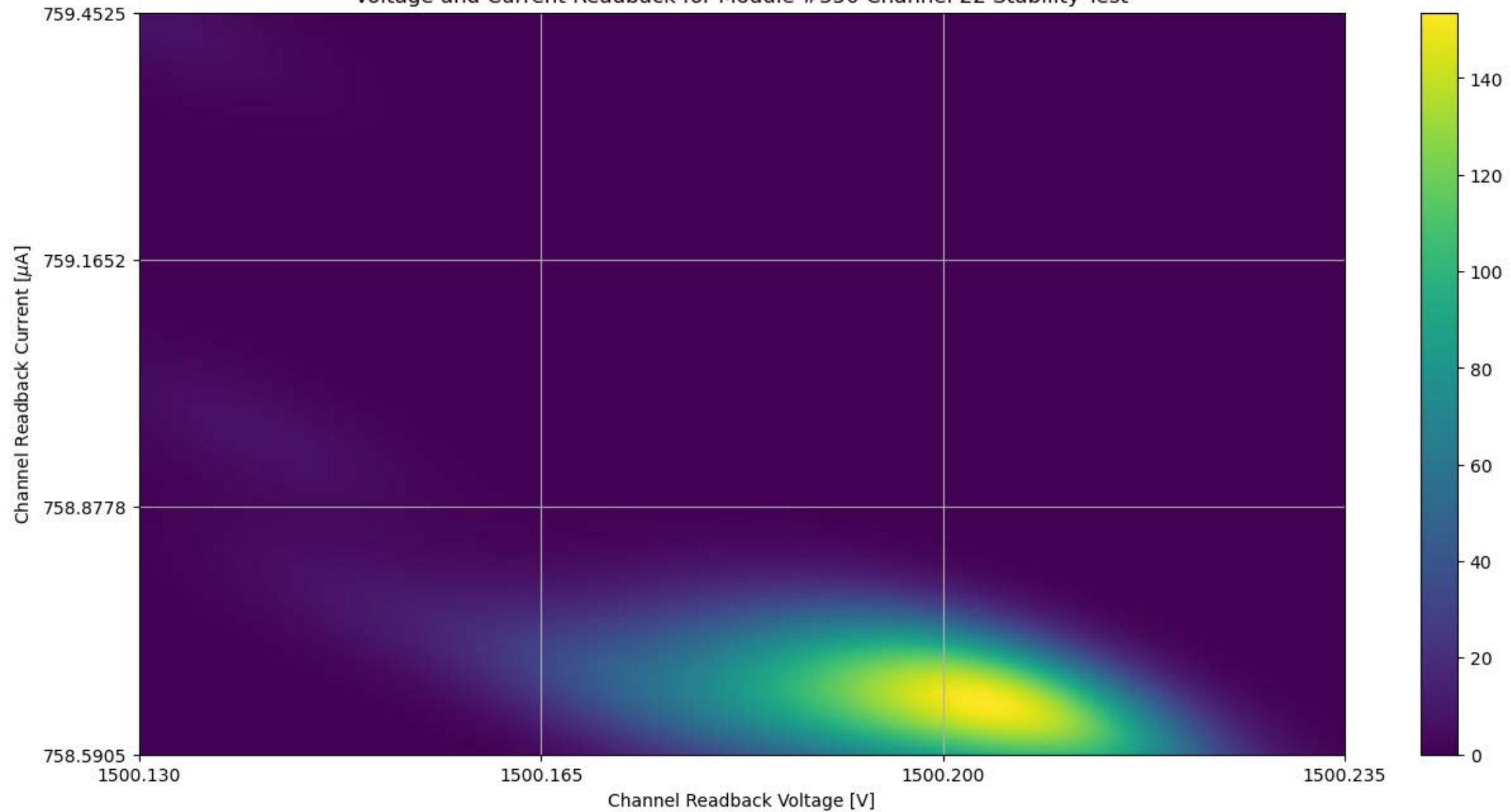
Voltage and Current Readback for Module #350 Channel 22 Stability Test
