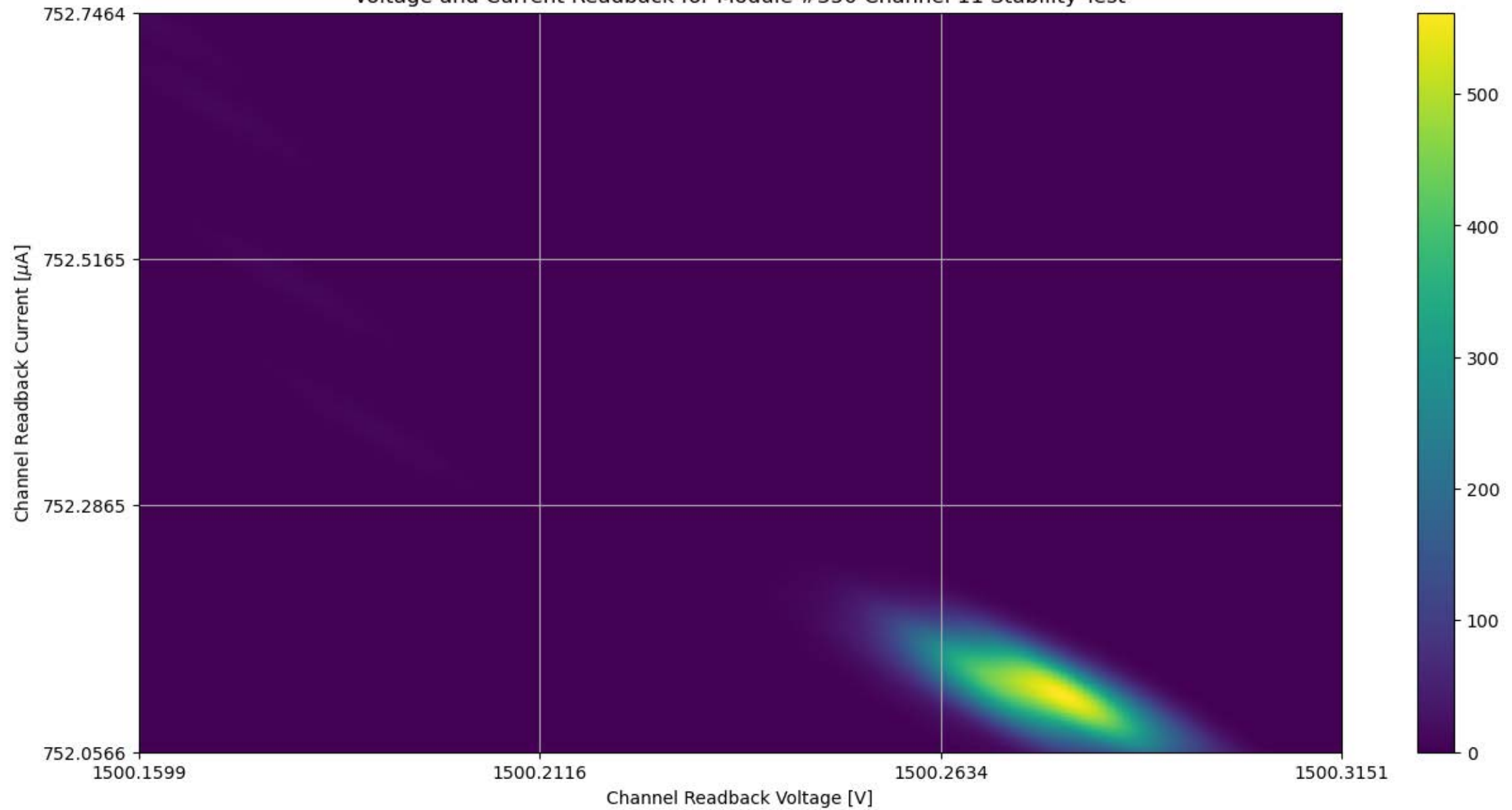
Voltage and Current Readback for Module #350 Channel 11 Stability Test
