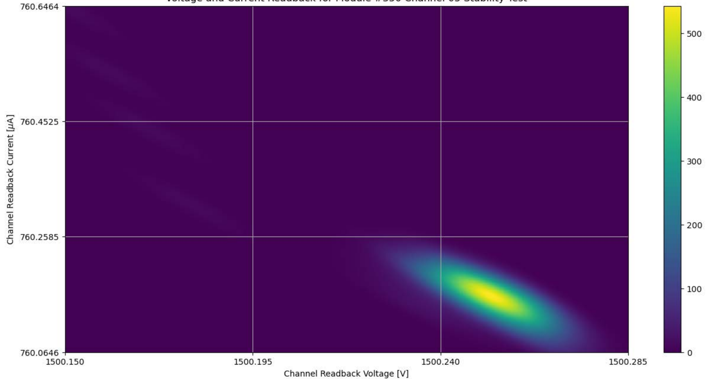
Voltage and Current Readback for Module #350 Channel 05 Stability Test
