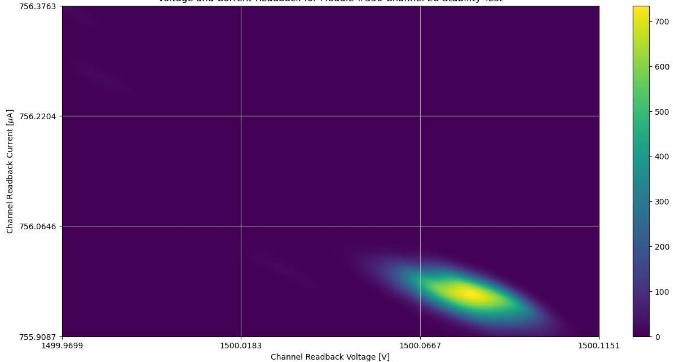
Voltage and Current Readback for Module #350 Channel 28 Stability Test
