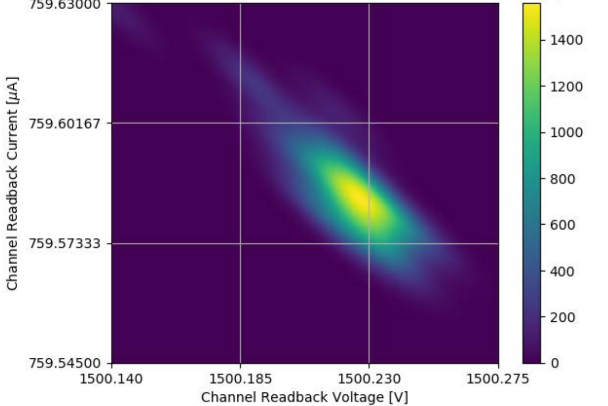
Voltage and Current Readback for Module #351 Channel 24 Stability Test
