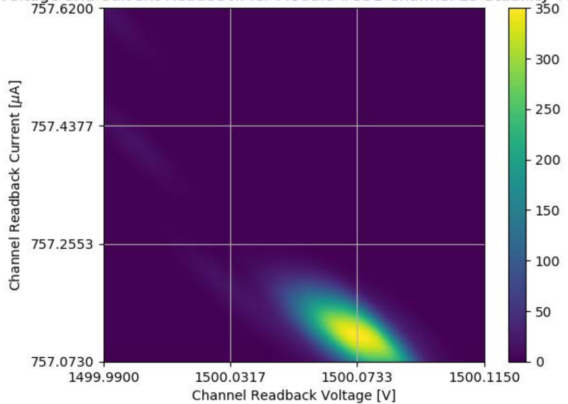
Voltage and Current Readback for Module #351 Channel 19 Stability Test
