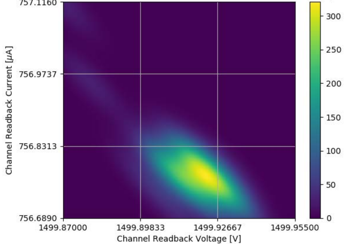
Voltage and Current Readback for Module #351 Channel 23 Stability Test
