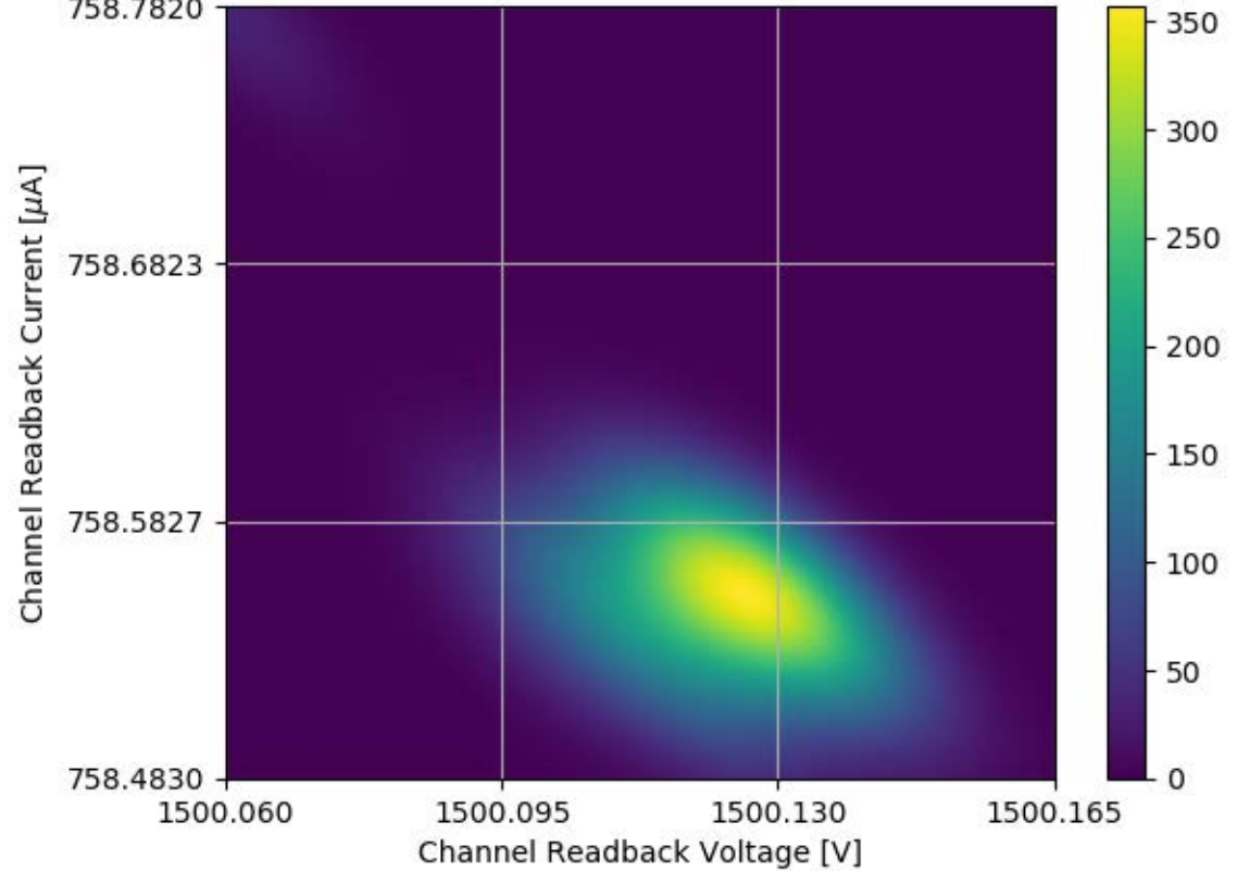
Voltage and Current Readback for Module #351 Channel 04 Stability Test
