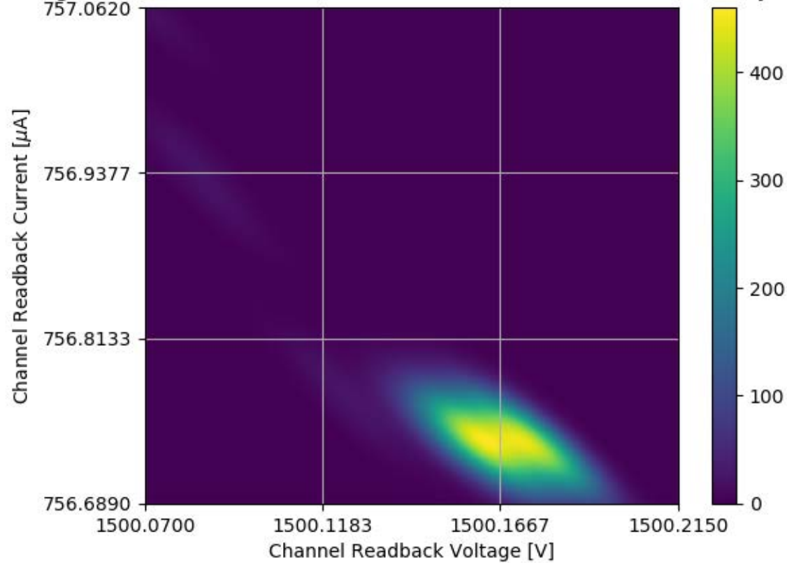
Voltage and Current Readback for Module #351 Channel 29 Stability Test
