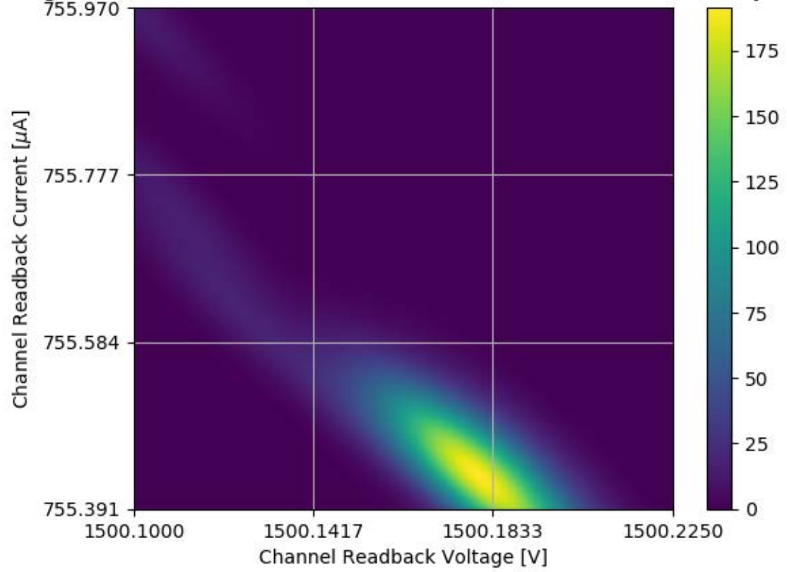
Voltage and Current Readback for Module #351 Channel 01 Stability Test
