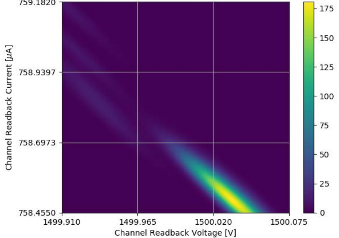
Voltage and Current Readback for Module #351 Channel 05 Stability Test
