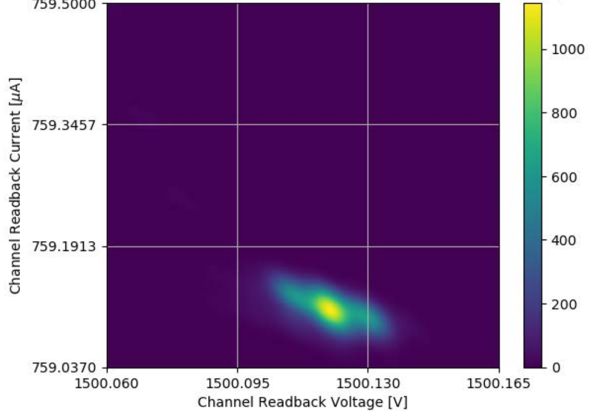
Voltage and Current Readback for Module #351 Channel 22 Stability Test
