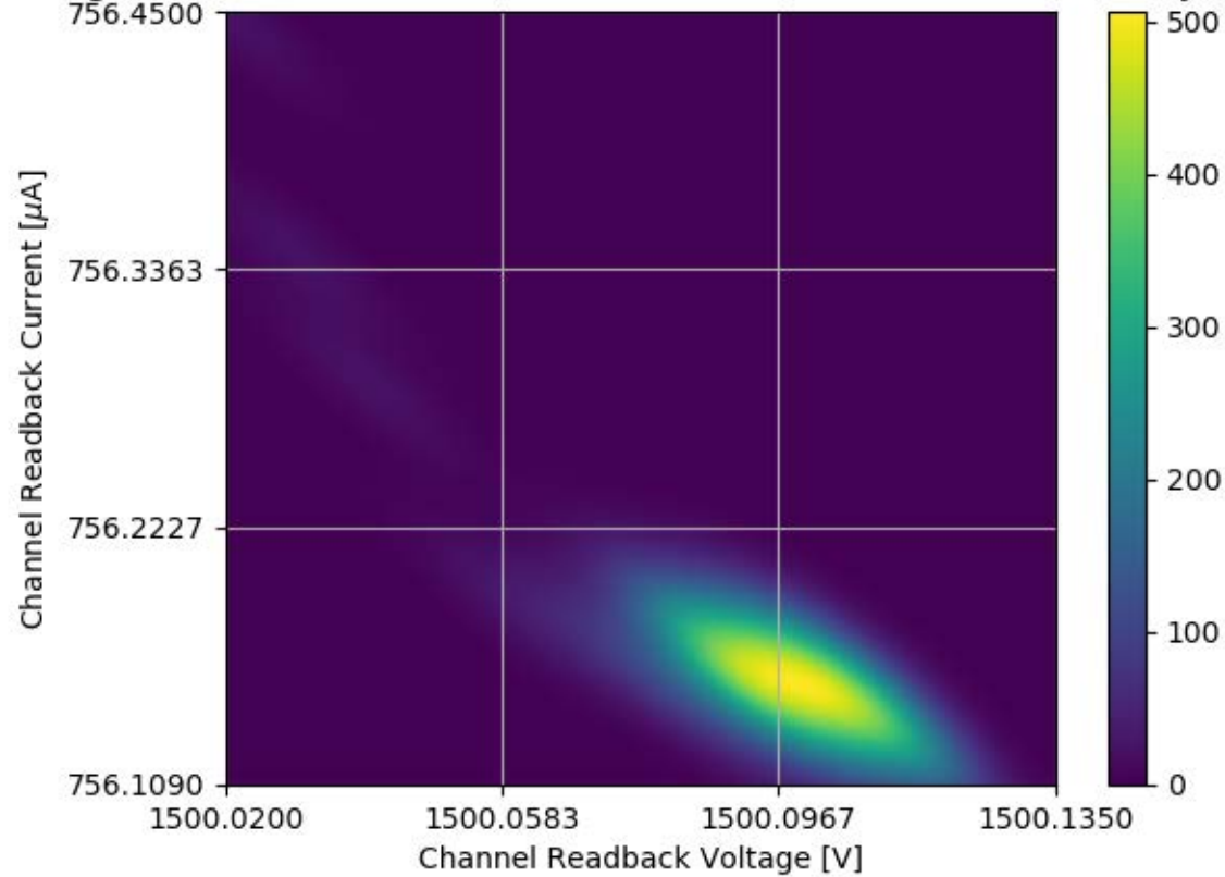
Voltage and Current Readback for Module #351 Channel 17 Stability Test
