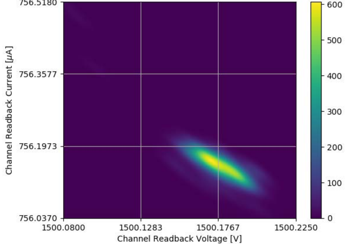
Voltage and Current Readback for Module #351 Channel 34 Stability Test
