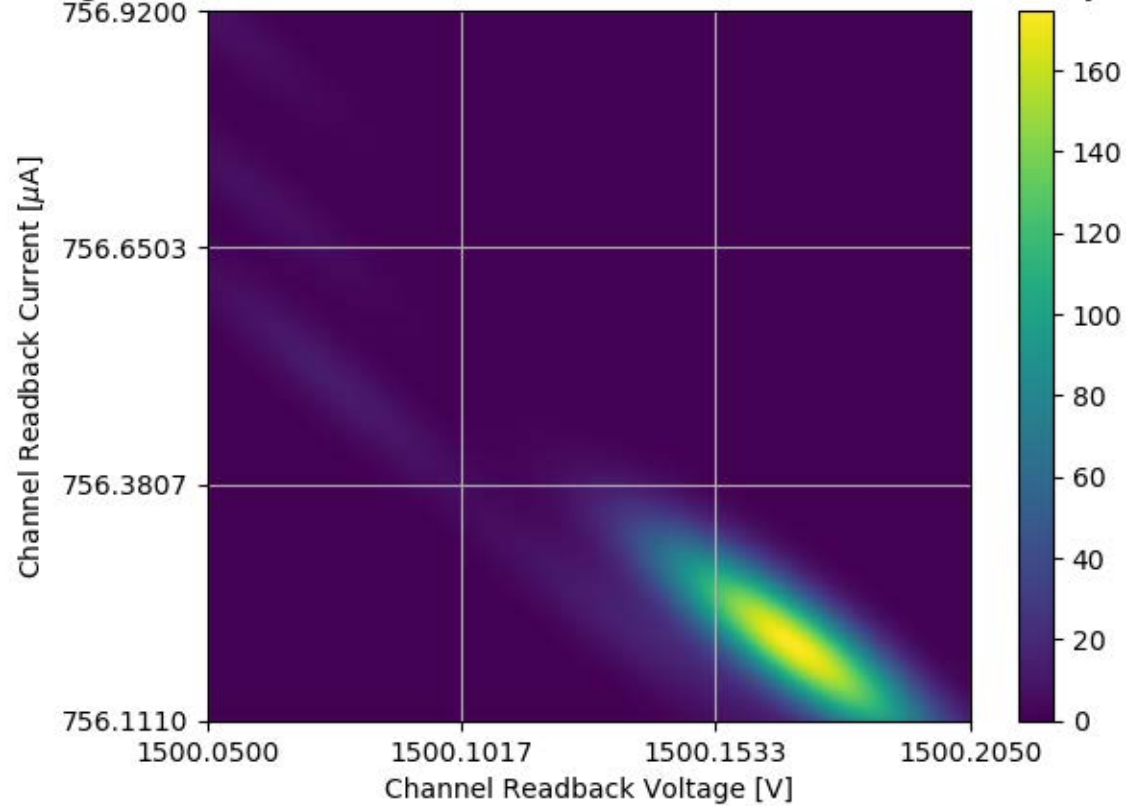
Voltage and Current Readback for Module #351 Channel 07 Stability Test
