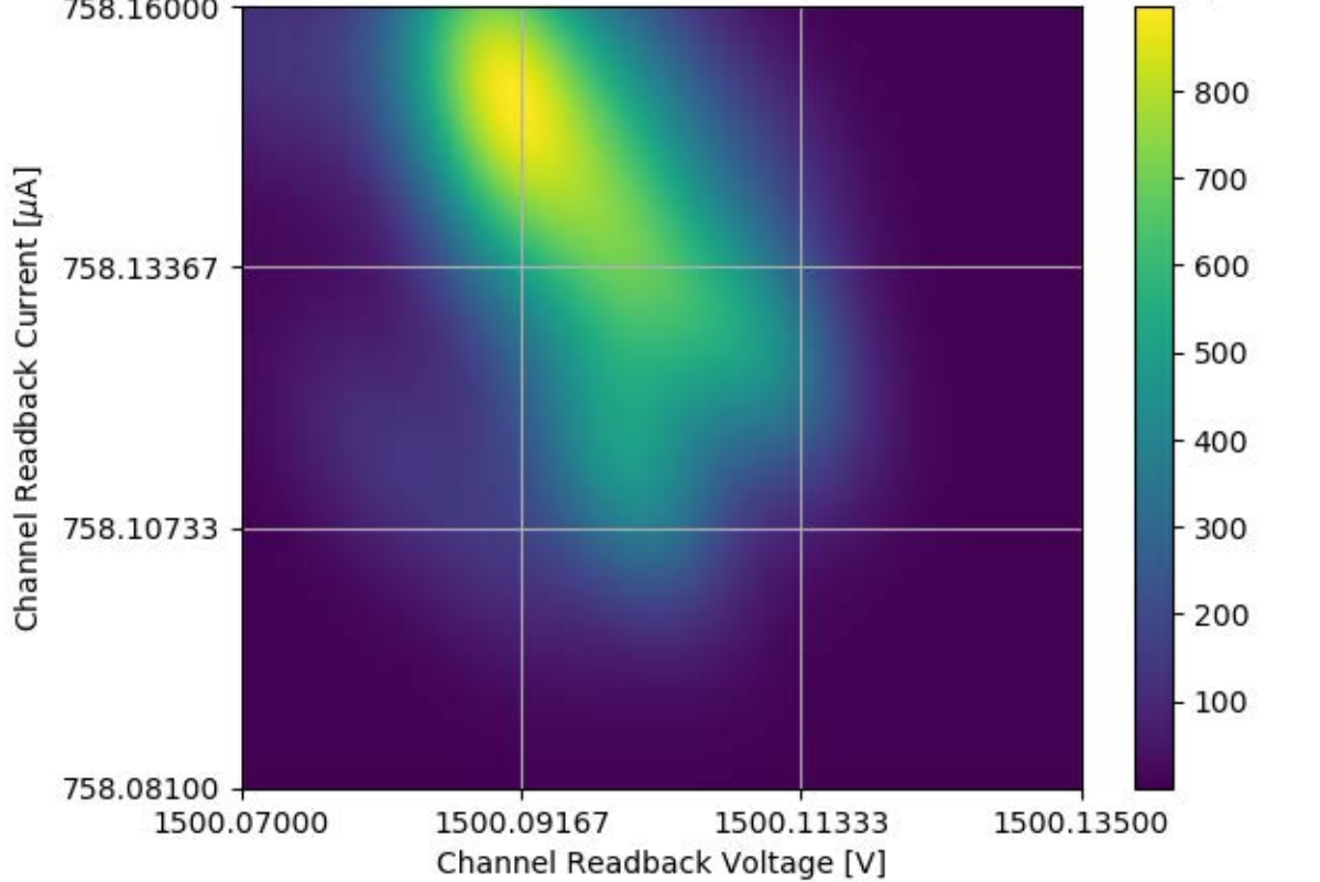
Voltage and Current Readback for Module #351 Channel 08 Stability Test
