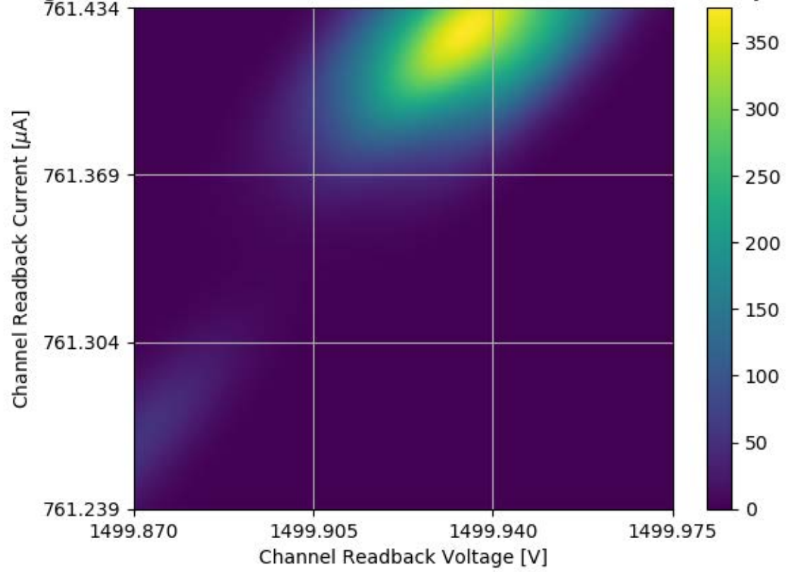
Voltage and Current Readback for Module #351 Channel 09 Stability Test
