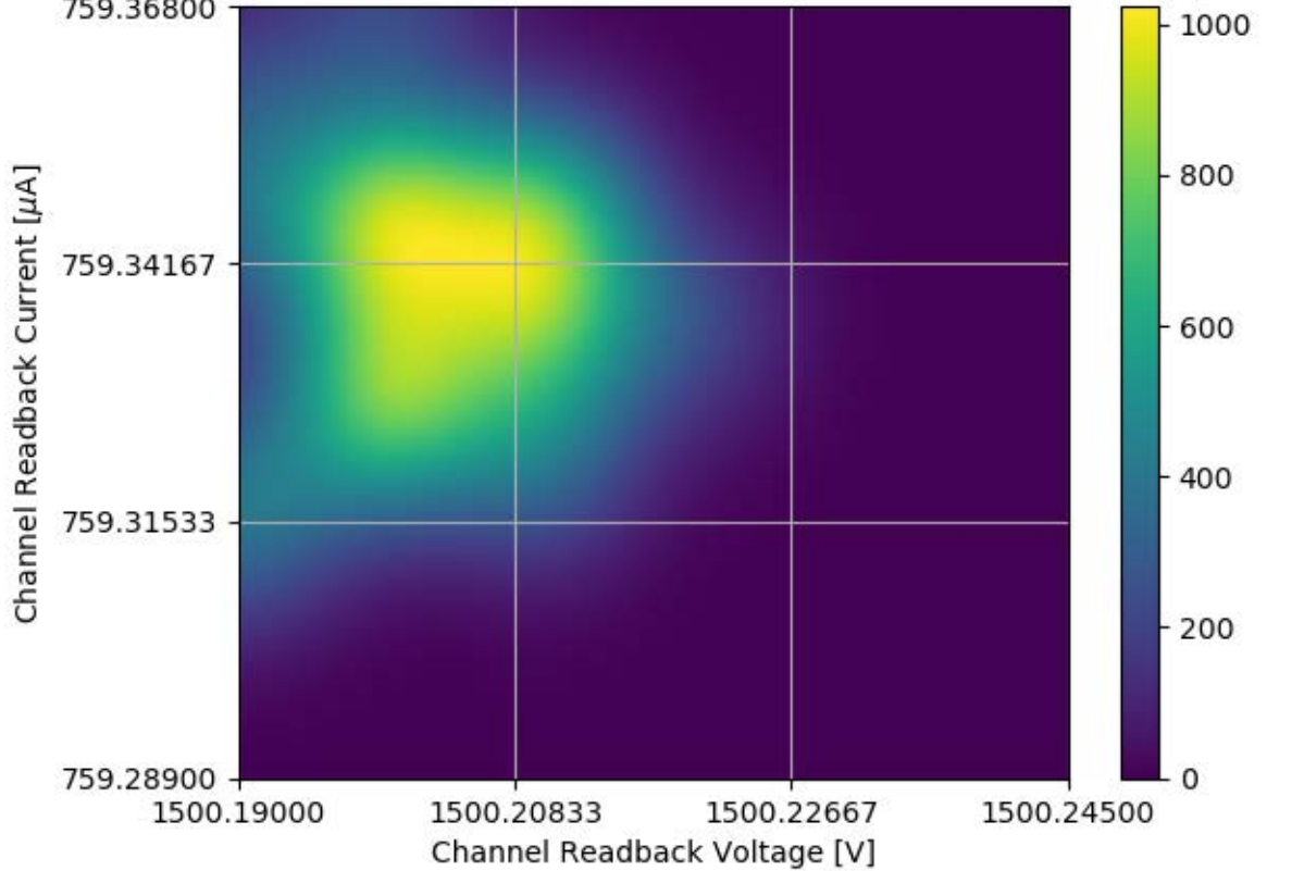
Voltage and Current Readback for Module #351 Channel 25 Stability Test
