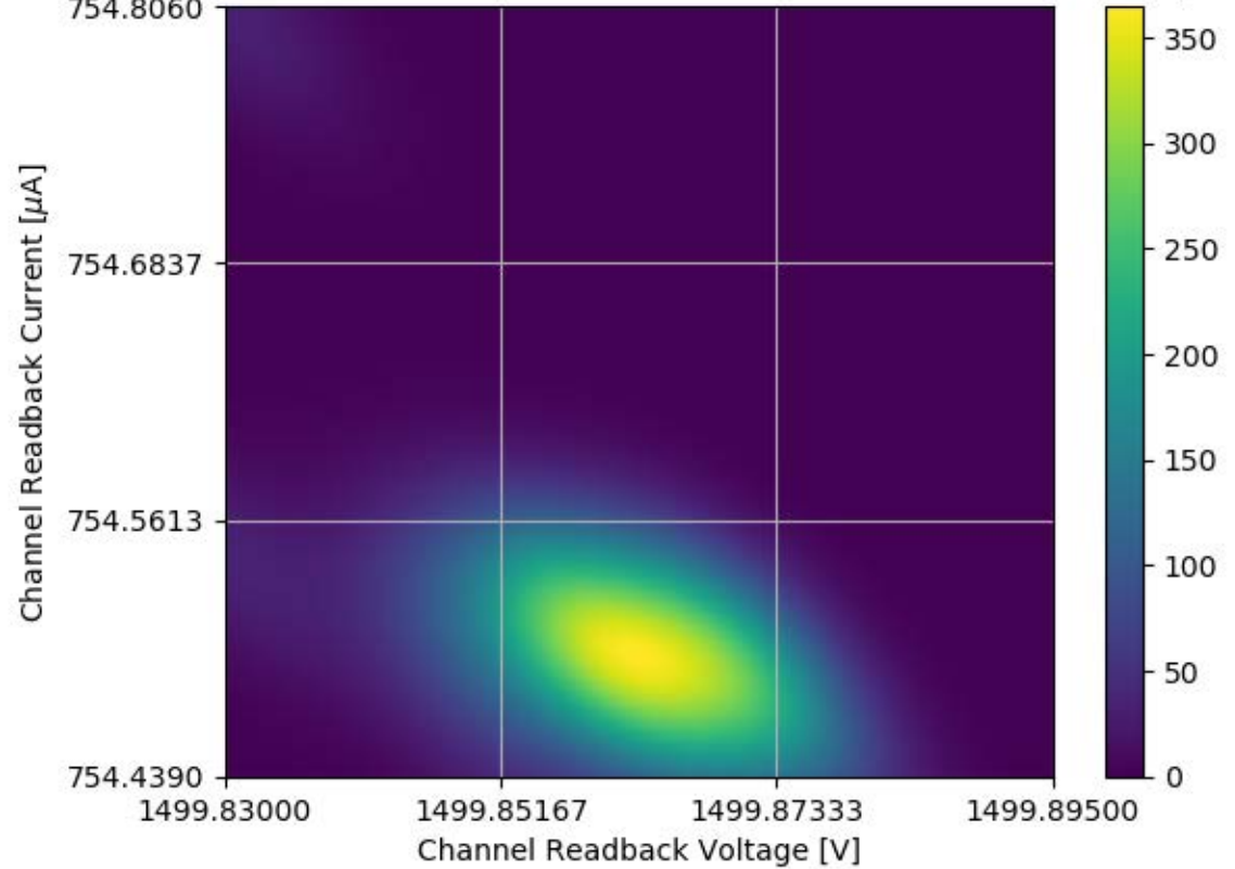
Voltage and Current Readback for Module #351 Channel 33 Stability Test
