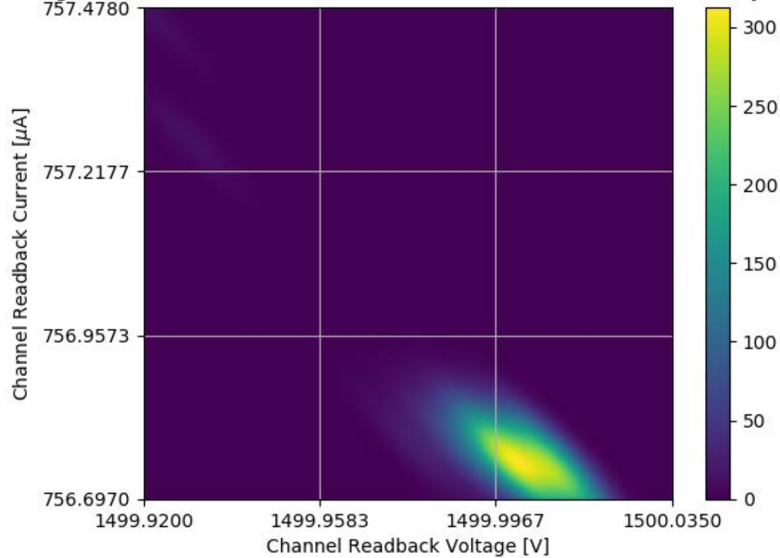
Voltage and Current Readback for Module #351 Channel 18 Stability Test
