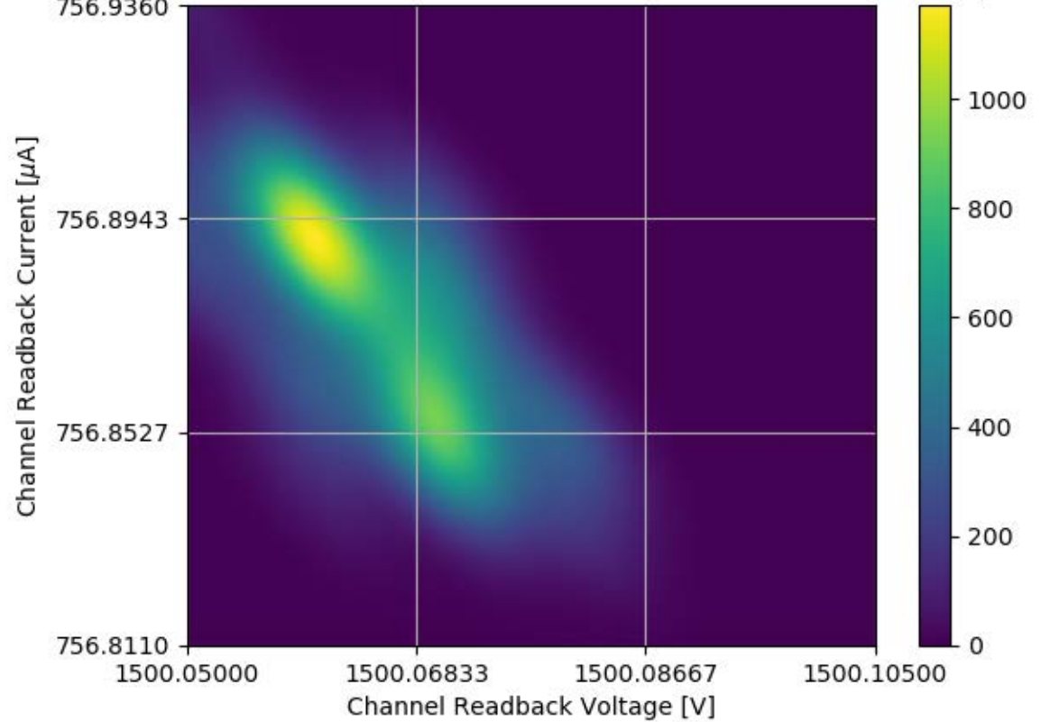
Voltage and Current Readback for Module #351 Channel 20 Stability Test
