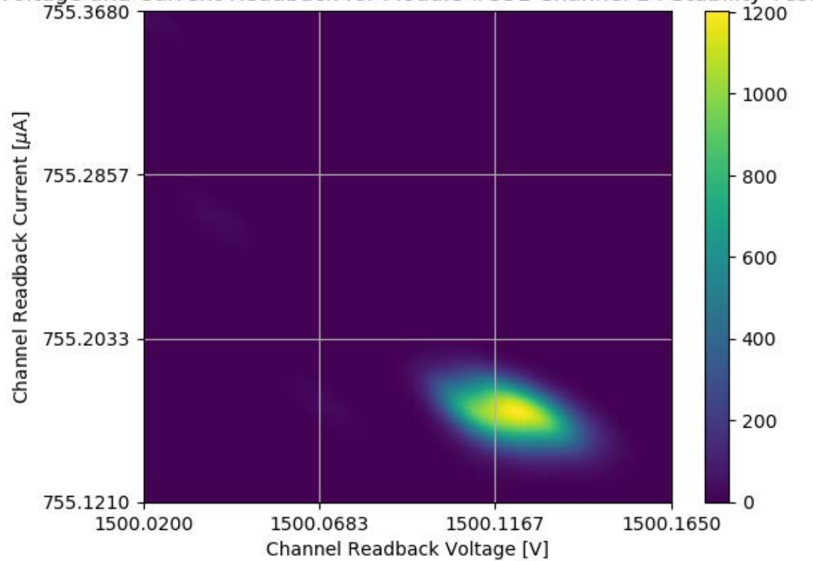
Voltage and Current Readback for Module #351 Channel 14 Stability Test
