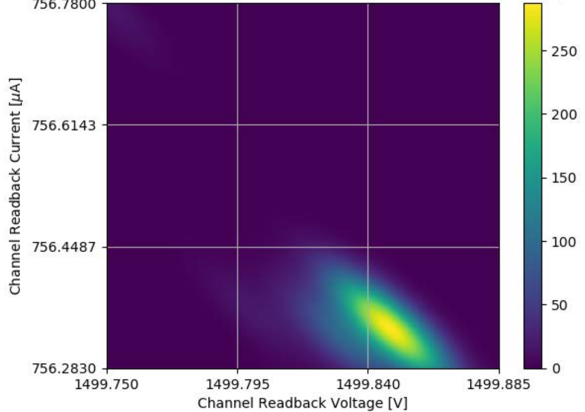
Voltage and Current Readback for Module #351 Channel 02 Stability Test
