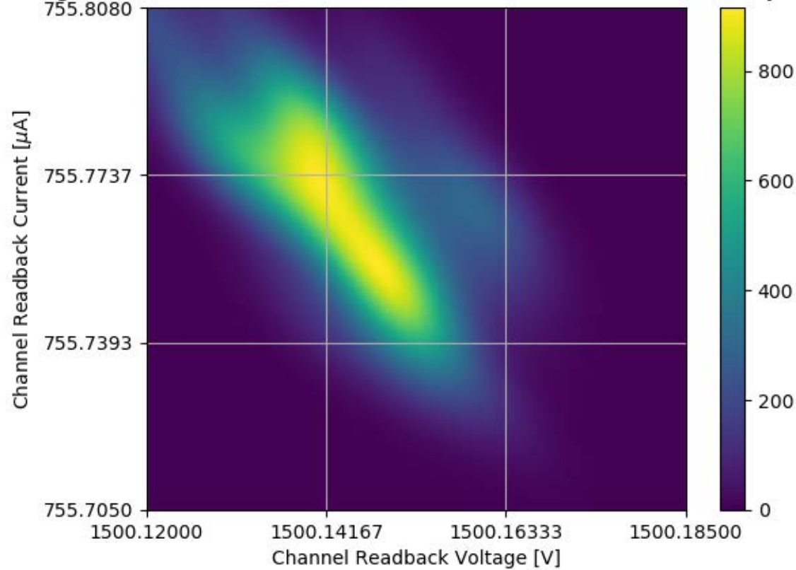
Voltage and Current Readback for Module #352 Channel 30 Stability Test
