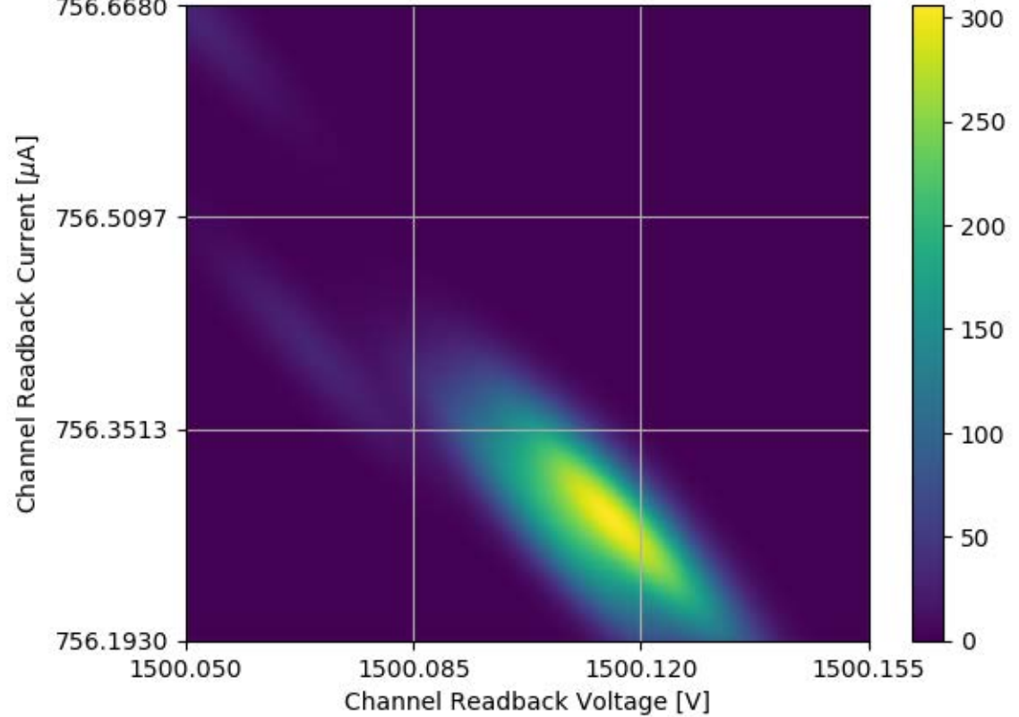
Voltage and Current Readback for Module #352 Channel 31 Stability Test
