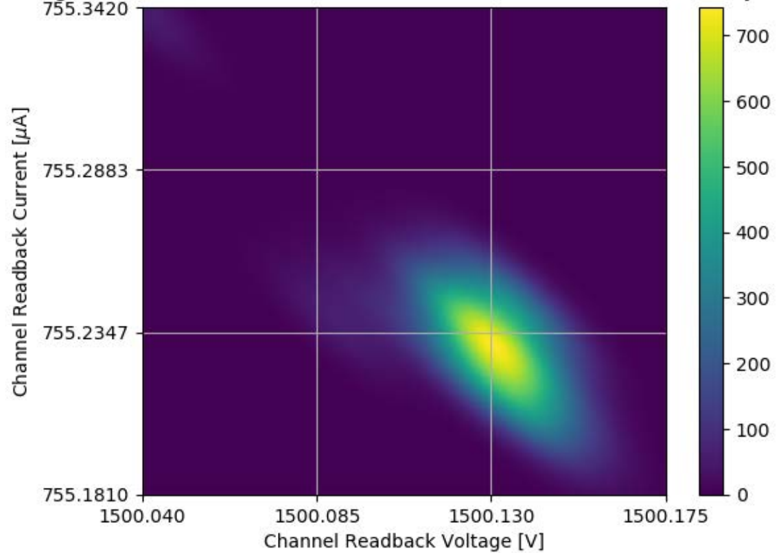
Voltage and Current Readback for Module #352 Channel 00 Stability Test
