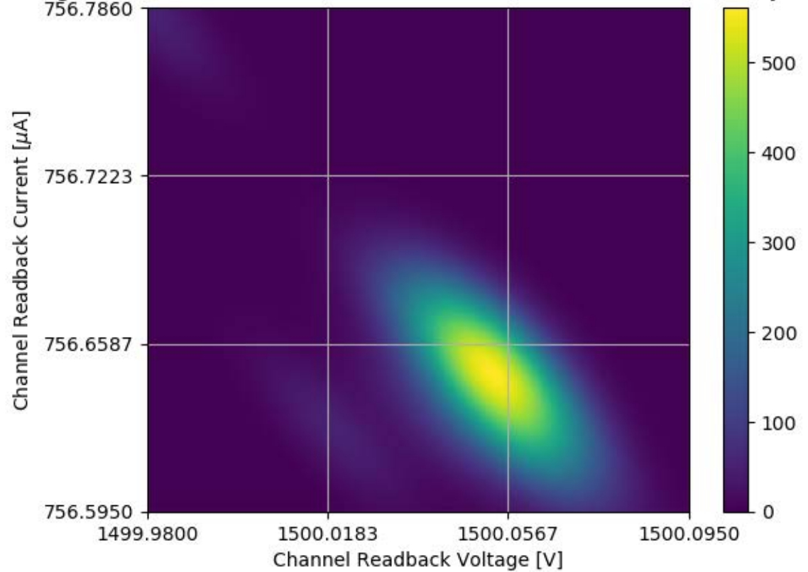
Voltage and Current Readback for Module #352 Channel 18 Stability Test
