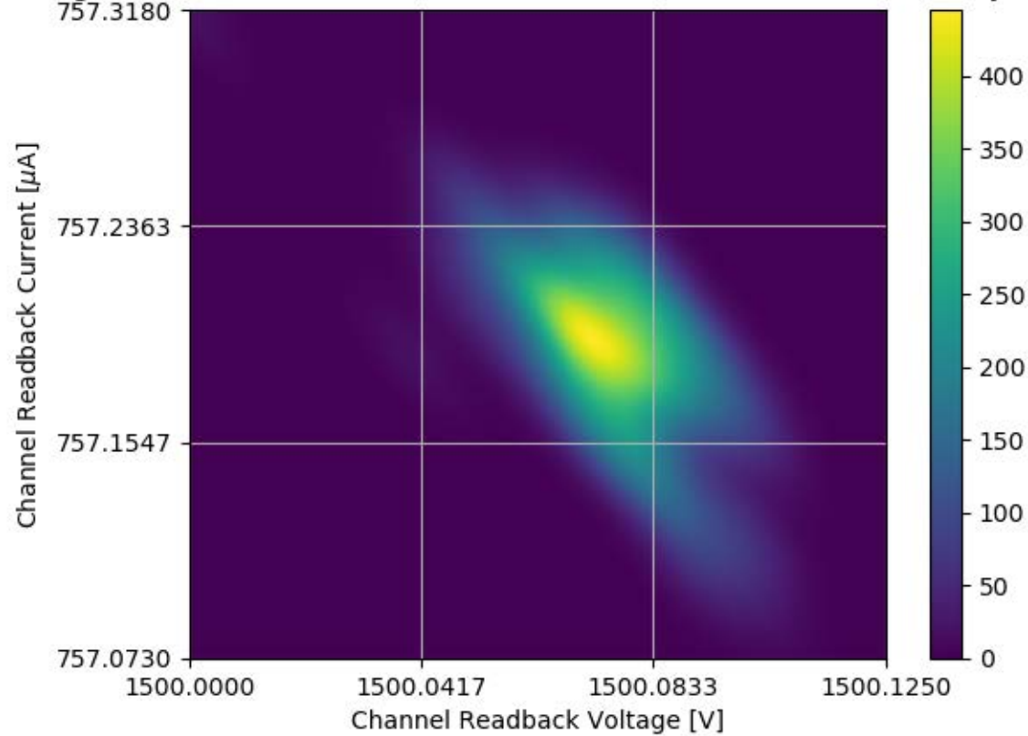
Voltage and Current Readback for Module #352 Channel 07 Stability Test
