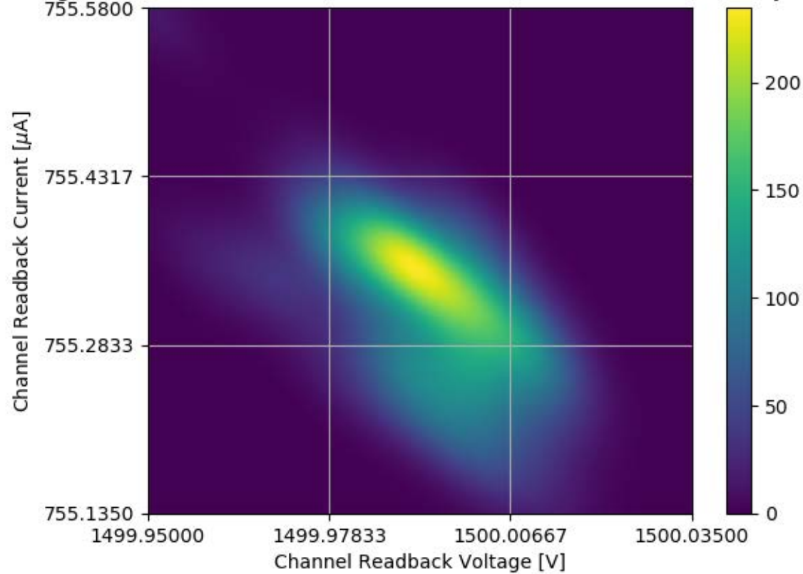
Voltage and Current Readback for Module #352 Channel 33 Stability Test
