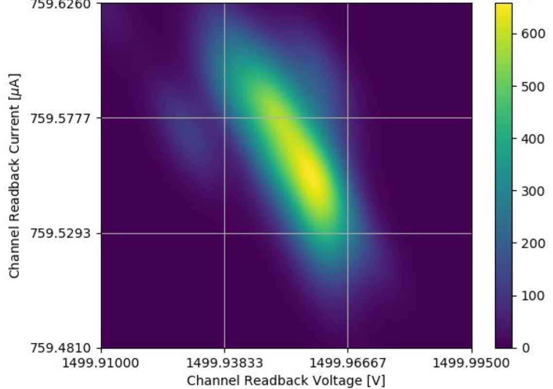
Voltage and Current Readback for Module #352 Channel 04 Stability Test
