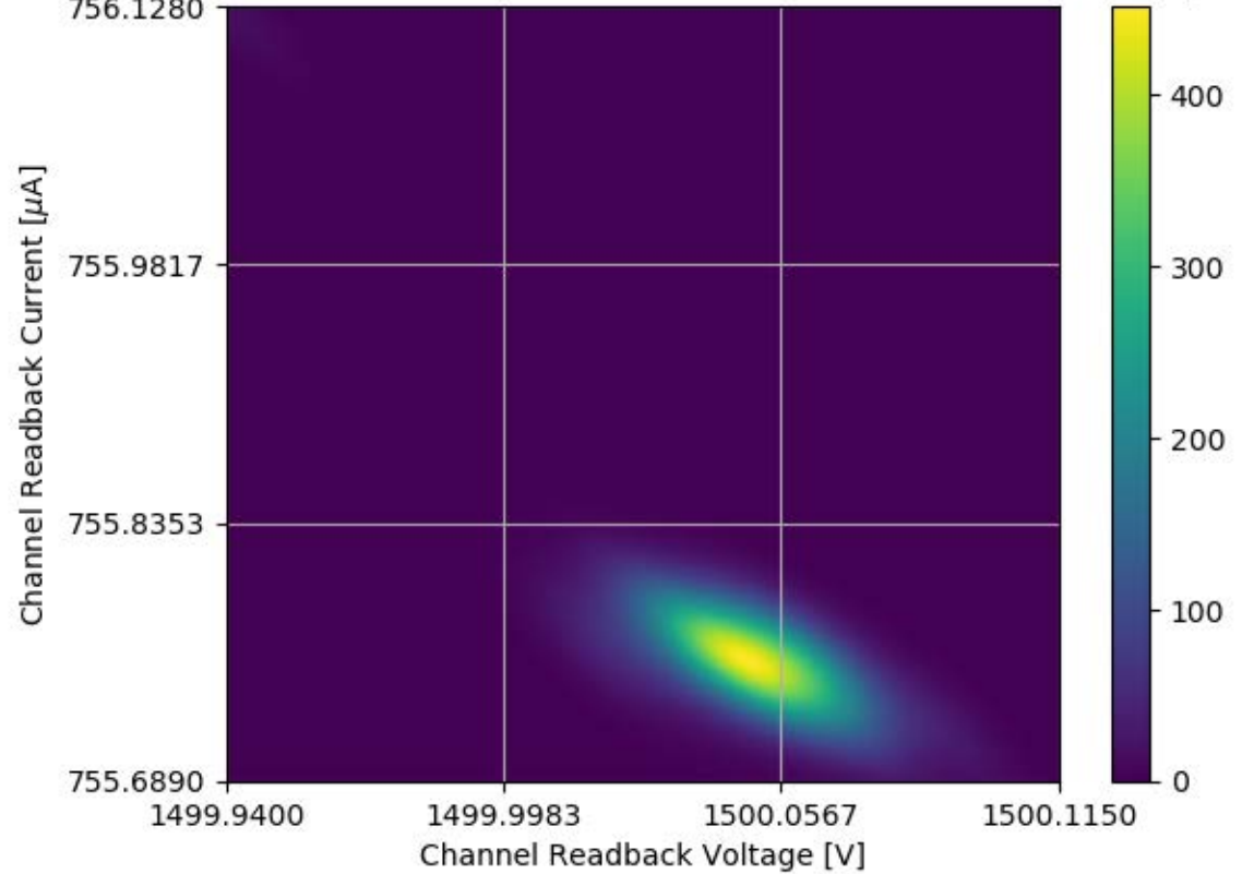
Voltage and Current Readback for Module #352 Channel 01 Stability Test
