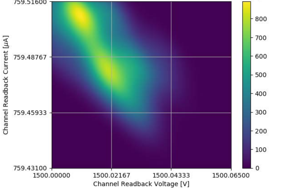
Voltage and Current Readback for Module #352 Channel 25 Stability Test
