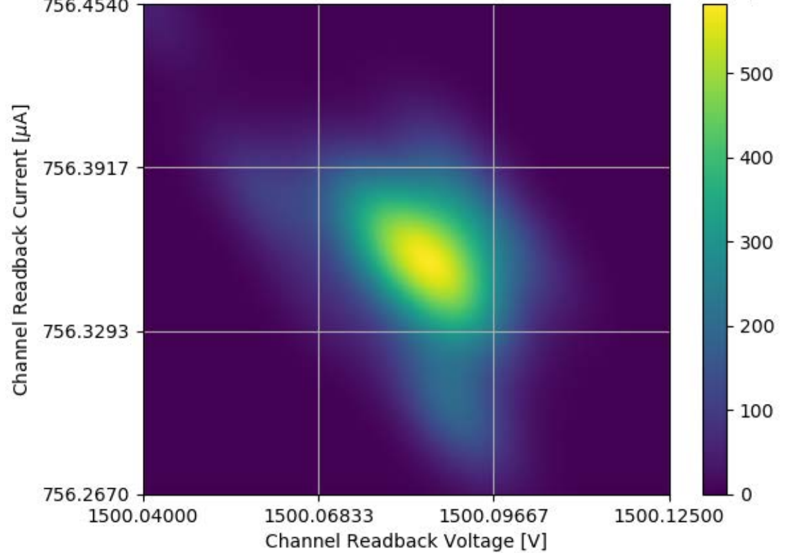
Voltage and Current Readback for Module #352 Channel 17 Stability Test
