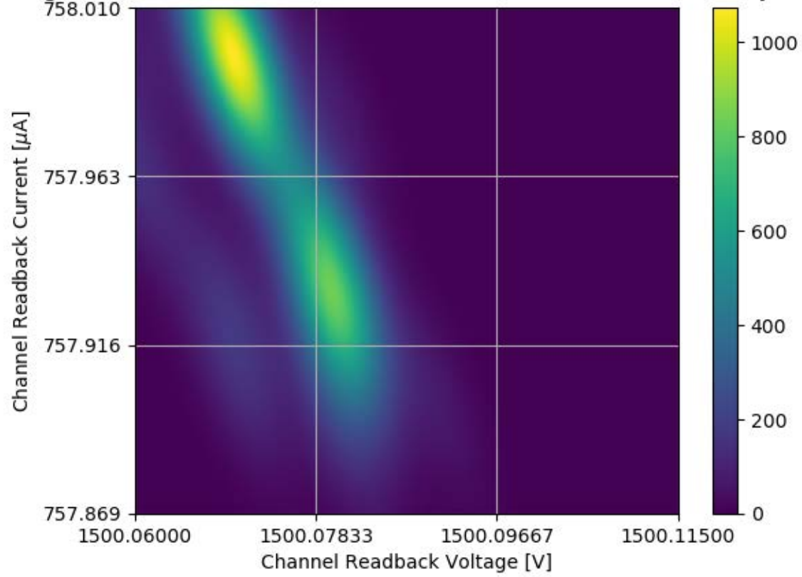
Voltage and Current Readback for Module #352 Channel 32 Stability Test
