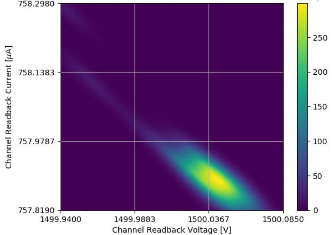
Voltage and Current Readback for Module #352 Channel 06 Stability Test
