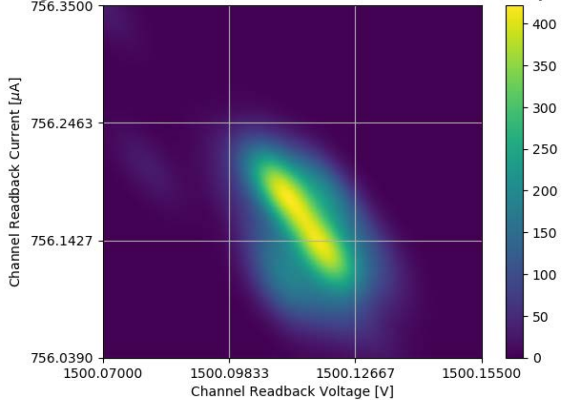
Voltage and Current Readback for Module #352 Channel 28 Stability Test
