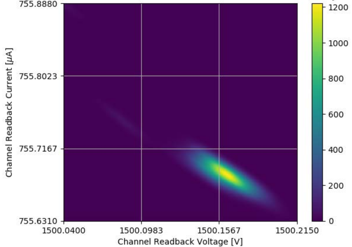
Voltage and Current Readback for Module #352 Channel 03 Stability Test
