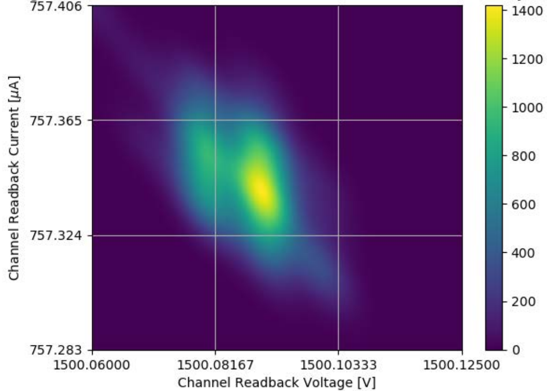
Voltage and Current Readback for Module #352 Channel 29 Stability Test
