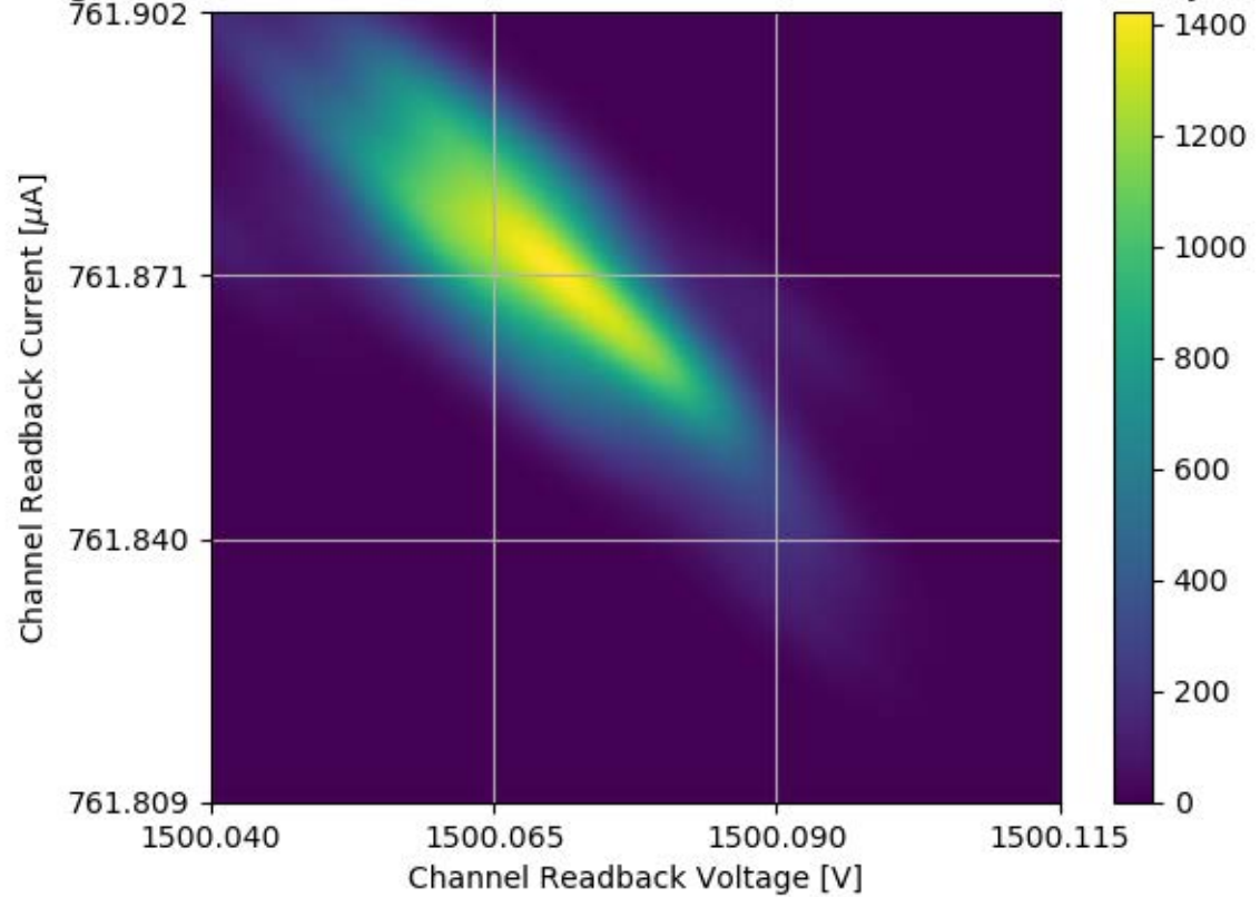
Voltage and Current Readback for Module #352 Channel 09 Stability Test
