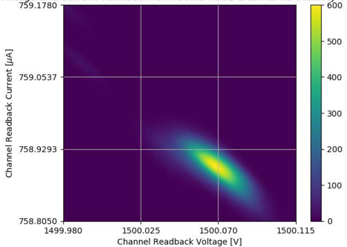
Voltage and Current Readback for Module #352 Channel 05 Stability Test
