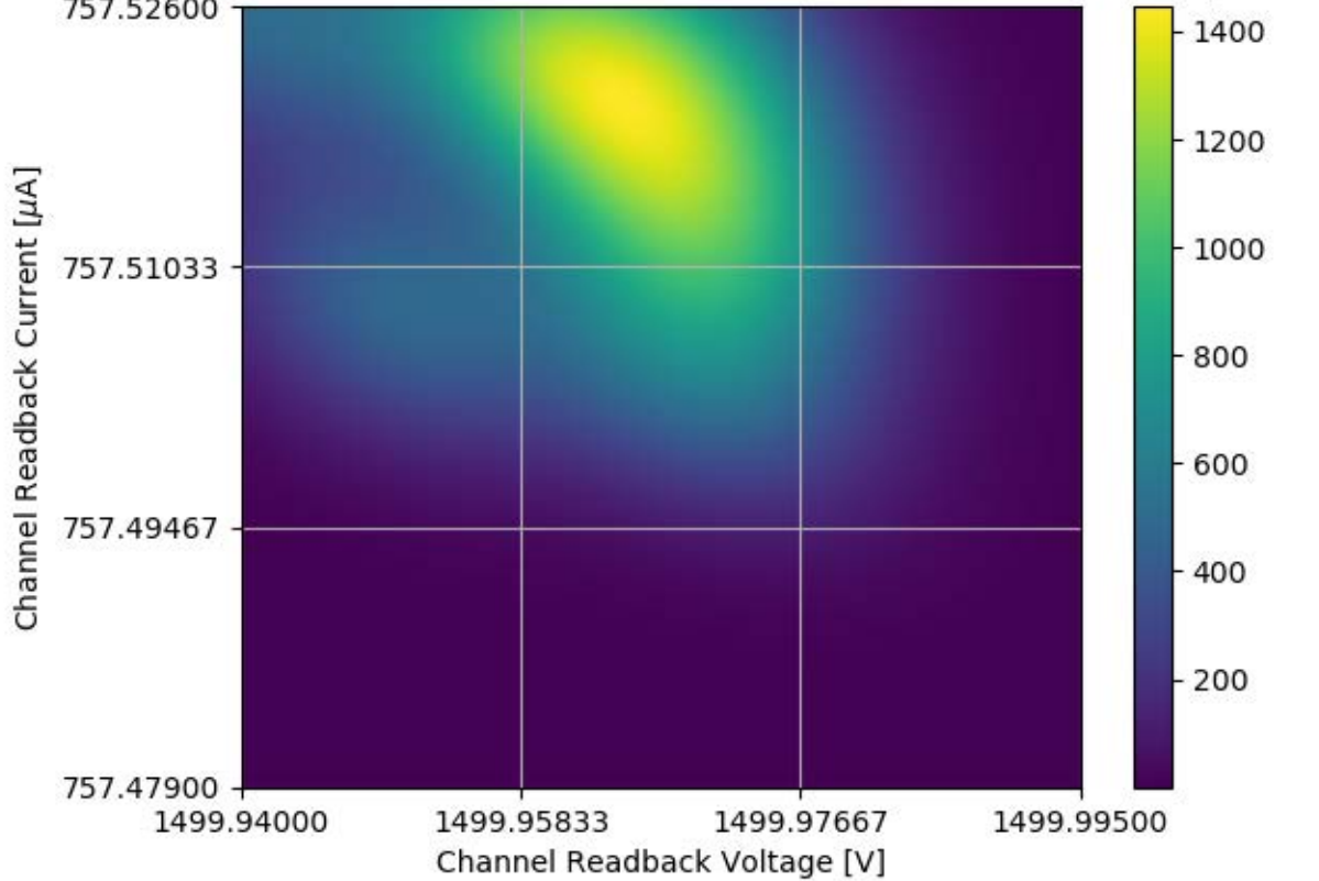
Voltage and Current Readback for Module #352 Channel 19 Stability Test
