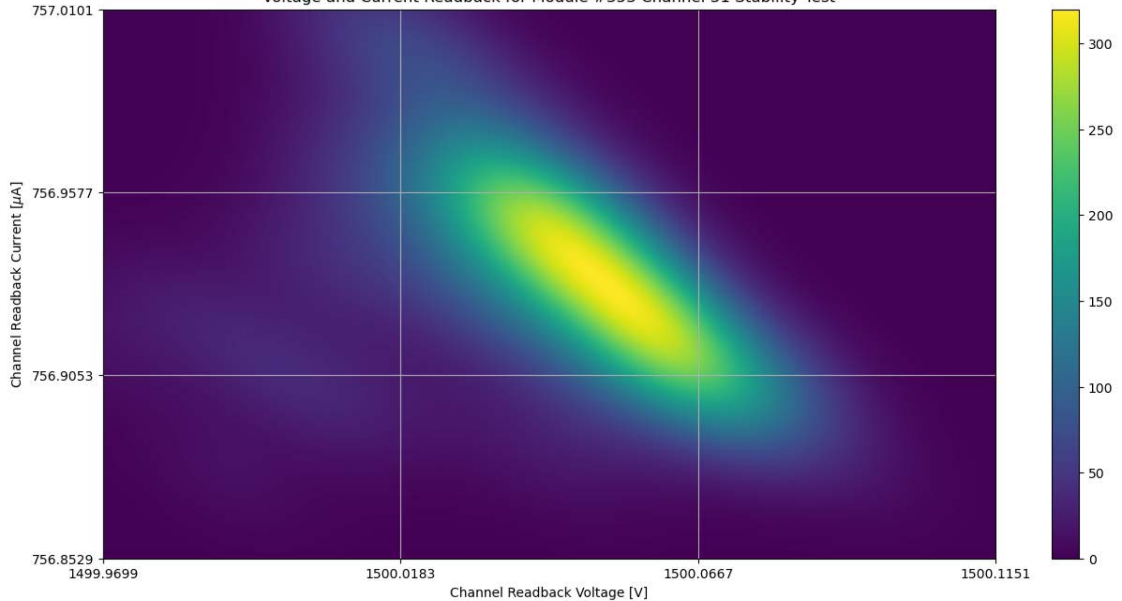
Voltage and Current Readback for Module #353 Channel 31 Stability Test
