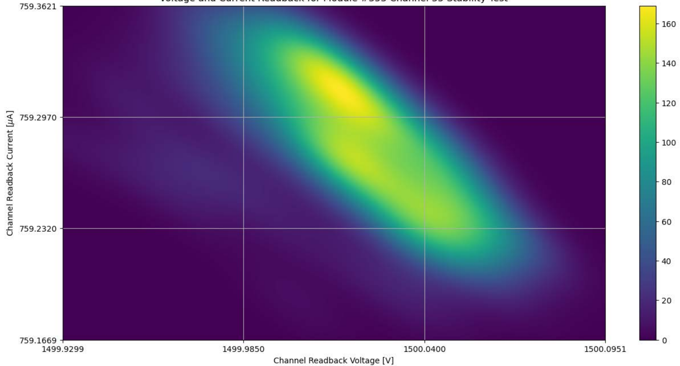
Voltage and Current Readback for Module #353 Channel 35 Stability Test
