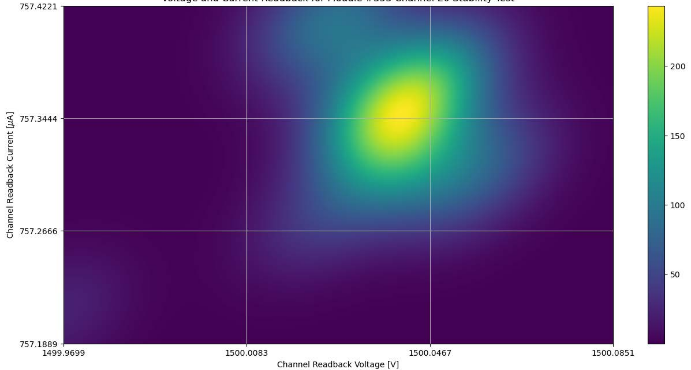
Voltage and Current Readback for Module #353 Channel 20 Stability Test
