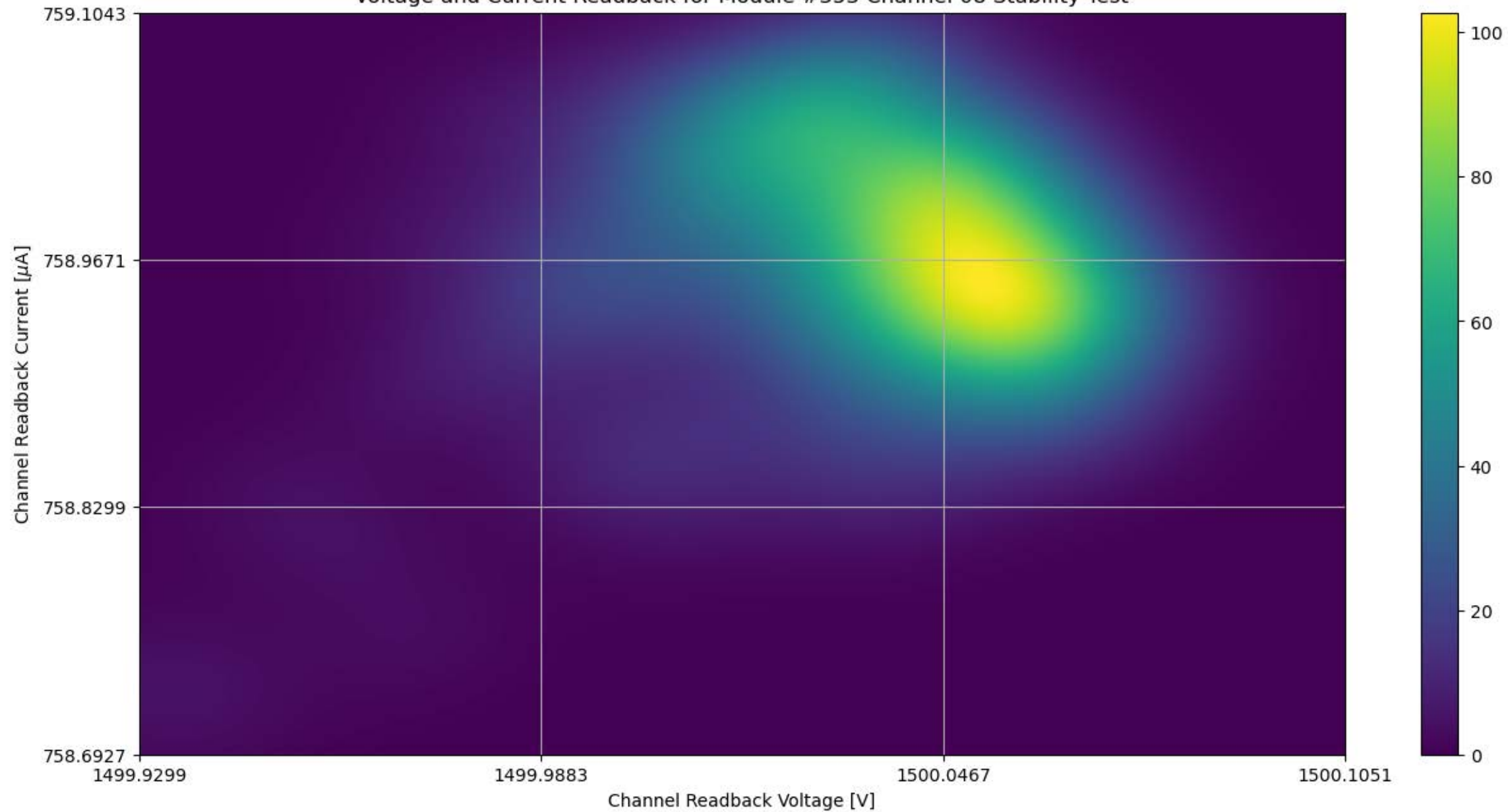
Voltage and Current Readback for Module #353 Channel 08 Stability Test
