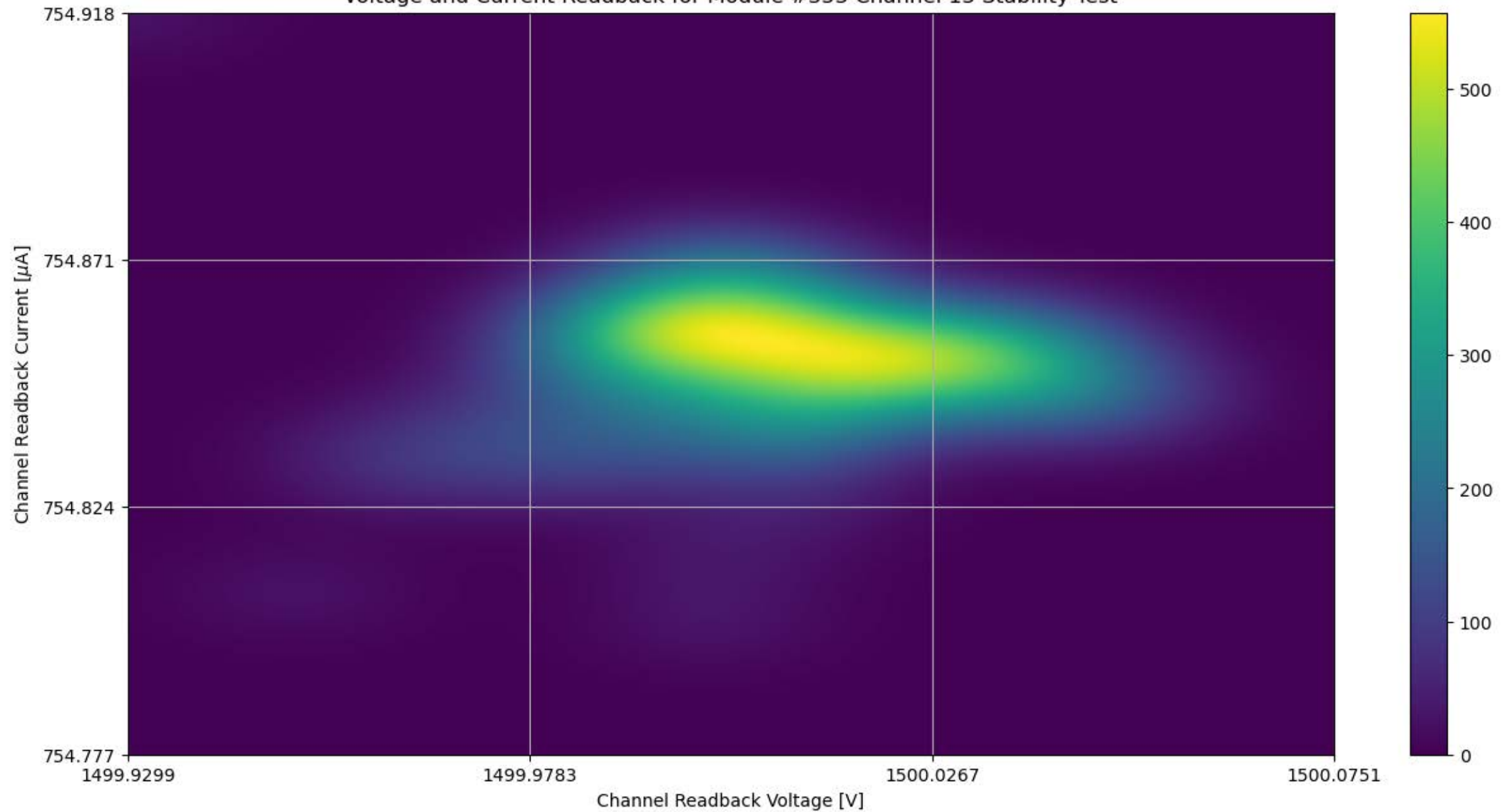
Voltage and Current Readback for Module #353 Channel 13 Stability Test
