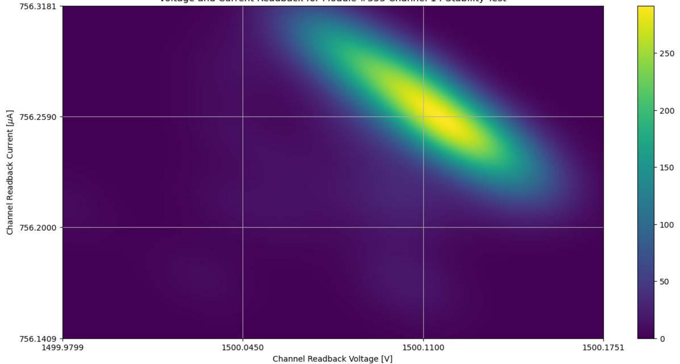
Voltage and Current Readback for Module #353 Channel 14 Stability Test
