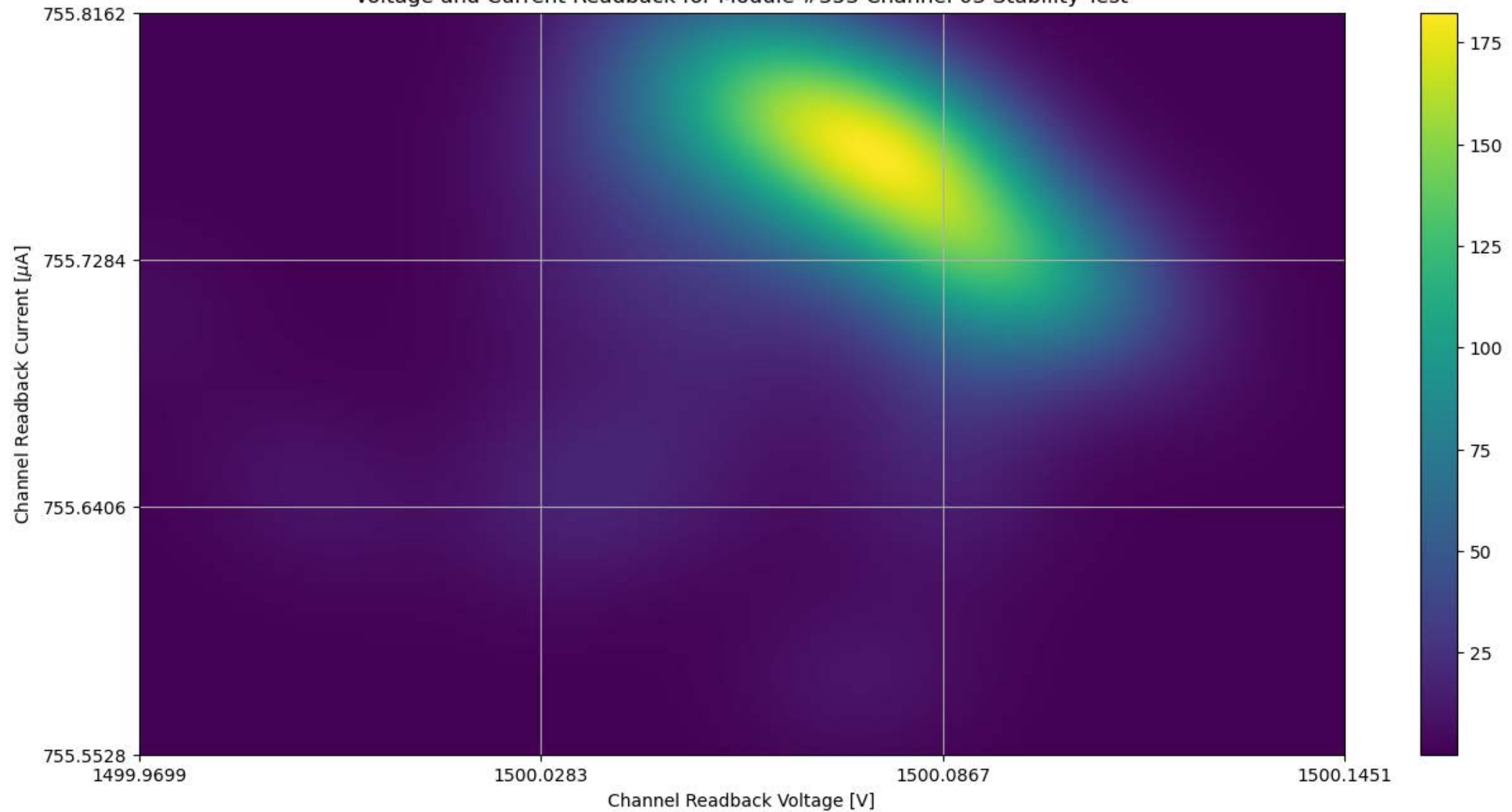
Voltage and Current Readback for Module #353 Channel 03 Stability Test
