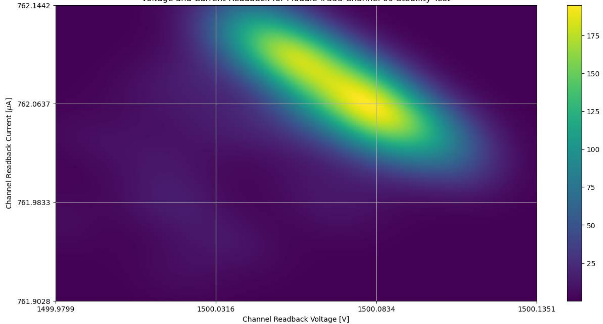
Voltage and Current Readback for Module #353 Channel 09 Stability Test
