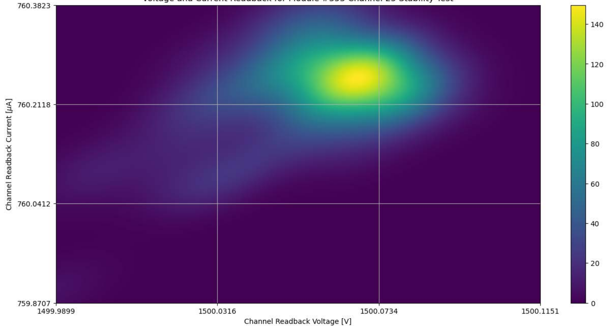
Voltage and Current Readback for Module #353 Channel 25 Stability Test
