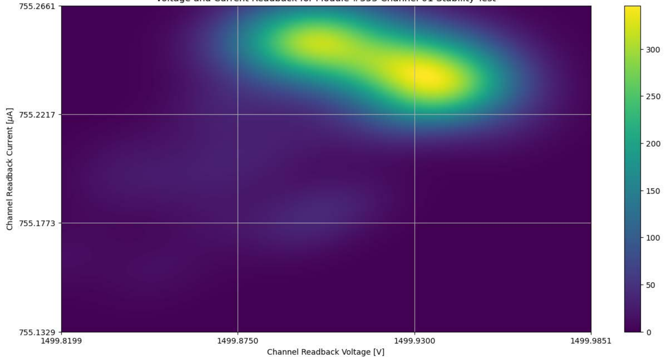
Voltage and Current Readback for Module #353 Channel 01 Stability Test
