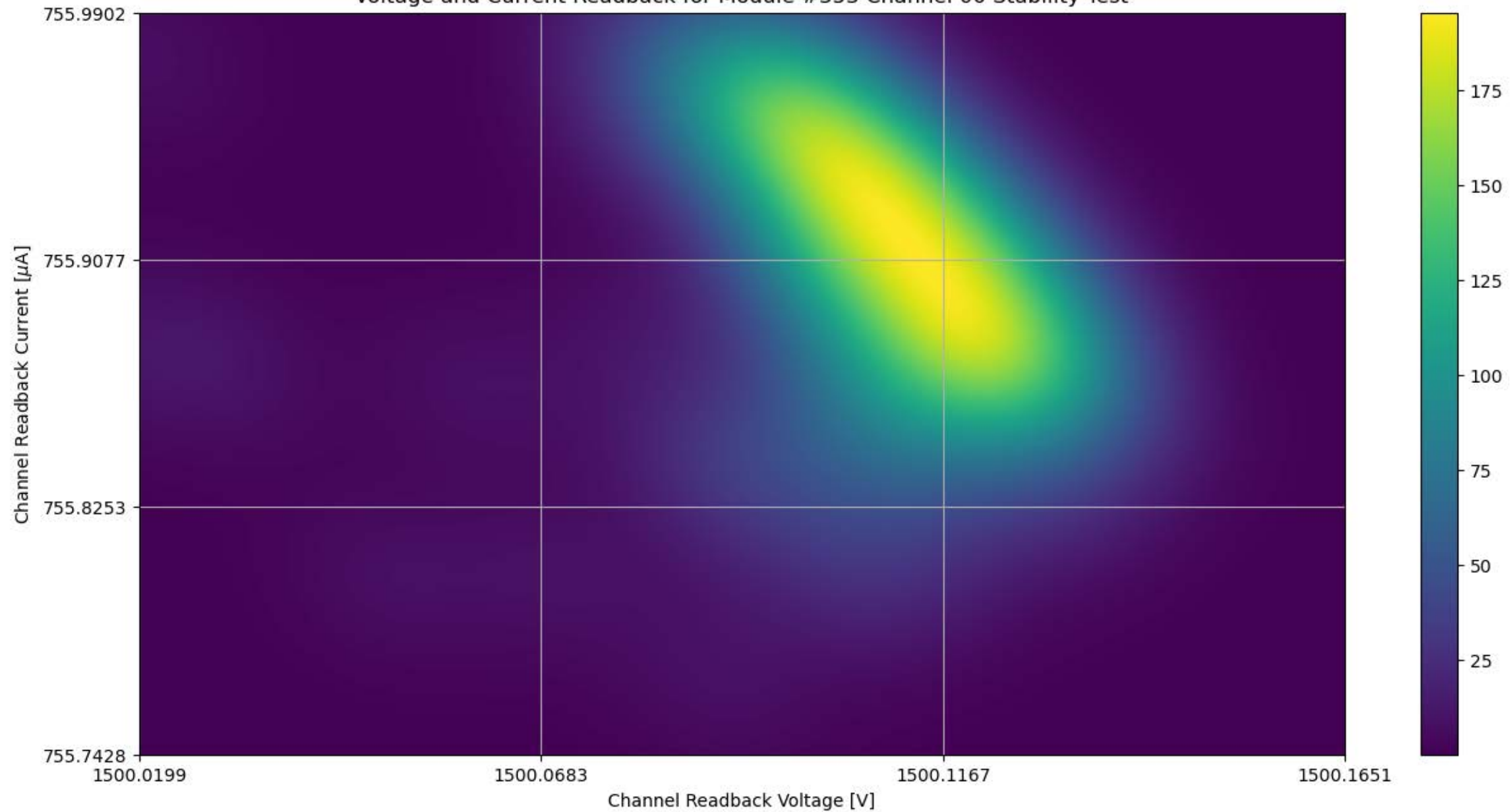
Voltage and Current Readback for Module #353 Channel 00 Stability Test
