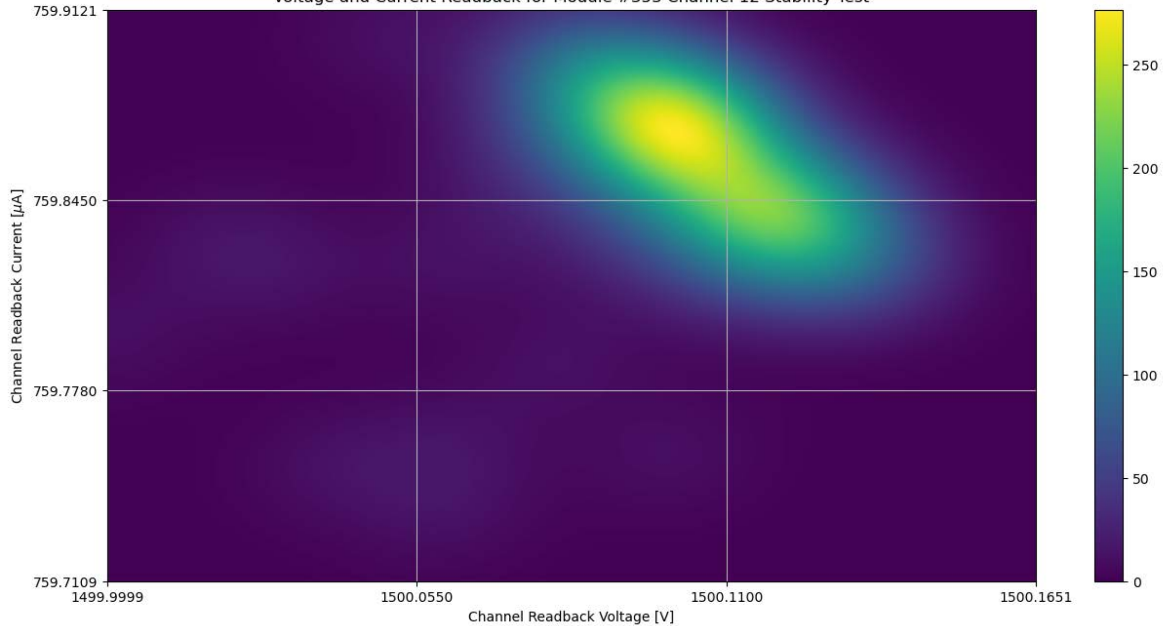
Voltage and Current Readback for Module #353 Channel 12 Stability Test
