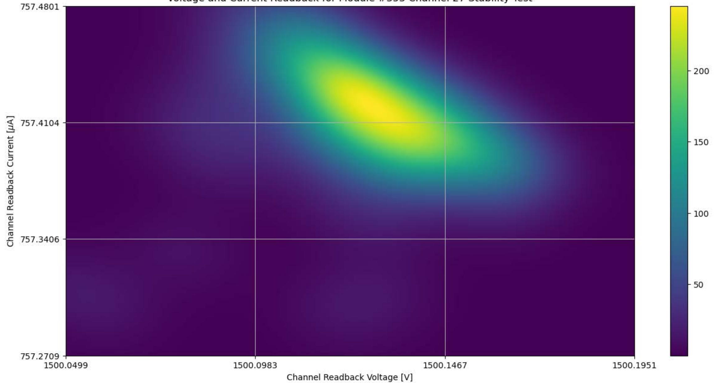
Voltage and Current Readback for Module #353 Channel 27 Stability Test
