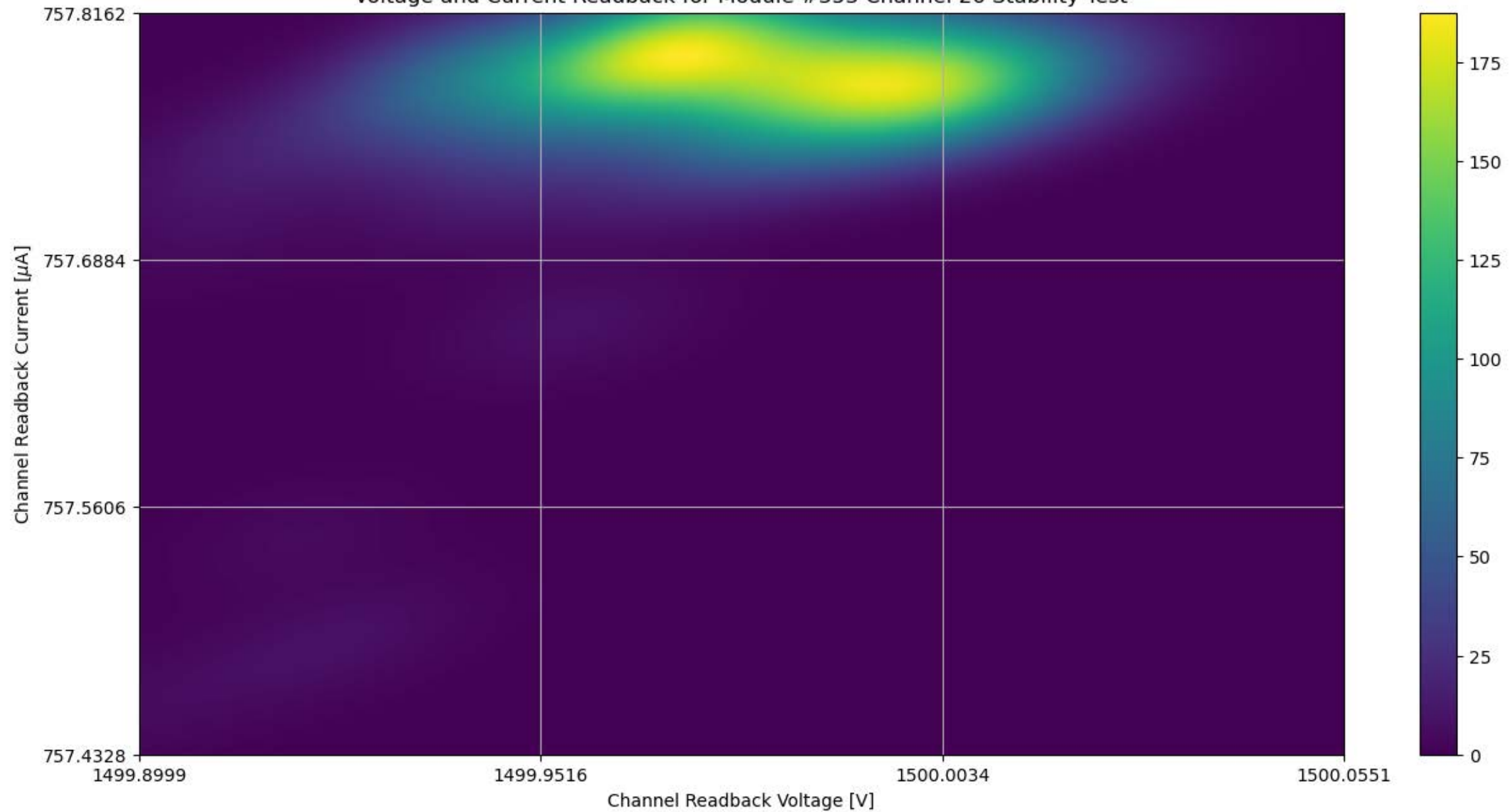
Voltage and Current Readback for Module #353 Channel 26 Stability Test
