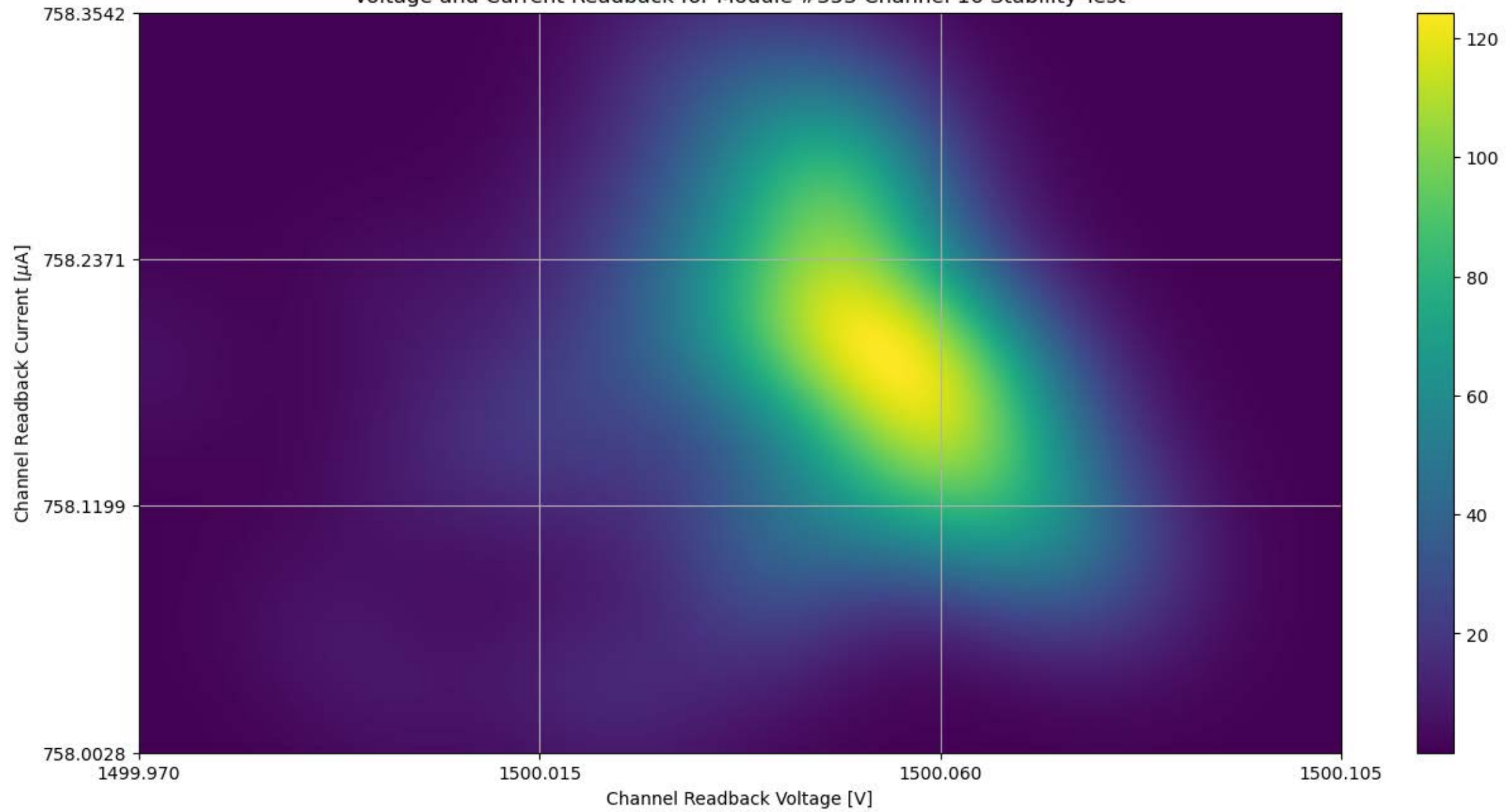
Voltage and Current Readback for Module #353 Channel 16 Stability Test
