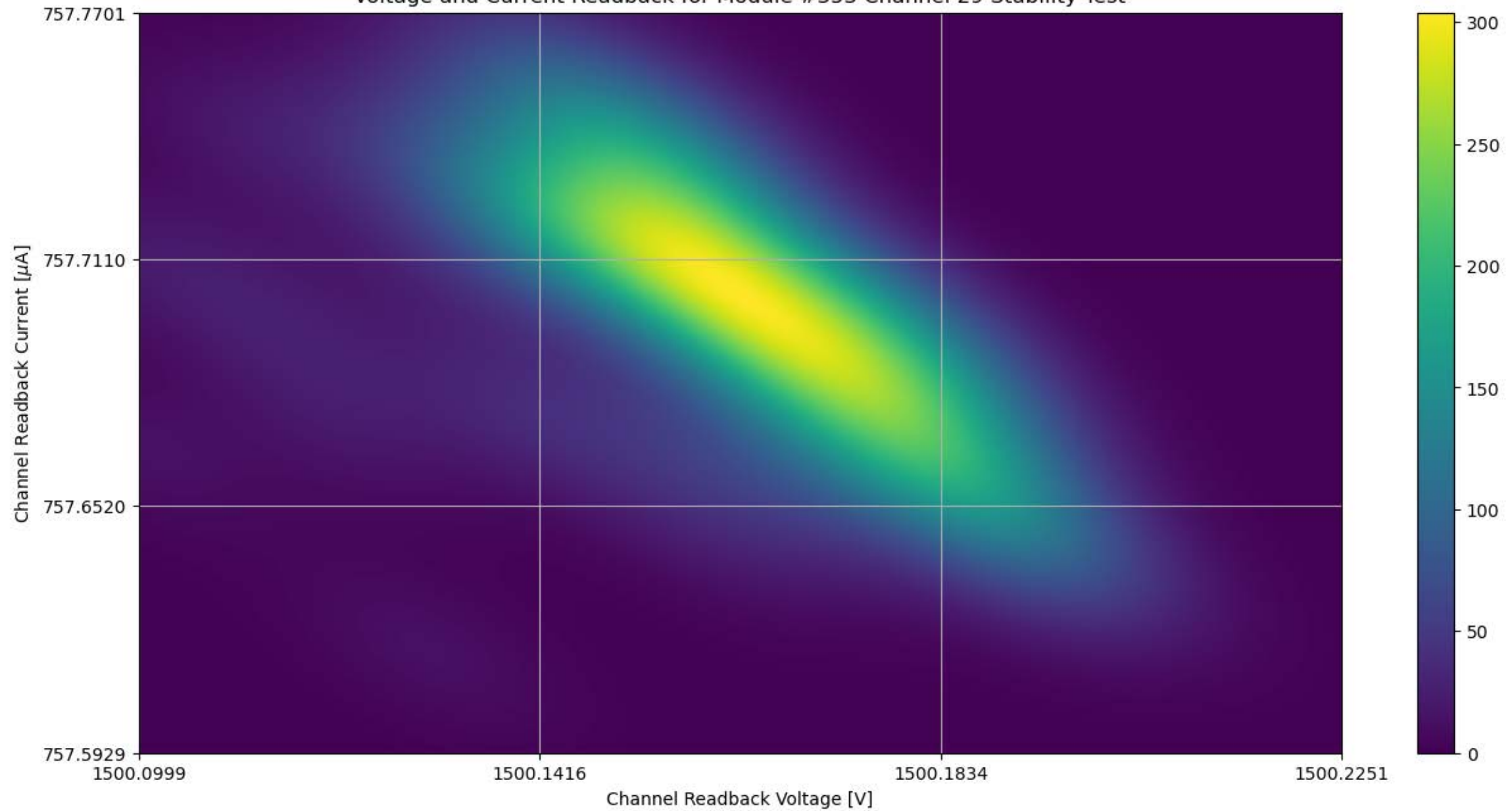
Voltage and Current Readback for Module #353 Channel 29 Stability Test
