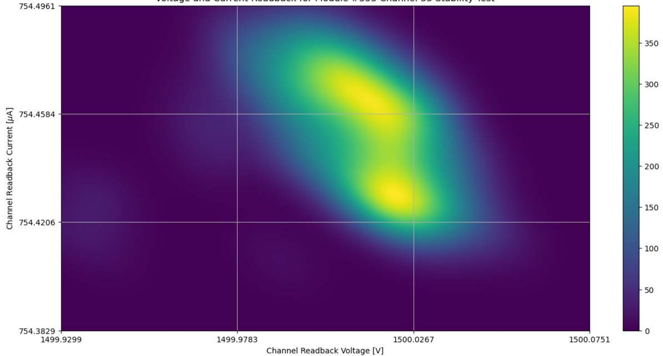
Voltage and Current Readback for Module #353 Channel 33 Stability Test
