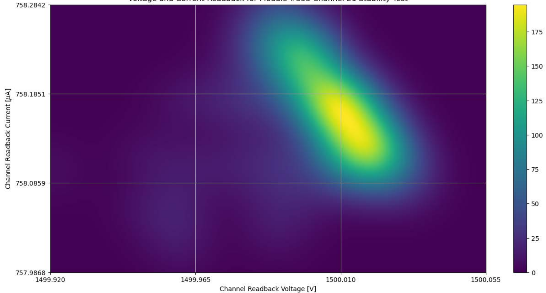
Voltage and Current Readback for Module #353 Channel 21 Stability Test
