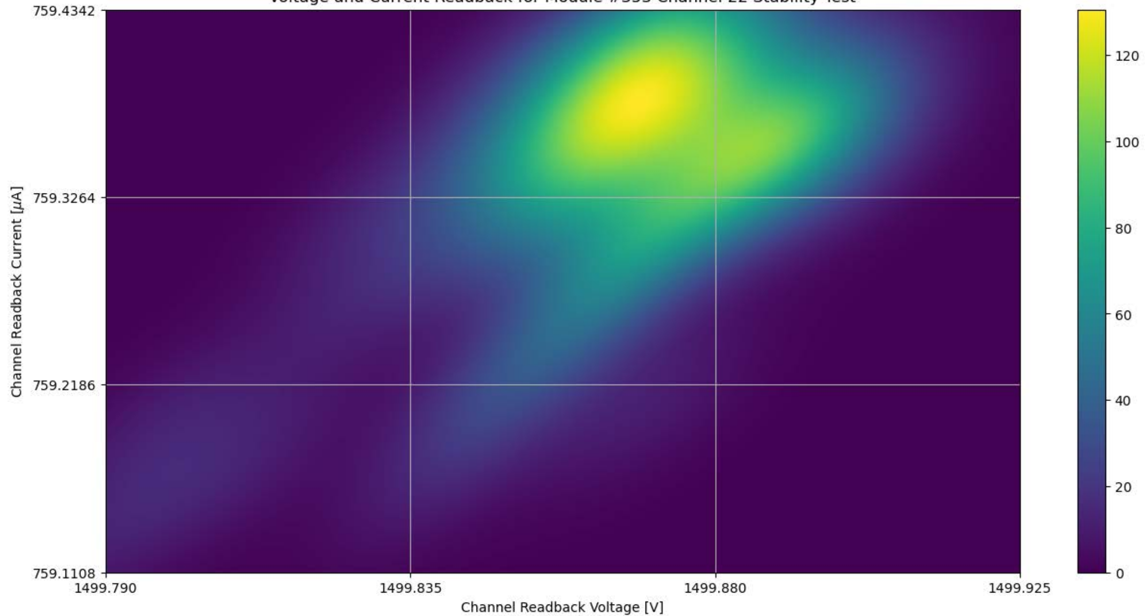
Voltage and Current Readback for Module #353 Channel 22 Stability Test
