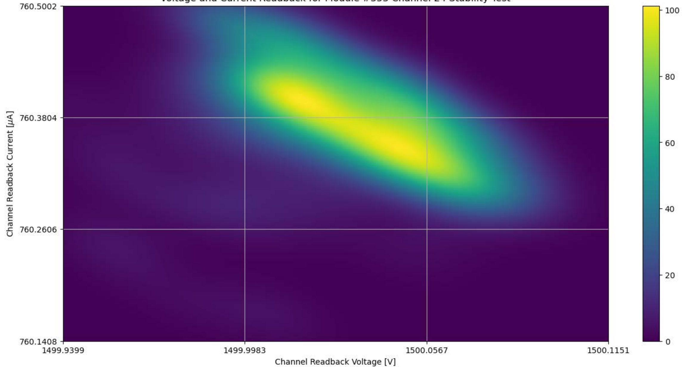
Voltage and Current Readback for Module #353 Channel 24 Stability Test
