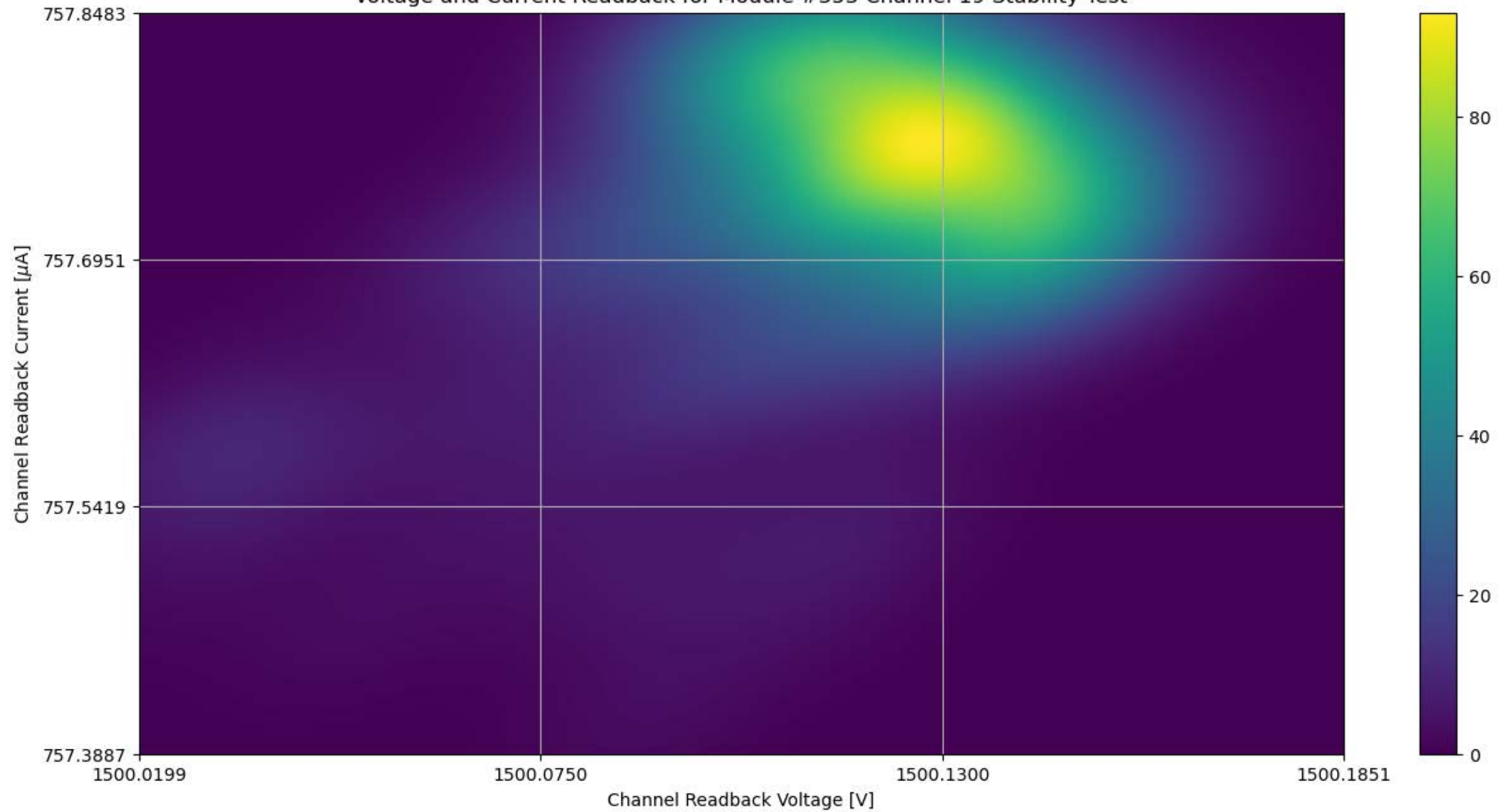
Voltage and Current Readback for Module #353 Channel 19 Stability Test
