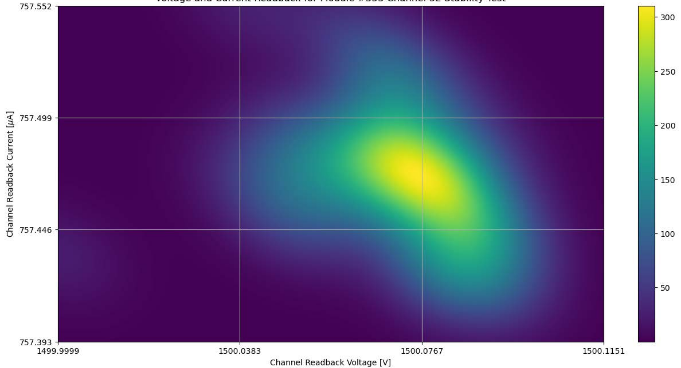
Voltage and Current Readback for Module #353 Channel 32 Stability Test
