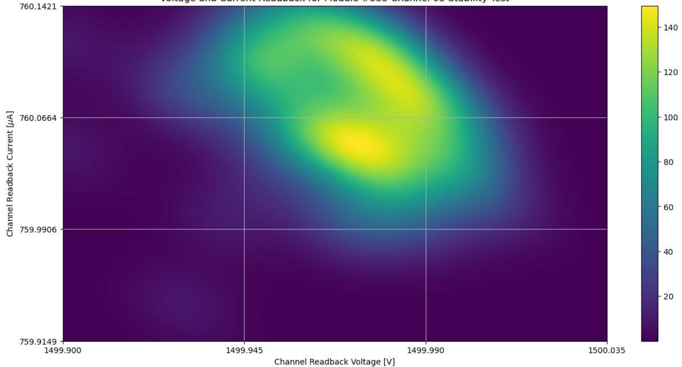
Voltage and Current Readback for Module #353 Channel 05 Stability Test
