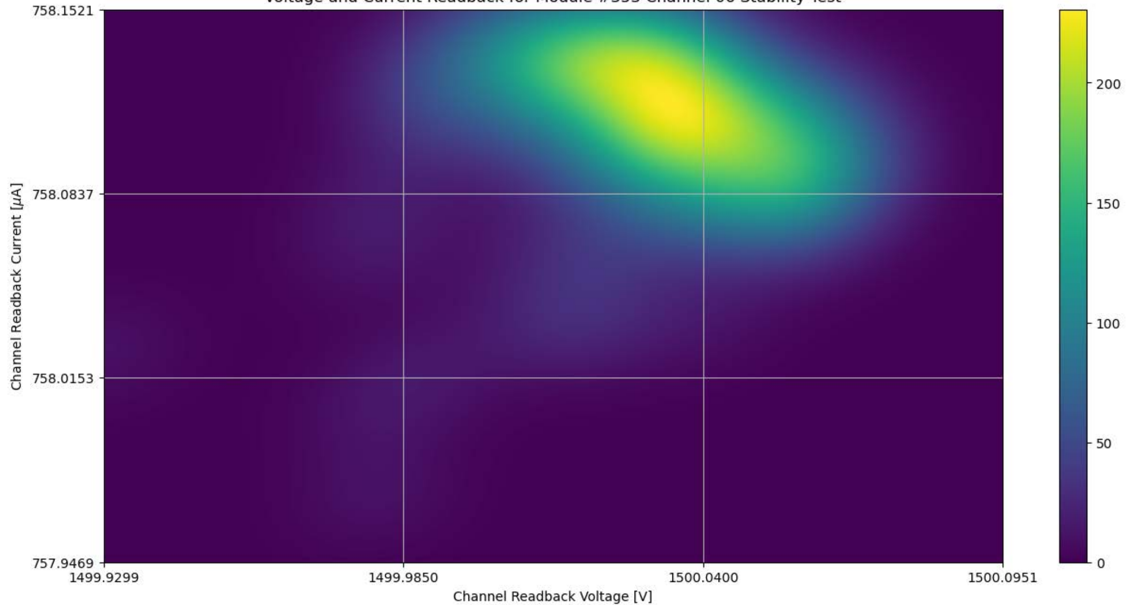
Voltage and Current Readback for Module #353 Channel 06 Stability Test
