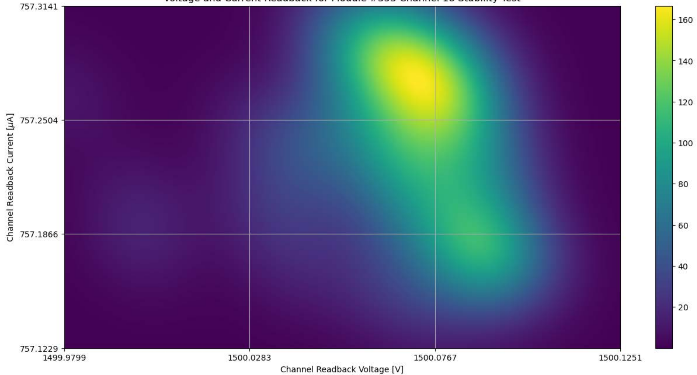
Voltage and Current Readback for Module #353 Channel 18 Stability Test
