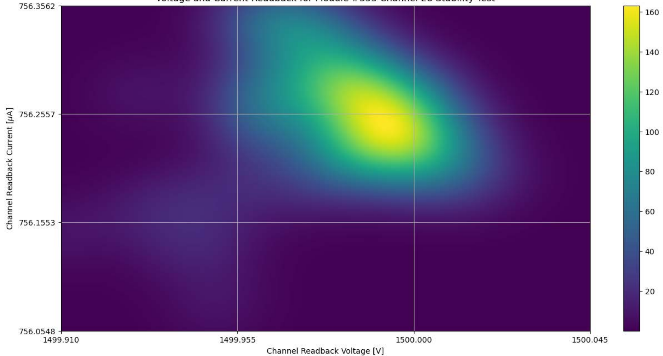
Voltage and Current Readback for Module #353 Channel 28 Stability Test
