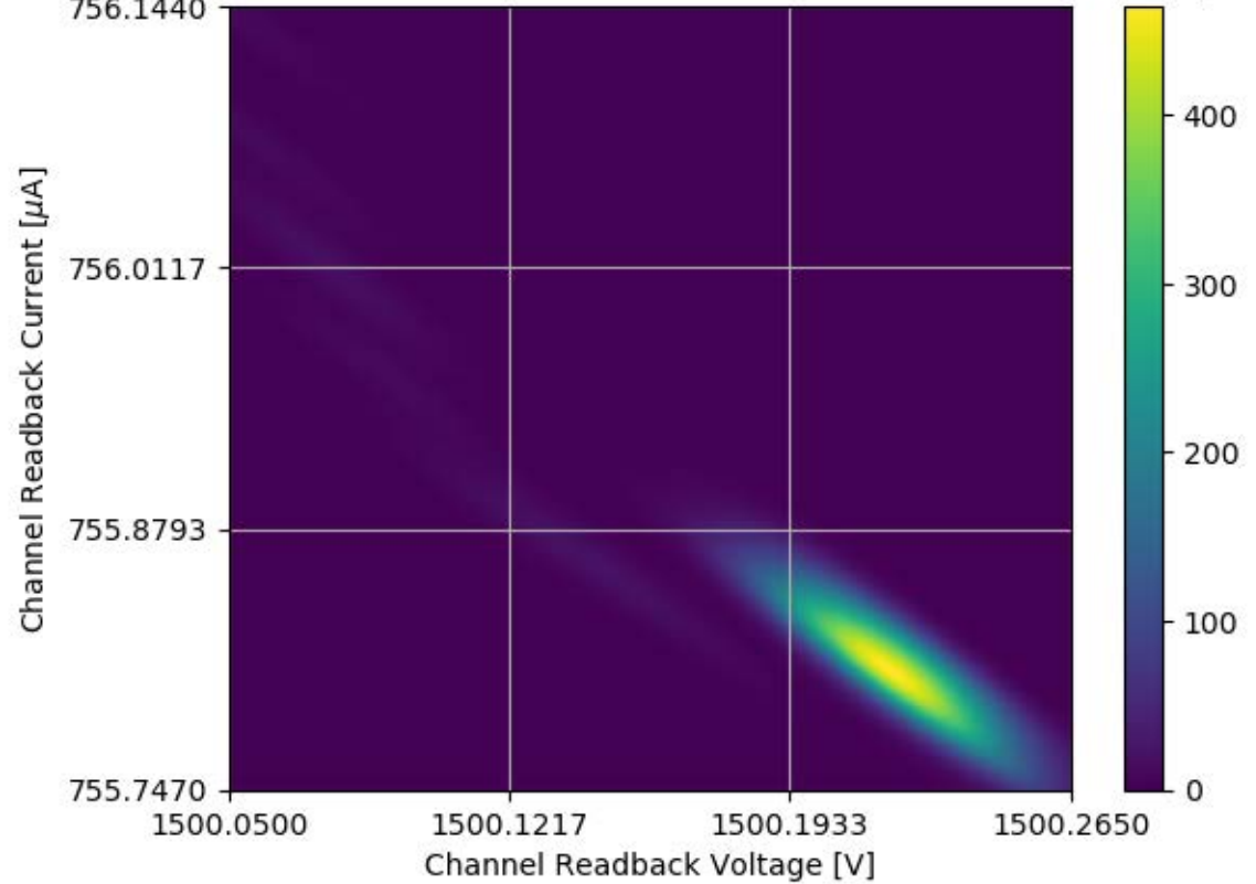
Voltage and Current Readback for Module #354 Channel 30 Stability Test
