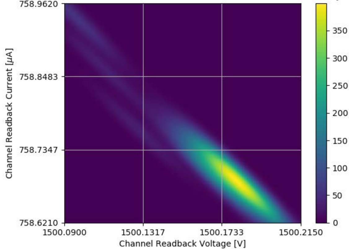
Voltage and Current Readback for Module #354 Channel 08 Stability Test
