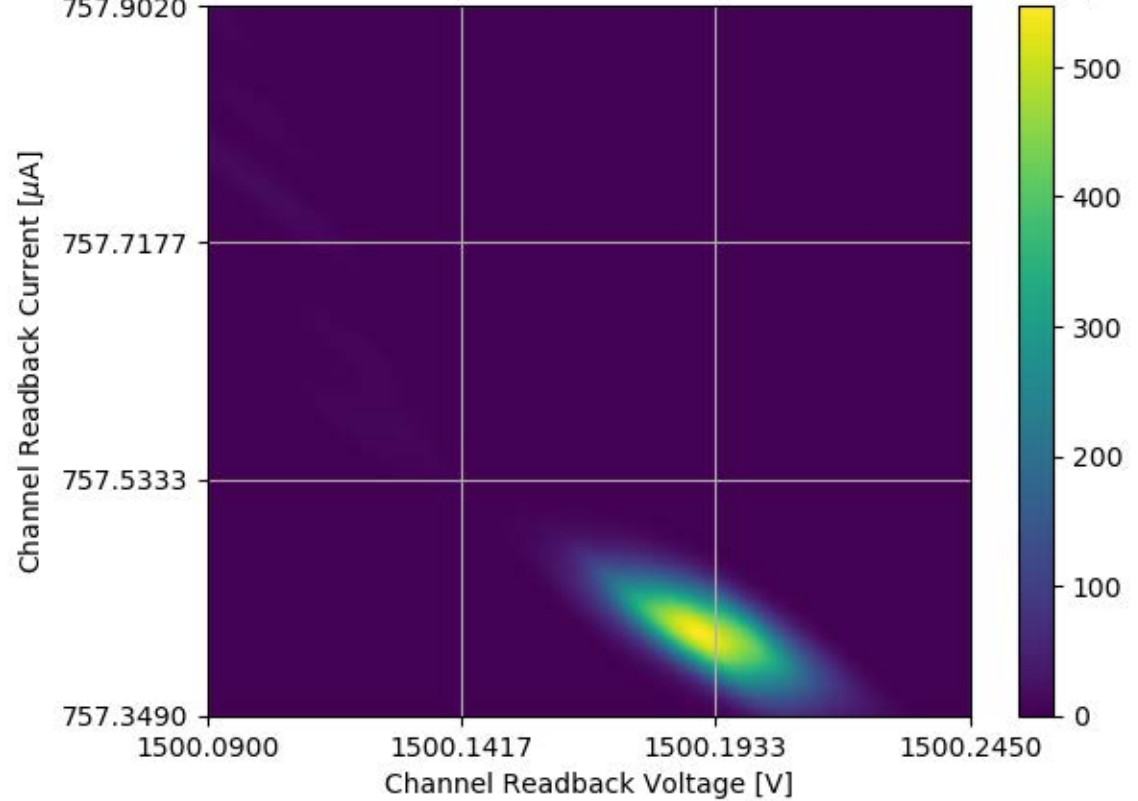
Voltage and Current Readback for Module #354 Channel 23 Stability Test
