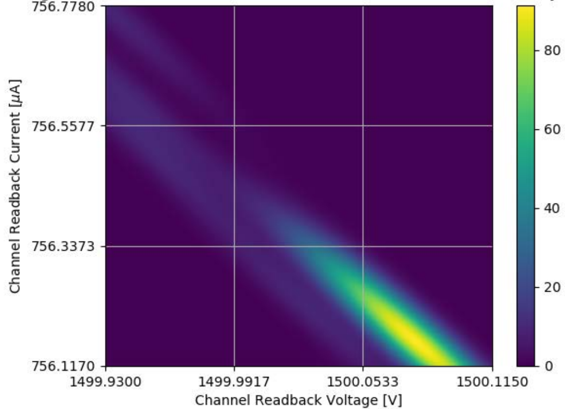
Voltage and Current Readback for Module #354 Channel 14 Stability Test
