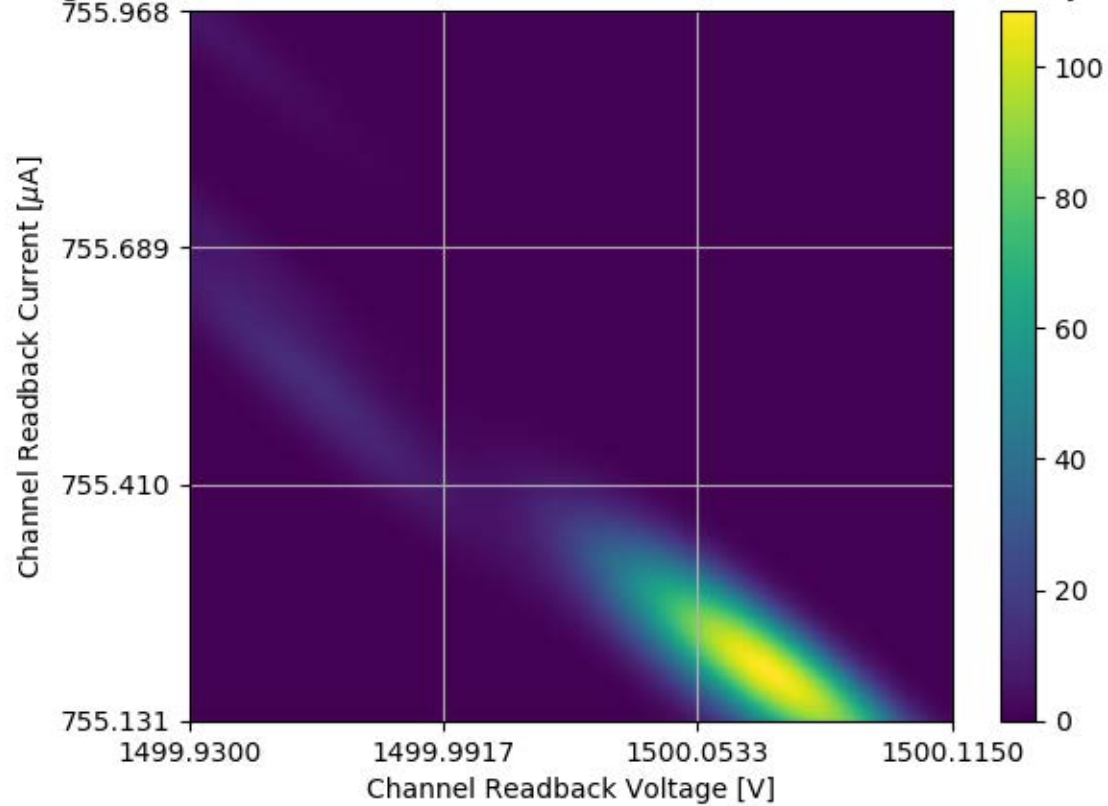
Voltage and Current Readback for Module #354 Channel 13 Stability Test
