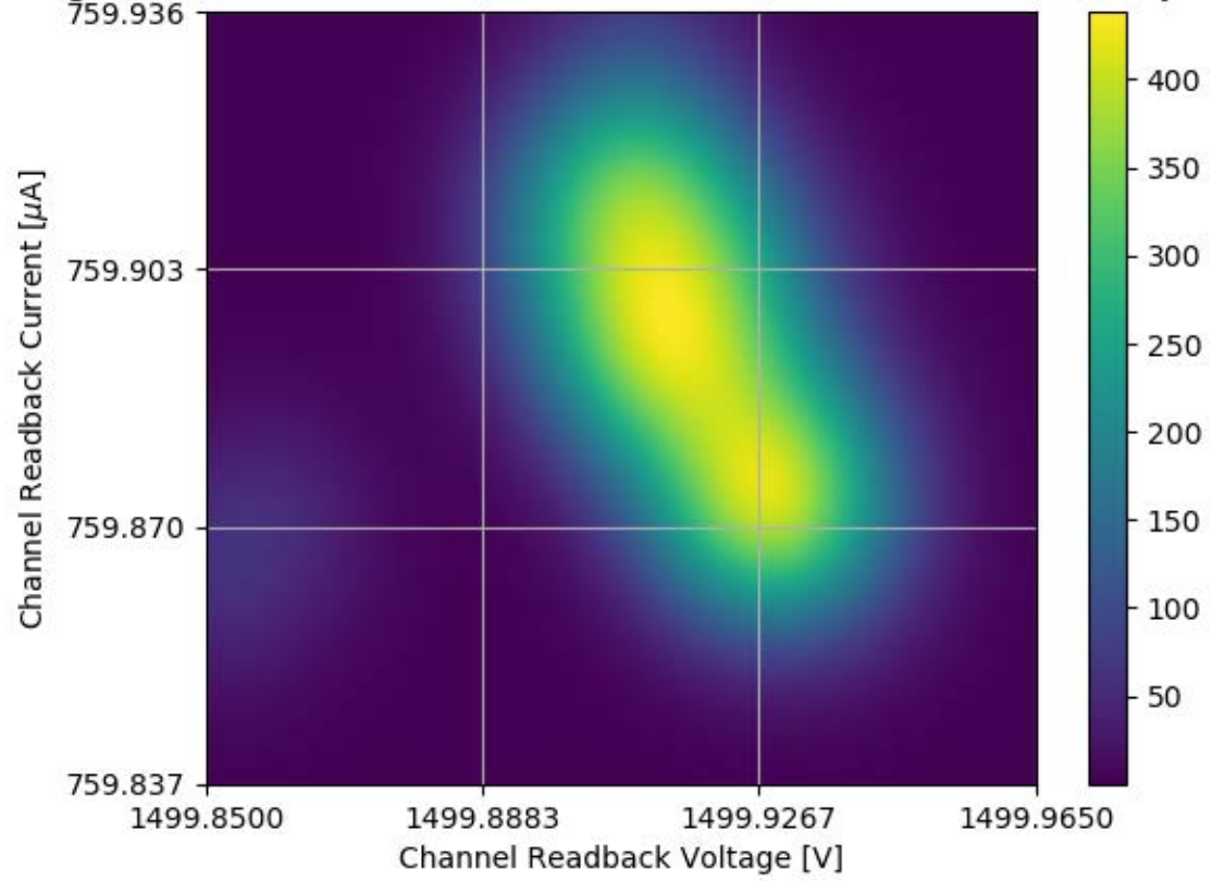
Voltage and Current Readback for Module #354 Channel 25 Stability Test
