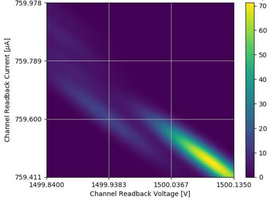
Voltage and Current Readback for Module #354 Channel 04 Stability Test
