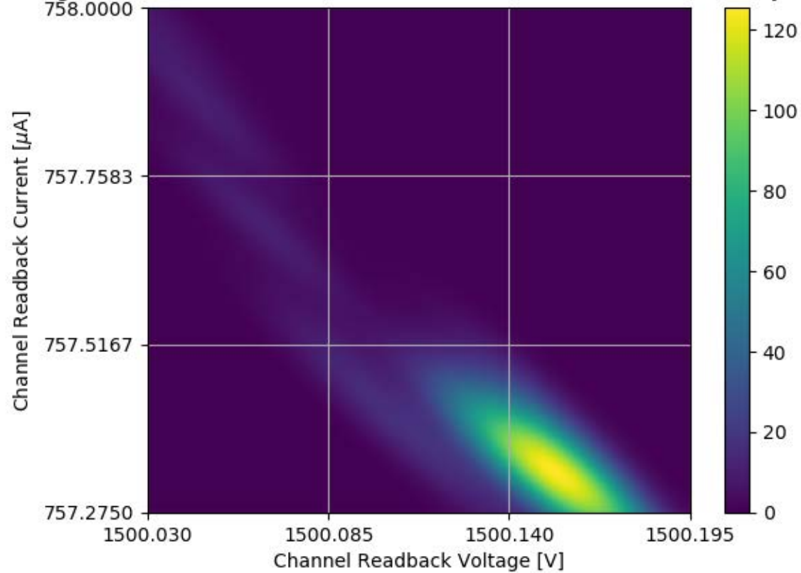
Voltage and Current Readback for Module #354 Channel 29 Stability Test
