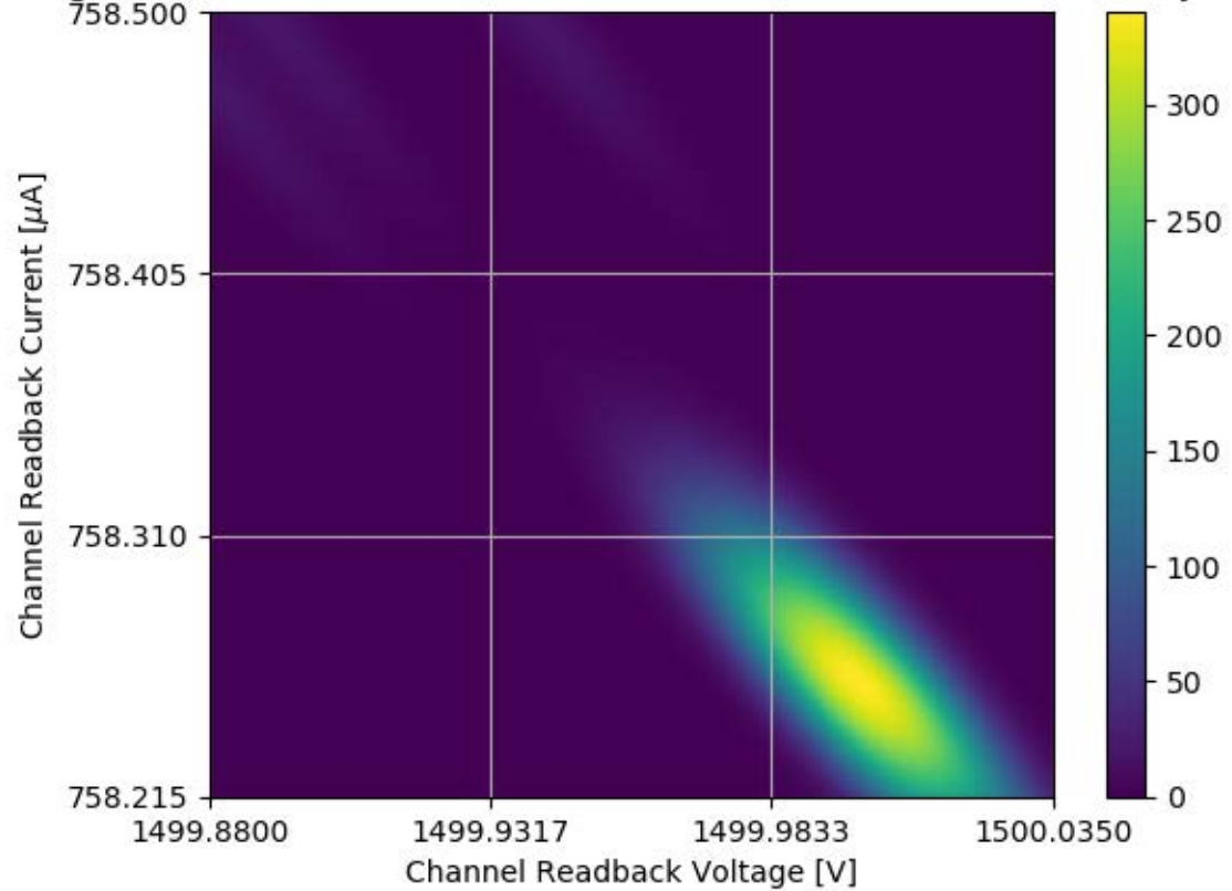
Voltage and Current Readback for Module #354 Channel 26 Stability Test
