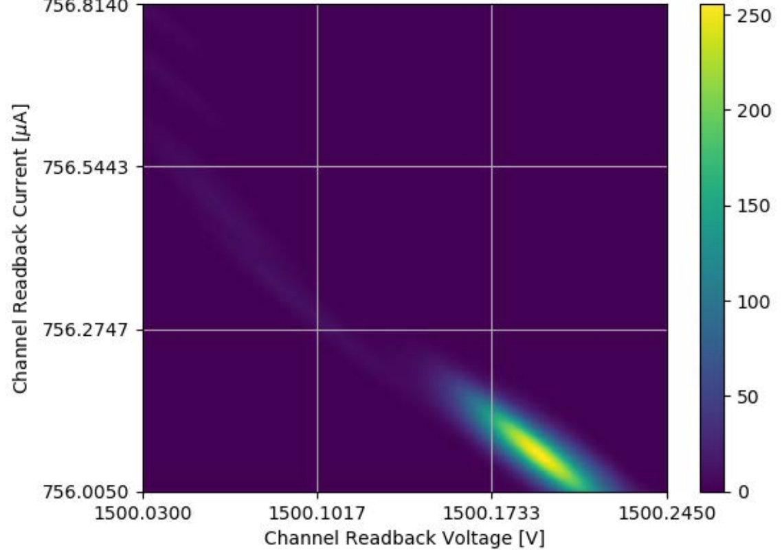
Voltage and Current Readback for Module #354 Channel 03 Stability Test
