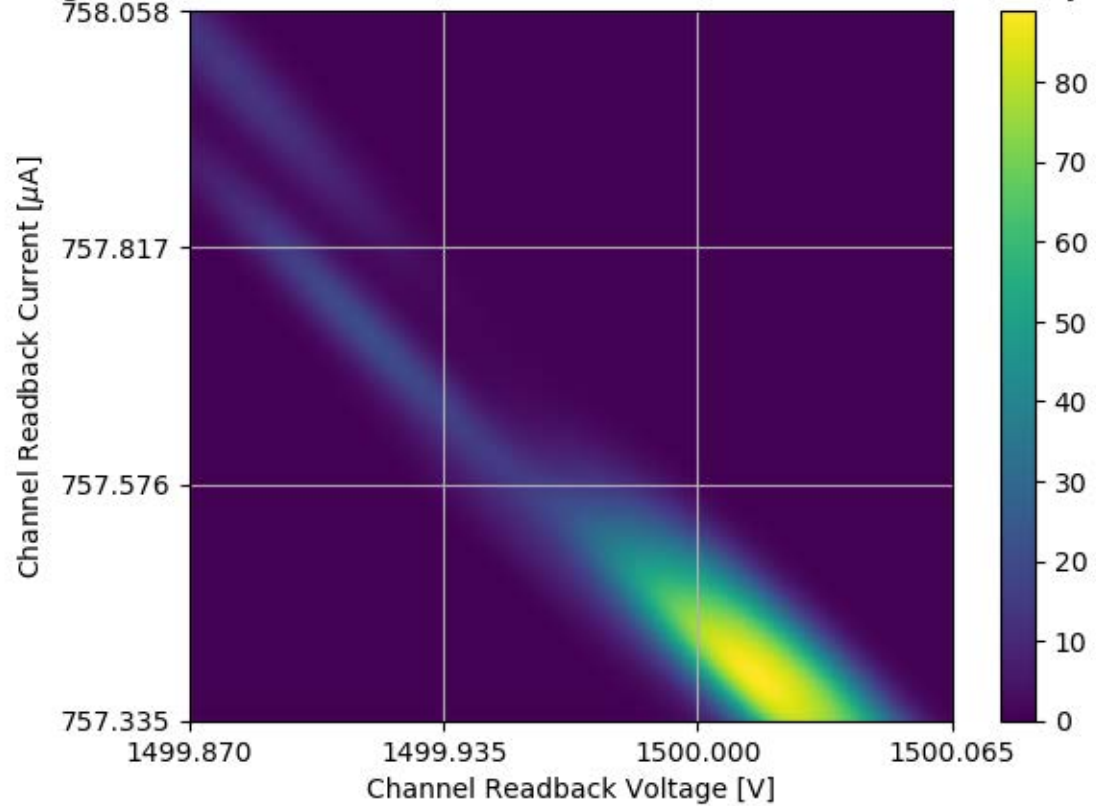
Voltage and Current Readback for Module #354 Channel 19 Stability Test
