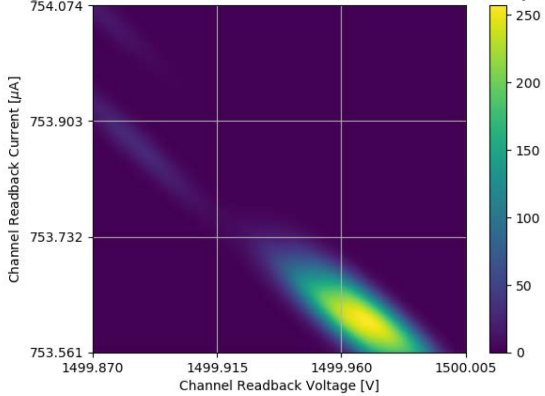
Voltage and Current Readback for Module #354 Channel 11 Stability Test
