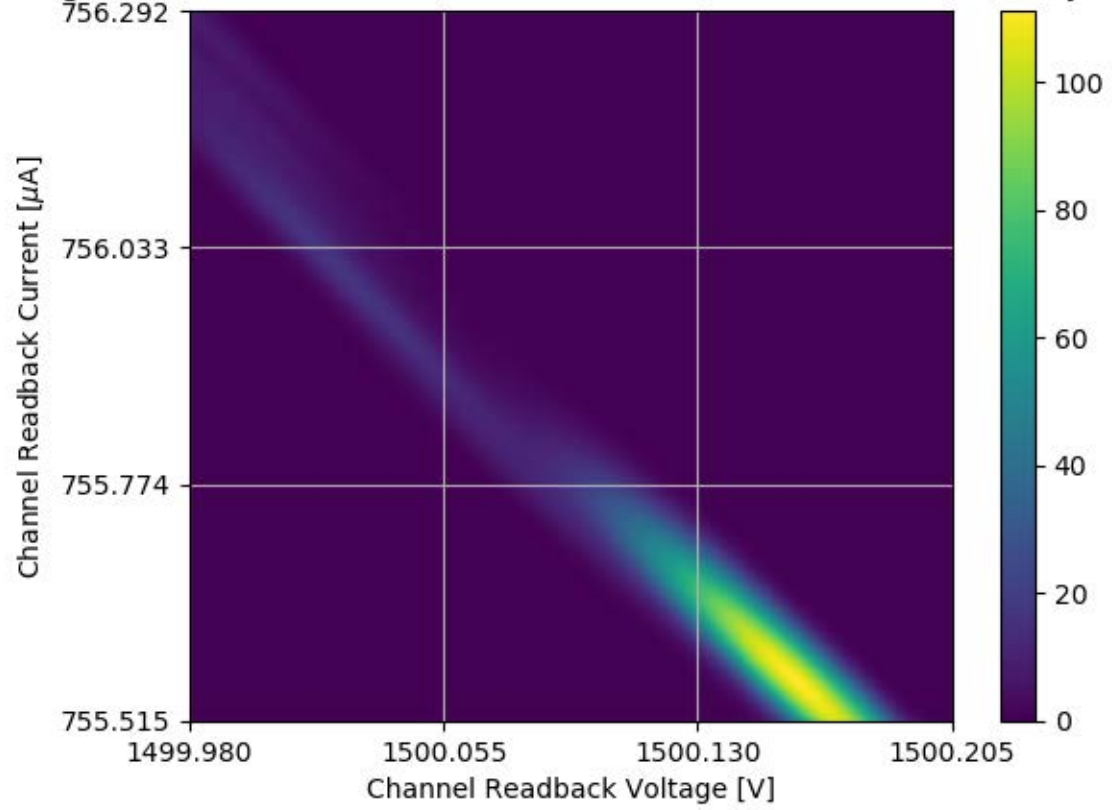
Voltage and Current Readback for Module #354 Channel 01 Stability Test
