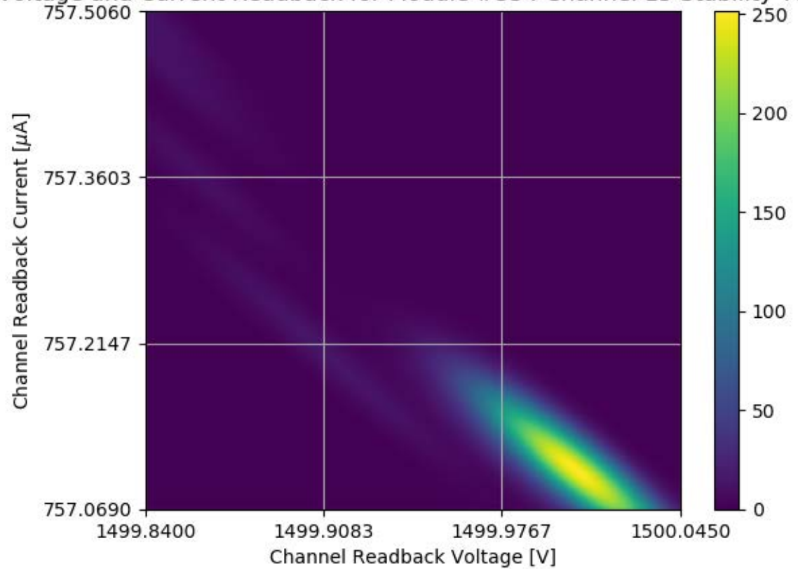
Voltage and Current Readback for Module #354 Channel 15 Stability Test
