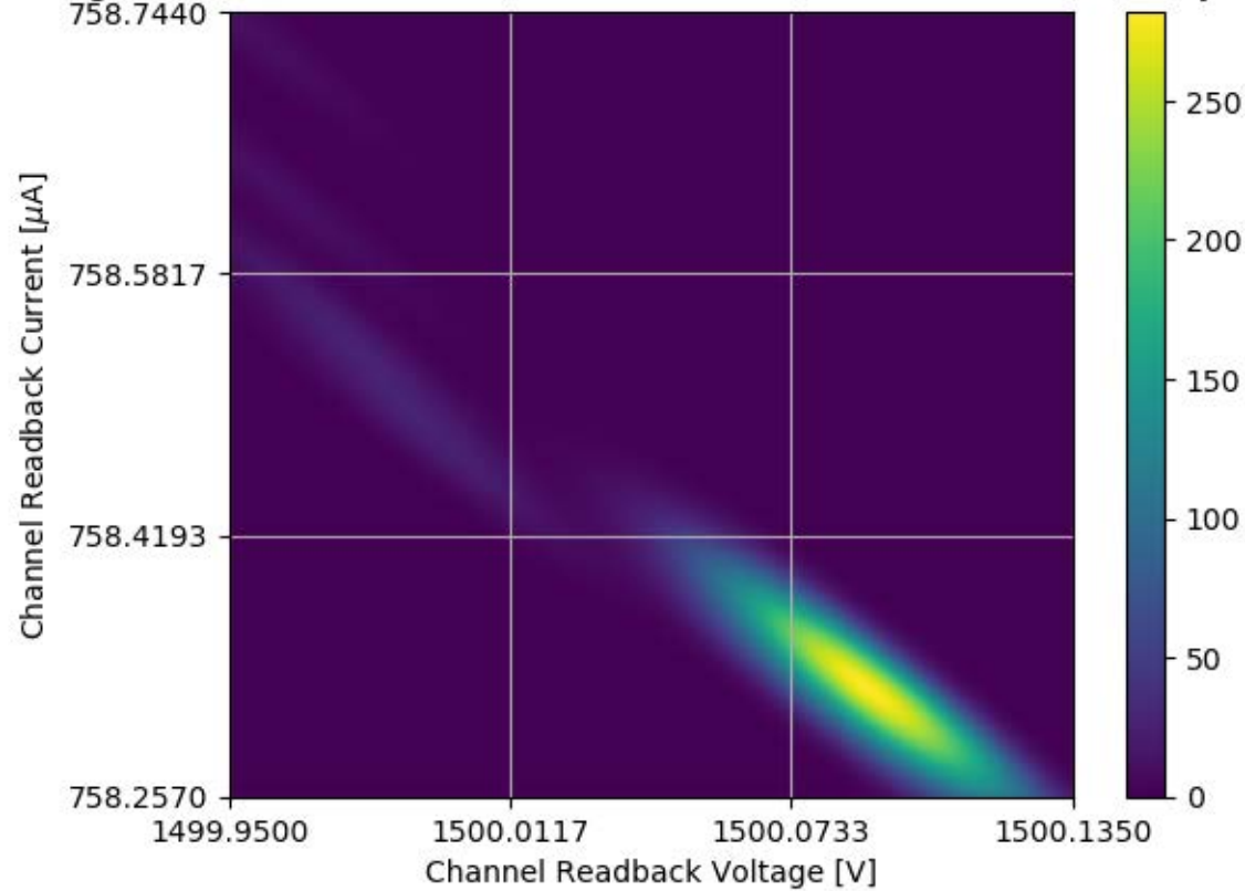
Voltage and Current Readback for Module #354 Channel 35 Stability Test
