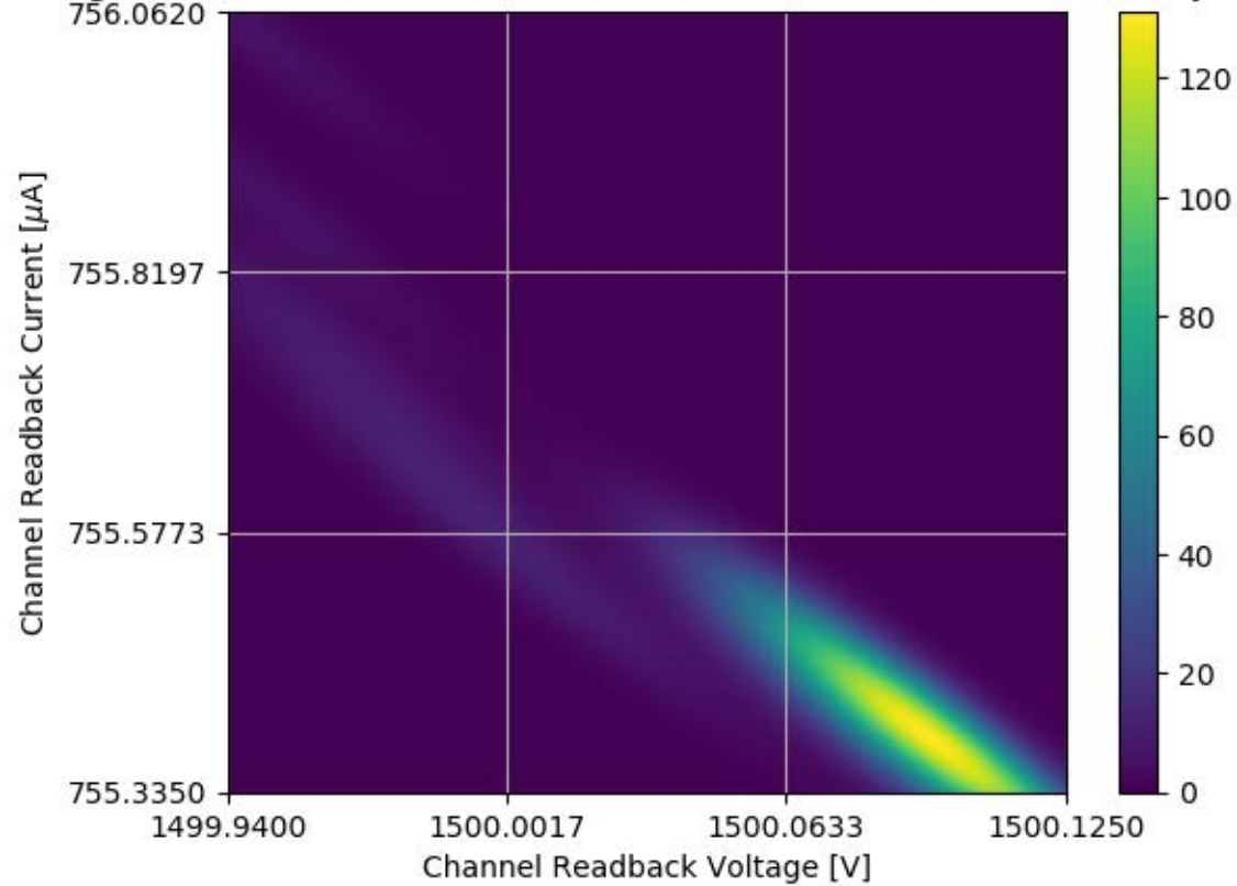
Voltage and Current Readback for Module #354 Channel 00 Stability Test
