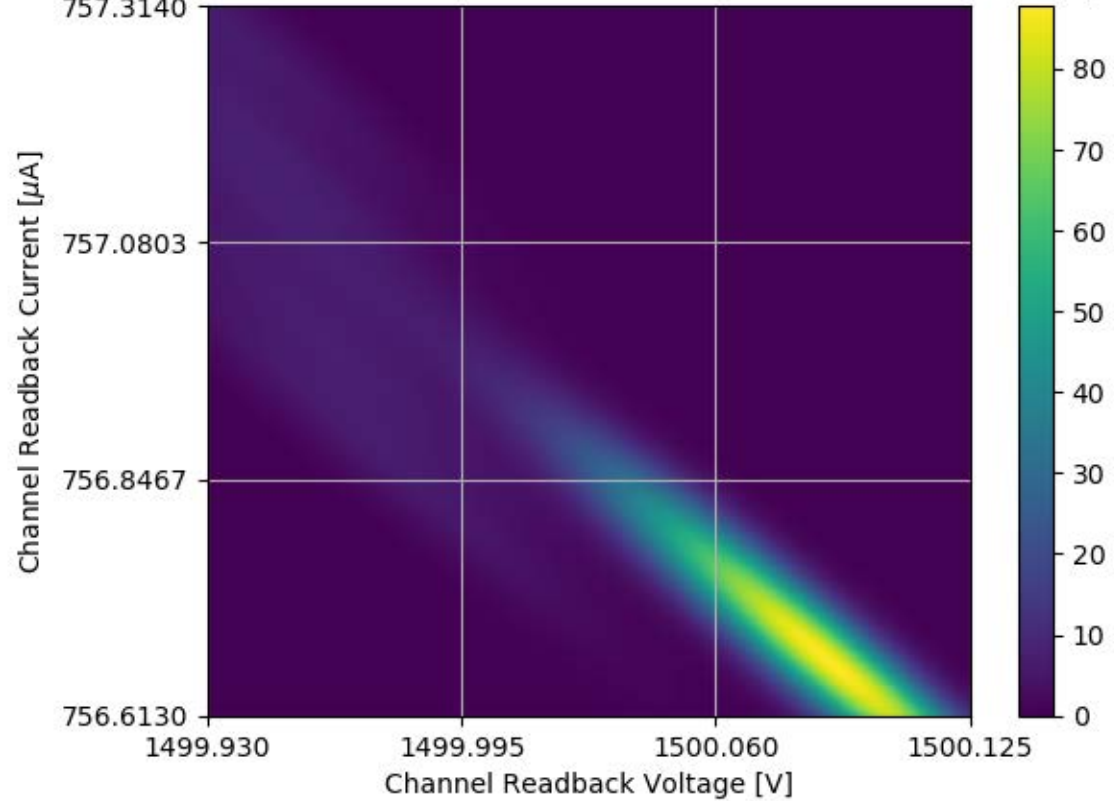
Voltage and Current Readback for Module #354 Channel 02 Stability Test
