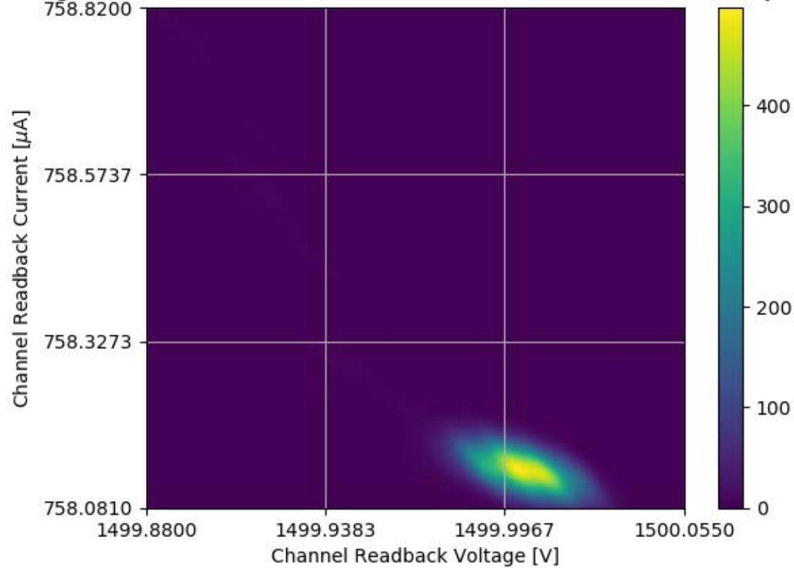
Voltage and Current Readback for Module #354 Channel 20 Stability Test
