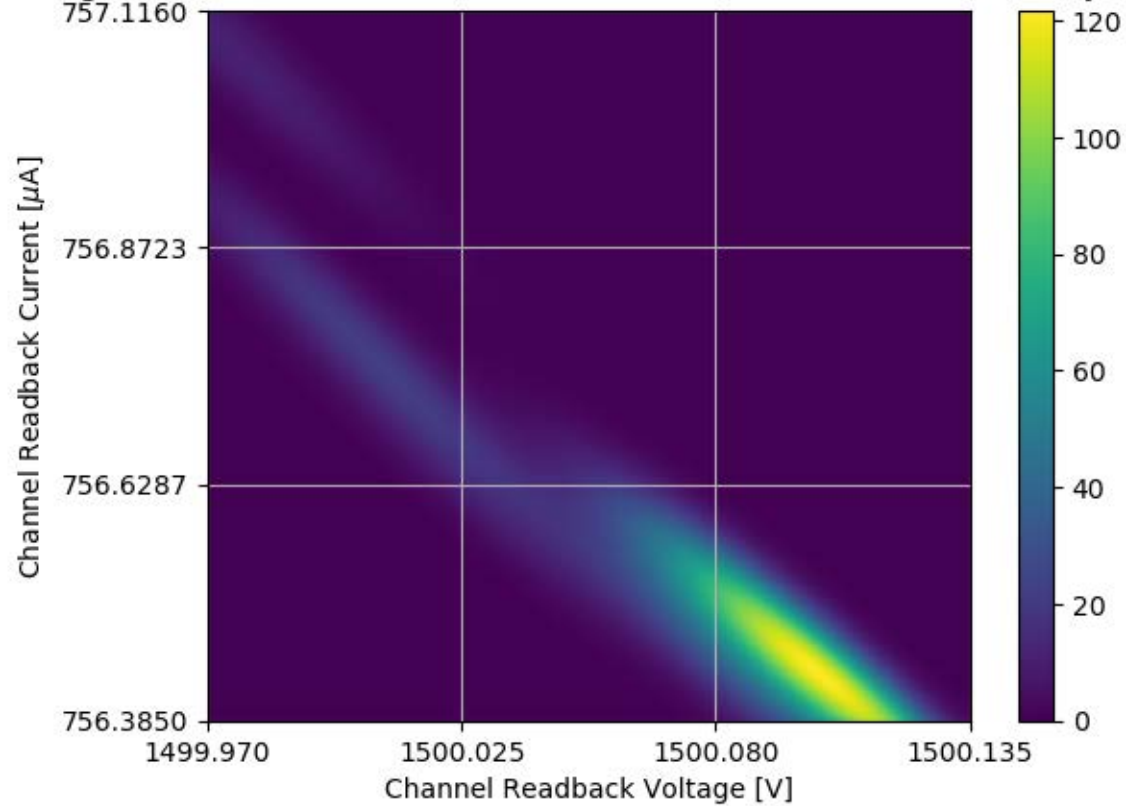
Voltage and Current Readback for Module #354 Channel 17 Stability Test
