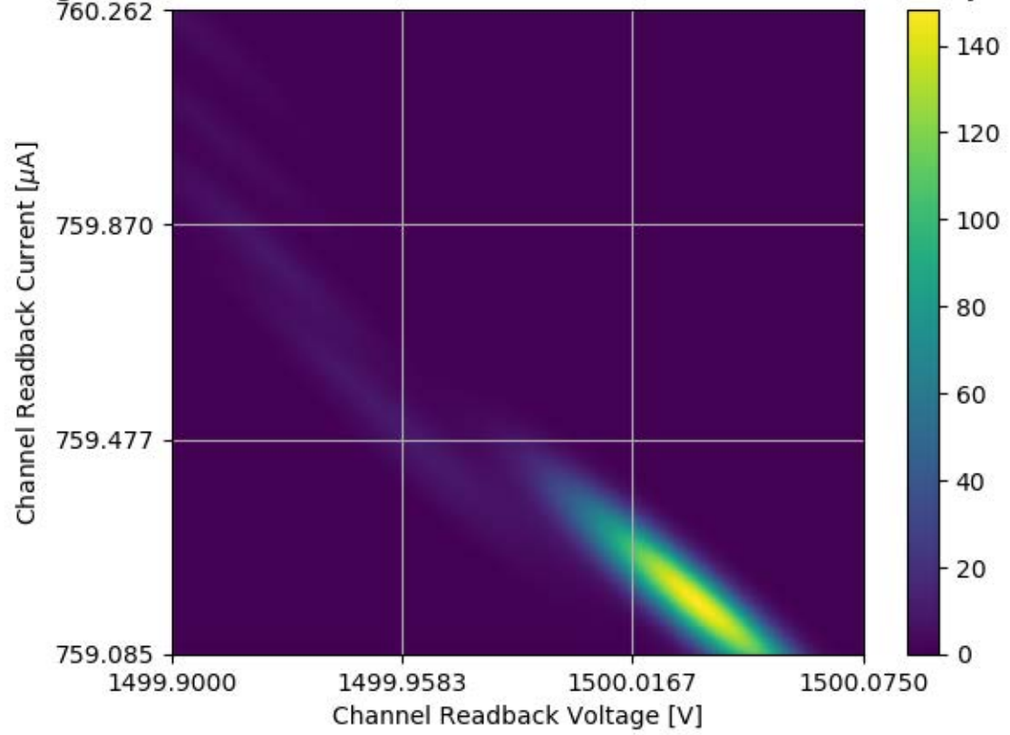
Voltage and Current Readback for Module #354 Channel 22 Stability Test
