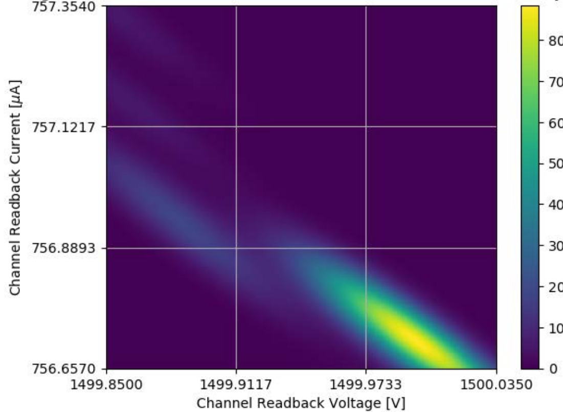
Voltage and Current Readback for Module #354 Channel 18 Stability Test
