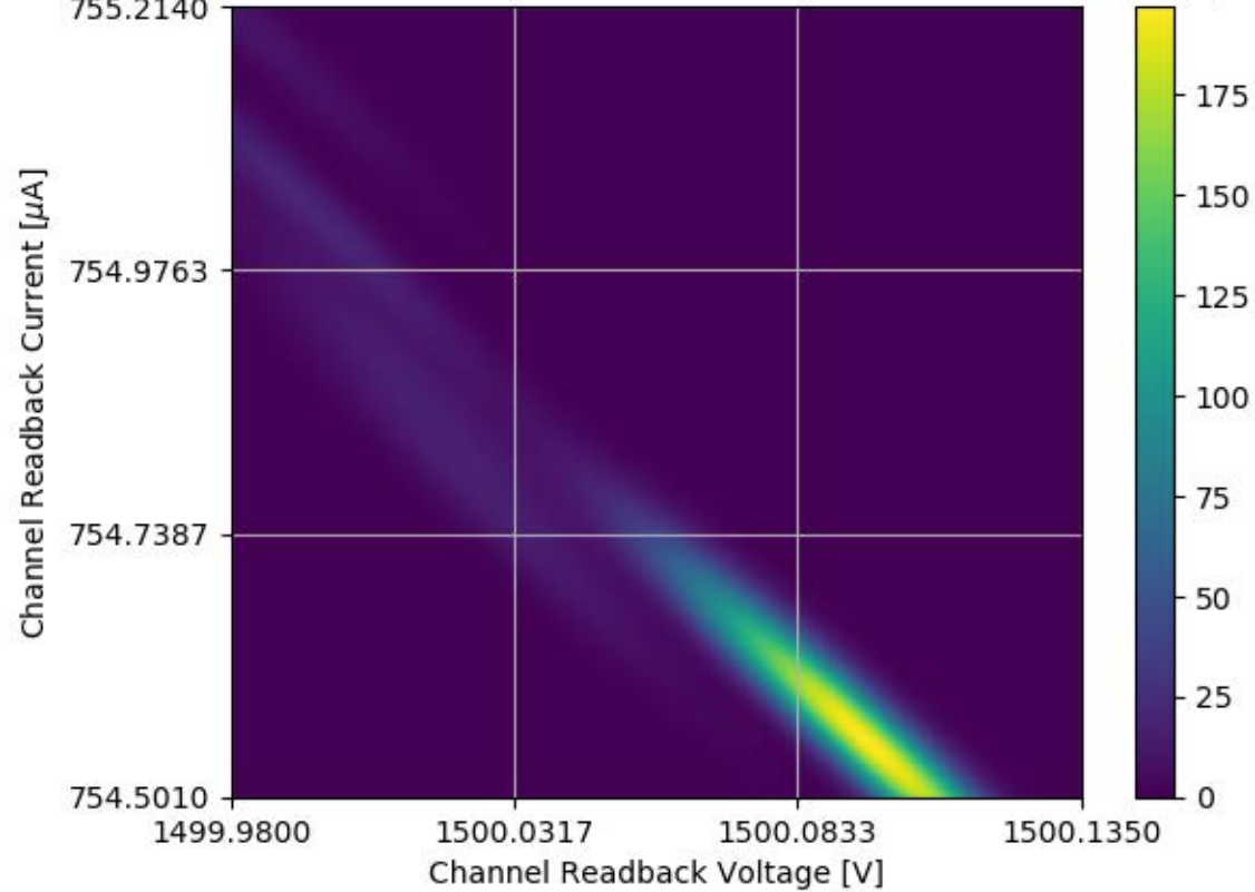
Voltage and Current Readback for Module #354 Channel 33 Stability Test
