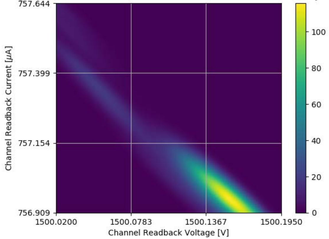
Voltage and Current Readback for Module #354 Channel 31 Stability Test
