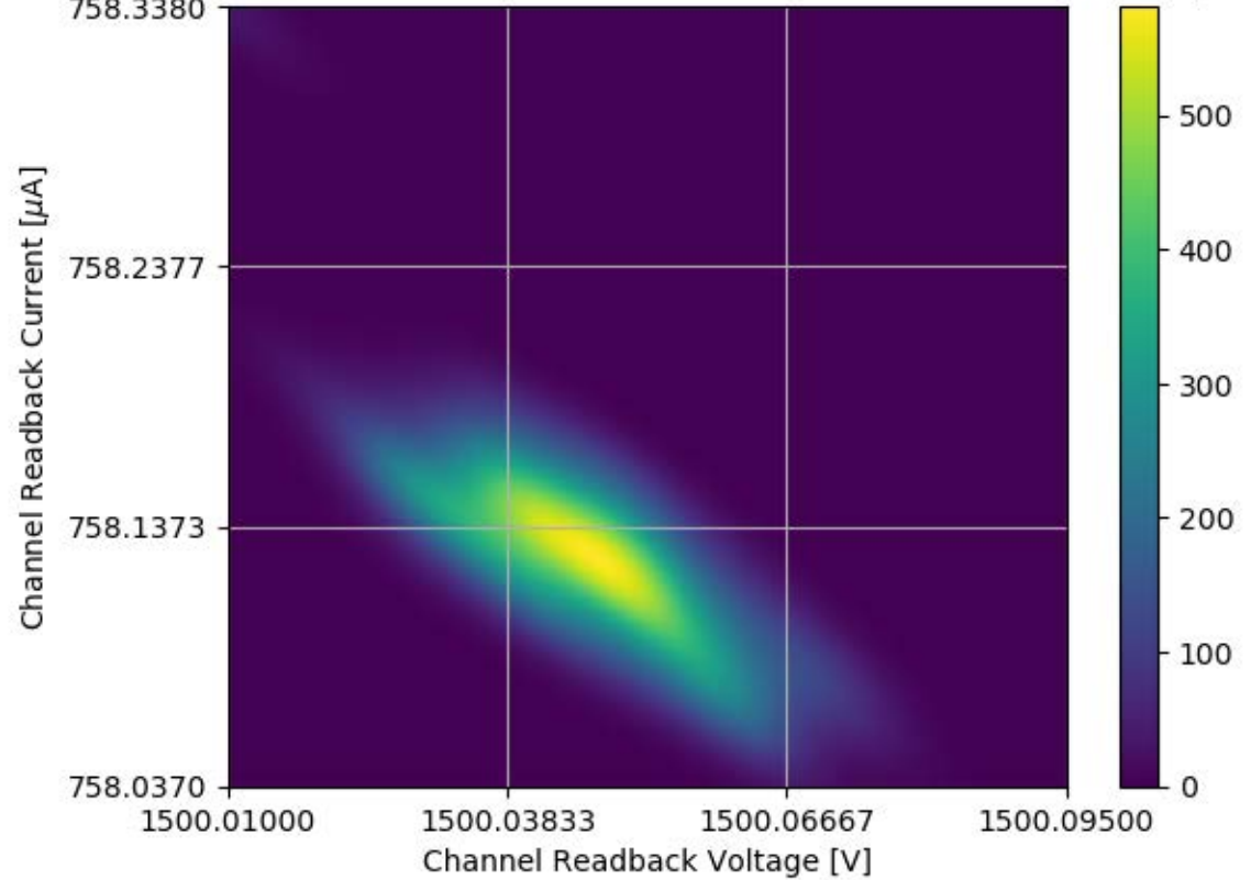
Voltage and Current Readback for Module #355 Channel 16 Stability Test
