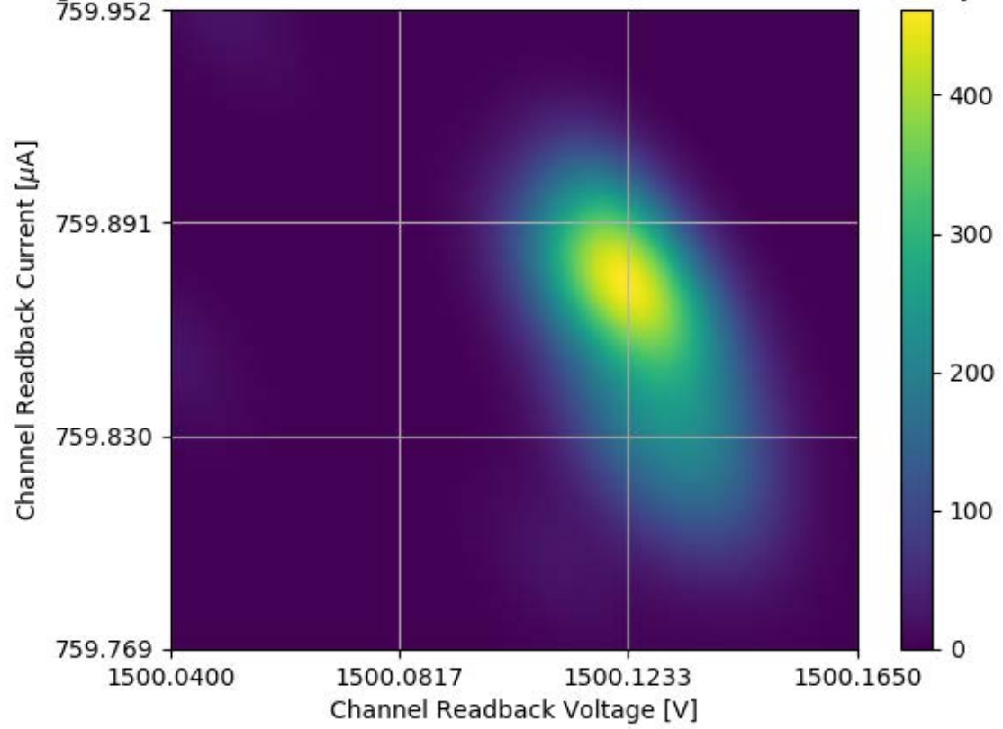
Voltage and Current Readback for Module #355 Channel 10 Stability Test
