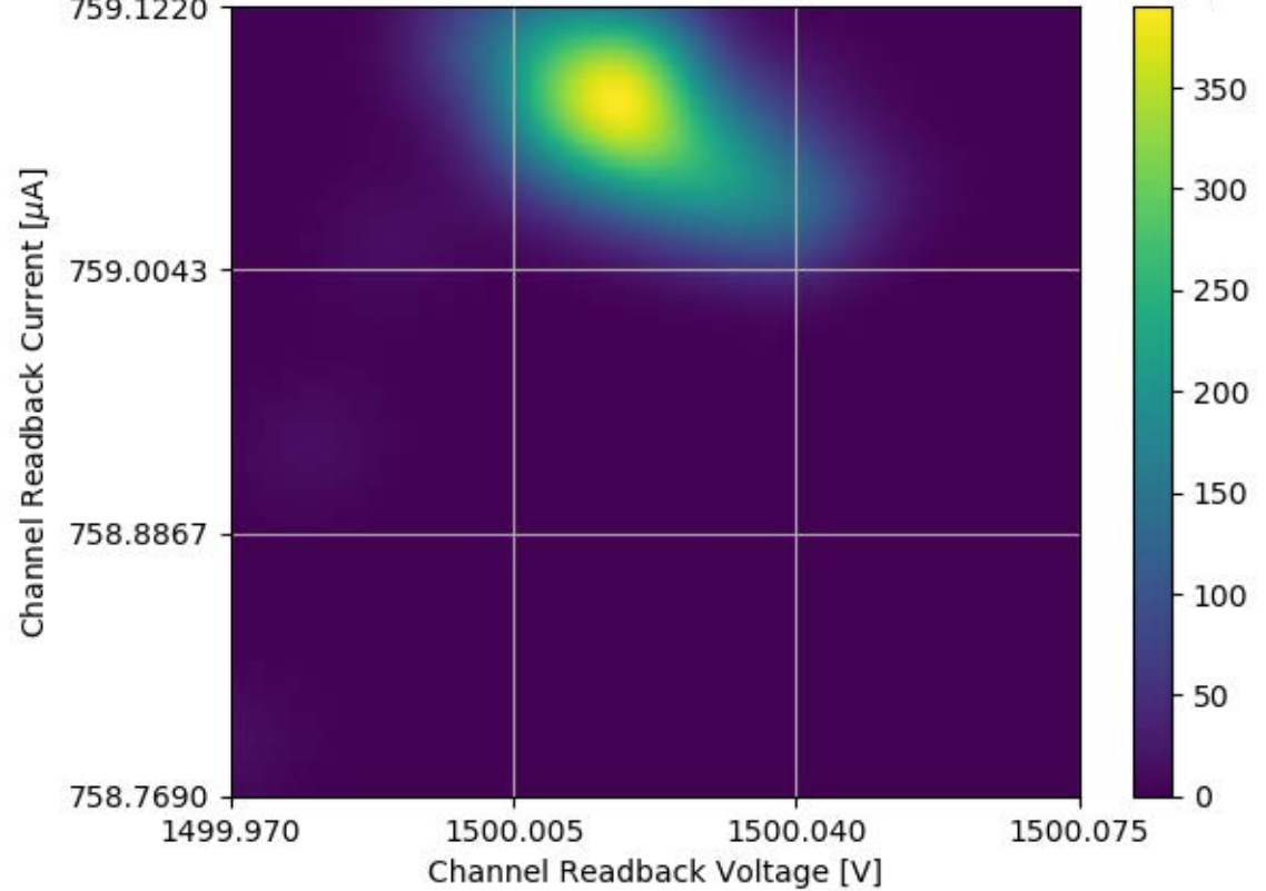
Voltage and Current Readback for Module #355 Channel 26 Stability Test
