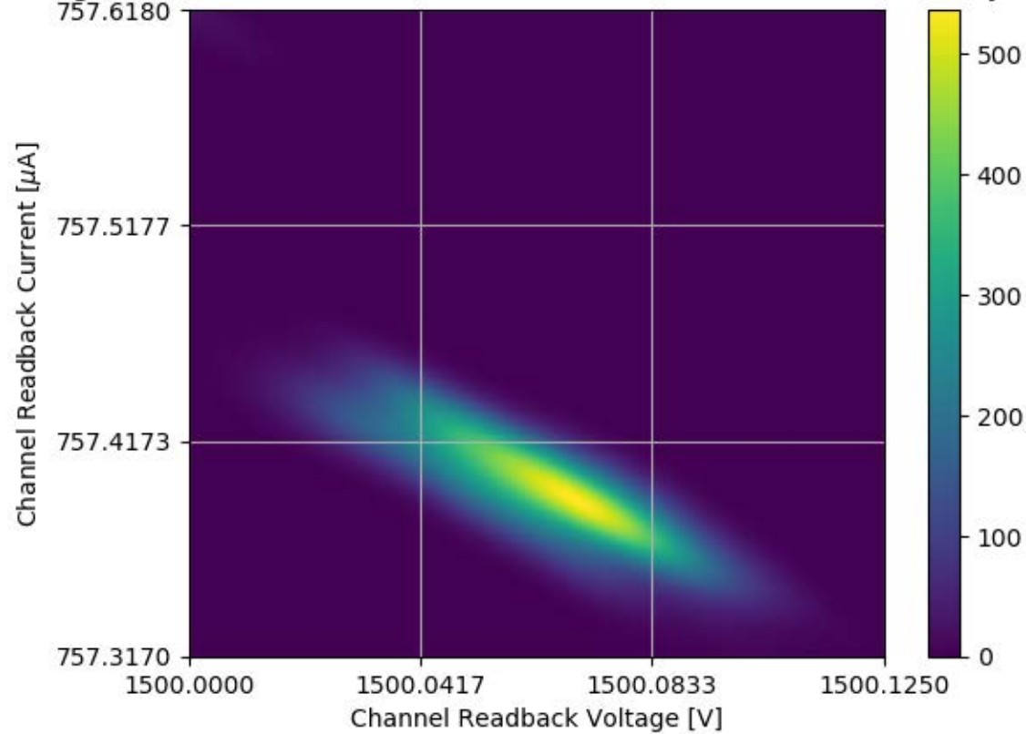
Voltage and Current Readback for Module #355 Channel 07 Stability Test
