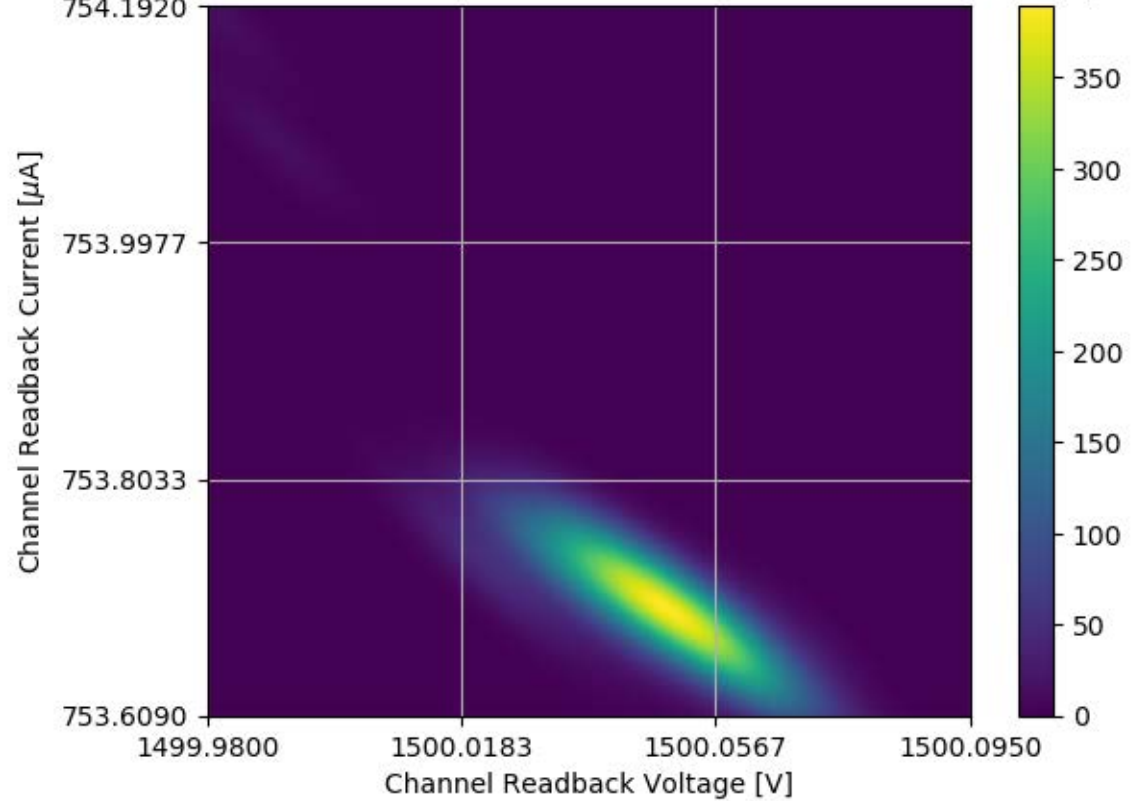
Voltage and Current Readback for Module #355 Channel 11 Stability Test
