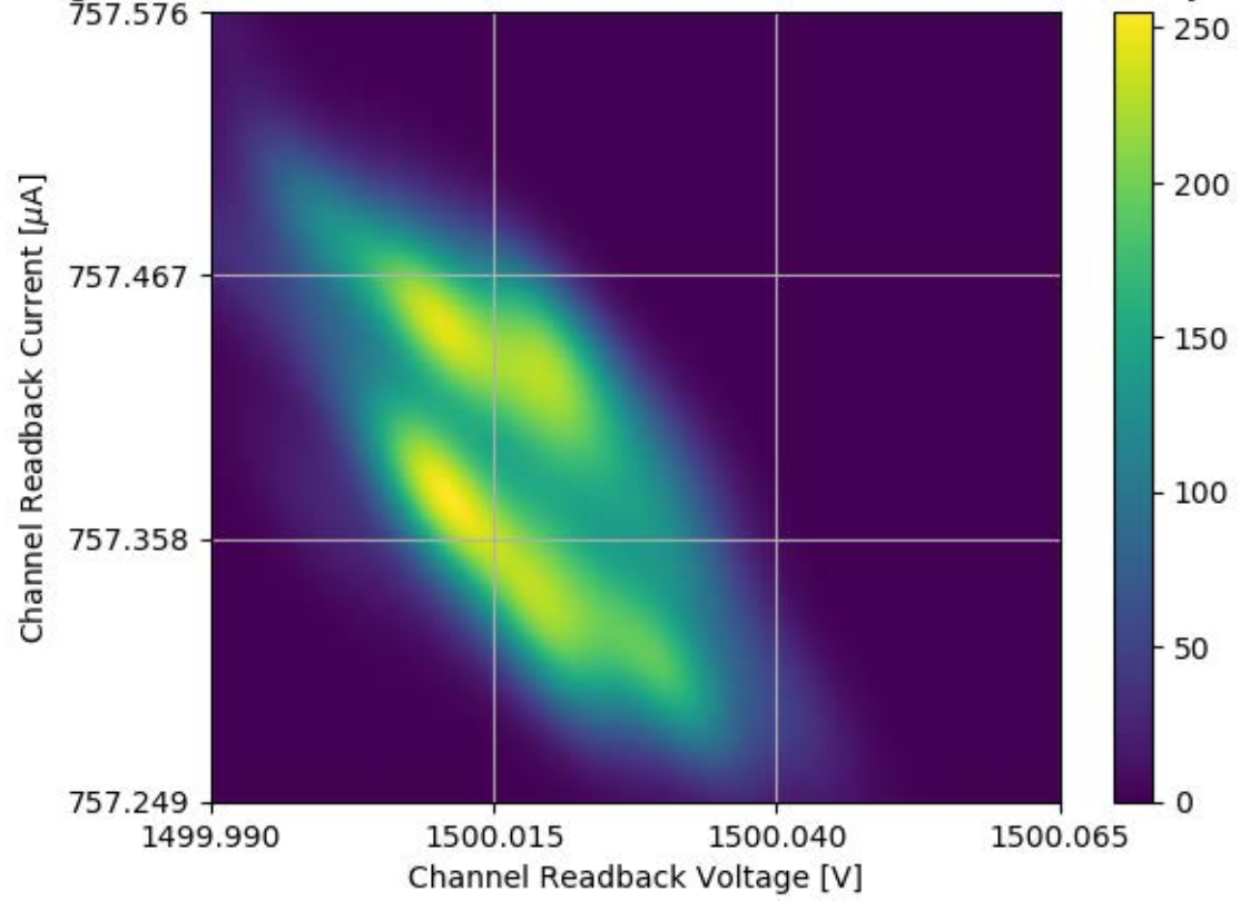
Voltage and Current Readback for Module #355 Channel 23 Stability Test
