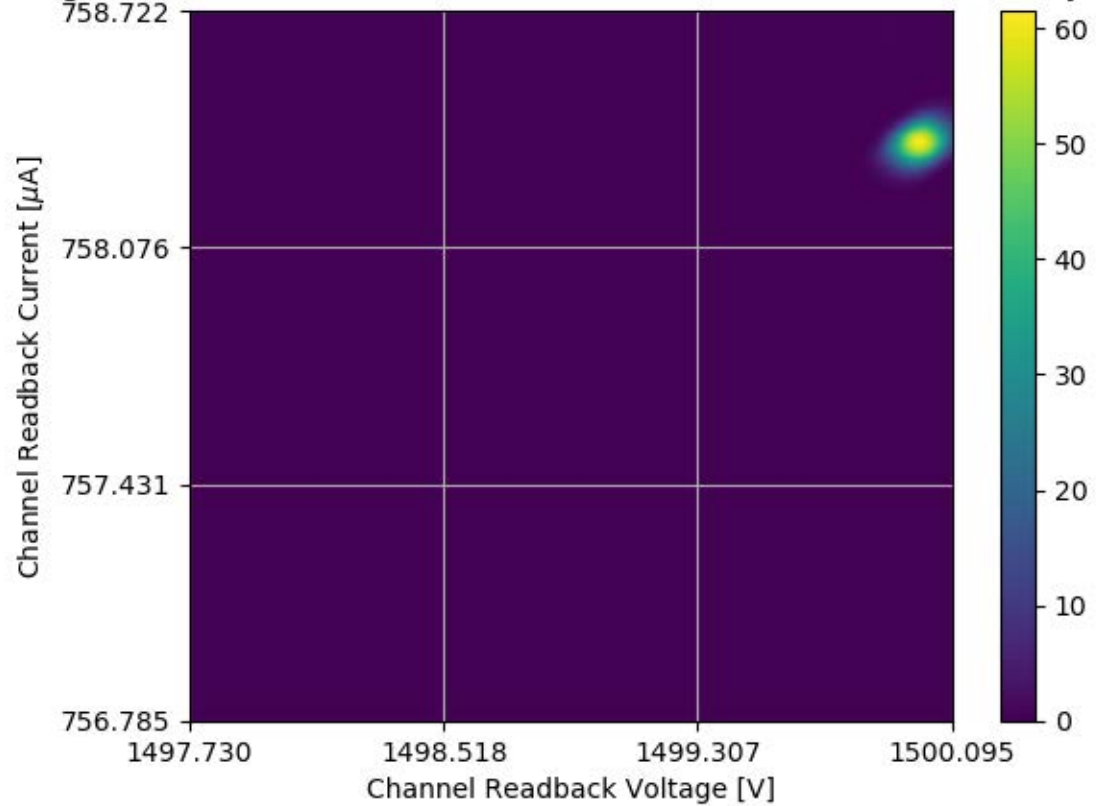
Voltage and Current Readback for Module #355 Channel 35 Stability Test
