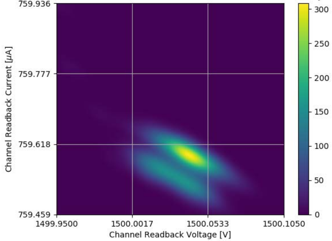
Voltage and Current Readback for Module #355 Channel 12 Stability Test
