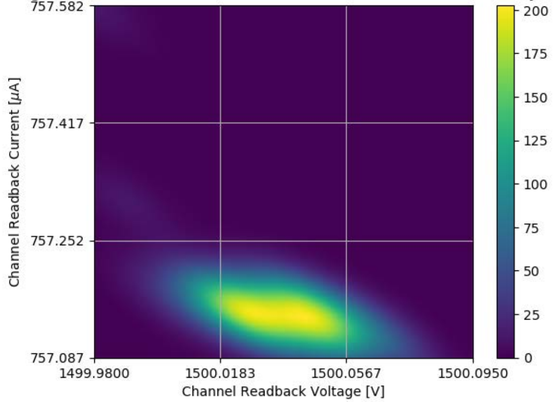
Voltage and Current Readback for Module #355 Channel 15 Stability Test
