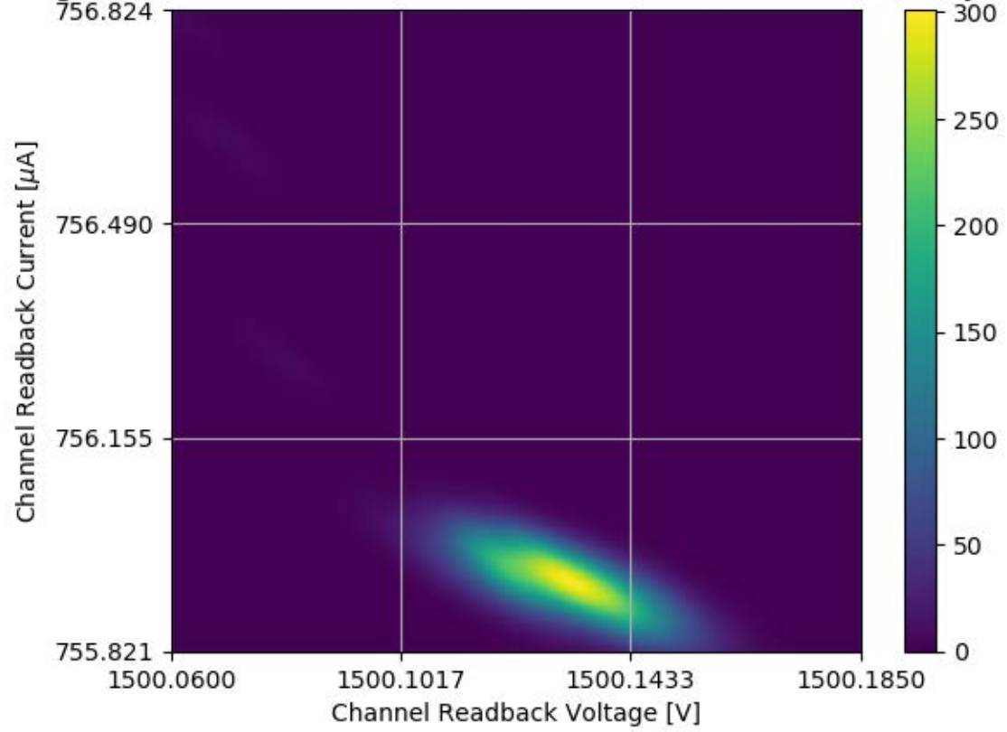
Voltage and Current Readback for Module #355 Channel 03 Stability Test
