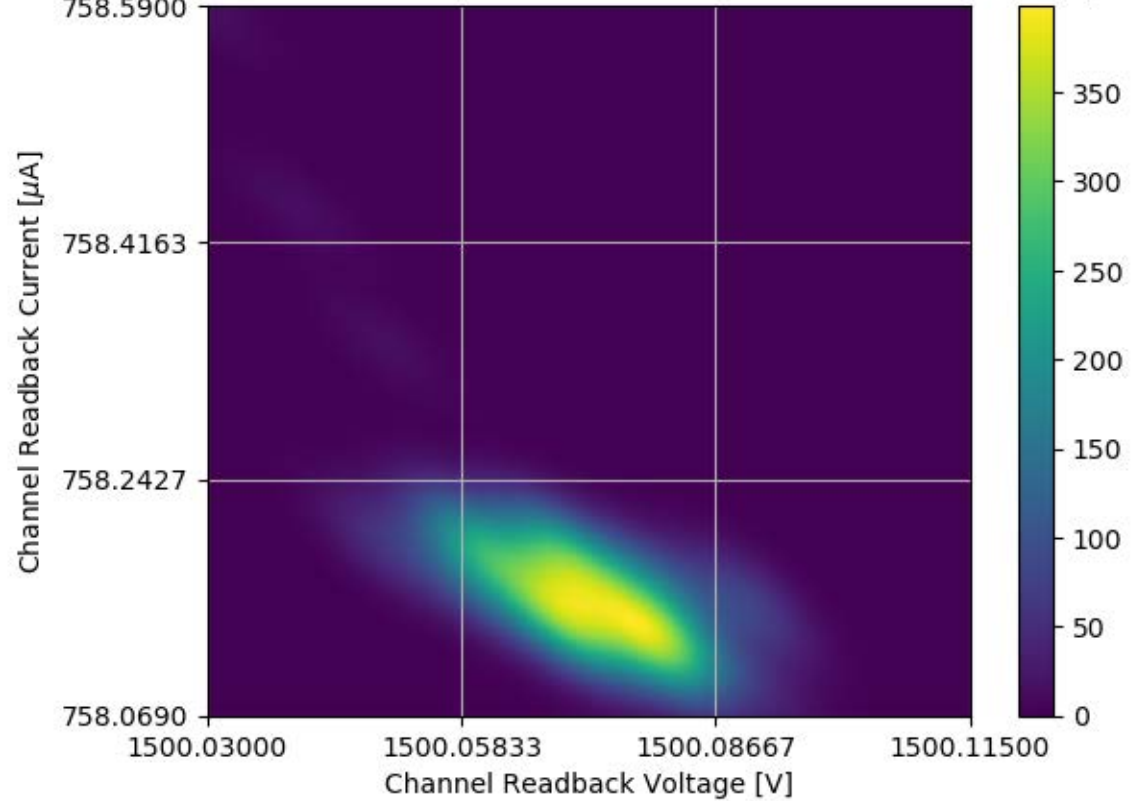
Voltage and Current Readback for Module #355 Channel 21 Stability Test
