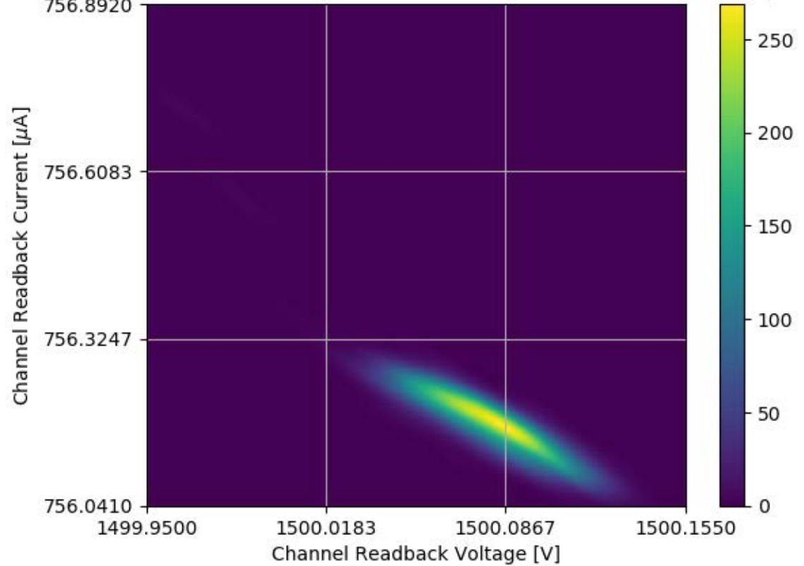
Voltage and Current Readback for Module #355 Channel 14 Stability Test
