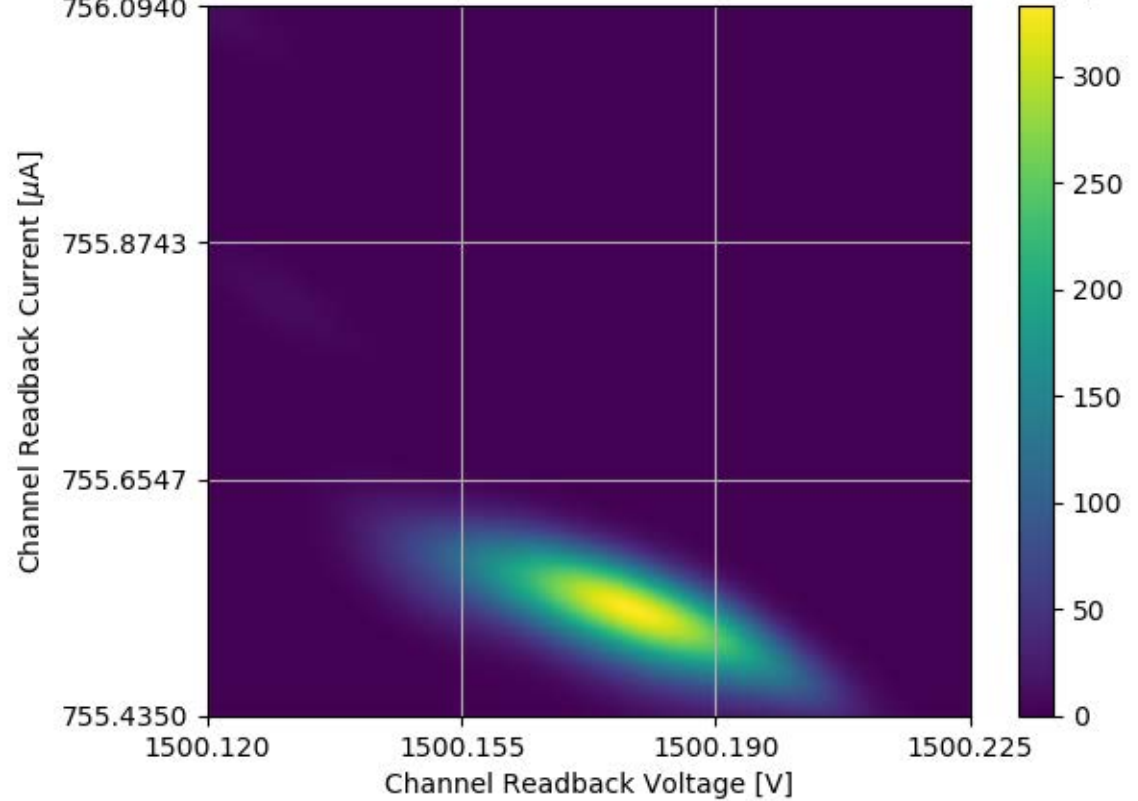
Voltage and Current Readback for Module #355 Channel 00 Stability Test
