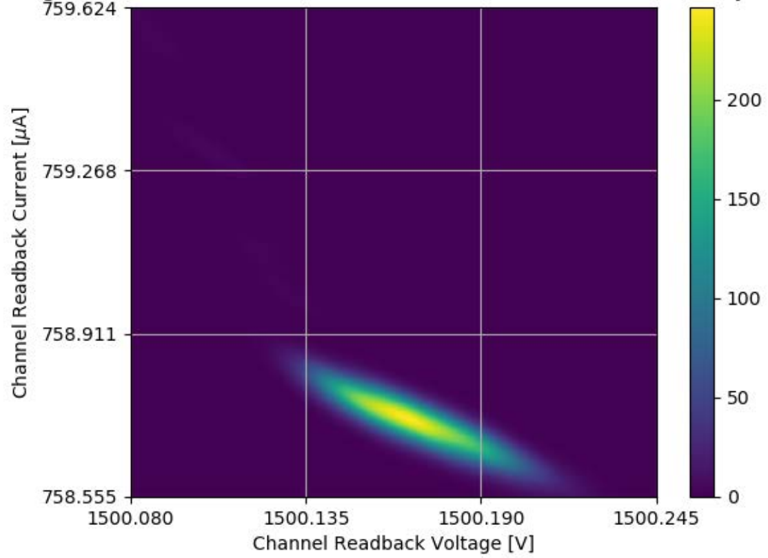
Voltage and Current Readback for Module #355 Channel 22 Stability Test
