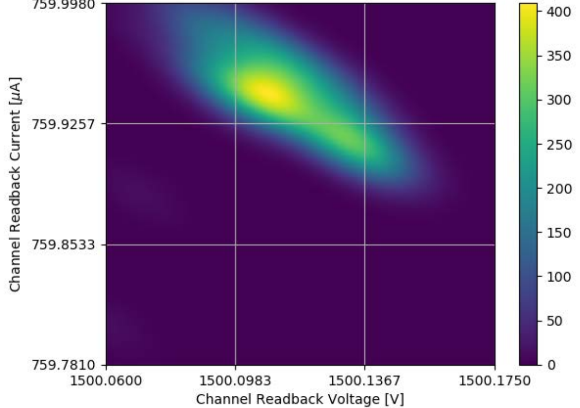
Voltage and Current Readback for Module #355 Channel 24 Stability Test
