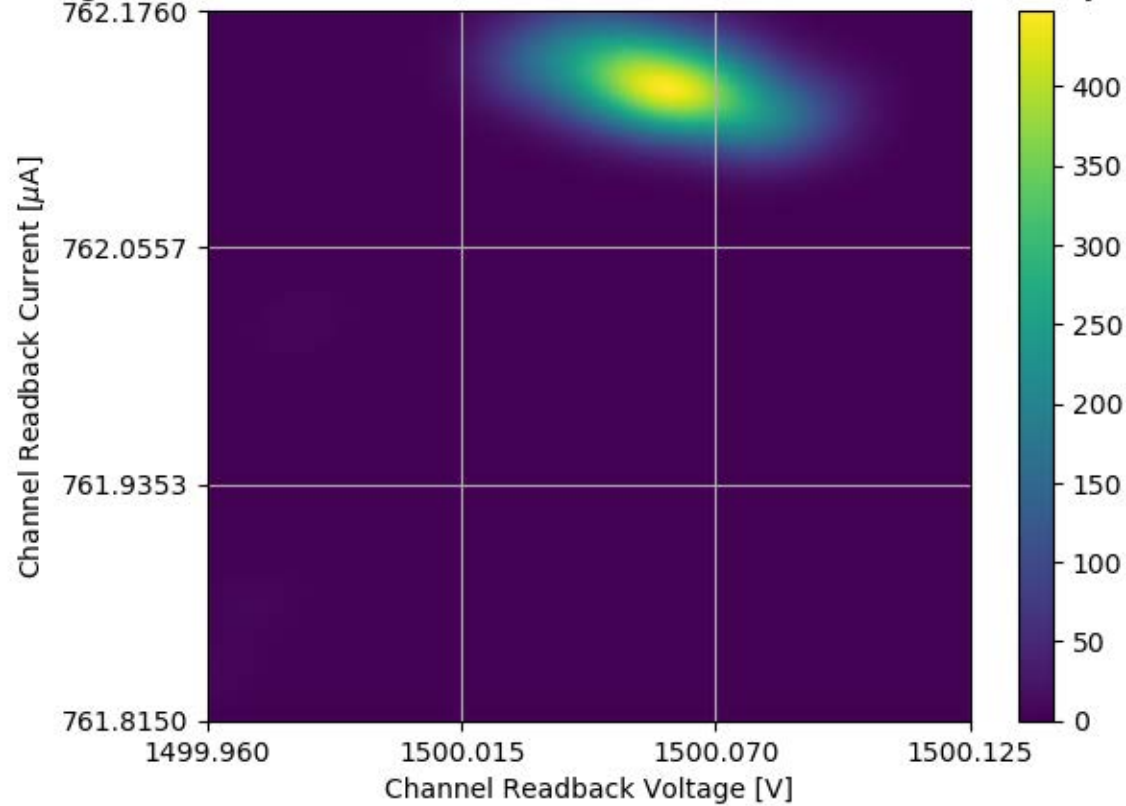
Voltage and Current Readback for Module #355 Channel 09 Stability Test
