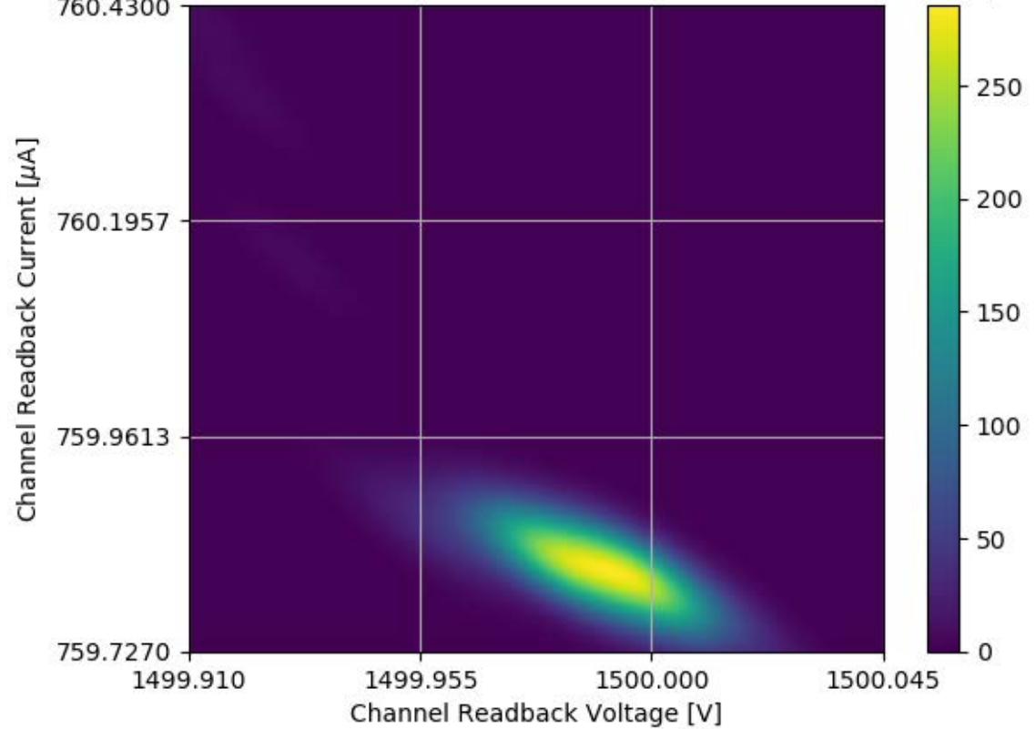
Voltage and Current Readback for Module #355 Channel 05 Stability Test
