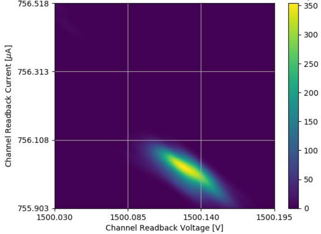
Voltage and Current Readback for Module #355 Channel 01 Stability Test
