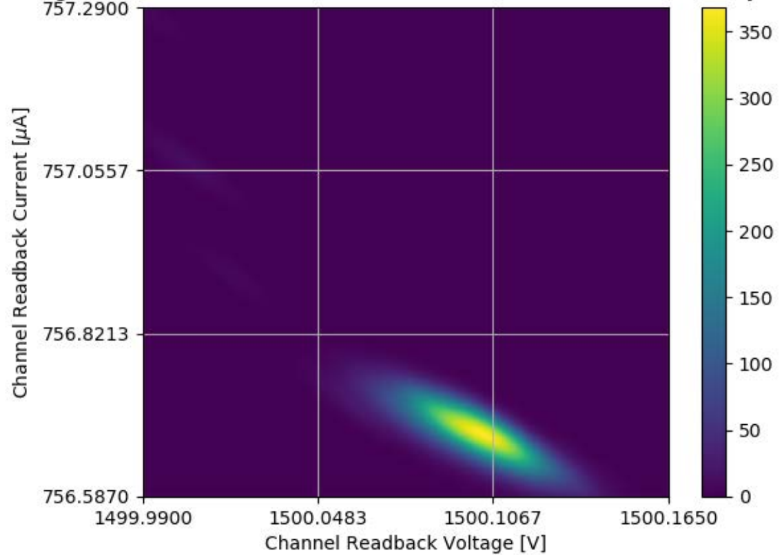
Voltage and Current Readback for Module #355 Channel 02 Stability Test
