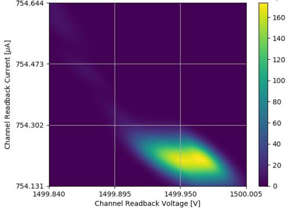
Voltage and Current Readback for Module #356 Channel 11 Stability Test
