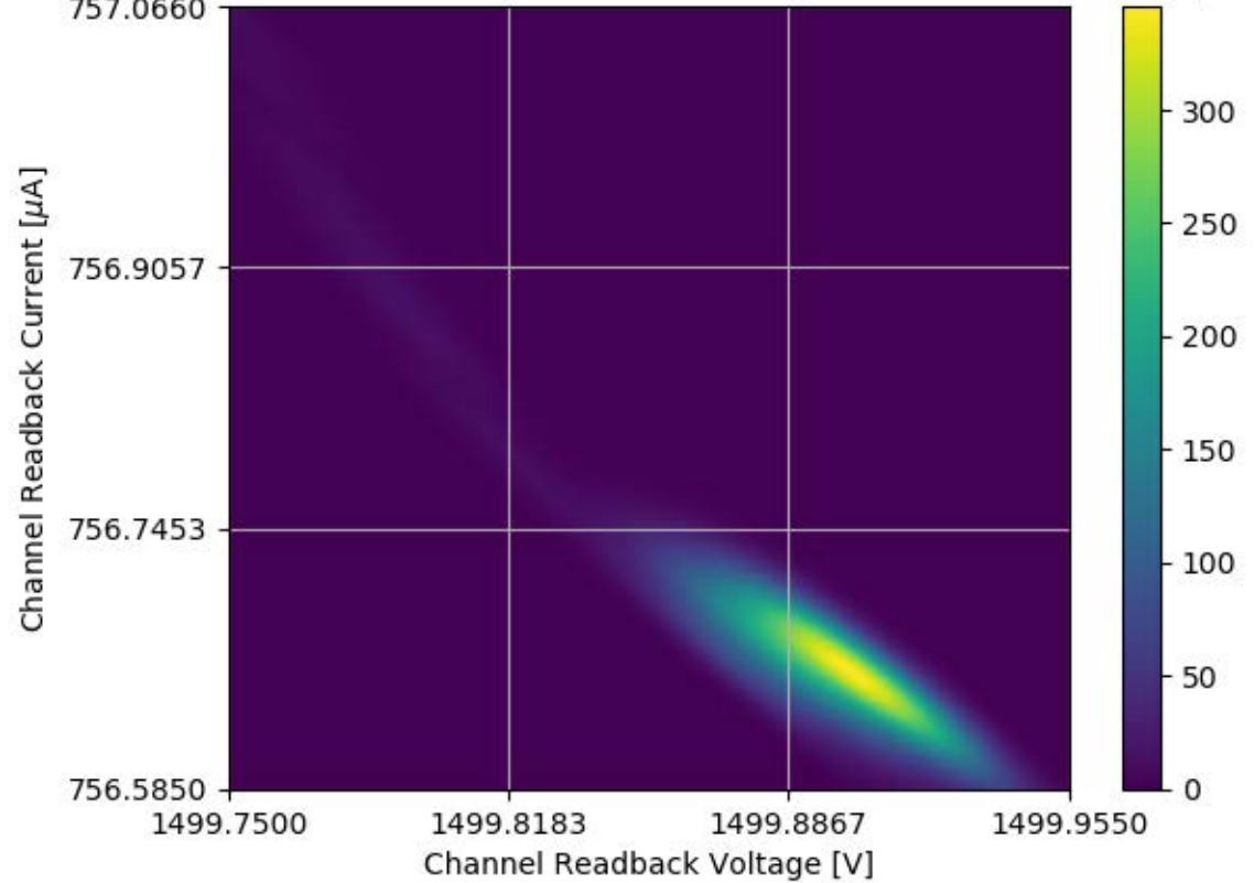
Voltage and Current Readback for Module #356 Channel 02 Stability Test
