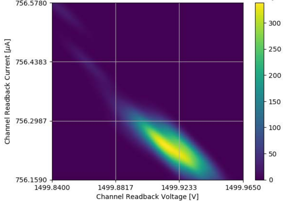
Voltage and Current Readback for Module #356 Channel 17 Stability Test
