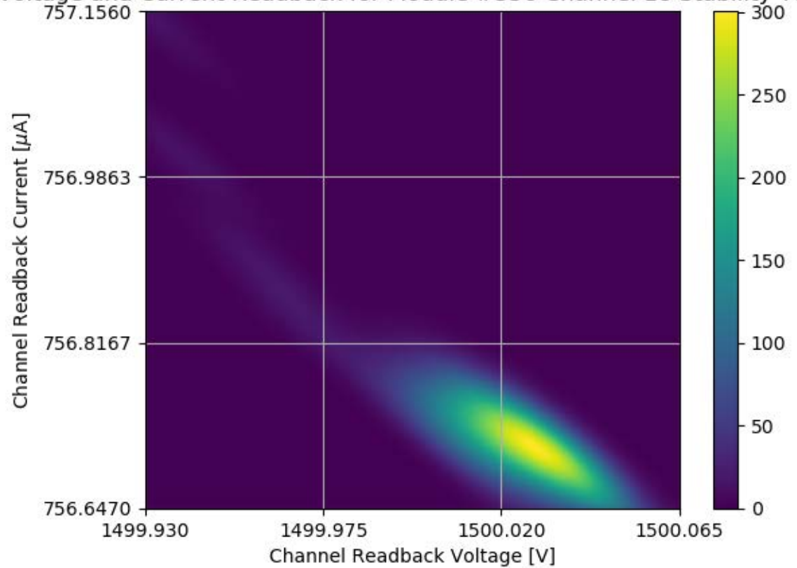
Voltage and Current Readback for Module #356 Channel 18 Stability Test
