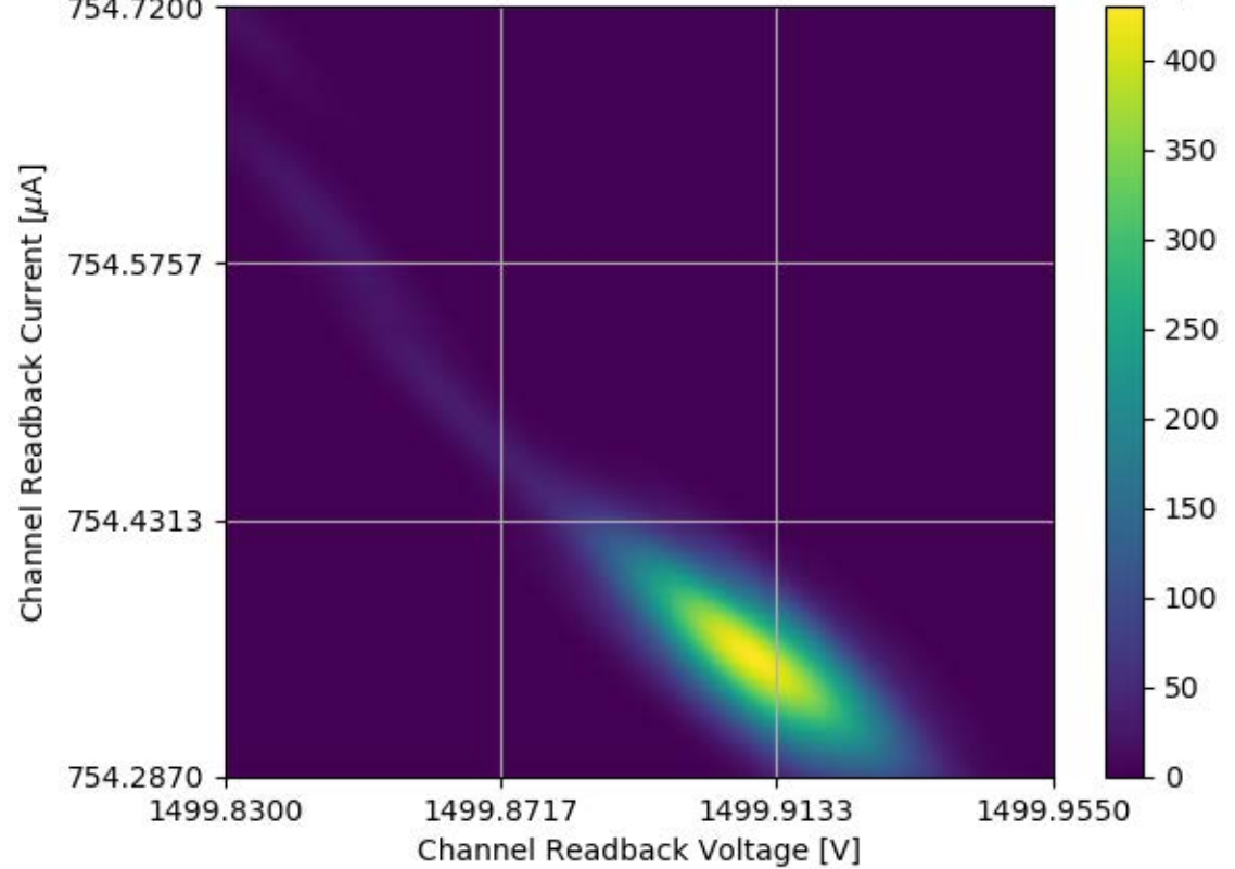
Voltage and Current Readback for Module #356 Channel 33 Stability Test
