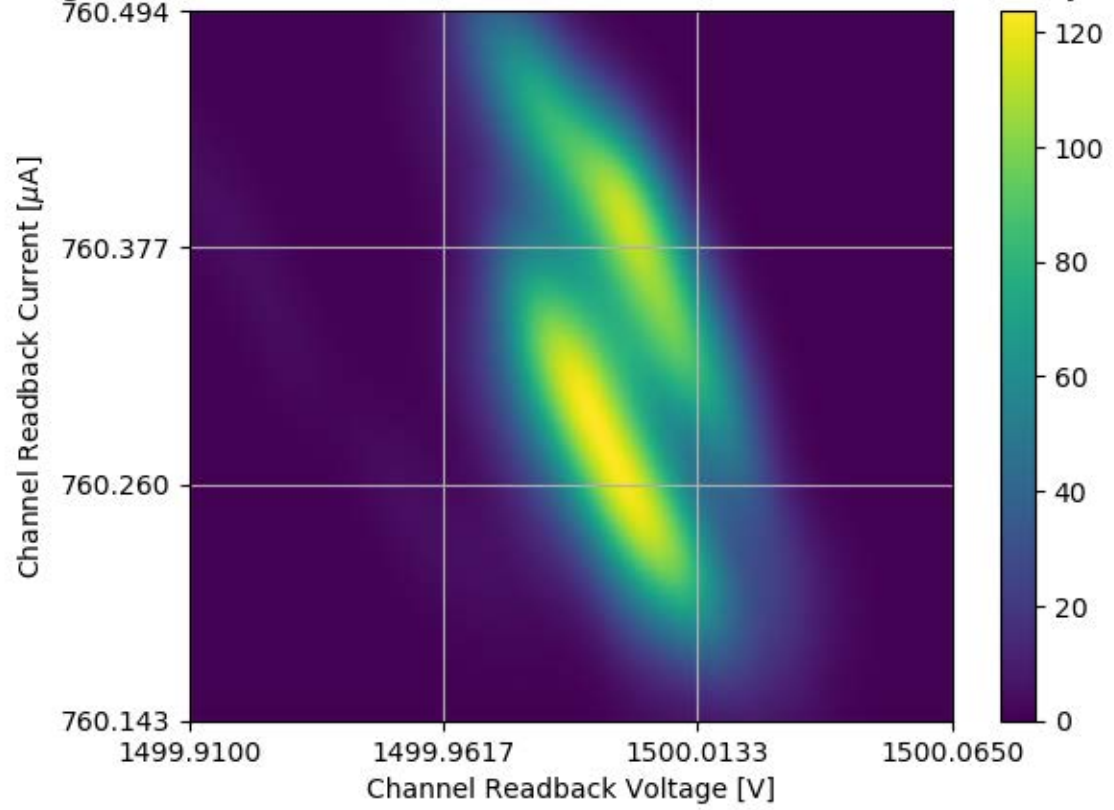
Voltage and Current Readback for Module #356 Channel 25 Stability Test
