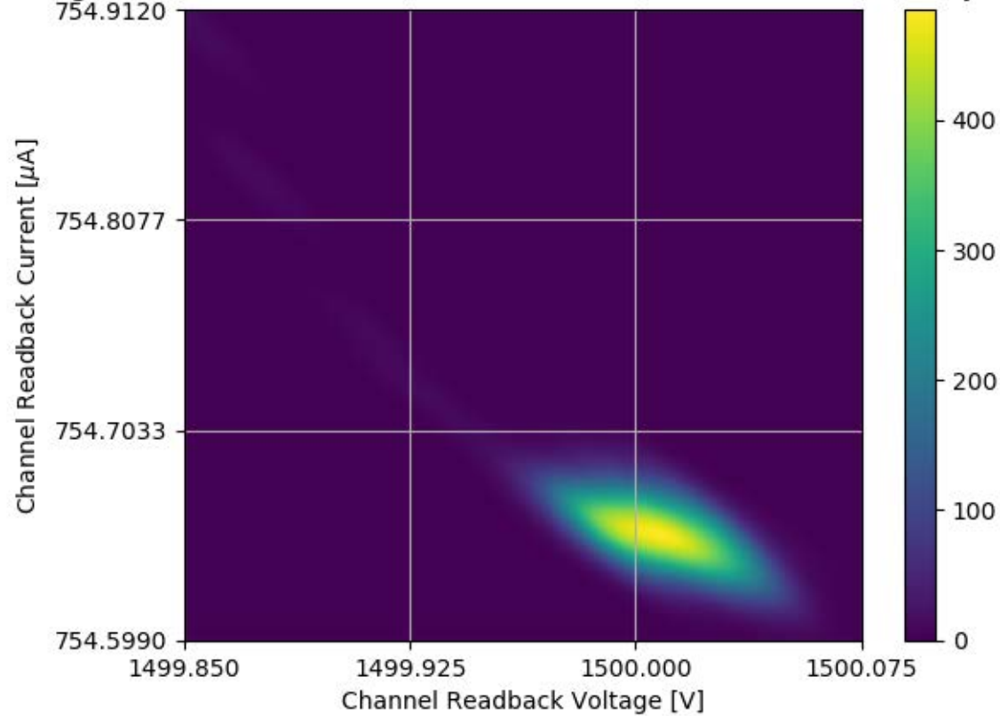
Voltage and Current Readback for Module #356 Channel 00 Stability Test
