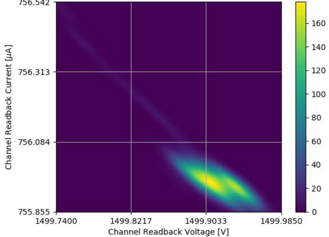
Voltage and Current Readback for Module #356 Channel 01 Stability Test
