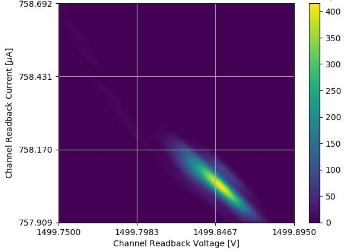
Voltage and Current Readback for Module #356 Channel 16 Stability Test
