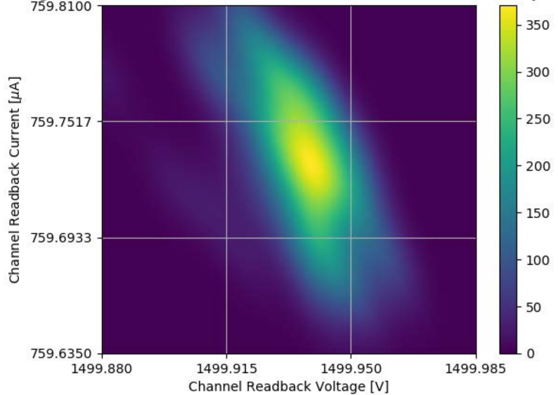
Voltage and Current Readback for Module #356 Channel 24 Stability Test
