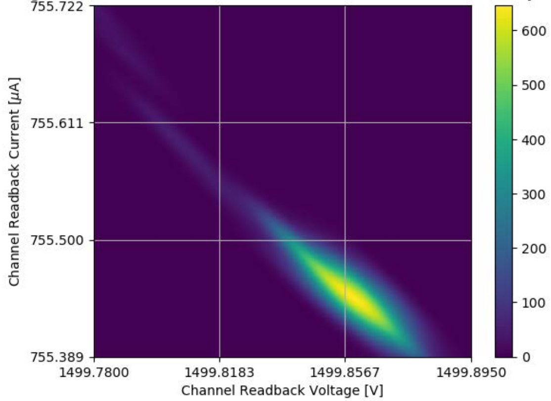
Voltage and Current Readback for Module #356 Channel 28 Stability Test
