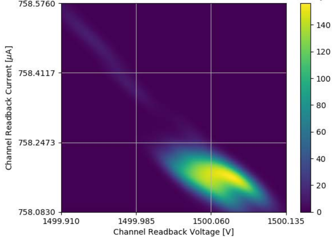
Voltage and Current Readback for Module #356 Channel 21 Stability Test
