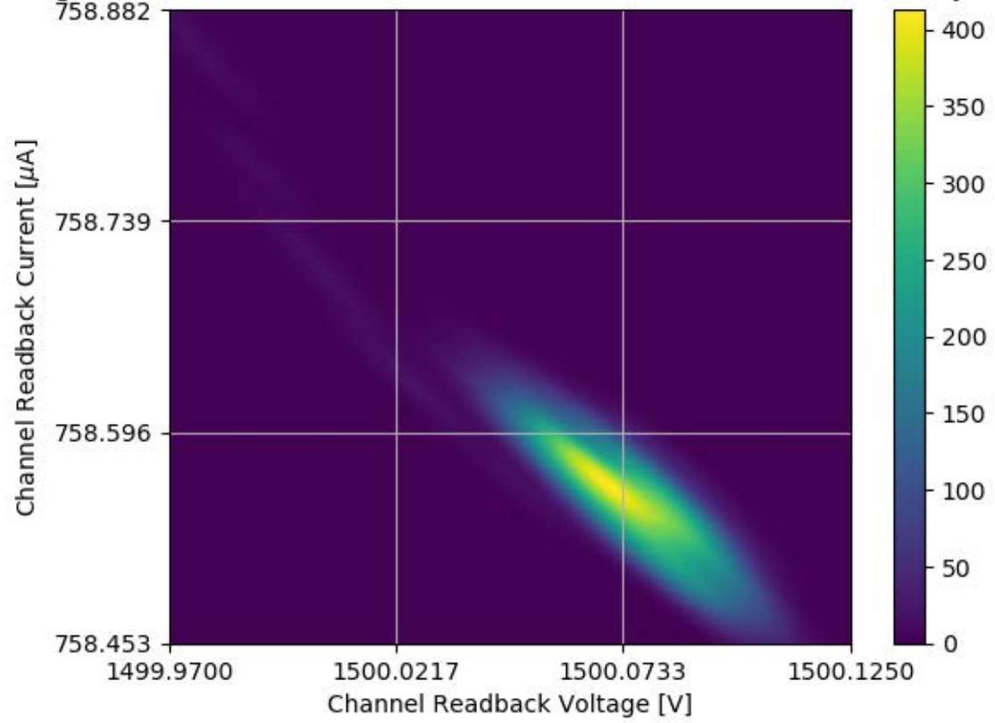
Voltage and Current Readback for Module #356 Channel 35 Stability Test
