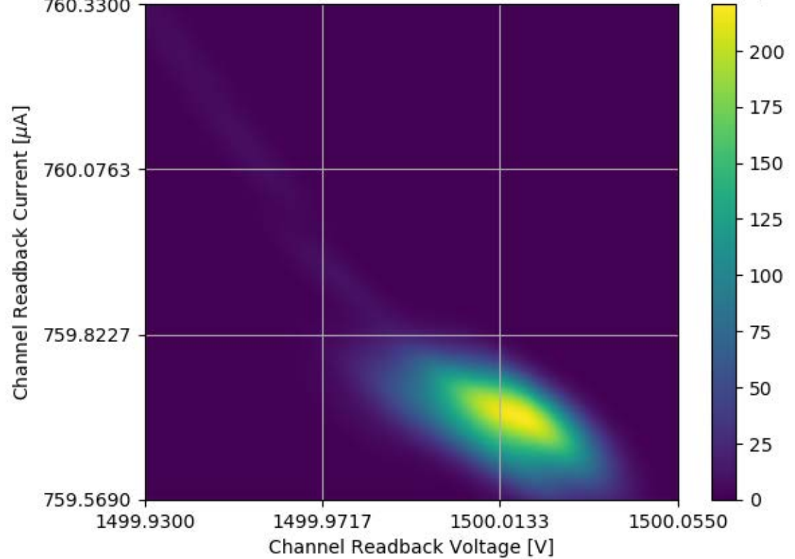
Voltage and Current Readback for Module #356 Channel 05 Stability Test
