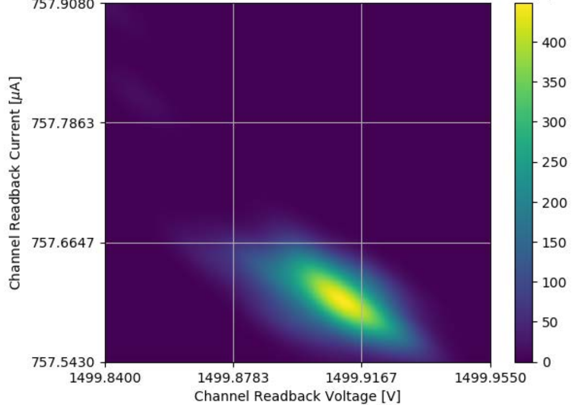
Voltage and Current Readback for Module #356 Channel 20 Stability Test
