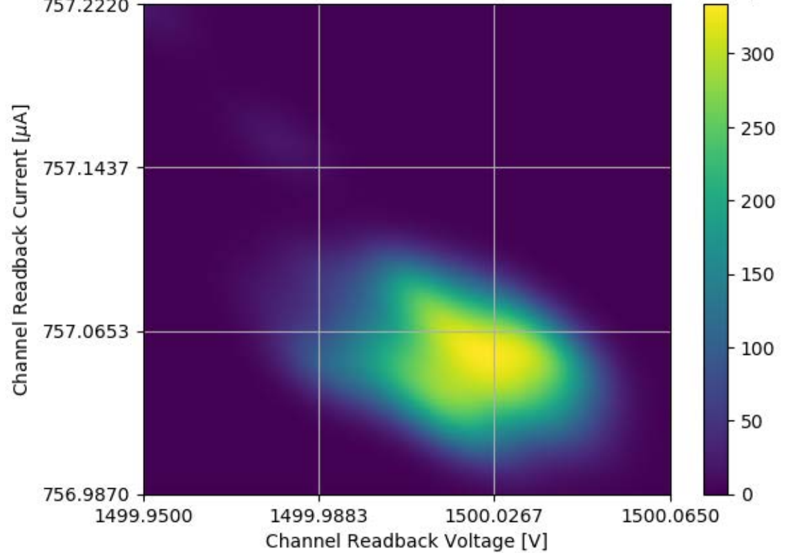
Voltage and Current Readback for Module #356 Channel 32 Stability Test
