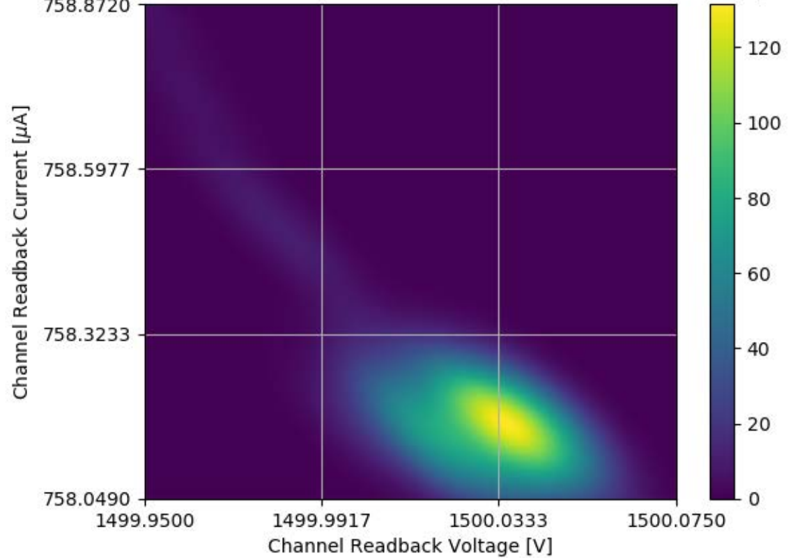
Voltage and Current Readback for Module #356 Channel 06 Stability Test
