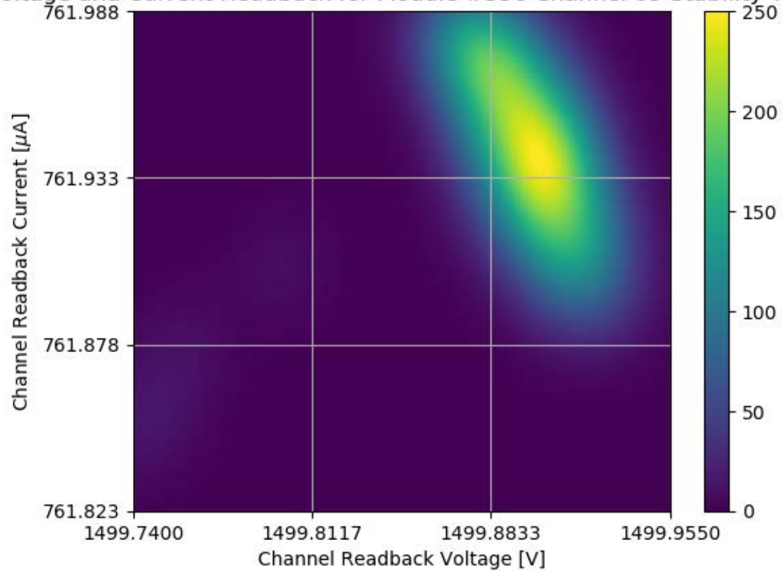
Voltage and Current Readback for Module #356 Channel 09 Stability Test
