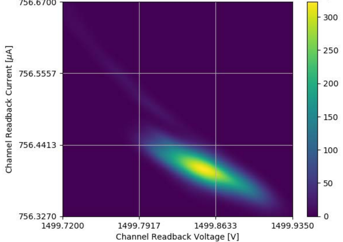
Voltage and Current Readback for Module #356 Channel 27 Stability Test
