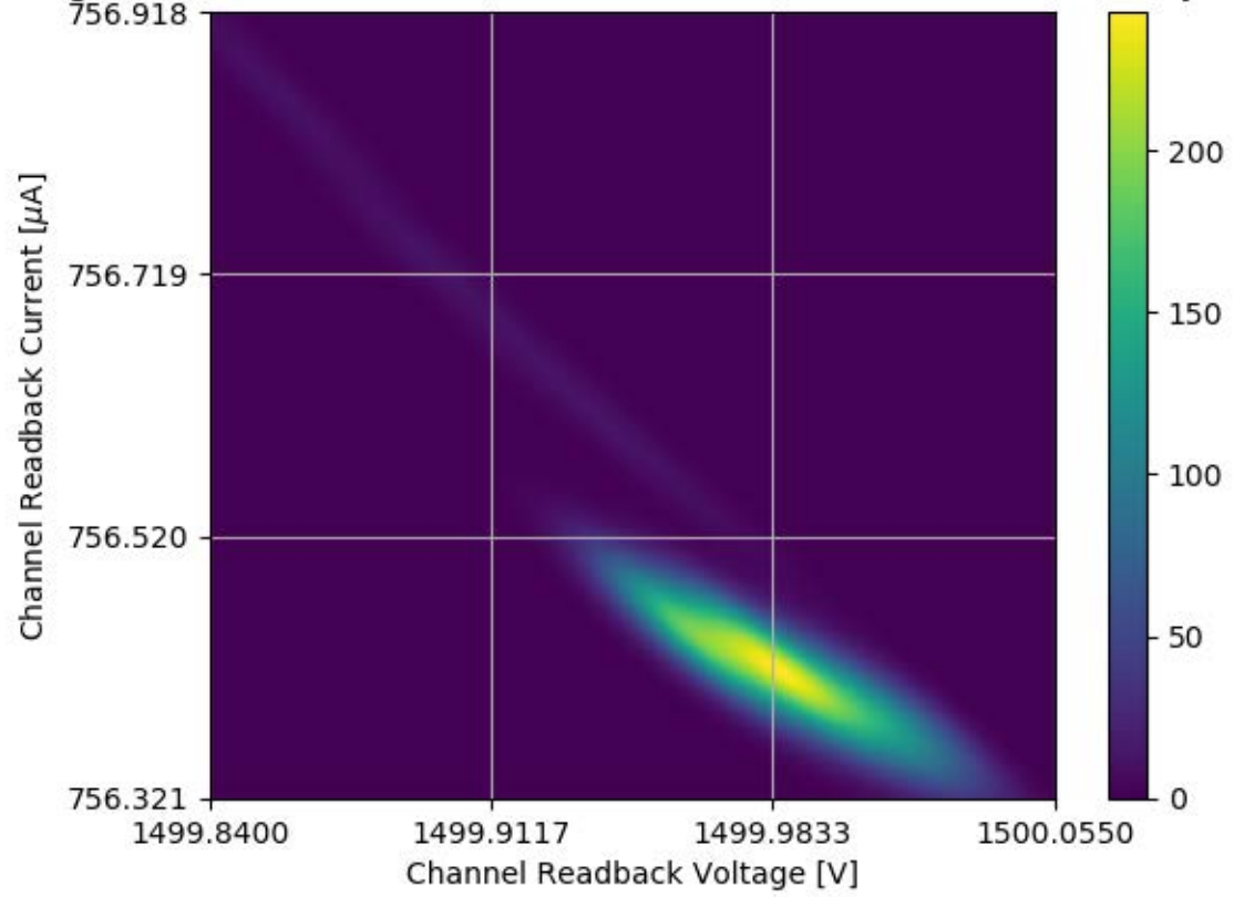
Voltage and Current Readback for Module #356 Channel 31 Stability Test
