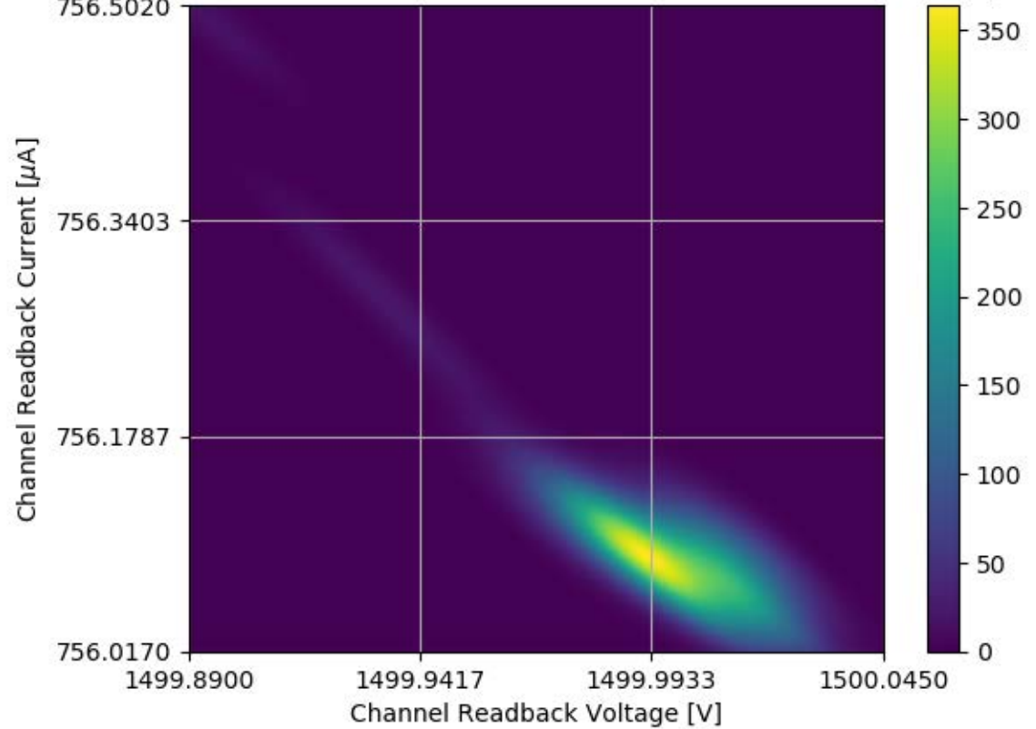
Voltage and Current Readback for Module #356 Channel 03 Stability Test
