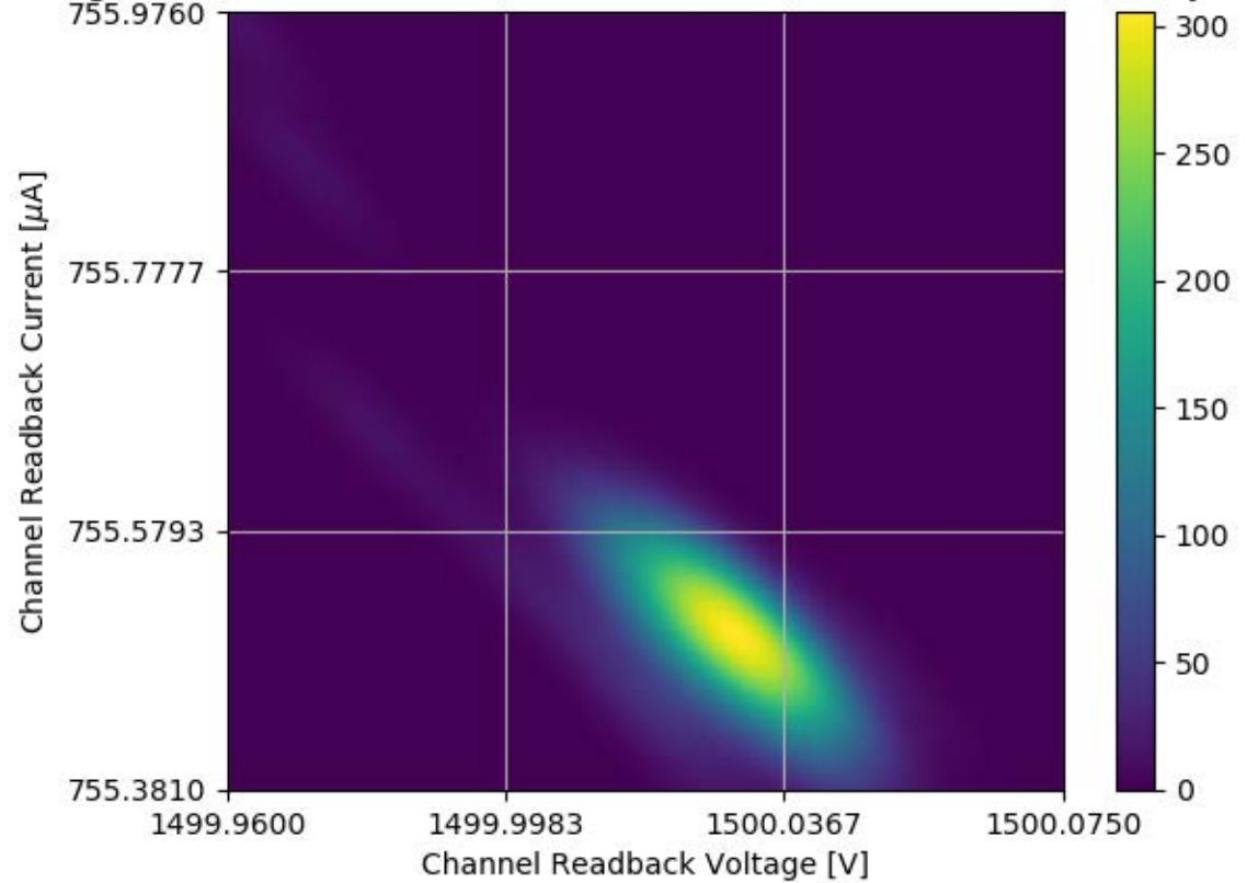
Voltage and Current Readback for Module #356 Channel 13 Stability Test
