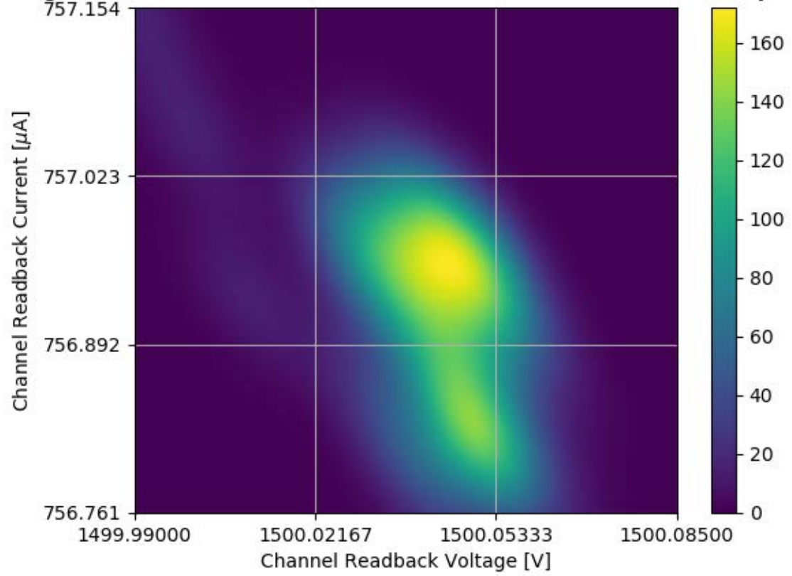
Voltage and Current Readback for Module #356 Channel 30 Stability Test
