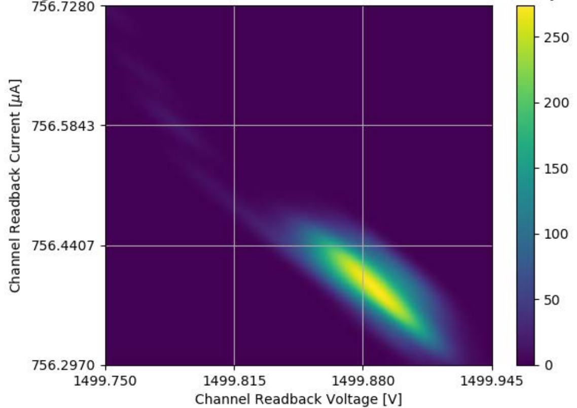
Voltage and Current Readback for Module #356 Channel 07 Stability Test
