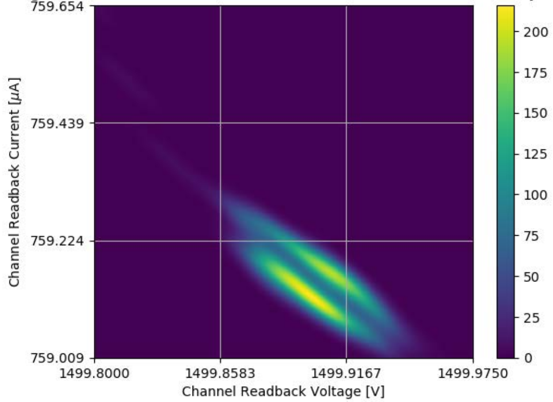
Voltage and Current Readback for Module #356 Channel 22 Stability Test
