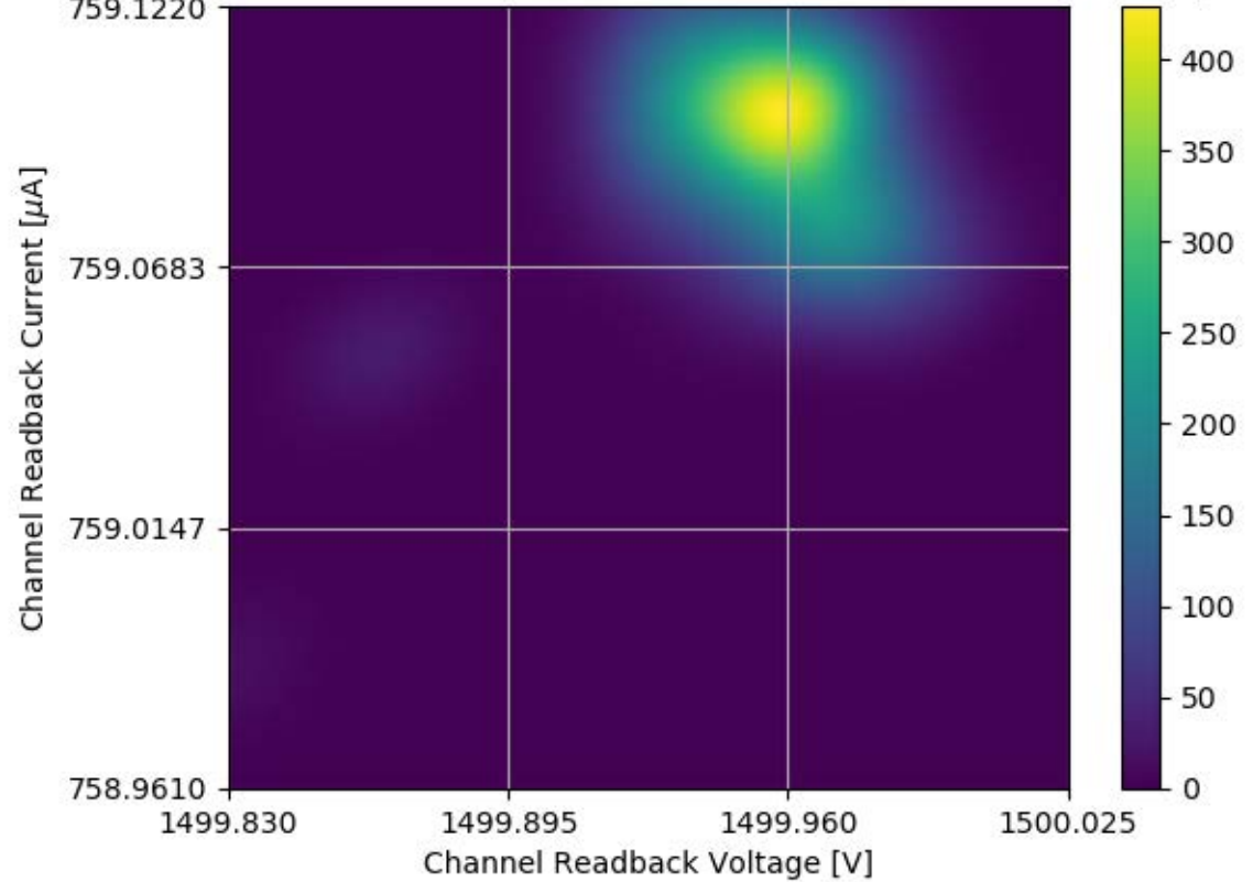
Voltage and Current Readback for Module #356 Channel 10 Stability Test
