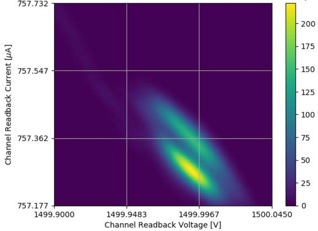
Voltage and Current Readback for Module #356 Channel 29 Stability Test
