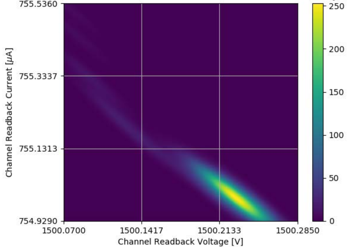
Voltage and Current Readback for Module #358 Channel 13 Stability Test
