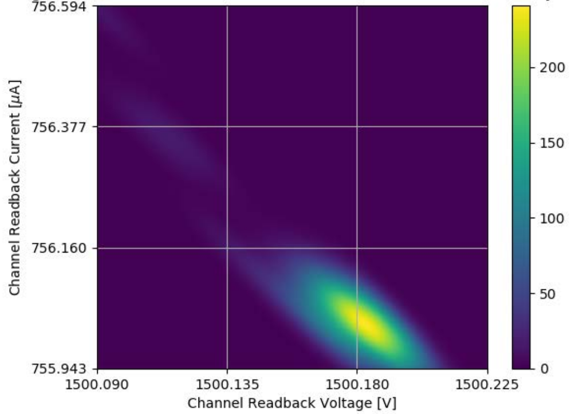
Voltage and Current Readback for Module #358 Channel 01 Stability Test
