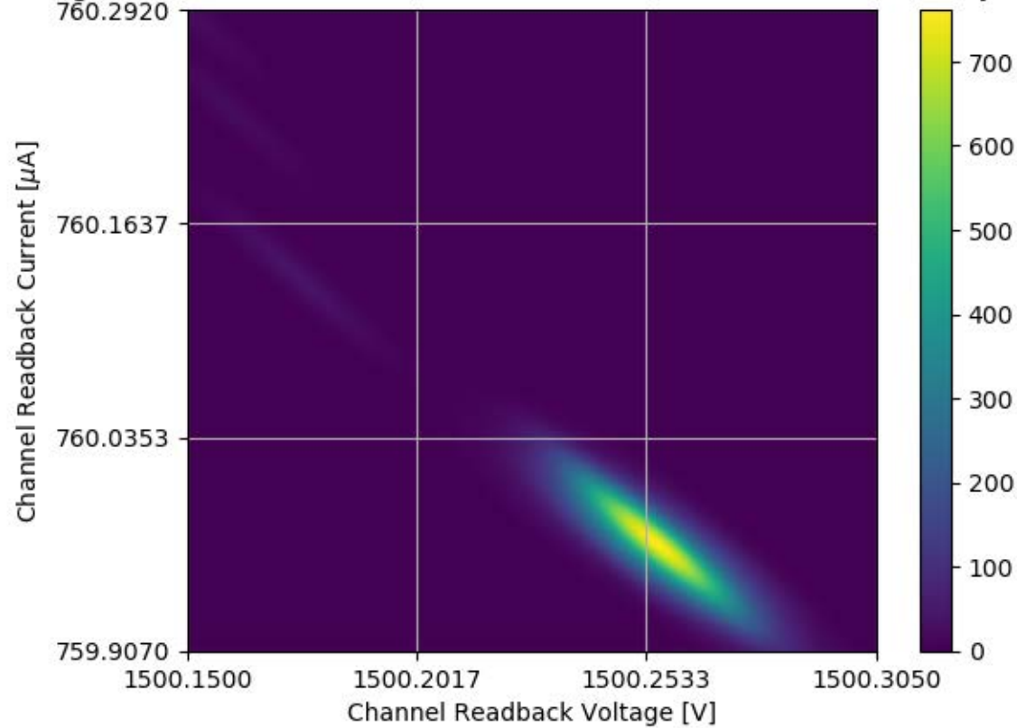
Voltage and Current Readback for Module #358 Channel 12 Stability Test
