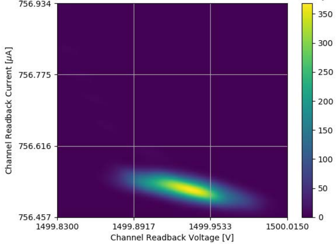
Voltage and Current Readback for Module #358 Channel 20 Stability Test
