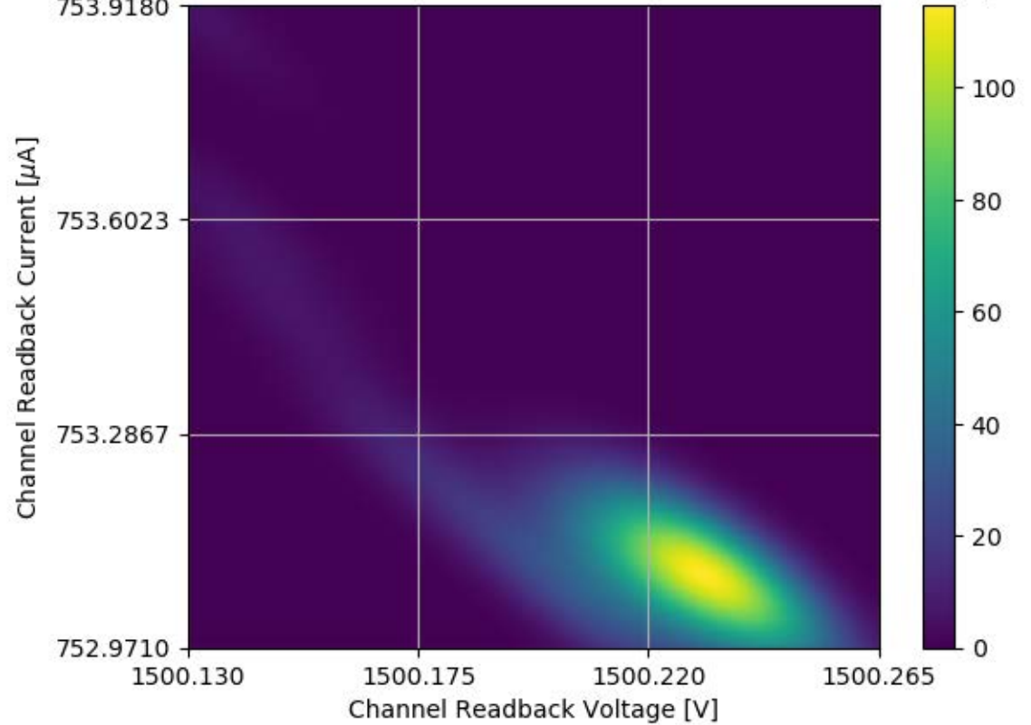
Voltage and Current Readback for Module #358 Channel 11 Stability Test
