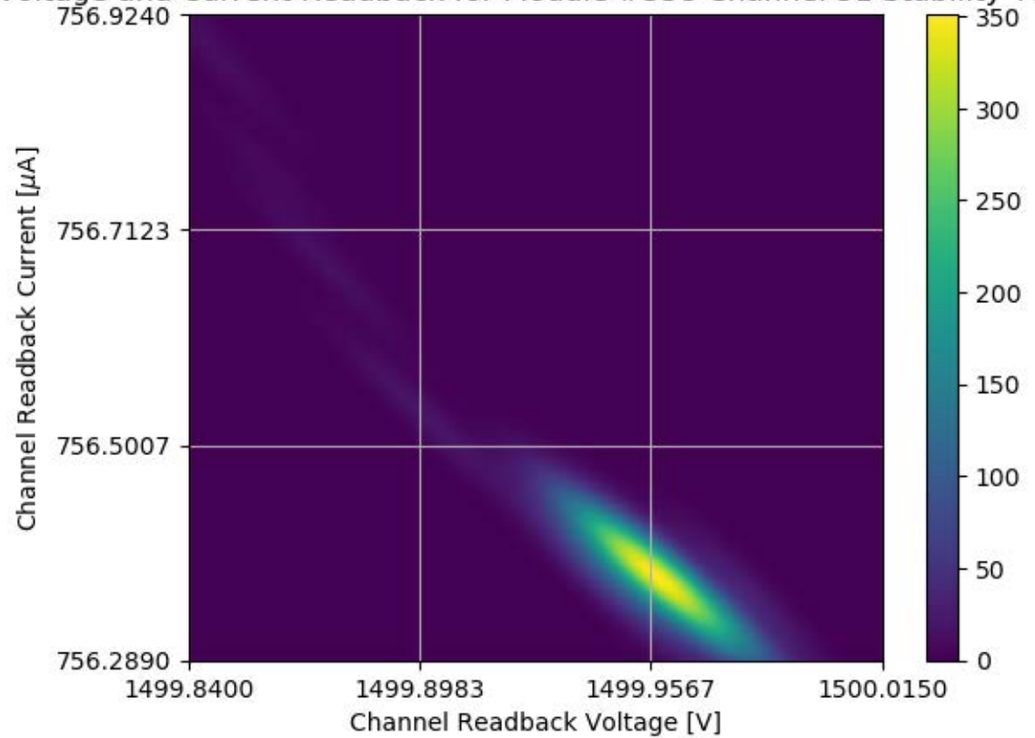
Voltage and Current Readback for Module #358 Channel 31 Stability Test
