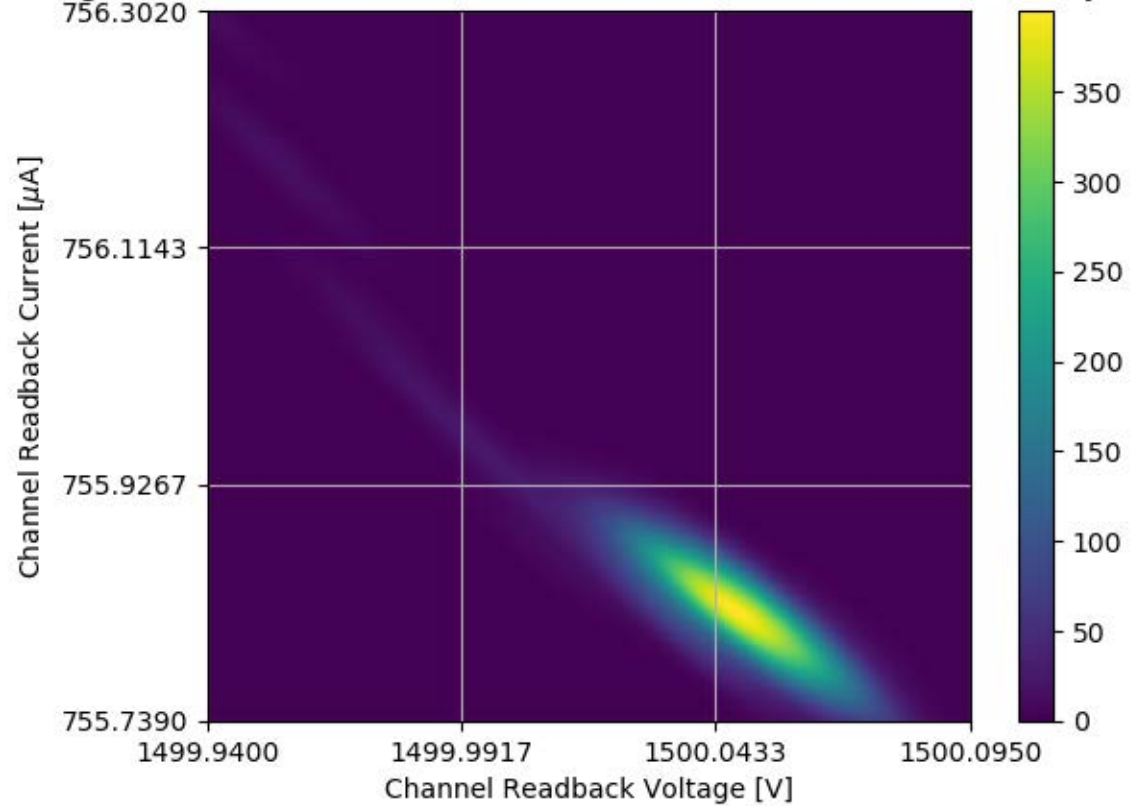
Voltage and Current Readback for Module #358 Channel 28 Stability Test
