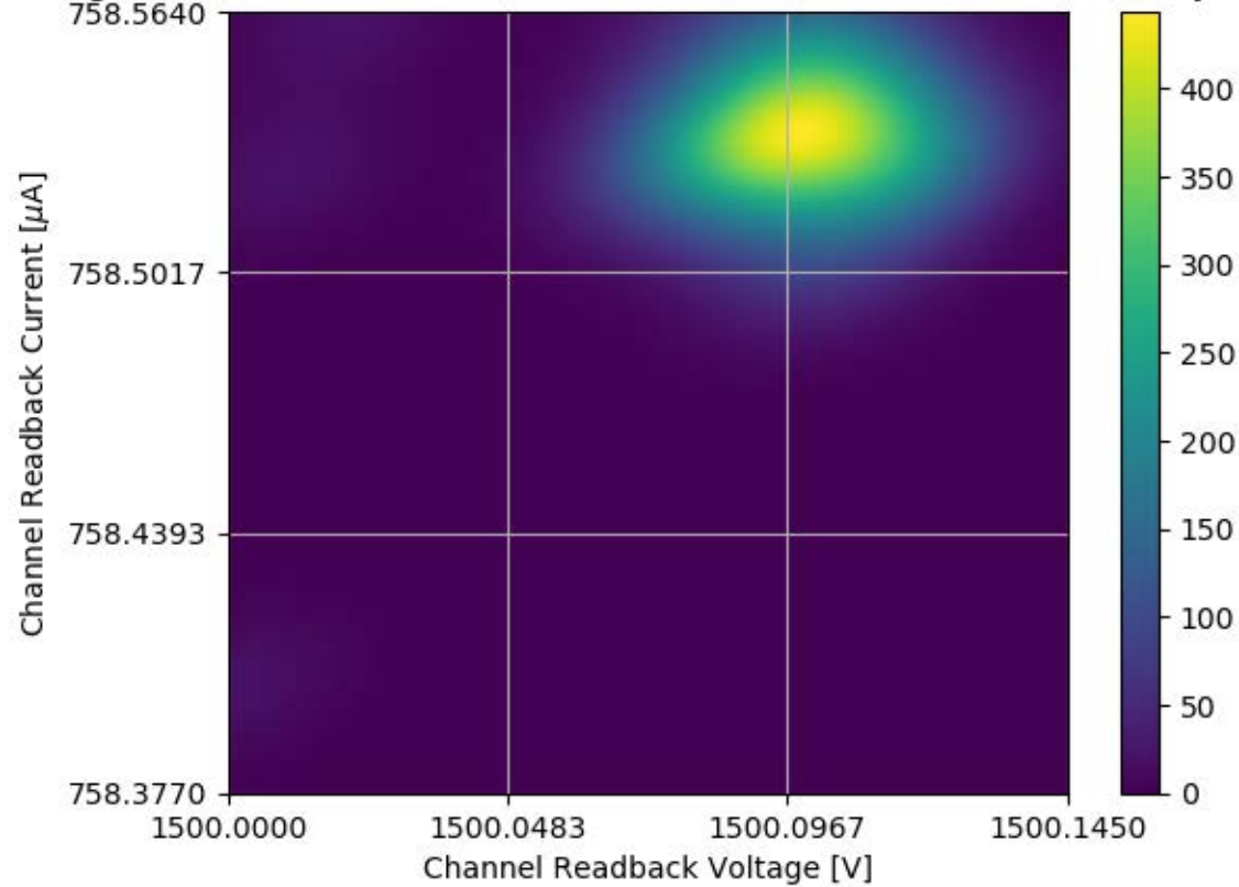
Voltage and Current Readback for Module #358 Channel 10 Stability Test
