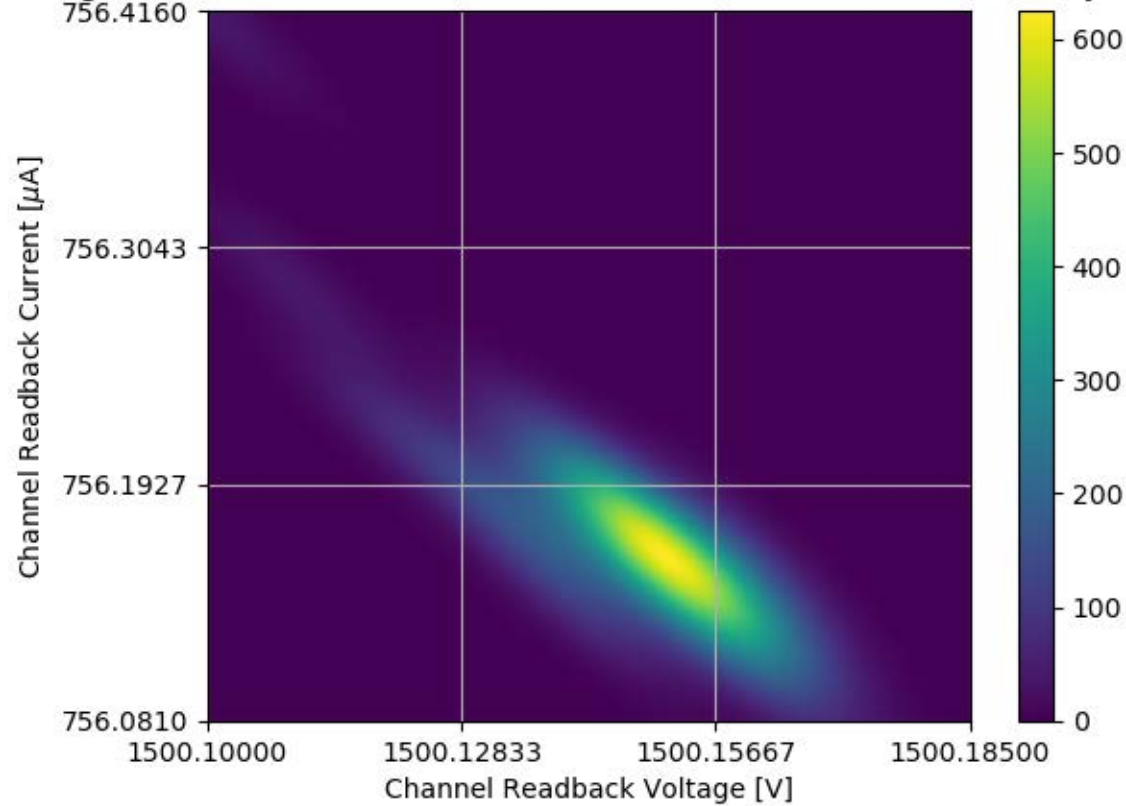
Voltage and Current Readback for Module #358 Channel 07 Stability Test
