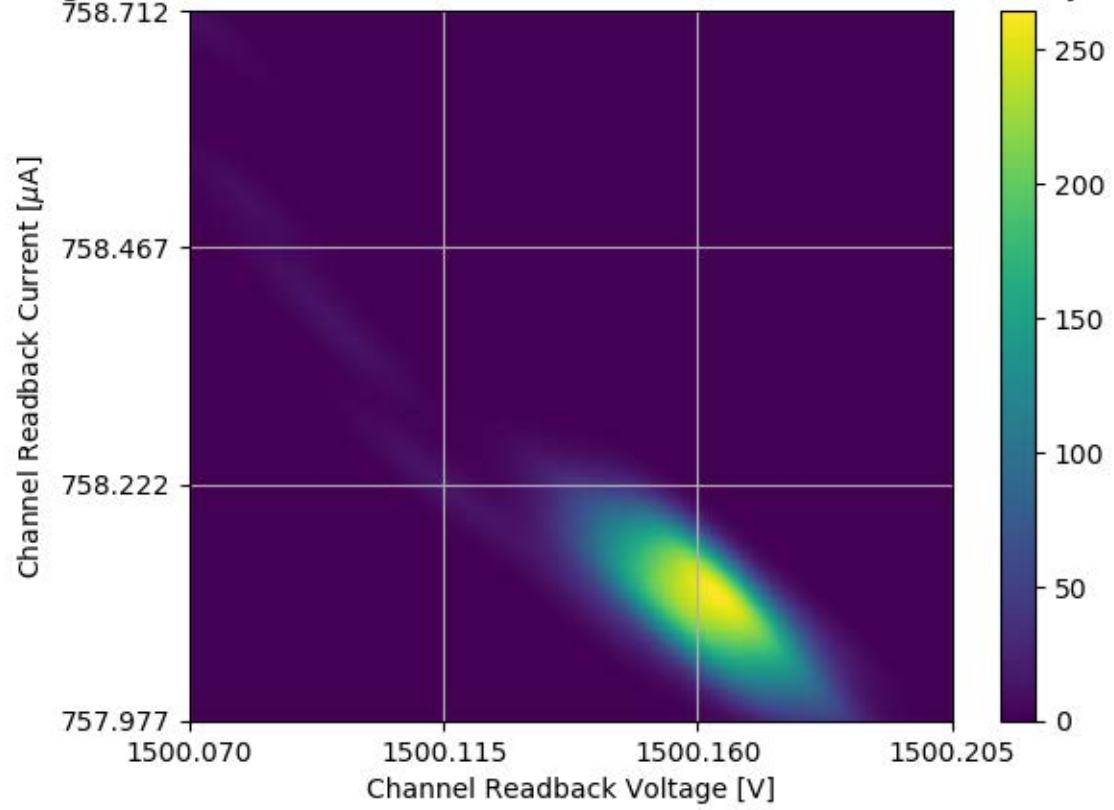
Voltage and Current Readback for Module #358 Channel 35 Stability Test
