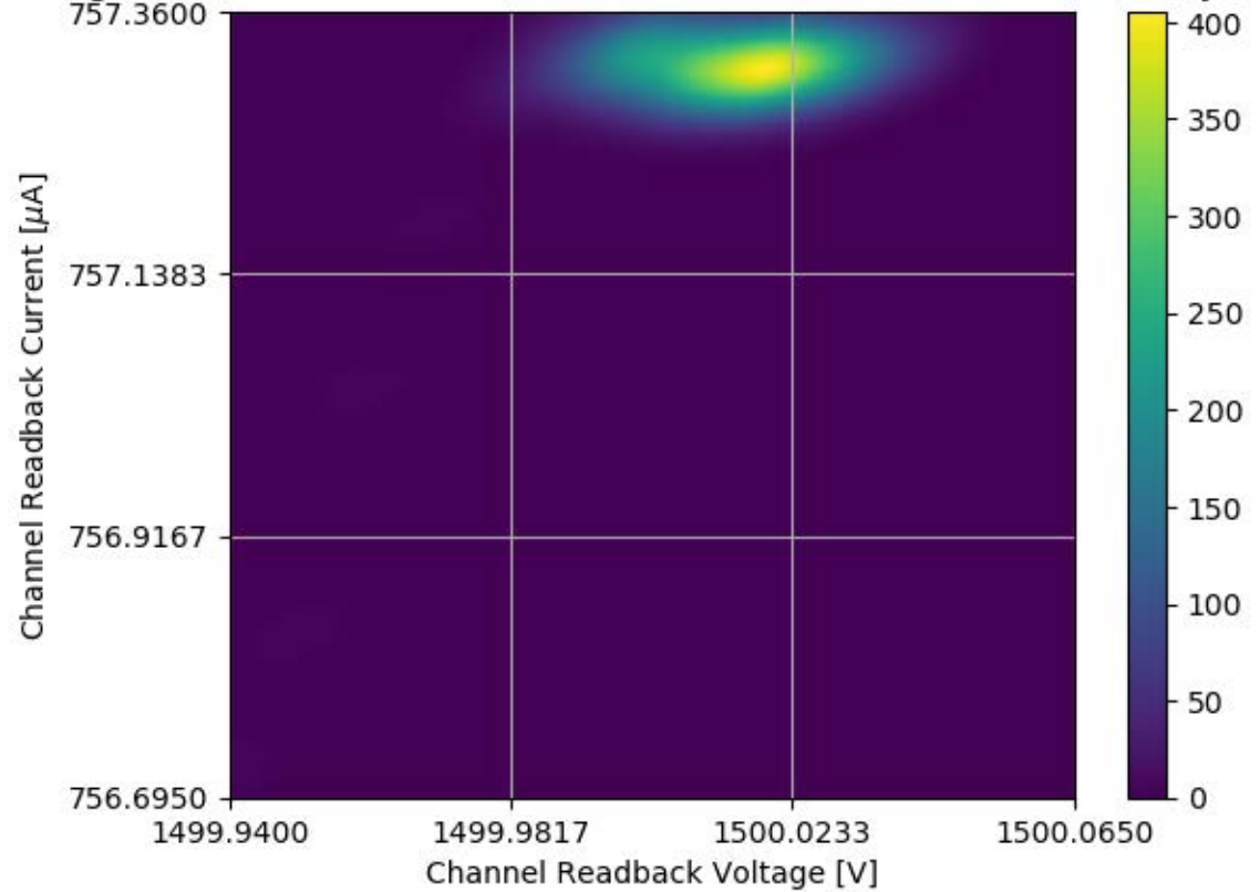
Voltage and Current Readback for Module #358 Channel 26 Stability Test
