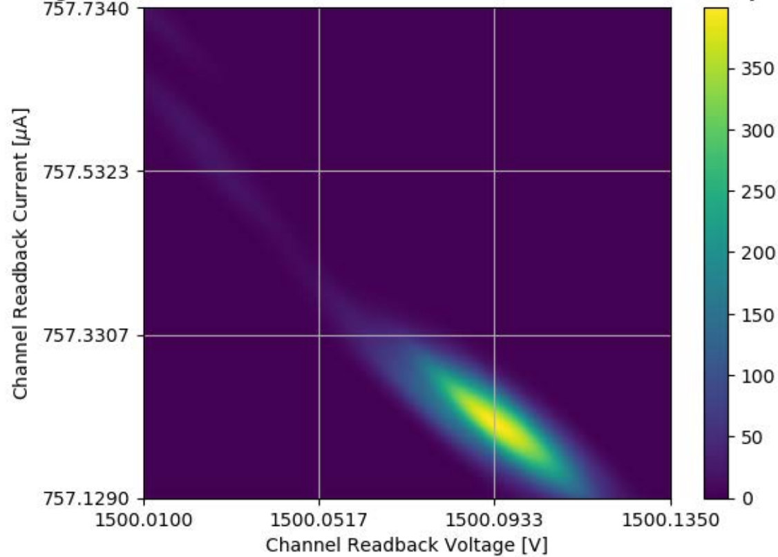
Voltage and Current Readback for Module #358 Channel 19 Stability Test
