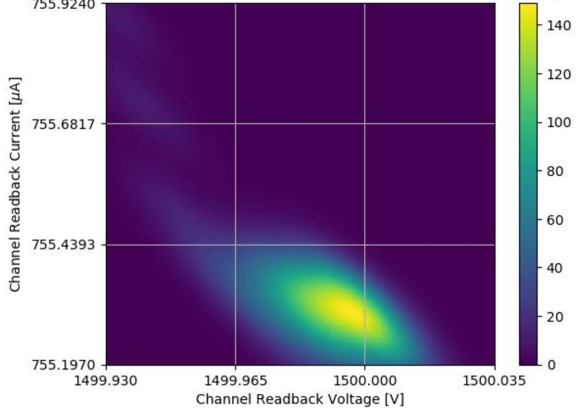
Voltage and Current Readback for Module #358 Channel 03 Stability Test
