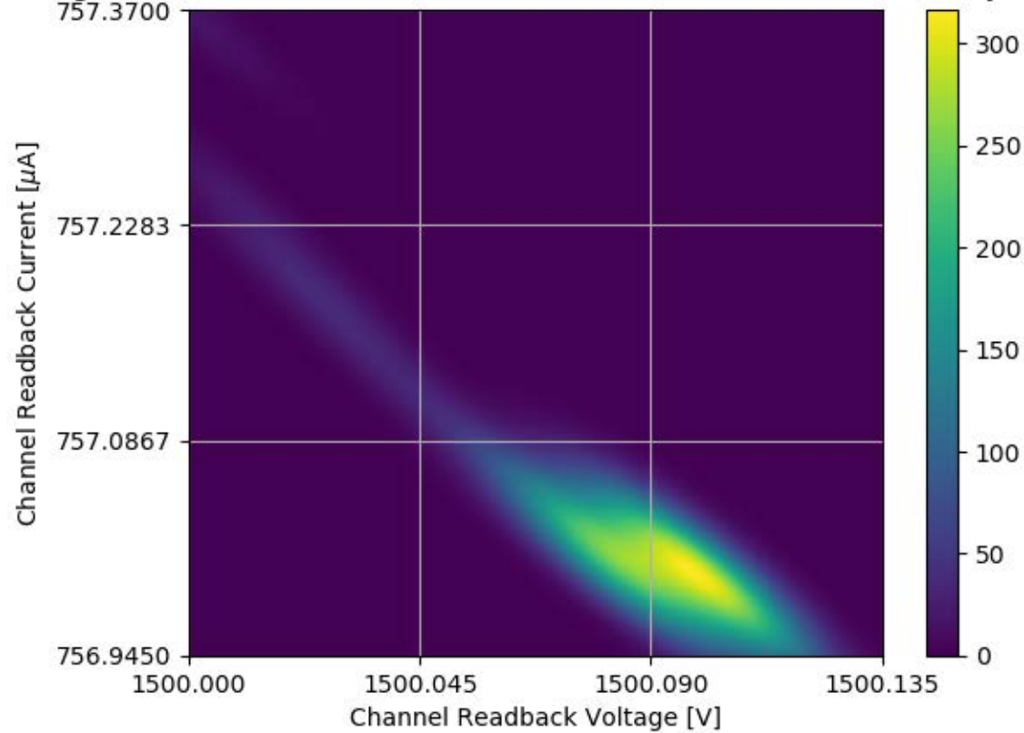
Voltage and Current Readback for Module #358 Channel 32 Stability Test
