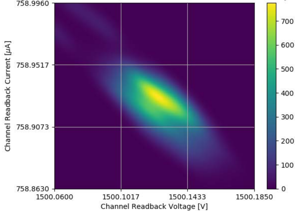
Voltage and Current Readback for Module #358 Channel 25 Stability Test
