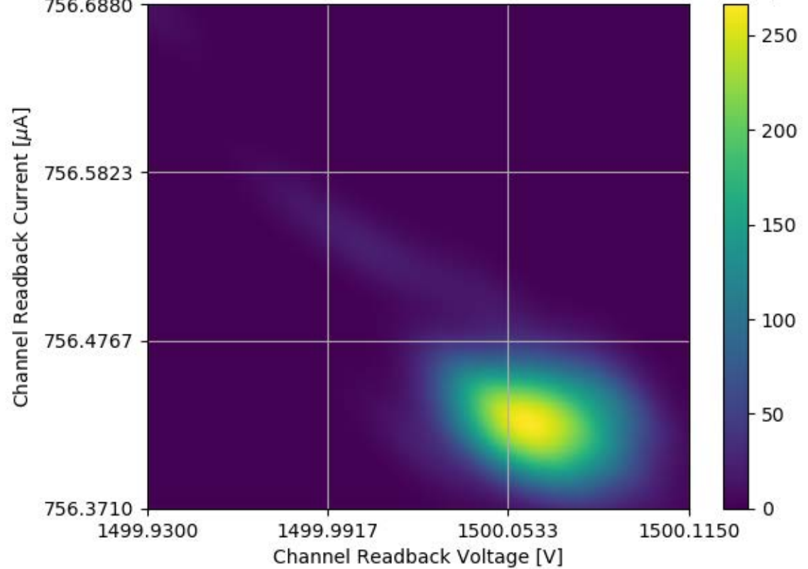
Voltage and Current Readback for Module #358 Channel 23 Stability Test
