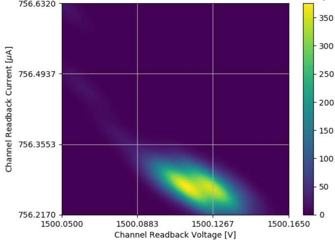
Voltage and Current Readback for Module #358 Channel 15 Stability Test
