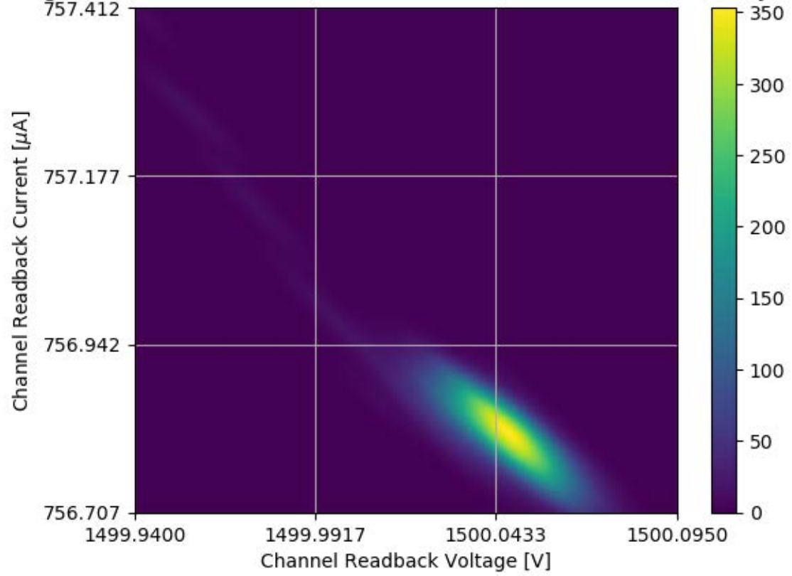
Voltage and Current Readback for Module #358 Channel 27 Stability Test
