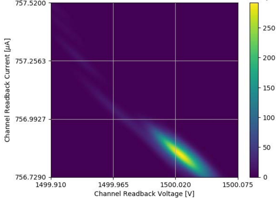
Voltage and Current Readback for Module #358 Channel 02 Stability Test
