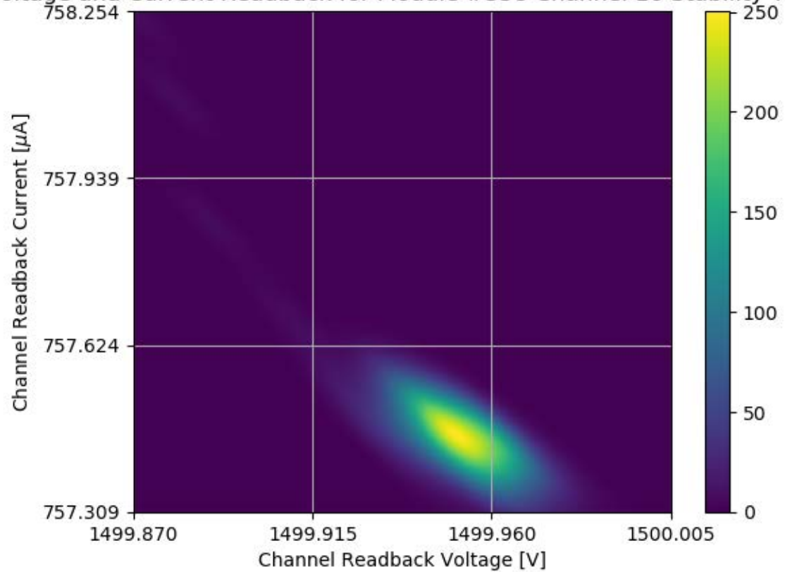
Voltage and Current Readback for Module #358 Channel 16 Stability Test
