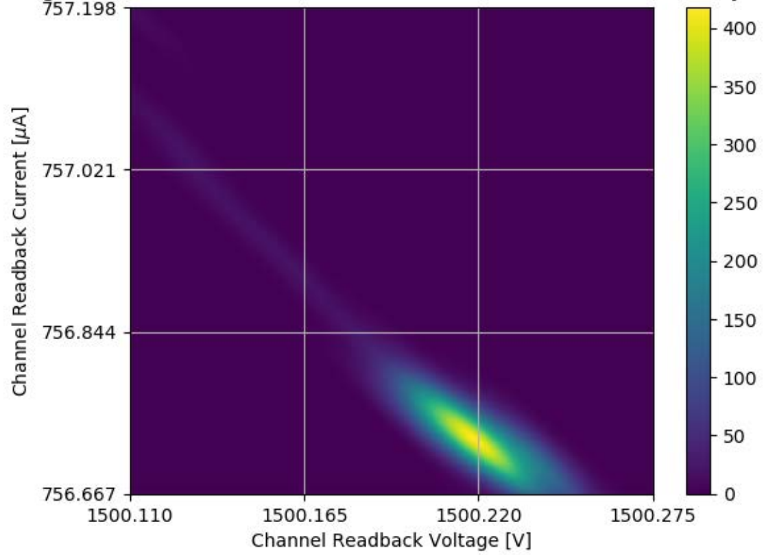
Voltage and Current Readback for Module #358 Channel 29 Stability Test
