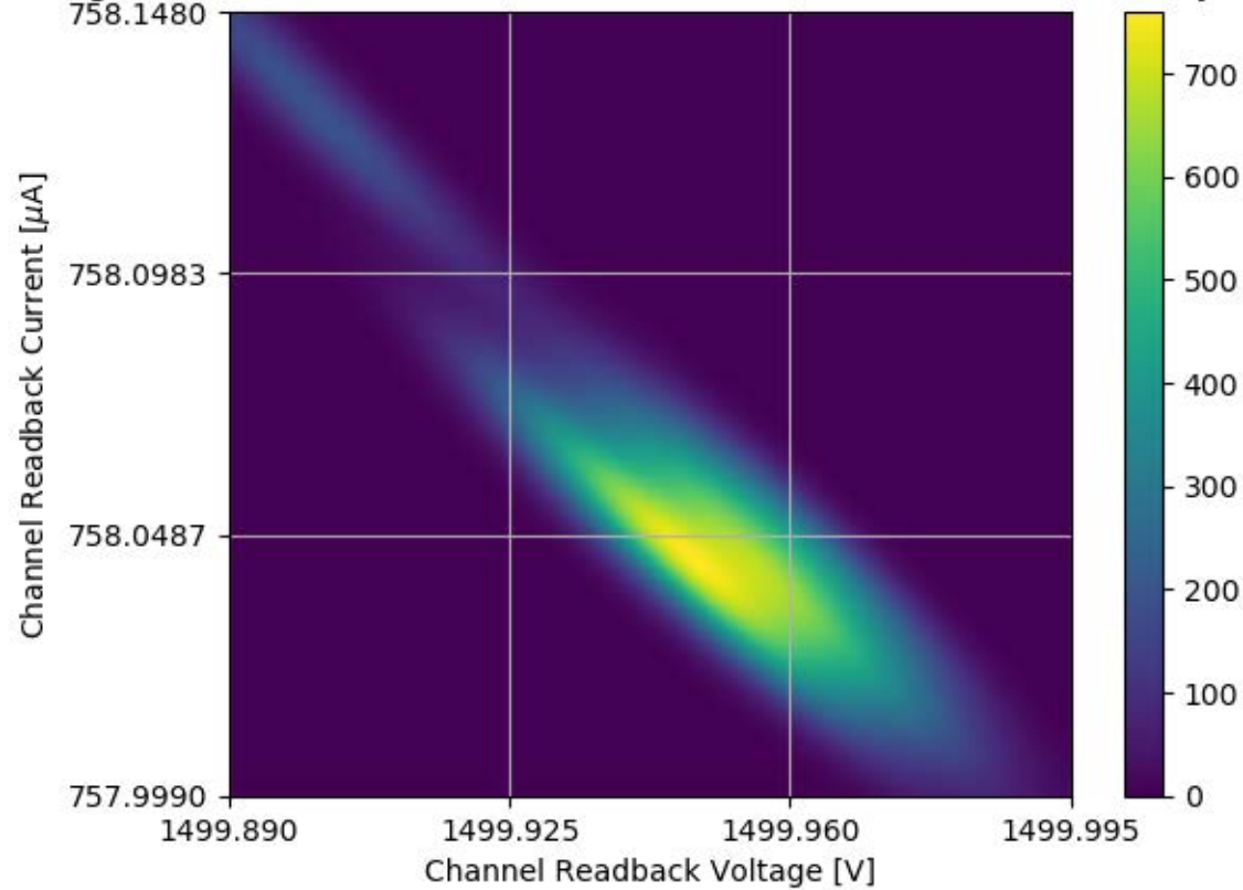
Voltage and Current Readback for Module #358 Channel 08 Stability Test
