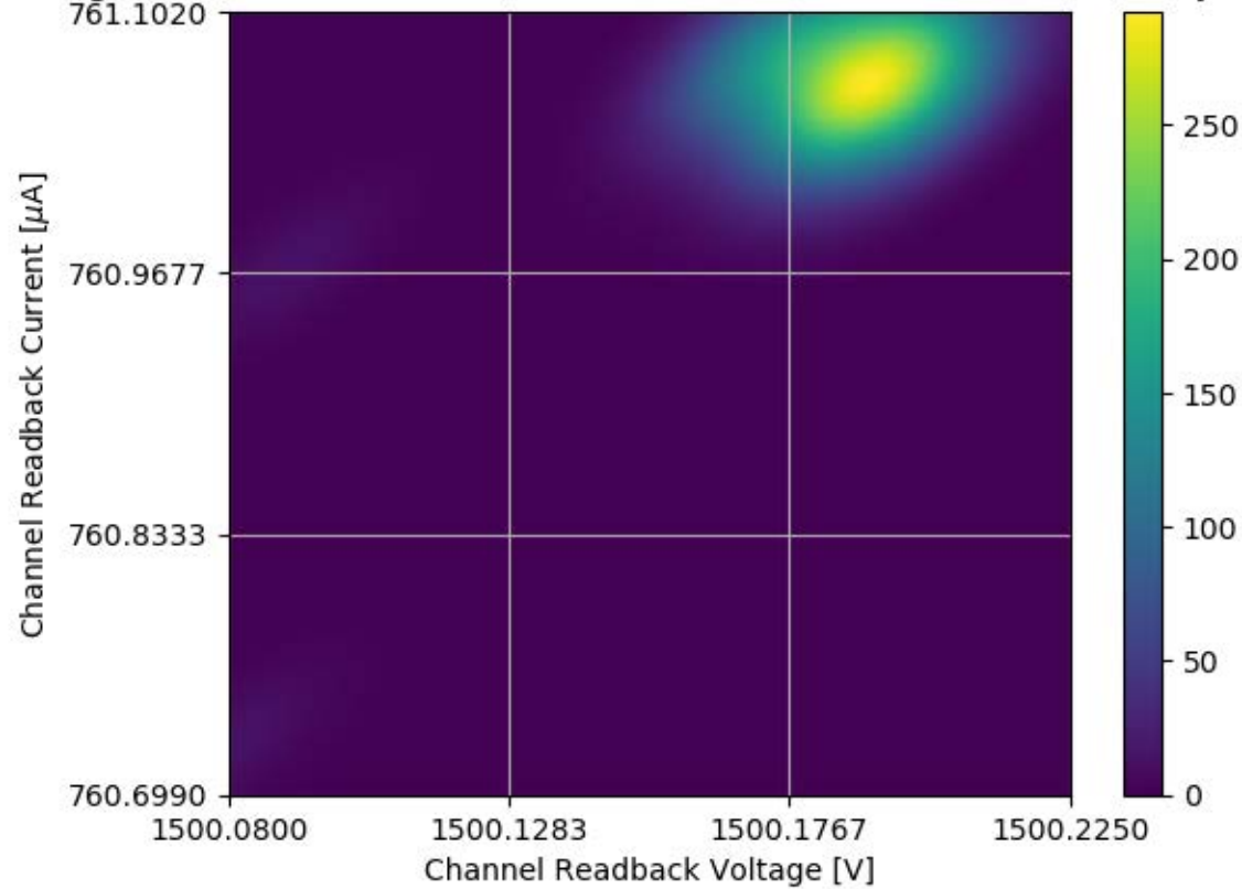
Voltage and Current Readback for Module #358 Channel 09 Stability Test
