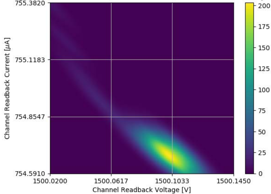
Voltage and Current Readback for Module #358 Channel 00 Stability Test
