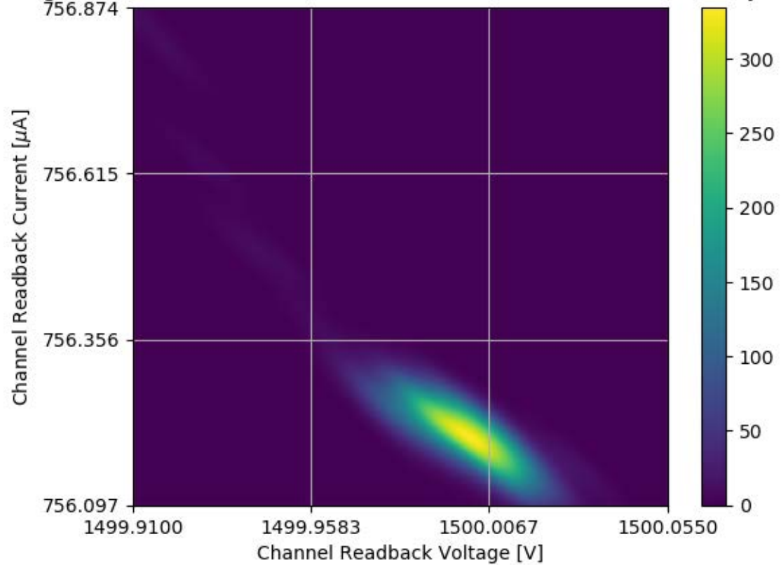
Voltage and Current Readback for Module #358 Channel 17 Stability Test
