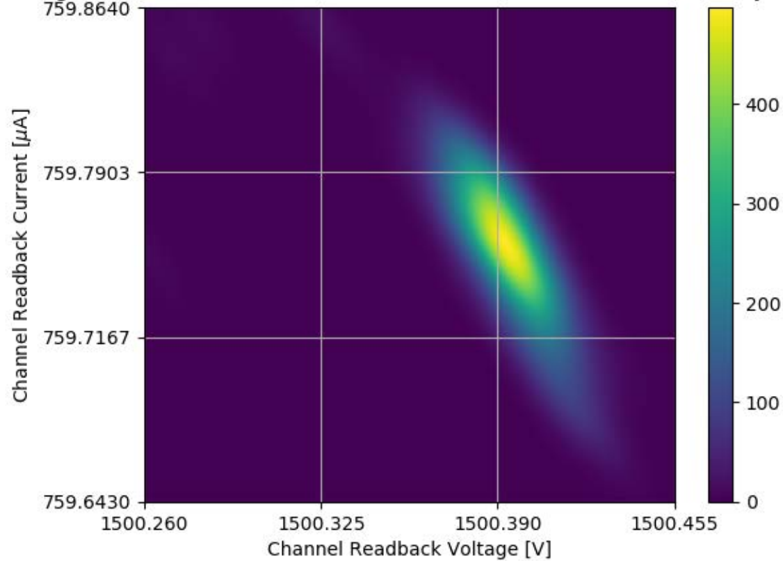
Voltage and Current Readback for Module #358 Channel 24 Stability Test
