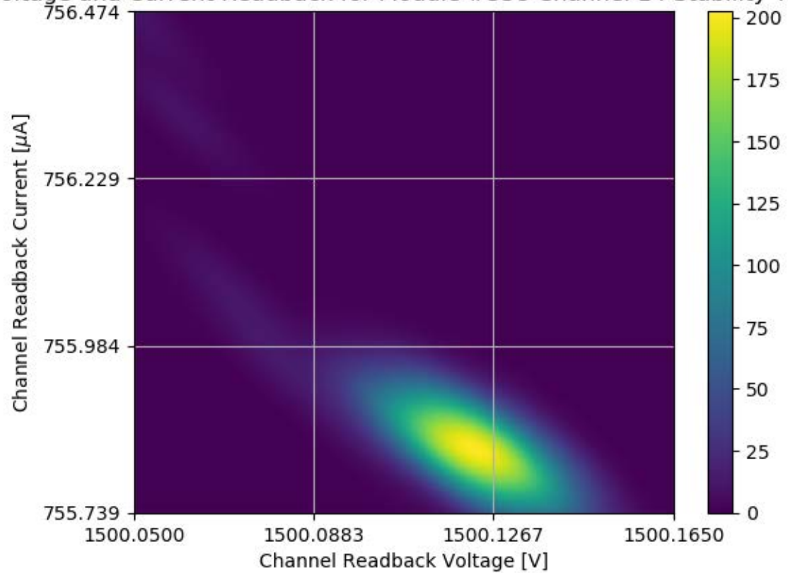
Voltage and Current Readback for Module #358 Channel 14 Stability Test
