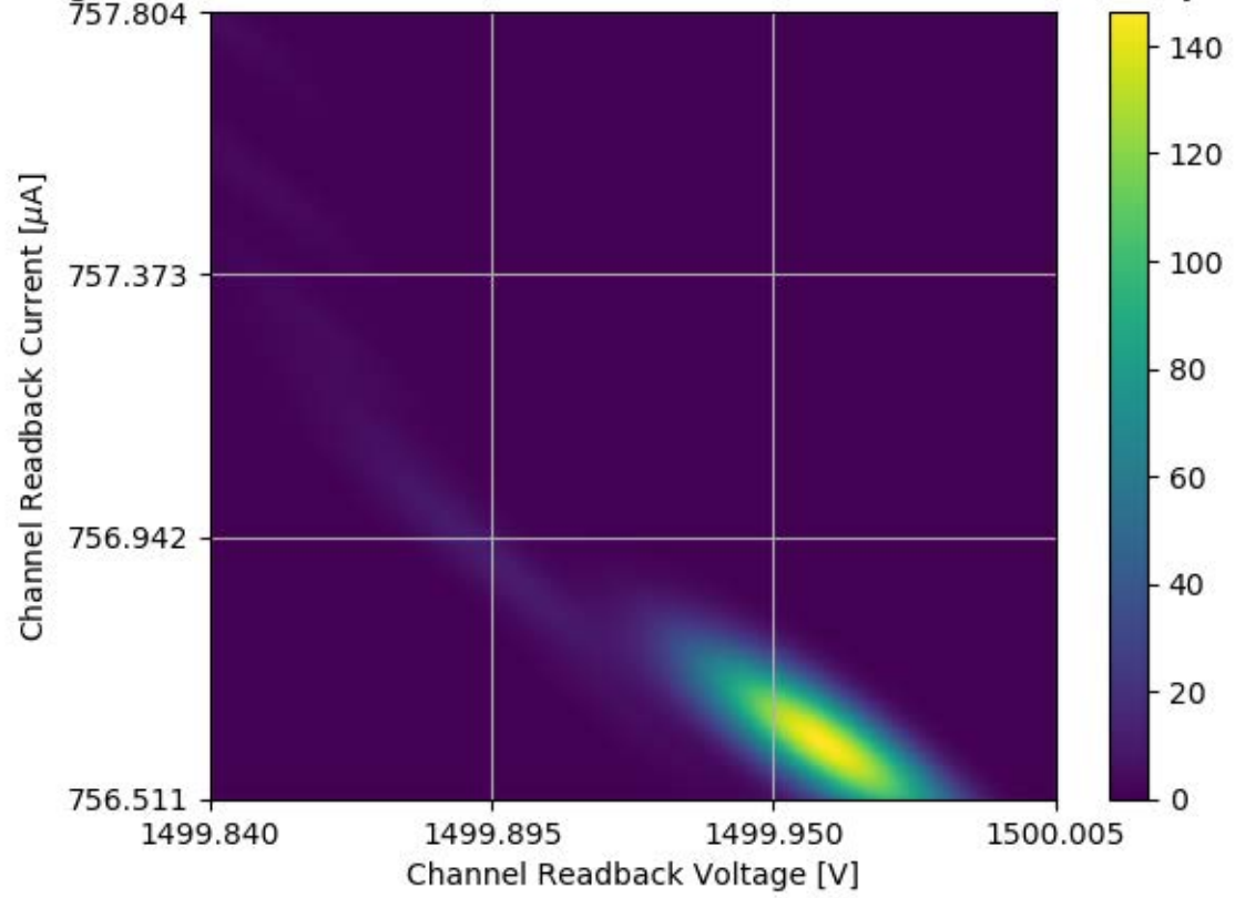
Voltage and Current Readback for Module #358 Channel 18 Stability Test
