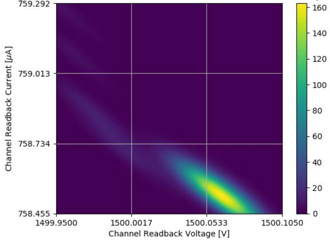
Voltage and Current Readback for Module #358 Channel 05 Stability Test
