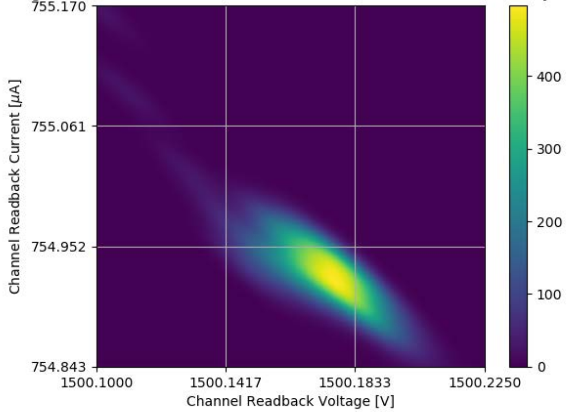
Voltage and Current Readback for Module #358 Channel 30 Stability Test
