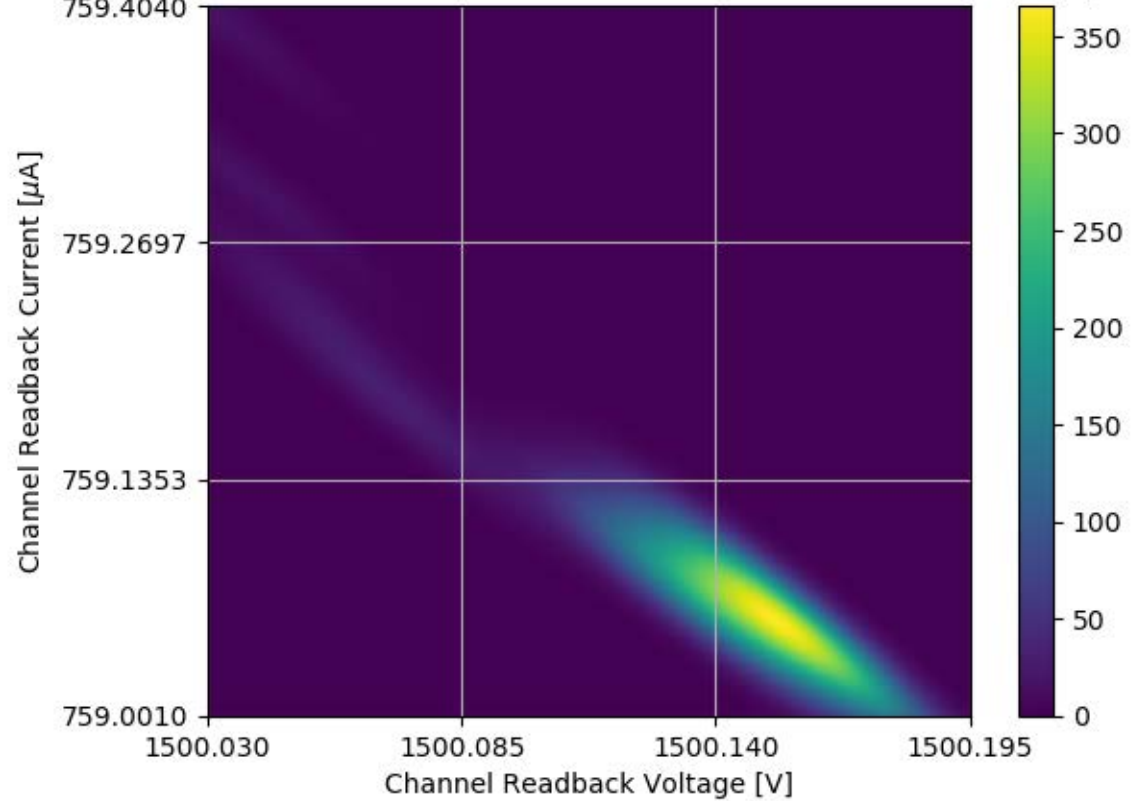
Voltage and Current Readback for Module #358 Channel 04 Stability Test
