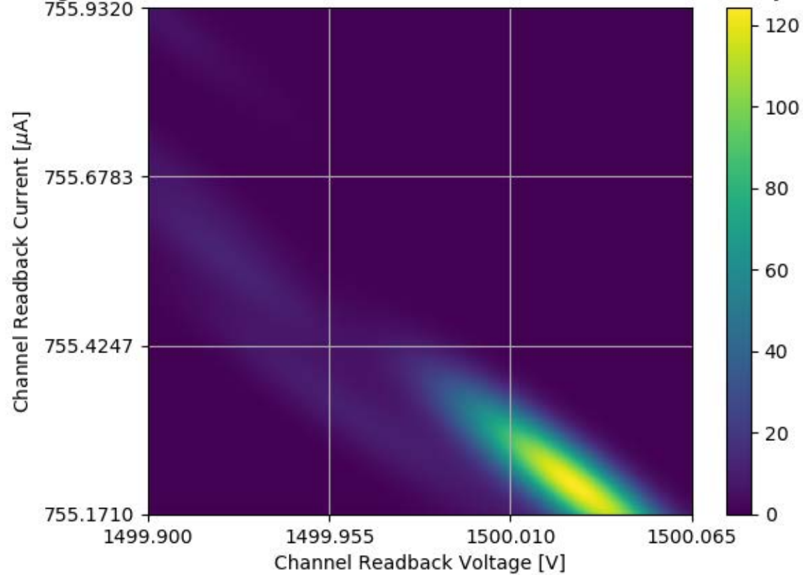
Voltage and Current Readback for Module #359 Channel 00 Stability Test
