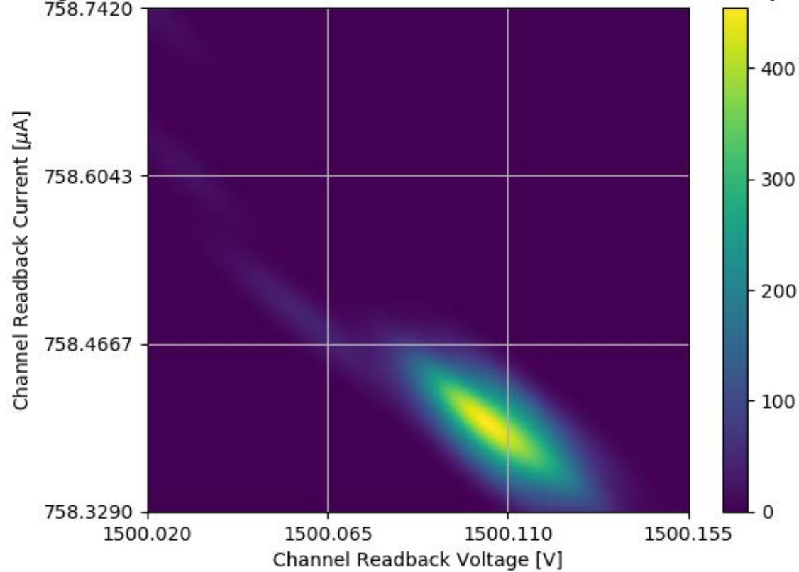
Voltage and Current Readback for Module #359 Channel 35 Stability Test
