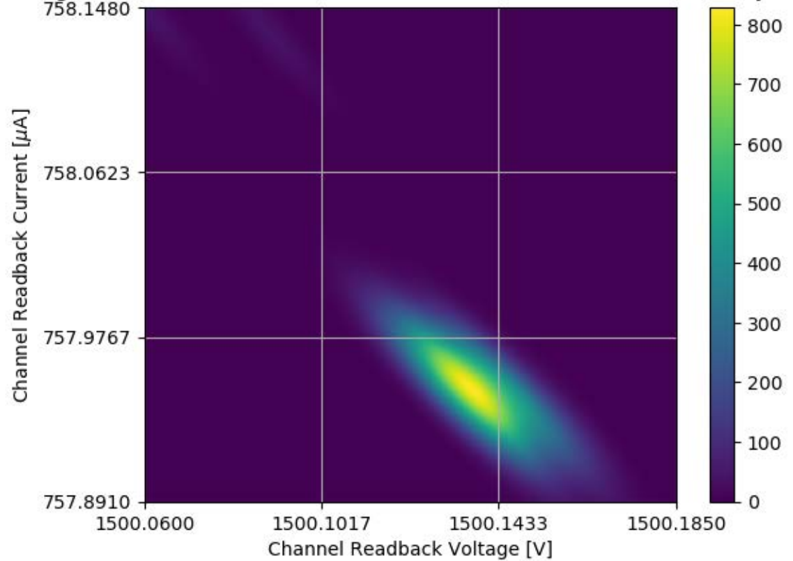
Voltage and Current Readback for Module #359 Channel 26 Stability Test
