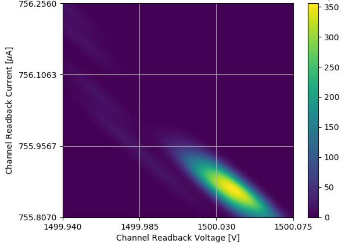
Voltage and Current Readback for Module #359 Channel 14 Stability Test
