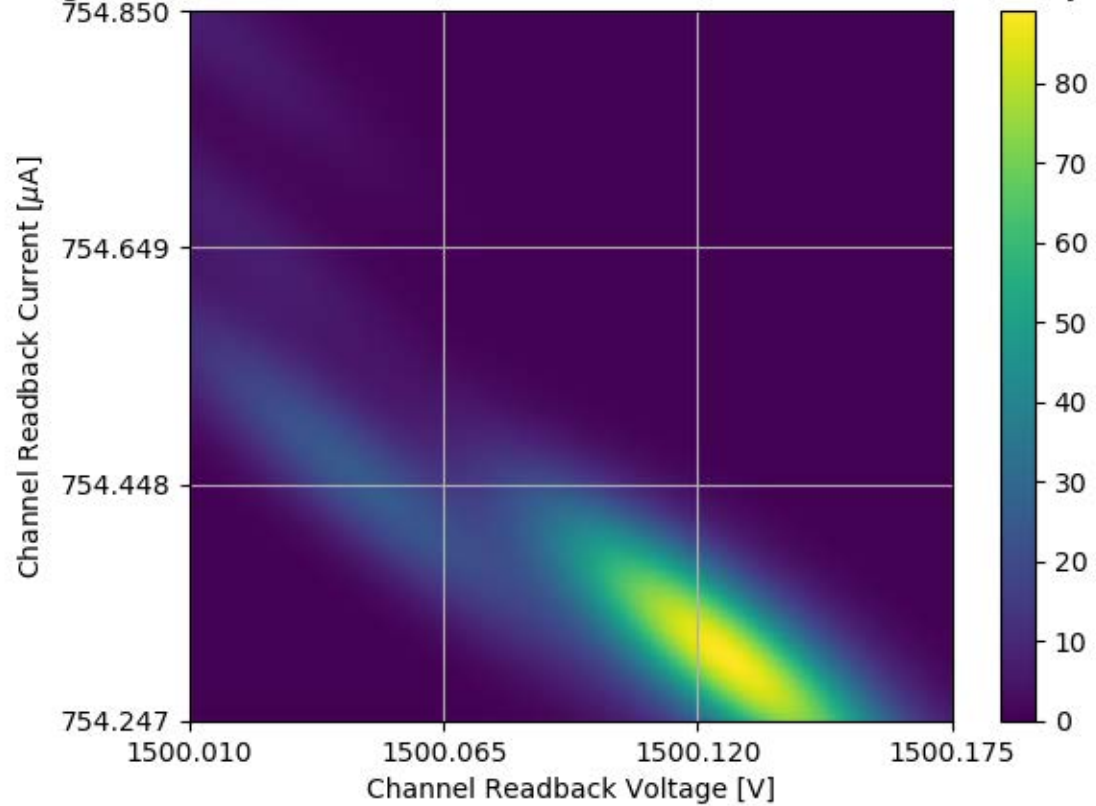
Voltage and Current Readback for Module #359 Channel 11 Stability Test
