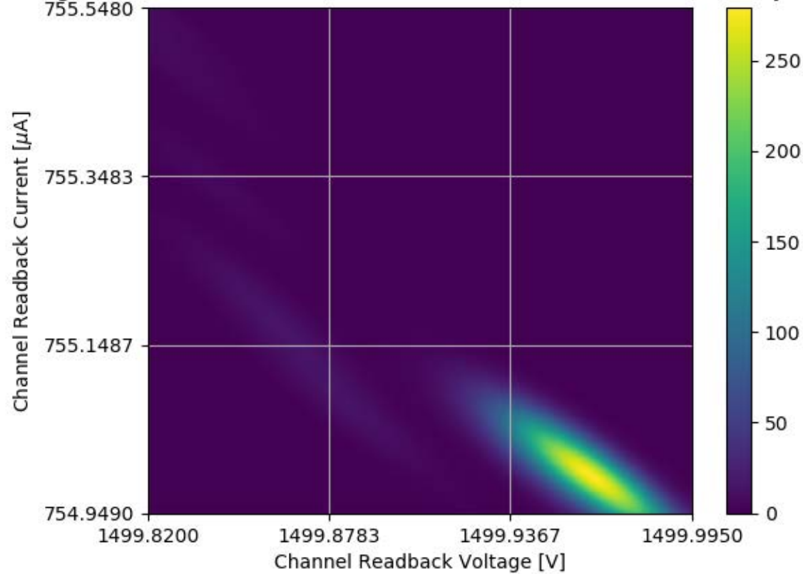
Voltage and Current Readback for Module #359 Channel 13 Stability Test
