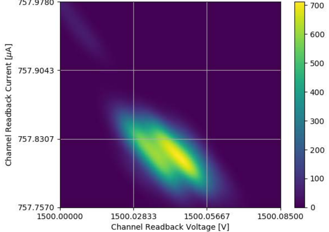
Voltage and Current Readback for Module #359 Channel 20 Stability Test
