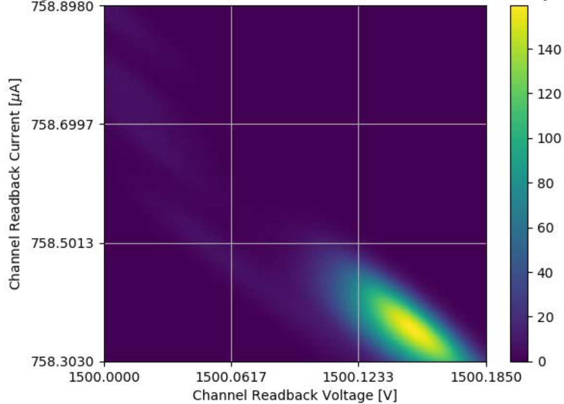
Voltage and Current Readback for Module #359 Channel 06 Stability Test
