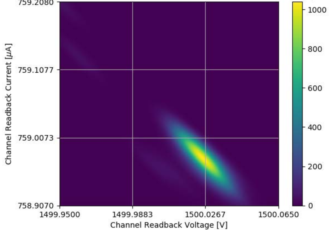
Voltage and Current Readback for Module #359 Channel 04 Stability Test
