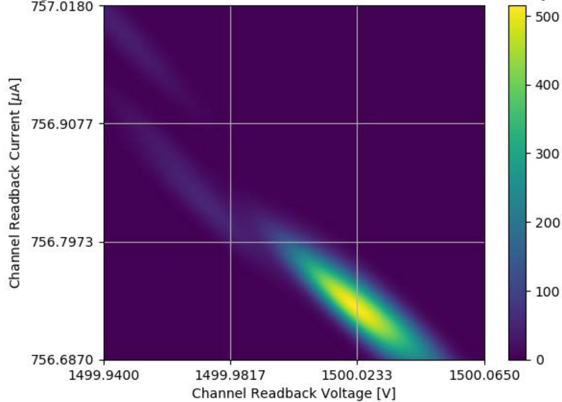
Voltage and Current Readback for Module #359 Channel 23 Stability Test
