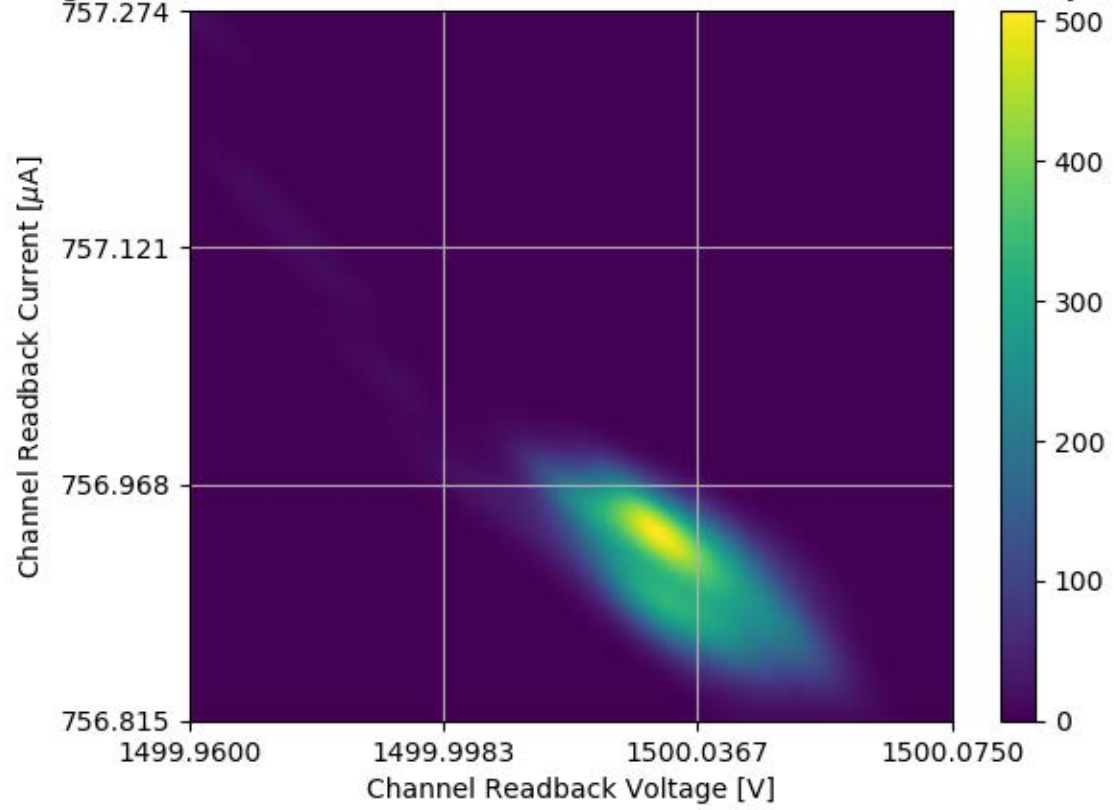
Voltage and Current Readback for Module #359 Channel 27 Stability Test
