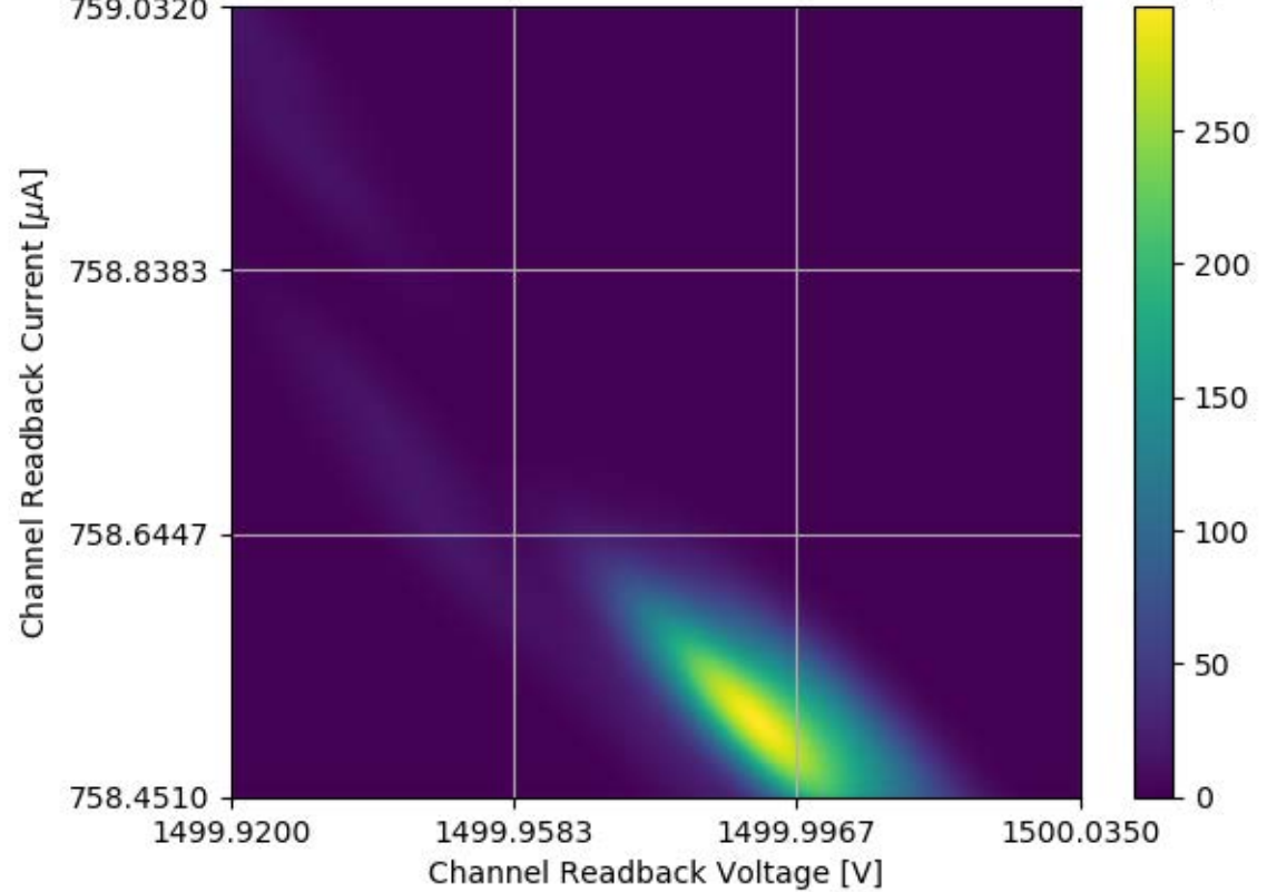
Voltage and Current Readback for Module #359 Channel 21 Stability Test
