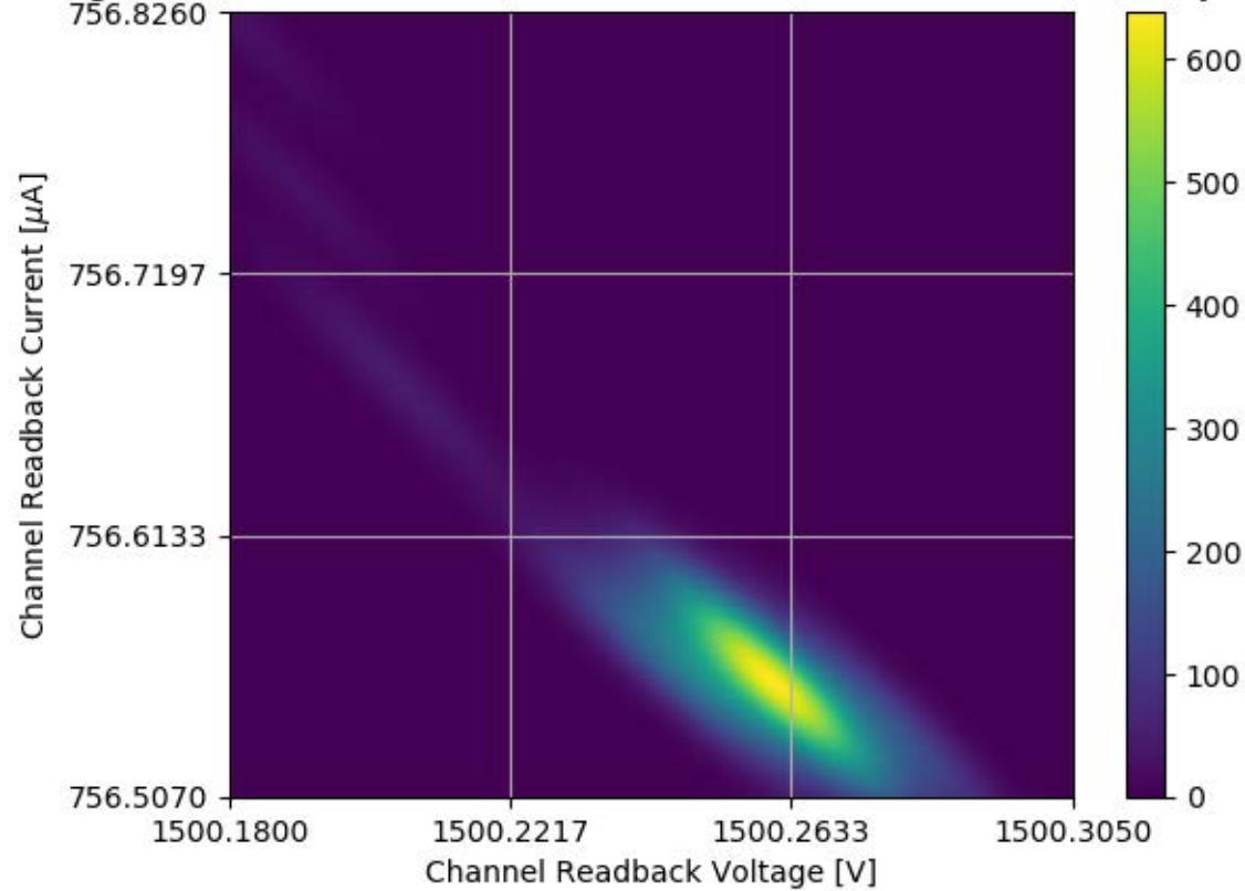
Voltage and Current Readback for Module #359 Channel 34 Stability Test
