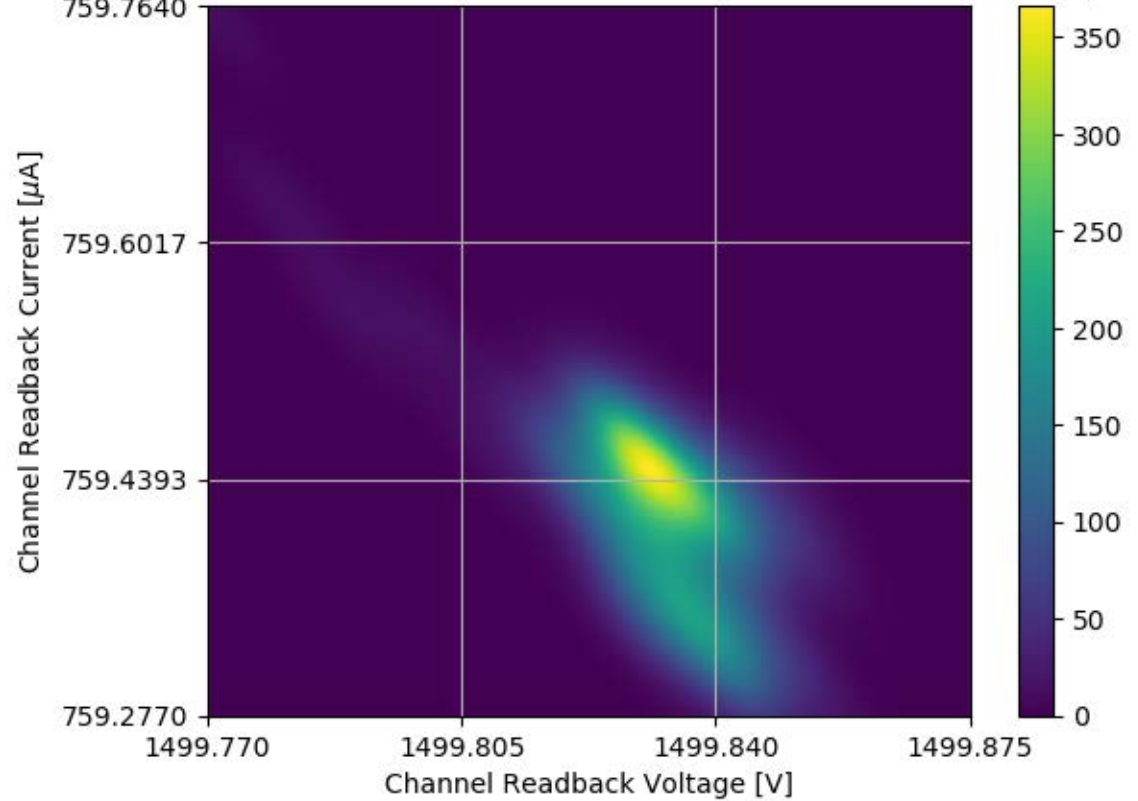
Voltage and Current Readback for Module #359 Channel 22 Stability Test
