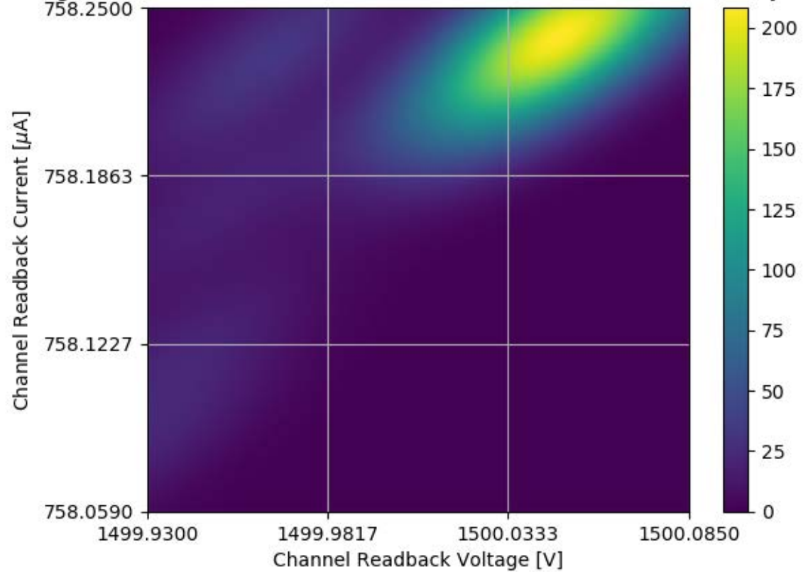
Voltage and Current Readback for Module #359 Channel 08 Stability Test
