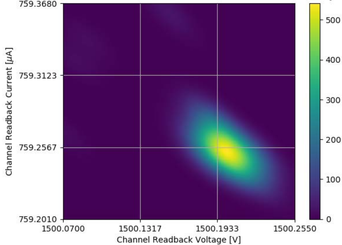
Voltage and Current Readback for Module #359 Channel 24 Stability Test
