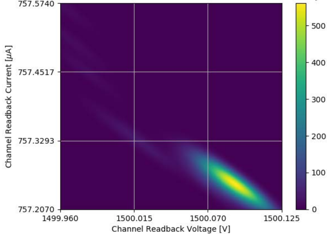
Voltage and Current Readback for Module #359 Channel 19 Stability Test
