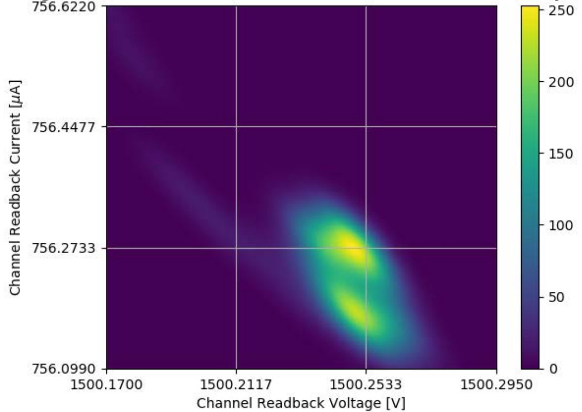
Voltage and Current Readback for Module #359 Channel 17 Stability Test
