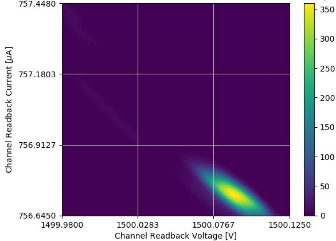
Voltage and Current Readback for Module #359 Channel 18 Stability Test
