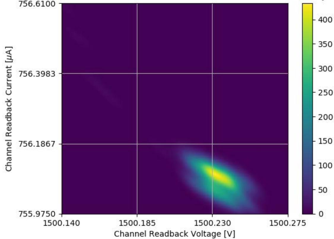
Voltage and Current Readback for Module #359 Channel 28 Stability Test
