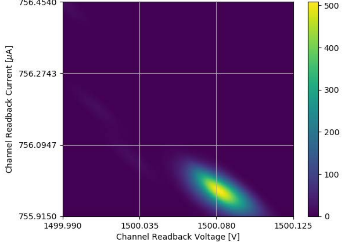
Voltage and Current Readback for Module #359 Channel 03 Stability Test
