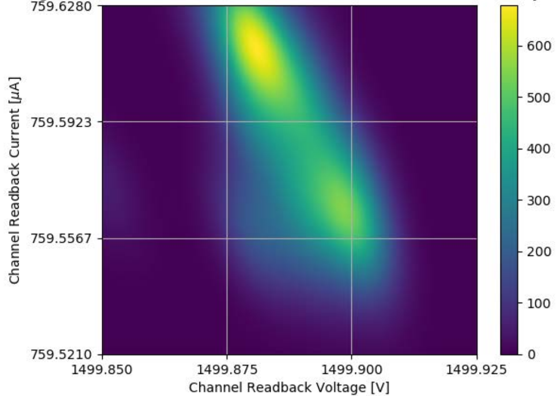
Voltage and Current Readback for Module #359 Channel 25 Stability Test
