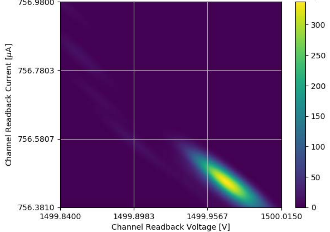
Voltage and Current Readback for Module #359 Channel 07 Stability Test
