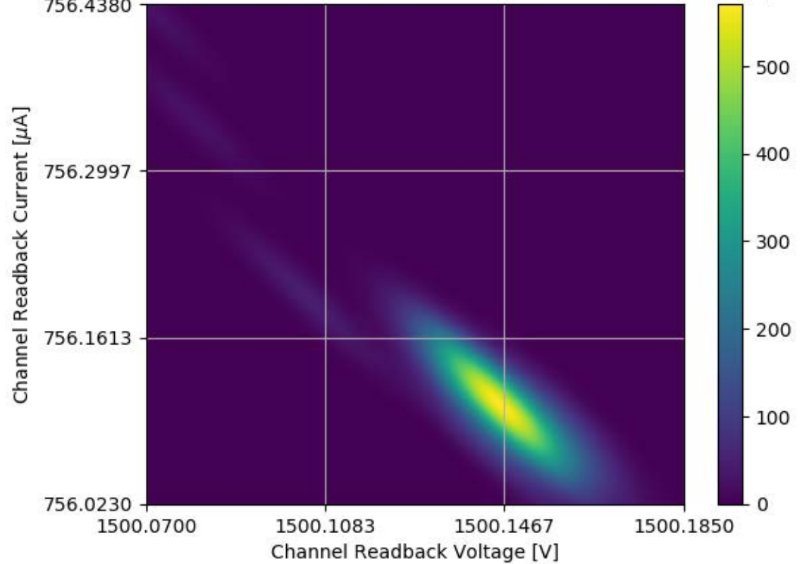
Voltage and Current Readback for Module #359 Channel 30 Stability Test
