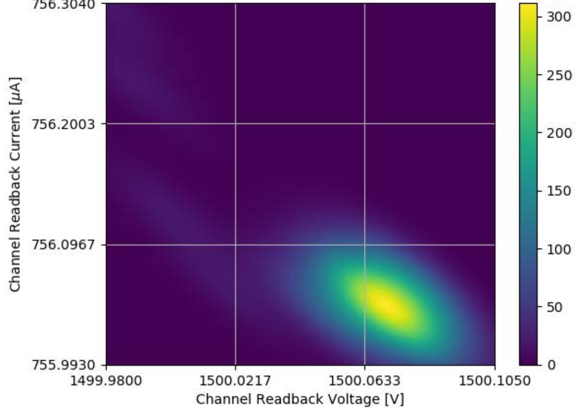
Voltage and Current Readback for Module #359 Channel 02 Stability Test
