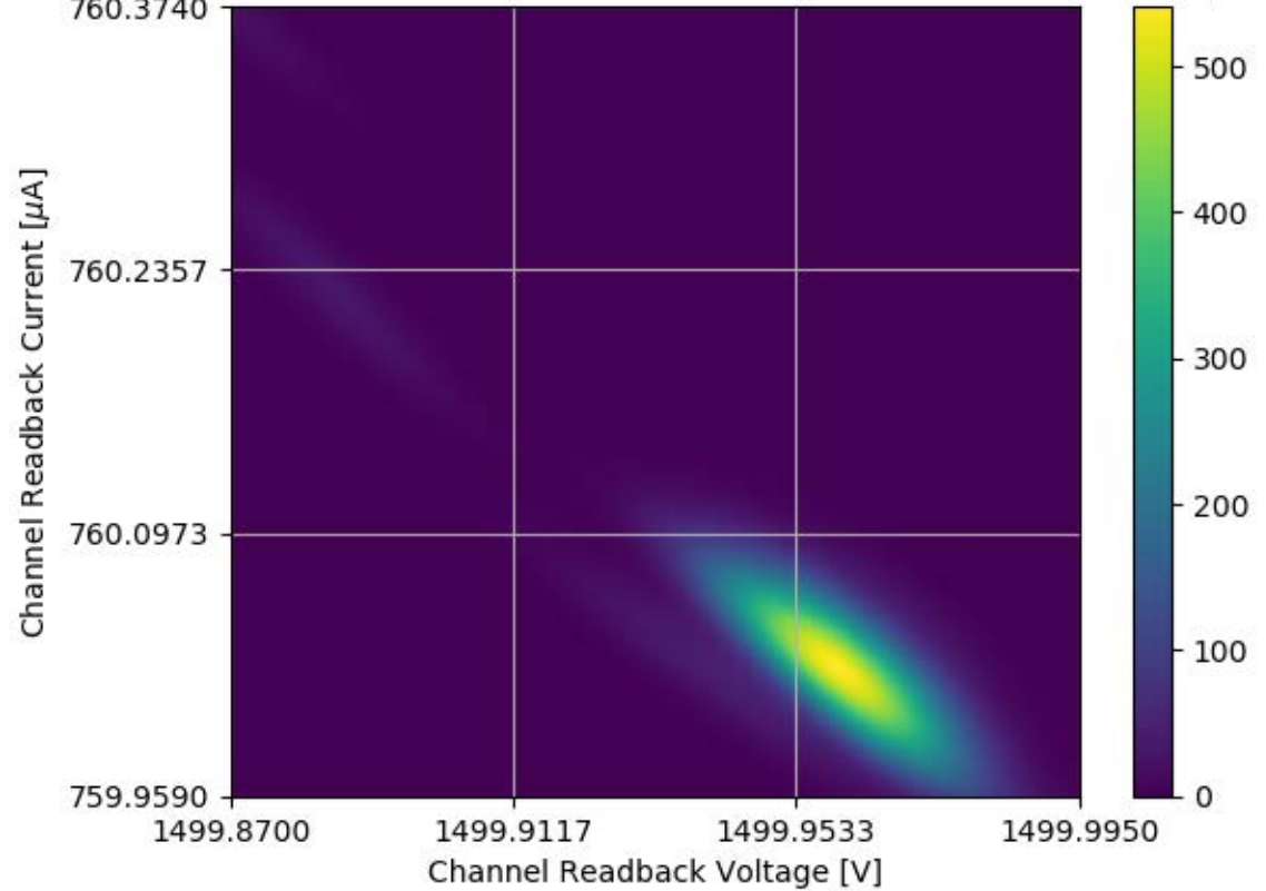
Voltage and Current Readback for Module #359 Channel 12 Stability Test
