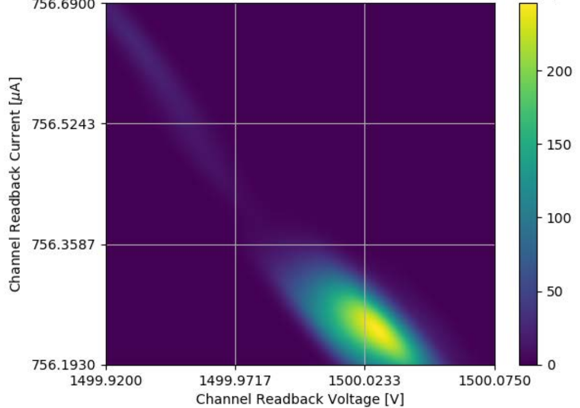
Voltage and Current Readback for Module #359 Channel 31 Stability Test
