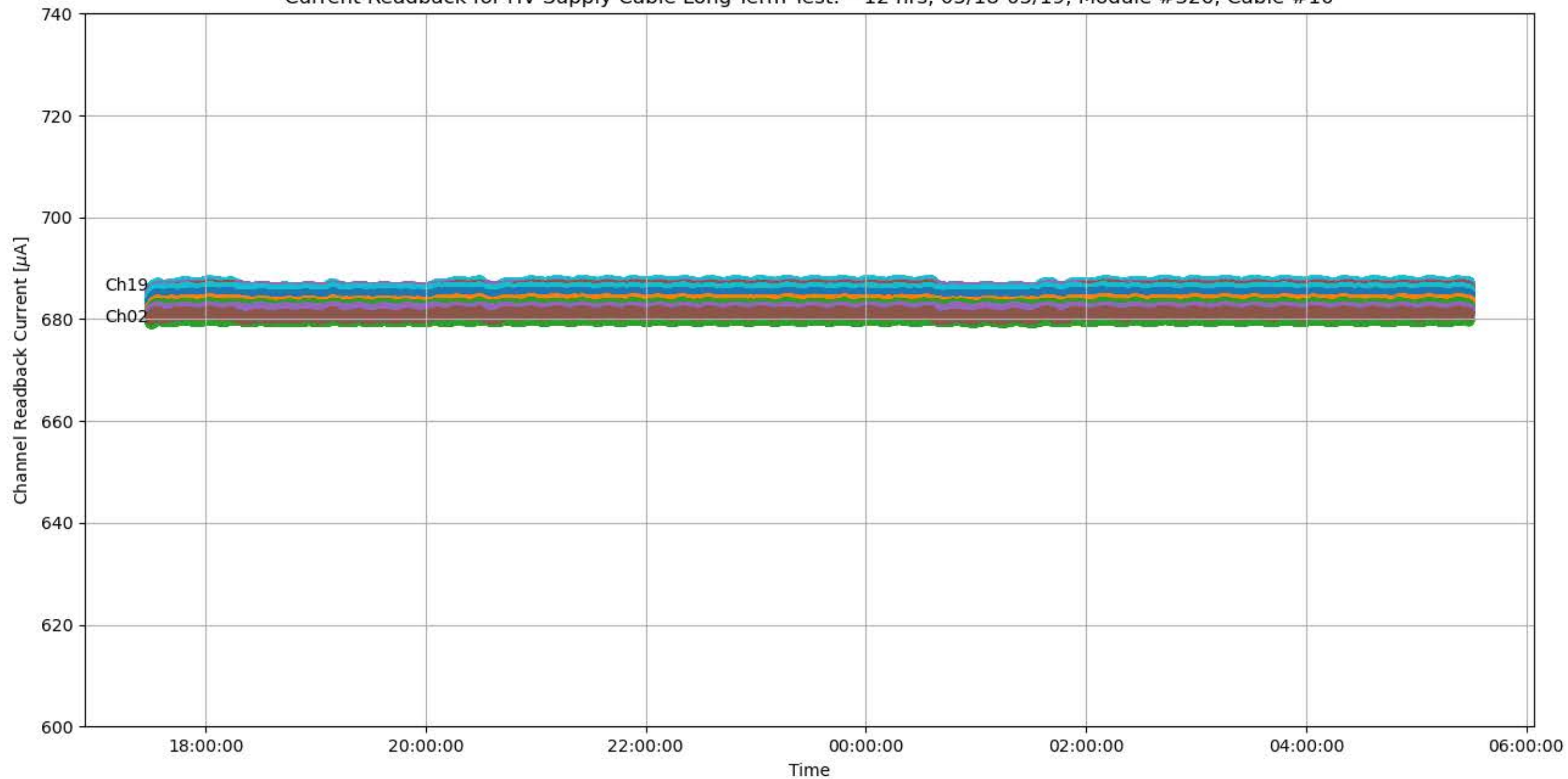
Current Readback for HV Supply Cable Long-Term Test: ~12 hrs, 05/18-05/19, Module #326, Cable #10
