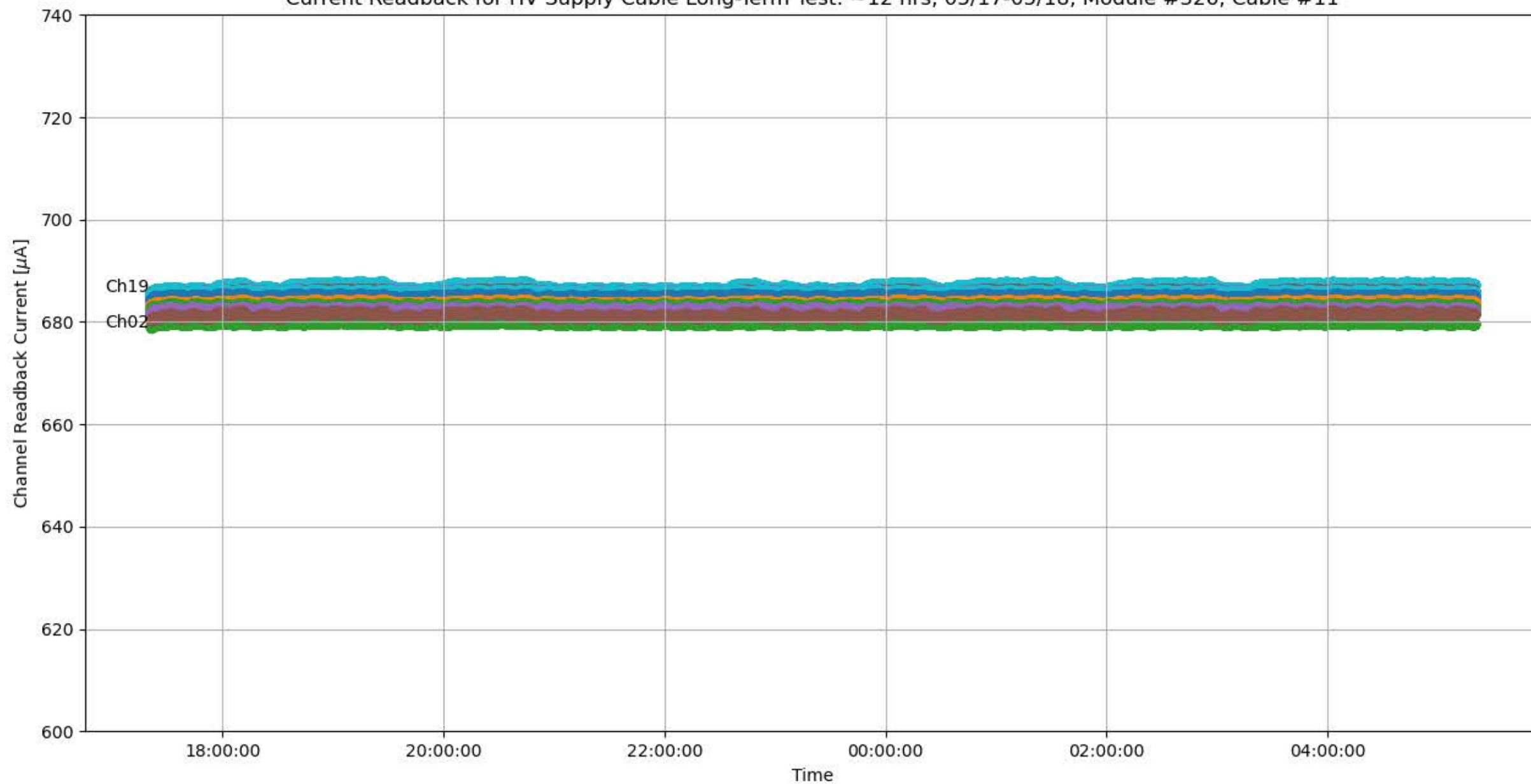
Current Readback for HV Supply Cable Long-Term Test: ~12 hrs, 05/17-05/18, Module #326, Cable #11
