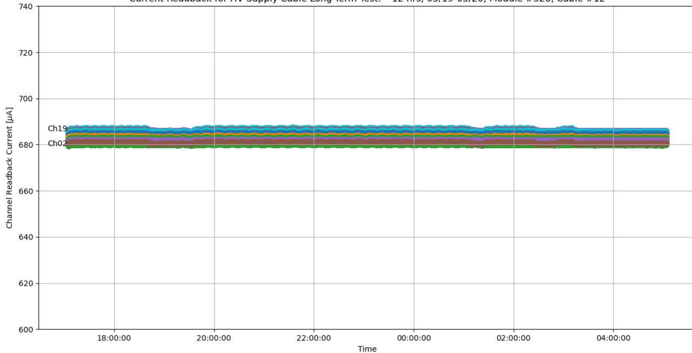
Current Readback for HV Supply Cable Long-Term Test: ~12 hrs, 05/19-05/20, Module #326, Cable #12
