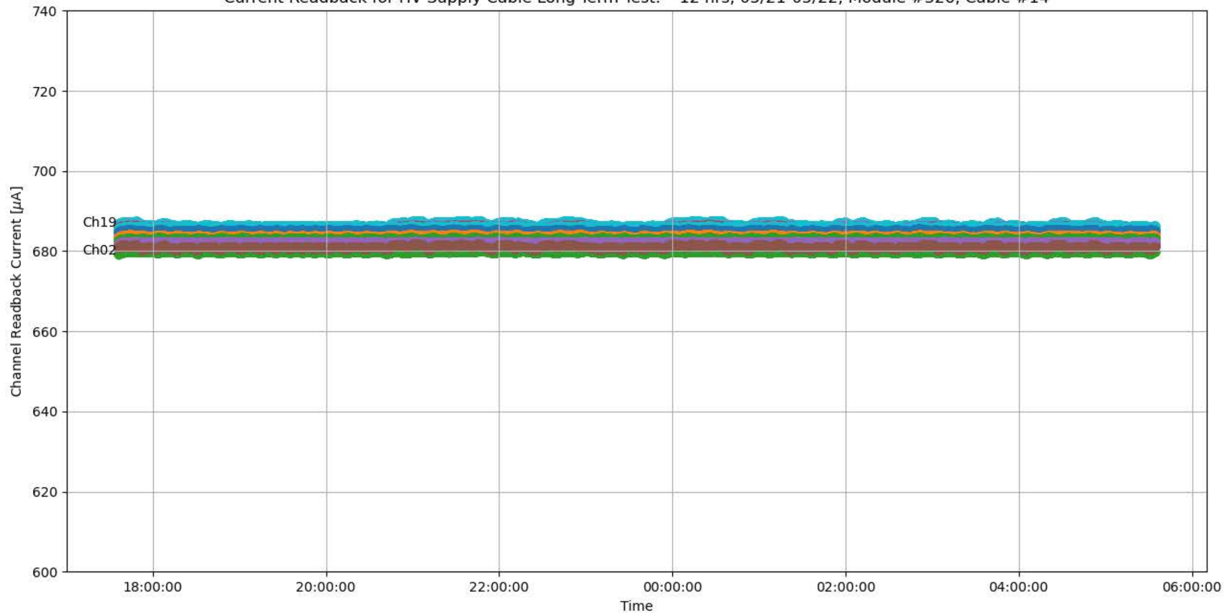
Current Readback for HV Supply Cable Long-Term Test: ~12 hrs, 05/21-05/22, Module #326, Cable #14
