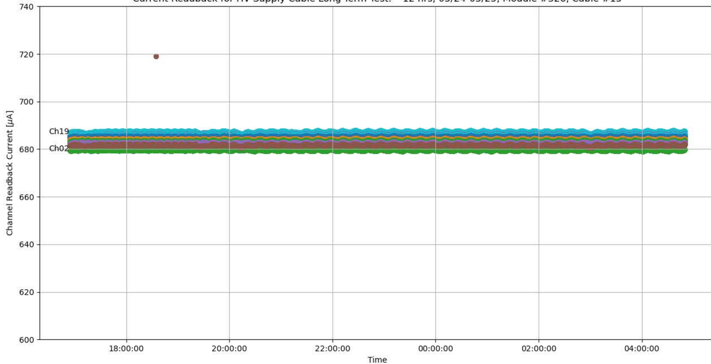
Current Readback for HV Supply Cable Long-Term Test: ~12 hrs, 05/24-05/25, Module #326, Cable #15
