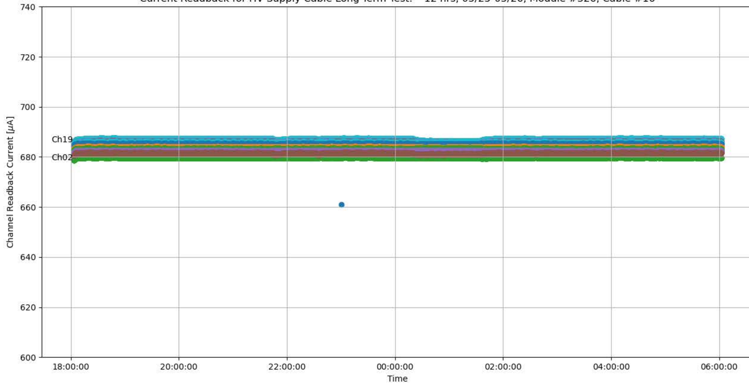
Current Readback for HV Supply Cable Long-Term Test: ~12 hrs, 05/25-05/26, Module #326, Cable #16
