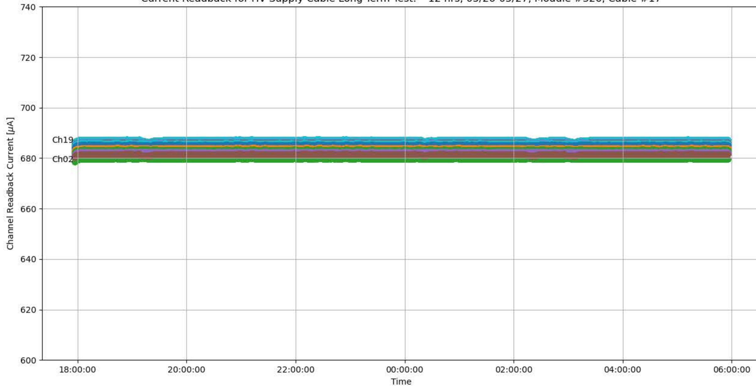
Current Readback for HV Supply Cable Long-Term Test: ~12 hrs, 05/26-05/27, Module #326, Cable #17
