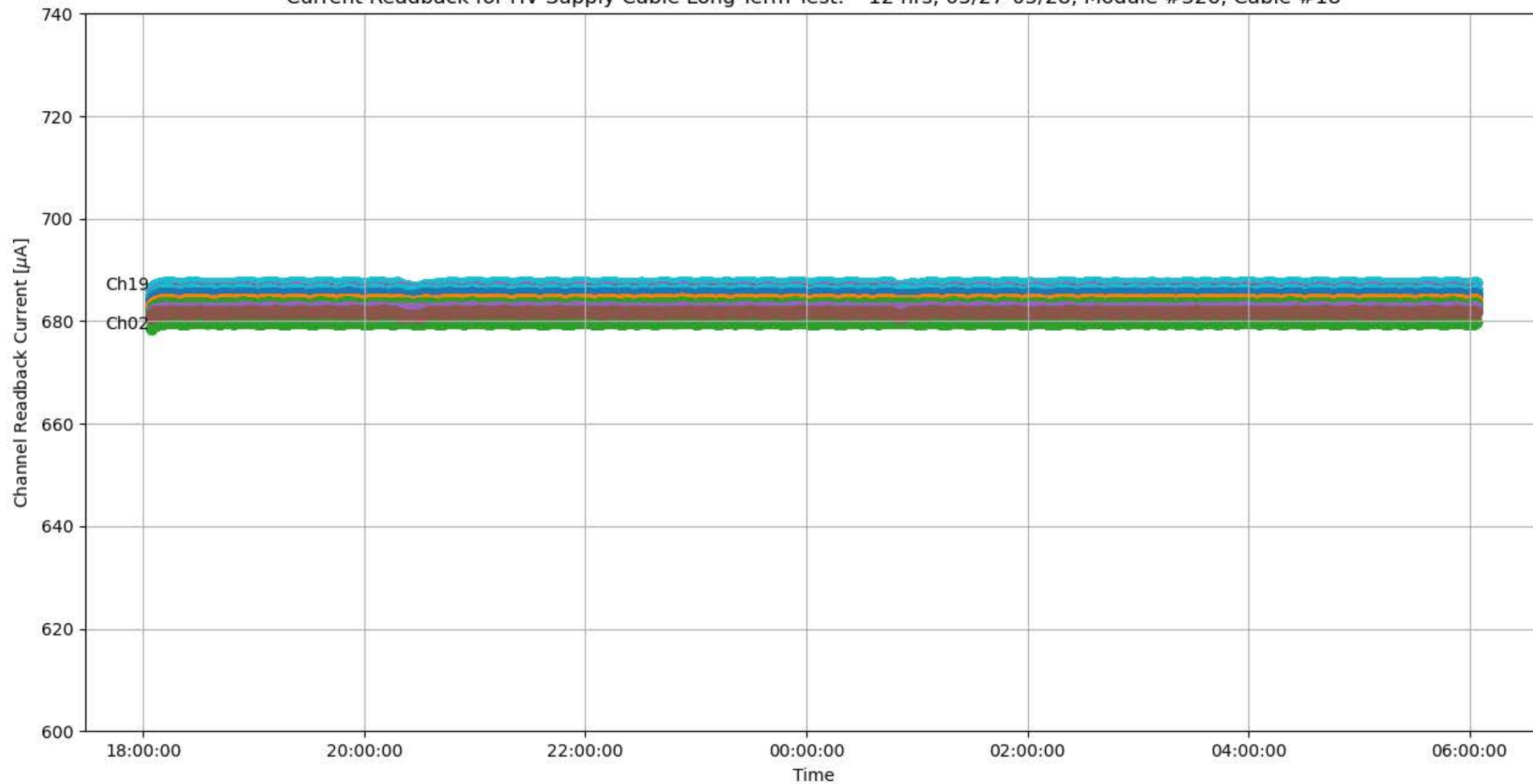
Current Readback for HV Supply Cable Long-Term Test: ~12 hrs, 05/27-05/28, Module #326, Cable #18
