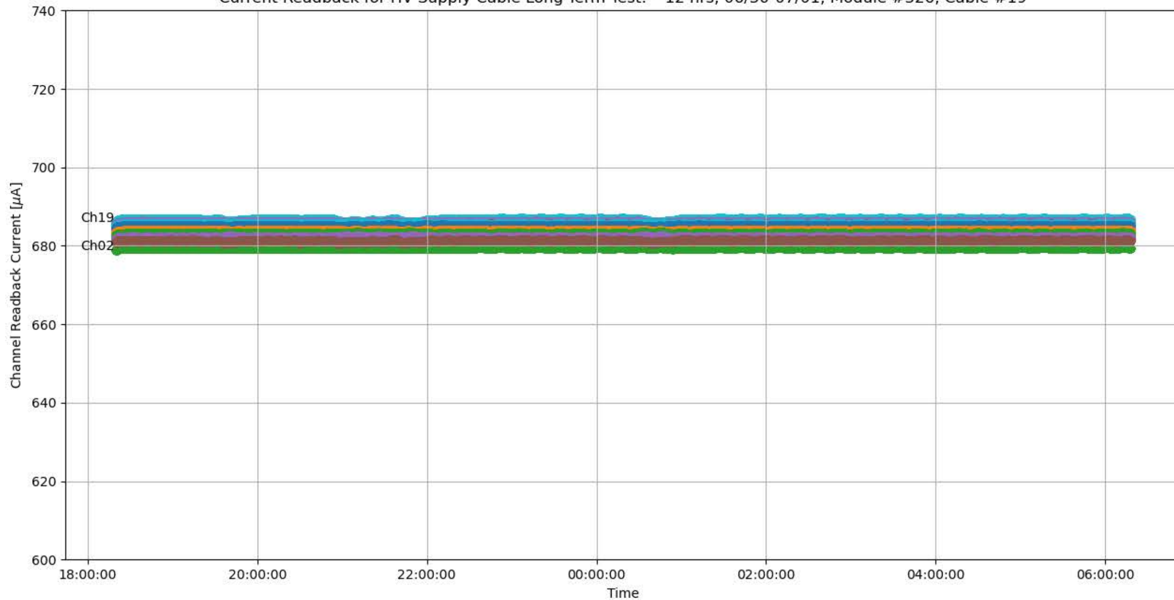
Current Readback for HV Supply Cable Long-Term Test: ~12 hrs, 06/30-07/01, Module #326, Cable #19
