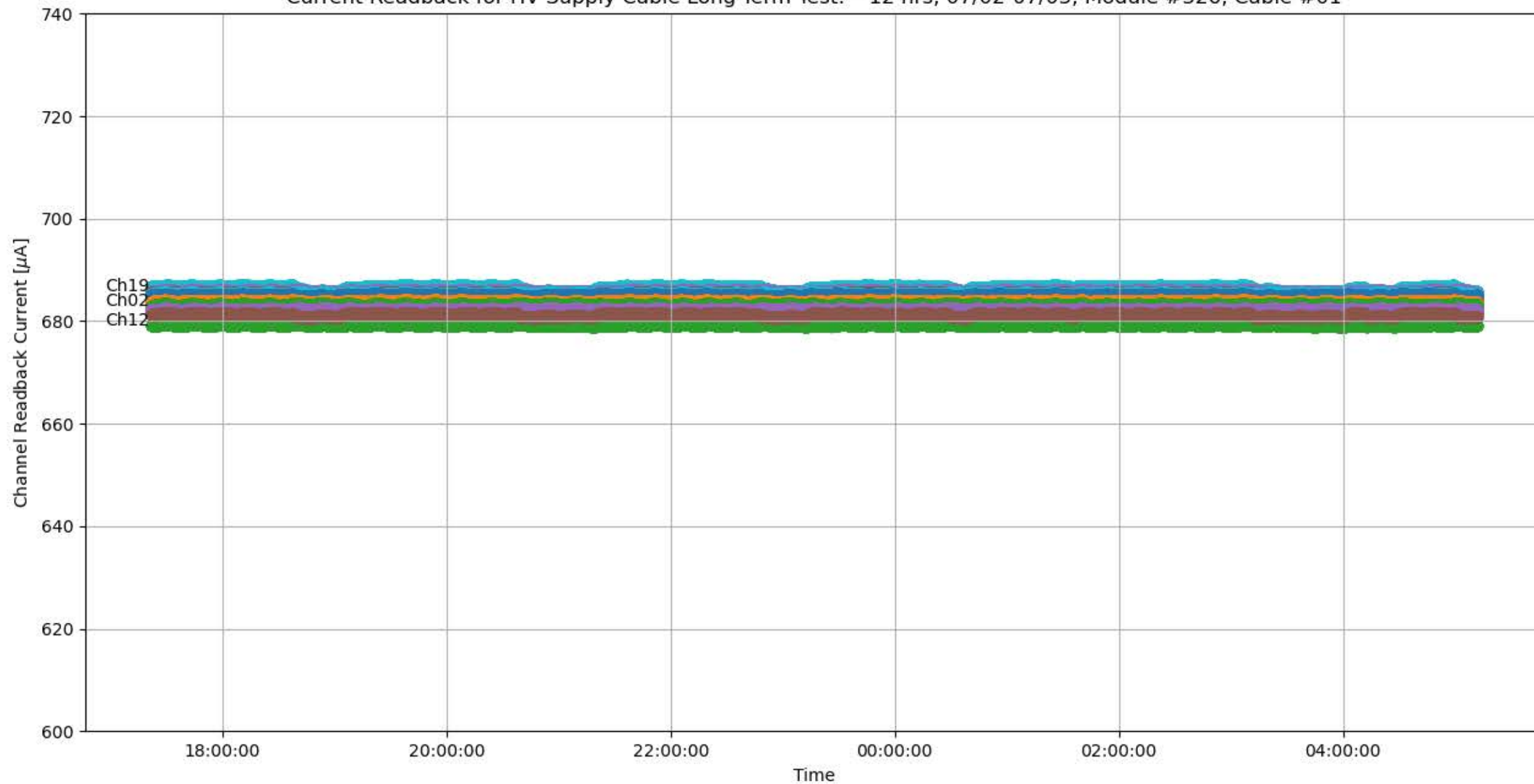
Current Readback for HV Supply Cable Long-Term Test: ~12 hrs, 07/02-07/03, Module #326, Cable #01
