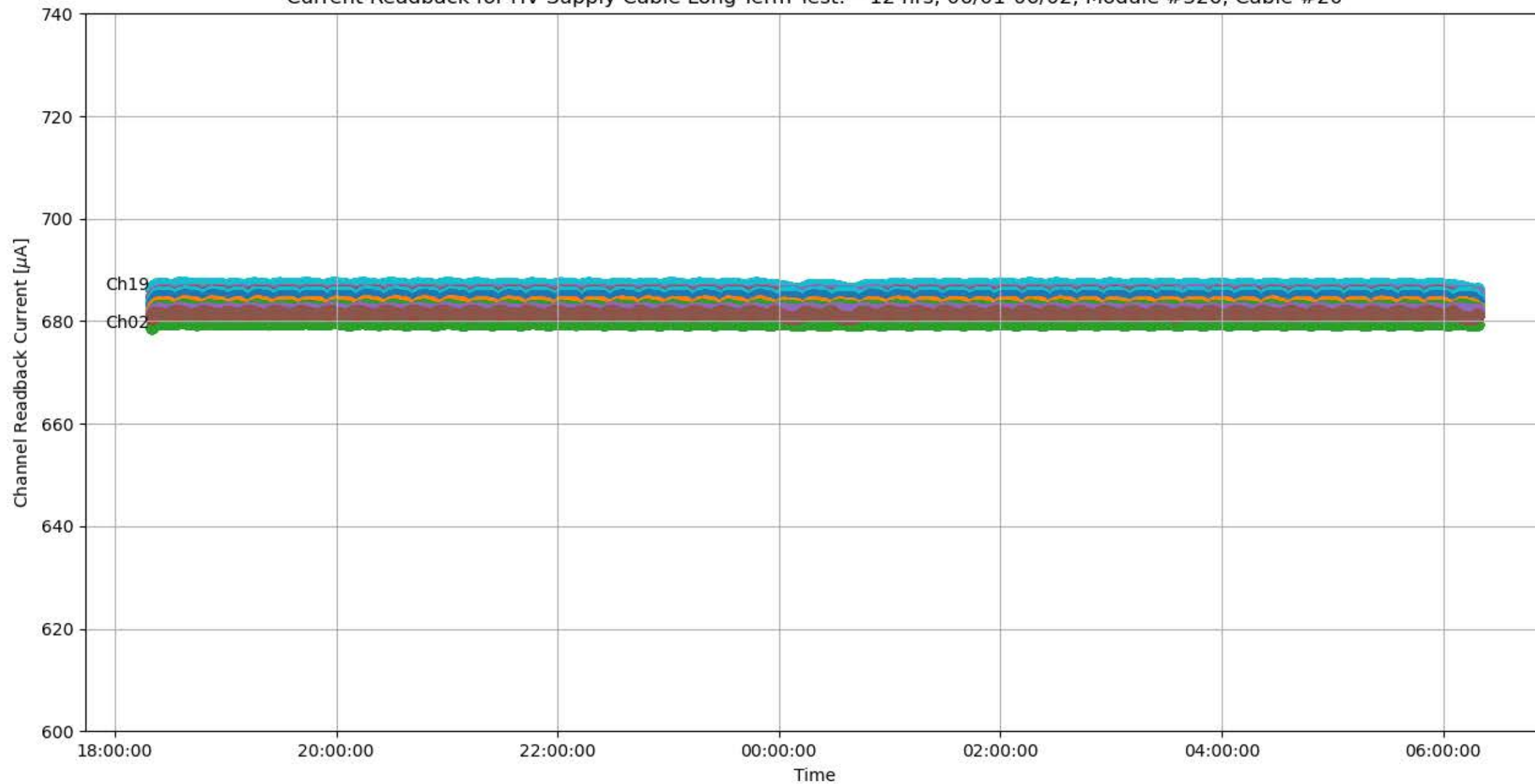
Current Readback for HV Supply Cable Long-Term Test: ~12 hrs, 06/01-06/02, Module #326, Cable #20
