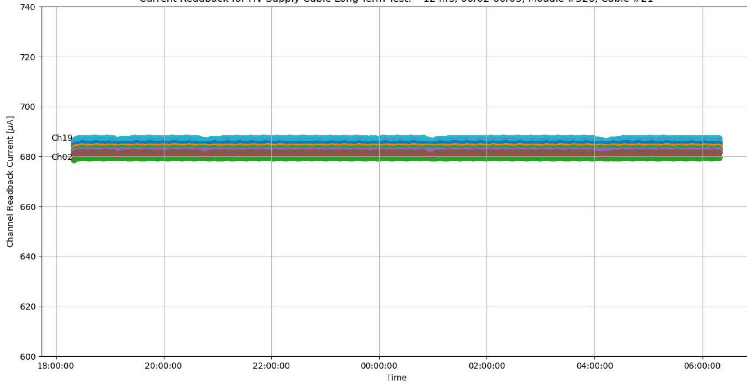
Current Readback for HV Supply Cable Long-Term Test: ~12 hrs, 06/02-06/03, Module #326, Cable #21
