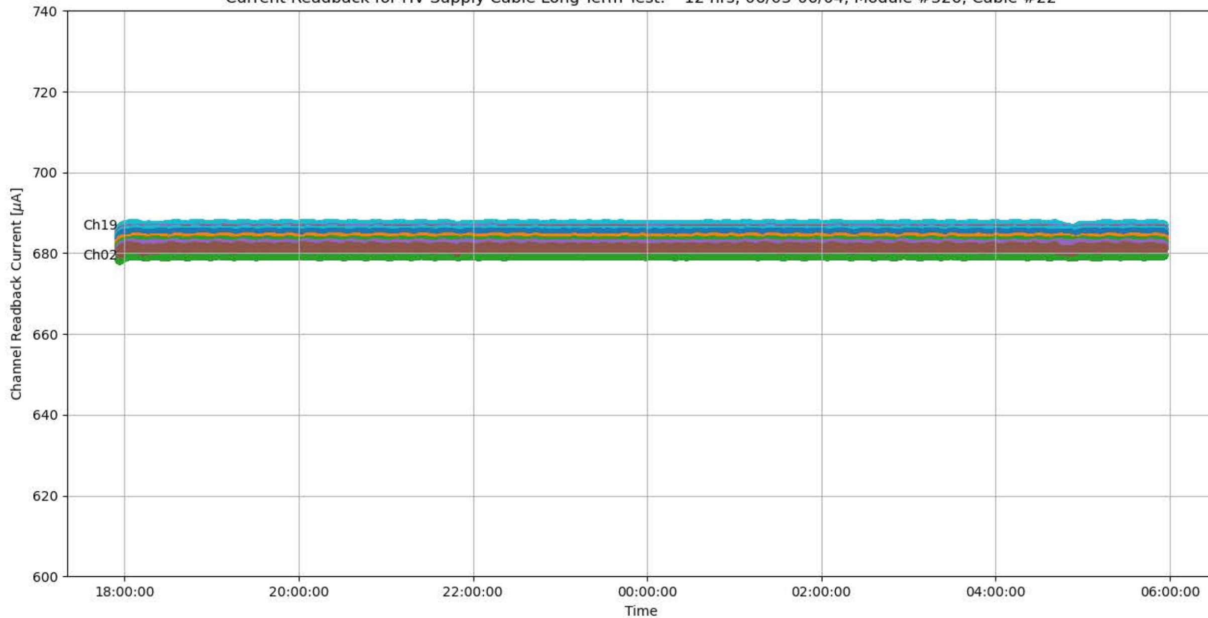
Current Readback for HV Supply Cable Long-Term Test: ~12 hrs, 06/03-06/04, Module #326, Cable #22
