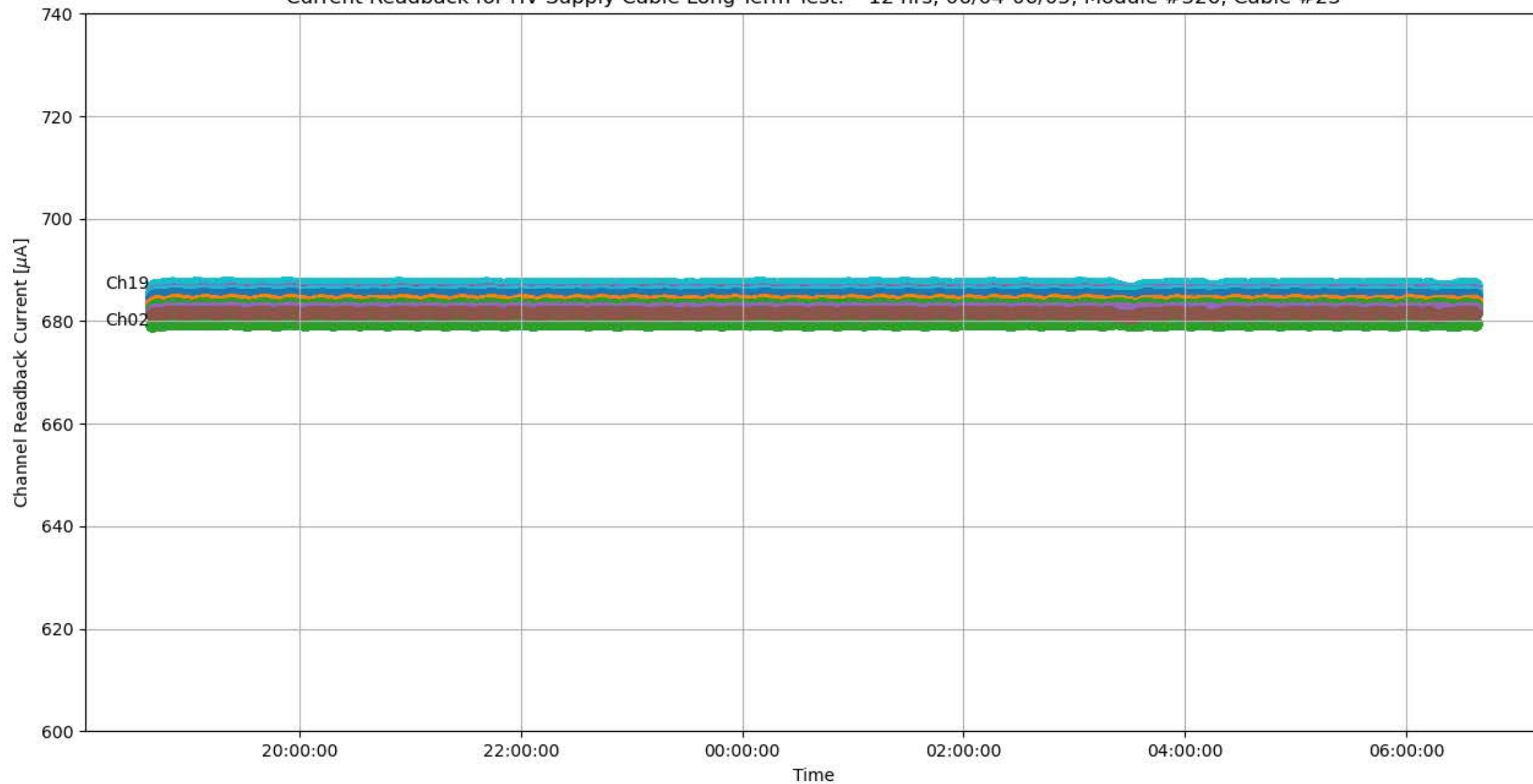
Current Readback for HV Supply Cable Long-Term Test: ~12 hrs, 06/04-06/05, Module #326, Cable #23
