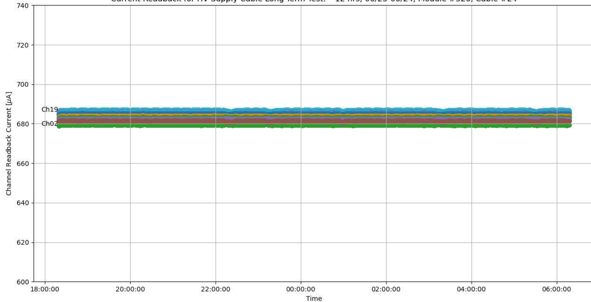
Current Readback for HV Supply Cable Long-Term Test: ~12 hrs, 06/23-06/24, Module #326, Cable #24
