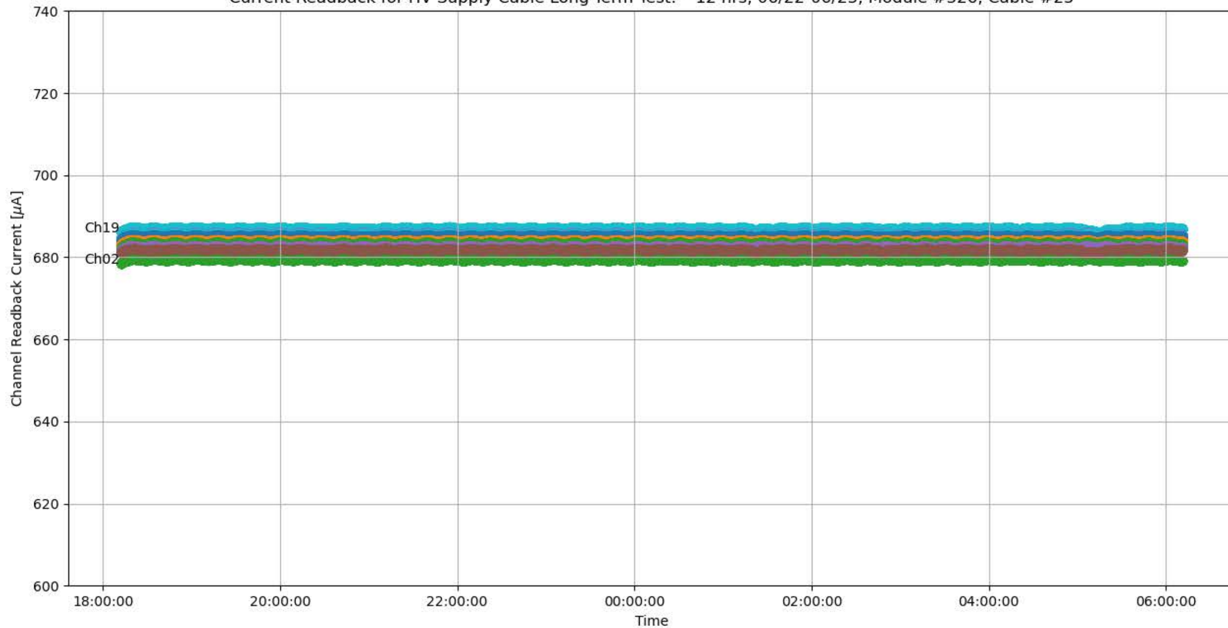
Current Readback for HV Supply Cable Long-Term Test: ~12 hrs, 06/22-06/23, Module #326, Cable #25
