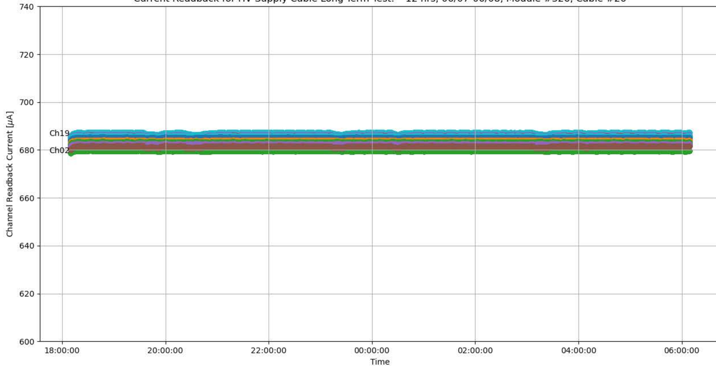
Current Readback for HV Supply Cable Long-Term Test: ~12 hrs, 06/07-06/08, Module #326, Cable #26
