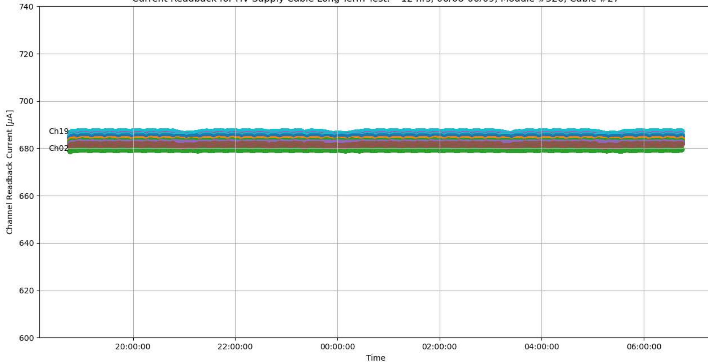
Current Readback for HV Supply Cable Long-Term Test: ~12 hrs, 06/08-06/09, Module #326, Cable #27
