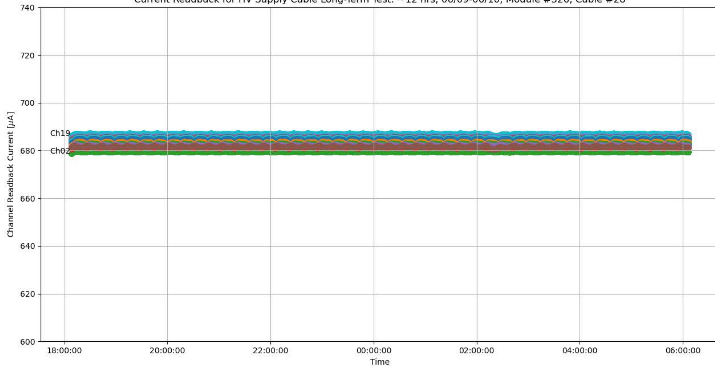
Current Readback for HV Supply Cable Long-Term Test: ~12 hrs, 06/09-06/10, Module #326, Cable #28
