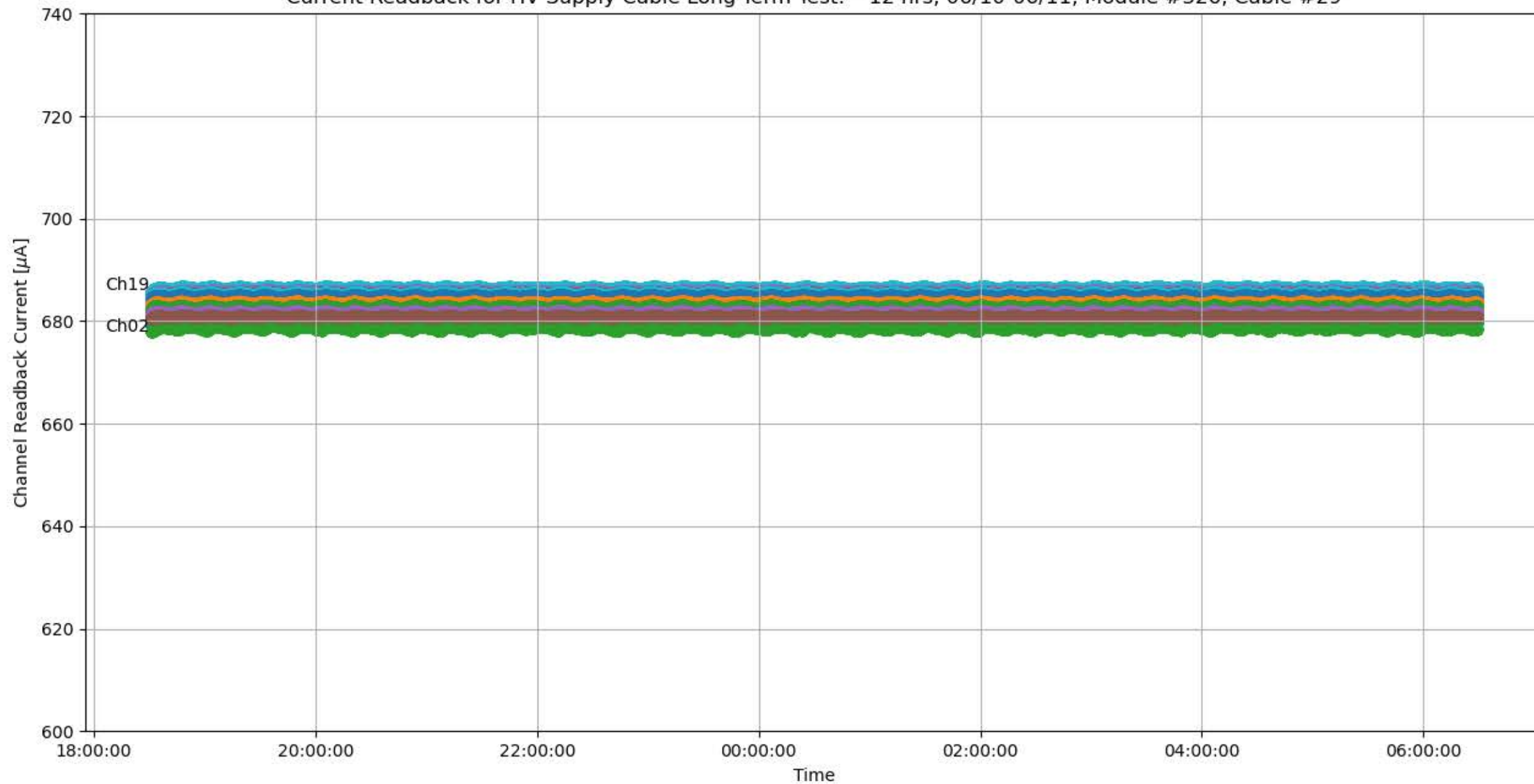
Current Readback for HV Supply Cable Long-Term Test: ~12 hrs, 06/10-06/11, Module #326, Cable #29
