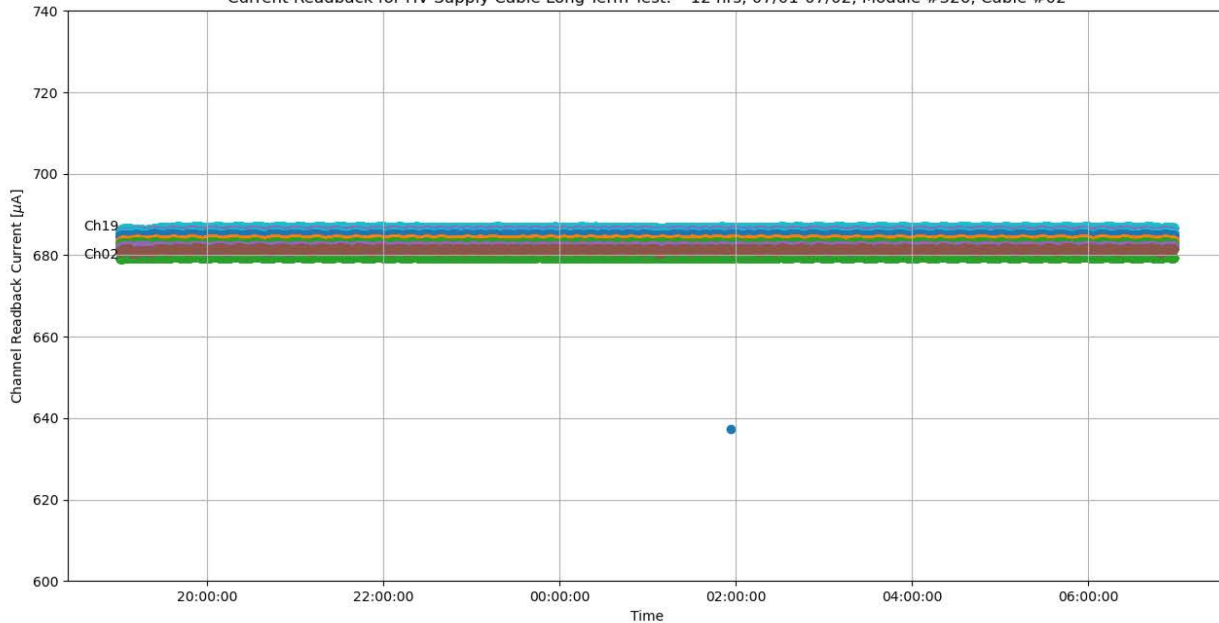
Current Readback for HV Supply Cable Long-Term Test: ~12 hrs, 07/01-07/02, Module #326, Cable #02
