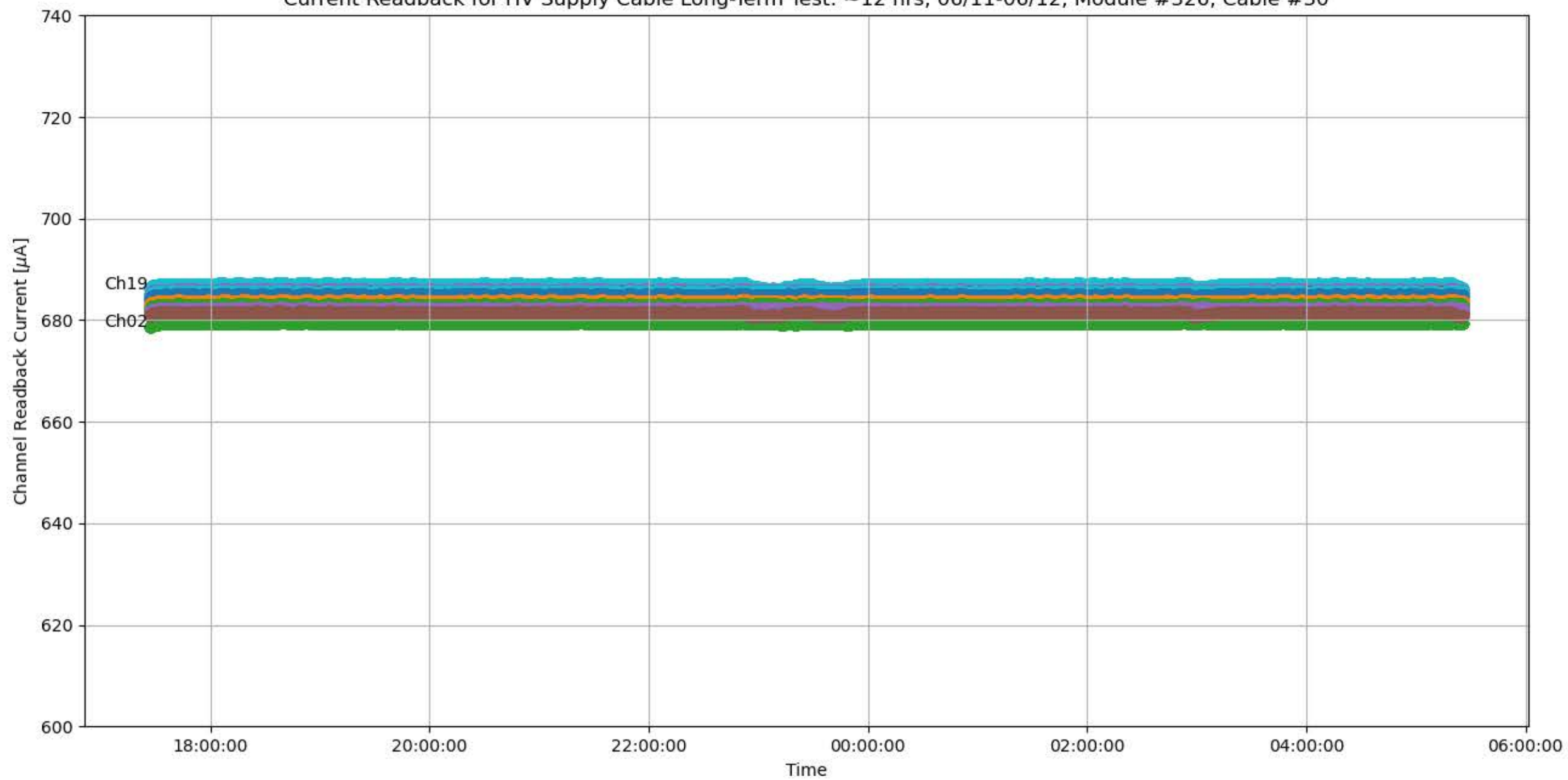
Current Readback for HV Supply Cable Long-Term Test: ~12 hrs, 06/11-06/12, Module #326, Cable #30
