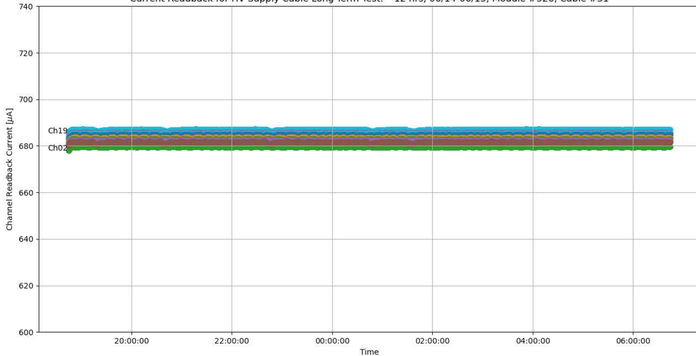
Current Readback for HV Supply Cable Long-Term Test: ~12 hrs, 06/14-06/15, Module #326, Cable #31
