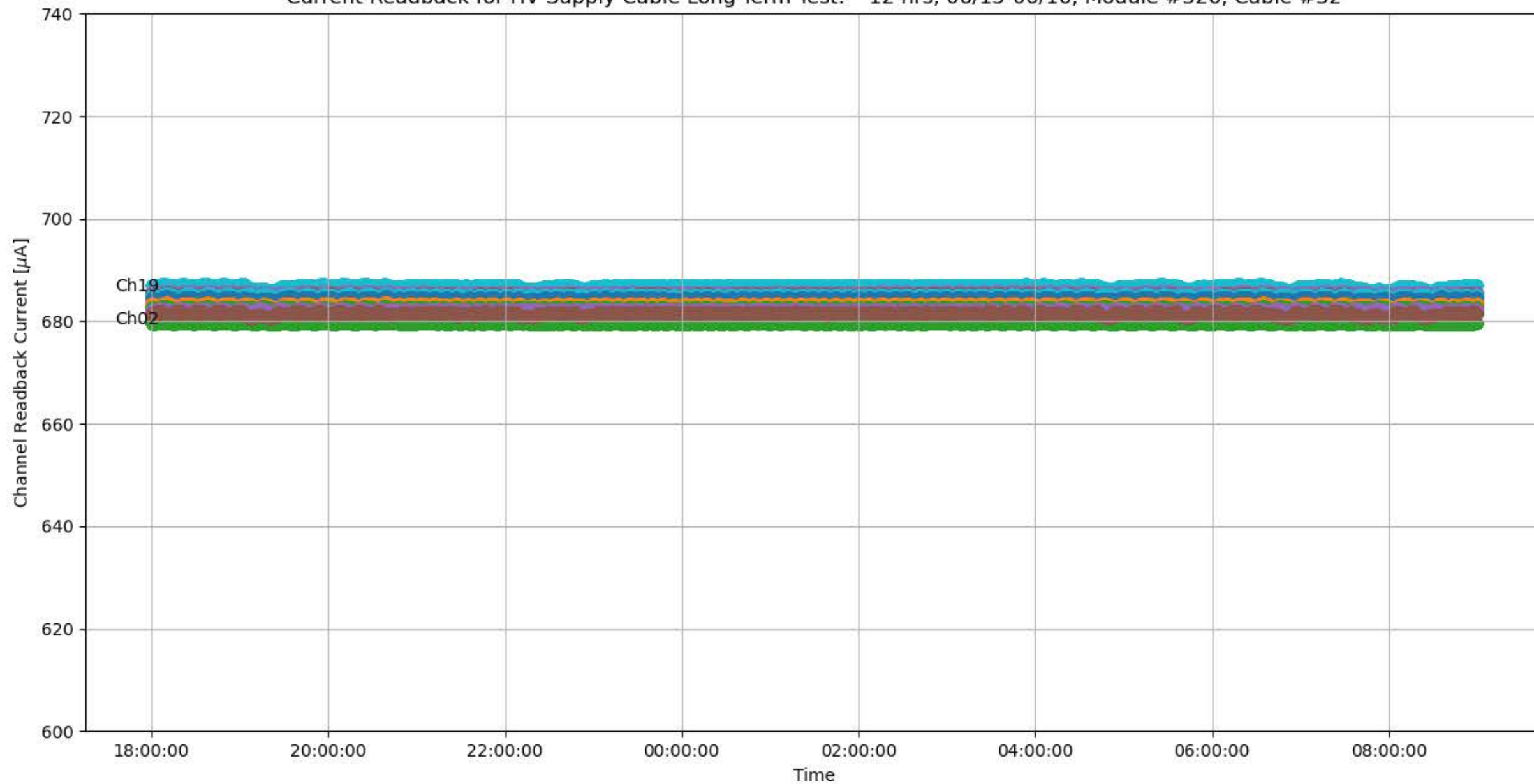
Current Readback for HV Supply Cable Long-Term Test: ~12 hrs, 06/15-06/16, Module #326, Cable #32
