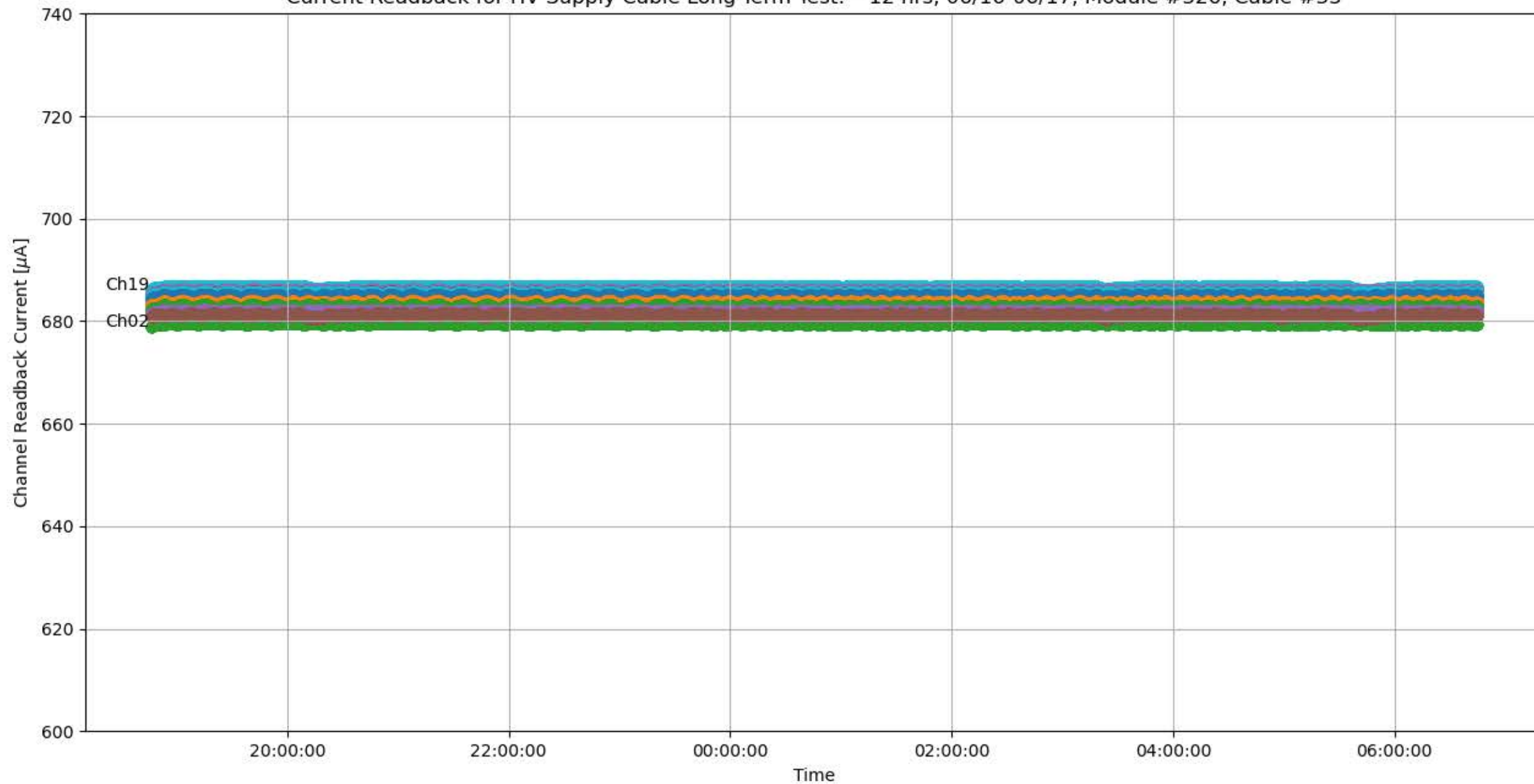
Current Readback for HV Supply Cable Long-Term Test: ~12 hrs, 06/16-06/17, Module #326, Cable #33
