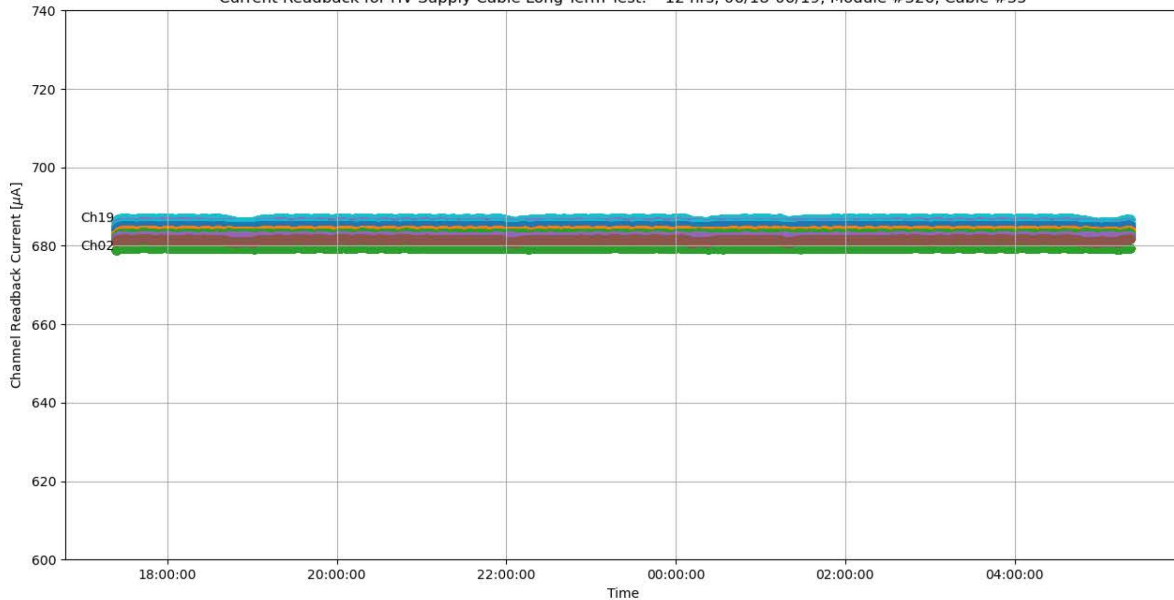
Current Readback for HV Supply Cable Long-Term Test: ~12 hrs, 06/18-06/19, Module #326, Cable #35
