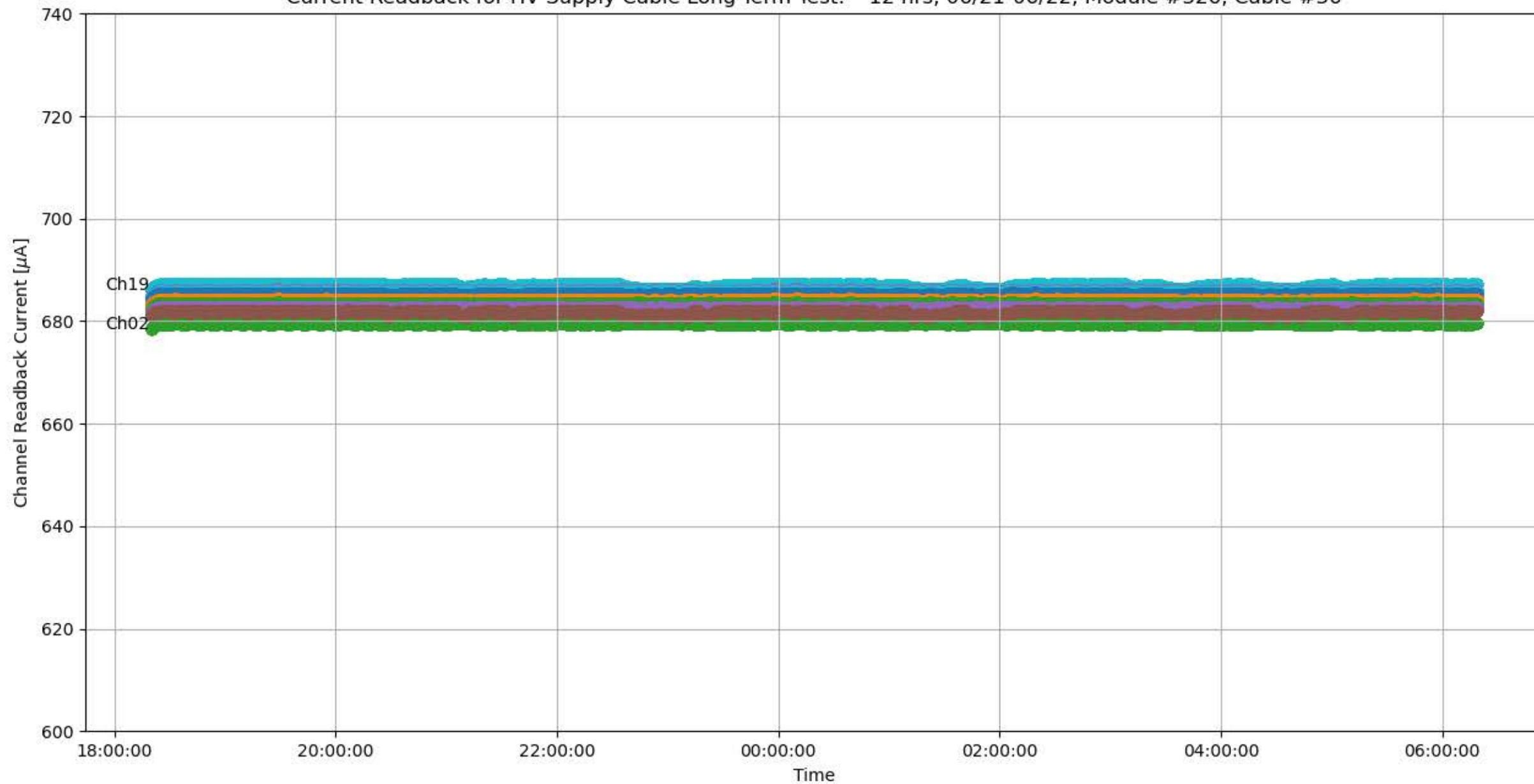
Current Readback for HV Supply Cable Long-Term Test: ~12 hrs, 06/21-06/22, Module #326, Cable #36
