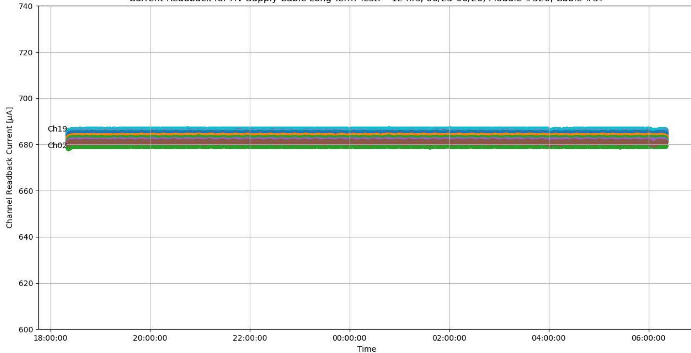
Current Readback for HV Supply Cable Long-Term Test: ~12 hrs, 06/25-06/26, Module #326, Cable #37
